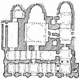
PLAN OF KACHRIEH DJAMI
