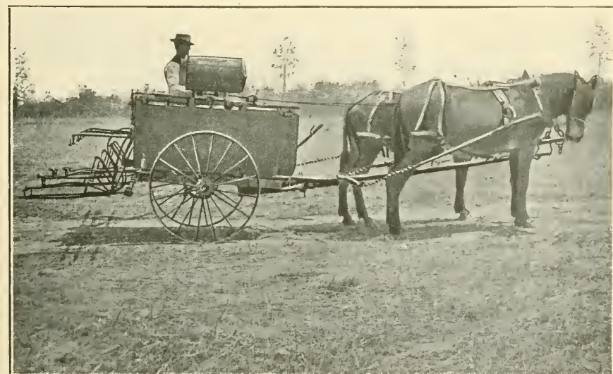
FIG. 217.—Field sprayer, with modifications, adapted for potato spraying, by L. C. Corbett, operating at the Virginia Truck Experiment Station, Norfolk, Va.
