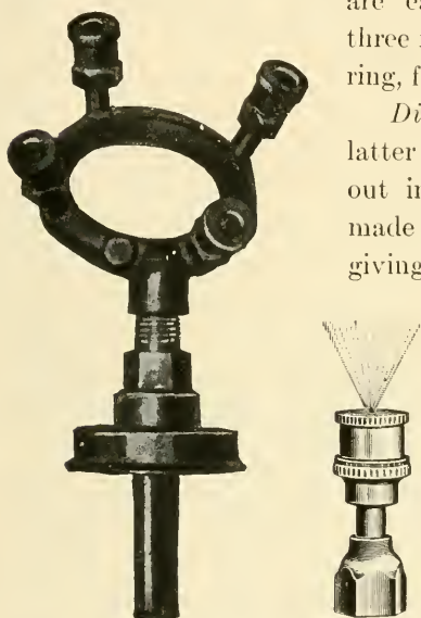
FIG. 44.—A cluster of spramotor nozzles and single nozzle of the same type.
