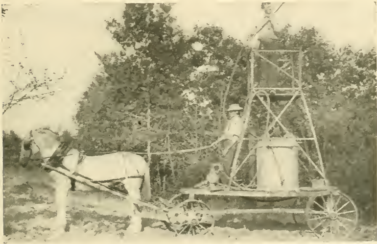
FIG. 42.—Carbonic-acid gas sprayer at work.
