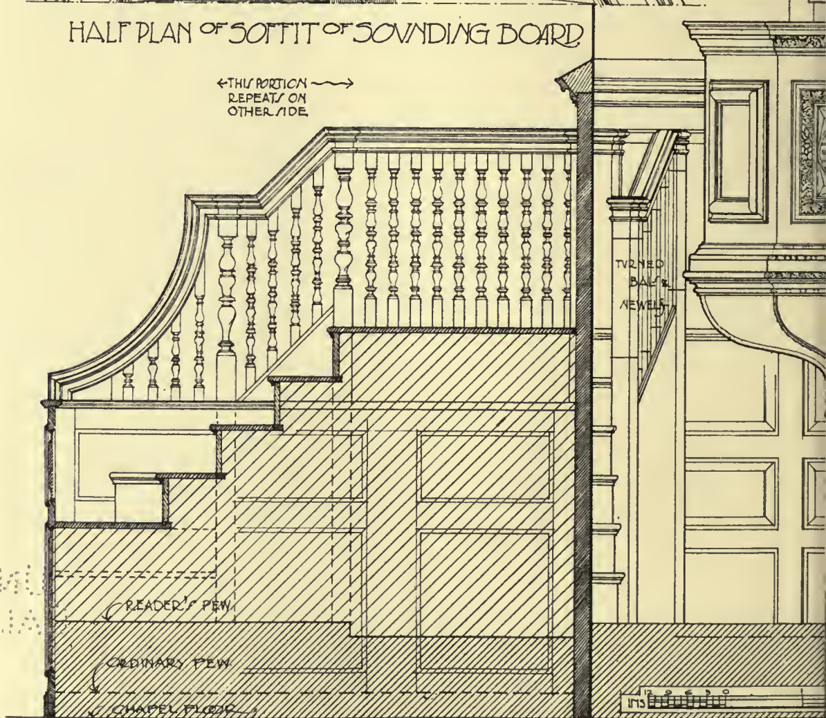
SECTION THRO' STAIRS SHEWING HANDRAIL
