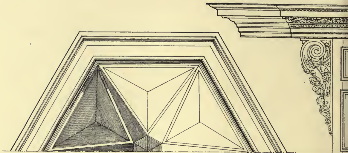
HALF PLAN OF SOFFIT OF SOUNDING BOARD
