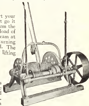
Louden Single Drum Power Hoist
