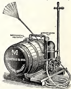
Myers Double-Acting Spray Outfit
