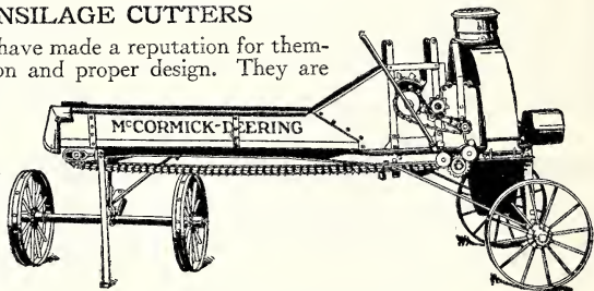
McCormick-Deering Ensilage Cutter
