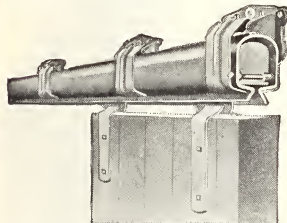
Bird-Proof Barn-Door Hanger
