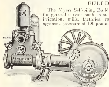
Bulldozer Pump
