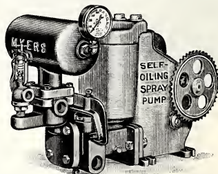
No. 16 Myers Special Chain-Driven Power Spray Pump
