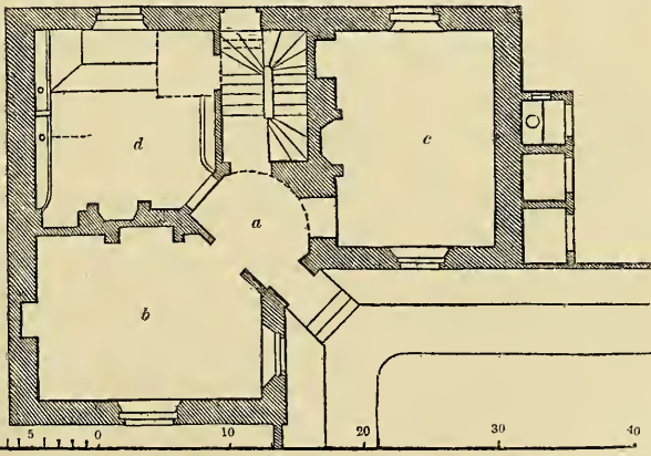
The principal floor contains: — a , Entrance lobby; b , kitchen; c , parlour; and d , office and library. There are cellars below, three bedrooms ( e ) above, and the usual offices outside.
