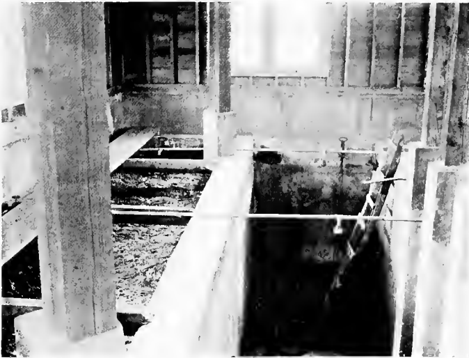
Fig. 43.—Two settling tanks—one empty and one filled.
