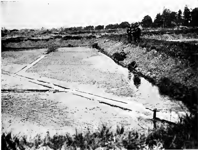
Fig. 47.—Sand filter of a sewage disposal plant.
