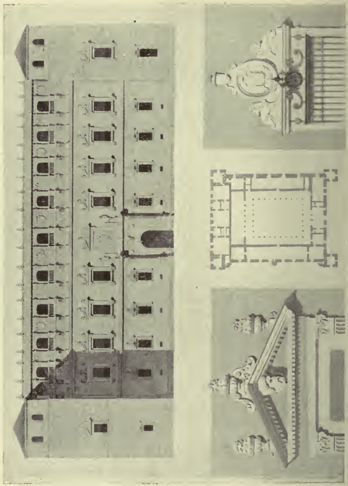
THE ALCAZAR. PLAN AND DETAILS. NORTH FAÇADE
