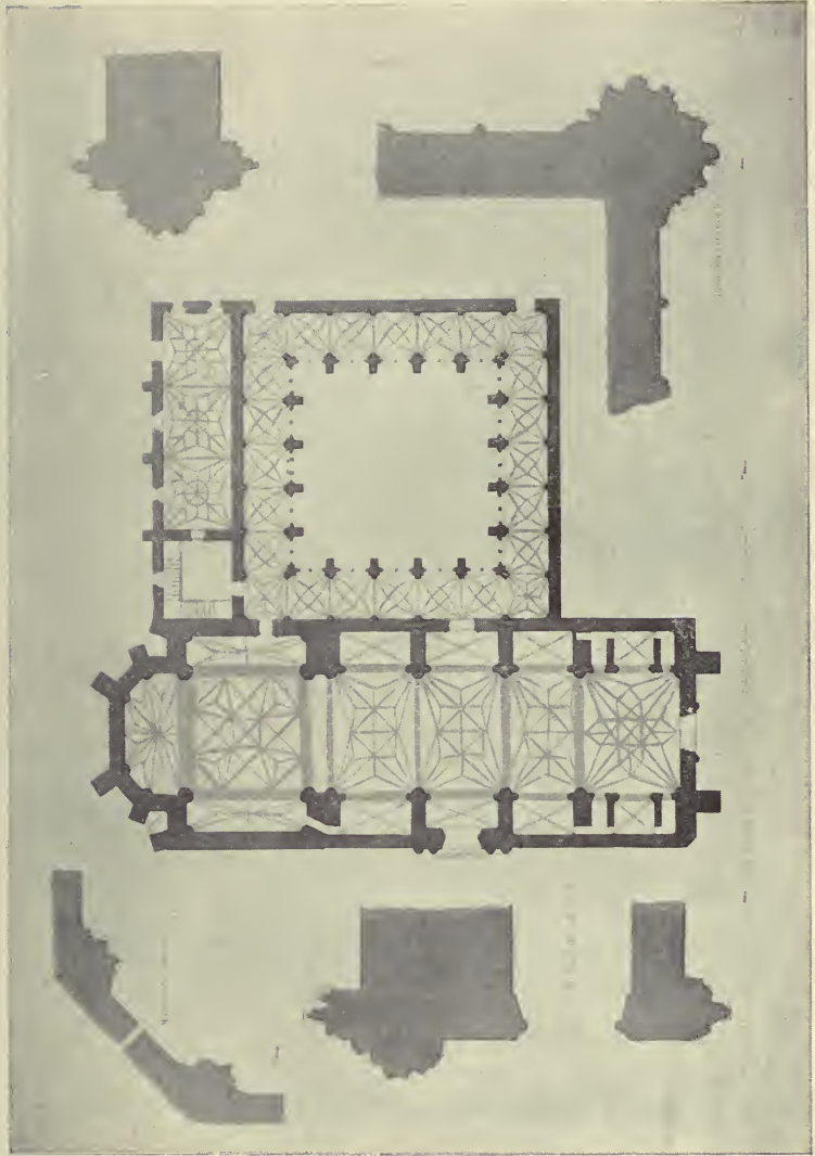
PLAN OF THE CHURCH AND PROCESSIONAL CLOISTER OF SAN JUAN DE LOS REYES
