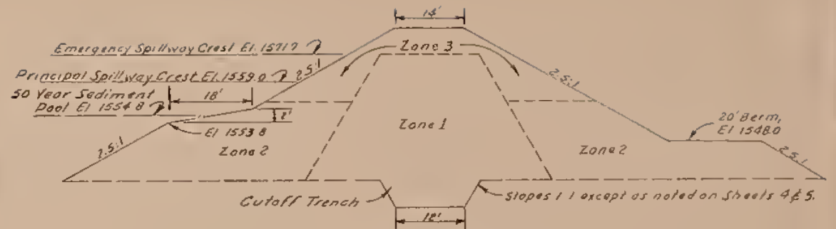
TYPICAL SECTION
