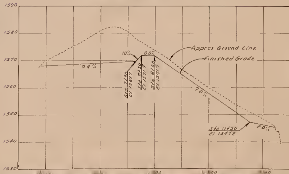
PROFILE ON Q OF EMERGENCY SPILLWAY
