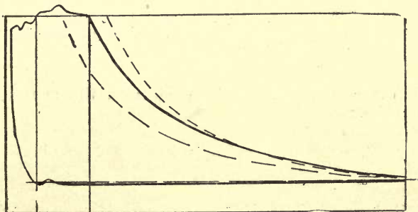
Cylinder, 8 in. bore; 12 in. stroke; revolutions, 140 per minute; I.H.P., 14.7, neglecting friction; air delivered, 93.5 per cent of cylinder capacity; clearance, 1.081 per cent; mechanical efficiency, neglecting friction, 80 per cent.
