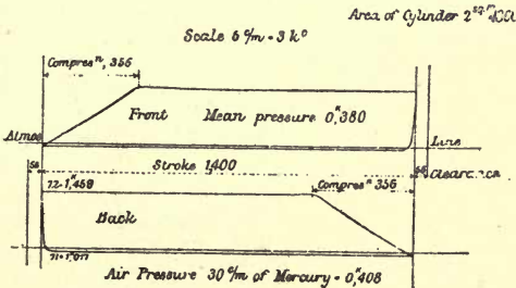
FIG. 46.—Diagrams from Air Cylinder.
