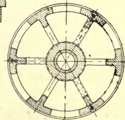
SECTION THRO' VALVE SEAT AT A.A.
