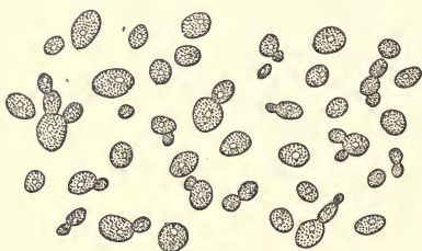
FIG. 4.—YEAST FROM BEER SEDIMENT SHOWING BUDDING (X 1270).
