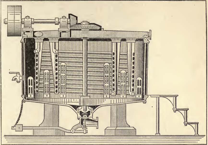
FIG. 2.—MASHING AND COOLING APPARATUS, CROSS SECTION.
