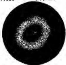
57 M Ring Neb in Lyra
