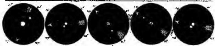
\gamma Andromeda \alpha Piscium \epsilon Equulei \gamma Delphini \zeta Aquarii
