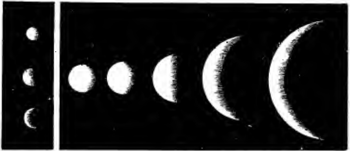
Mercury
