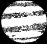
Jupiter.
