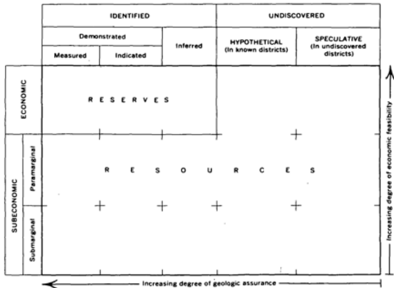
FIGURE 1.—Classification of mineral resources.
