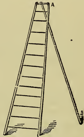
FIG. 151. Self-supporting ladder
