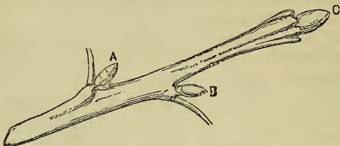
FIG. 19.—LATERAL BRANCH.
