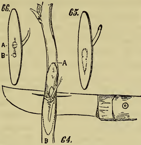
FIGS. 64 TO 70, BUDDING.
