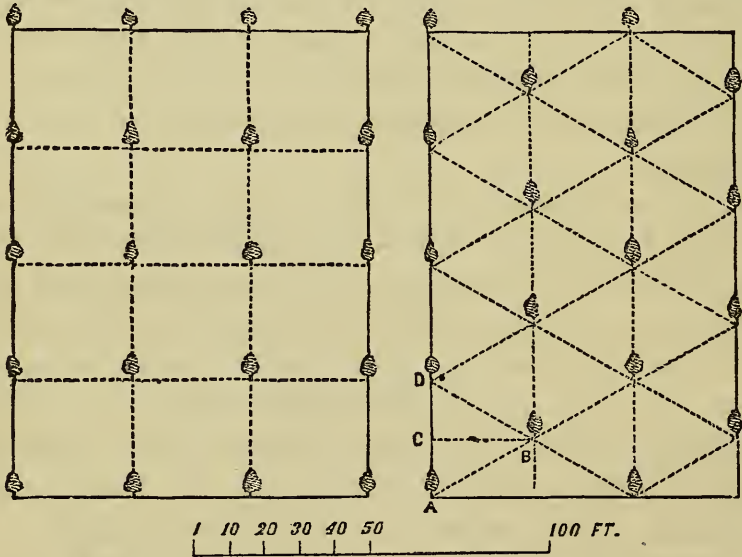
Fig. 93, square planting.
