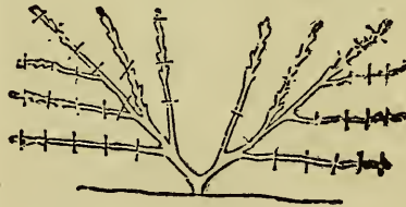
FIG. 120. Seventh year.
