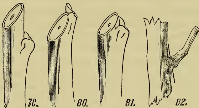
FIGS. 79 TO 82, PRUNING.
