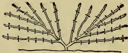
FIG. 121. Eighth year.
