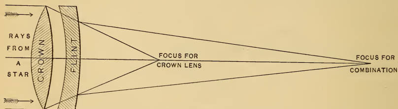
Illustrating Principle of Achromatic Object Glass
