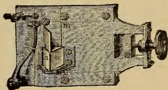
Slit and the Comparison Prism
