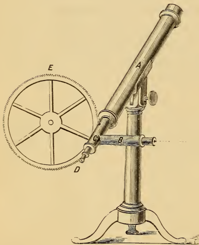
Finding Velocity of Light
