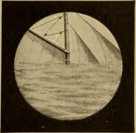
Ship's Rigging Distinct, Water Hazy
