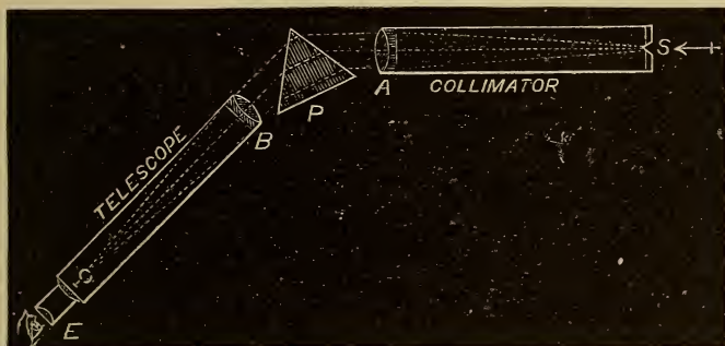
A Single-prism Spectroscope in Outline
