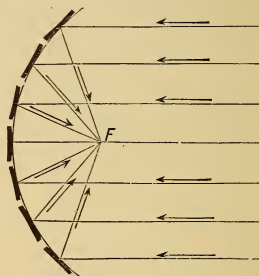
Concave Mirror reflects Parallel Rays to Focus
