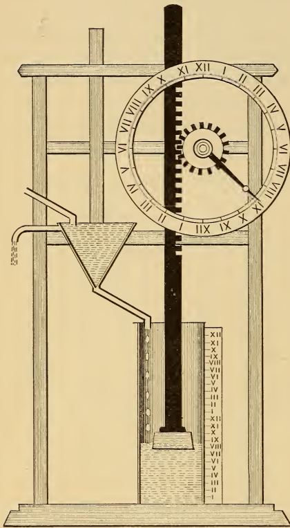
Antique Form of Clepsydra
