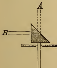
Course of Rays in Comparison Prism
