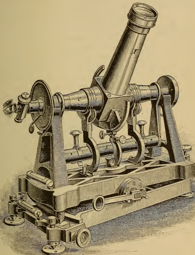
A Compact Modern Transit Instrument (from a Design by Heyde)
