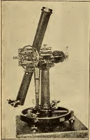
Zenith Telescope (Warner & Swasey)
