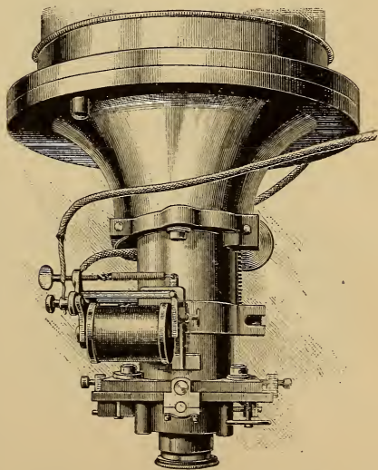
The Photo-chronograph (Fargis-Saegmüller)
