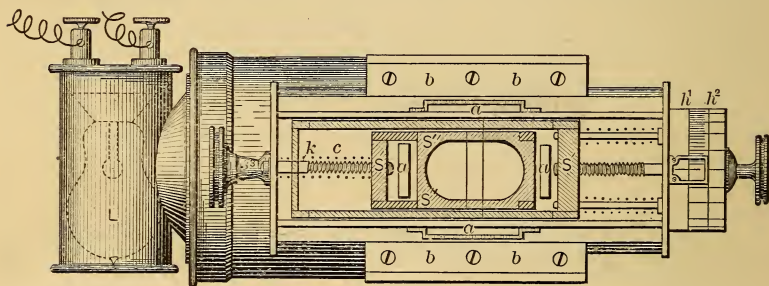
A Modern Micrometer with Electric Illumination (Ellery)
