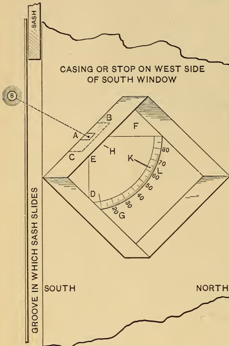
The Latitude-box in Position
