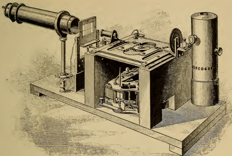
Machine for determining Personal Equation (Eastman)
