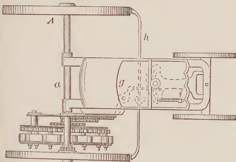
69701—G. W. Pressy—Stump Extractor.
