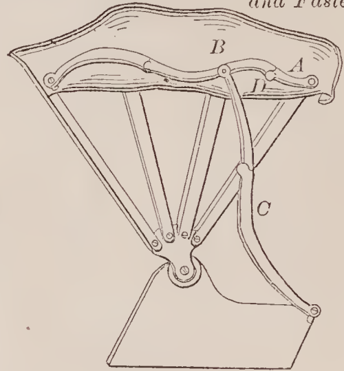
67418—H. M. Curtis—Buggy Top Joint and Fastening.
