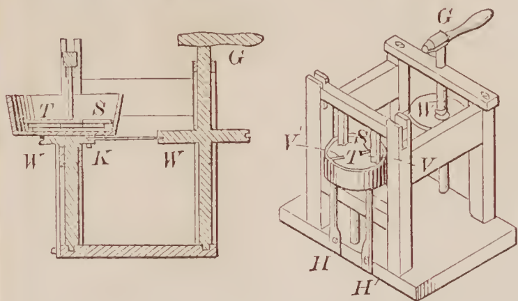
72177—C. Drexler—For Securing and Feeding Soft Crabs.
