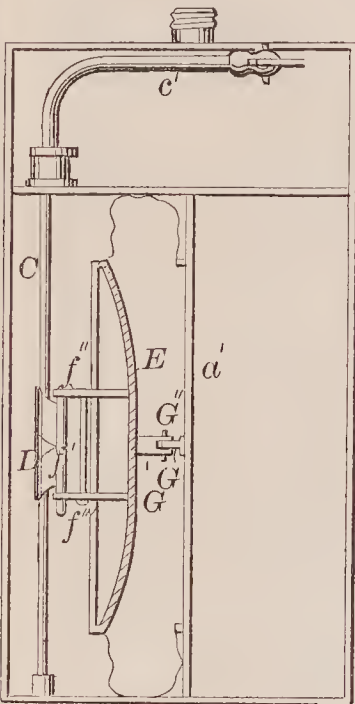
71518—C. C. Lloyd—Dry Gas Meter.
