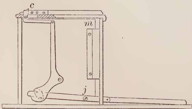
69661—J. B. Hannimann—Water Closet.
