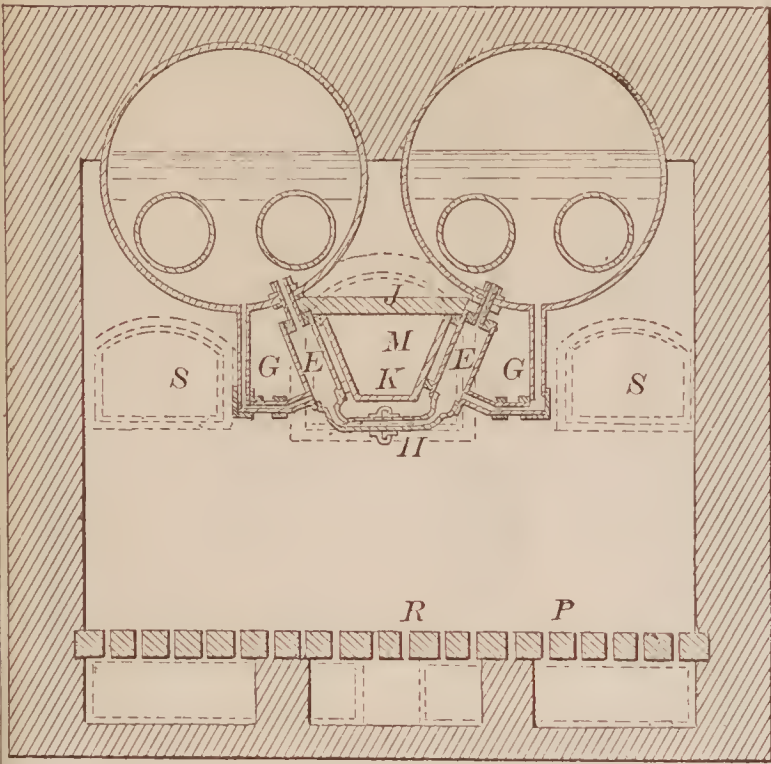
68703—F. Cook—Vaporizing and Burning Hydro Carbons.
