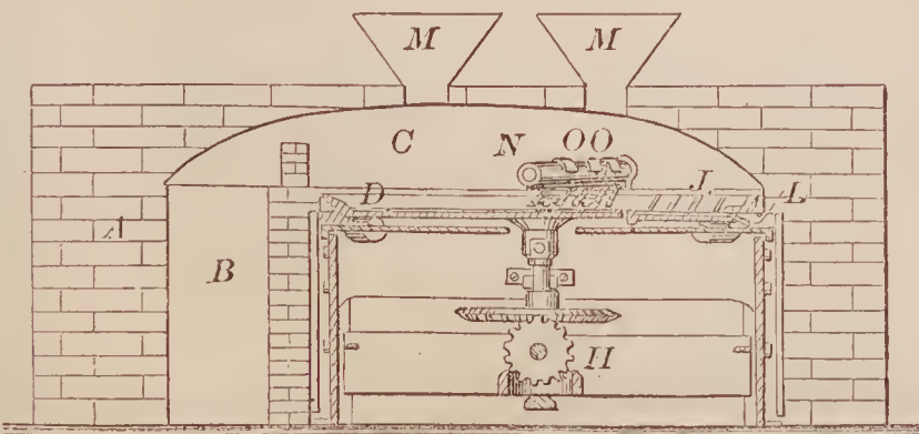
68406—Agrell & Klepzig—Furnace for Roasting Ores.
