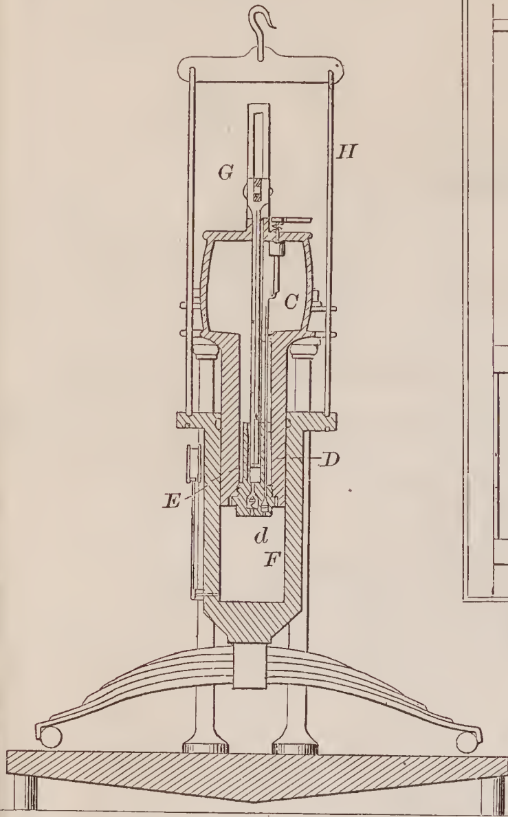
67531—C. Graham—Hydrostatic Press.
