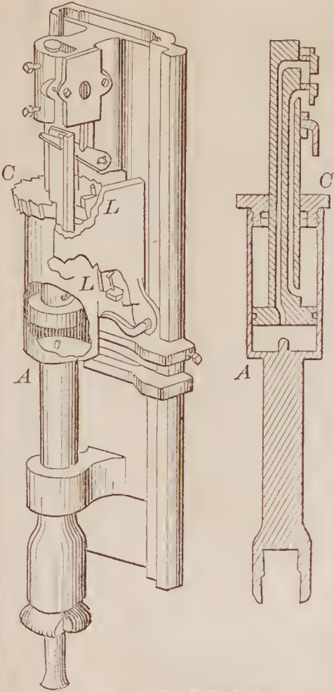
71329—Robinson & Wood— Rock Drilling Machine.
