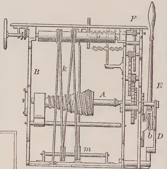
72608—C. M. Currey—Mechanical Movement.
