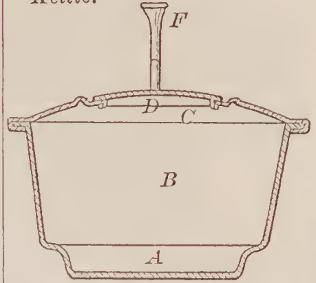
67425—S. B. Everitt—Tea Kettle.
