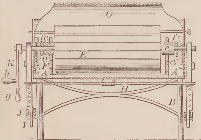
68155—E. Beckwith—Washing Machine.
