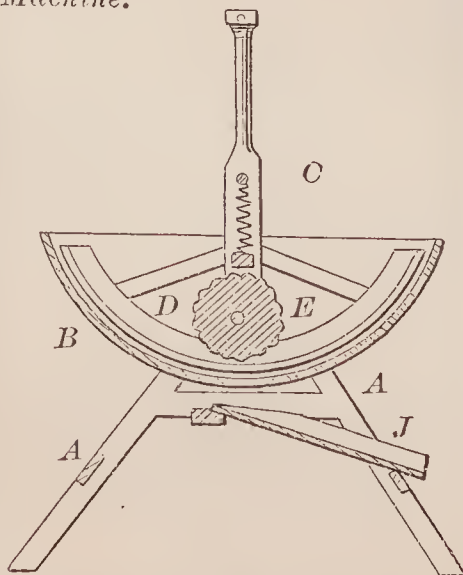
66831—W. Goodman—Washing Machine.
