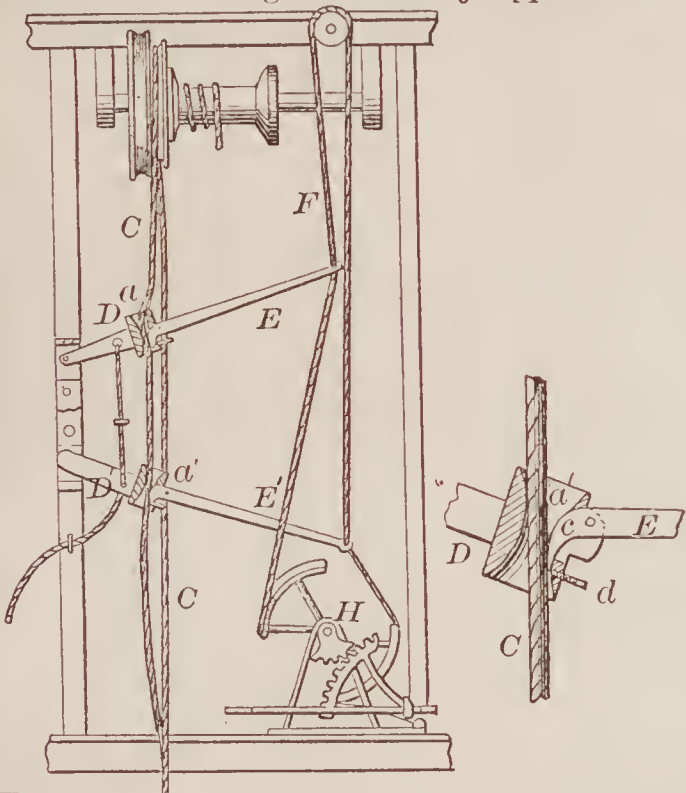
69977—C. C. Fellows—Clothes Line Clamp.
