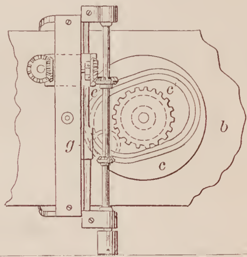
70451—S. McWorter—Sorghum Evaporator.
