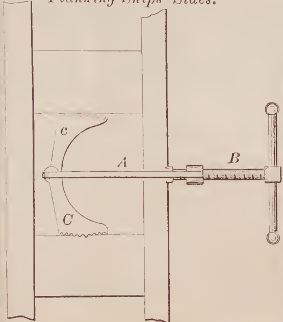
71387—J. J. Hill—Clamp for Planking Ships' Sides.
