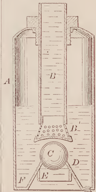
71007—R. H. Hilton—Air Chamber of Pumps.
