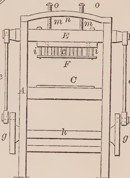
72492—E. A. Hill— For Punching Rubber Inner Soles.
