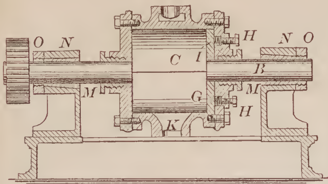
69383—M. L. Andrew—Rotary Engine.
