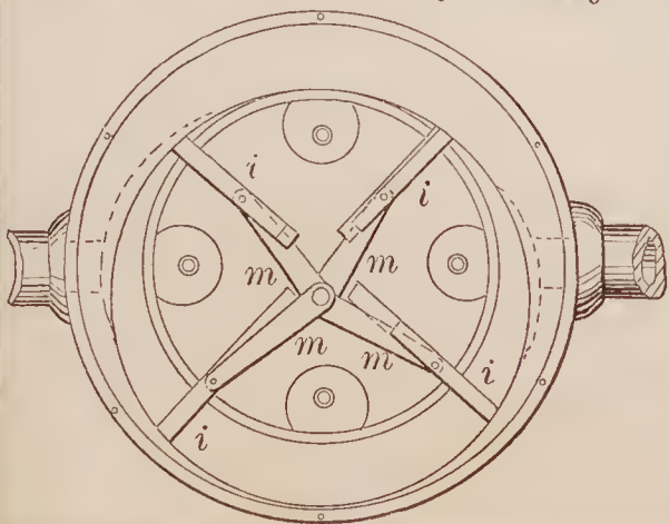
70242—Moore & Emery—Rotary Meter.
