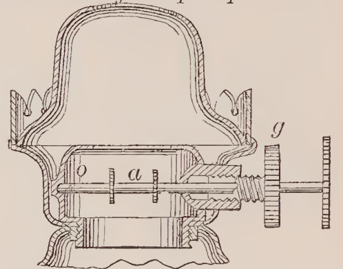
71872—C. P. Grosvenor— Preventing Lamp Explosions.
