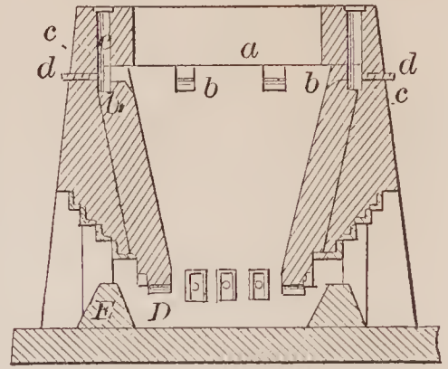
70046—A. Thoma—Furnace for Smelting Iron Ore.
