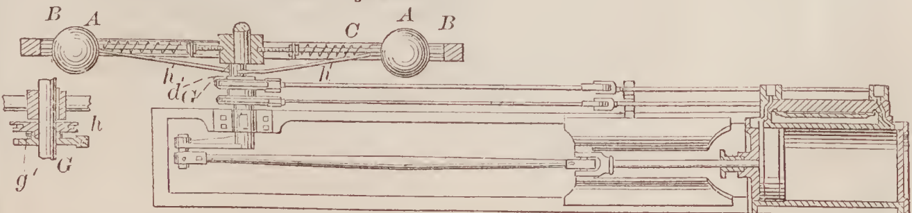
67936—J. H. Wooster—Steam Engine Governor.
