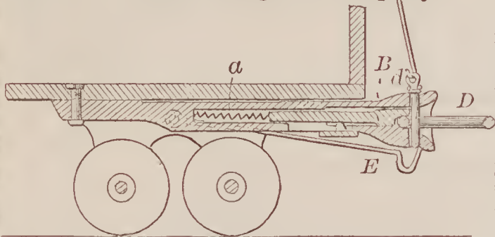
67368—W. S. Shortwell—Draw Head for Railroad Cars.
