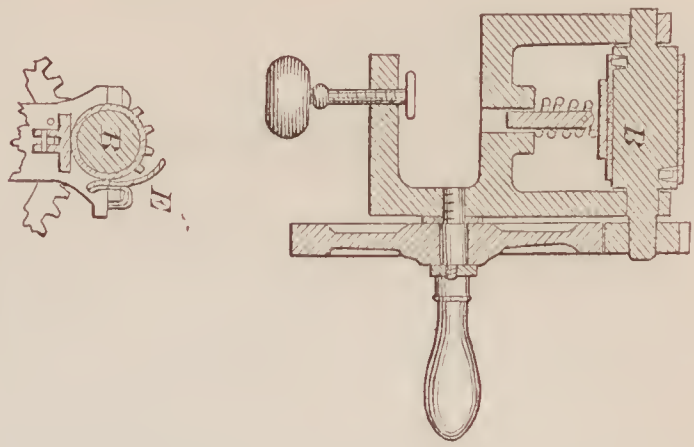
69906—F. Fisher—Tuyere.
