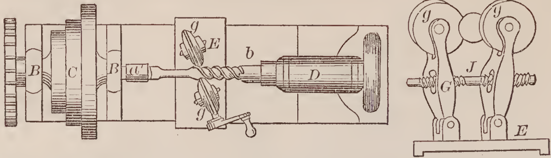
67396—W. Ashton—Screw Plate.
