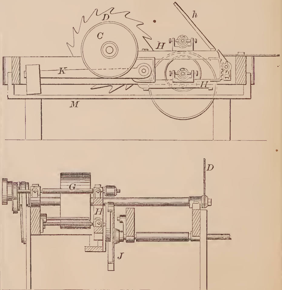
72763—J. Todd—Circular Saw Mill.
