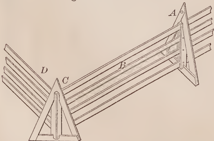
69214—J. C. Hughes—Portable Fence.
