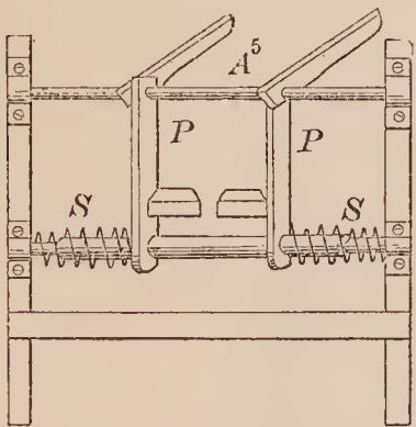
68973—J. Gerdom, Jr.—Chair, Lounge and Step Ladder.
