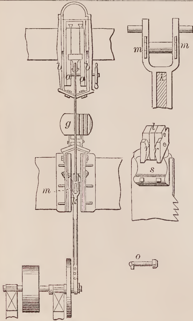
72155—A. P. Barlow—Saw Mill.
