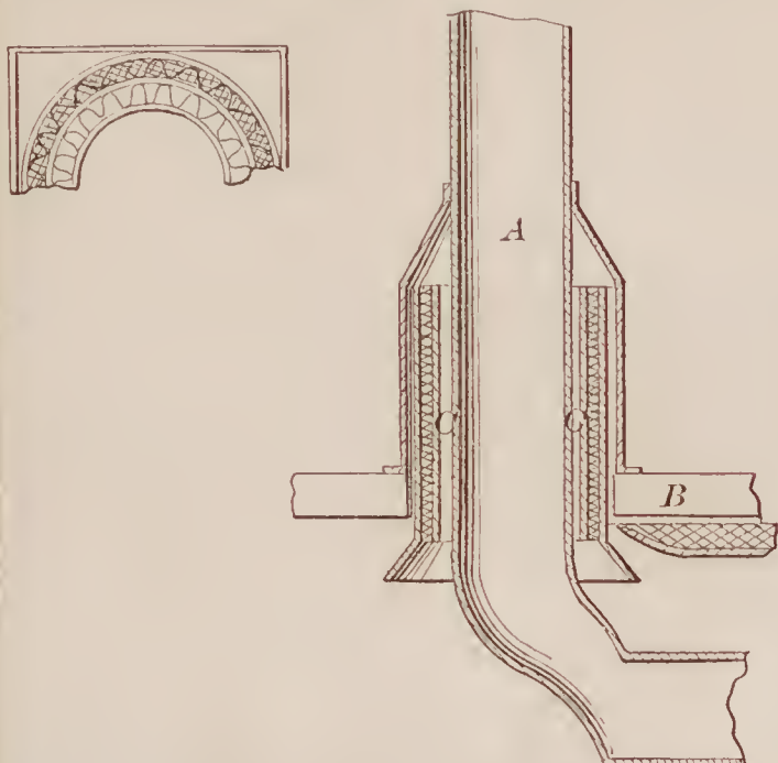
71300—J. B. Harris— Packing for Smoke Flues.
