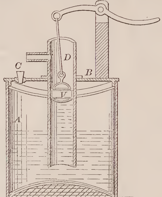
71044—E. Nickerson— Pump and Reservoir.
