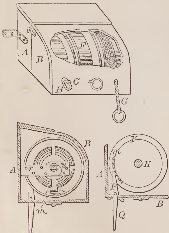
67459—J. D. Starritt—Clothes Line Reel.
