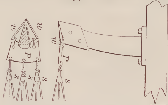
71578—W. H. Capewell—Glassmakers' Pot. A
