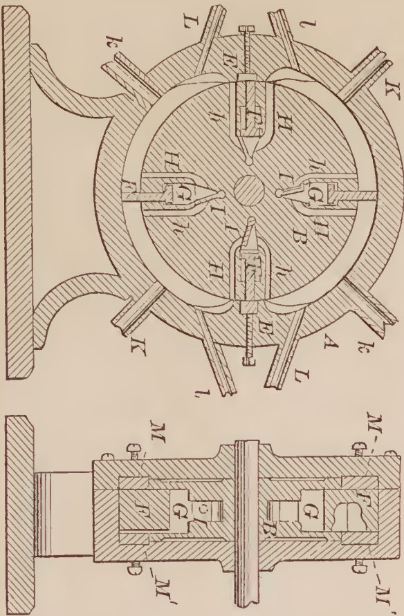
72537—R. D. Pettit—Rotary Steam Engine.
