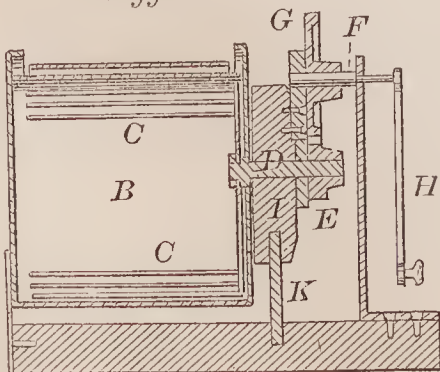
68037—G. E. Bridger— Egg Beater.
