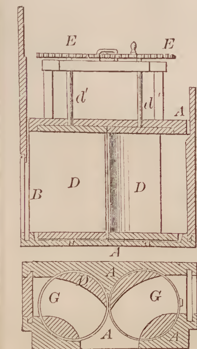
68692—C. D. Blakeslee—Gate for Water Wheels.
