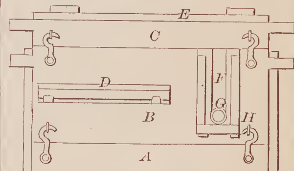
70740—B. C. Painter—Flask for Casting Tapers.
