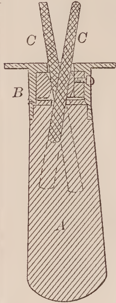
67011—McC. Young—Knife Sharpener.
