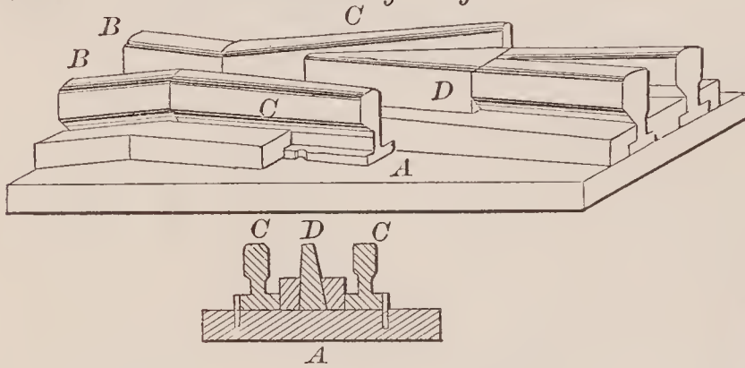
71905—S. N. Park— Railway Frog.
