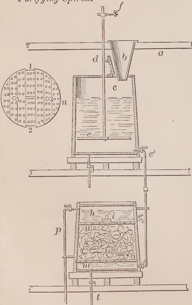
69390—W. F. Bearns—For Filtering and Purifying Spirits.
