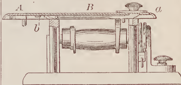
67635—E. H. Craige—Cloth Plate for Sewing Machines.
