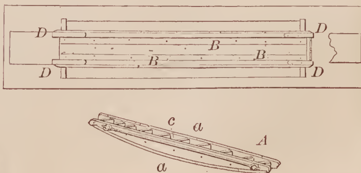
68391—S. Sowle—Staging.
