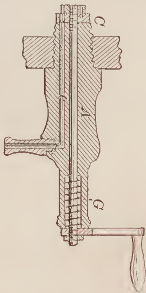
69702—J. G. Raymond—Boiler Gauge Cock.
