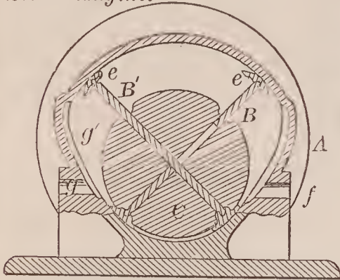
68186—S. G. Hall—Rotary Steam Engine.
