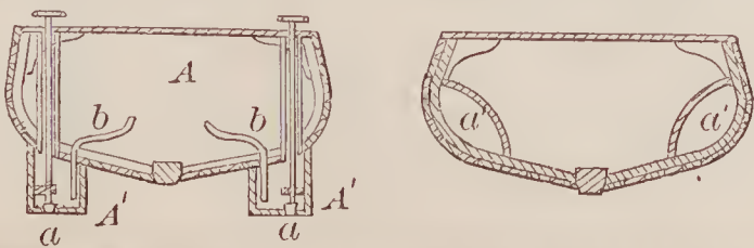
67241—N. F. Weston—Construction of Vessels.
