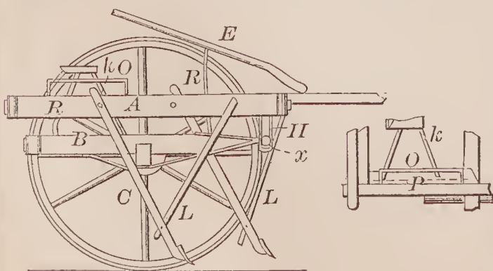
68124—W. A. Sisson— Wheel Cultivator.
