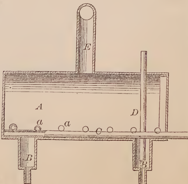
68974—S. Gibbons—For Refining and Distilling Oil.
