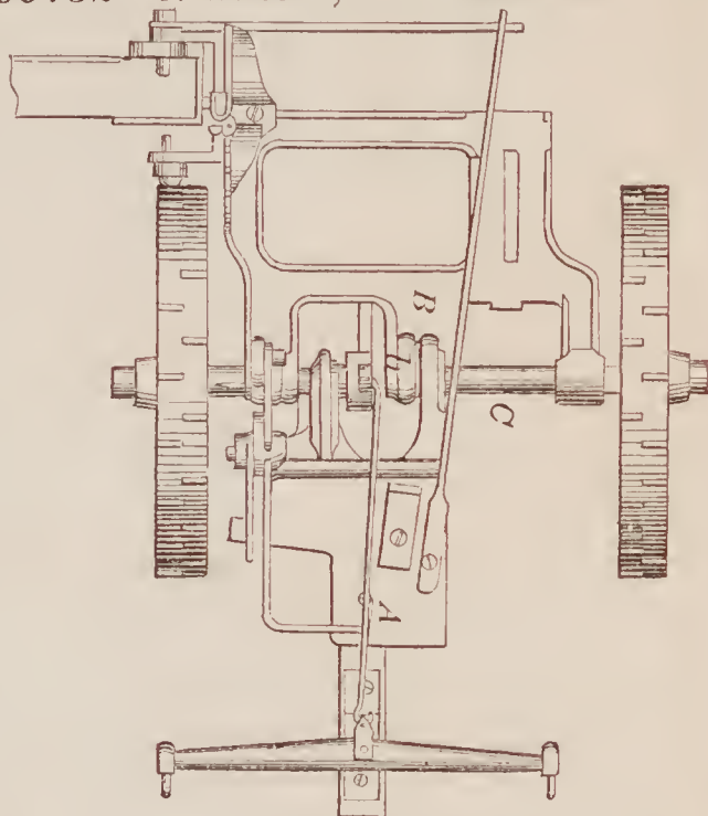
69732—C. Wheeler, Jr.—Harvester.
