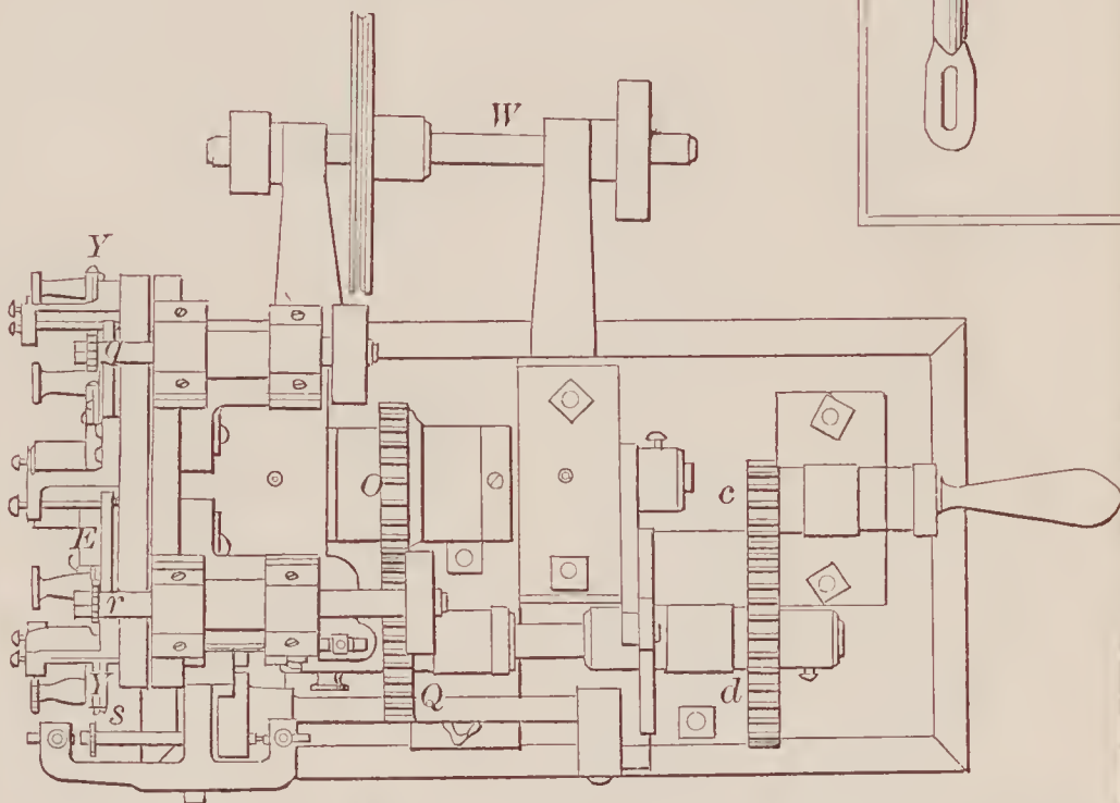
71839—A. Barberin—For Securing Ends of Wire Rope.
