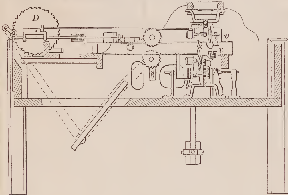
70382—F. W. White— For Making Blind Slats.
