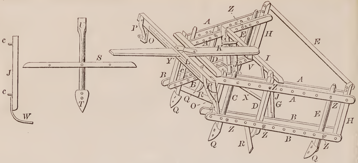
72109—E. Stewart—Harvester Rake.
