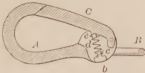
67020—C. B. Bristol—Snap Hook.
