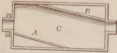
71448—W. Bruckner—Ore Roasting Furnace.
