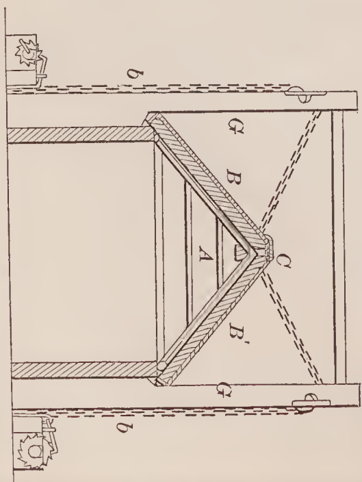
71855—M. Dek. Cuts—Construction of Roofs.
