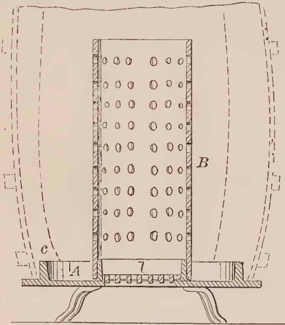
67062—J. F. Little— Barrel Cresset.
