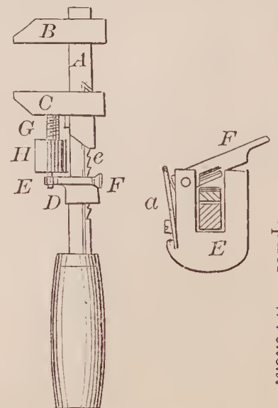
68168—T. D. Christopher—Wrench.
