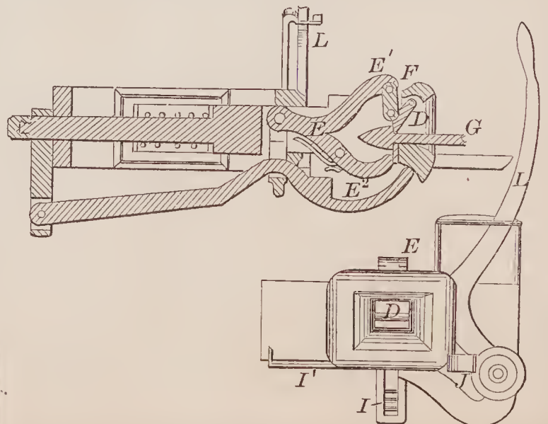
69693—Moore & Baker— Car Coupling.
