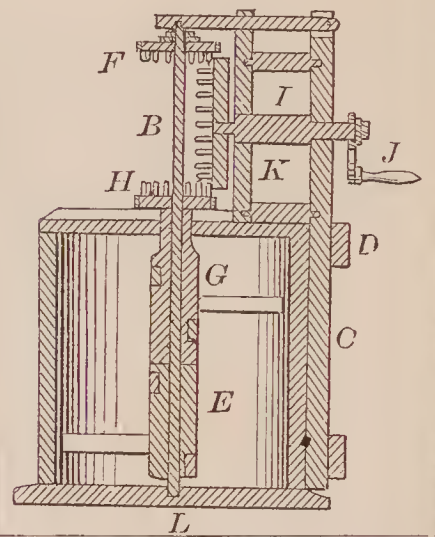
68806—A. D. Tingley—Brake for Horse Power.
