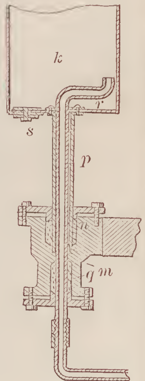
67329—W. J. McLea—Alarm Whistle.
