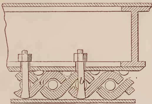
68474—T. Whitby—Armor for Ships of War.
