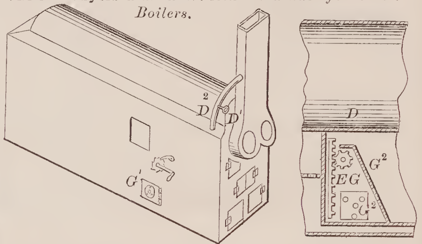
71503—T. Munger—Gate.
