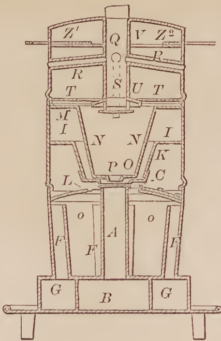
72580—Adams & Peckover—Coal Stove.
