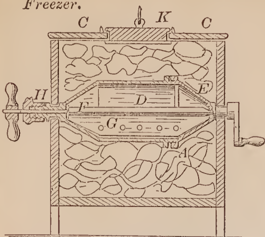
68968—F. H. Duc—Ice Cream Freezer.
