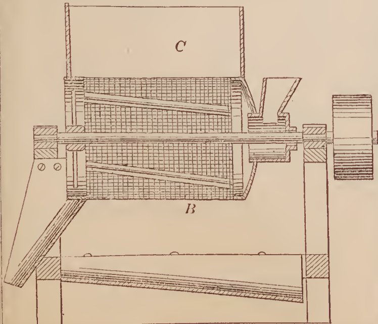
68915—D. H. Turner— Cooling and Purifying Animal Charcoal.
