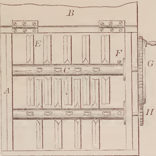
68062—G. B. Garlinghouse— Baling Press.
