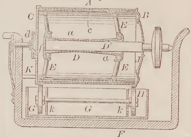
67931—Underwood & Johnson—For Soldering Cans.
