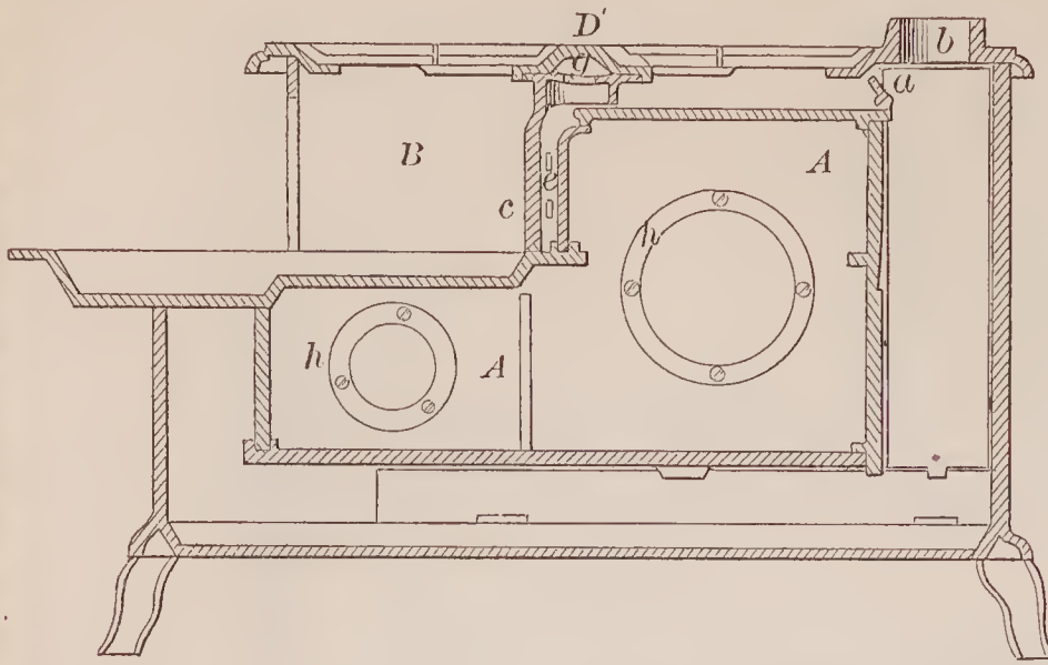
69536—C. H. Buck—Cooking Stove.
