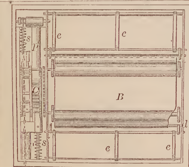
68997—G. T. Lape—Railroad Station Indicator.
