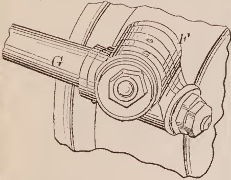
70661—W. N. Whiteley— Pitman Head and Crank Wrist Connection.
