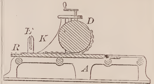
68033—W. E. Bird— For Making Cores for Pipe Casting.
