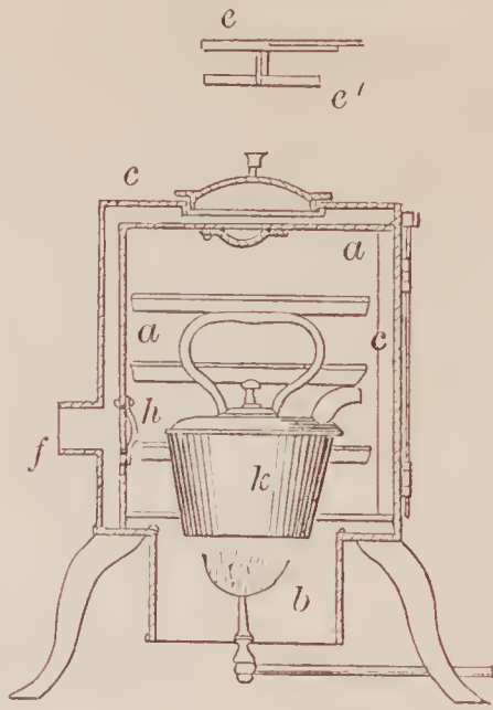
70207—D. G. Haskins— Gas Cooking Apparatus.
