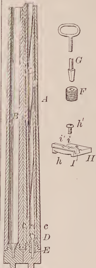
72063—S. McCulloch— Convertible Shot Gun and Rifle.
