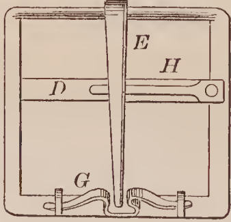
68204—W. B. Johnson—Buckle.
