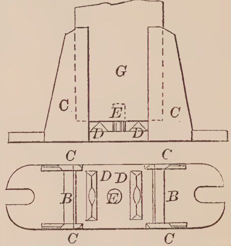
68907—H. C. Sergeant—Brick Machine.
