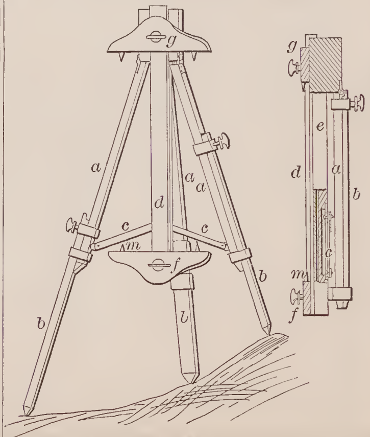
71858—P. Dechausc—Painters' Easel.
