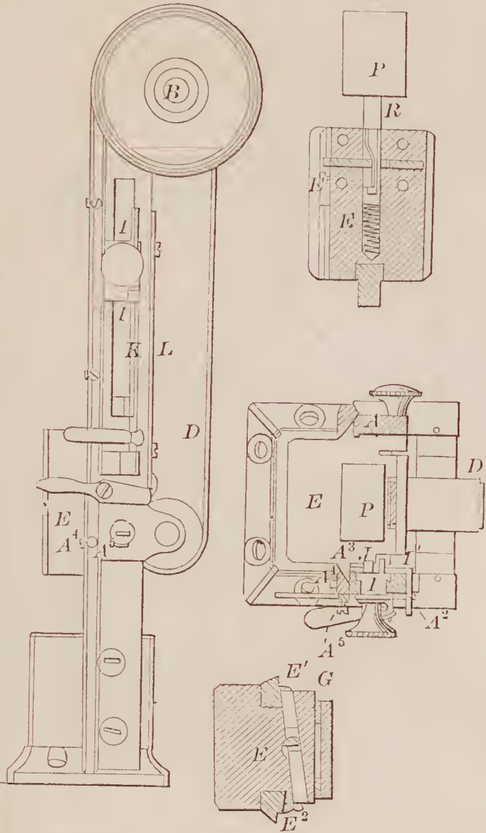
71081—E. Stimson—Door and Gate Spring.
