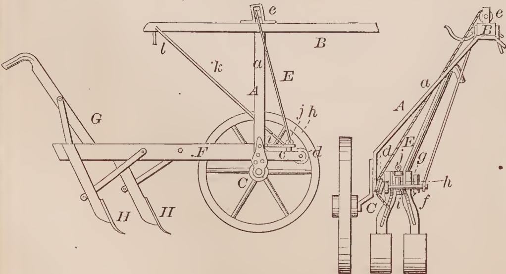
69071—M. C. Buffington—Corn Plow.
