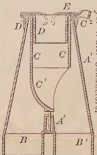
68682—E. B. Armstrong—Cut-off for Water Conductors.
