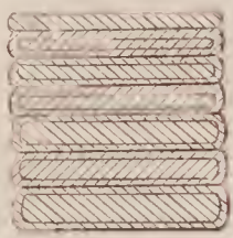
67683—W. A. Sweet—Fagot for Railroad Rails.
