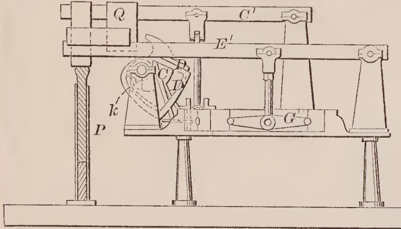
72288—R. Gracey—Bolt Heading Machine.
