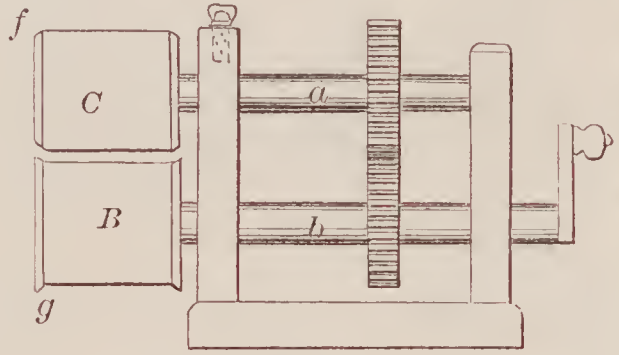
71680--C. Barry--For Making Tin Cans.
