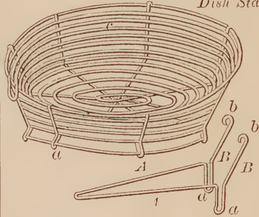
72770—Woods & Sherwood— Wire Dish Stand.
