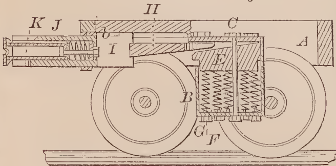
72891—S. Pennock—Railway Car.
