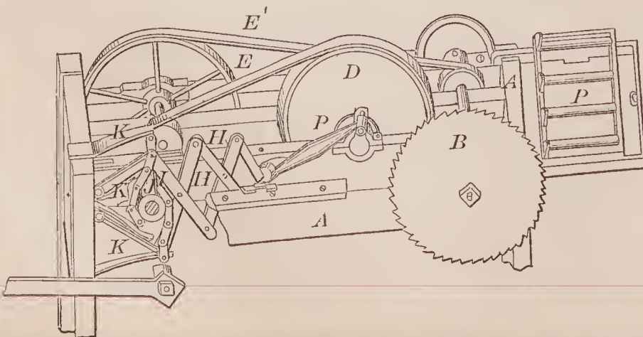
68074—E. Healy—Mechanical Movement for Working Saws, &c.
