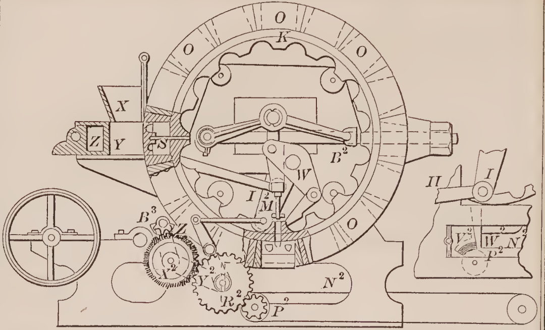
72220—J. North—Brick Machine.
