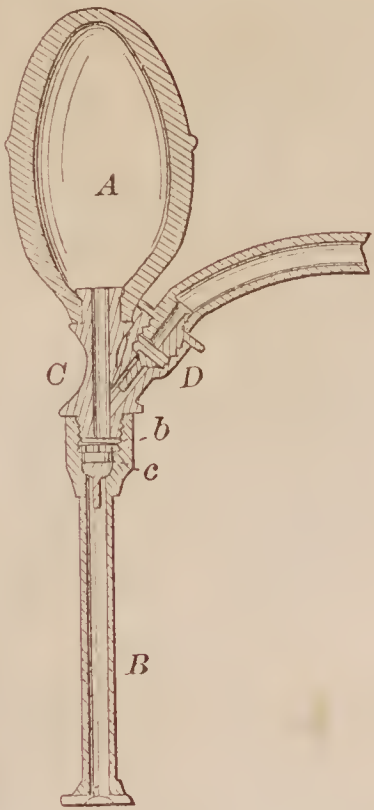
68630—E. J. Leyburn—Cupping Instrument.
