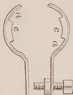
71838—L. J. Atwood—For Sizing Lamp Chimneys.
