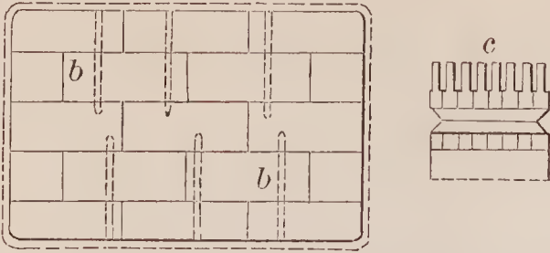
69707—J. Rupertus—Cartridge for Fire Arms.
