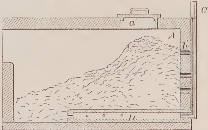
72694—H. Speeler— Heating Pottery Oven.
