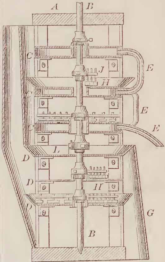
67256—H. Boden—Grain Dryer.
