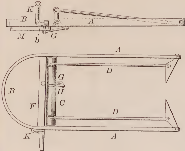
72288—R. Gracey—Bolt Heading Machine.
