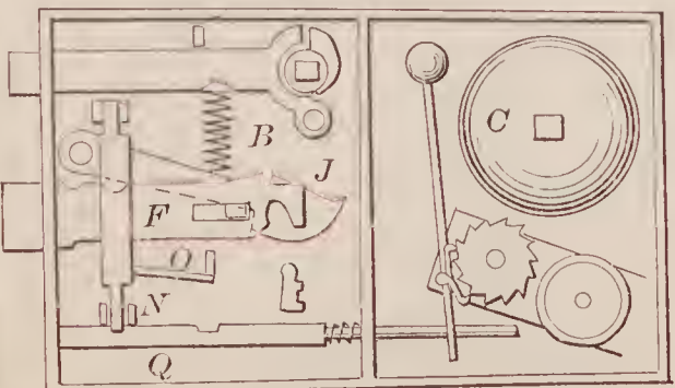
71822—E. Tracy—Burglar Alarm Door Lock.
