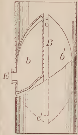
68062—G. B. Garlinghouse— Baling Press.
