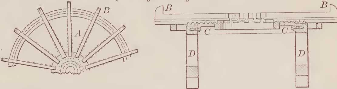
69818—H. Killam—For Compressing Carriage Wheels.
