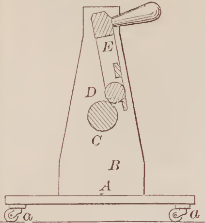
67388—C. E. Wareham— Mop Wringer.
