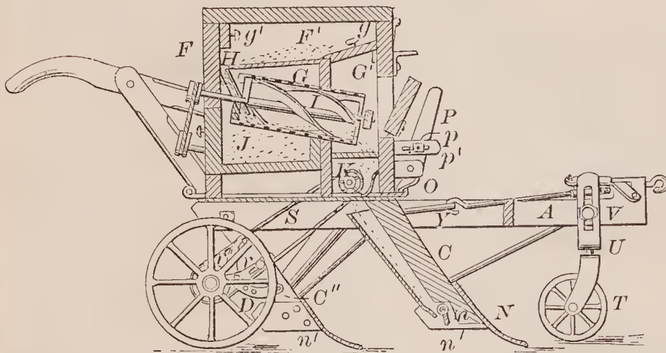
70897—J. Rancevan— Disconnecting Horses from Vehicles.
