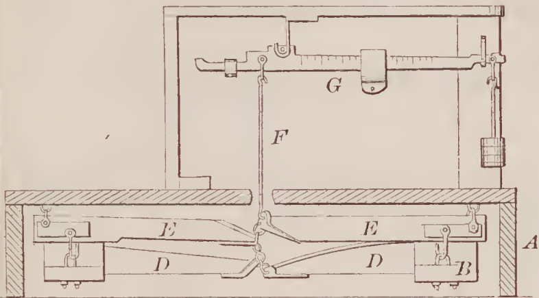
67596—L. M. Severance— Platform Scales.
