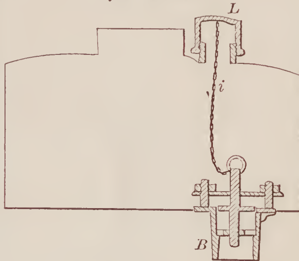
69745—S. Andrews— Safety Valve for Oil Stills.
