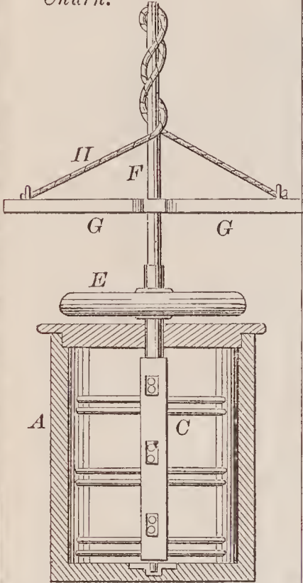
69624—M. M. Brown—Churn.
