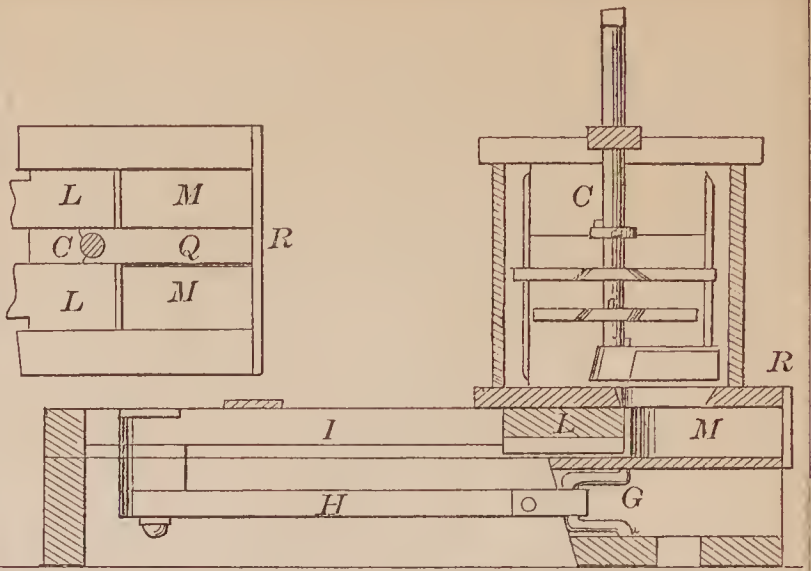
68987—H. Howard—For Heating Water and Generating Steam.
