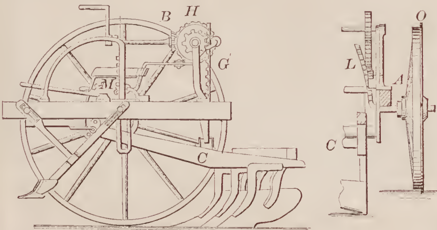
71053—H. L. Perry—Gang Plow.
