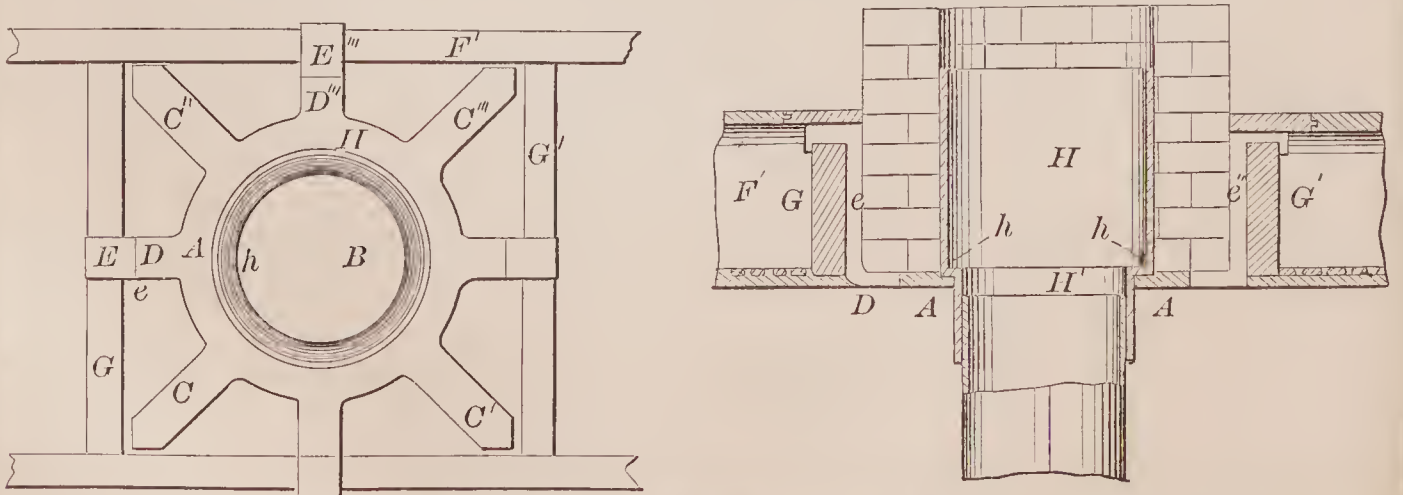
68628—A. Hutchinson—Stove Pipe Thimble.
