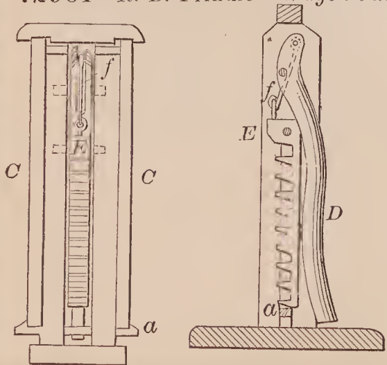
72901—R. B. Prindle—Wagon Jack.
