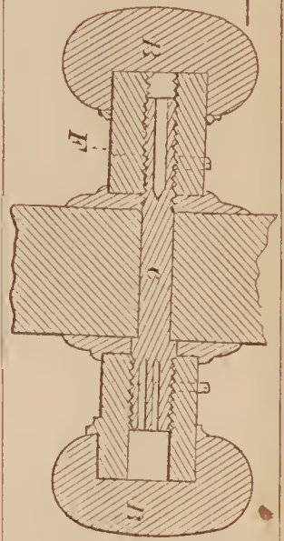
72815—A. Dawes—Spindle Knob.
