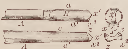
67825—D. Warner—Drill.
