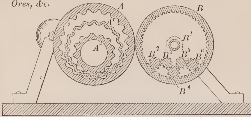
69656—Goodwin & Squire—For Crushing Rocks, Ores, &c.
