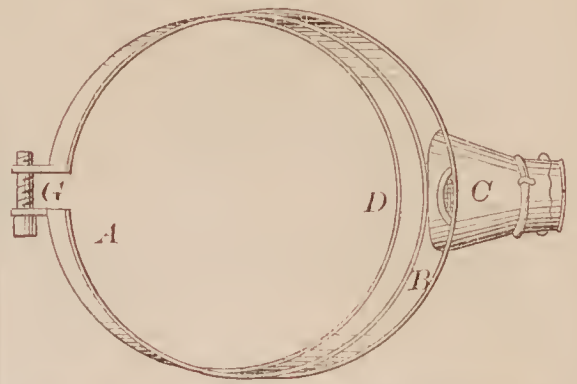
68793—W. F. Rossman—Milk Strainer.
