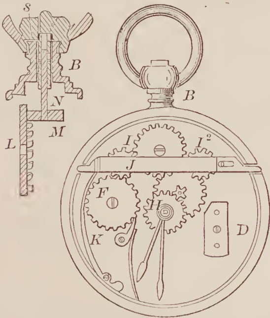
67823—A. Wadsworth—Stem Winding Watch.
