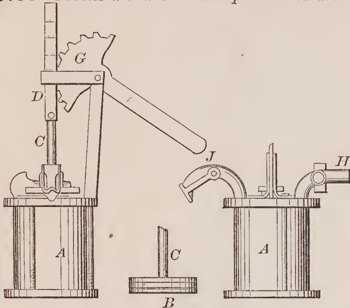
69756—Brooks & Munson—Pump and Measure.
