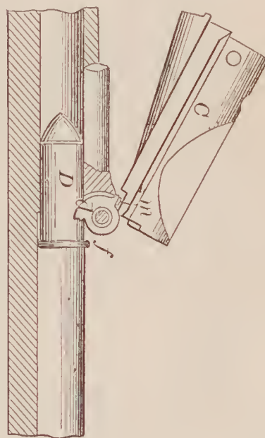
68099—W. H. & G. W. Miller—Cartridge Ejector for Breech-Loading Fire Arms.
