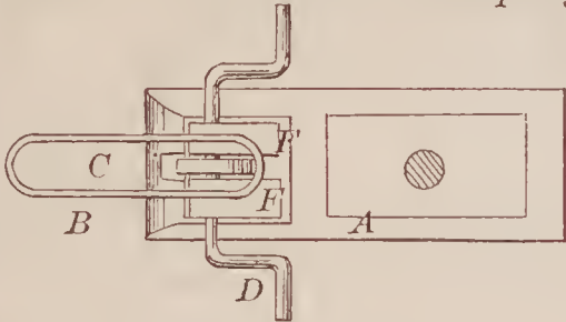
69266—S. H. Smith— Car Coupling.
