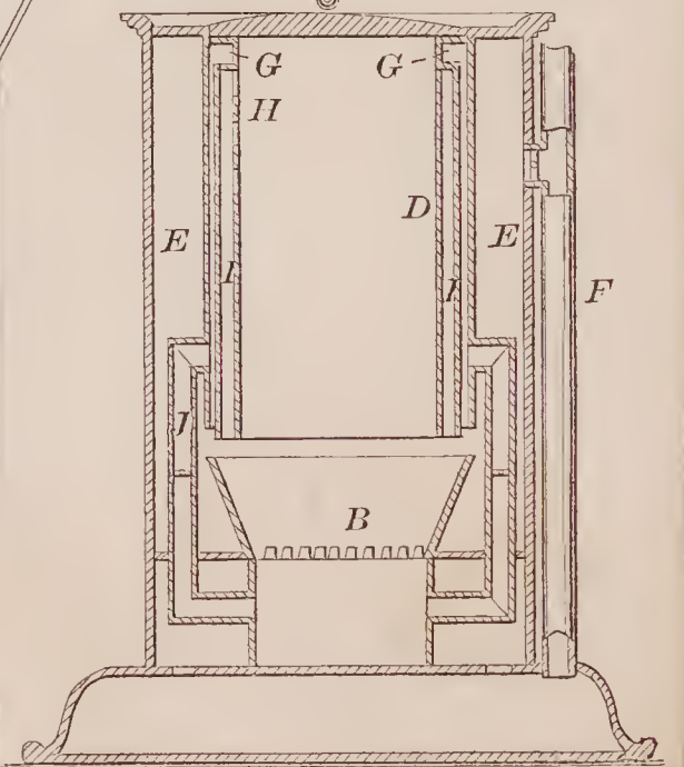
71347—C. M. Whelden—Stove.
