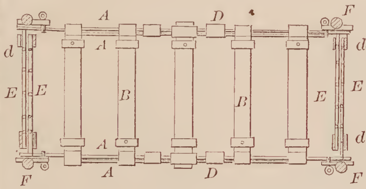
67055—J. Holzman— Extension Bedstead.
