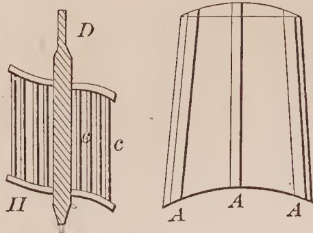
69064—W. D. Baughn—Metal Sleigh Knee.
