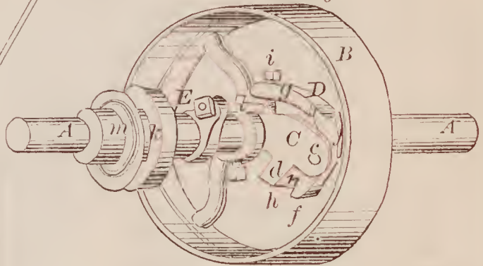
70888—C. D. Palmiter— Friction Clutch Pulley.
