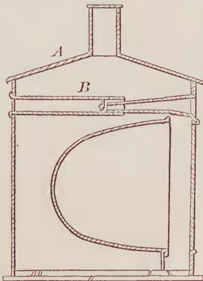
67192—E. L. Hall— Locomotive Head Light.
