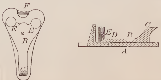
69646—J. H. Elward—Clamp for Ropes and Wires.
