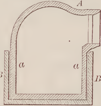
71578—W. H. Capewell—Glassmakers' Pot. A
