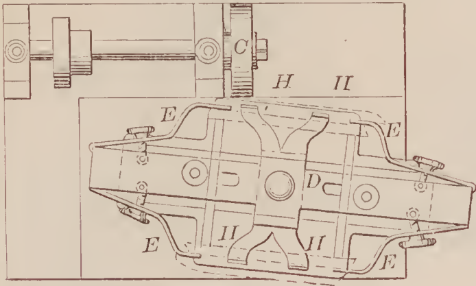
66853—A. Kipp, Jr.—For Grinding Skate Runners.
