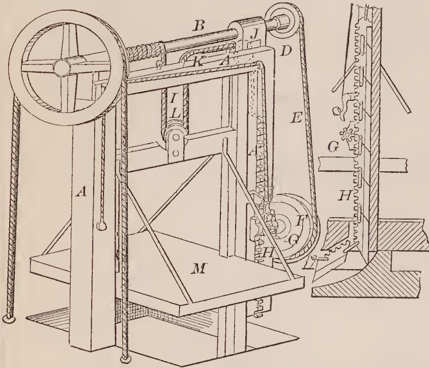
70565—P. Higdon—Hoisting Apparatus.
