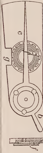
69053—A. Warren— Regulating Device for Watches.
