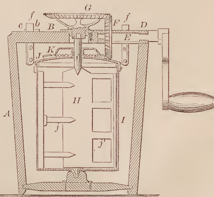
67133—C. W. Packer—Ice Cream Freezer.
