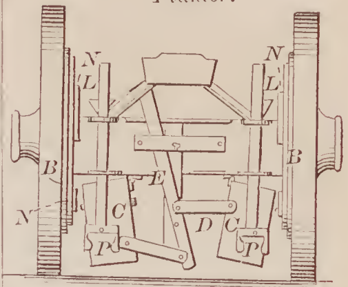
71488—S. C Hunter—Seed Planter.
