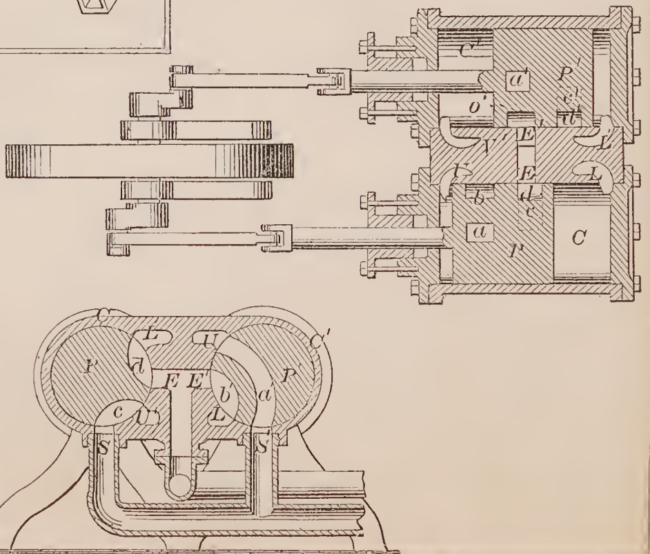
70590—E. McClintock—Steam Engine.
