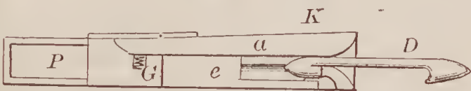
67468—Warner & Palmer—Car Coupling.
