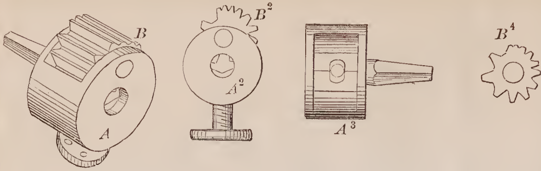
70113—A. S. Phillips—For Spooling Thread.
