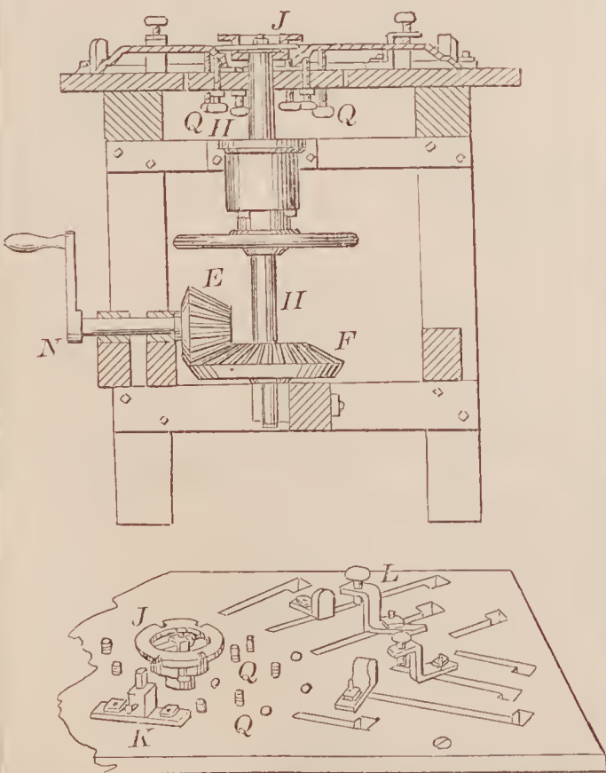
66992—A. P. Rich—For Fitting up Boiler Hole Seats.
