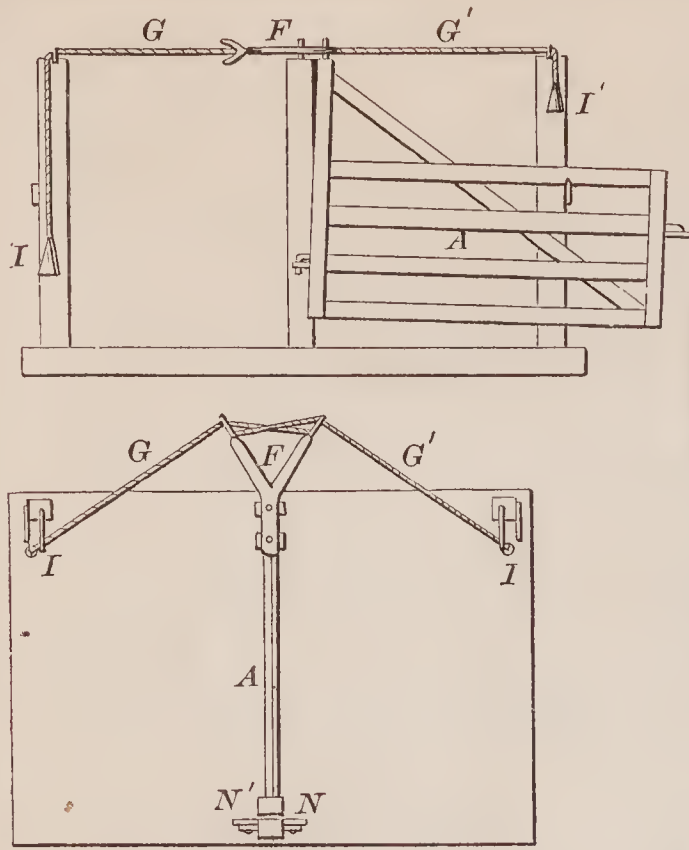
69788—D. Flint—Gate.
