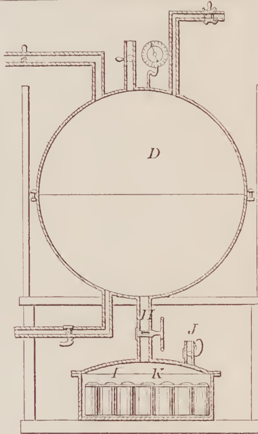
69920—W. Partington—For Cooling Malt Liquor.
