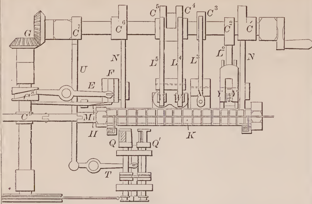
68593—R. T. Barton—For Making Needles.
