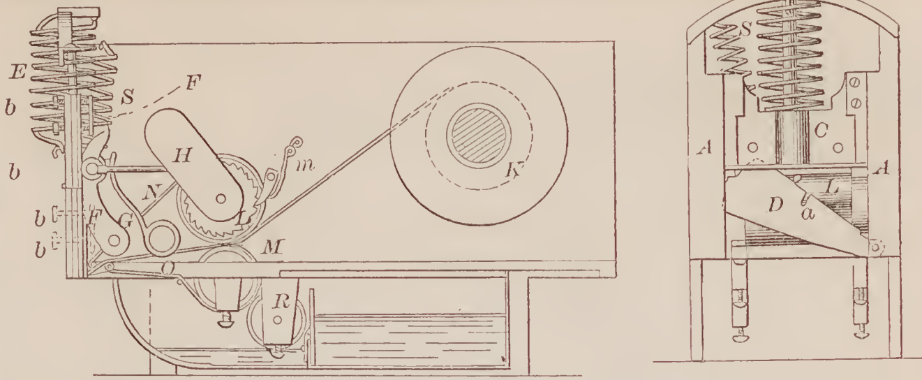
67833—J. F. Zacharias—For Attaching Labels.
