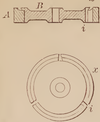
72405—C. Kingsland— Constructing Car Wheels.
