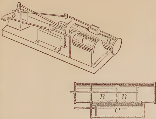
68938—Bancroft & Ward— Steam Engine.
