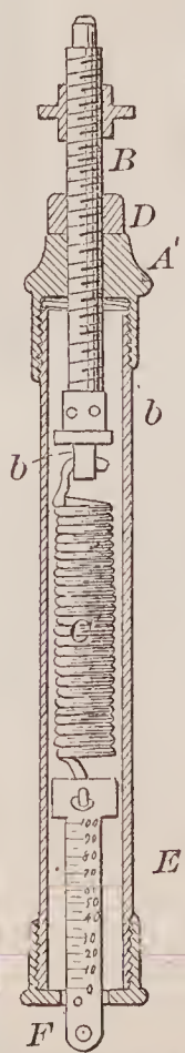
67482—W. G. Barker—Spring Balance.
