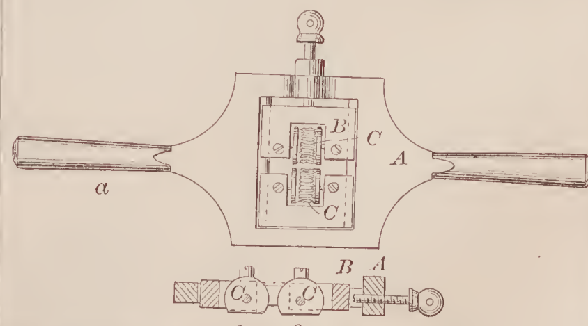
68498—H. Gill— Screw Plate for Cutting Screws.
