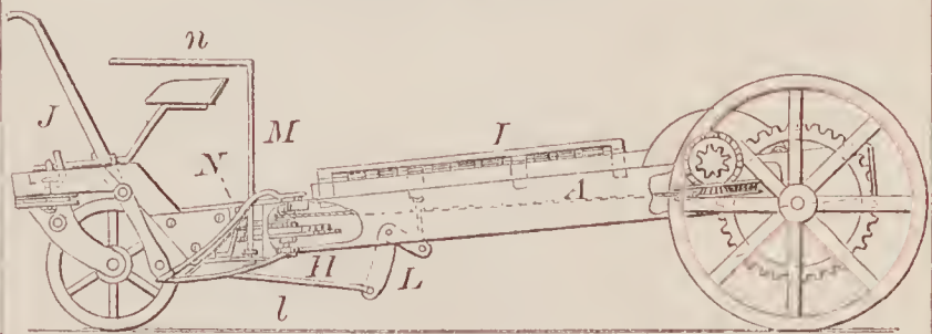
67955—Clinton, Prather & Hutchinson— Corn and Cane Harvester.
