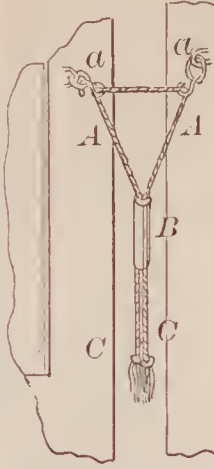
70300—W. H. Wayne—Shutter Fastener.
