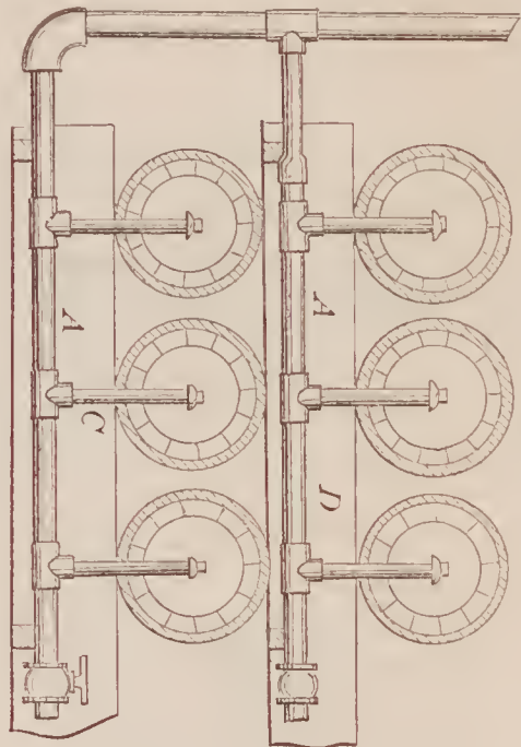
68181—S. Gibbons— Drying Barrels.
