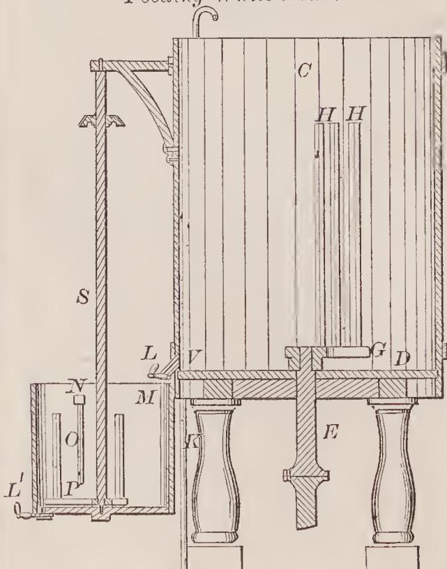
71612—J. Haslett, Jr— For Mixing and Feeding White Lead.
