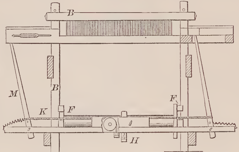
70186—G. W. Friestone—Hand Loom.
