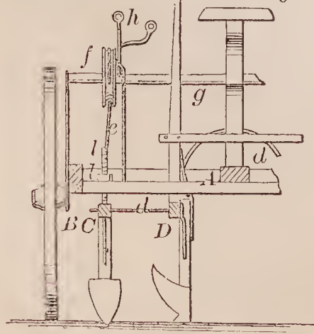
70615—J. H. Rankin—Sulky Plow.
