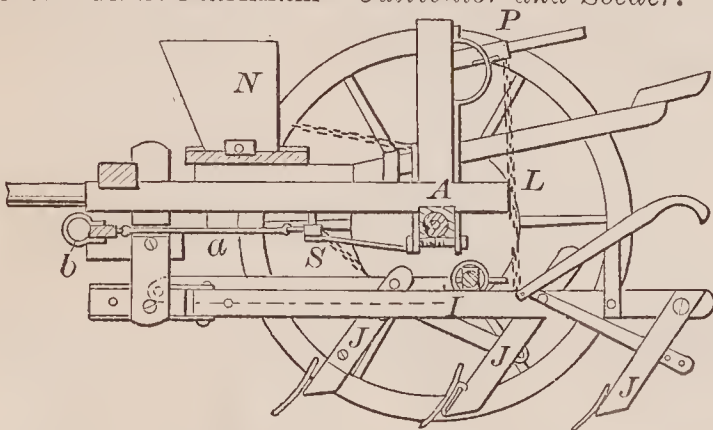
70345—A. S. Markham—Cultivator and Seeder.
