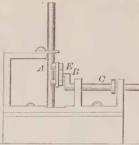
67957—E. R. Cole—Crank Connection.
