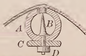
69341—G. G. Hickman—For Preventing Horses from Cribbing.
