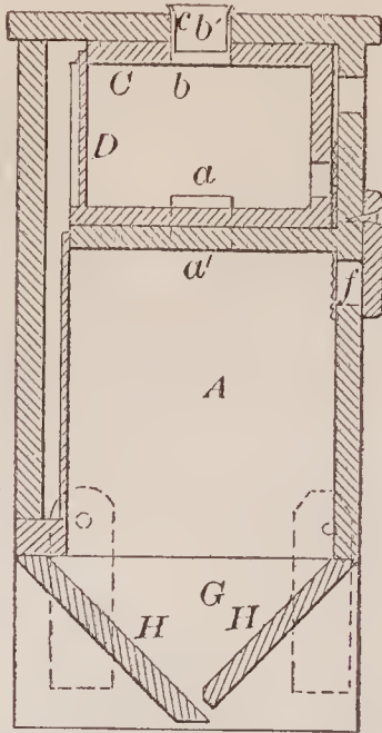
69574—J. Milne—Car Coupling.
