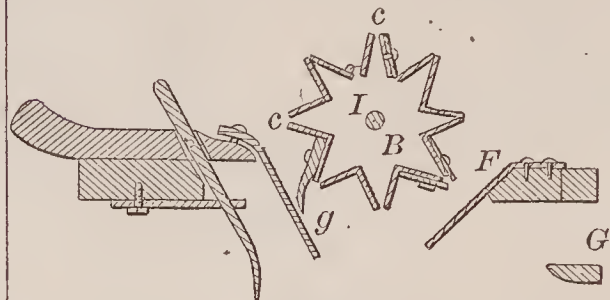
67484—E. Bennett—Thill and Pole Coupling.
