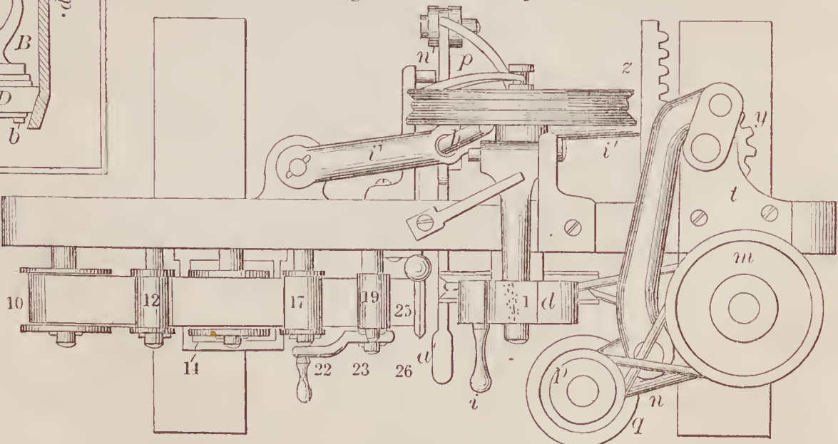
67669—Orr & Wright—For Making Paper Boxes.
