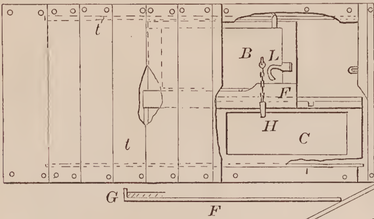
68694—S. E. Bright—Door for Grain Cars.
