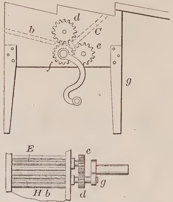
67568—I. C. Nichols— Beef Steak Preparer.
