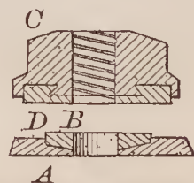
67539—D. B. Hart—Nut and Washer.
