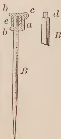
67029—S. Davidson—Tongue for Breastpins.
