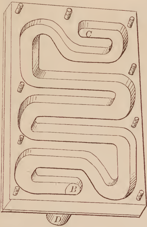
72723—Crum & Irwin—Burglar Alarm.
