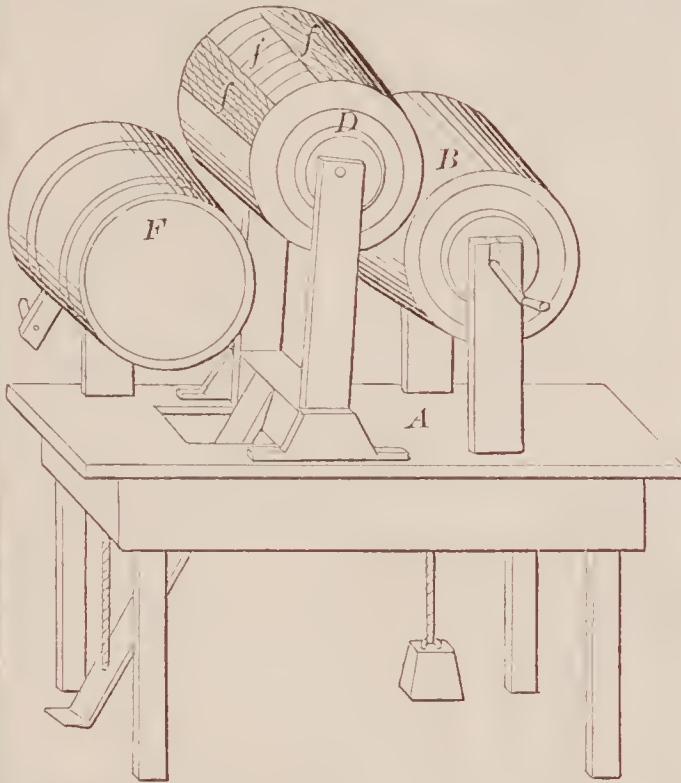
71978—J. Carter—For Graining Pails, &c.
