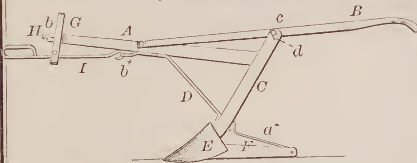
67595—S. F. Seely— Cultivator and Plow.
