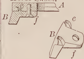
69208—C. P. Hawley—Wagon Spring.
