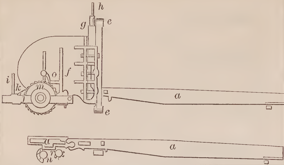
68144—Andrews & Tucker—For Making Match Splints.
