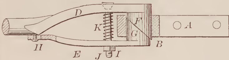
70225—W. J. Keeney—Pitman Coupling.
