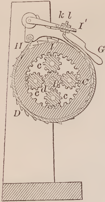
70181—T. B. Emerson—Clothes Wringer.
