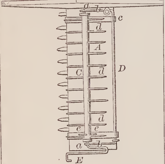
69838—K. H. C. Preston— Harvester.
