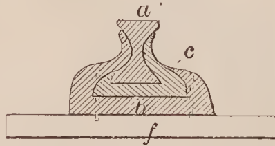
66930—L. M. Woodcock— Railway Chair.
