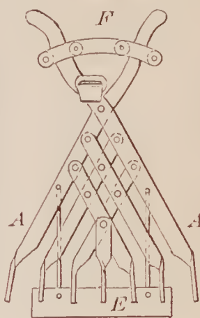
70669—D. Woodbury— For Making Bricks.
