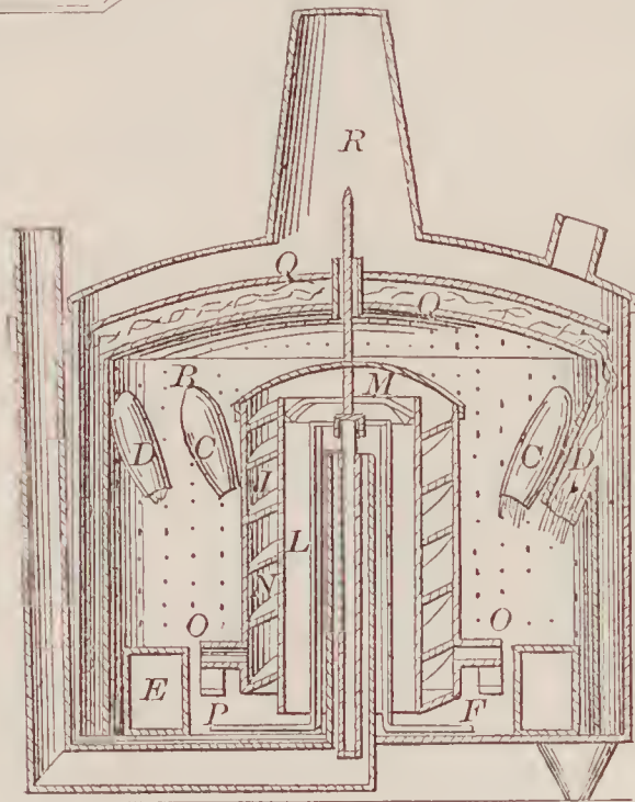
71665—Thompson & Hall— Carburizing Apparatus.
