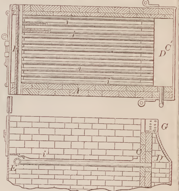
69505—W. Stevens—Furnace.
