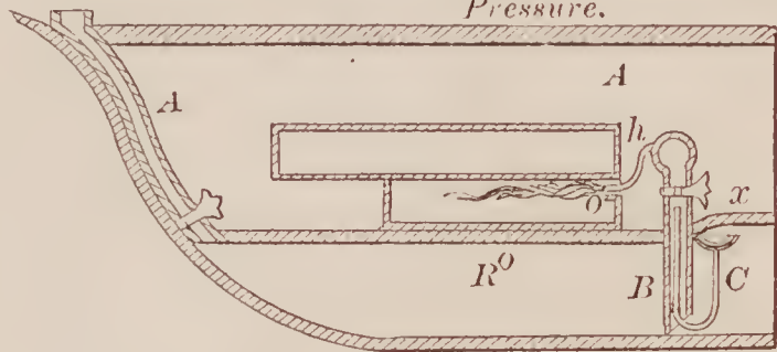
72101—J. II. Smith—Raising Oil by Pneumatic Pressure.
