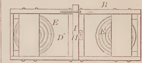
68112—J. H. Rhodes—Adjustable Pipe Joint.
