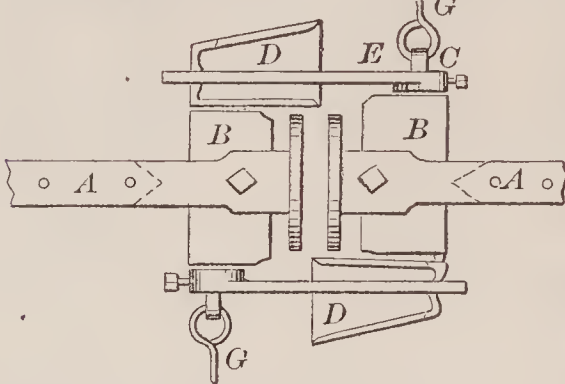
69574—J. Milne—Car Coupling.
