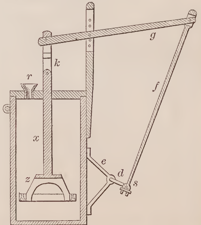
71469—W. T. Eastes— Churn.
