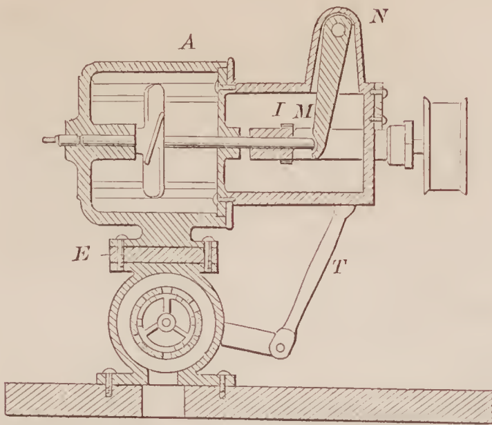
71016—A. Hutton— Steam Engine Valve.
