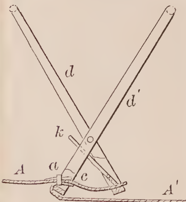
72325—C. O. Pike—Belt Fastener.
