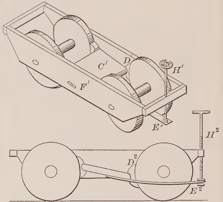
71856—S. Davis—Car Brake.
