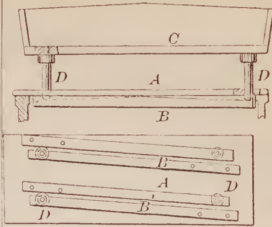
70619—R. N. Rockwell—Wagon Seat.
