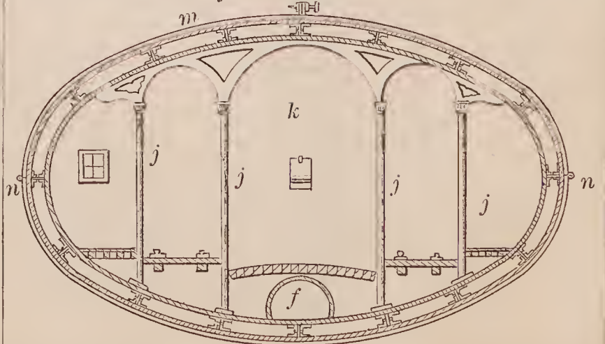
67035—R. Foley—Tunnel.
