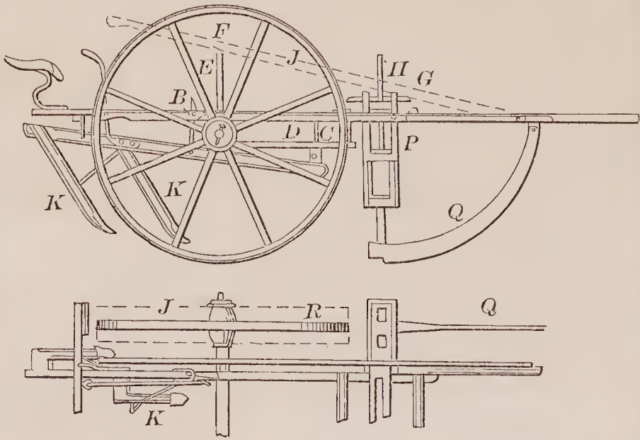
71134—I. H. Chappell—Planter and Cultivator.
