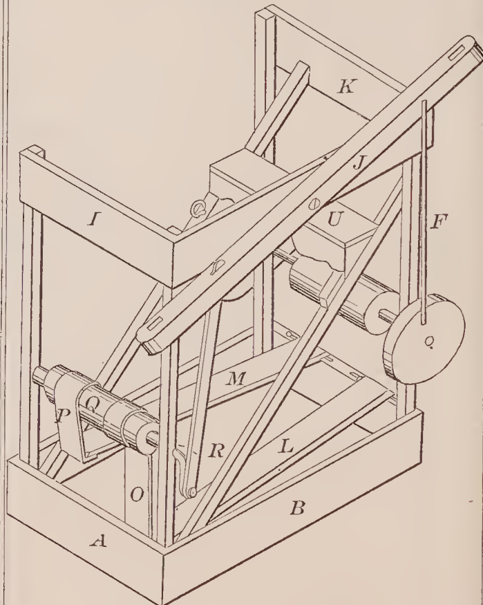
69382—W. C. Abbott—Treadle for Propelling Machinery.
