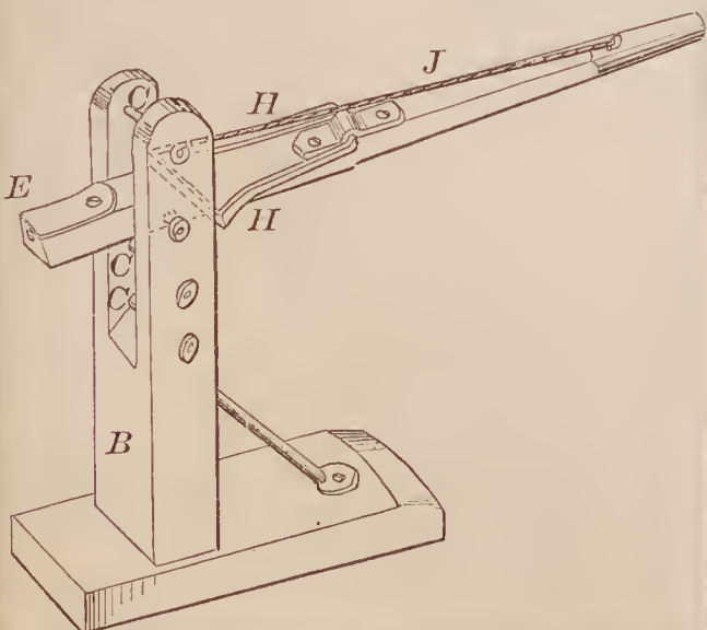
68837—A. C. Brinser— Lifting Jack.
