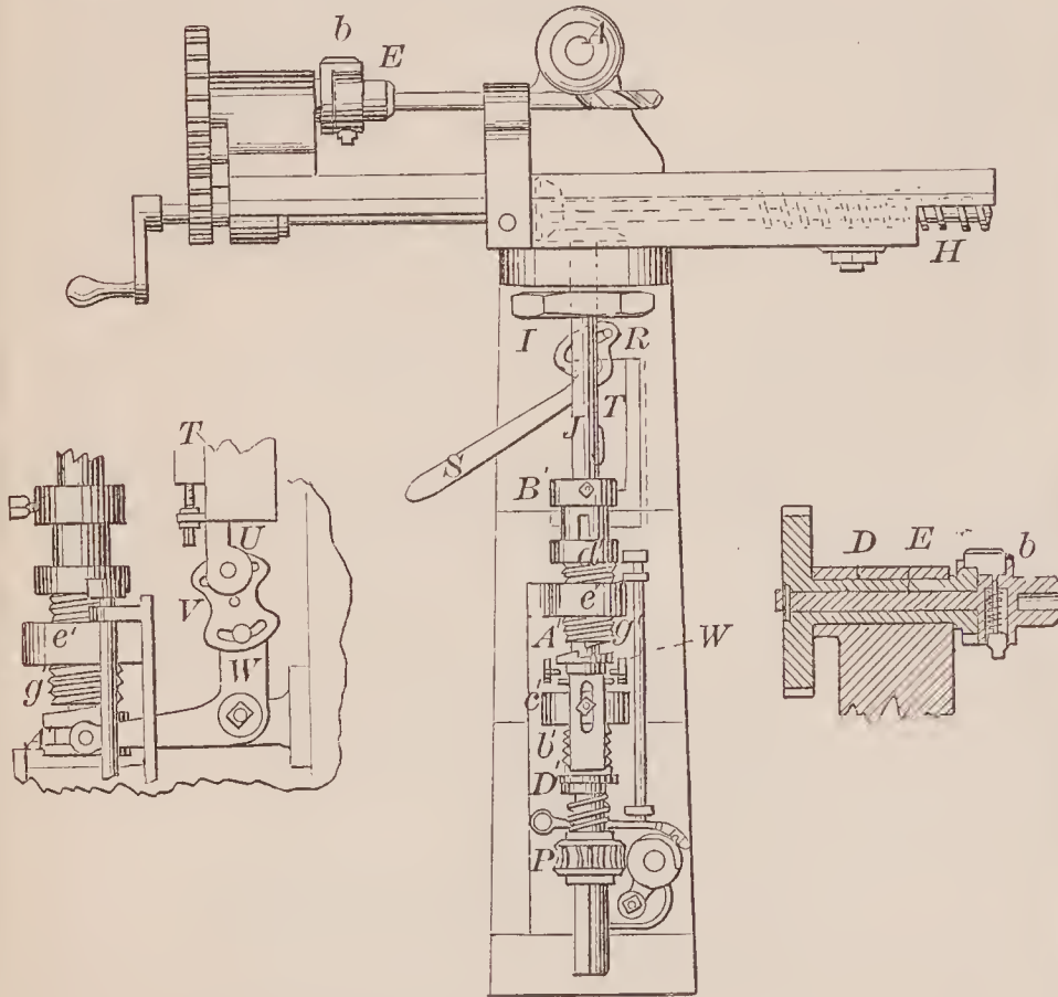
69466 —L. B. Miller— For Milling Twist Drills.
