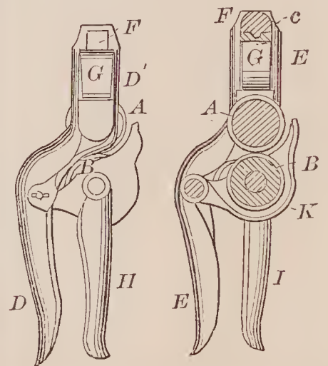
66836—Harrison & Harris—Clothes Wringer.
