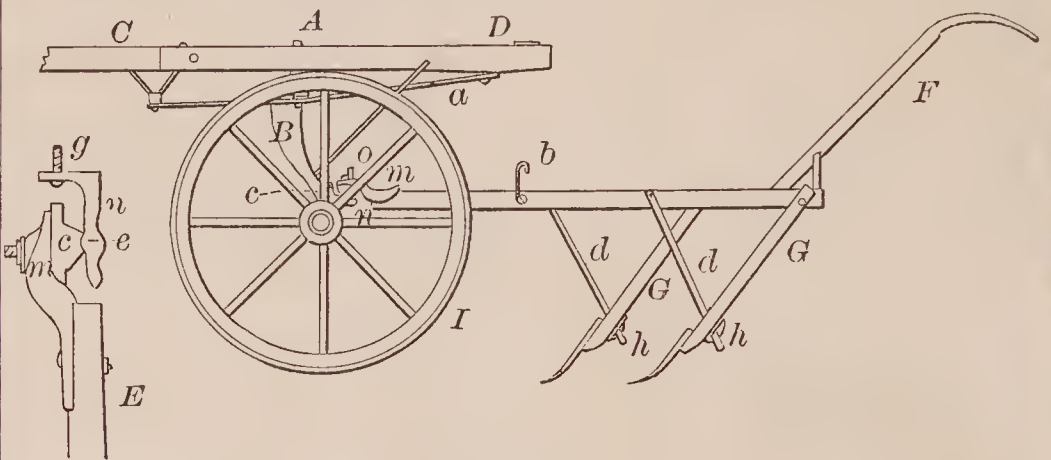
68643—G. Moore—Cultivator.
