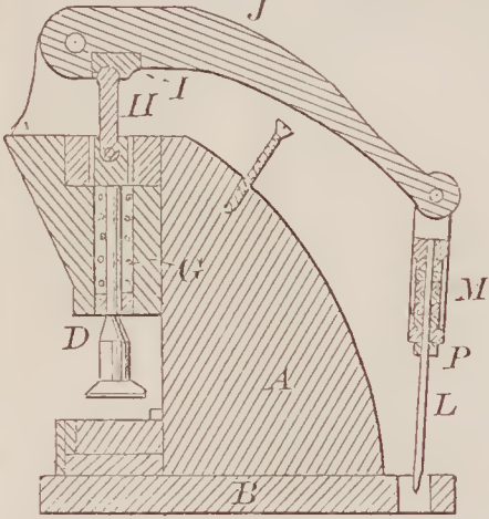
67650—C. H. Helms—Heel Press for Boots.
