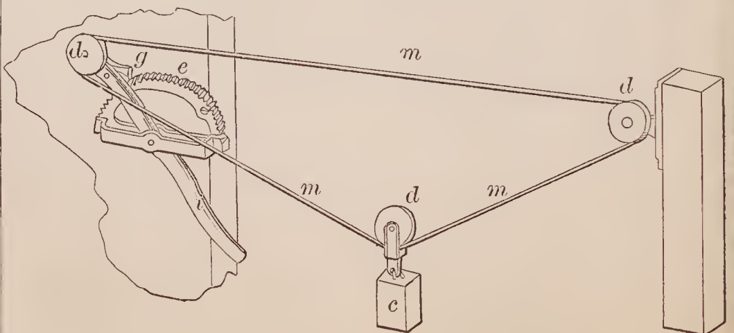
70665—J. L. Willcox—Clothes Line Holder.
