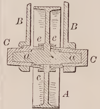
71057—L. B. Pitcher—Roller Wheel for Plows.
