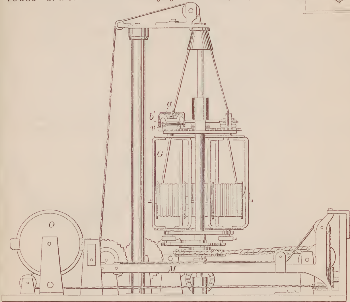
70685—S. & J. A. Bazin—For Laying and Twisting Rope
