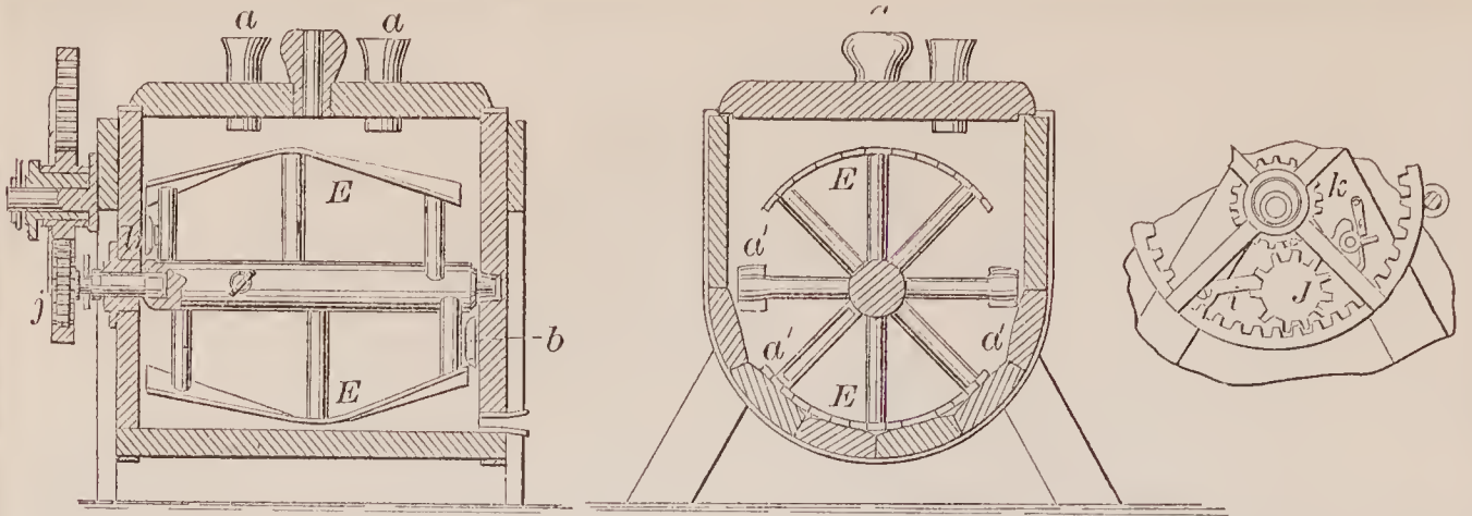
69624—M. M. Brown—Churn.
