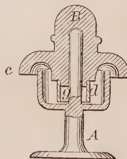
71418—W. E. Simonds— Telegraph Insulator.
