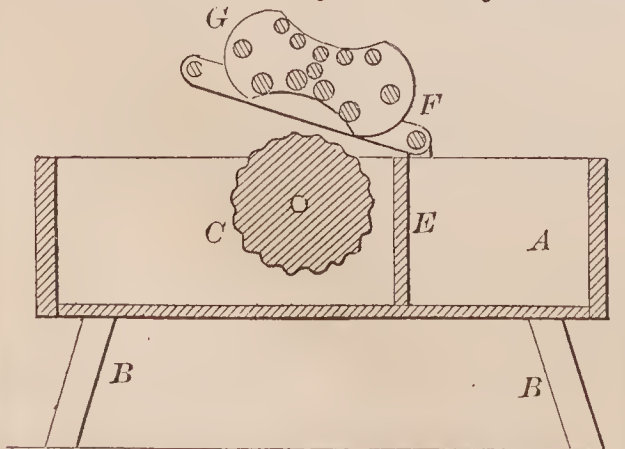
67069—Platt & Gray— Washing Machine.
