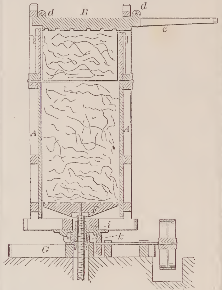
67961—J. G. Cummings—Cotton Press.
