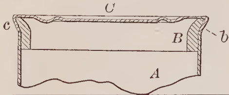
67280—W. Foster—Railway Chair.
