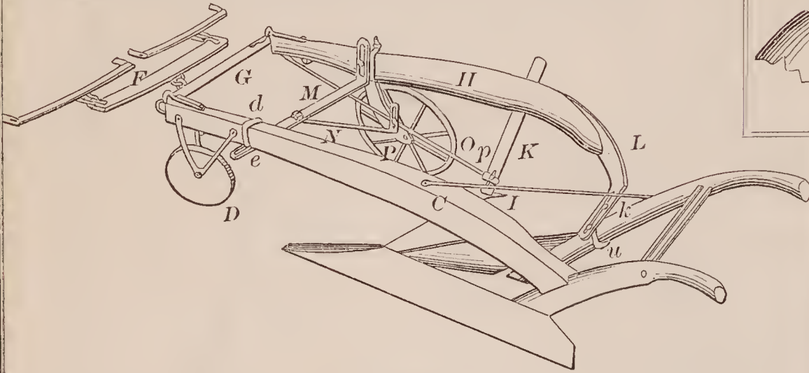
68099—M. R. Jones—Subsoil Plow.
