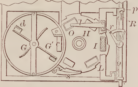
67541—P. Hayden—Brick Machine.
