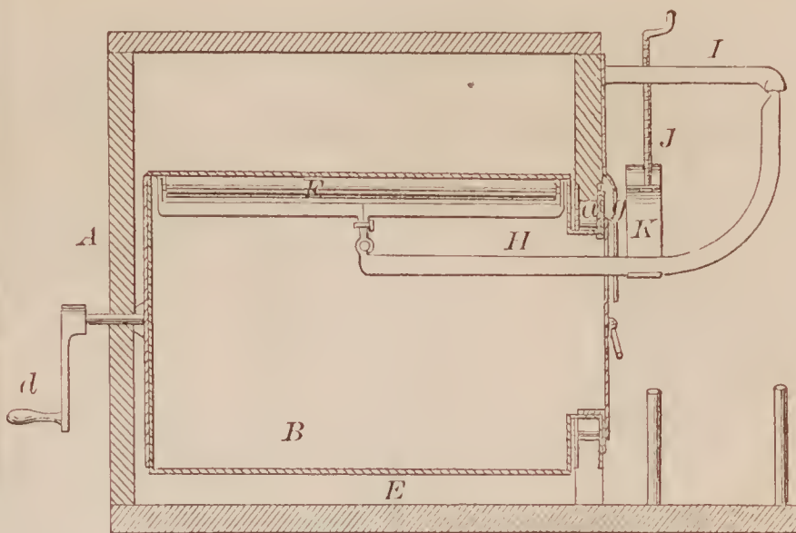
68734—J. Gray— Ice Cream Freezer.
