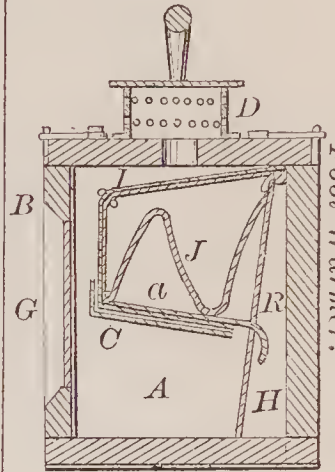
67622—Wirts & Swift— Lantern and Foot Warmer.
