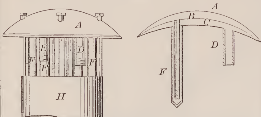
71605—W. T. Gillinder— For Forming Threads on Sheet Metal Caps.
