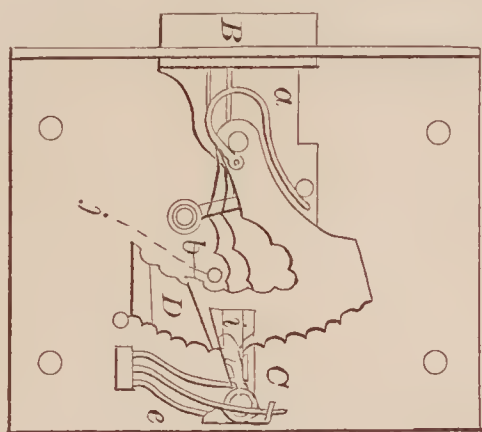
72499—H. Jackson—Door Lock.
