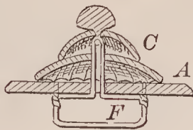
70253—F. Painter—Tension Regulator for Looms.
