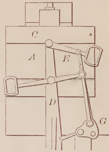
68061—A. M. Freeland— Belt Shifting Device.
