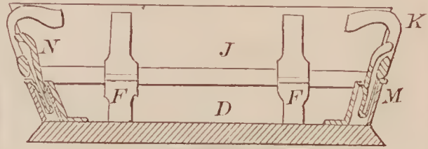
68716—J. Dimelow—Kiln for Burning Clay Pipes.
