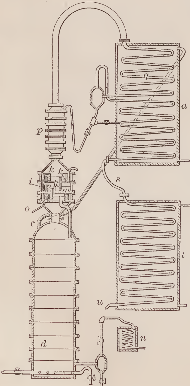
67863—A. Foubert— For Distilling and Rectifying Spirits.
