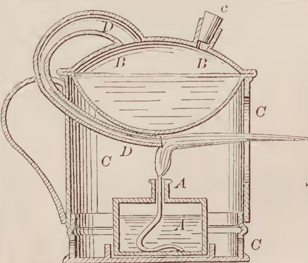
71826—G. Wanier—Plumbers' and Painters' Lamp.
