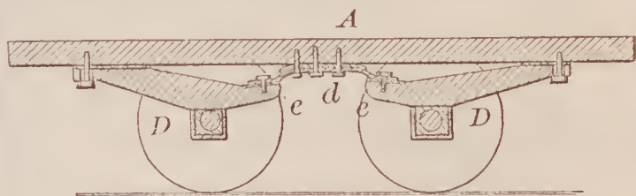
70269—D. T. Robinson— Railway Car.
