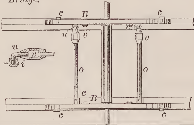
71672—B. F. Williamson—Scroll Saw Mill.
