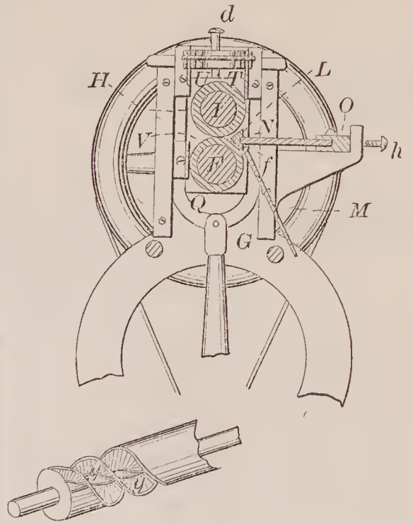
67923—Spofford & Hersey— Cotton Gin.
