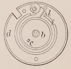
71639—O. E. Pillard— Tumbler for Permutation Locks.
