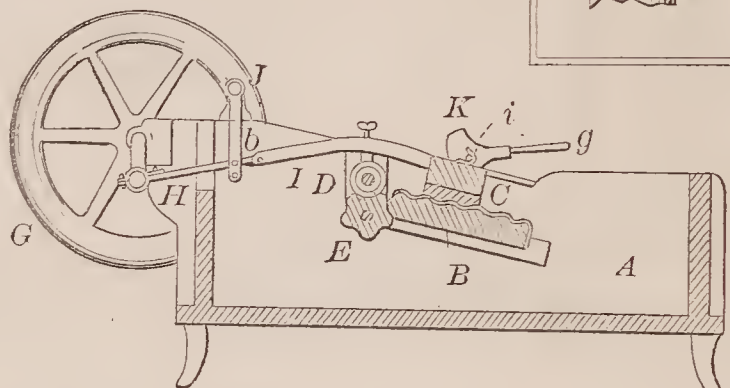
69261—H. F. Seinders—Washing Machine.
