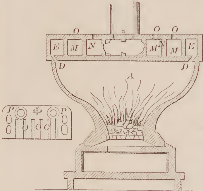
72242—J. P. Troxell—Sad Iron Heating Stove
