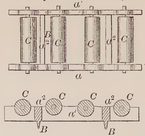
69868—R. M. Van Sickler— Roller Frame for Elevator Platforms.
