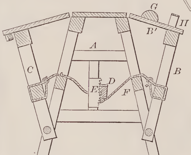
72674—O. & C. Perry— Sheep Shearing Table.
