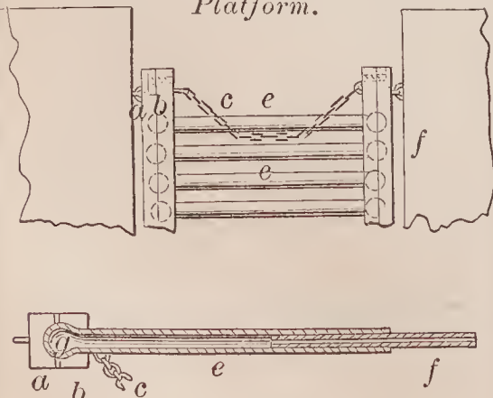
68543—C. R. Abbot—Safety Car Platform.
