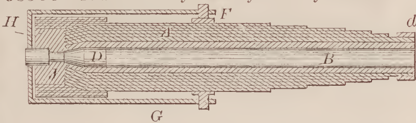
68509—T. N. Hornsby— Manufacture of Cannon.
