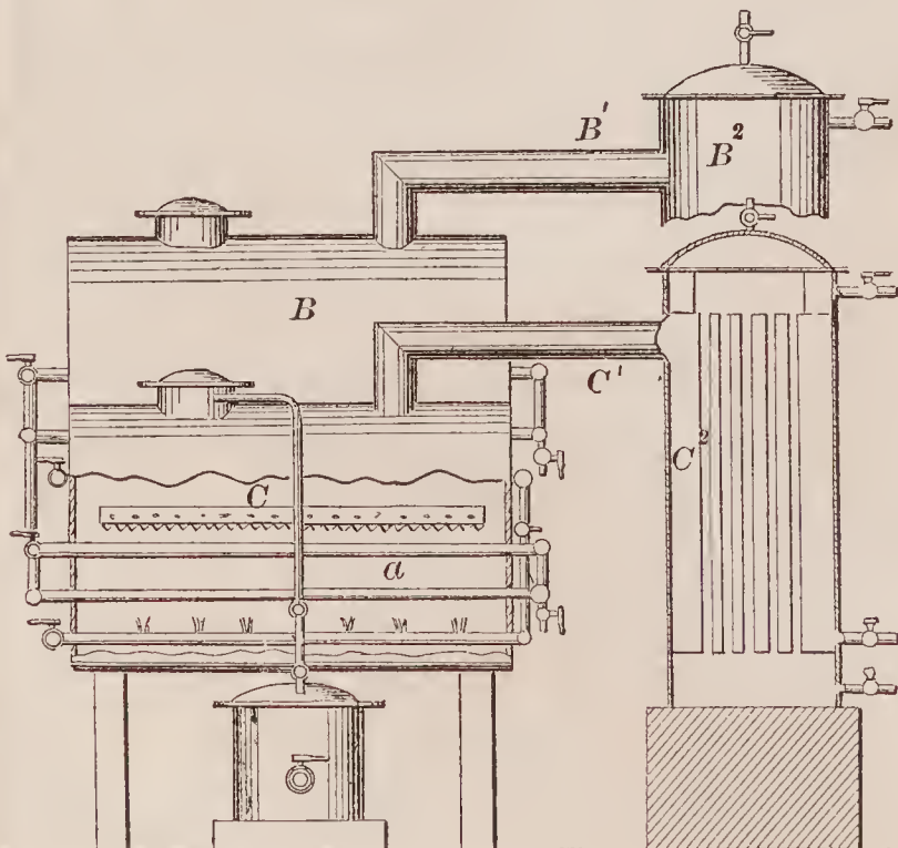
72126—H. W. C. Tweddle— Distilling Hydro-Carbon Oil.
