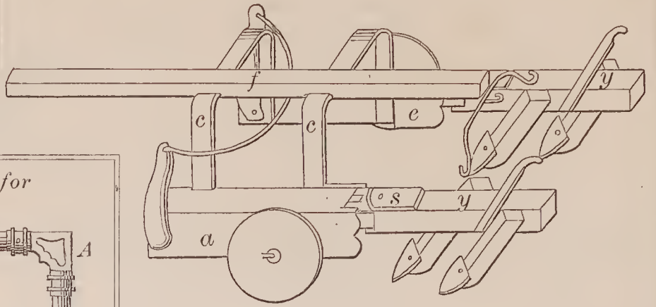
68104—E. Newlon— Cultivator.
