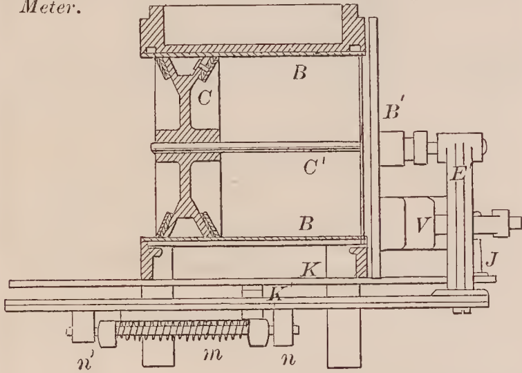
68746—Horton & Hawkins— Liquid and Fluid Meter.
