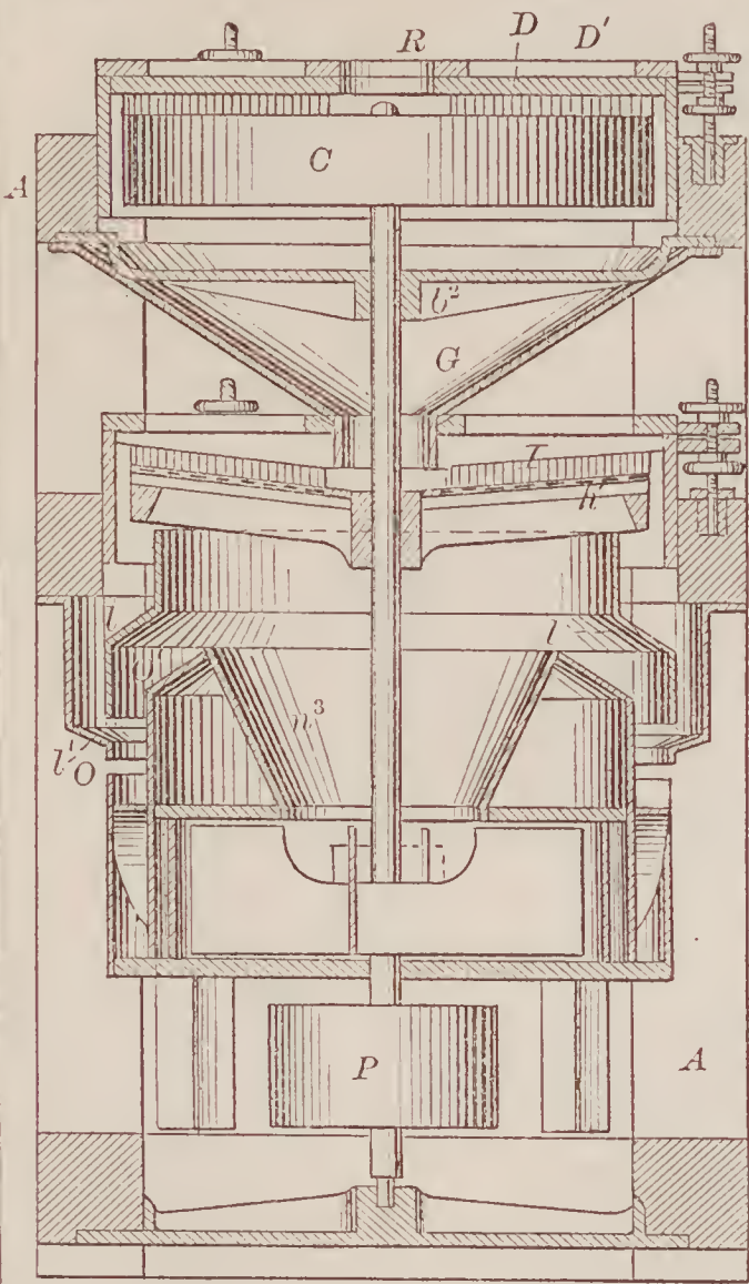
67423—P. T. Elting—Smut Machine.
