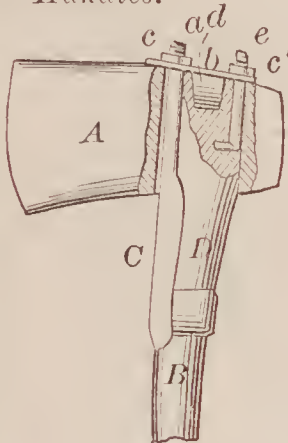
70284—J. Stewart—Attaching Axes to Handles.
