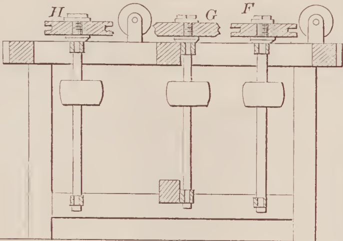
71609—H. W. Harper—For Dressing Slate Frames.
