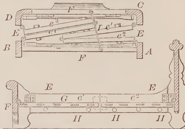
68023—B. F. Woodside—Bedstead.
