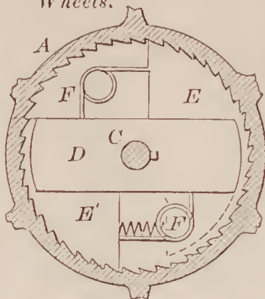
70371—W. W. Smith—Ratchet for Driving Wheels.
