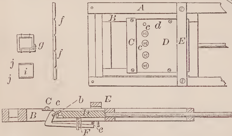
68173—H. V. Davis—Seed Drill.
