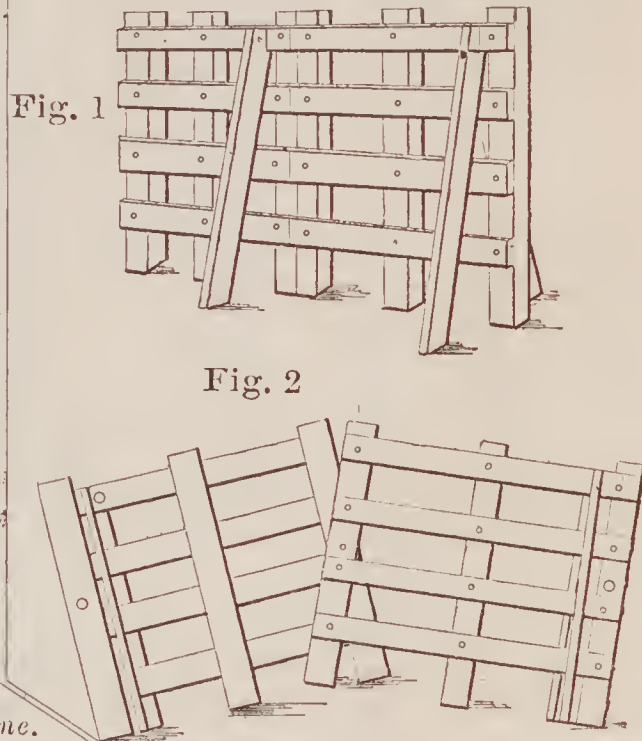
67564—S. Miles—Portable Fence.
