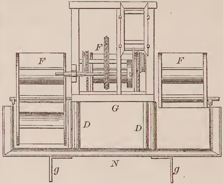
70419—C. Daniels— Floating Water Power.
