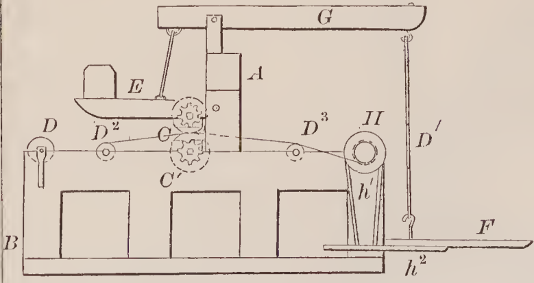
67198—A. Judson—Printing Press.
