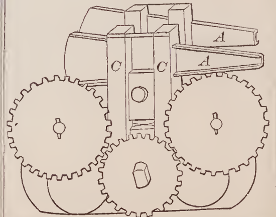
69916—G. Huntington— Bending Machine.
