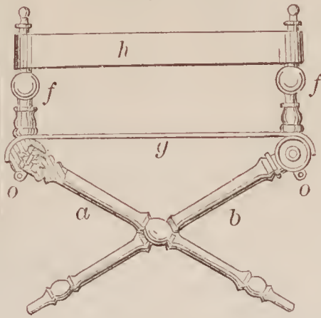
67759—P. J. Hardy— Folding Chair.
