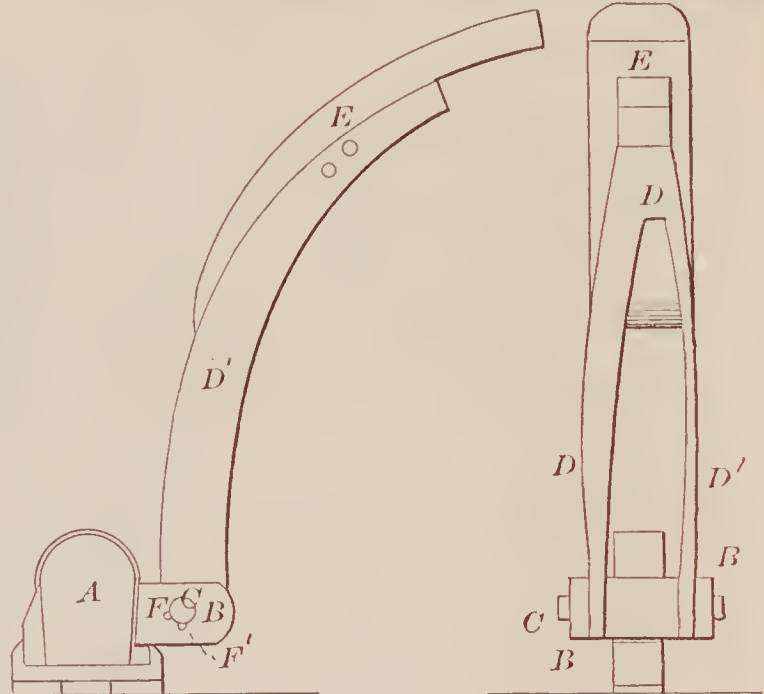
68277—G. C. Avery—Gang Plow.
