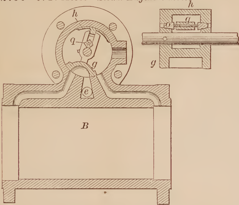
72750—J. F. Morse—Steam Engine Valve.
