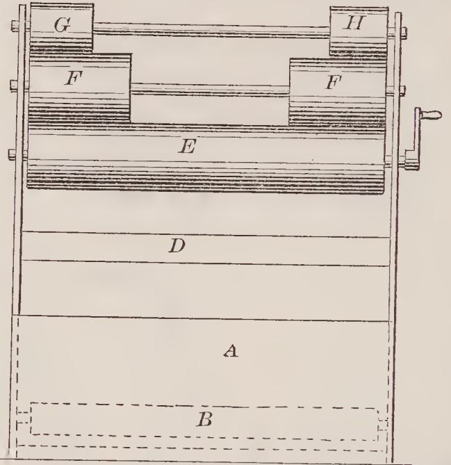
72647—J. Lee, Jr.—Cloth Washing Machine
