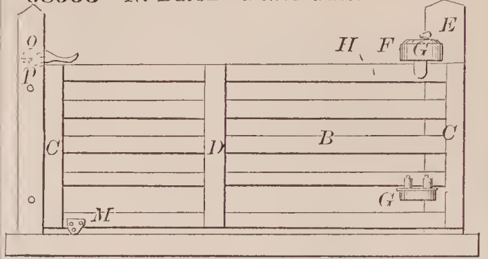
68553—N. Burch—Fence Gate.
