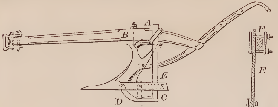
69117—Nichols & Clark—Plow.
