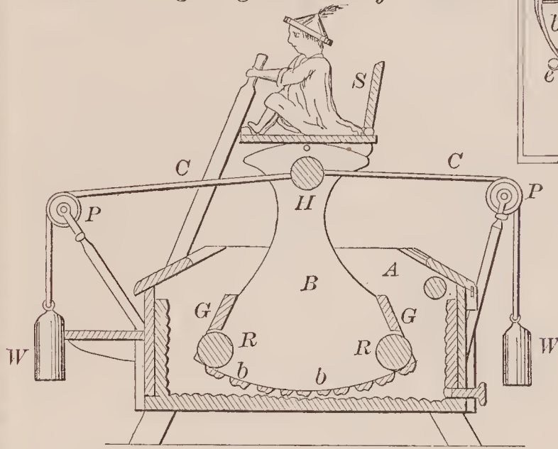
68626—J. Highbarger—Washing Machine.
