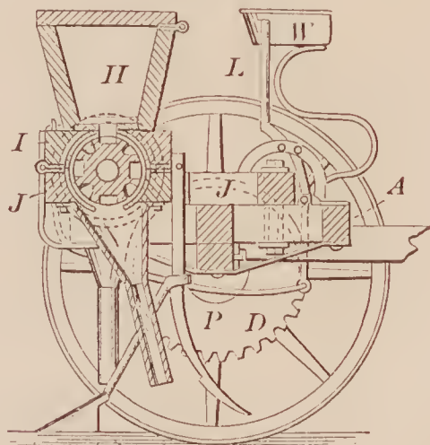
67152 —H. Zurbrick— Cultivator and Seed Sower.
