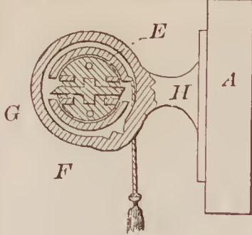
67465—L. A. Tripp— Window Shade Fixture.
