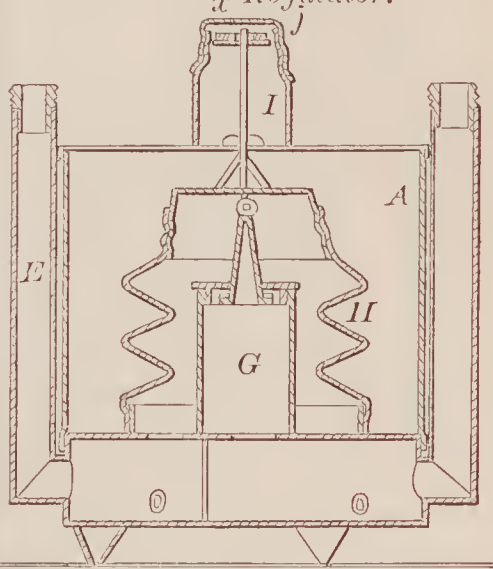
71757—J. B. Hoffman—Dry Gas Regulator.
