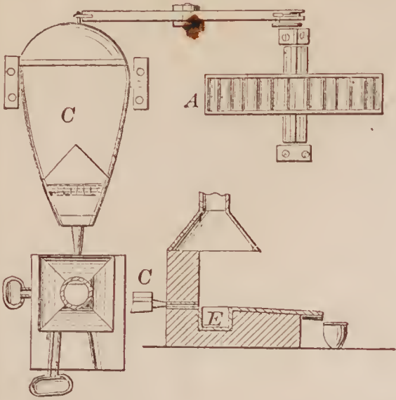
69025—A. H. Richardson—For Smelting Ores of Silver.
