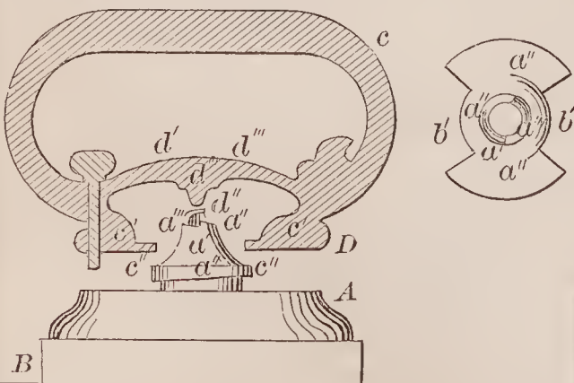
71974—Butterfield & Read—Sad Iron.
