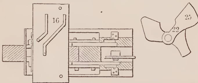
71028—J. D. Lynde—For Charging Soda Water.
