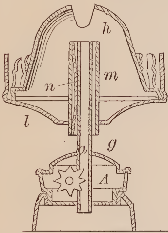
72418—S. W. Powell—Bone and Plaster Mill.
