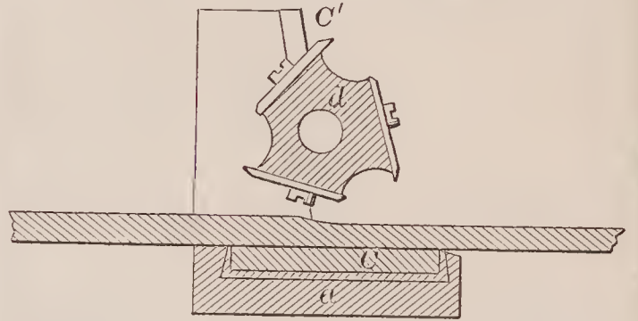
71818—J. Temple— Stitching Clamp.
