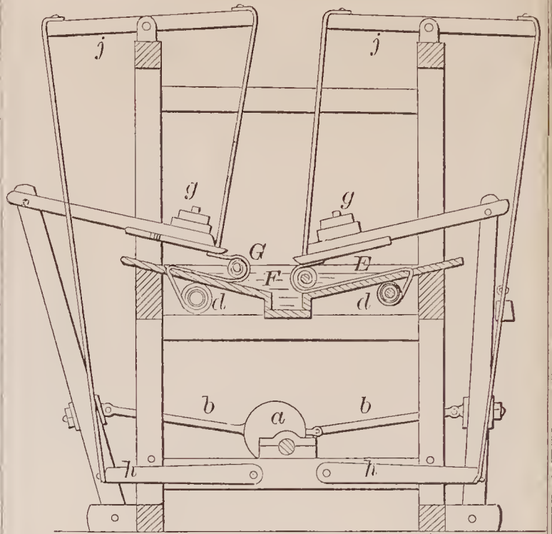
71516—Lodge & Platner—Felting Machine.
