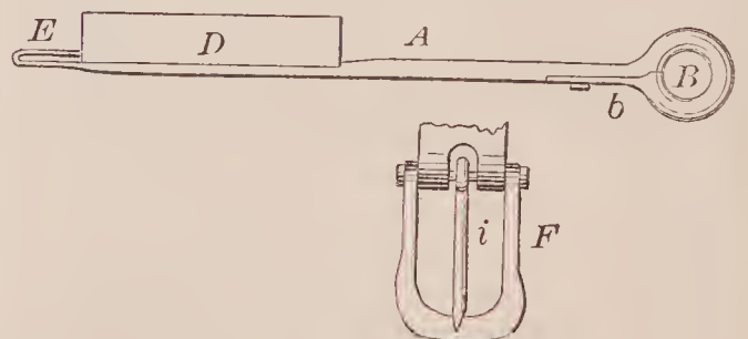
69418—D. F. Elmer— Index Gauge and Calipers.
