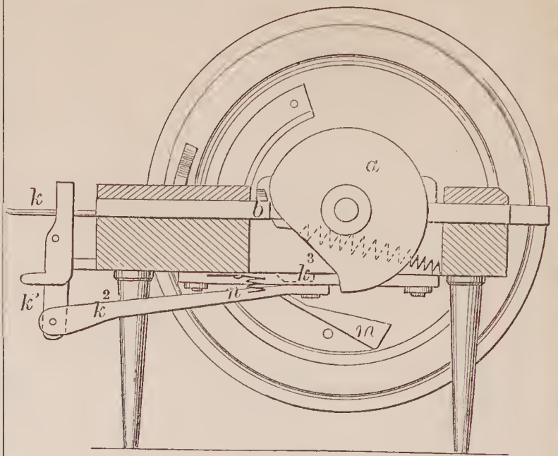
69481—C. H. Remington— Bullet Machine.
