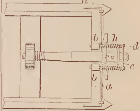
72441—C. P. Bachelder—Car Coupling.
