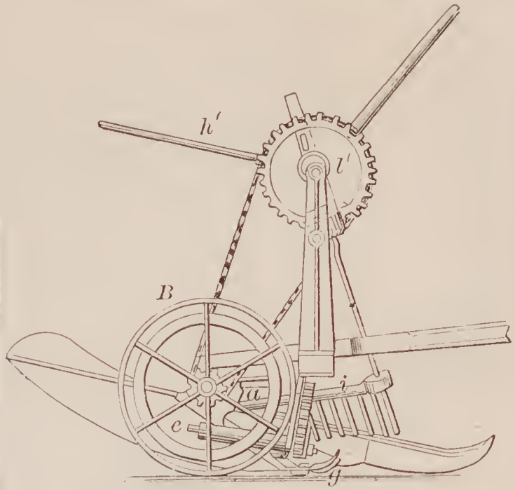
71175—Howard & Bousfield—Harvester.
