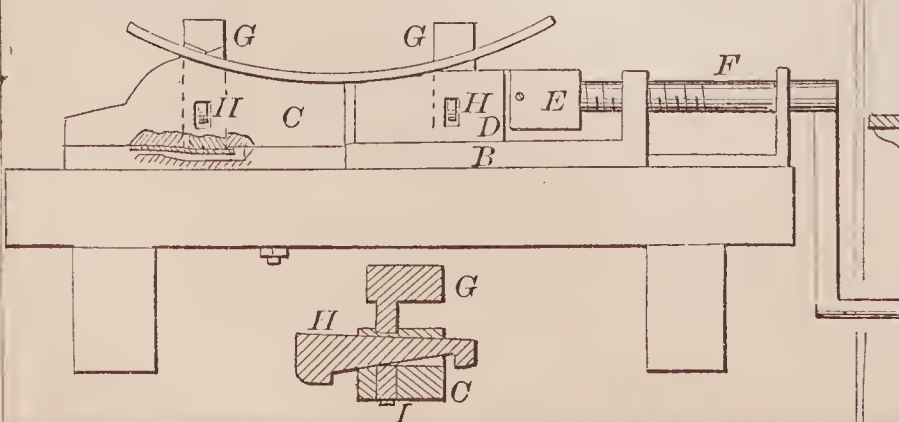
70854—J. B. & M. R. Jackson— For Shrinking Tires.
