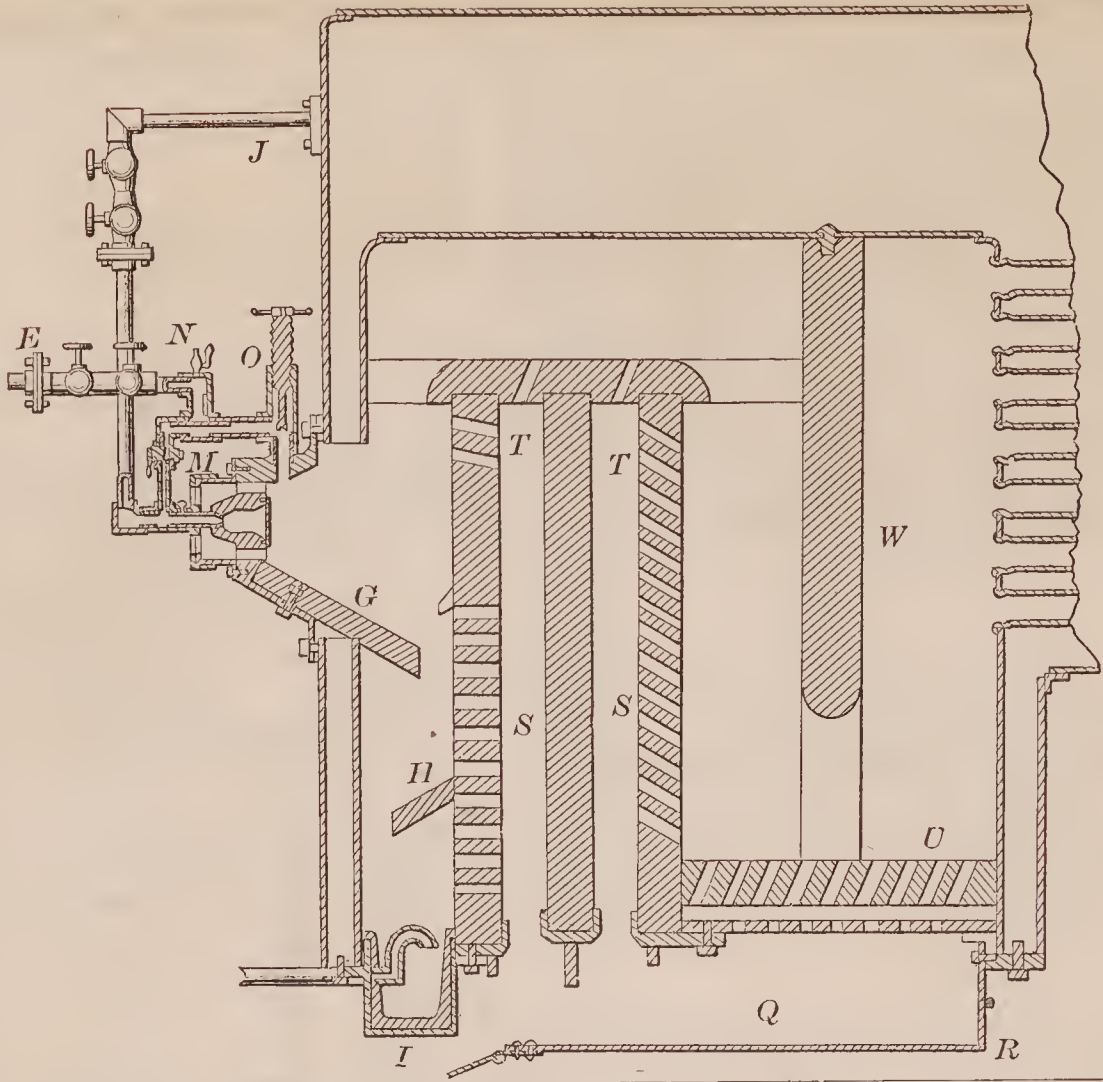
68708—Cook & Bassett—For Vaporizing and Decomposing Hydro-Carbon Liquids.
