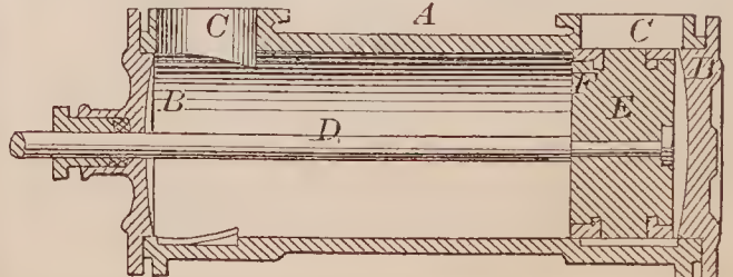
68747—S. W. Hudson— Steam Engine.
