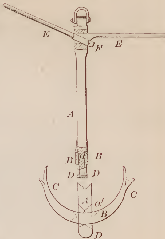
70498—Armstrong & Browne— Anchor.
