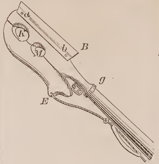
69310—J. C. Brown—Cane Stripper.
