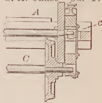
70696—S. A. Chase—Car Truck.
