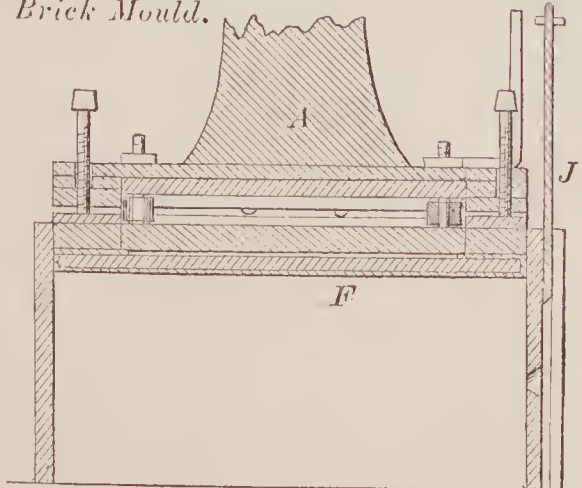
69909—Franklin, McIntire & Whitely—Brick Mould.
