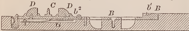
70568—N. Hopkins—Register Point for Printing Presses.
