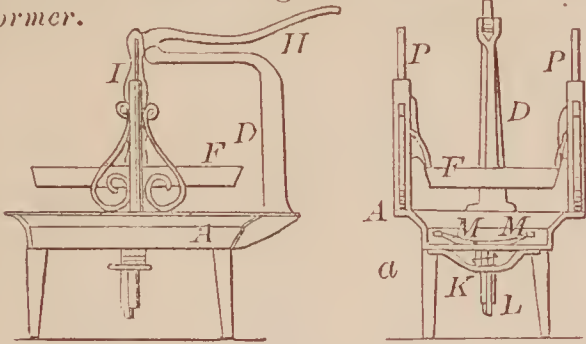
68964—H. O. Demarest—Boiler Feeder.
