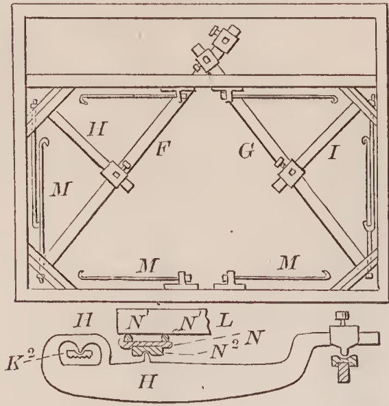
67871—W. P. Goolman—Platform Scale.
