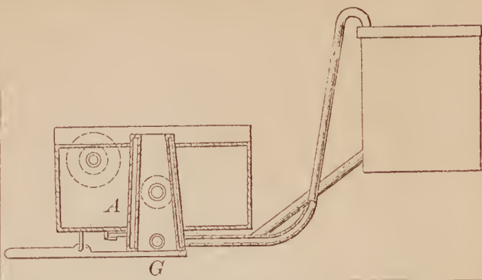
68940—J. F. Boynton— Fire Extinguisher.
