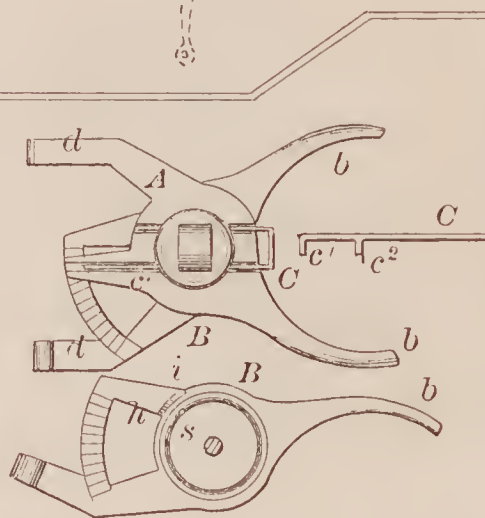
68197—W. L. Hopper—For Catching Animals.
