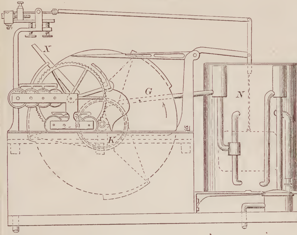
69714—Siemens & Halske—Spirit Meter.
