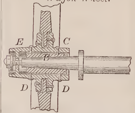
68017—S. B. Welton—Wagon Wheel.
