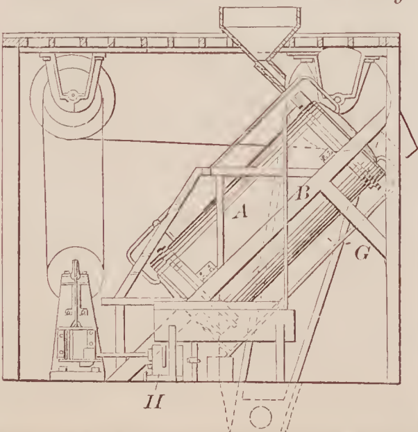
71981—G. Clark—Vacuum Grain Dryer.
