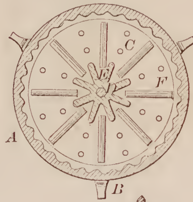
72328—Reneky & Keiss—Washing Machine.
