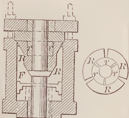
71664—C. M. Templeton— Stuffing-Box Packing.
