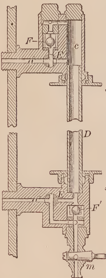
72793—N. H. Bundy—Boiler Water Gauge.
