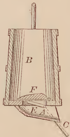
72725—J. Daykin—Water Drawer.
