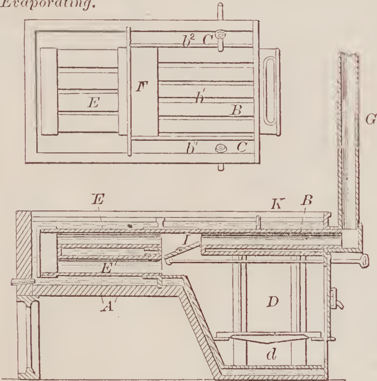
67742—Farquhar & Doan—For Heating and Evaporating.
