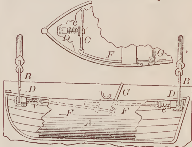
67547—L. Hover—Boat Detaching Tackle.
