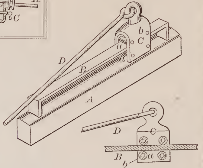
67638—D. H. Dotterer— Axle Box and Hanger.
