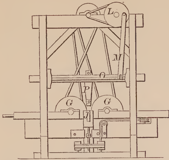
72953—D. Whisler—Ditching Machine.
