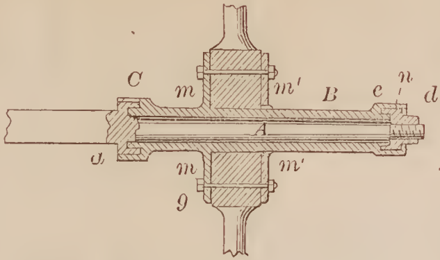
68813—J. B. Walker—Flexible Rammer for Turret Guns.
