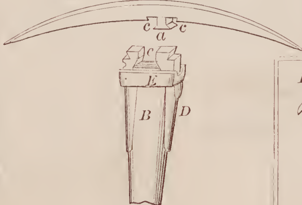
72245—J. P. Walsh—Attaching Picks to Handles.
