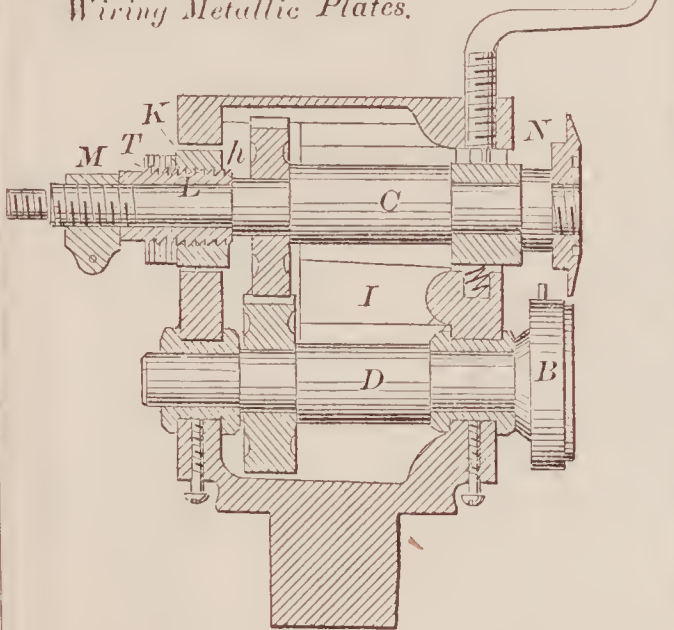
70917—O. W. Stow— For Flanging and Wiring Metallic Plates.
