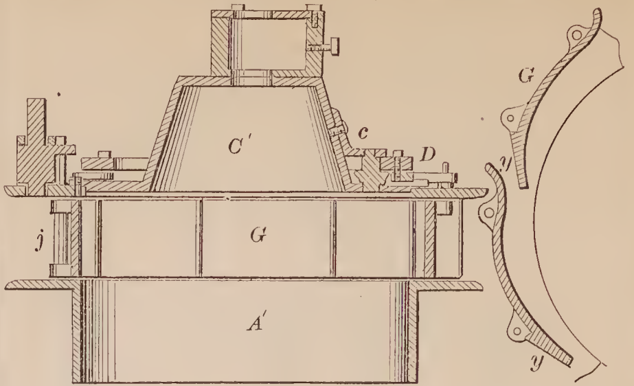
72450—N. F. Burnham—Guide for Water Wheels.
