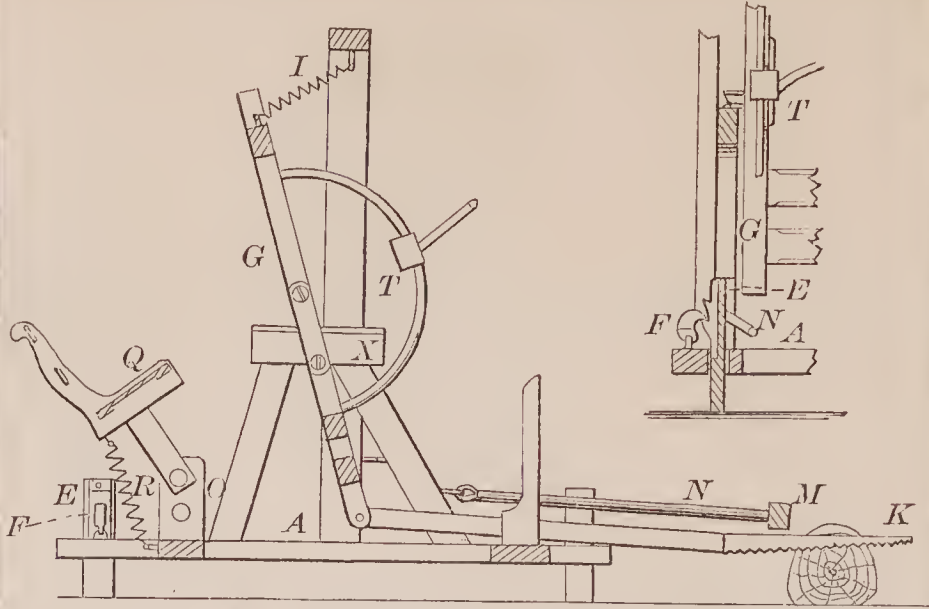
68517—G. C. Lathrop—Sawing Machine.
