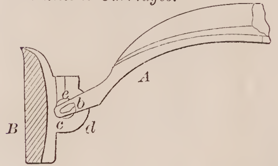
71078—W. Starkey—Attaching Thills to Carriages.
