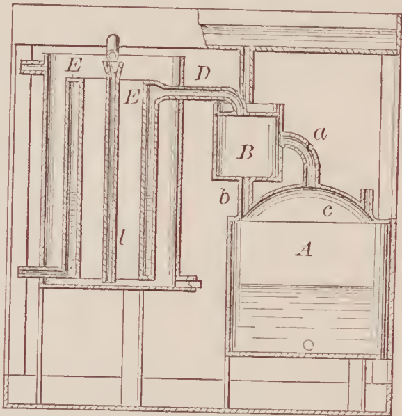
71744—T. Grundmann— Distilling Apparatus.
