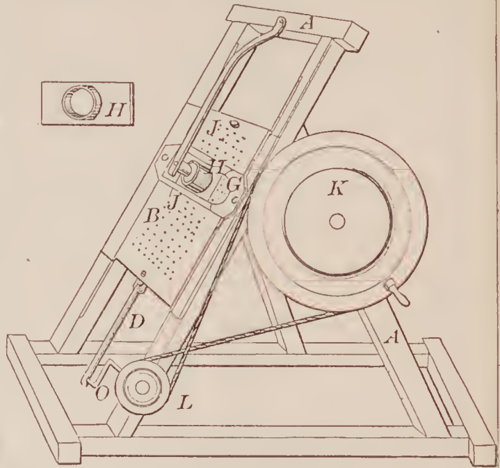
69150—C. Worden— Nutmeg Grater.
