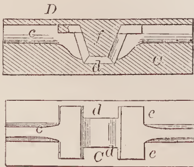
69827—E. Mecker—Carriage Clip.
