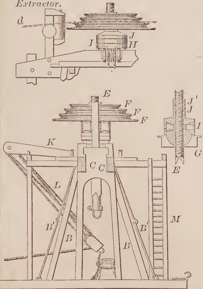
69209—Hazen & Hitchcock—Stump Extractor.
