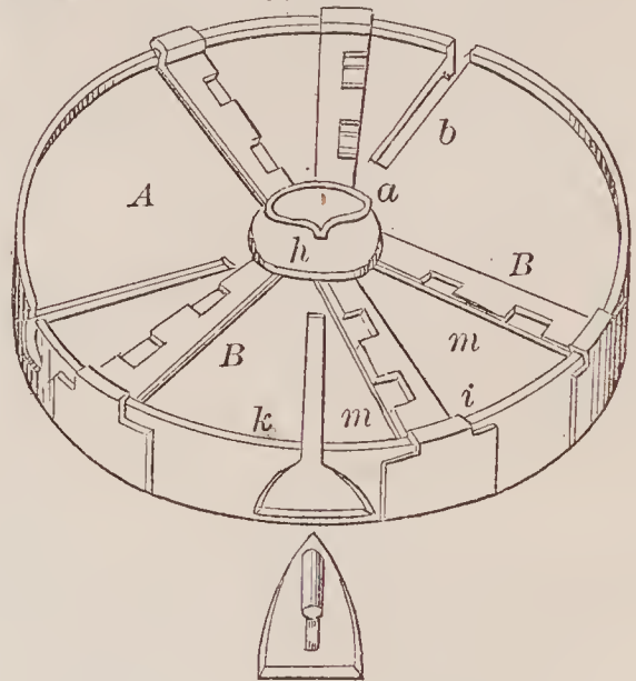
67381—D. Utley, 2d— Sad Iron Heater.
