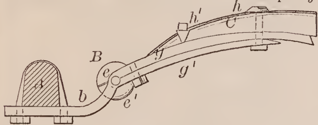
68758—L. Legran— Artificial Leg.
