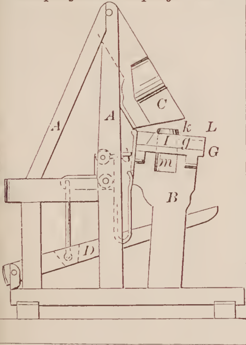
70561—J. H. Hartsuff— Curb for Water Wheels.
