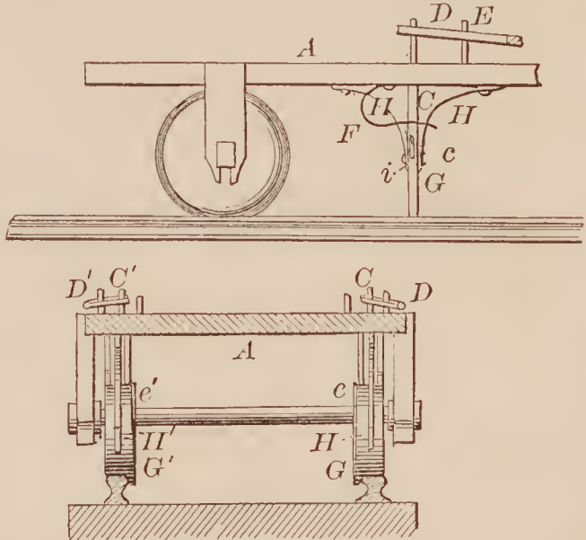
71704—Cogan & Russell—Track Clearer.
