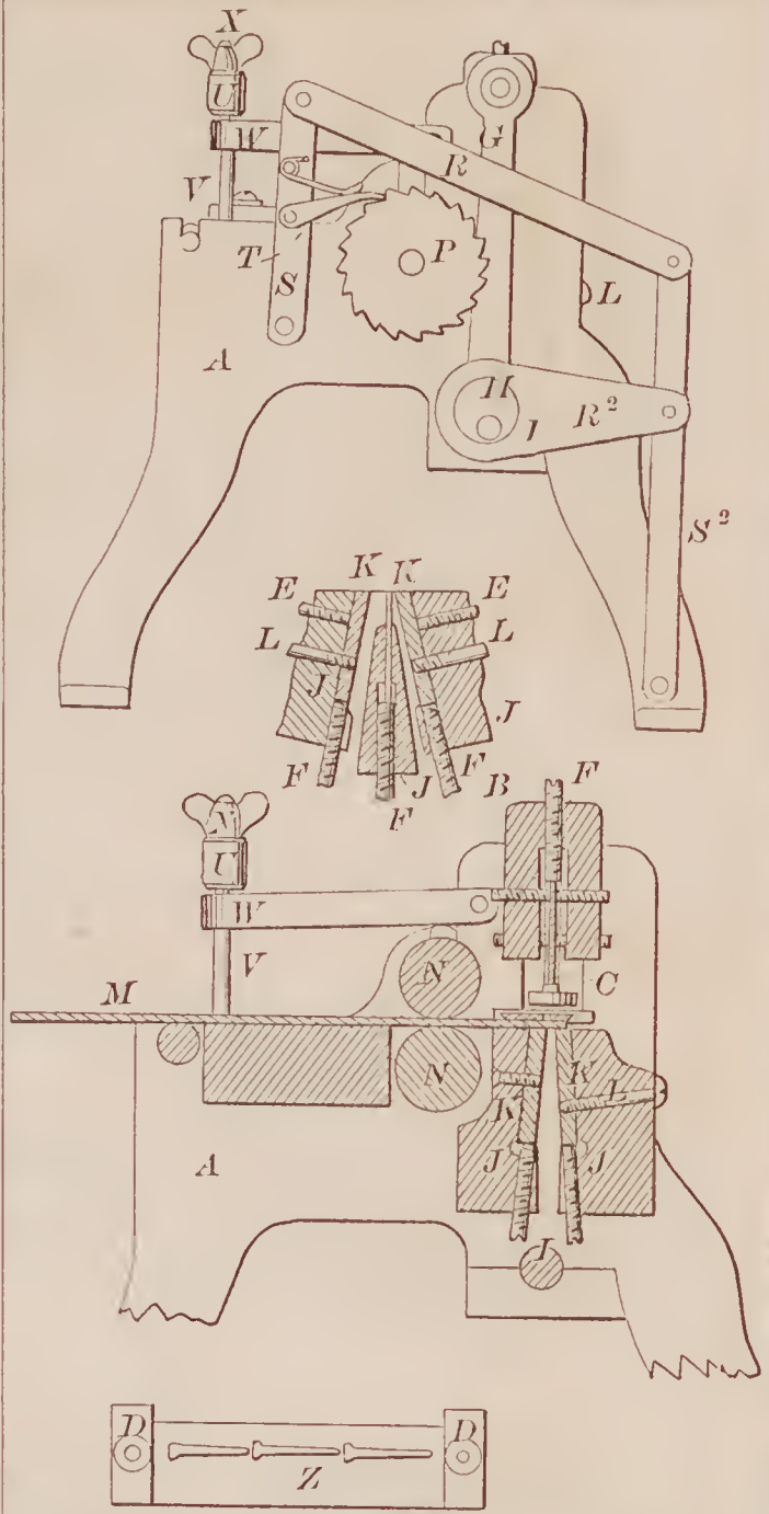
72230—B. Robinson—For Making Nails.
