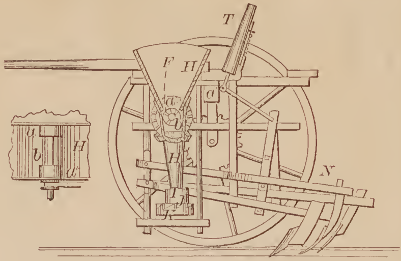
72799—C. Churchill— Cultivator and Seeding Machine.
