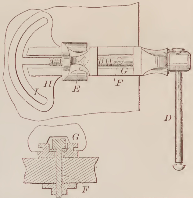
67686—Teale & Brassington—Steering Apparatus.
