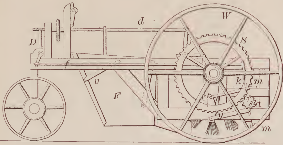
71894—McConnell & Pringle—Street Sweeper.
