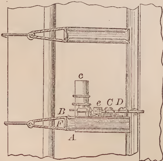
68857—C. A. Eaton—Burglar Alarm.
