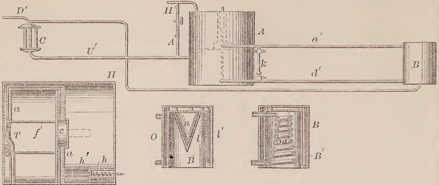
66777—Barker & Gilbert—For Carburetting Air and Gas
