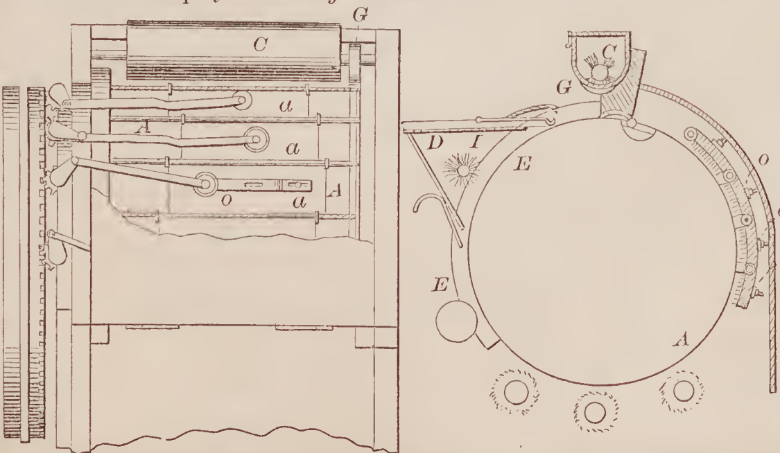
71085—J. F. Tapley—Bronzing Machine.
