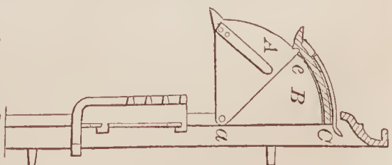
69982—W. T. Foster—Hood for Coal Grates and Fireplaces.
