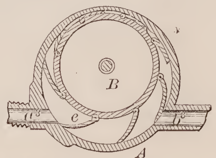
67928—J. D. Summer— Water Meter.
