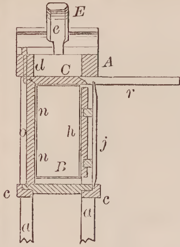
68185—H. G. Hall—Ring for Spinning.
