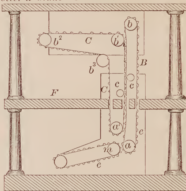
68390—W. J. Sloan—Threshing Machine.
