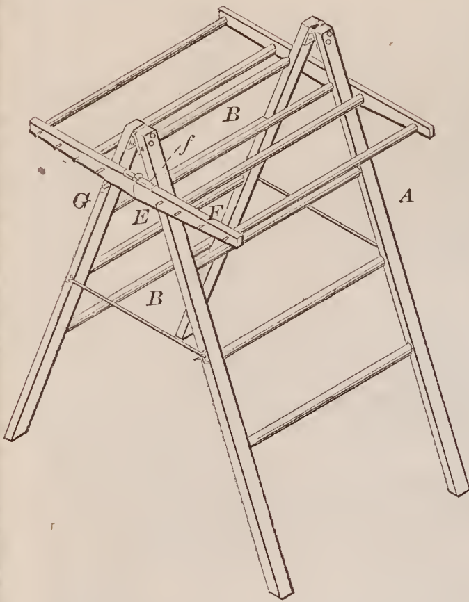
67567—J. J. Newman— Clothes Dryer.
