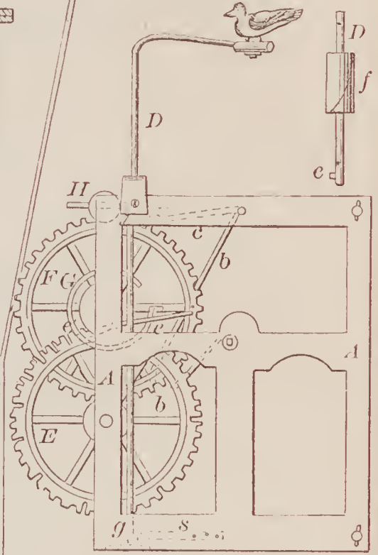
69561—C. K. Giles— Cuckoo Clock.
