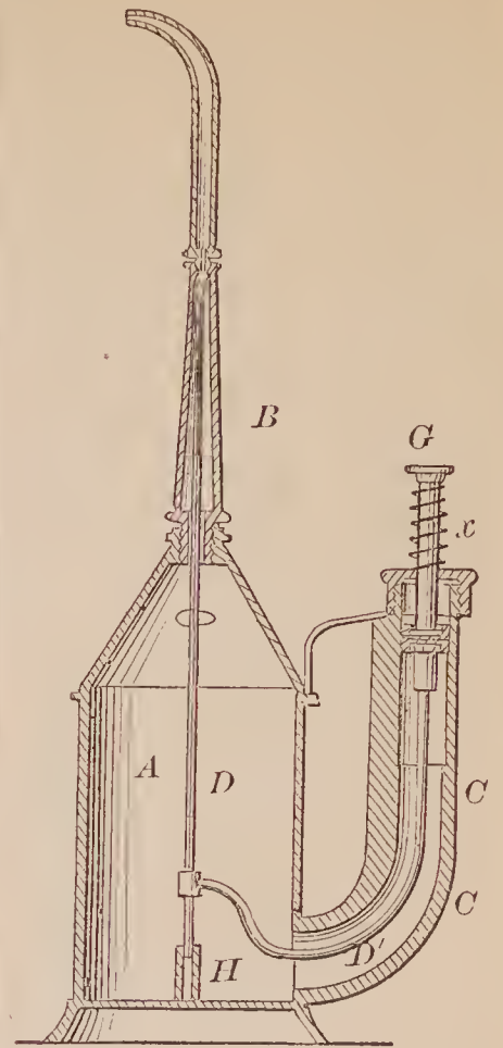
72384—J. B. Gayle—Oil Can.
