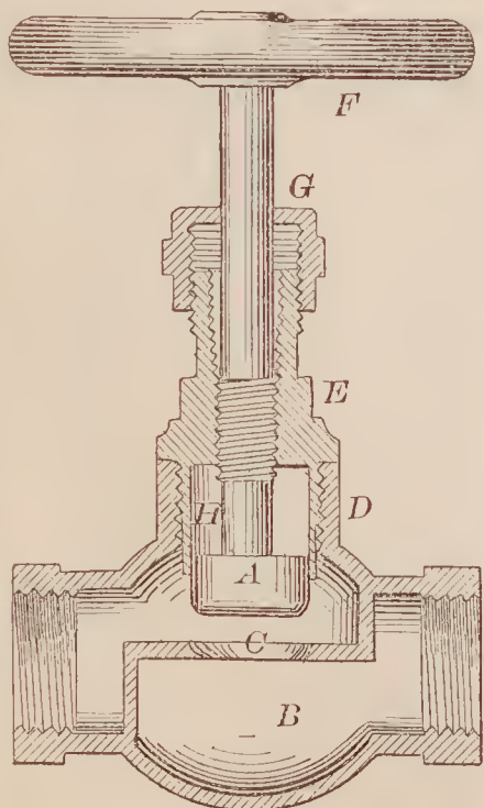
66757—J. H. Webster—Steam Globe Valve.
