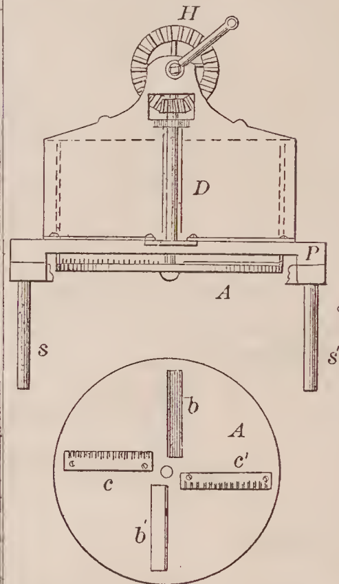
69232—J. McConnell—Steam Engine Valve.
