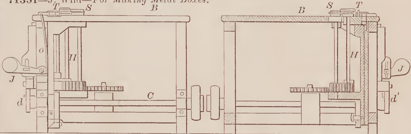
71352—L. Wilson—Bed Bottom.
