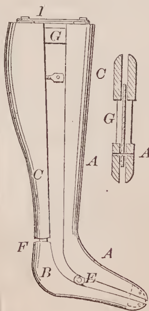
69293—S. J. Wright—Stretchers for Hosiery.
