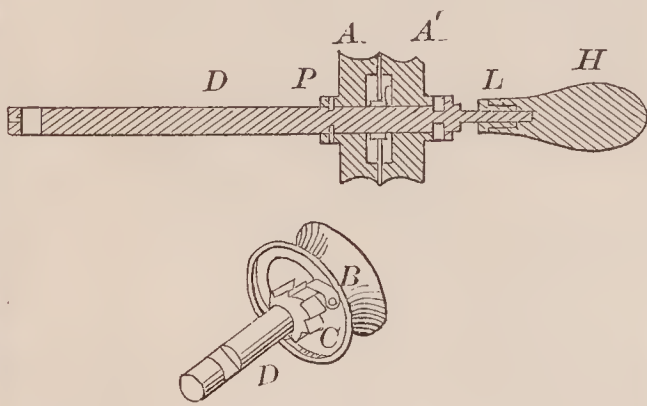
68071—D. F. Hartford—Bow Drill Stock.
