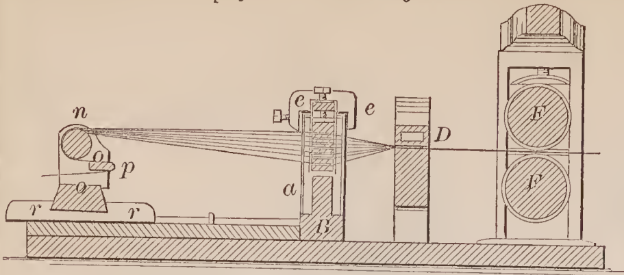
70706—H. Dunphy—Cloth Folding Machine.
