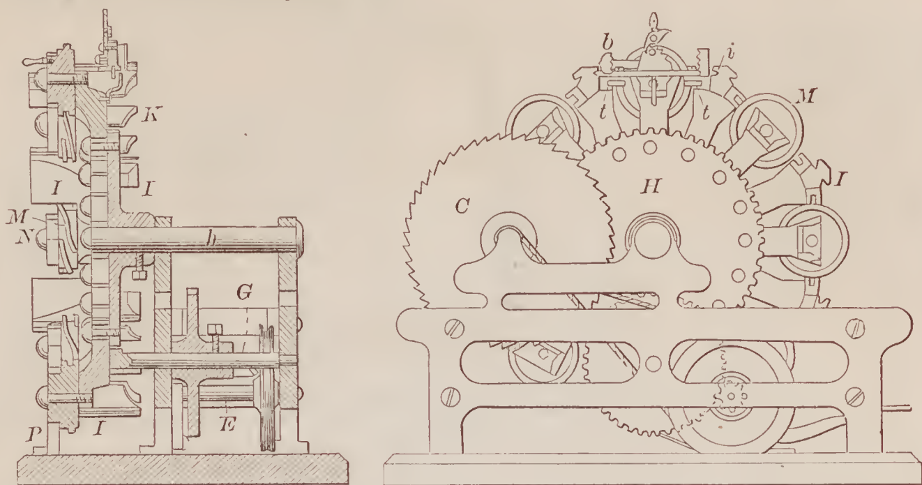
67724—E. B. Cook— Shingle Machine.
