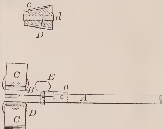
71545—A. Smith—For Reducing Cracklings.
