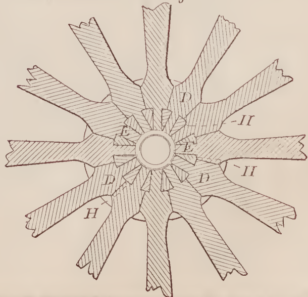
71774—J. Maris—Wagon Wheel.
