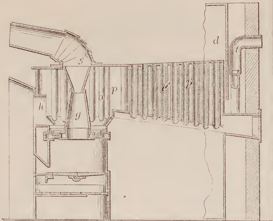
71244—J. M. Thatcher— Air Heating Furnace.
