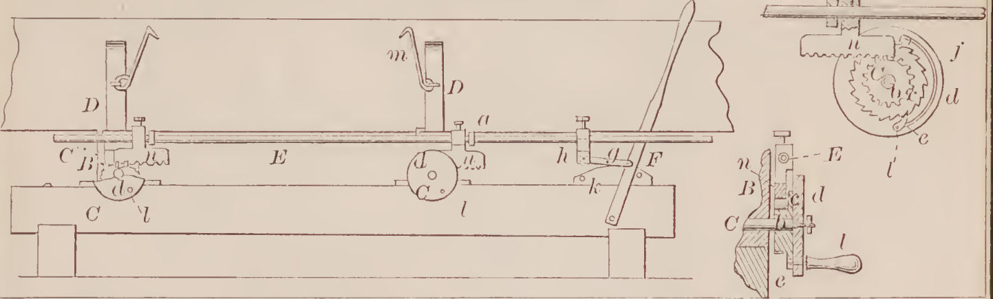
70951—I. S. & C. N. Brown— For Grinding Saw Teeth.
