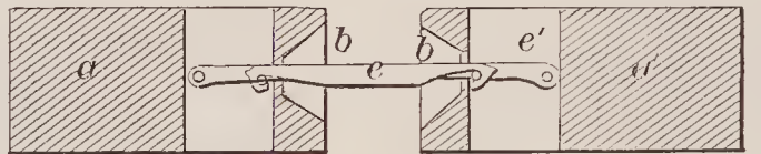
72664—W. J. Millar—Car Coupling.
