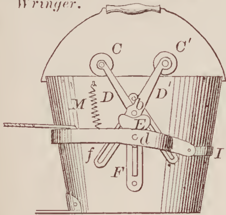
69942—R. W. Soper—Mop Wringer.
