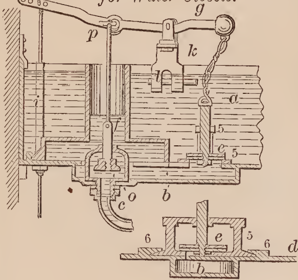
72810—H. H. Craigie—Water Supply for Water Closets.
