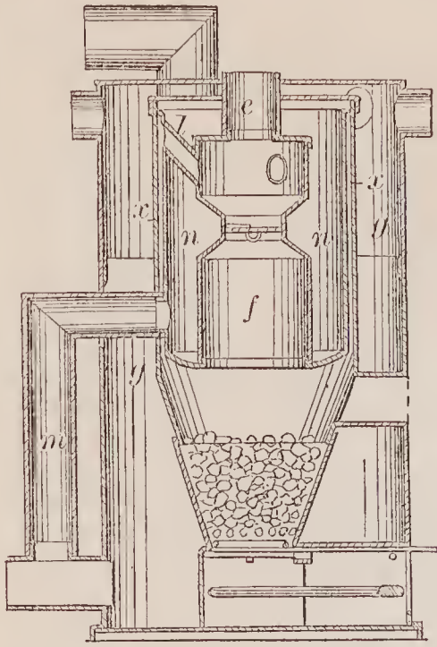
69821—J. F. Latimer—For Accumulating Power.
