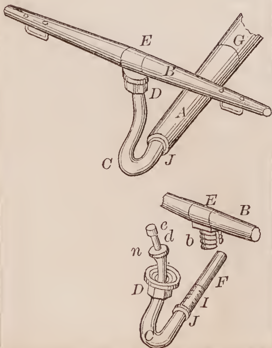
71312—H. J. Lamm— Neck Yoke Fastening.
