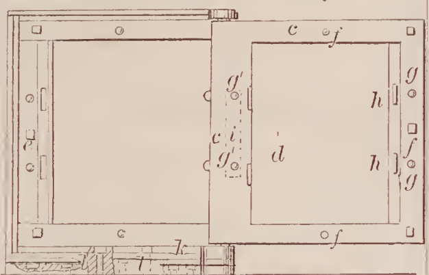
72283—W. Gardner—Iron Safe.
