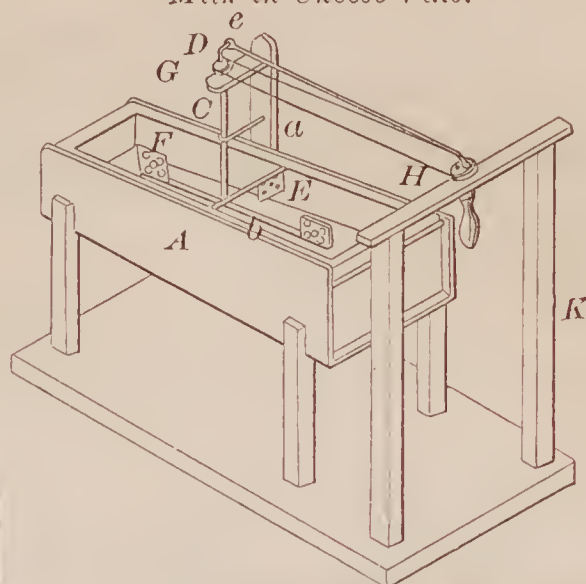
68198—J. C. House—For Agitation of Milk in Cheese Vats.
