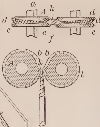
71360—G. B. Brayton—Dic for Threading Screws.
