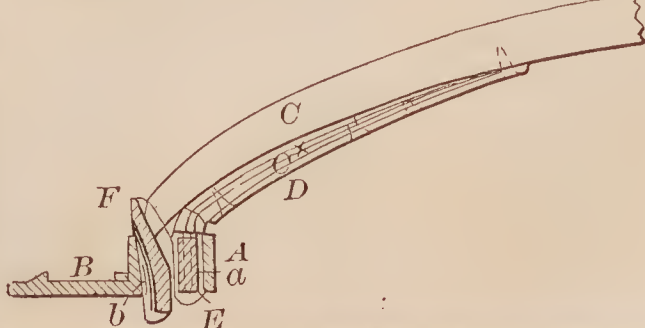
71705—J. P. Collins—Thill Coupling.
