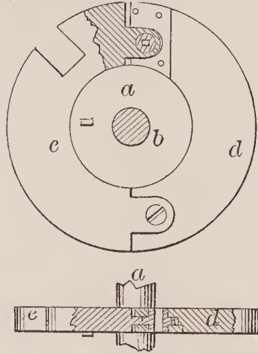
71640—J. H. Porter— Tumbler for Permutation Locks.
