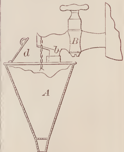
67869—J. Gatley—Cooler for Liquors on Draught.
