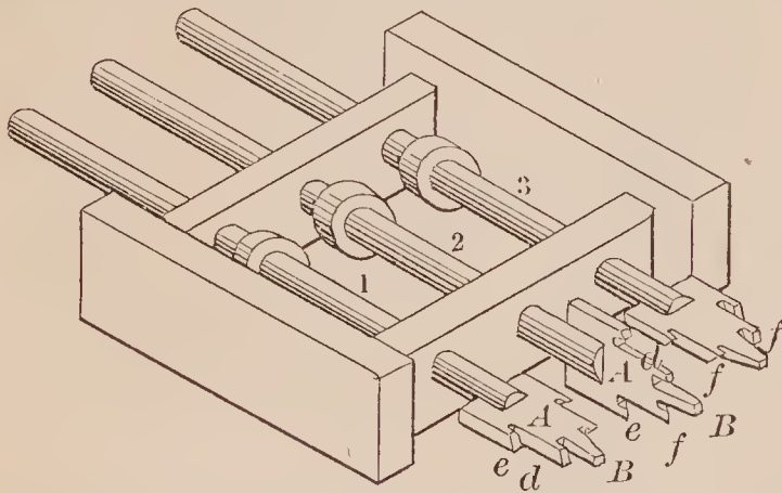
72389—S. Gissinger—Coal Boring Bit.
