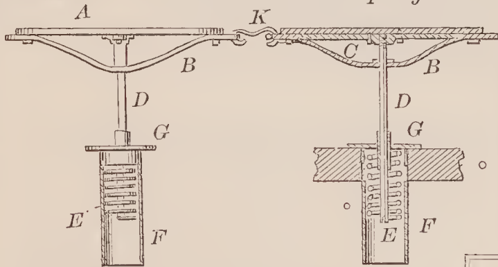
66849—J. Johnson—Bed Bottom Spring.
