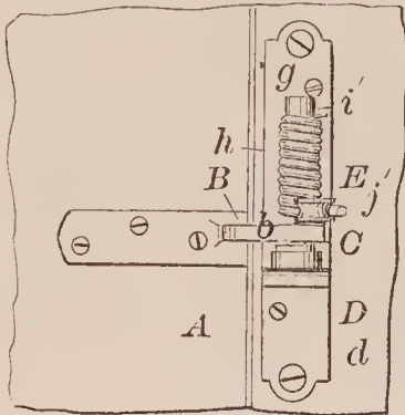
66927—A. Wiswall— Door Spring and Hinge.
