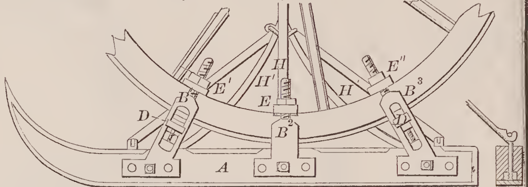
71576—F. T. L. Boyle—Runner for Wheeled Vehicles
