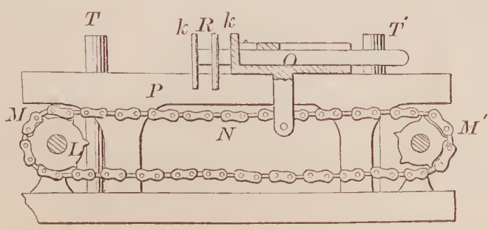
70289—C. Tholl—Carriage Shaft Connection.
