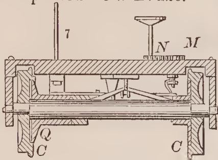
70911—C. Spofford—Car Brake.
