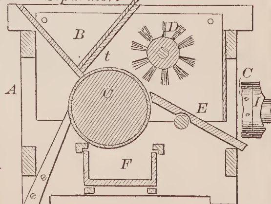
66872—J. W. Neal— Cockle and Garlic Separator.
