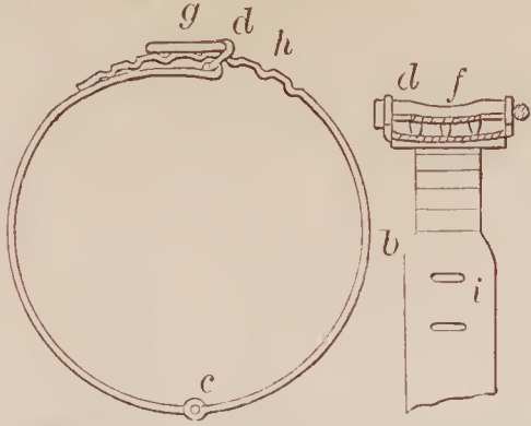
70239—G. D. Melotte—Clutch for Hay Forks.
