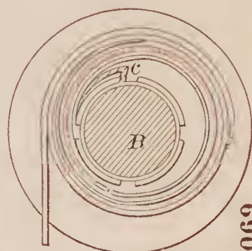
69044—J. W. Taylor—Shaft Coupling.
