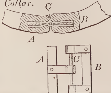
67201—D. Lincoln—Horse Collar.
