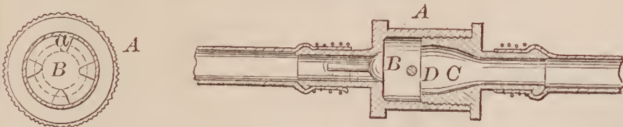
72508—N. Lawrence—Syringe Valve.
