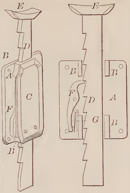
71821—W. T. Thornton—Seat Fastener.
