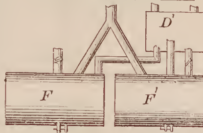
68425—S. V. Essiek—Knitting Machine.
