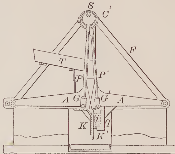
69656—Goodwin & Squire—For Crushing Rocks, Ores, &c.
