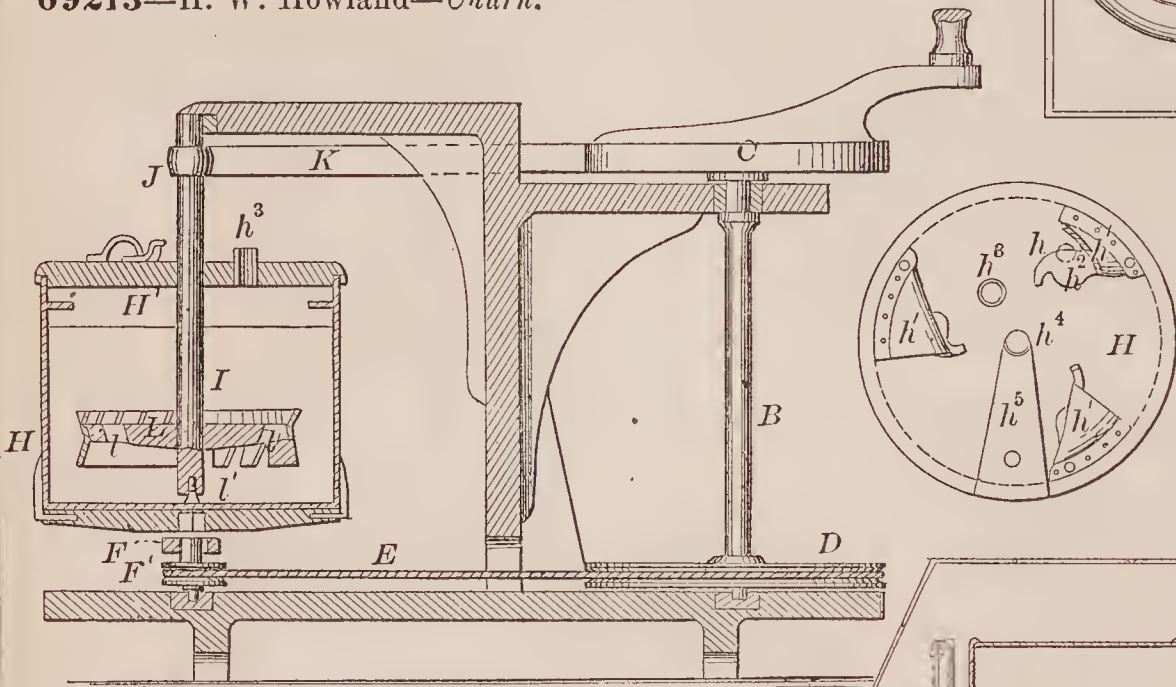
69213—H. W. Howland—Churn.
