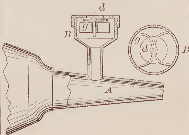
71866—C. C. Fornerook— Tuyere.
