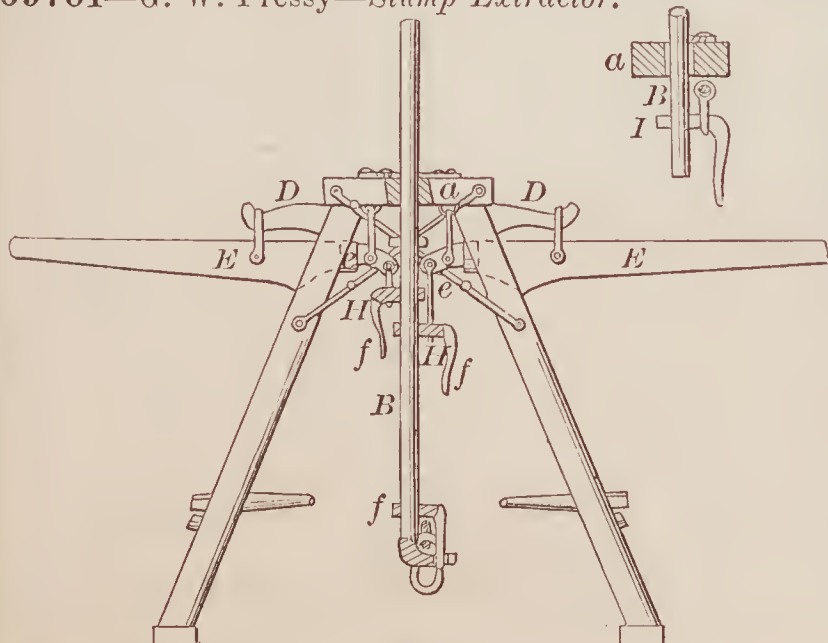
69701—G. W. Pressy—Stump Extractor.
