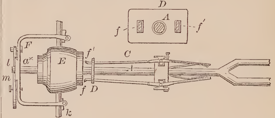
72887—D. J. Owen—For Boring Hubs.
