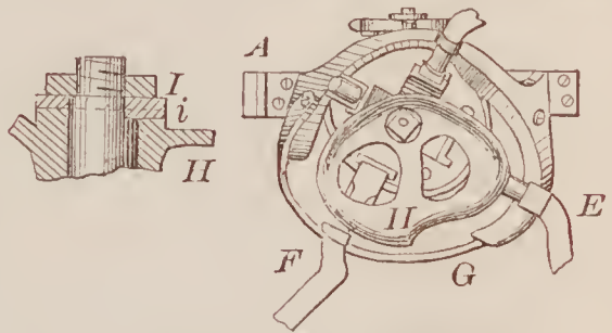
67851—J. A. Dodge—Harvester Rake.
