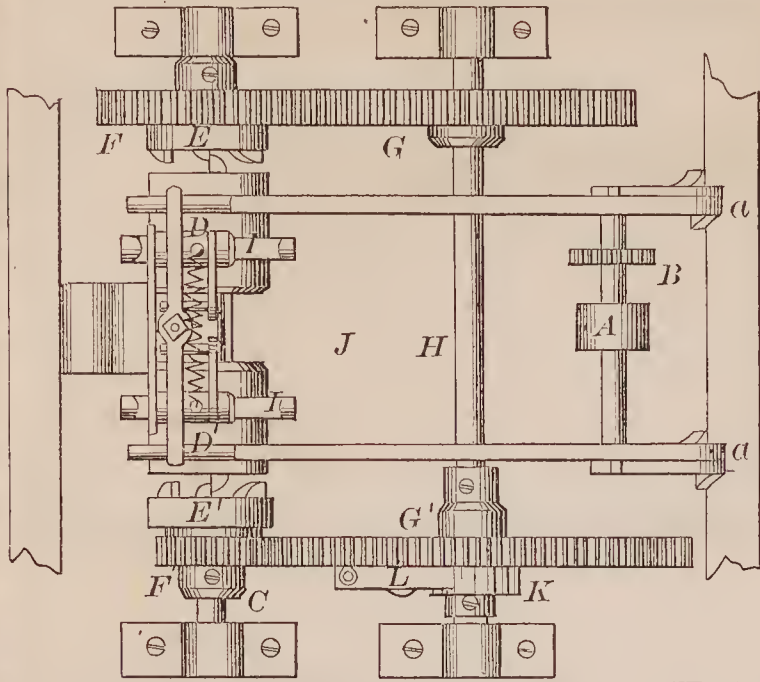
68746—Horton & Hawkins— Liquid and Fluid Meter.
