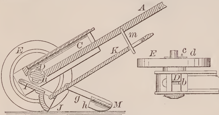
68050—H. V. Davis—Hand Seed Planter.
