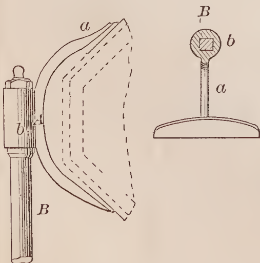
70422—M. De Voursney— Fastening for Coach Lamps.
