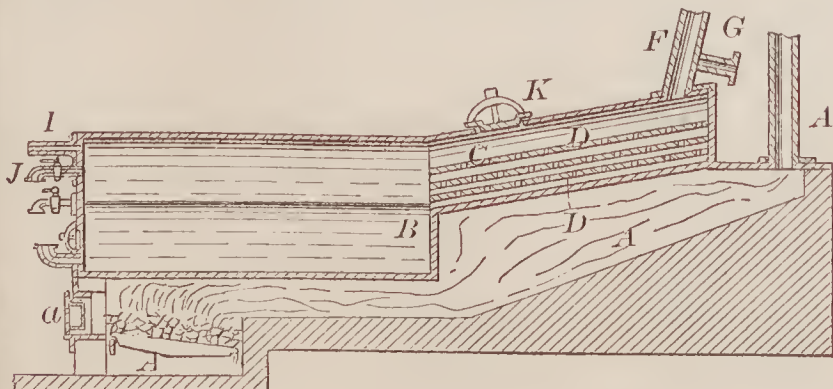
67988—E. G. Kelley—Petroleum Still.
