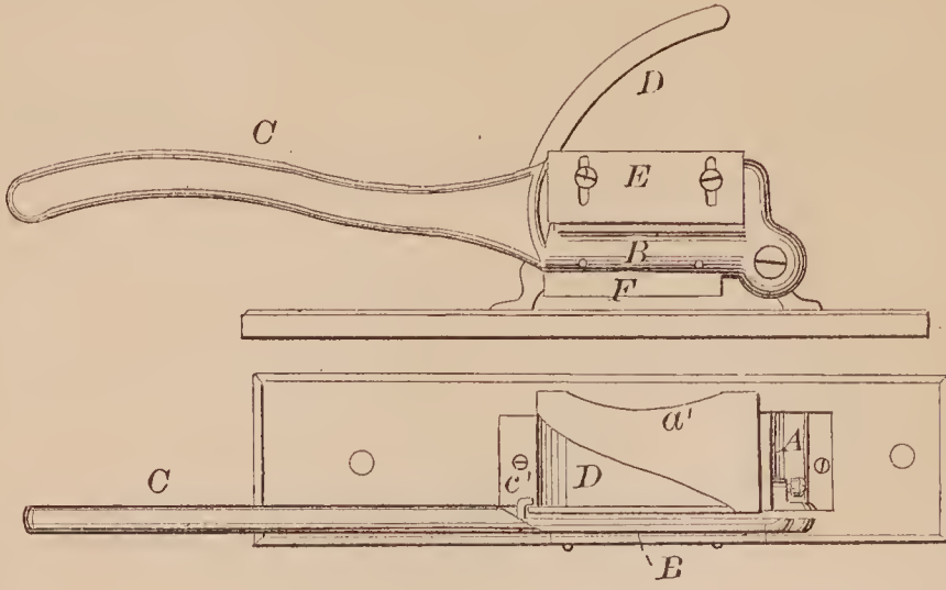
72762—C. Taft—Shingle Carriage.
