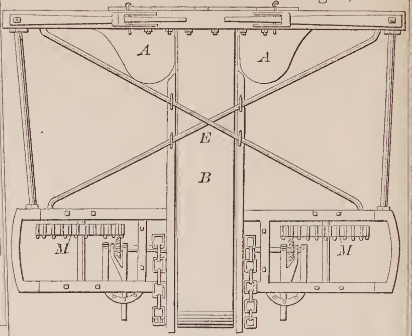
71747—T. C. Hammond— Grading and Excavating Machine. Fig. 1, I
