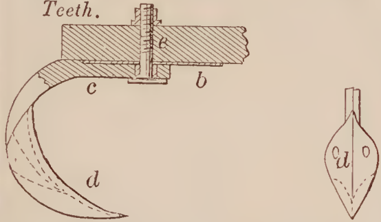
68443—D. W. Jacoby—Corn Planter.
