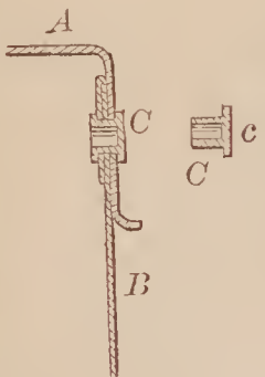
72948—Wemple & Richardson—Sash and Shutter Fastener.
