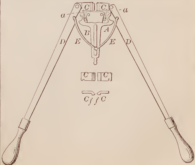
70563—J. E. Heath— Tool for Cutting Bolts.
