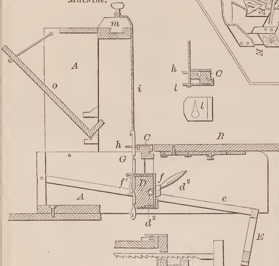
66899—F. Sims—Book Sewing Machine.
