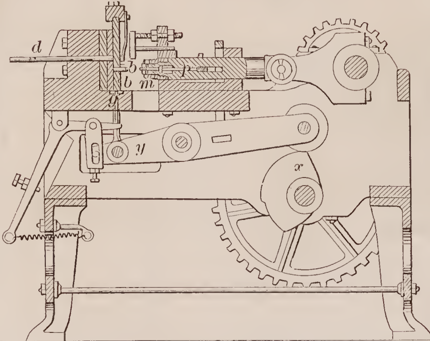
72137—P. V. Westfall—Brick Machine.
