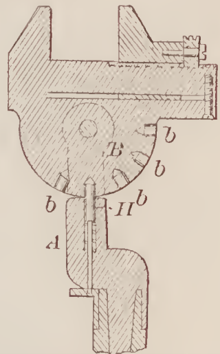
69910—J. P. Gates—Bridle Bit.
