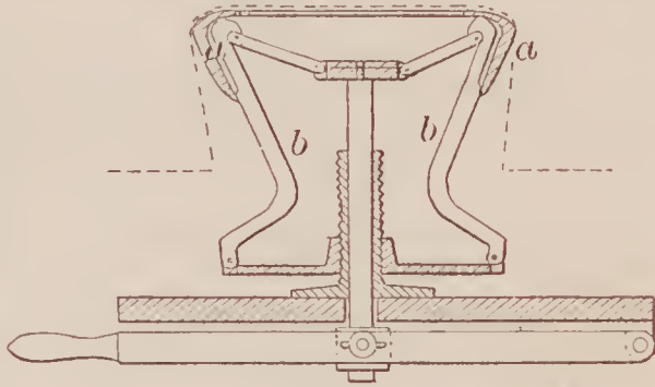
69371—J. Sheldon—Hat Blocking Machine.
