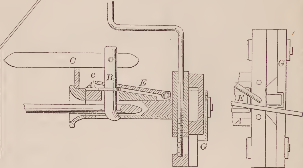
70776—P. Baker— Car Coupling.
