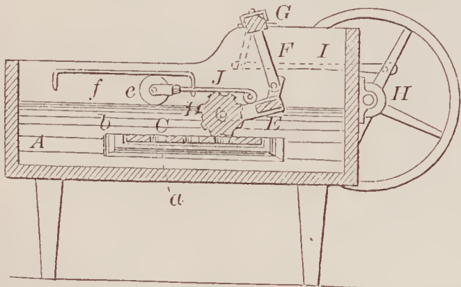
67275—J. C. Delavigne—Saw Mill.
