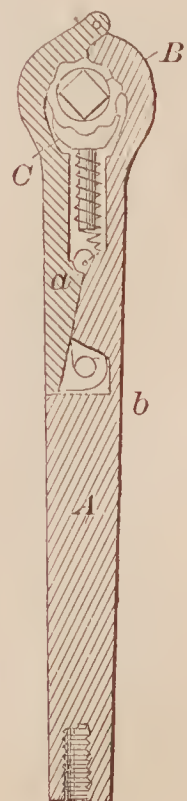
68780—R. Nickson— Carriage Joint.
