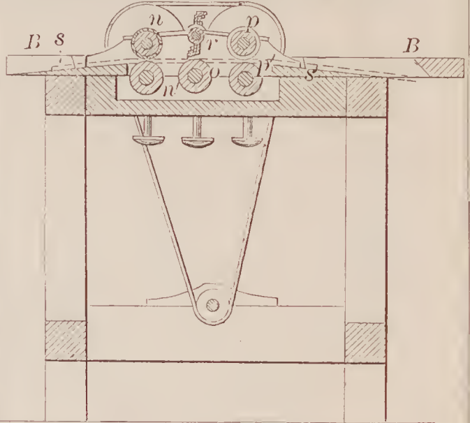
71277—F. O. Clark—Stave Machine.
