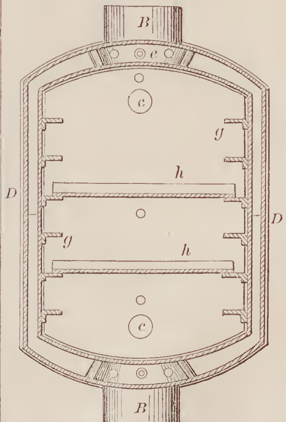
67172—G. Diffenderfer— Portable Oven for Drying Fruit.
