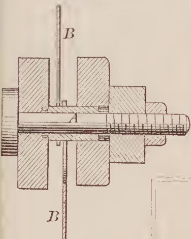
71455—W. H. Christie—Planing Machine.
