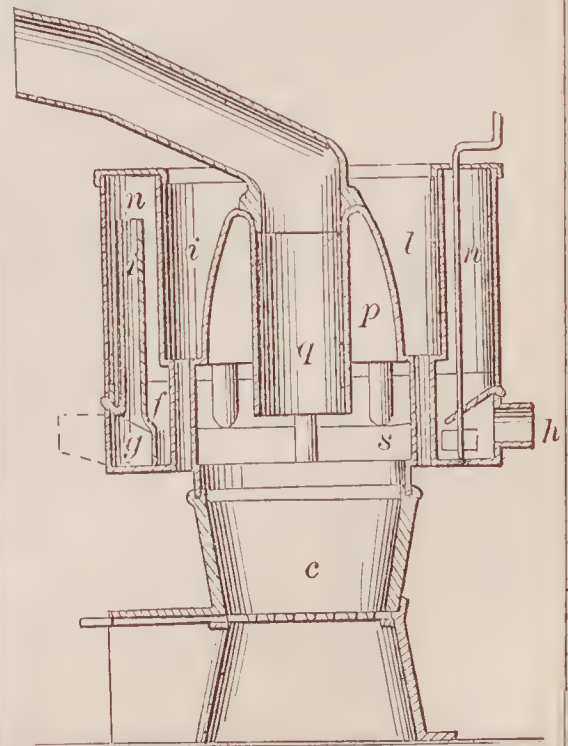
71176—M. C. Hull—Heating Stove.
