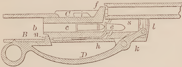
66751—E. L. Sturtevant—Magazine Fire Arm.
