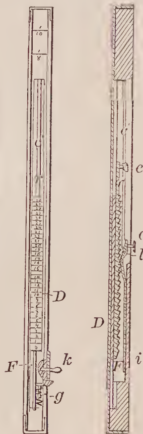
72210—Lupton & Talbot—Registering Yard Stick.
