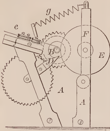
68516—S. B. Lane—For Making Button Rings.
