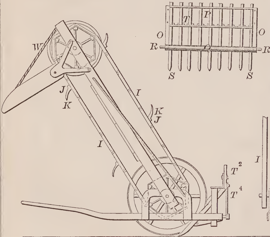
71764—H. Kewley—Hay Raker and Loader.
