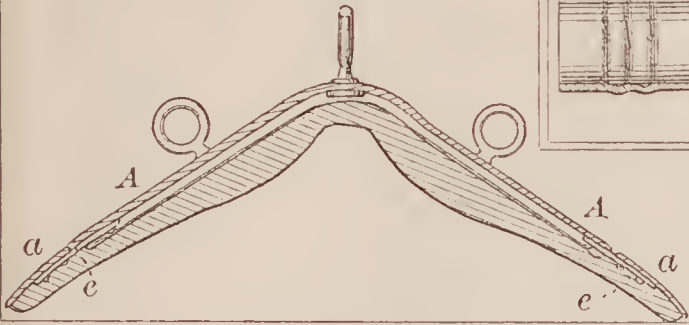
70633—Shaw & Dawson— Harness Pad Tree.
