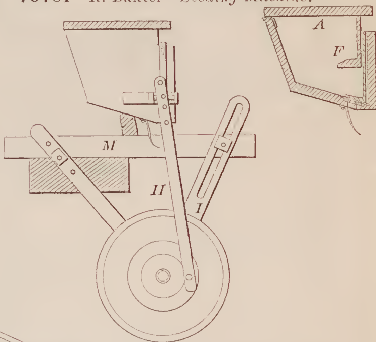
70781—R. Baxter—Seeding Machine.
