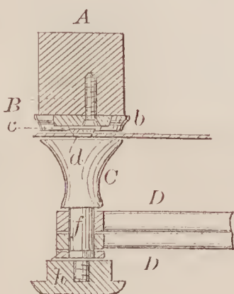
67968—W. Finn— Carriage Prop.
