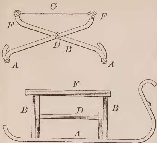
68534—J. Shaaber—Sled.
