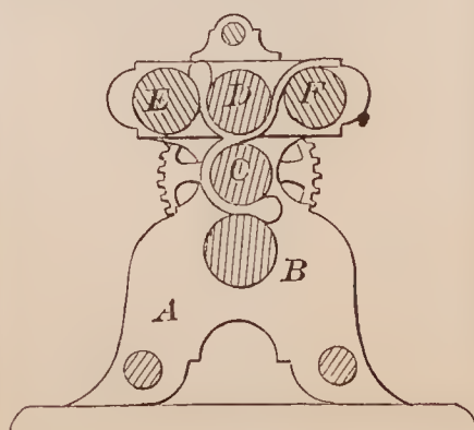
68365—D. C. Hull—For Rolling Rubber into Sheets.
