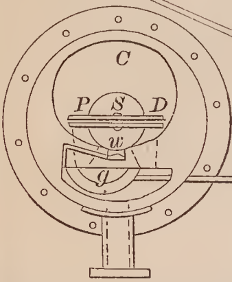
68920—J. Q. Welch— Rotary Steam Engine.
