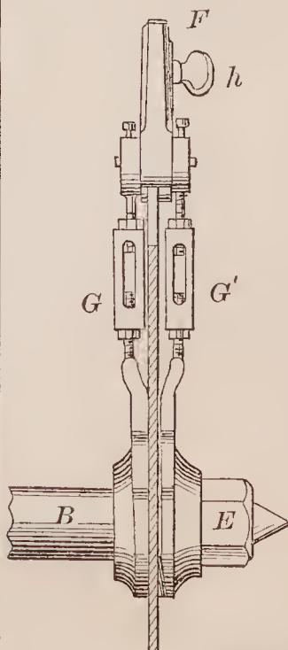
70422—M. De Voursney— Fastening for Coach Lamps.
