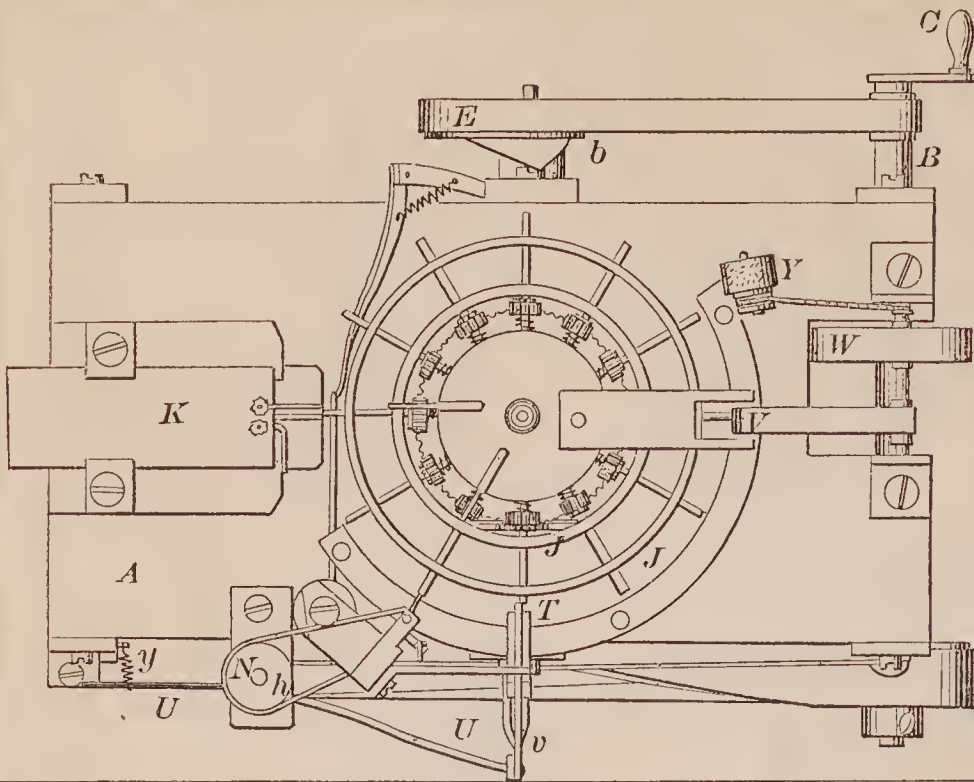
68430—T. Fowler—For Reducing Wires for Needle Blanks.
