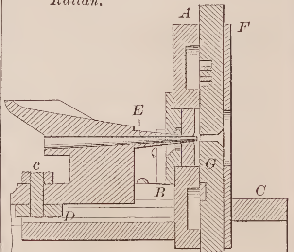
72291—L. Heywood—For Splitting Rattan.
