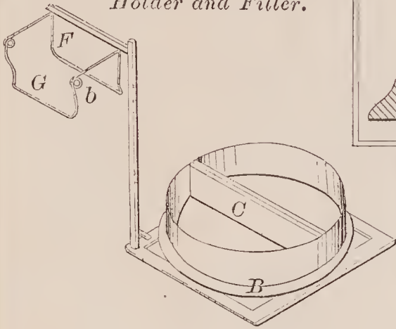
71286—A. M. Darling— Bag Holder and Filler.
