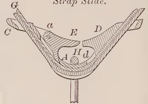
71901—O. B. North— Breast Strap Slide.
