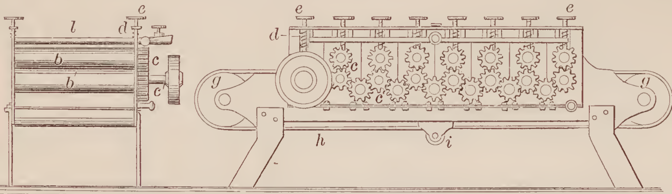
66839—I. Hogeland—Washing and Wringing Machine.
