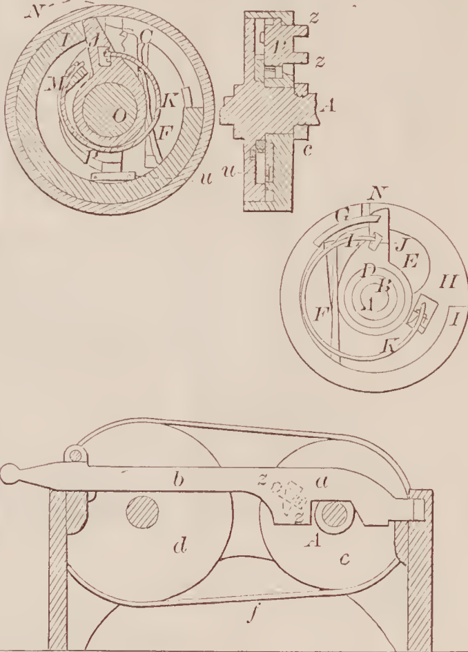
72014—J. P. Gates— Tight and Loose Pulley.
