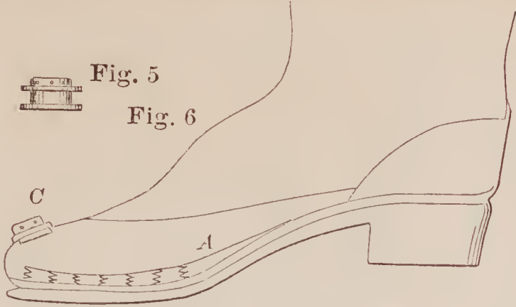
70915—A. Stocker— Ventilating Boots and Shoes.
