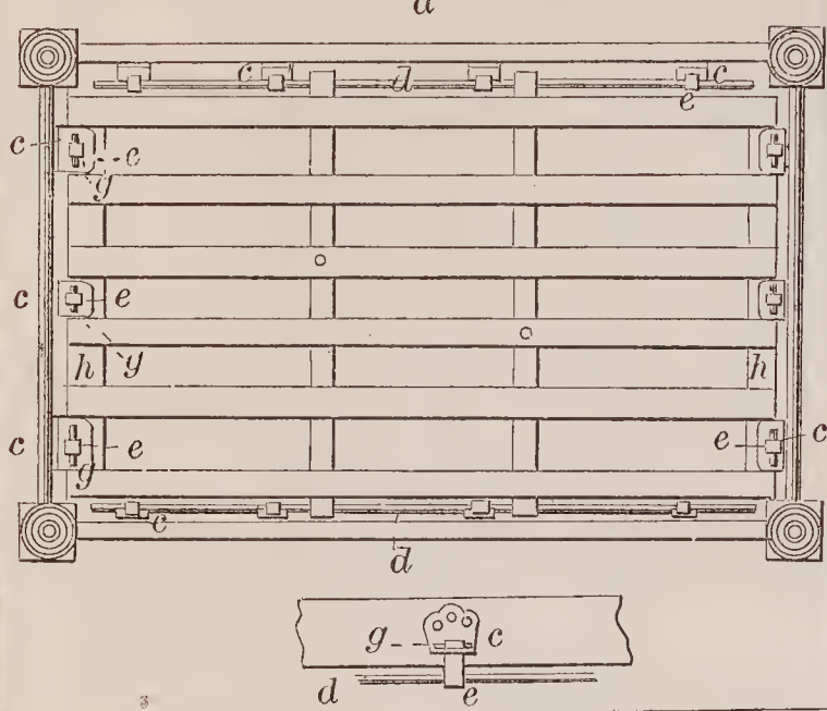
67604—W. Stickney—Bed Bottom.
