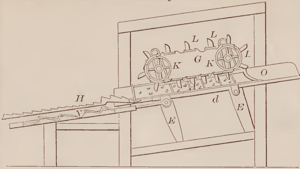
71093—S. D. Warner— Threshing Machine.
