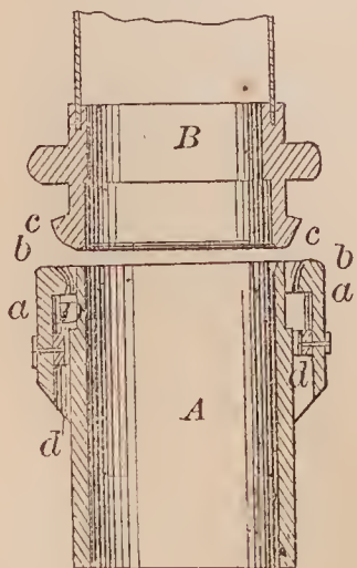
68993—J. Kerns—Hose Coupling.
