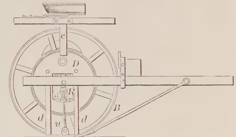
67211—H. Pease—Harvester.
