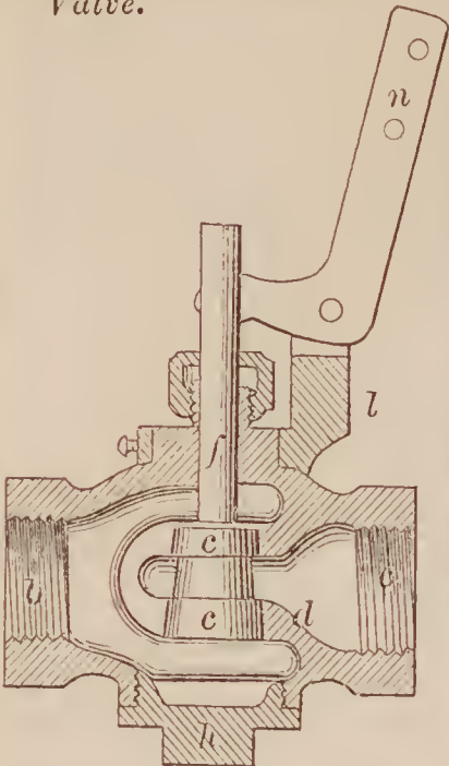
67018—J. Briggs—Globe Valve.
