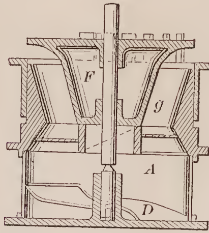
72169—G. M. Connor—Water Wheel.
