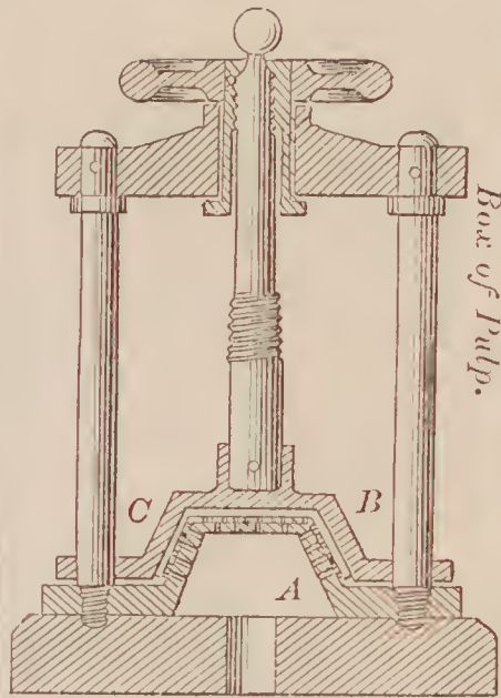
66920—Wheeler & Jerome—Making Blanks for Paper Boxes.
