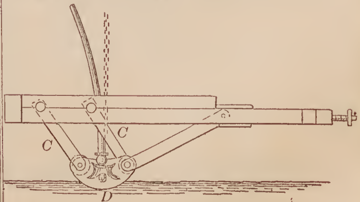
69000—E. T. Ligon—Submarine Plow.
