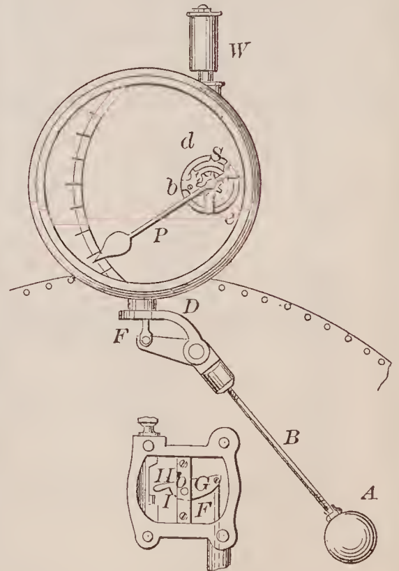
67608—D. M. Swain—Boiler Water Gauge.
