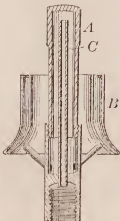
72188—E. P. Gleason—Gas Heating Burner.
