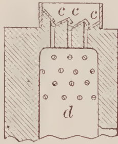
67492—J. Bühner—For the Combustion of Fuel.
