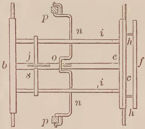
66917—S. Warren—Wagon Brake.
