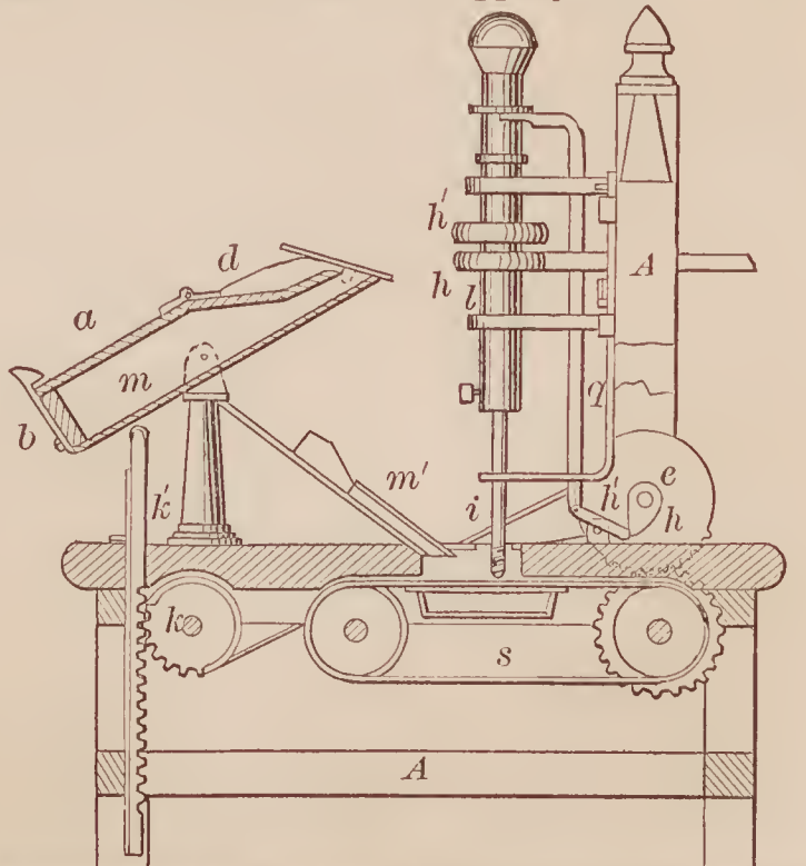
72487—Hart & Blakeslee—Tapping Nuts.
