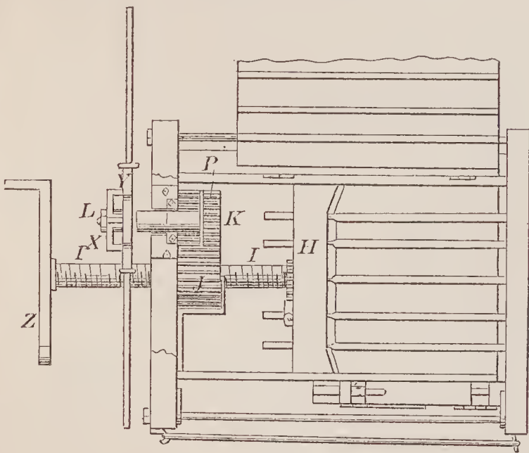
69657—T. D. Guthrie, Jr.—Baling Press.
