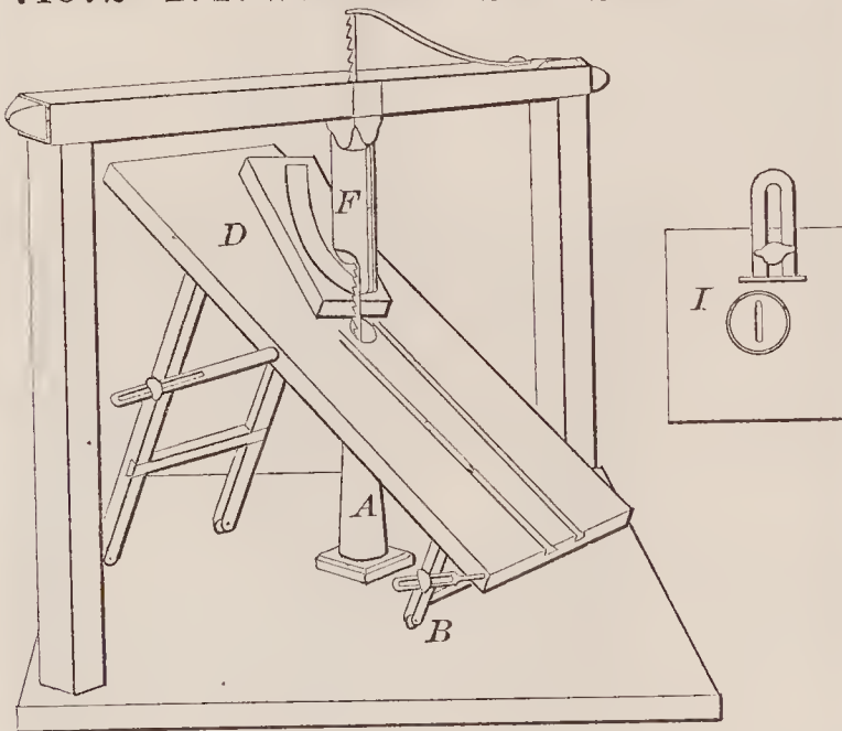
71672—B. F. Williamson—Scroll Saw Mill.
