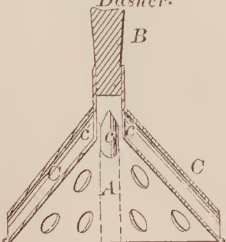
68067—H. Grass— Churn Dasher.
