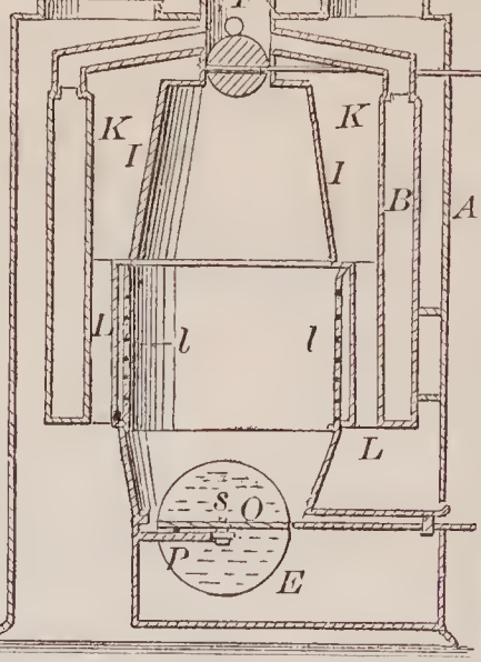
67732—G. B. Davis—Hot Air Furnace.
