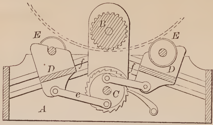
72476—J. Gettemy—Tire Bending and Shrinking.
