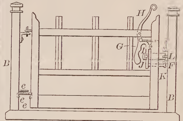
66832—B. Greenside—Gate.
