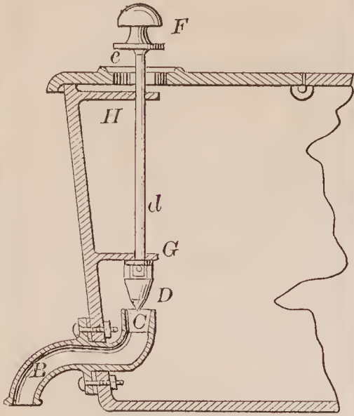
70815—J. B. Crowley—Faucet for Stove Reservoirs.
