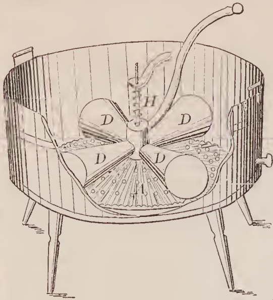
69835—J. Park— Washing Machine.
