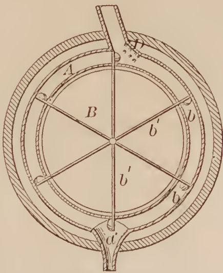
68472—J. C. Walker—Grain Meter.
