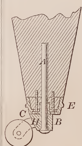
71363—L. F. Cerf—Furniture Caster.
