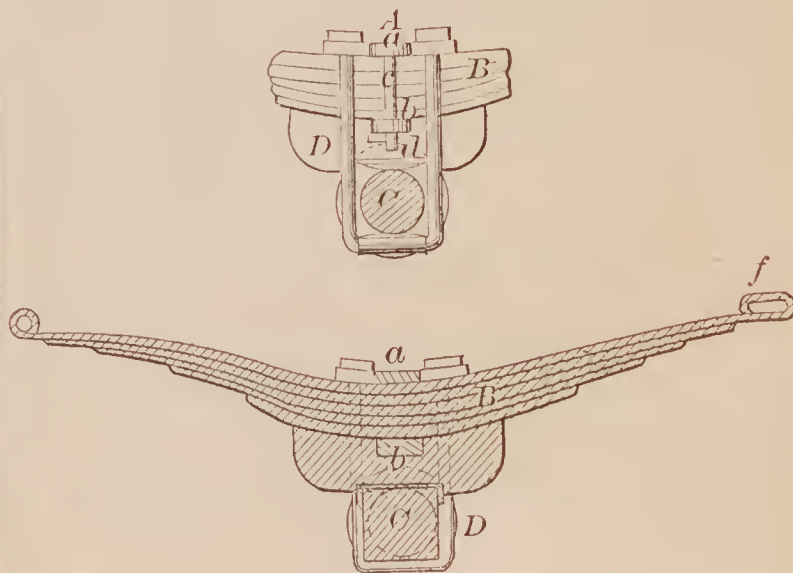
72425—J. Sebastian— Wagon Spring.
