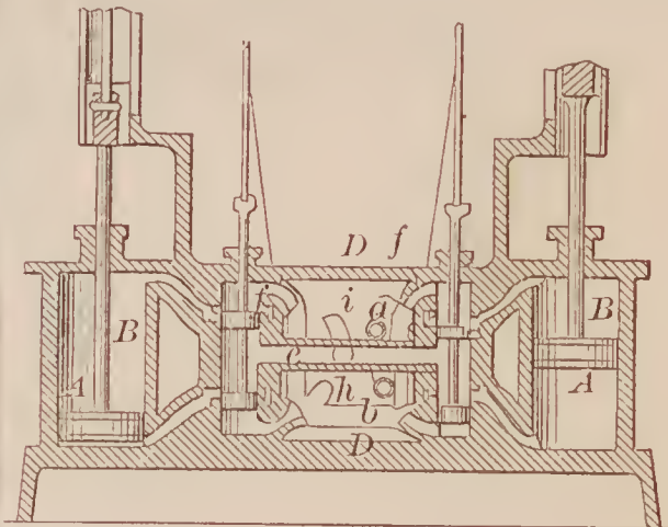
68783—C. R. & N. P. Otis— Steam Engine Valve.
