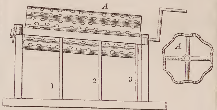
71099—E. W. Weston—Revolving Coal Screen.
