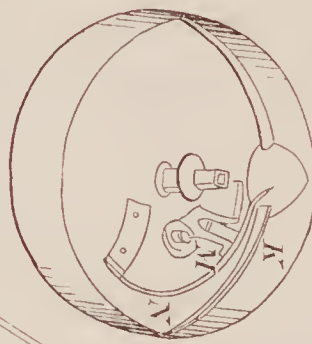
71264—W. D. Baughn—Thimble Skein for Axles.
