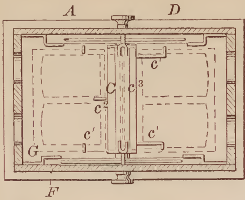
72480—O. Goerke—Stereoscope.
