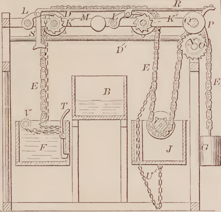
72343—P. Week—Tidal Water Elevator.
