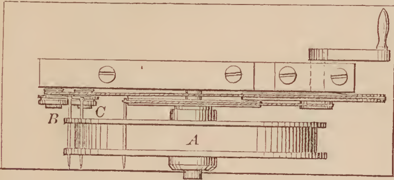
72718—E. F. Bradley—Head Roll for Pin Machines.
