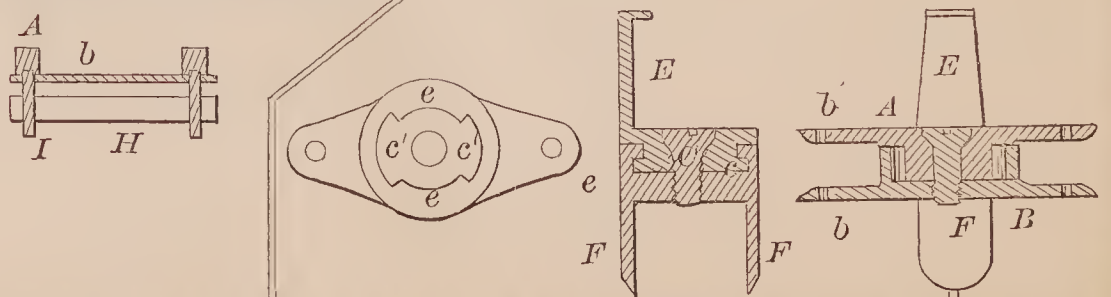
72888—M. J. Palmer—Whiffletree Coupling.
