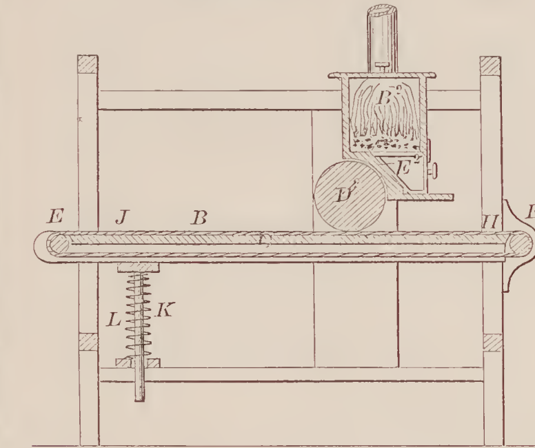
71758—C. R. Hoyt—For Ironing Clothes.
