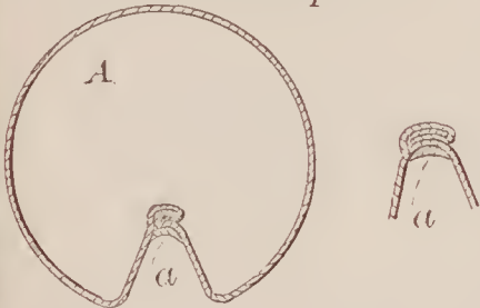
71222—J. C. Rohrman—Conductor Pipe.
