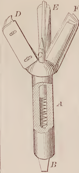
72031—C. F. Hall—For Refitting Conical Valves
