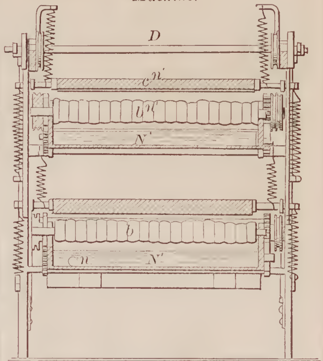
71959—J. W. Blackham—Hat Felting Machine.
