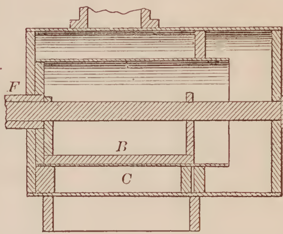
68477—Witt & Sina—Hemp Brake.
