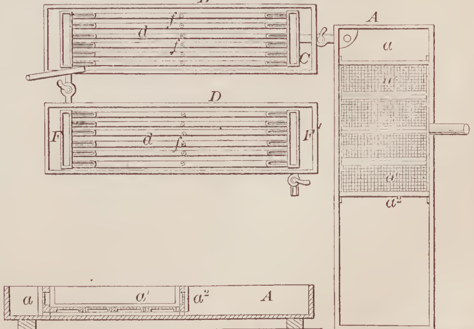
69920—W. Partington—For Cooling Malt Liquor.
