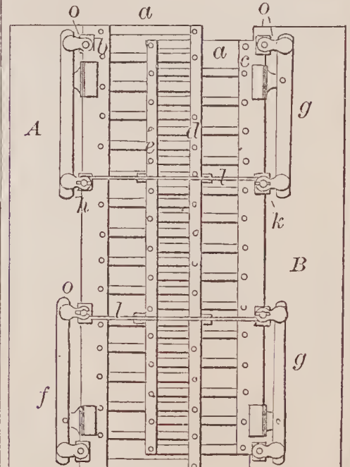
67700—J. Adams—Cotton Cultivator.
