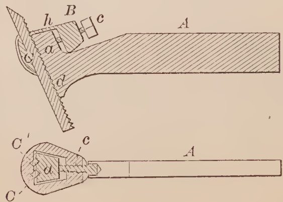
72468—J. Edson—Lathe Tool Holder.
