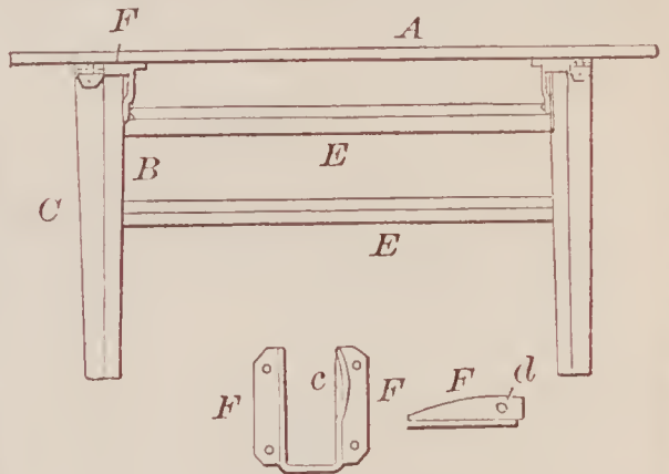
67406—J. P. Brown—Folding Table.
