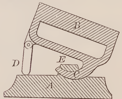
67979—C. C. Hare—Sad Iron.
