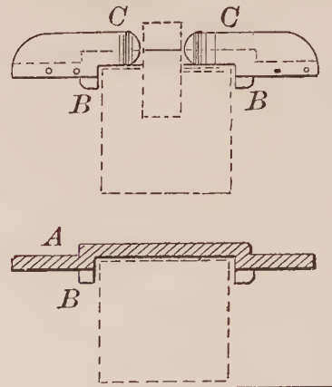
69723—J. B. Stryker—Metal Roofing.
