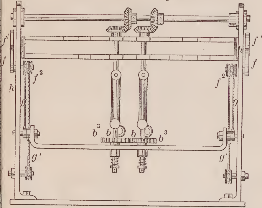
69159—S. Barbour—For Finishing Thread.
