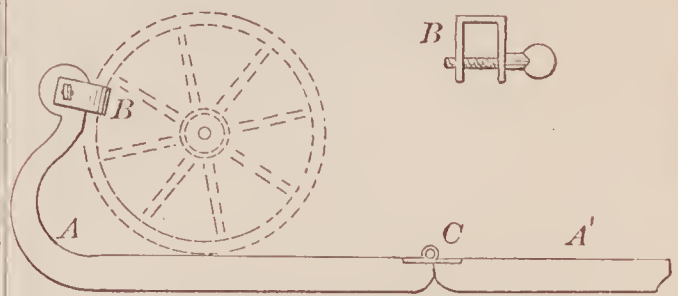
69509—A. Tandy—Gate.
