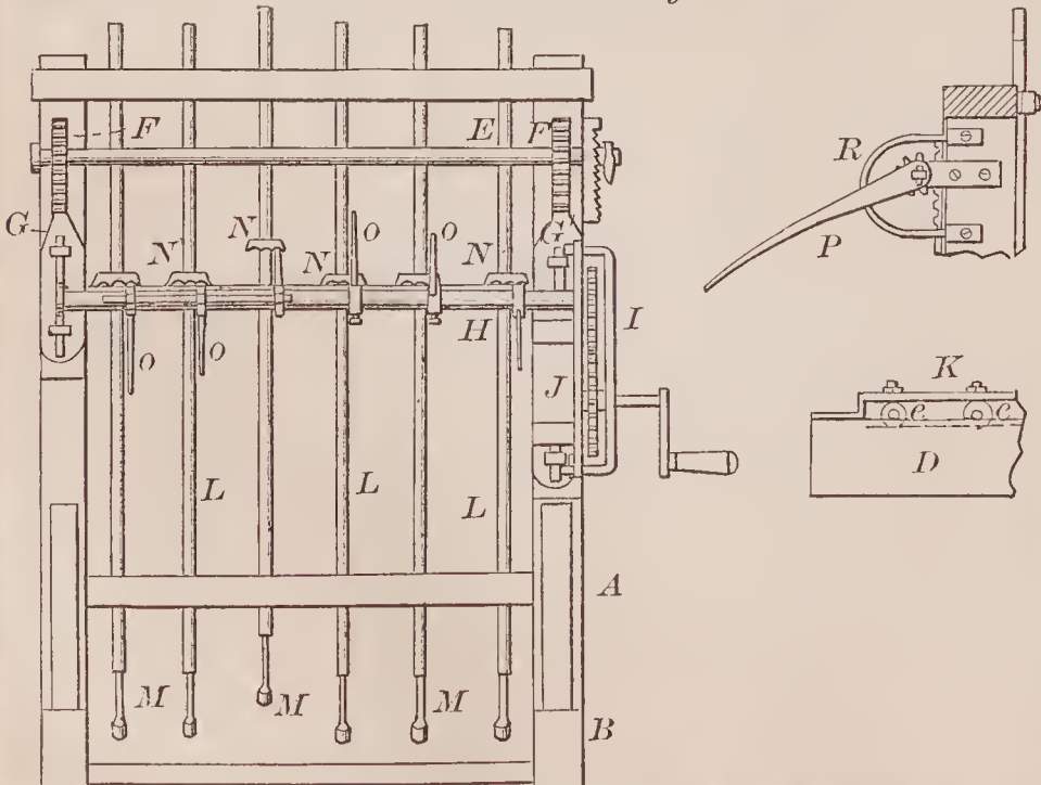
68580—A. M. Southard— Stone Drilling Machine.
