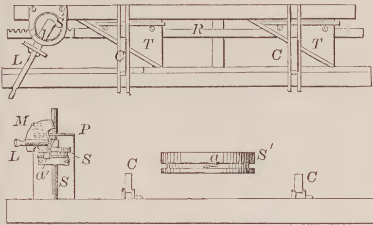
71678--T. C. Ball--Head Block for Saw Mills
