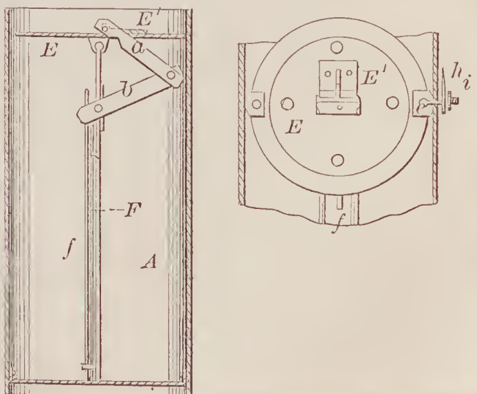
67687—G. A. Townsend—Automatic Damper.
