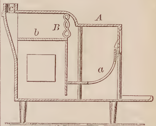
69204—F. Gearing—Market Box.
