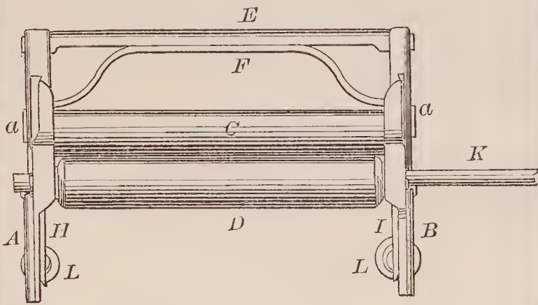
66835—Harrison & Harris—Clothes Wringer.
