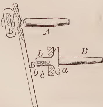
68505—C. Hayden— Trace Fastener.
