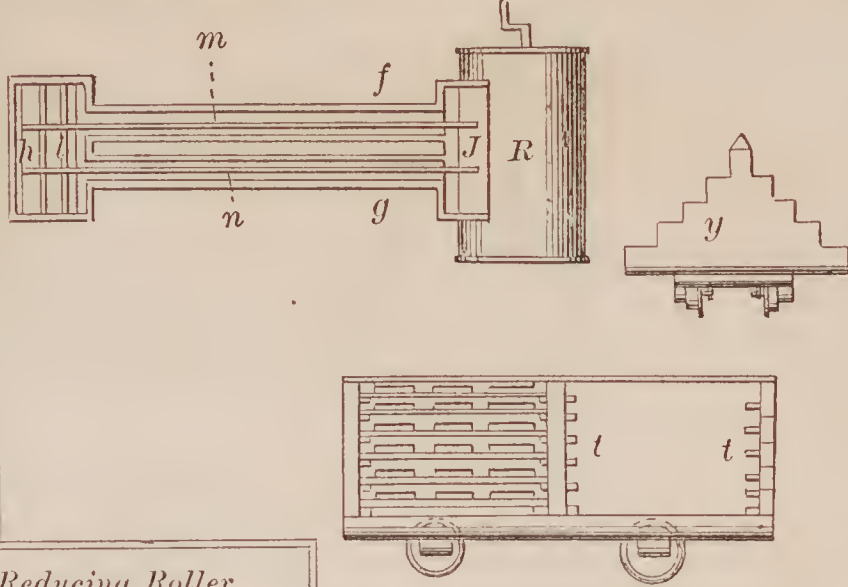
69217—J. J. Johnston—Brick Dryer.
