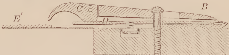
72443—L. Bailey—Carpenters' Plane.
