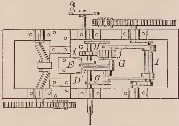
72549—J. Shartle— Gate.
