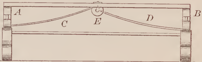
69386—M. Barker—Elliptic Spring Brace.
