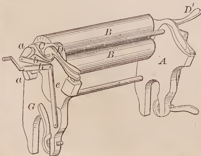
68732—F. A. Gleason— Clothes Wringer.
