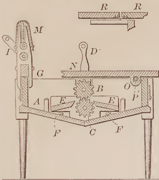
68270—J. Whitney—Washing and Wringing Machine.
