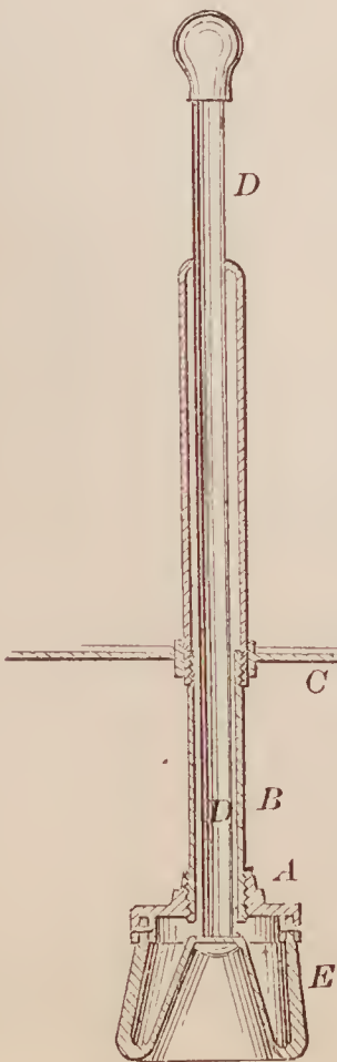
70600—C. P. Moyer— For Administering Balls to Horses.
