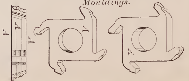
71817—J. Temple— Cutter Head for Mouldings.
