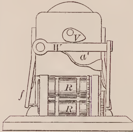
68224—Minor & Ward—For Filling Ruts and Leveling Roads.
