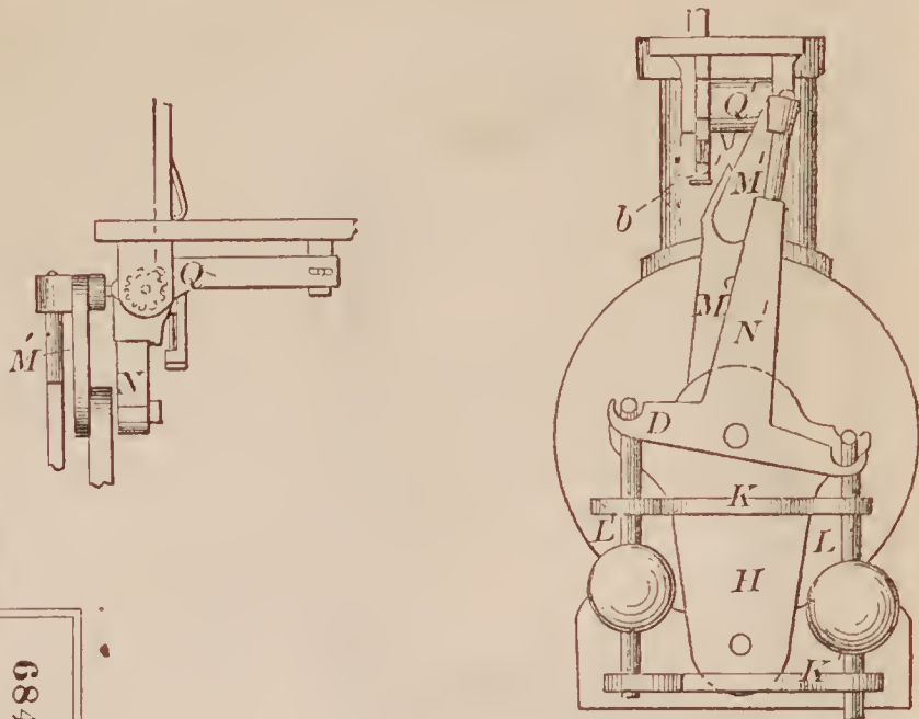
68473—J. V. Weitz—Low Water Detector for Steam Generators.
