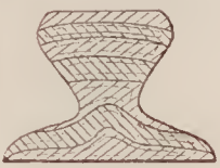
67683—W. A. Sweet—Fagot for Railroad Rails.
