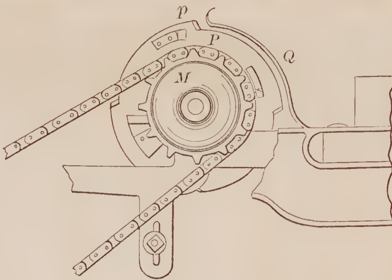
69188—H. Crossman— Self-Acting Mule.
