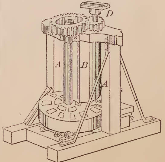
68907—H. C. Sergeant—Brick Machine.
