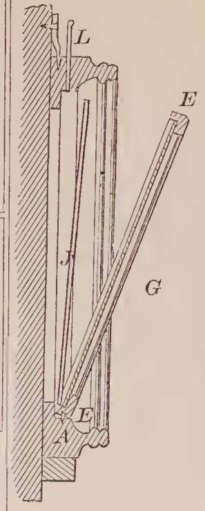
70116—C. P. Poirier—Frame for Pictures, &c.
