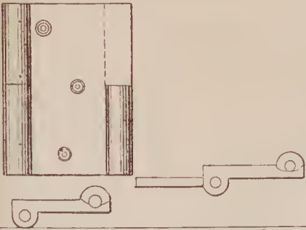
69368—G. W. Sanders—Mop Head.
