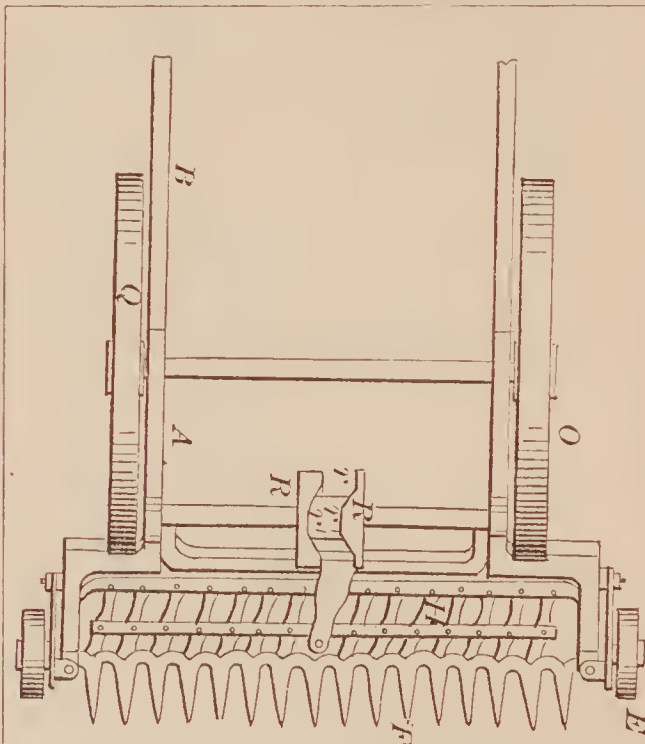
72722—R. F. Cooke—Harvester.
