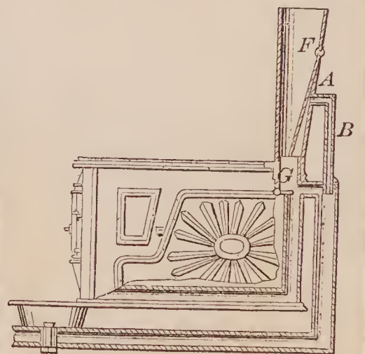
68437—E. Hamburger—Stove Pipe.
