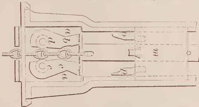
70848—A. H. Howe—Self-Adjusting Thill.
