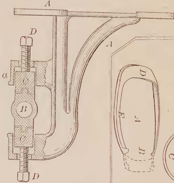
68826—J. Yocom, Jr.—Hanger for Shafting.
