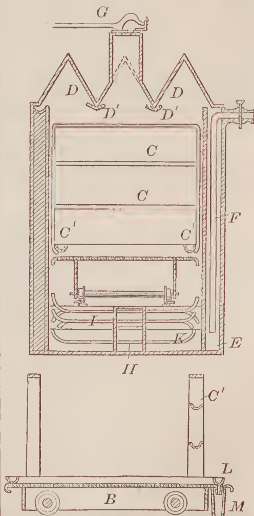
68044—S. Chapman—Kbin for Drying and Preparing Peat.
