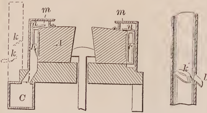
72318—W. R. Mozier—Seed Planter.
