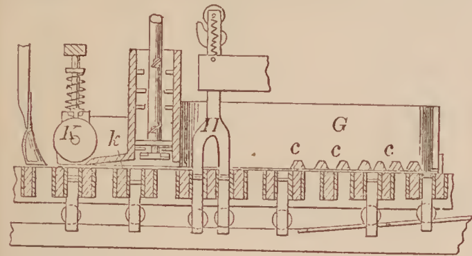
68896—C. D. Page—Brick Press.
