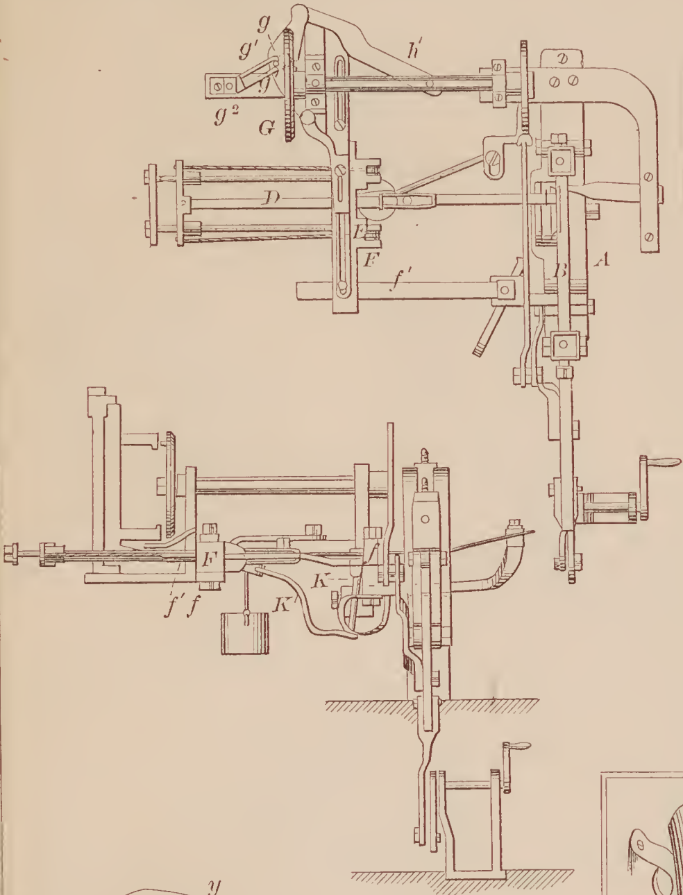
72392—F. Hain— For Feeding Nail Plates.
