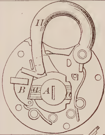
72166—C. J. Clements—Padlock.
