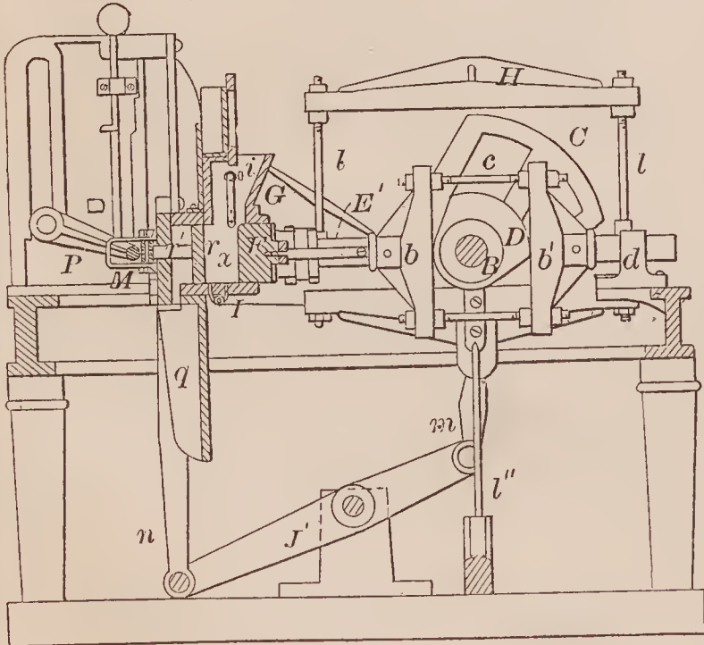
68396—L. Sylvester— Brick Machine.
