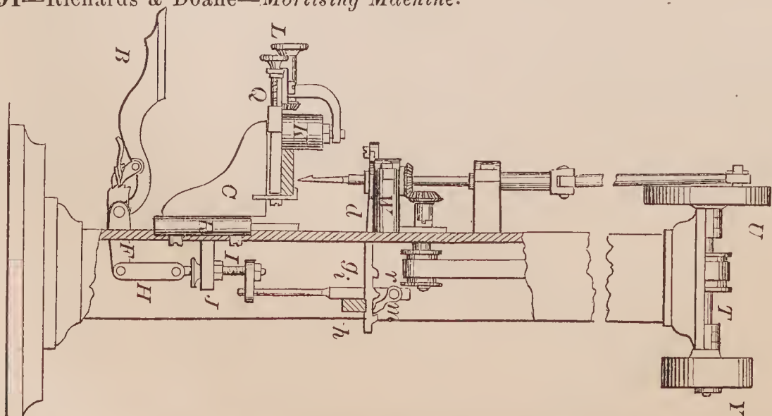
68791—Richards & Doane—Mortising Machine.
