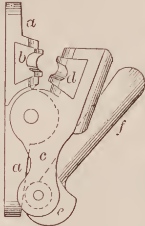
68304—W. Morse—Line Holder.
