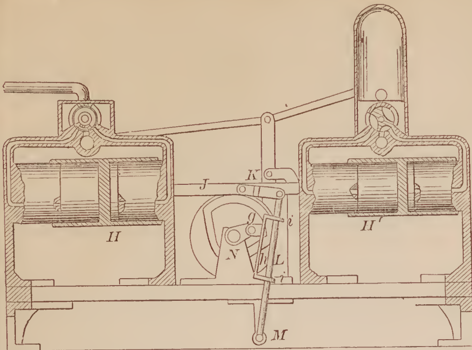
68994—J. C. King—For Operating Valves of Force Pumps.
