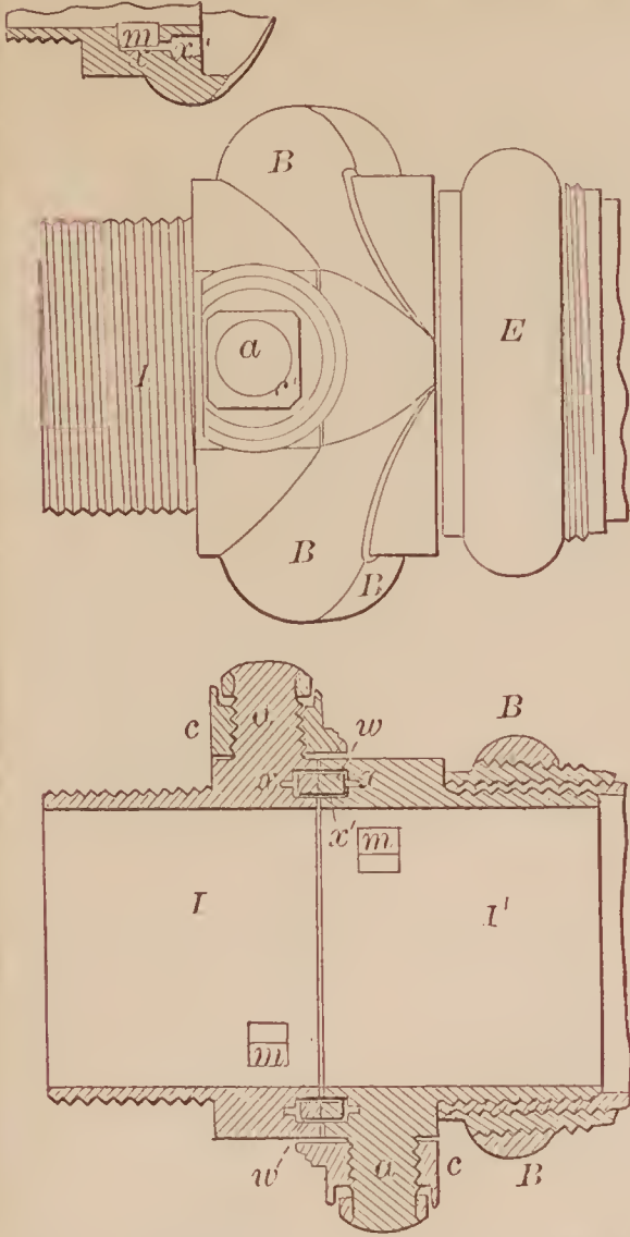
72892—Perkins & Hovey—Hose Coupling.
