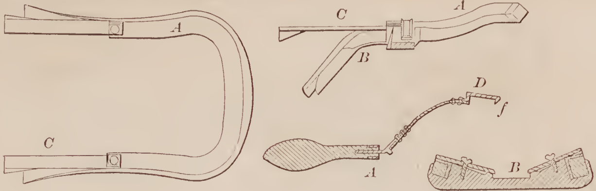
72292—L. Heywood—For Bending Wood.
