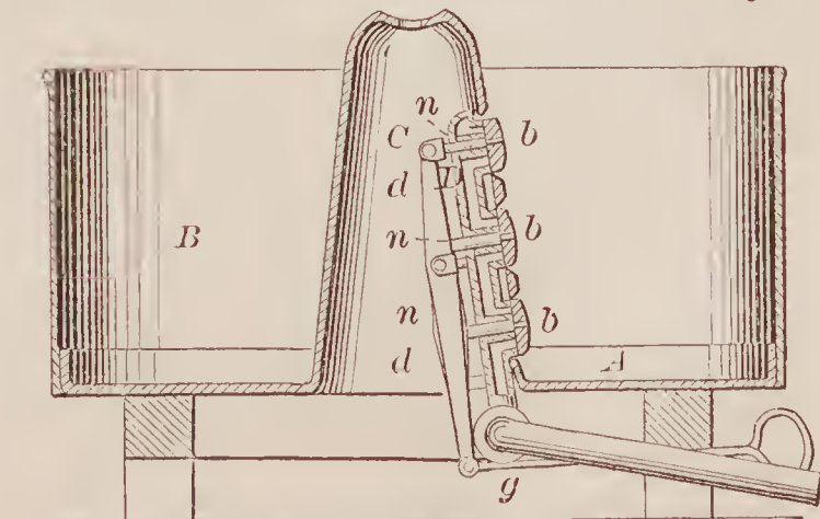
72182—S. Fountain—Concentrator and Amalgamator.
