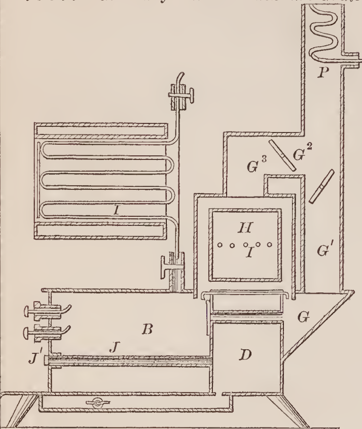
70077—G. Dewey—Water Back and Grate of Stoves.
