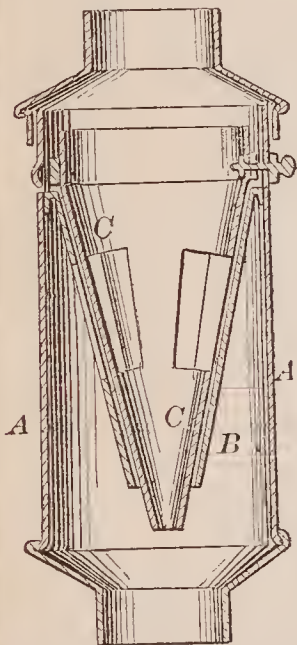
70659—E. Webster— Stove Pipe Drum.
