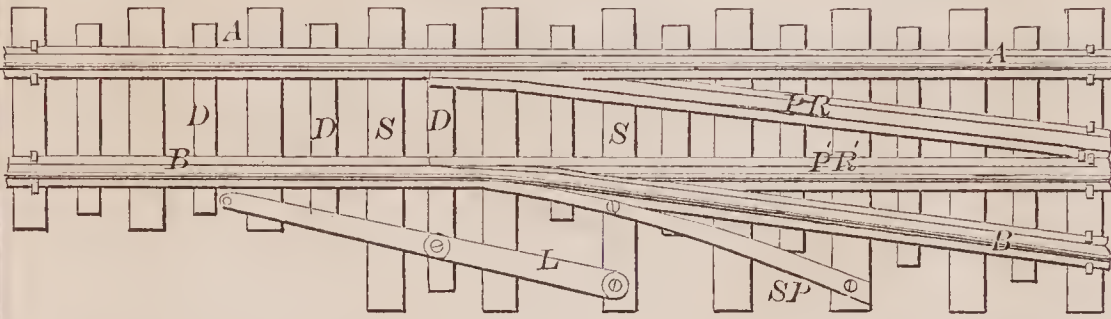
71308—C. W. Jones— Railway Switch.
