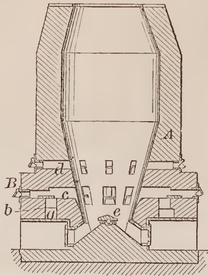
70045—A. Thoma—Kiln for Roasting Iron Ore.
