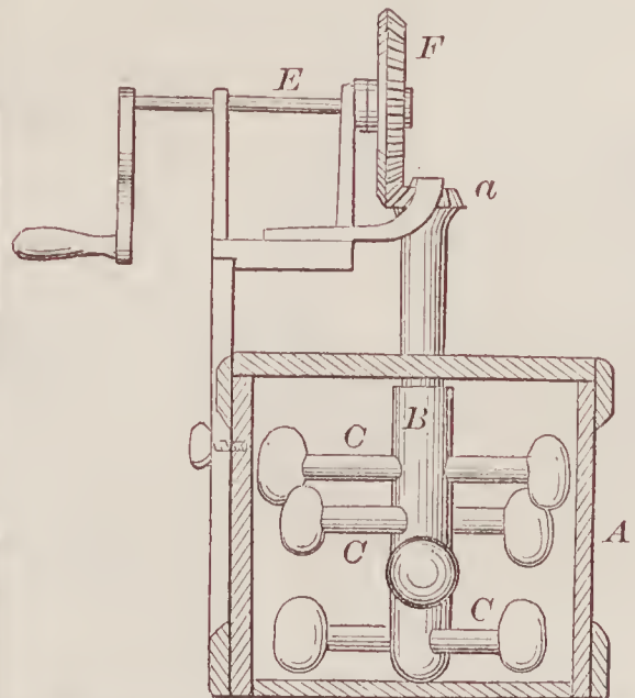
72682—J. Risher—Churn.
