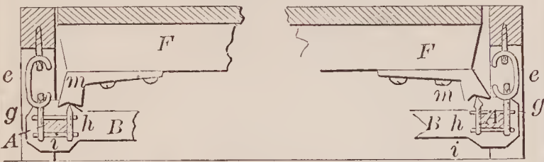
71179—G. W. Jackson— Platform Scale.
