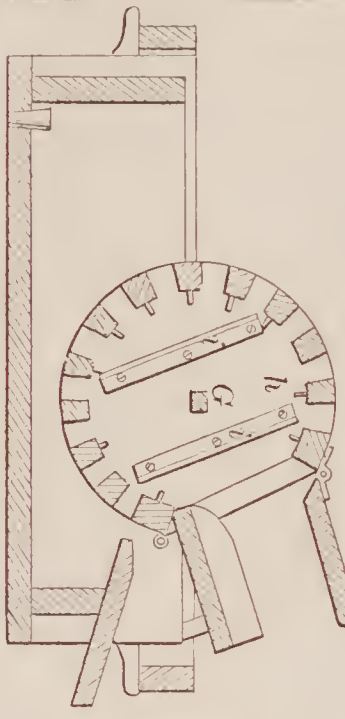
71433—J. Watson—Furnace Door.
