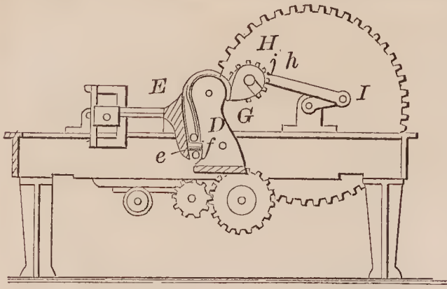
72547—R. B. Sears— For Bending Hooks.
