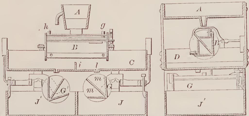
72698—I. P. Tice— Spirit Meter.
