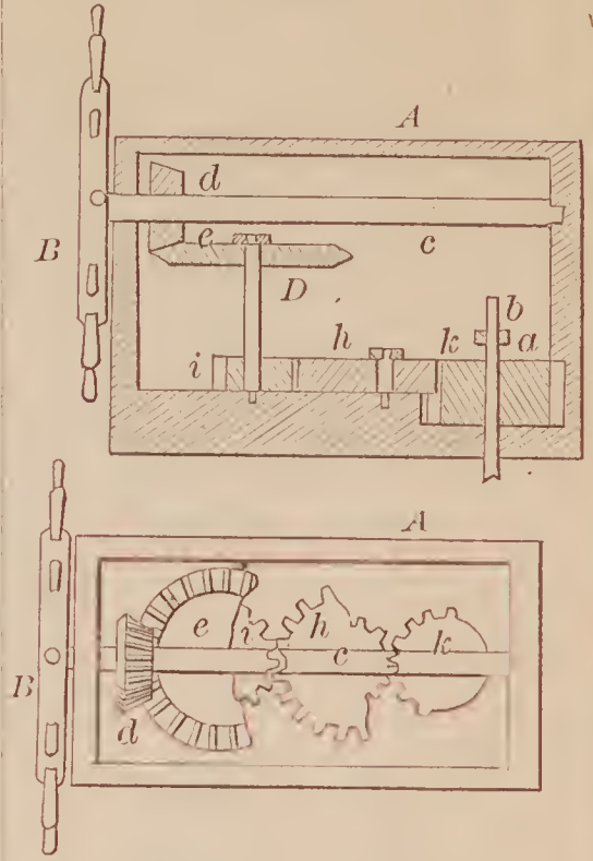
72945—J. H. Weaver—Steering Apparatus.
