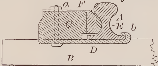
67280—W. Foster—Railway Chair.
