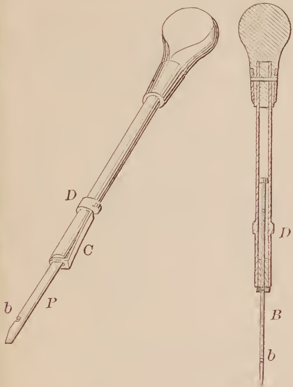
72465—F. B. Doering— For Boring Rocks.
