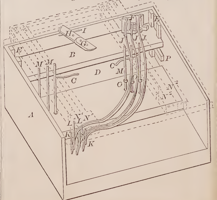
71314—Ling & Chandler— Organ Coupling.
