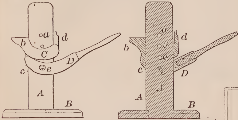
68454—J. Palmer—Die for Making Heads for Elliptic Springs.
