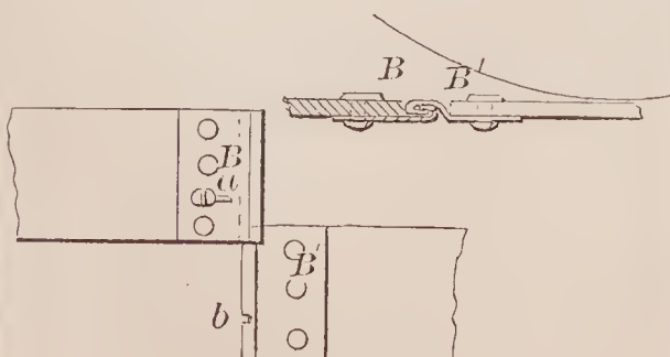
70930—D. Wigger—Belt Fastener.
