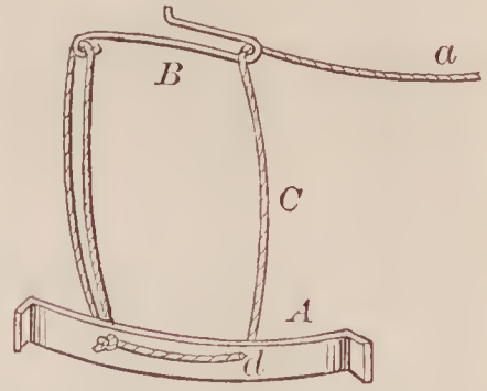
71738—A. I. Goodrich— Regulator for Marine Clocks.
