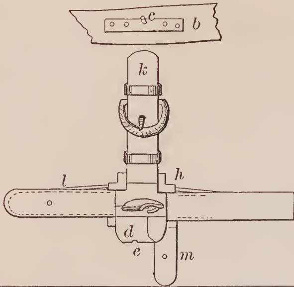
69276—C. S. Twitchell—Folding Chair.
