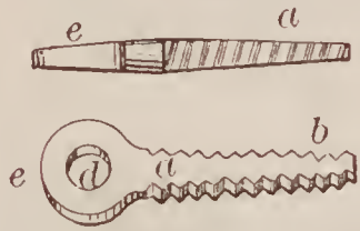
67578—J. Pepper—Door Fastener.
