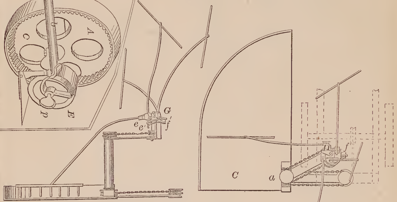
72839—W. F. Goodwin—Harvester Rake.
