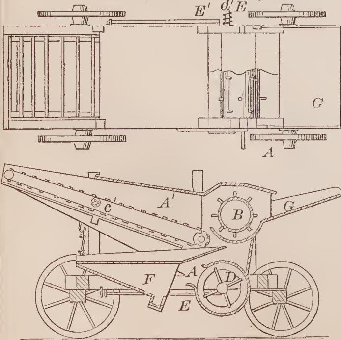
70280—C. L. Snyder—Threshing Machine.
