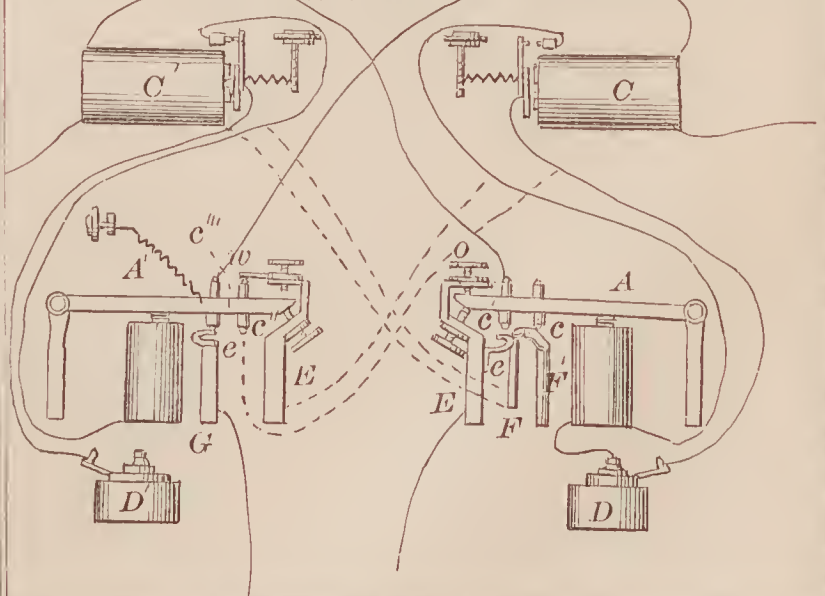
66945—Brownson & Shull—Telegraph Repeating Instrument.
