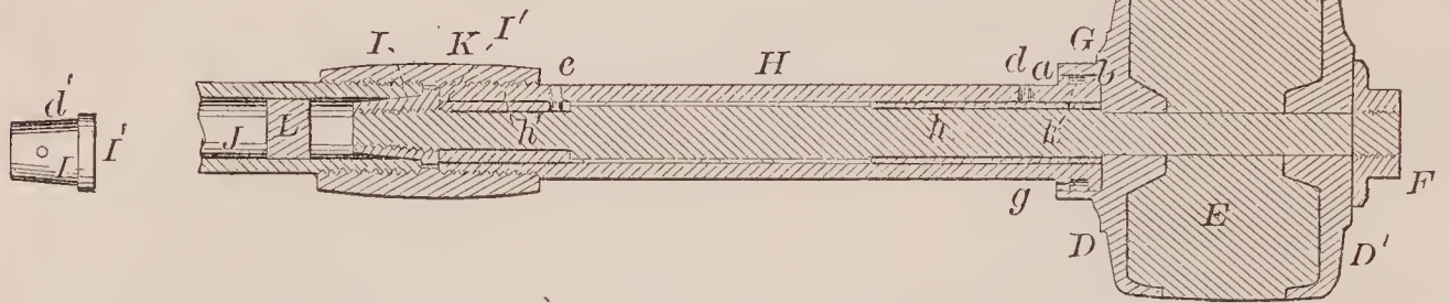
68594—A. Beale—Carriage Wheel.
