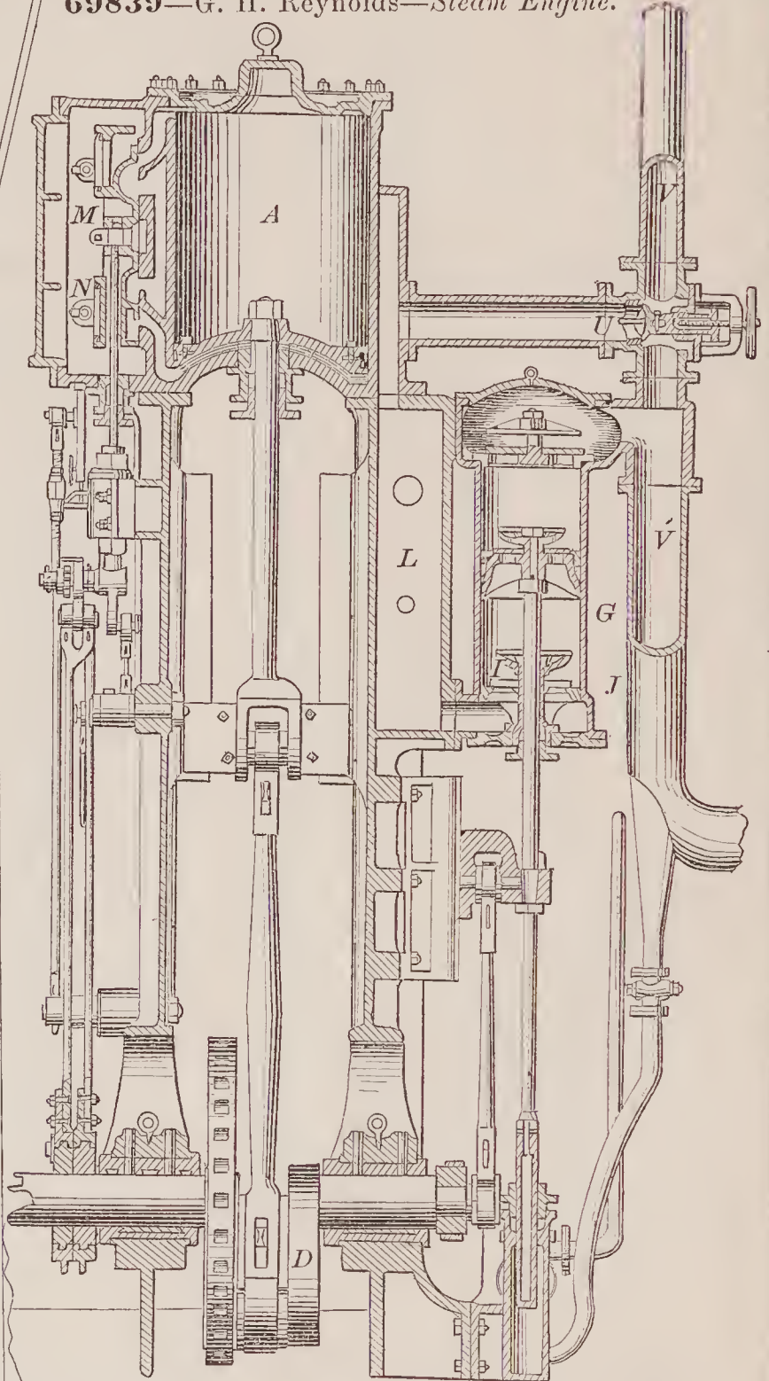
69839—G. H. Reynolds— Steam Engine.
