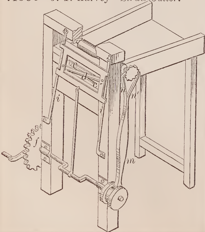
71000—J. T. Harvey— Straw Cutter.
