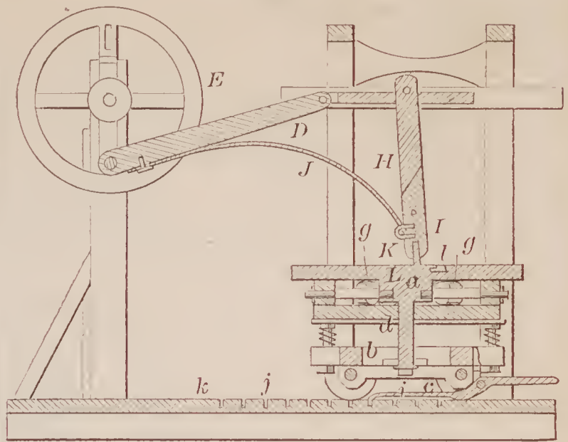
70268—Roberts & Lennox— For Beaming Hides or Skins.
