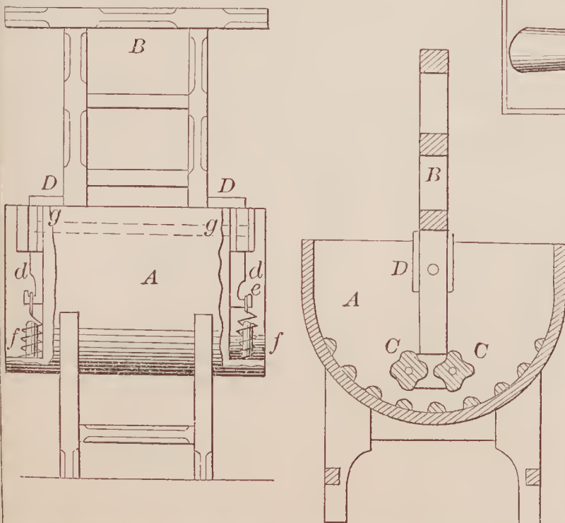
69493—J. Schermerhorn—Washing Machine.
