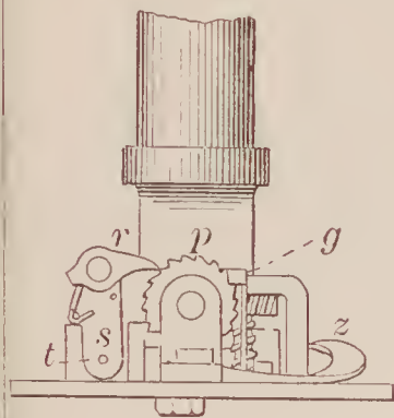
69504—Stevens & Drake—Odometer.
