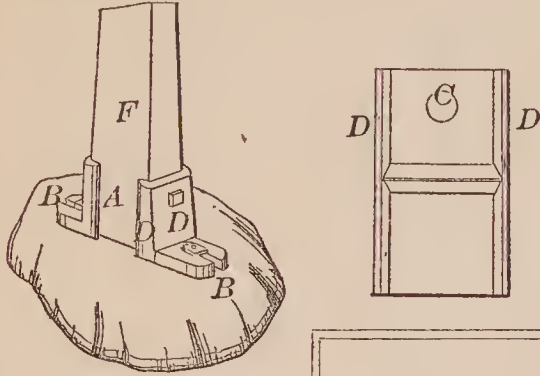
68888—E. G. Lamson— Operating Drill.
