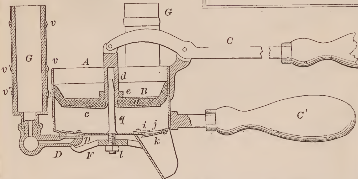
68362—W. D. Grimshaw—Drilling Machine.
