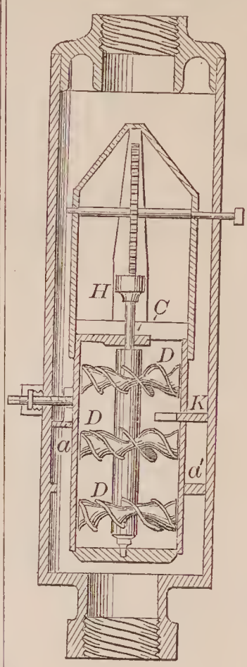
68830—R. H. Atwell— Liquid Meter.
