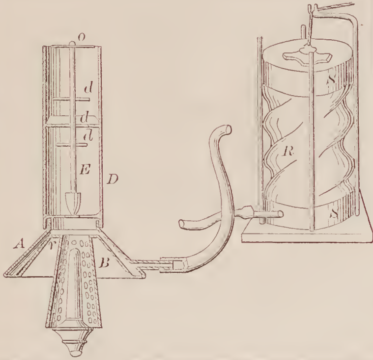
71002—D. G. Haskins—Gas Heating Apparatus.
