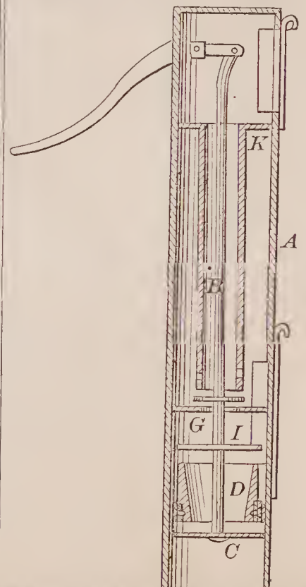
71122—J. Bean—Pump.
