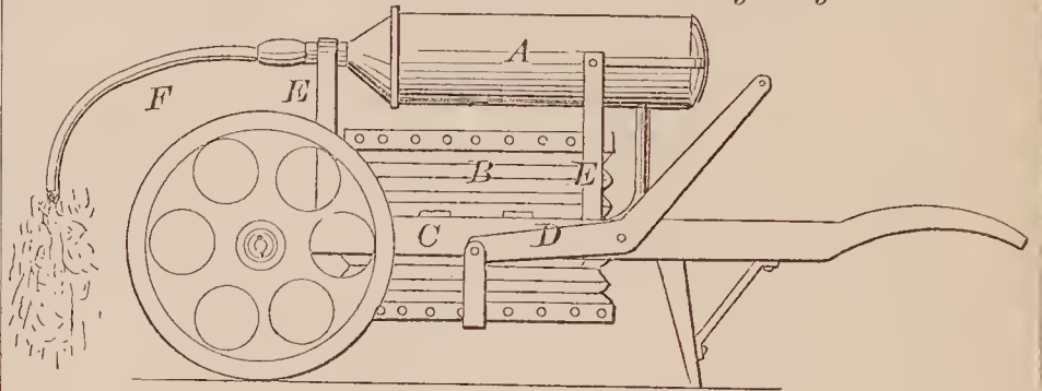
72419—C. C. Preston—For Fumigating Plants.
