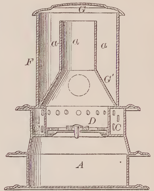
69537—C. H. Buck—Heating Stove.
