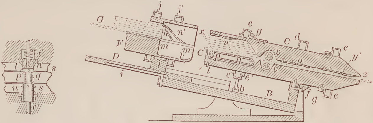
71521—E. B. Lake— Nail Plate Feeder.
