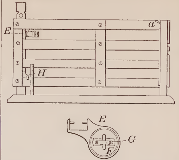
69914—L. Hermance— Gate.
