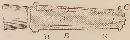
68460—H. Richardson— Axle Bearing for Wagons.
