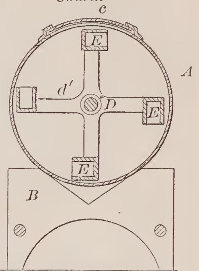
67266—C. J. Chalfant— Churn.
