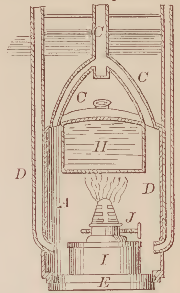
66752—C. C. Taintor—Petroleum Lamp Heater.
