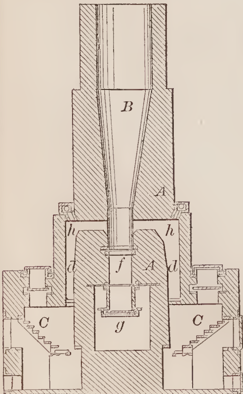
70047—A. Thoma—For Reducing Iron Ore.
