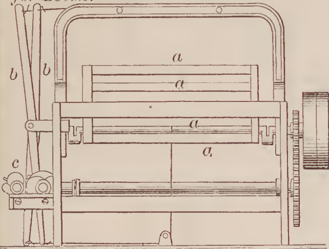
68303—L. J. Knowles—Harness Motion for Looms.
