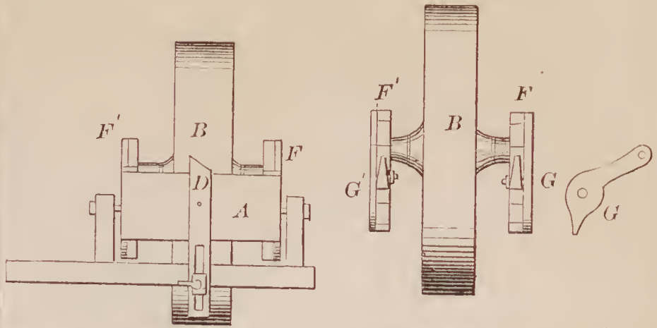
70798—J. Burke—Harvester.
