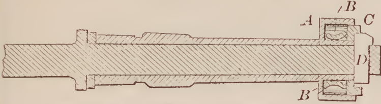
70594—J. Miller, Jr.— Securing Wheels on Axles.
