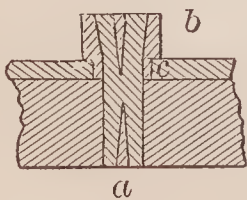
70151—J. Baird—Treenail.
