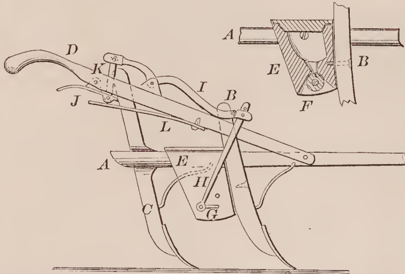
72318—W. R. Mozier—Seed Planter.
