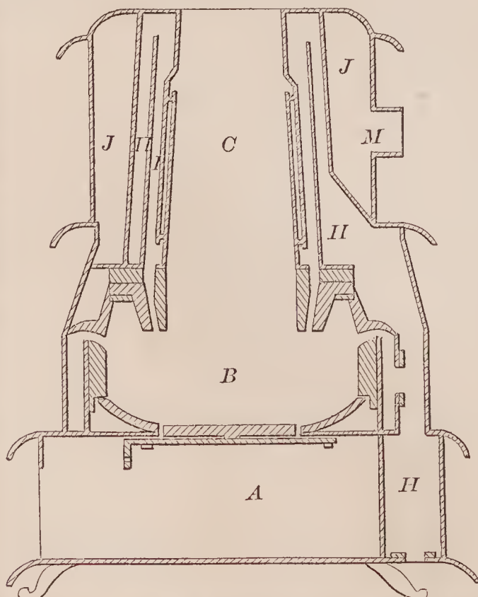
72339—J. Tiffany—Base Burning Stove.
