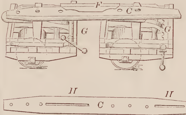
70596—J. H. Moore— For Moving Buildings.
