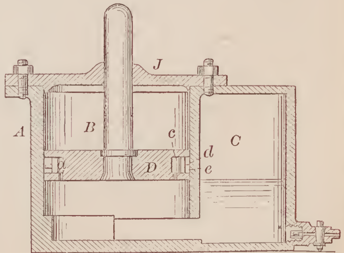
70177—W. A. Dripps—Pneumatic Spring.
