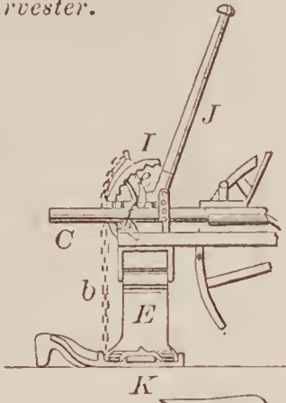
67490—W. F. Brabrook—Harvester.
