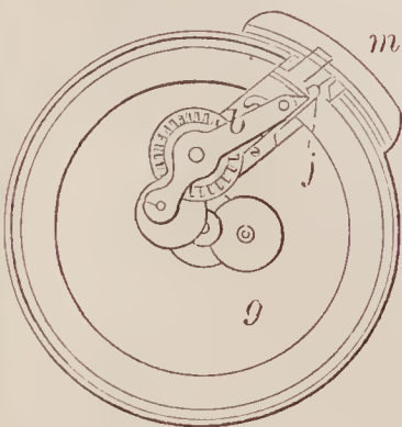
67692—C. V. Woerd—Stem Winding and Setting Watch.
