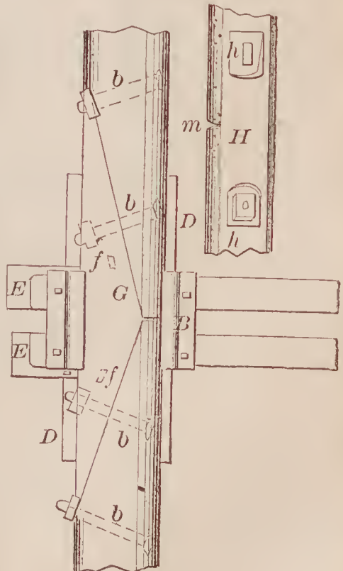
69241—G. Palmer—Joint and Railroad Rail.
