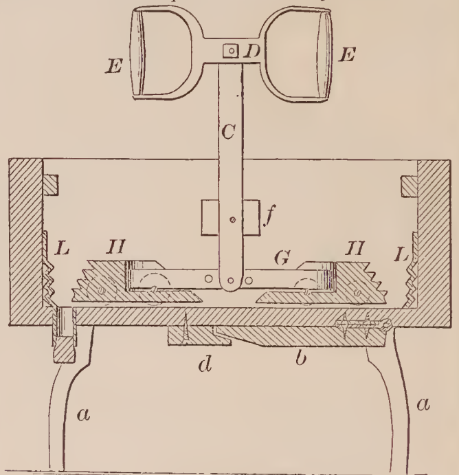
69141—H. Thompson—Washing Machine.
