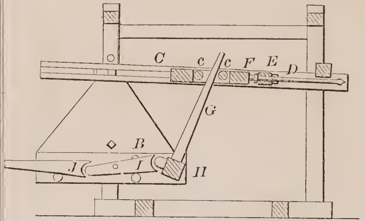
71056—W. Pierce—Rock Drilling Machine.
