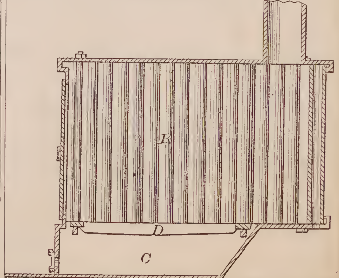
68731—F. Gilman— Coal Stove.
