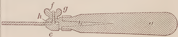
68585—A. Weed— File Handle.
