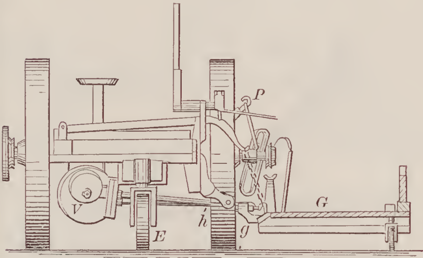
72681—A. C. Richards—Hay Press.
