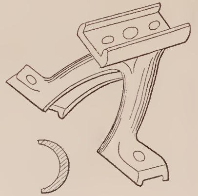
71025—G. Larson—Sleigh Knee.
