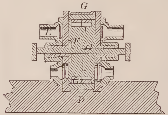
68574—C. C. Reynolds— Threshing Machine.
