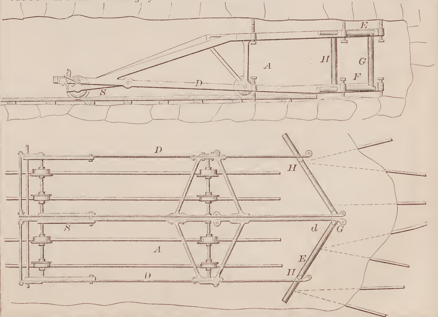
71999—T. Doane—Carriage for Rock Drills.
