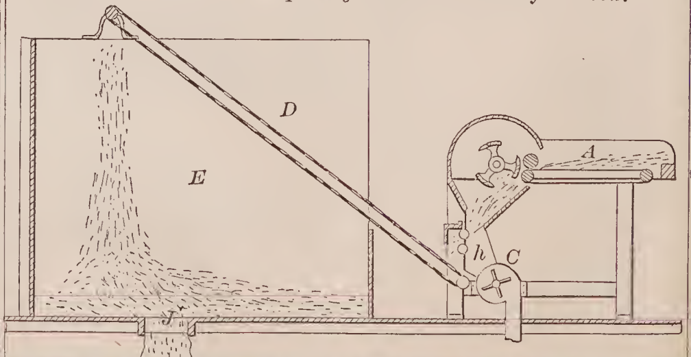
68345—C. Brown—Preparing Short Cut Straw for Feed.
