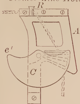
72908—P. Riordan—Clothes Line Holder.
