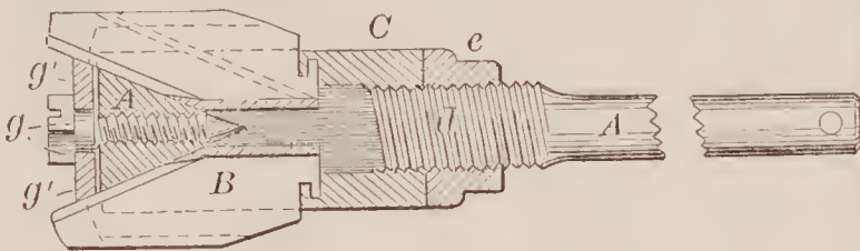
71943—C. Allardice—Reamer.
