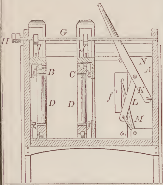
69668—S. R. Holmes—Washing Machine.
