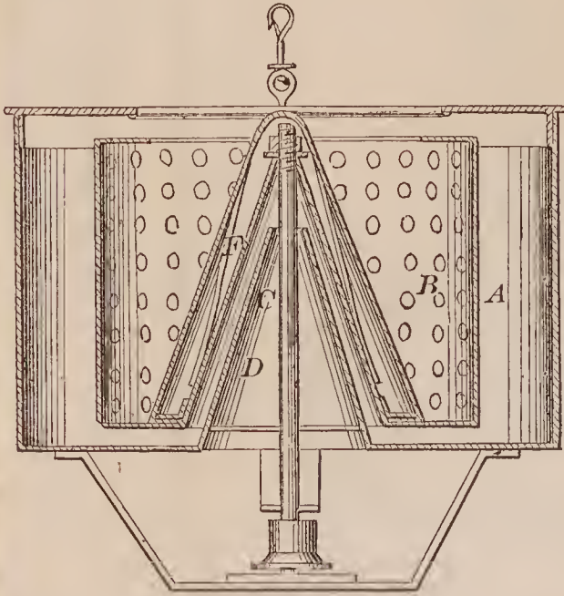
68356—G. E. Evans—For Washing Sugar.
