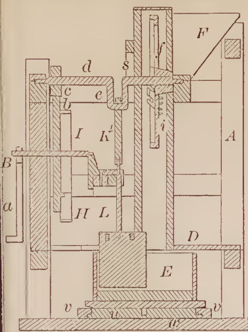
69073—H. Chamberlain—For Chopping Meat.
