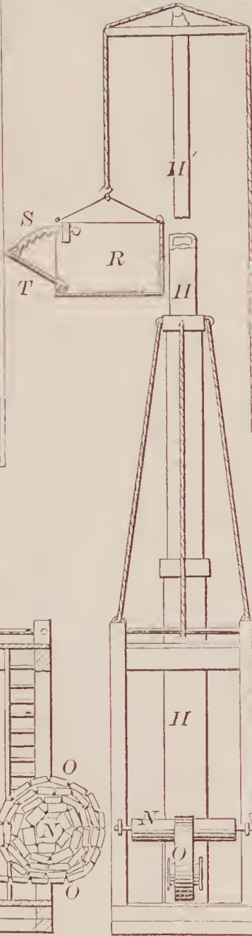
71960—J. E. Bliss—Builders' Scaffold.
