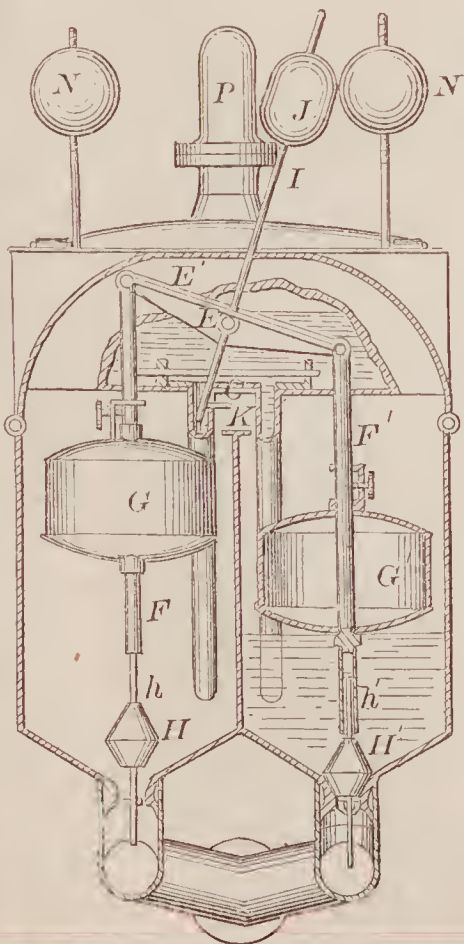
68025—R. W. Young—Liquid Meter.
