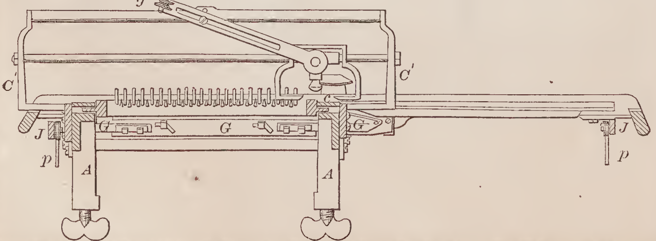
69776—T. Crane—Knitting Machine.
