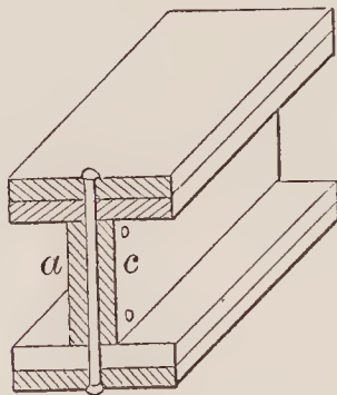
69872—Walters & Shaffer— Fagot for Beams.
