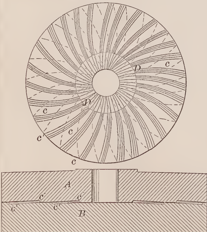
71733—A. N. Garland—Dress for Mill Stones.
