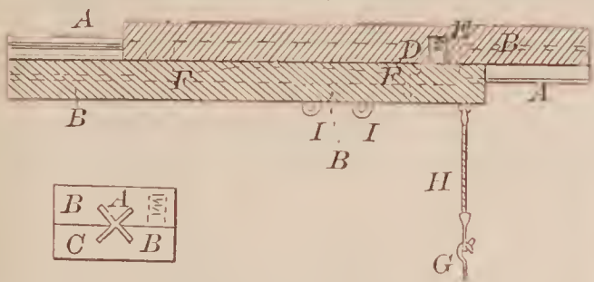
68782—H. Olds— Slide for Extension Tables.
