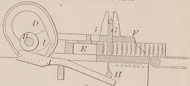
68494—W. L. Drake— Brick Press.
