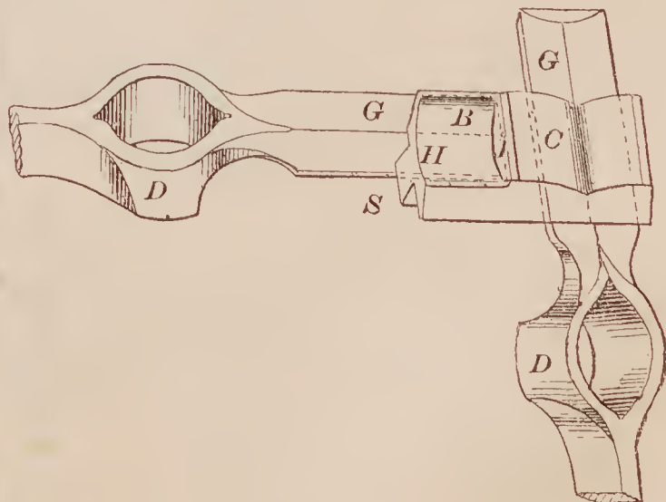
68446—C. Konold—Die for Swaging Mattocks &c.
