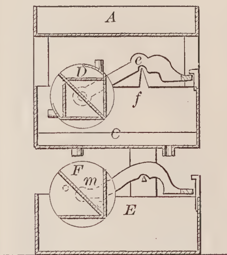
72702—I. P. Tice—Spirit Meter.
