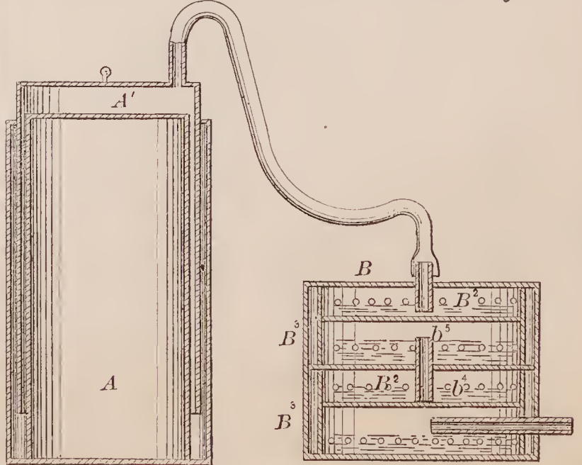
70809—Cozzens & Jones—For Carburetting Air.
