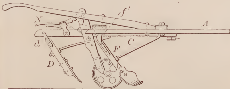
72297—H. Howe—Cultivator.
