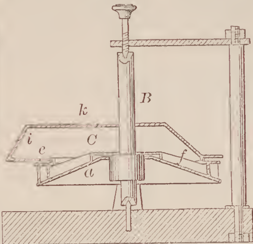
66828—J. F. Gebhart—Harness Motion for Looms.
