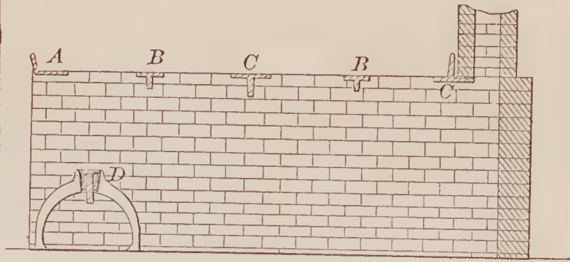
69781—G. S. Deane—Arch Bar for Furnaces.
