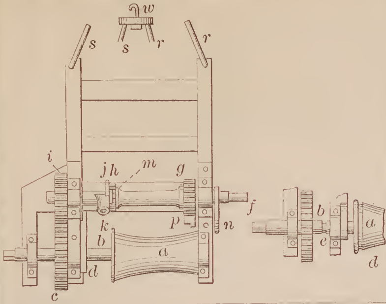
68792—R. D. Rogers—Winch.
