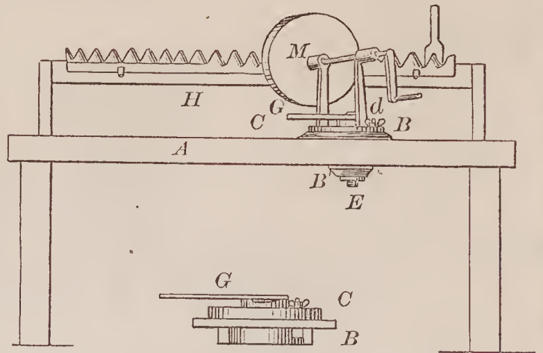
67355—E. M. Scott—For Grinding Reaper Knives.
