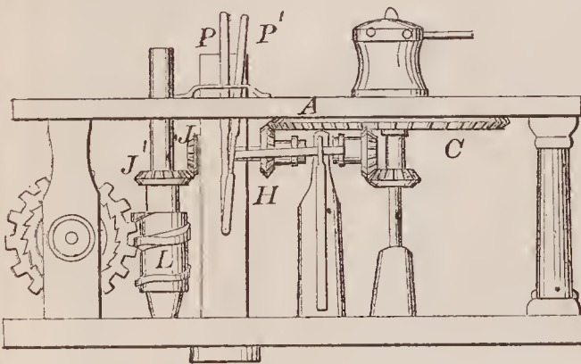
67569—D. P., Nickerson— Windlass.
