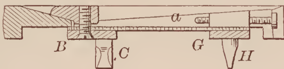
72487—Hart & Blakeslee—Tapping Nuts.
