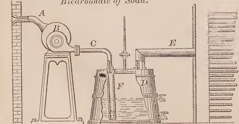
67087—A. P. Von Pornhoff—Manufacture of Bicarbonate of Soda.
