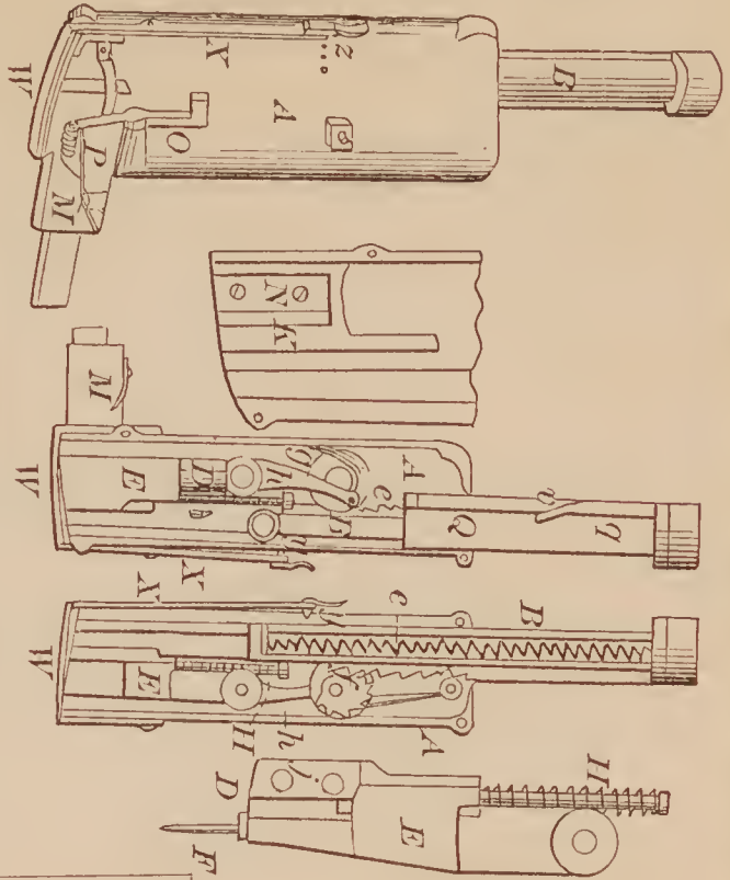
72753—D. D. Palmer—For Pegging Boots and Shoes.
