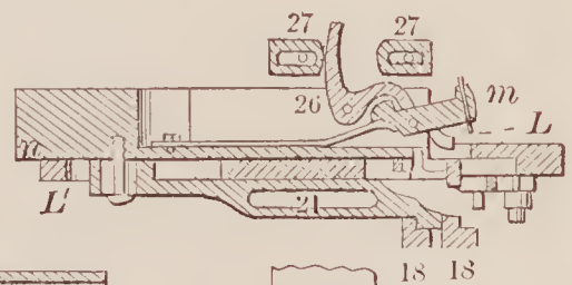
71852—G. W. Chandler—Loom for Weaving Palm Leaf, &c.
