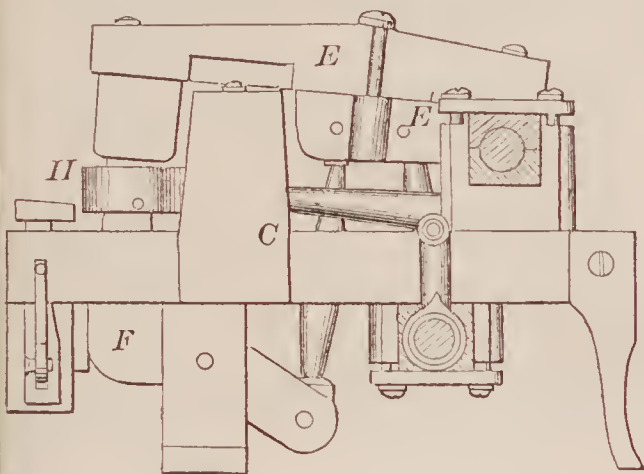
70374—A. St. Louis—Horse Shoe Nail Machine.
