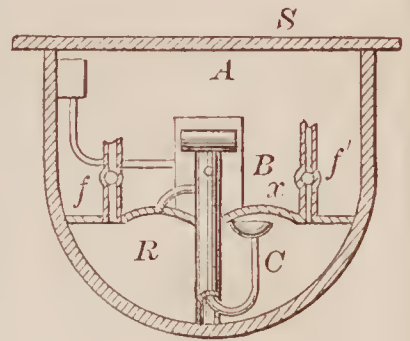
72106—Spedden & Stafford—Propelling Vessel.
