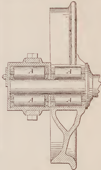
71527—C. H. Parshall— Anti-Friction Journal for Car Wheels.
