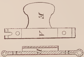
70315—J. C. Baxter—Check Piece for Bridles.
