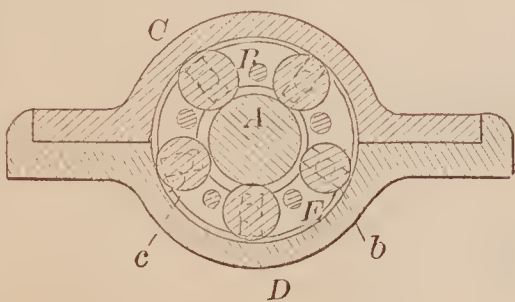
72942—E. Wadhams—Roller Journal Box.
