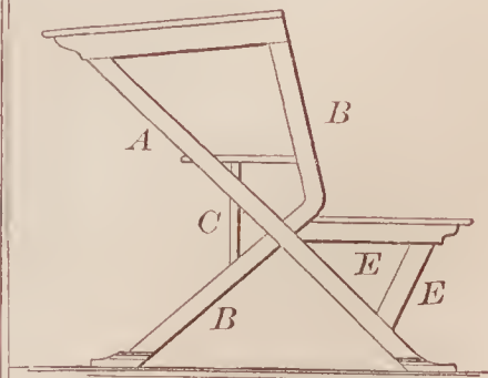
69523—D. C. Wilson— School Desk and Seat.
