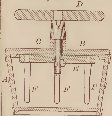
67127—W. L. Lowrey—Manufacture of Illuminating Gas.
