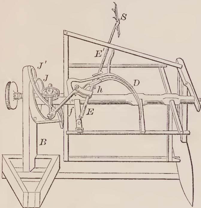
70007—E. J. Leyburn— Harvester Rake.
