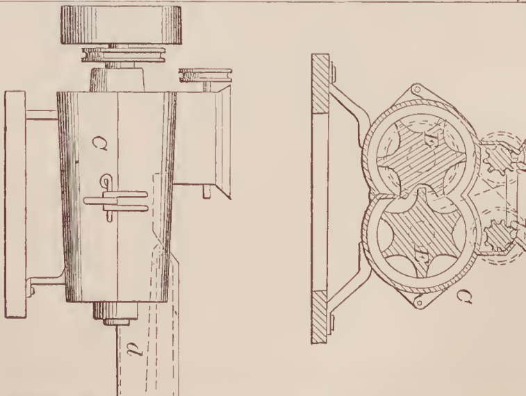
68101—S. Mills—For Grinding Peat.
