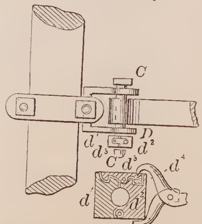
70866—V. Lapham—Bolt Fastening.
