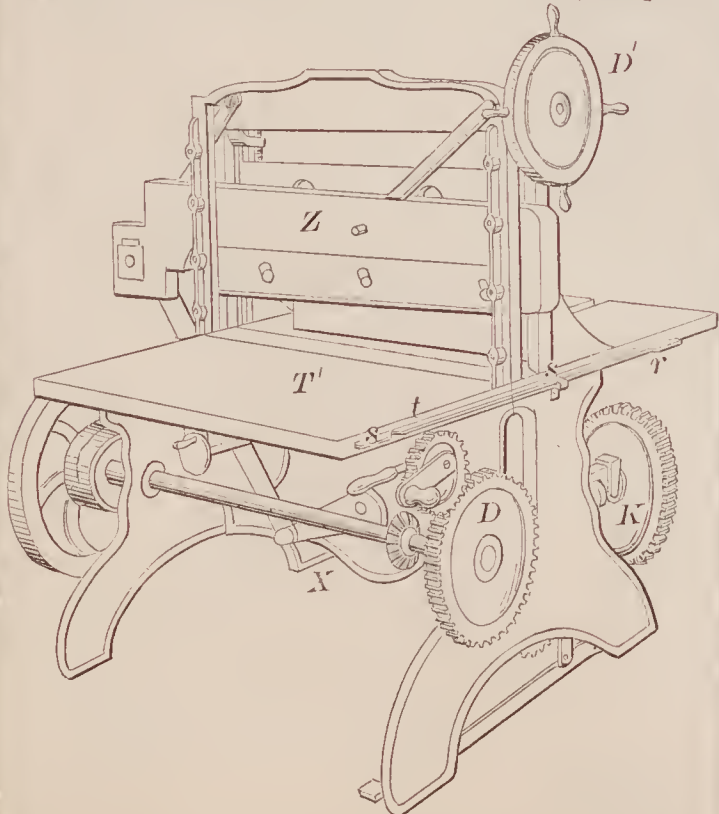
71793—G. H. Sanborn—For Cutting Paper.
