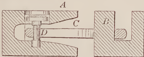
67311—W. R. Jamison—Car Coupling.
