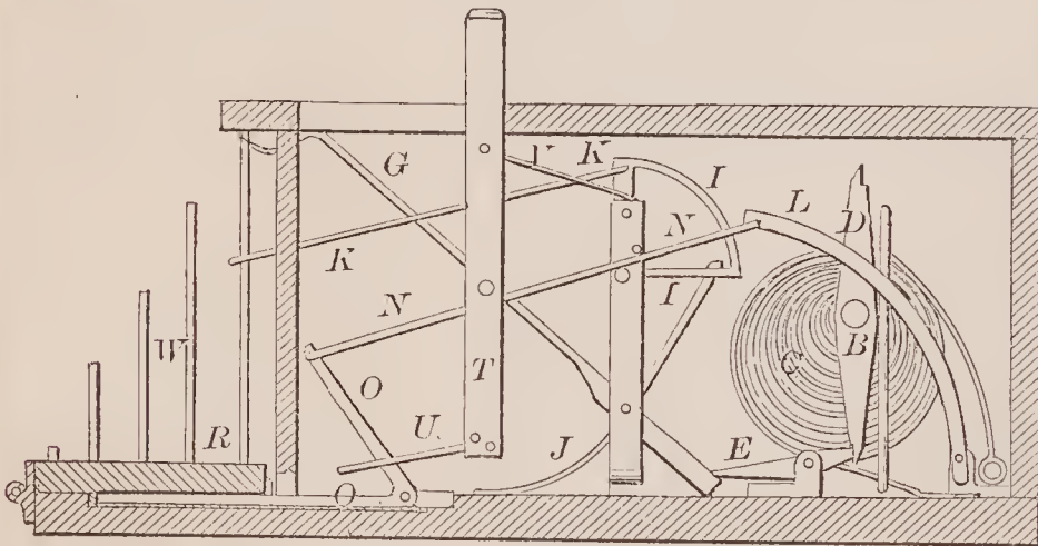
70929—A. Wilkin—Self-Setting Game Trap.
