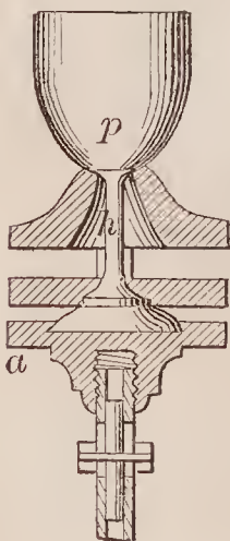
71447—O. B. Brigham—Snap for Glassware Makers.
