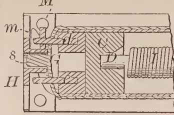
68552—E. T. Briggs—Curtain Fixture.
