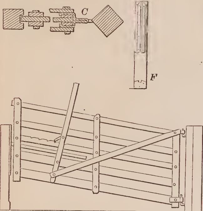
69138—States & Lutts—Farm Gate.
