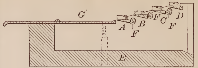
70545—N. Goddard—For Splitting Whalebone.
