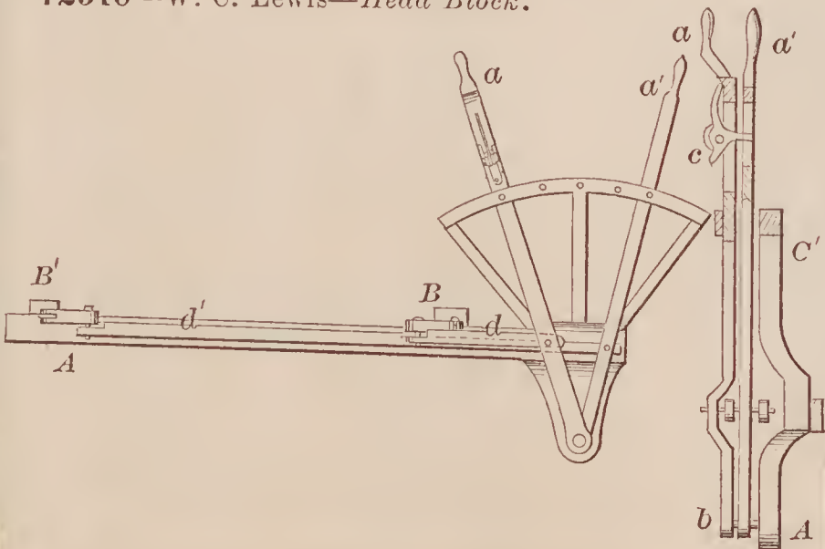
72510—W. C. Lewis—Head Block.
