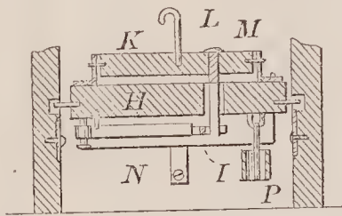
67960—G. Crandell—Churning Machine.
