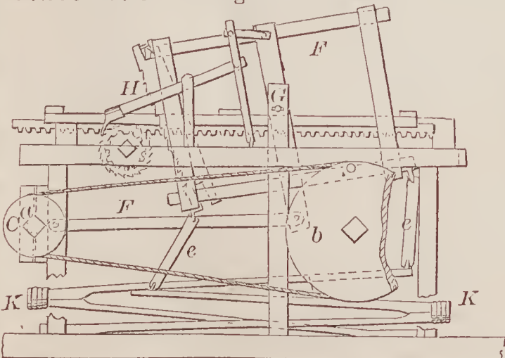
67275—J. C. Delavigne—Saw Mill.
