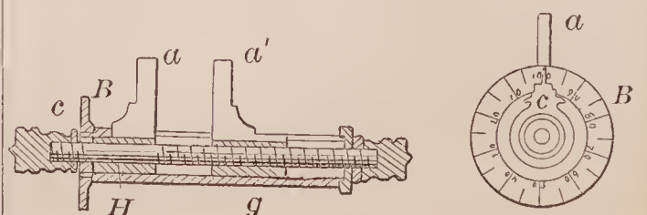
69418—D. F. Elmer— Index Gauge and Calipers.
