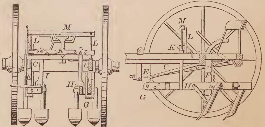
72780—J. T. Baltimore—Cultivator.
