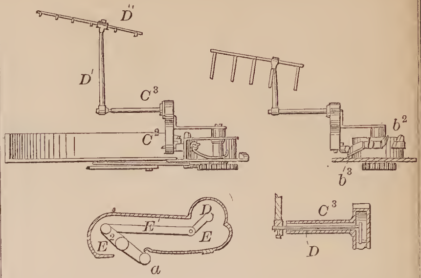
72839—W. F. Goodwin—Harvester Rake.
