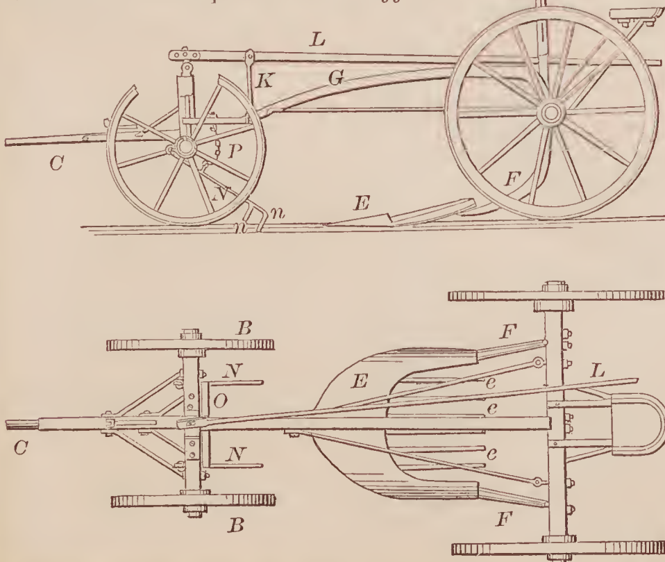
72552—T. W. Shepard—Potato Digger.
