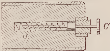
71863—J. M. Fairchild— Self-Adjusting Relay Magnet.
