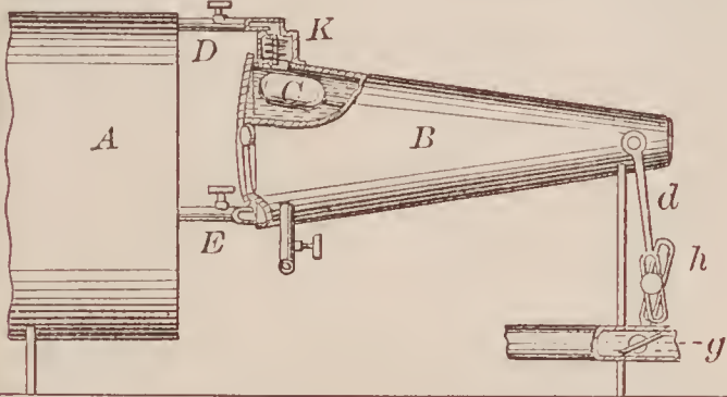
69218—R. J. Jordan—Boiler Water Regulator.
