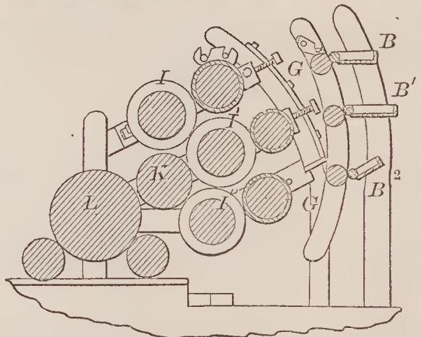
67402—C. F. Bosworth—Plate Lifter.
