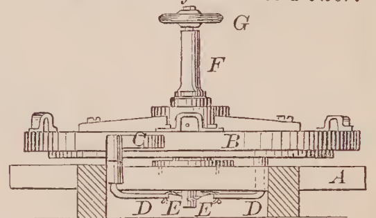
68806—A. D. Tingley—Brake for Horse Power.
