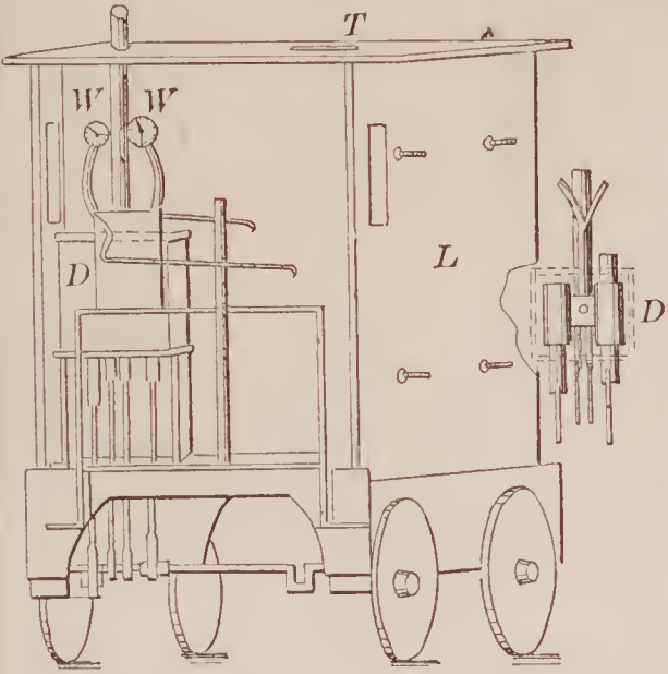
70410—J. Chandler— Telegraph Clock.
