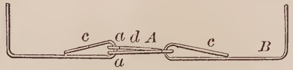
69275—R. D. Turner—For Ageing and Refining Wines and Liquors.
