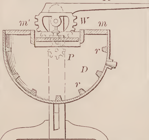
72052—J. Q. Leflingwell—Washing Machine. II
