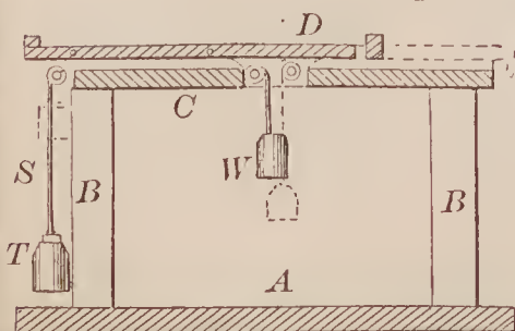
68137—R. V. Whiting—Circular Sawing Machine.
