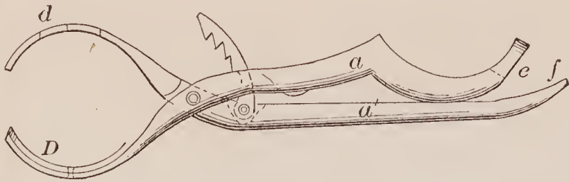
69897—A. Broadnax—For Rendering Lard and Tallow.
