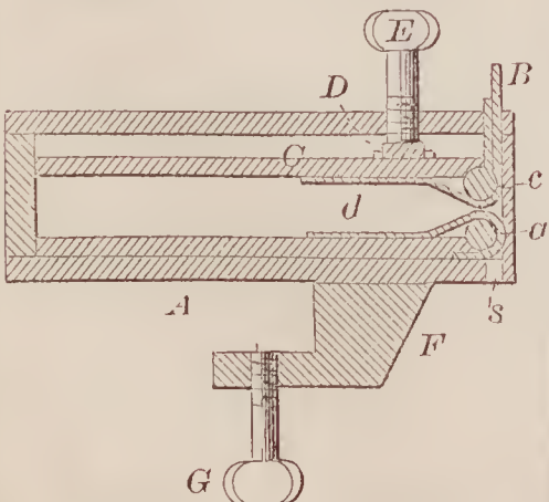
67169—C. F. Dean— Knife Cleaner.
