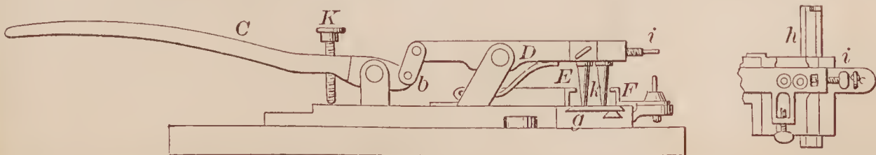
69031—Schindler & Metzger—Punch.
