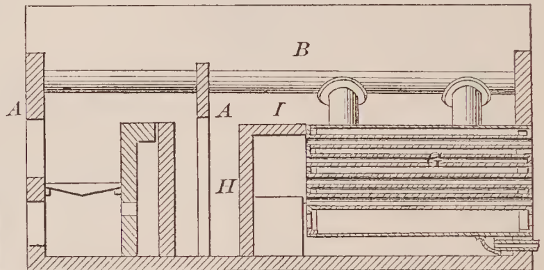
70790—C. T. Boardman—Setting Steam Boilers.
