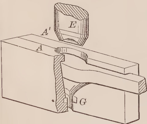
68187—H. M. Hamilton—Die for Forming the Eyes of Picks.
