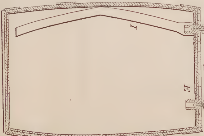
70414—T. R. Cook— Lining Barrels with Sheet Metal
