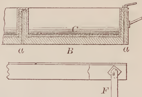
69831—L. Mooney—Kneeling Case for Churches.
