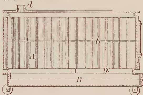
72145—T. W. Wisner—Stove.
