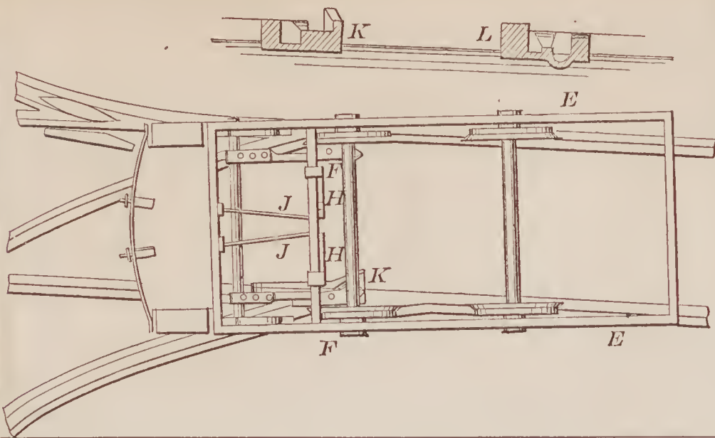
69744—L. Anderson— Saw Mill.
