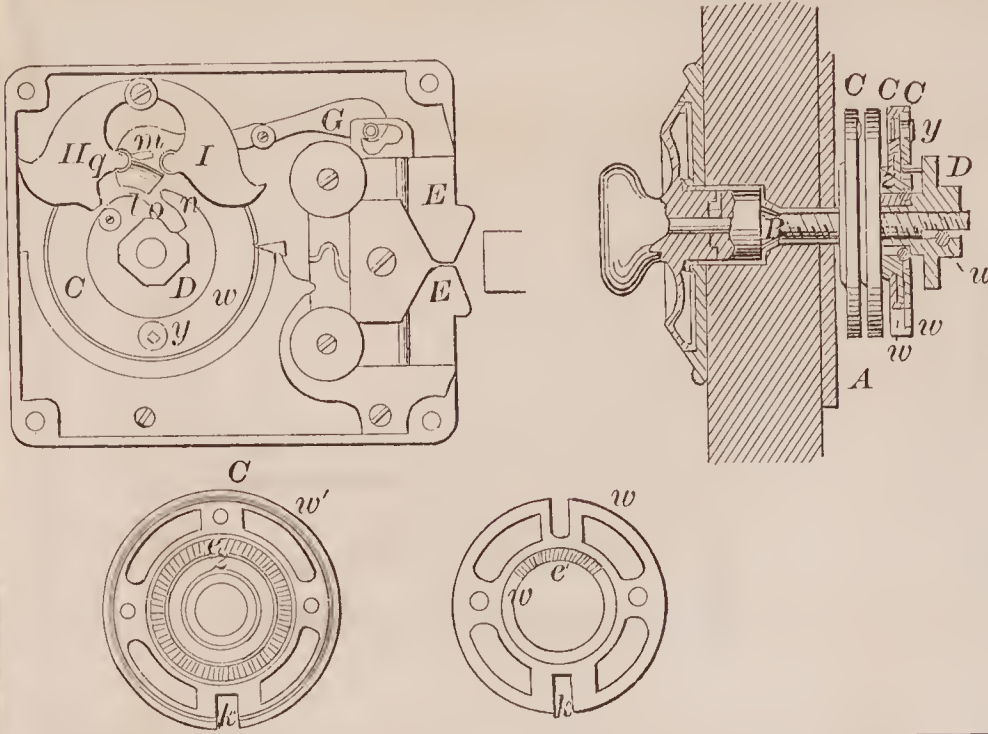
71373—C. Flesch—Permutation Lock.
