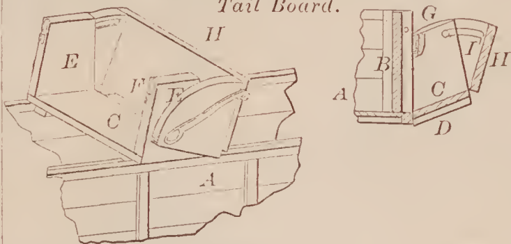
68766—C. Matheny—Wagon Seat, Manger and Tail Board.
