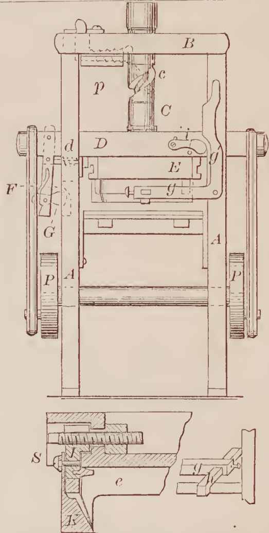
70481—E. M. Stevens—For Cutting Boot and Shoe Soles.
