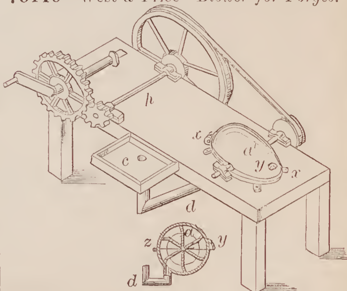
70140—West & Price—Blower for Forges.
