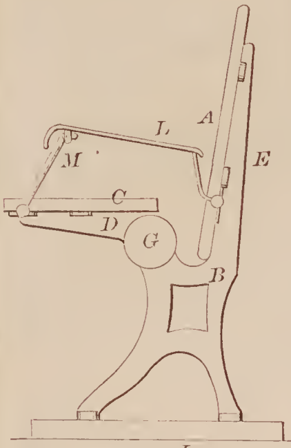
67107—F. J. Dibble— Folding Seat and Arm.
