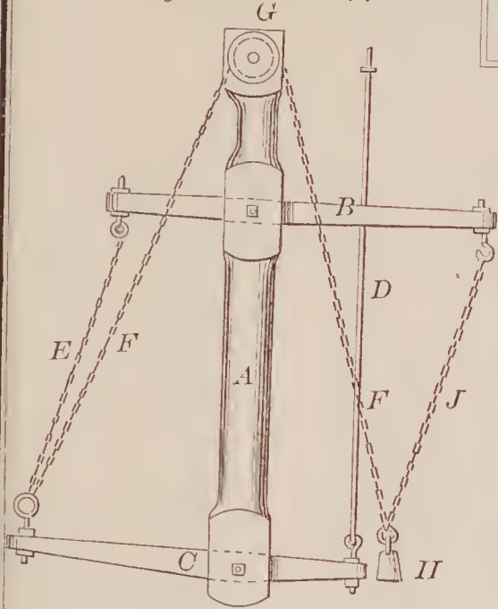
68495—J. Eddy— Steam Engine Governor.
