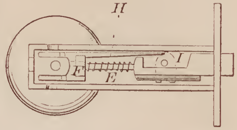
70860—E. King— Door Latch.
