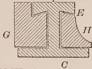
70606—F. Pidjeon—Rail Clamp Joint.
