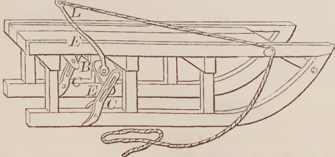
67838—J. Ast—Sleigh Brake.
