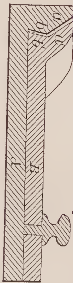
70996—S. S. Gray— For Moulding Collars.
