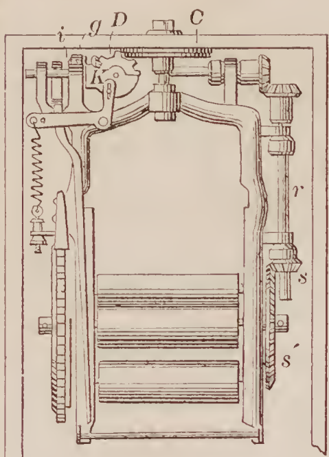
72115—J. Teachout—Rotary Take-up for Knitting Machines.
