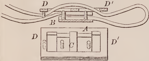
71118—J. R. Ashley—Carriage Spring.
