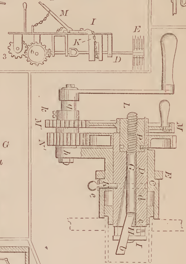
72927—W. B. Smith— Boiler Tube Cutter.
