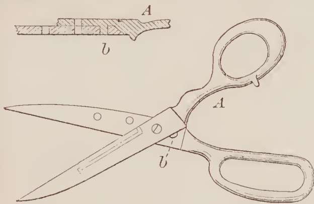
69960—W. B. Barnard— Scissors and Shears.
