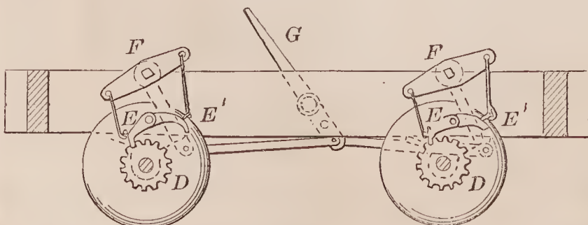
70235—A. Z. Long—Car Brake.
