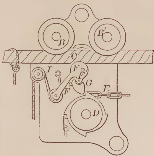
68193—W. H. Hawley—Elevating Block.
