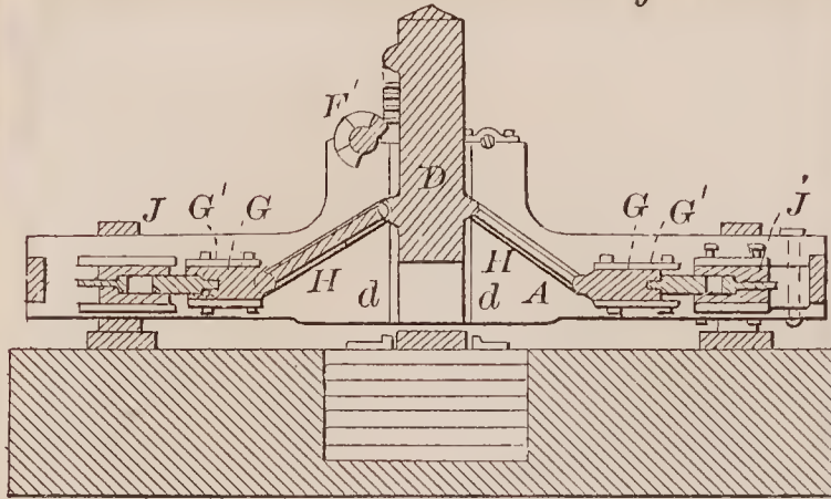
72152—A. Alexander—Bolt Making Machine.
