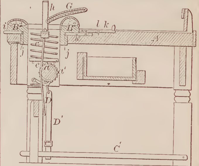
69334—B. Gantner— Shoemakers' Bench.
