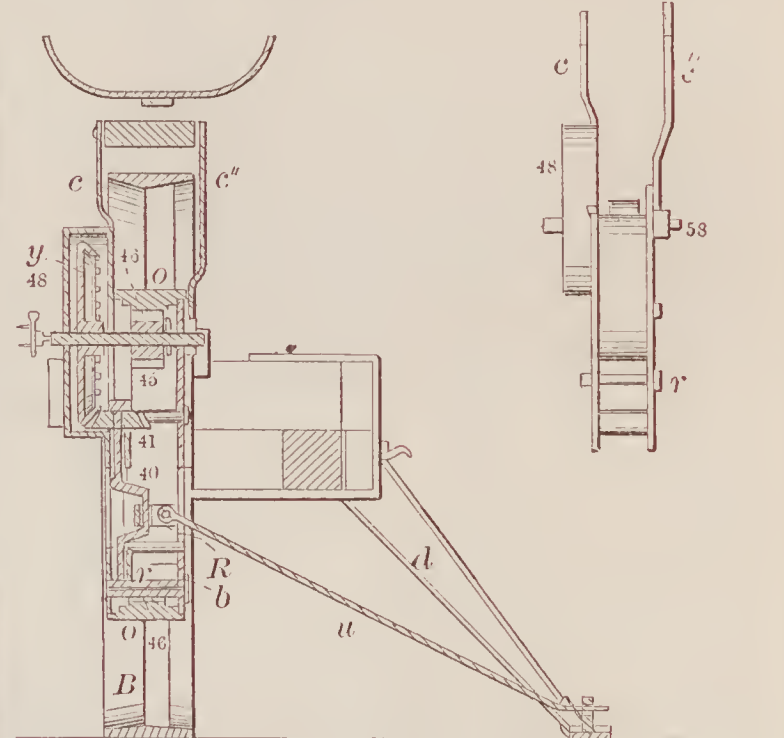
67213—N. Petre—Lock Latch.
