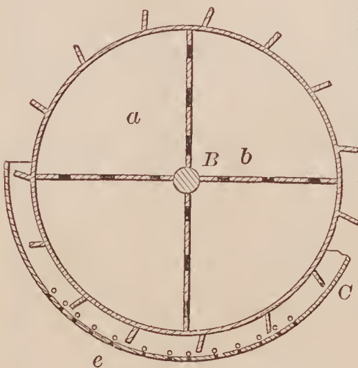
72585—E. H. Ashcroft—For Washing Sheep Skins.
