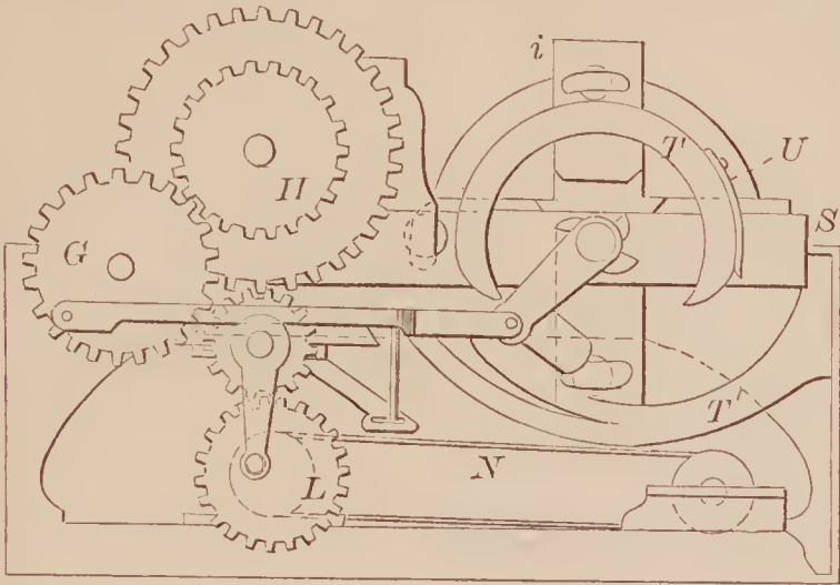
72883—M. C. Motch—Rotary Brick Machine.
