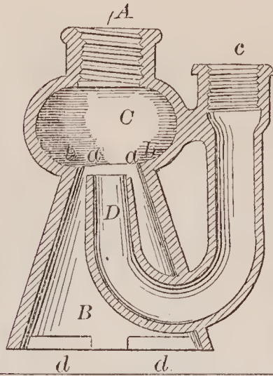
67413—N. L. Chappell—Steam Ejector.
