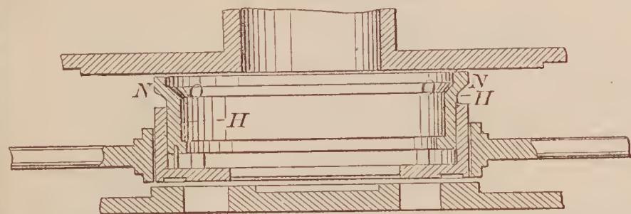
68932—Adams & Parson—Slide Valve.
