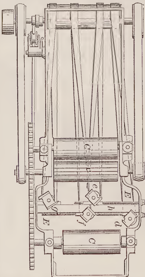
72619—B. Fitts—Planing Machine.
