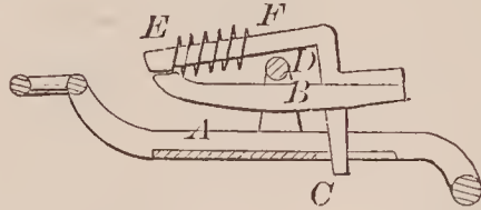
68757—C. C. Lawrence— Thill Coupling.
