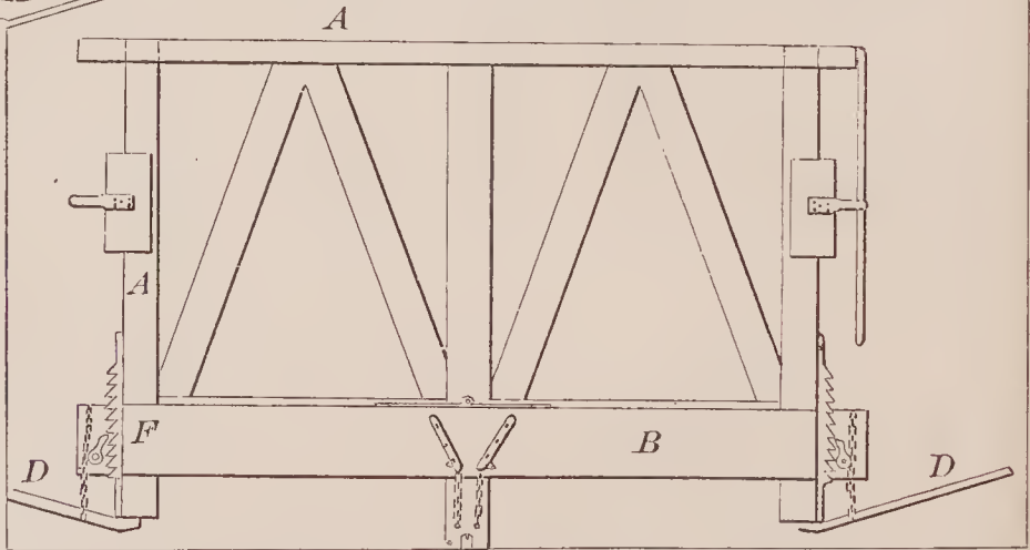
69329—C. T. Faber—Lid Support for Pianos, Desks, &c.
