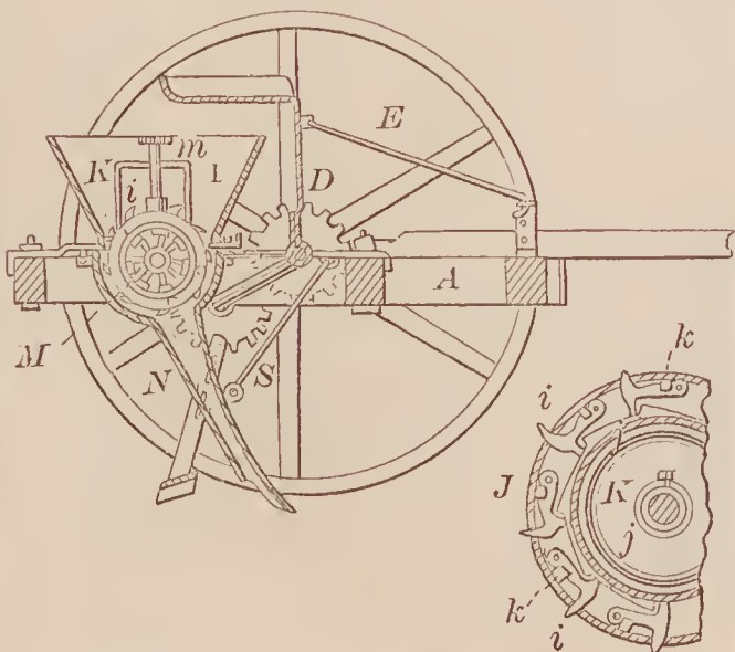
66924—Wilcox & Caldwell—Cotton Seed Planter.
