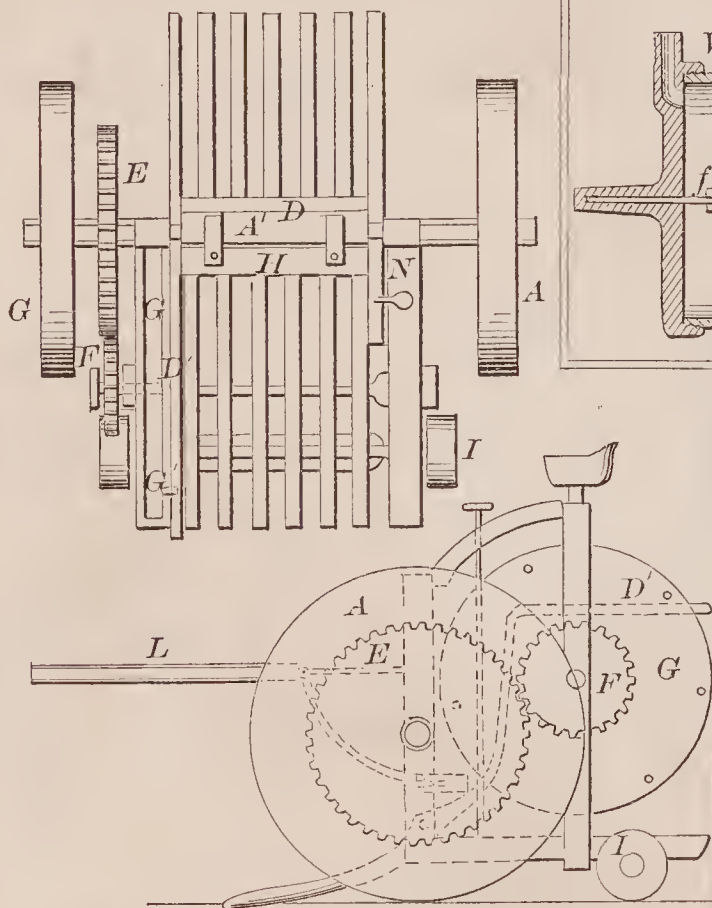
72289—E. V. W. Griffith—Potato Digger.
