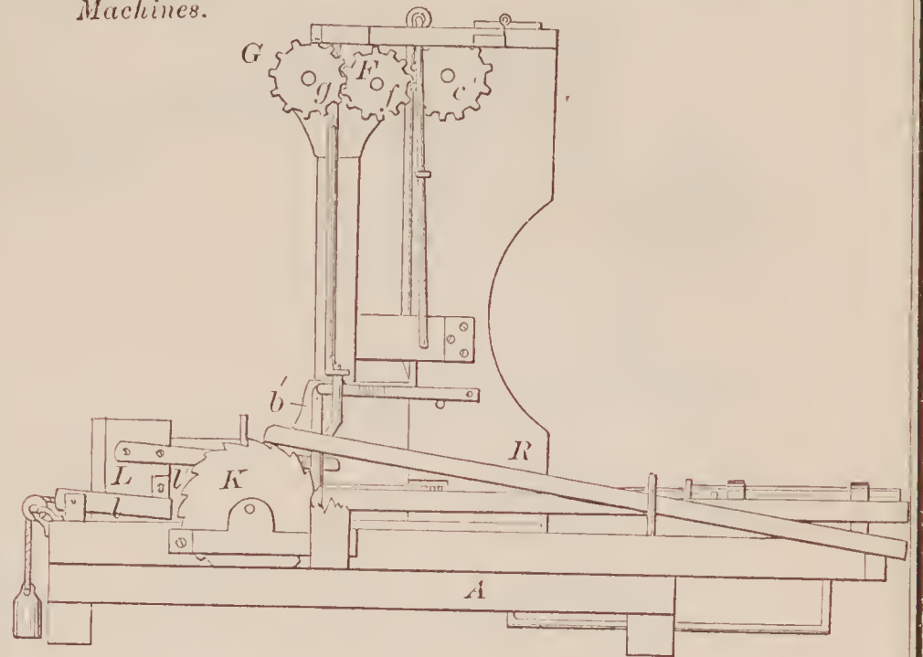
66876—E. B. Olmsted—Packing Apparatus for Envelope Machines.
