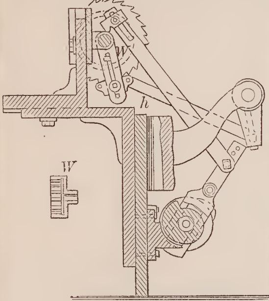
70293—J. Underwood— For Cutting Teeth of Wheels.
