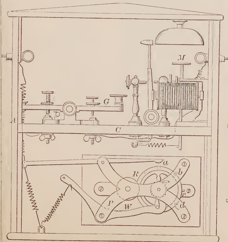
70672—J. M. Fairchild—Fire Alarm Telegraph.
