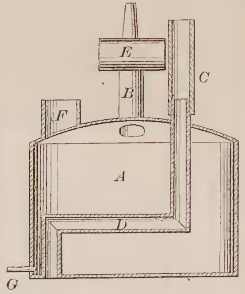
71271—Brady & Sloan— Furnace for Roasting Ores.
