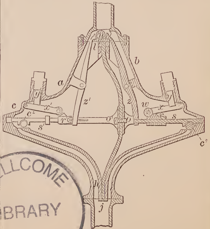
72958—W. Baldwin—Water Meter.
