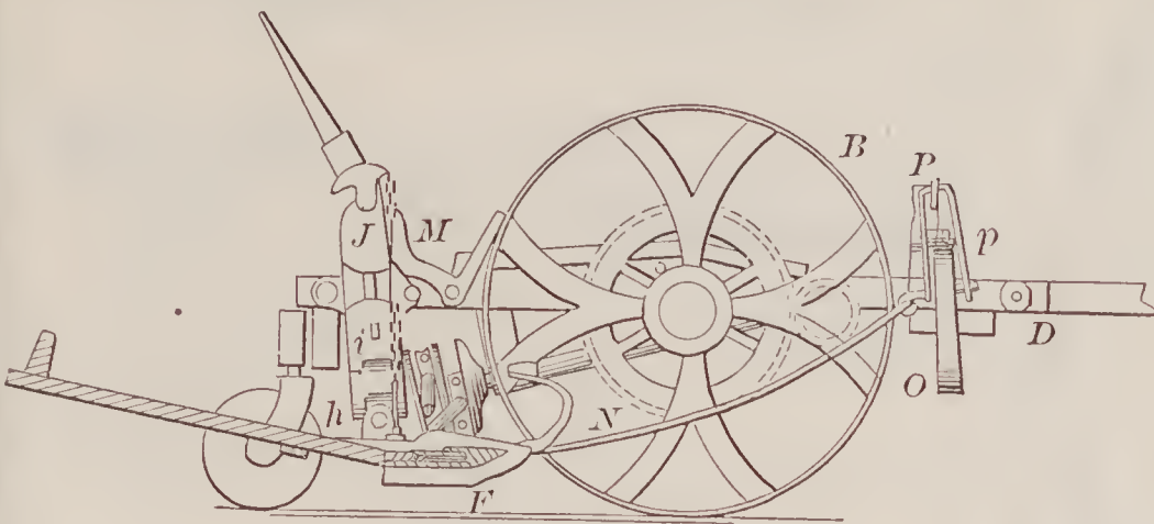
72678—Quick, Opie & Ferrand—Harvester.
