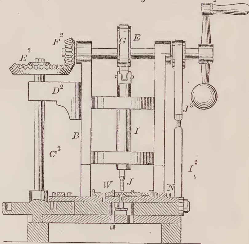
67253—A. S. Blake— For Lining Percussion Caps.
