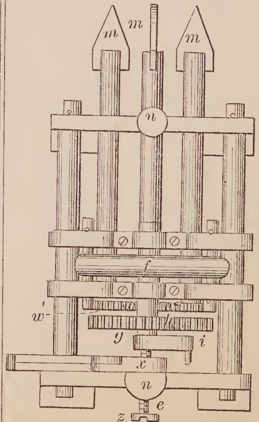
72390—S. Gissinger—Coal Mining Machine.
