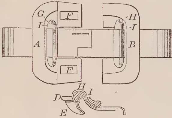
68167—M. D. Cheek—Cotton Bale Tie.
