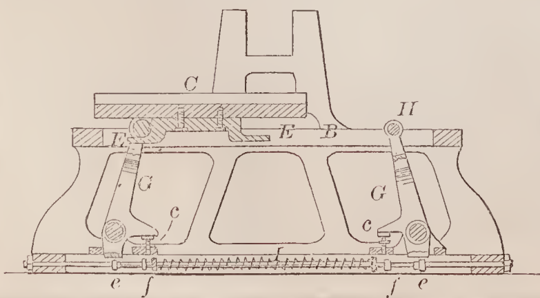
68001—C. Potter, Jr.—Printing Press.
