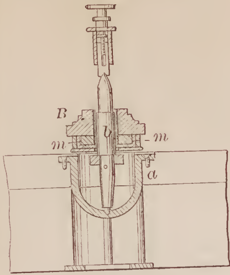
70266—W. Ring— Tram Staff for Grinding Mills.
