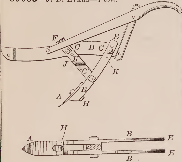
69083—J. D. Evans—Plow.
