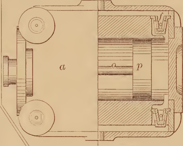
72707—C. Whittier— Slide Valve.
