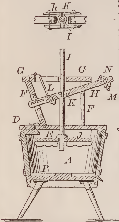
67499—J. B. Coffin—Washing Machine.
