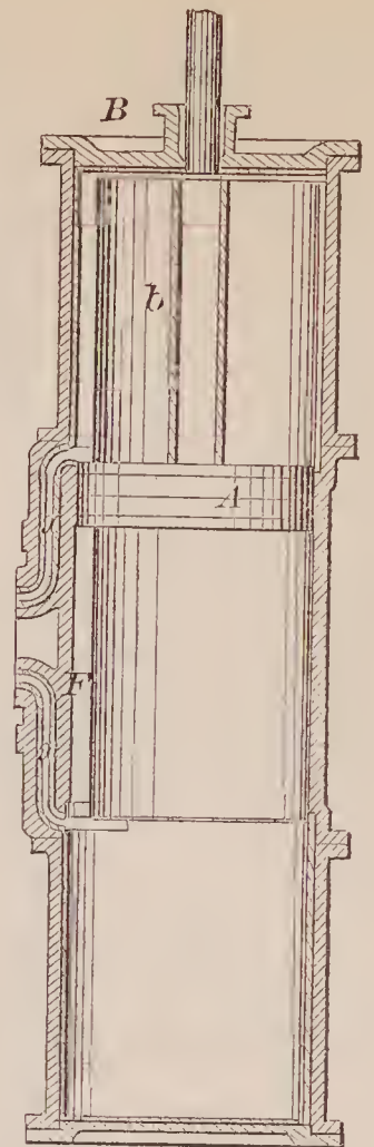
70707—C. E. Emery—Steam Engine.
