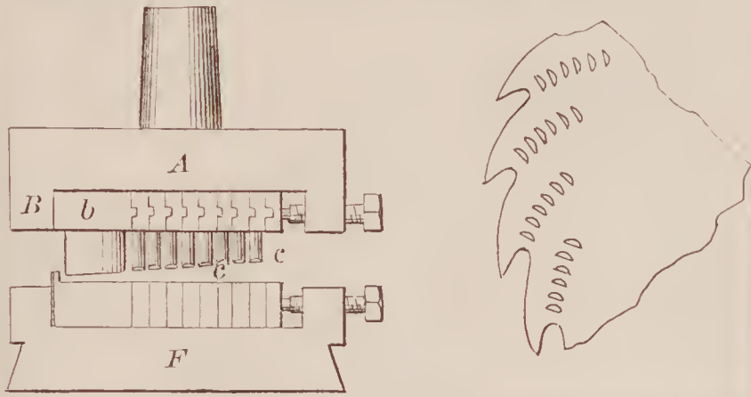
71473—J. E. Emerson—For Punching Saw Teeth.
