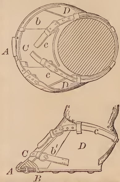
72594—T. B. Bishop— Horse Shoe.
