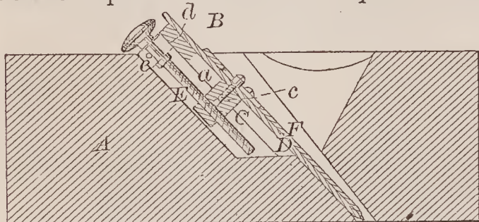
67458—Spooner & Johnson—Carpenter's Plane.
