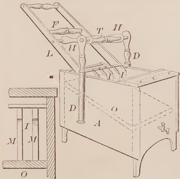
72316—J. Mitchell—Washing Machine.
