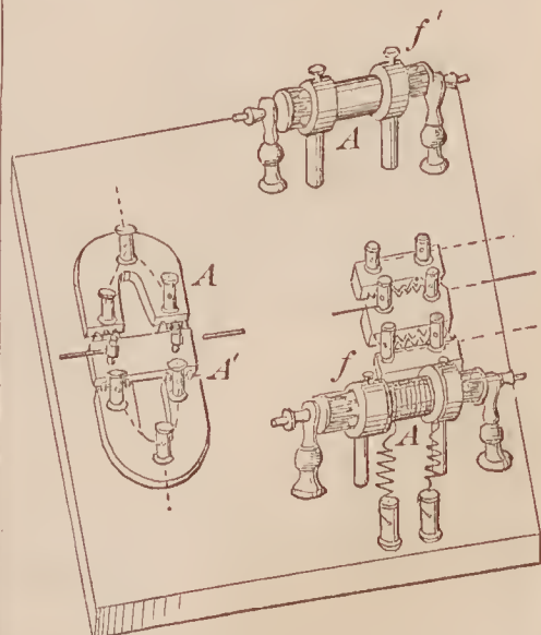
68407—A. Barbarin—Lightning Arrester.
