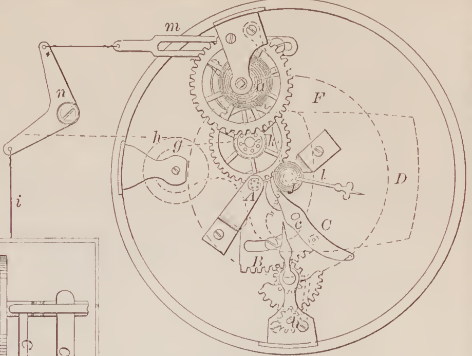
69648—A. & E. Fontaine— Annunciating Fire Alarm.
