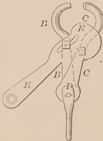
72866—M. A. Lanagan— Boat Detaching Apparatus.
