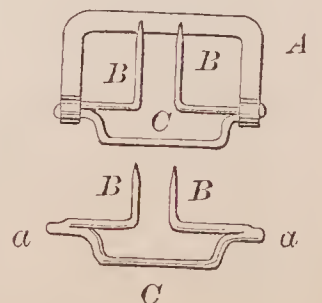
70944—E. C. Blakeslee—Buckle.
