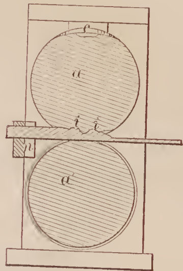
72512—M. Loughran—For Rolling Clevis Blanks.
