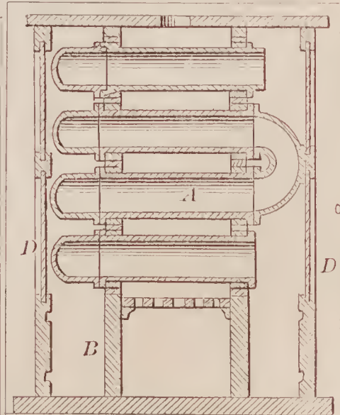
72056—R. Long—Furnace.
