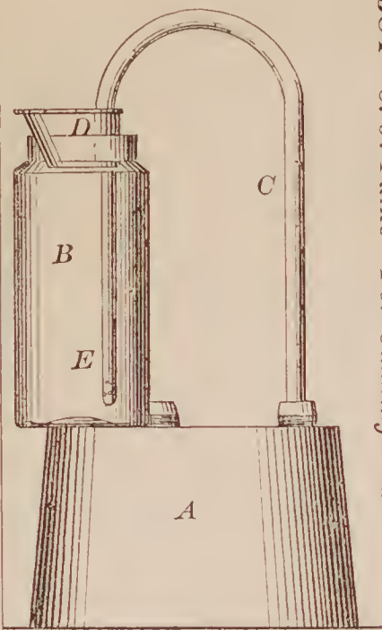
68386—Potter & Crane—Cotton Elevator.
