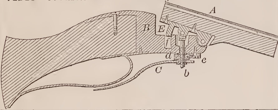
71149—J. Elson—Breech-Loading Fire Arm.
