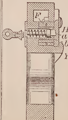
68436—E. Hamburger—Lock for Car Seats.
