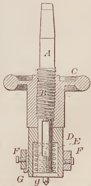
67194—W. H. Menhall— Tube Hole Cutter.
