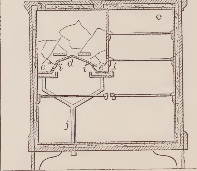
69812—J. C. Jewett—Refrigerator.
