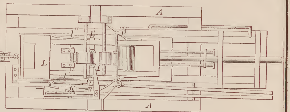
66875—G. H. Ober—For Tenoning Spokes.
