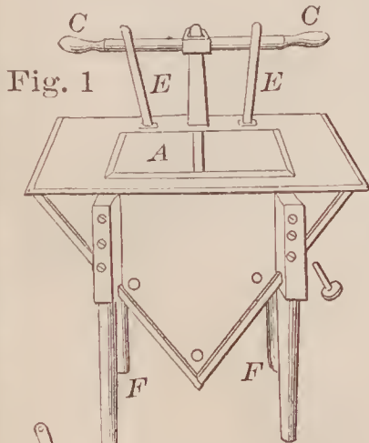
68100—M. B. Mills—Churn.
