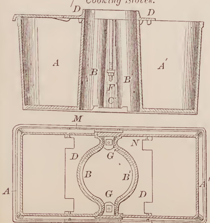
70206—Harris & Zoiner— Water Reservoir for Cooking Stoves.
