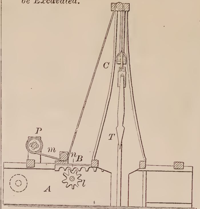
68411—W. H. Butler—For Loosening Earth to be Excavated.
