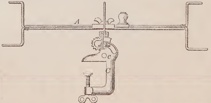
69579—J. Foreman—Reel.
