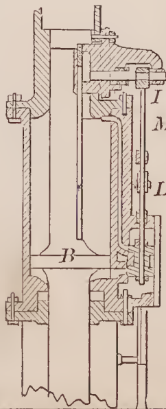
70369—W. & C. Sellers—Value Gear.
