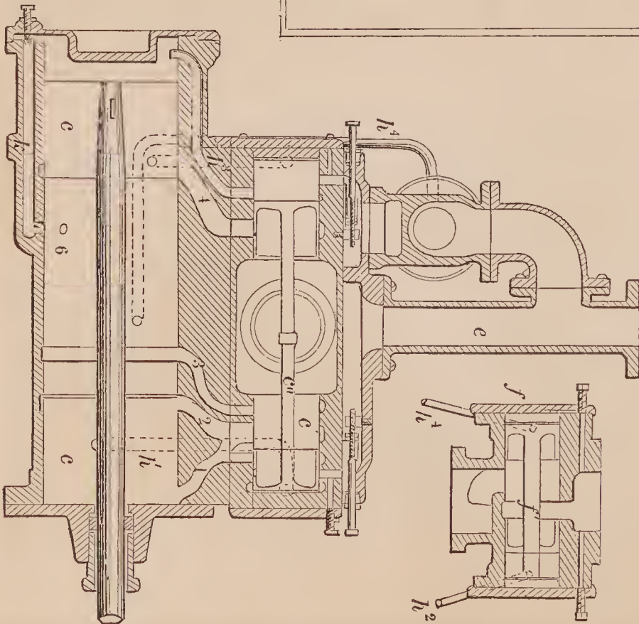
72714—W. Ball— Steam Engine.
