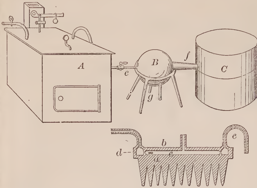
68118—S. C. Salisbury— Converting Iron and Steel.
