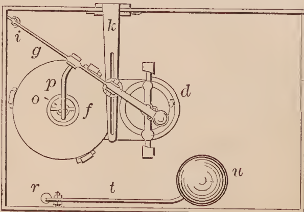
72807—R. H. Cooper—Window Sash Stop
