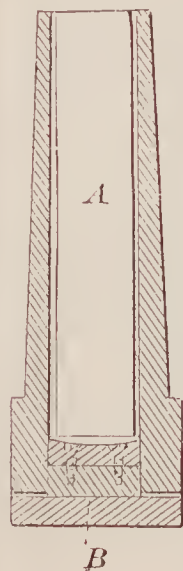
67171—H. Dickinson— Mould for Casting Ingots.
