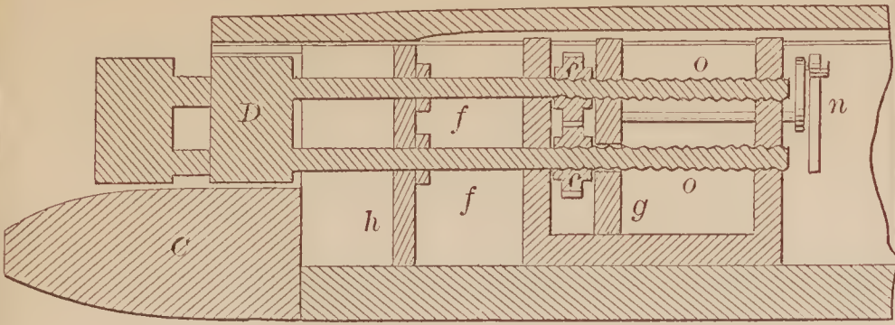
72391—W. Hagerty— Ram for Vessels.
