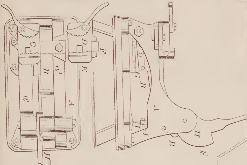
70902—J. J. Rose—For Cutting, Punching and Upsetting Iron.
