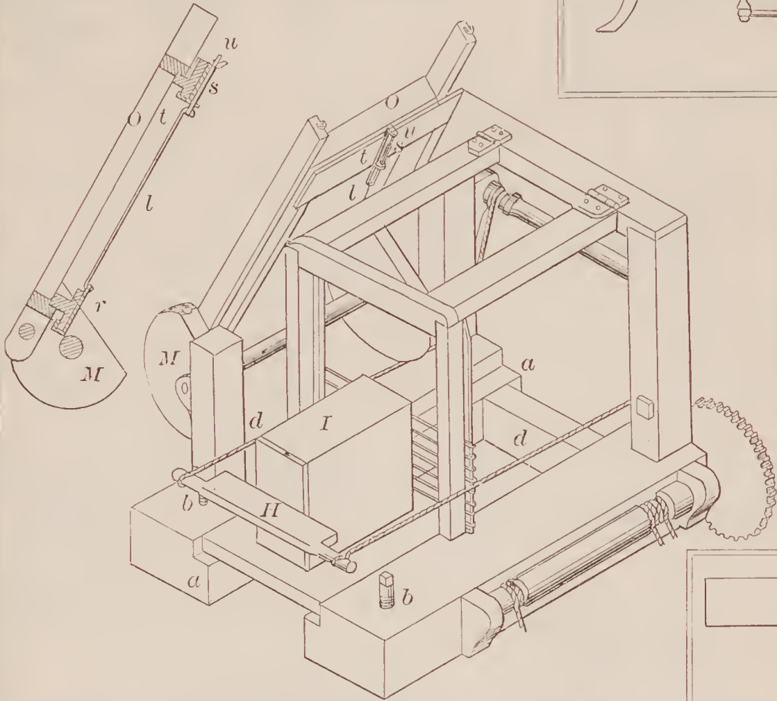
70205—C. H. Hardy— For Cutting Soap.
