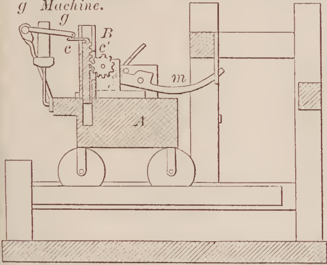
69152—G. W. Young— Carpet Cleaner.
