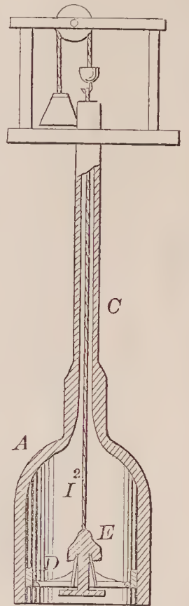
71781—A. Norris—Water Elevator.
