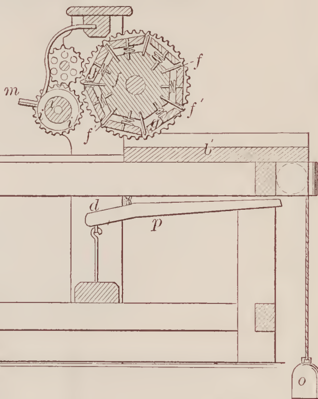
71864—L. Felker— Corn Cake Cutter.
