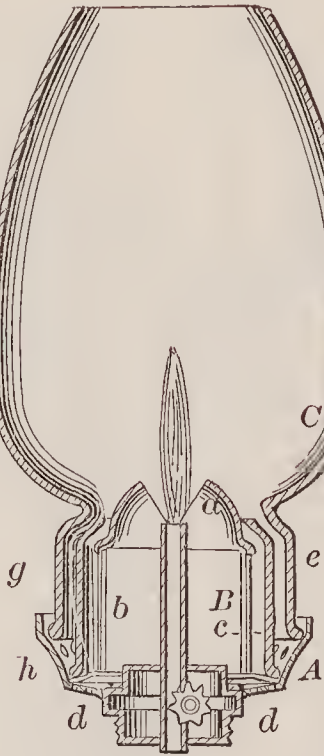
72683—Russell & Clifford— Lamp.
