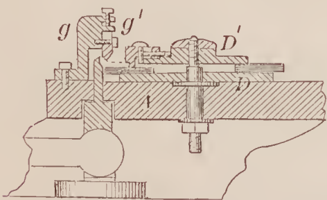
68533—Seger & Smith— Clamp for Hinges.
