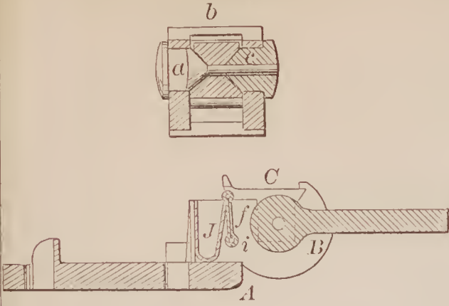
69469—E. M. Naramore— Thill Coupling.
