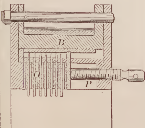
71020—J. J. Kents— Slitting Machine.
