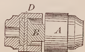
70334—W. P. Haskins—Ball and Socket Joint.
