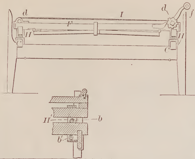
67611—I. P. Tice—Spirit Meter.
