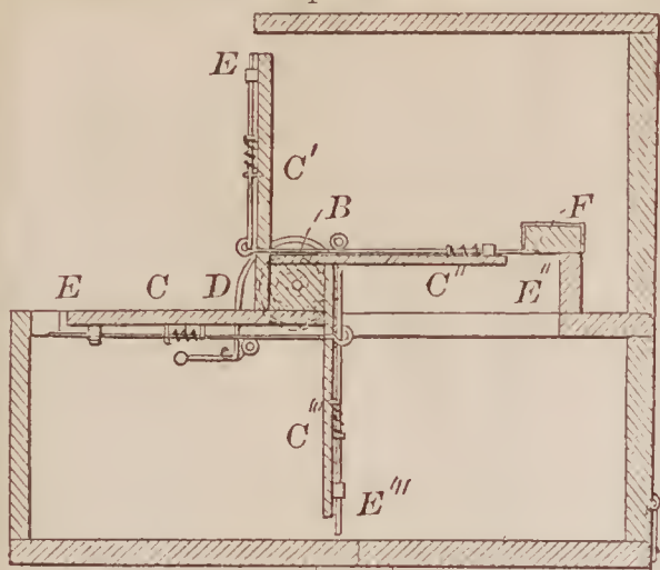
70370—R. Simpson—Animal Trap.
