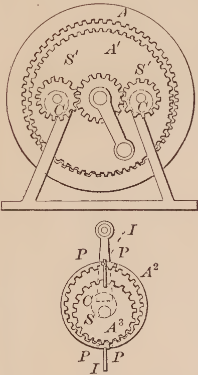
72792—A. W. Browne—Mechanical Movement.
