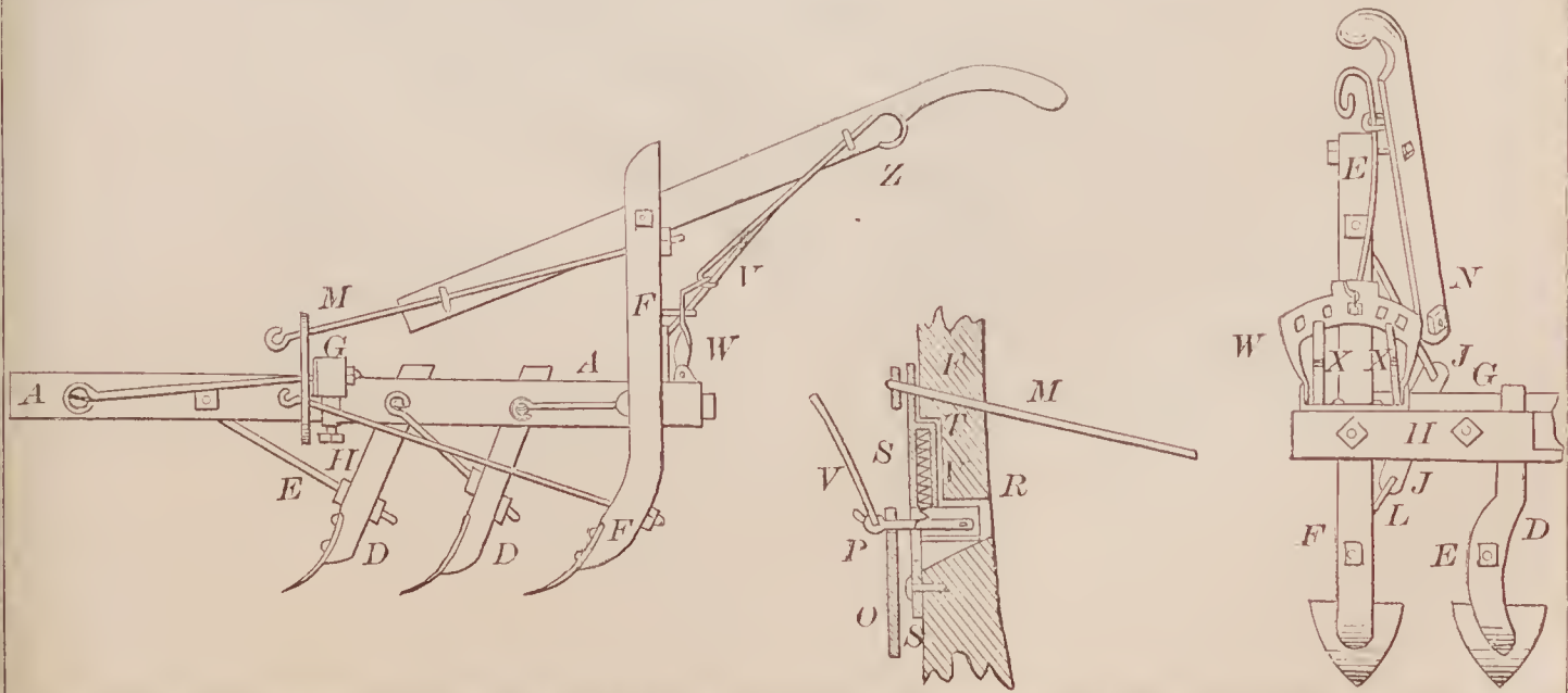
70258—E. W. Pike— Cultivator.
