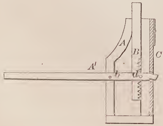
69810—J. Hunt, Jr.—Wagon Jack.
