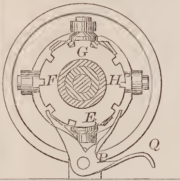
68015—E. Ware—For Propelling Steam Carriages.
