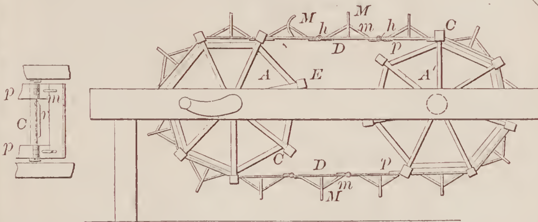
70036—A. B. Smith—Endless Chain Propeller.
