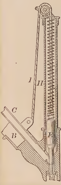
67159—W. Brown—Carpet Stretcher and Tack Driver.
