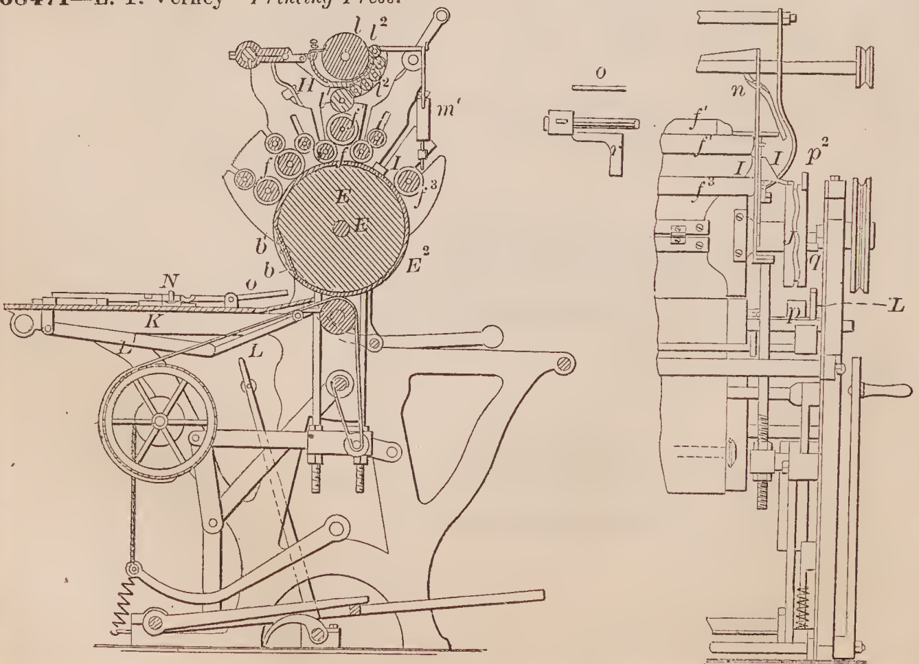
68471—L. T. Verney—Printing Press.
