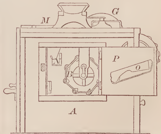
69489—J. Sattison—Grain and Seed Cleaner.
