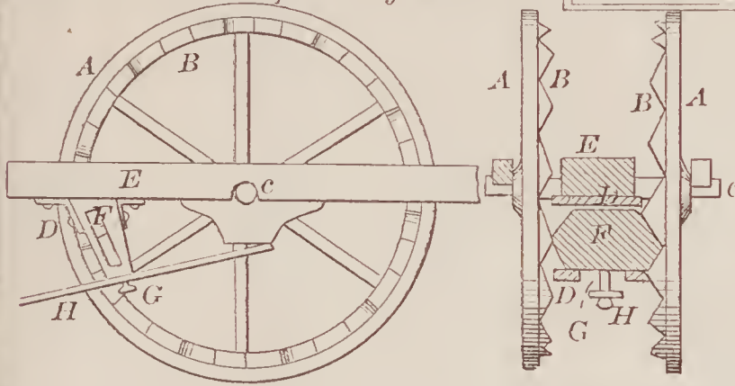
69584—T. & C. Plumleigh— Converting Circular into Reciprocating Motion.
