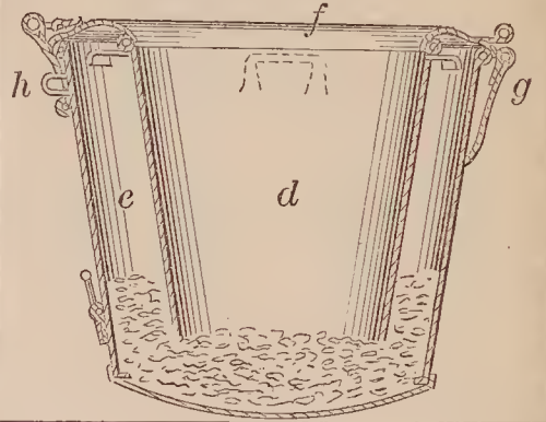
72935—R. C. Sturges—Feed Bucket.
