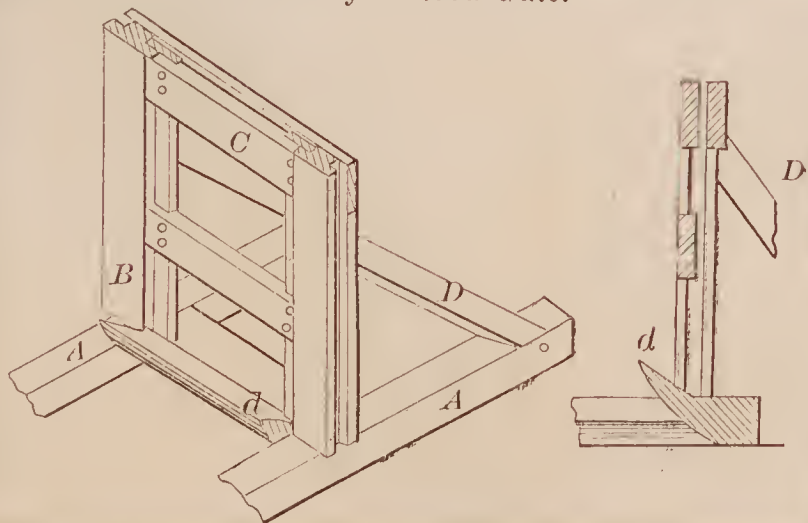
68767—C. B. McKinney—Flood Gate.
