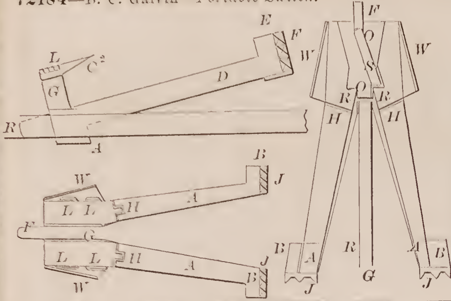
72185—B. C. Galvin—Railway Switch.
