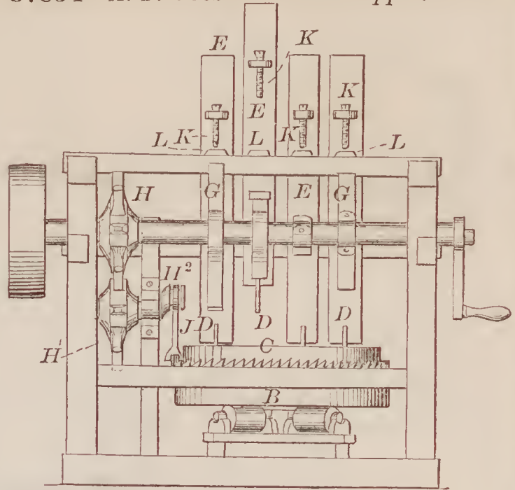
67853—Dodge, Stevenson & Stevenson—Harvester Rake.
