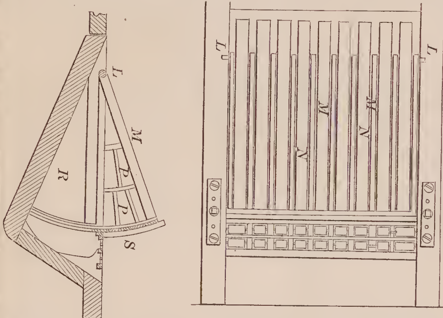
68832—A. E. Bigelow— For Dressing Weavers' Harness.
