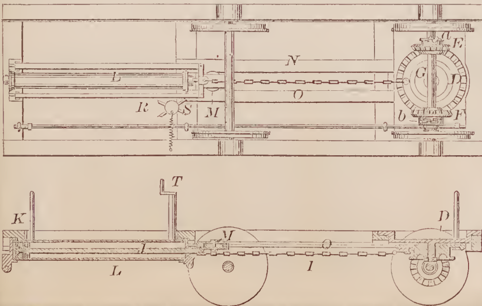
70814—A. G. Crossman— Starting and Stopping Cars.
