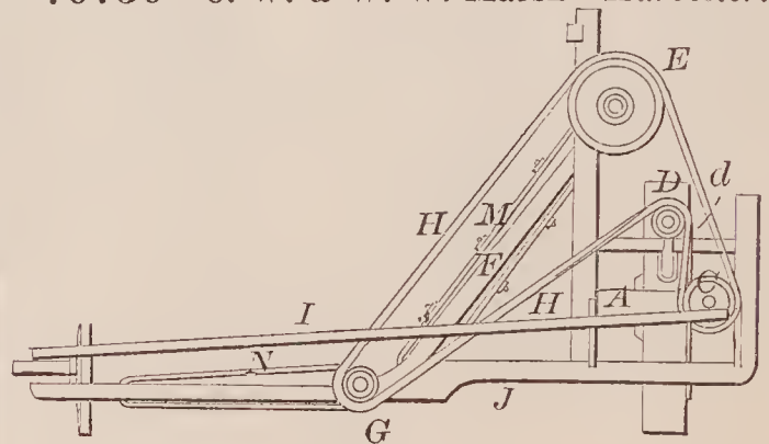
70730—C. W. & W. W. Marsh— Harvester.
