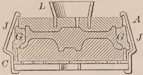
70290—W. R. Thomas— Flask for Casting Car Wheels.
