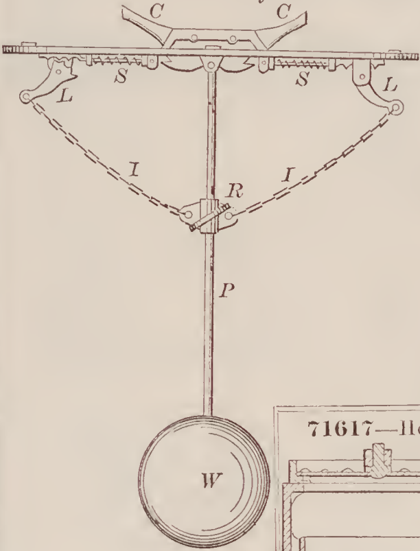
71615—L. Hill—Cleat for Sail Boats.
