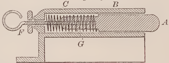
70149—G. F. Atkinson—Spring Bolt for Doors.
