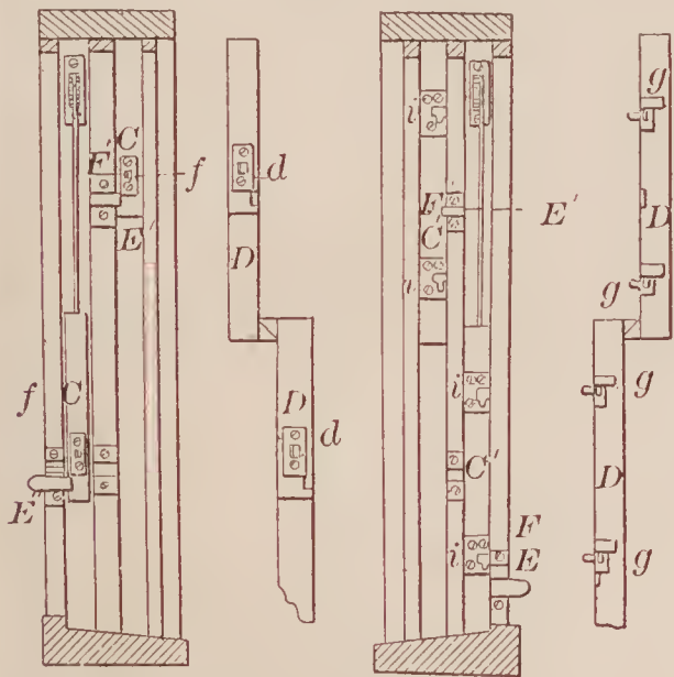
69046—R. Thomas—Window Sash.
