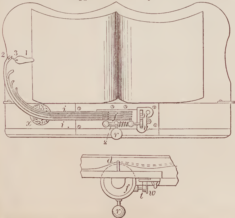
69770—C. C. Clapp—For Turning the Leaves of Books.
