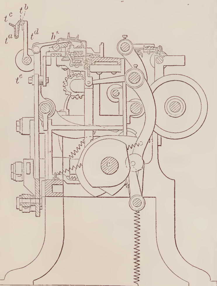
67727—W. Cotton— Knitting Machine.
