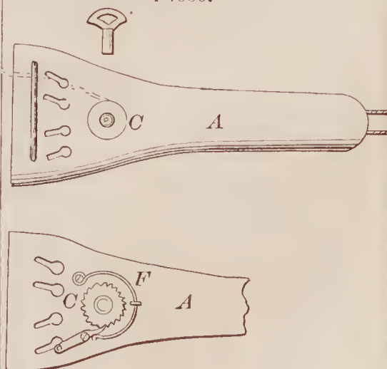
72121—J. Thoms—Violin Tail Piece.
