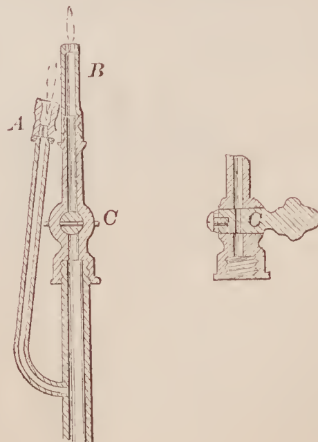
70272—E. P. Russell— Lighting Street Gas Burners.
