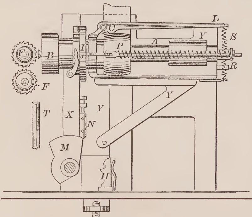
71908—E. S. Pierce— For Shaving and Slotting Screws.
