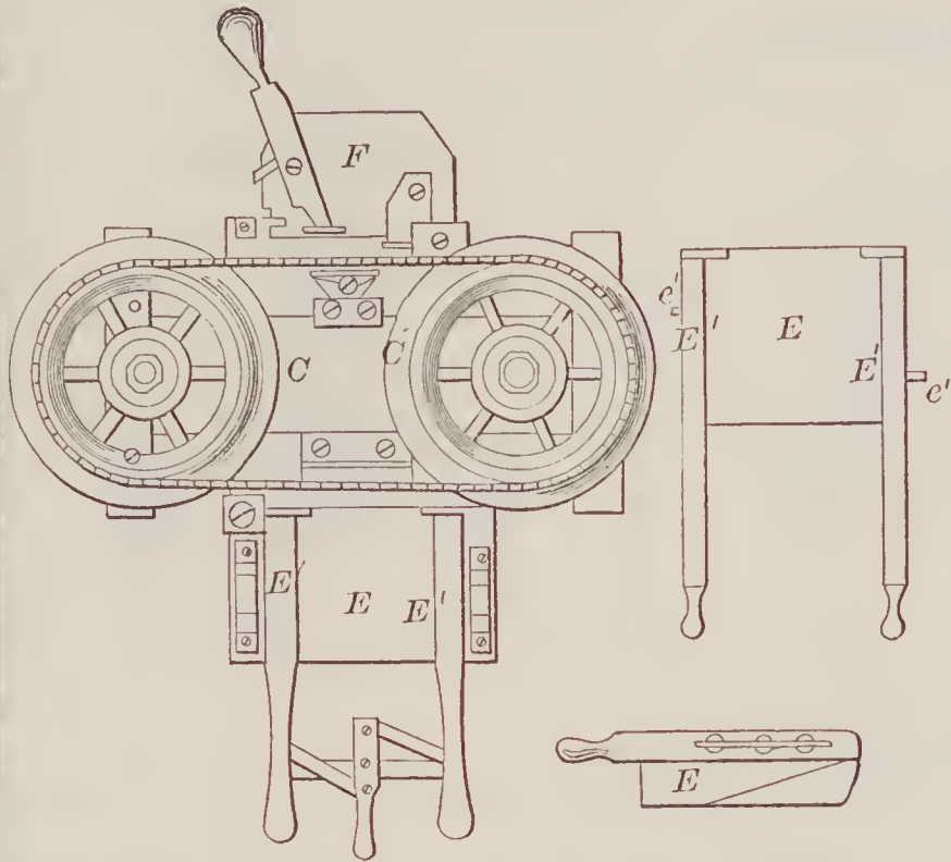
72639—C. J. Holman— For Sawing Barrel Heading.
