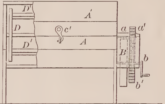
69324—W. Davis—Churn.
