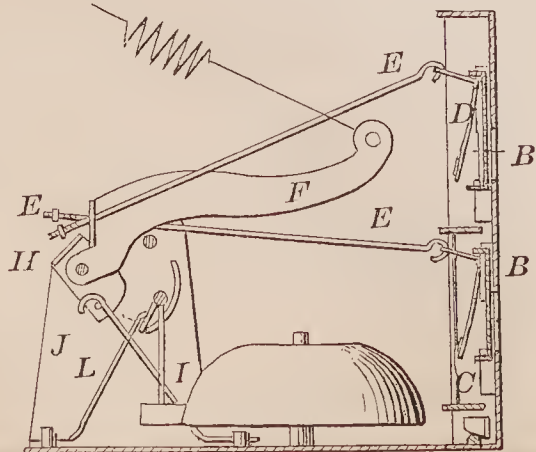
70552—Gross & Yingling—Annunciator.
