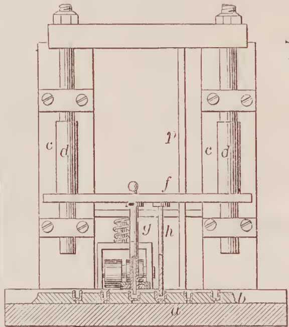
67192—E. L. Hall— Locomotive Head Light.
