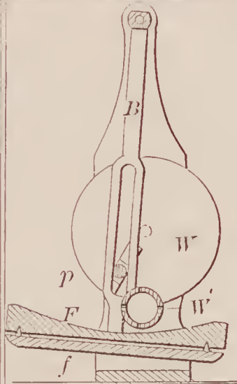
72053—F. C. Levalley—Door Fastener.
