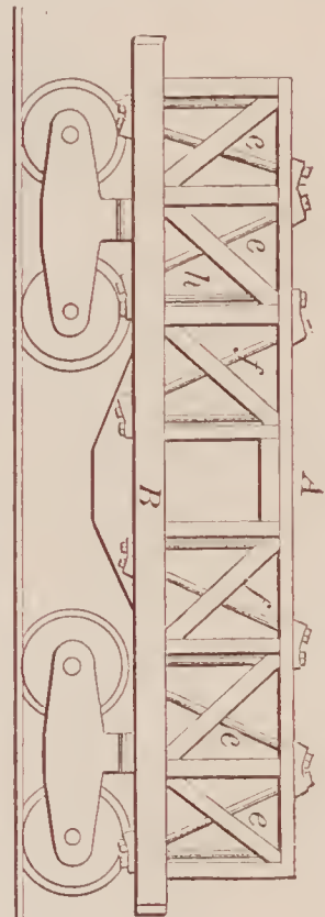
68619—J. Foreman—Railway Car.
