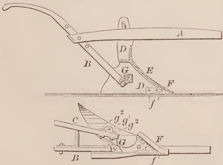
66774—B. F. Avery—Plow.
