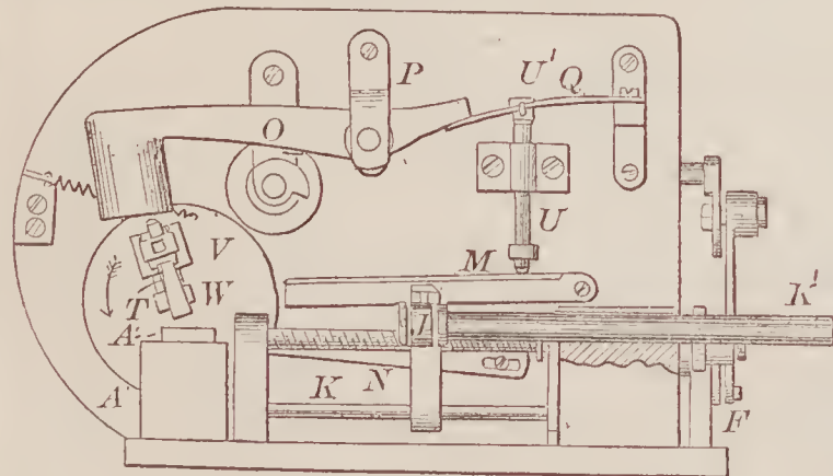
67374—S. A. Sutton—For Cutting Files.
