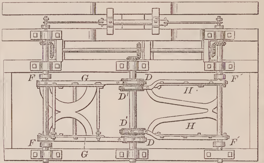
70131—J. Swan—Car Coupling.
