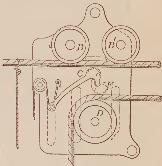
68874—W. H. Hawley— Elevating Block.
