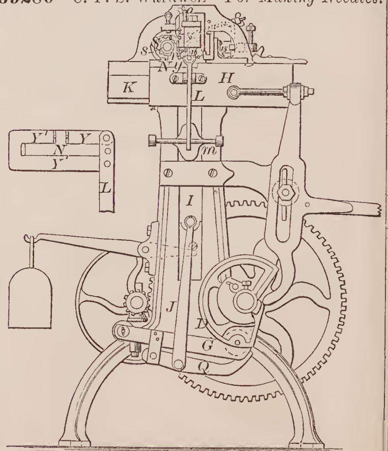
69280—C. P. S. Wardwell—For Making Needles.
