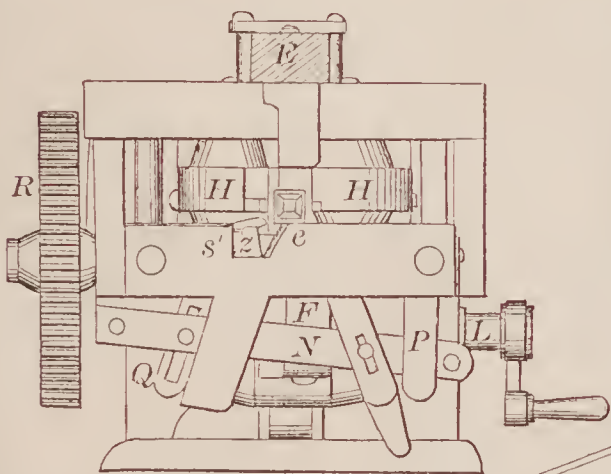
70374—A. St. Louis—Horse Shoe Nail Machine.
