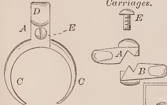
69291—F. Wood—Securing Whip Soekets to Carriages.
