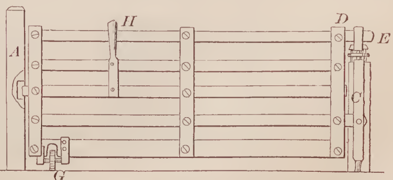
69509—A. Tandy—Gate.
