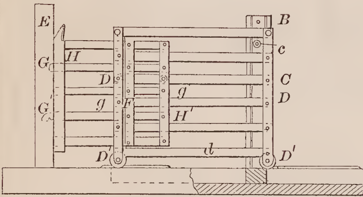
70626—L. M. Scothorn—Gate.
