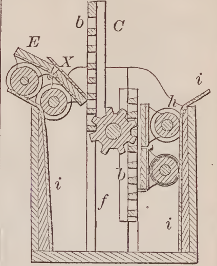
67734—H. Disston—Hardening and Straightening Steel Blades.
