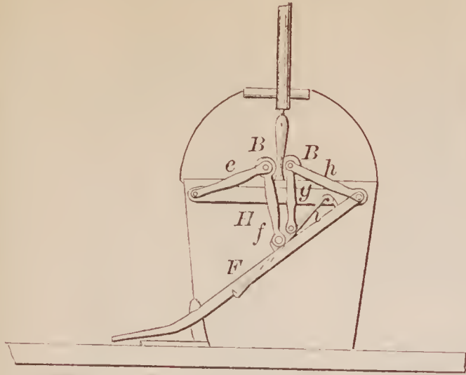
70694—A. L. Carrier—Attaching Ferrules to Handles.
