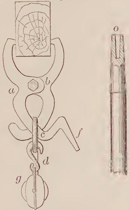
70239—G. D. Melotte—Clutch for Hay Forks.
