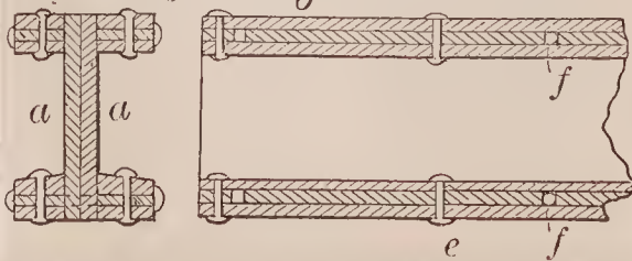
68267—Walters & Shaffer—Pile for Wrought Iron Beams or Girders.
