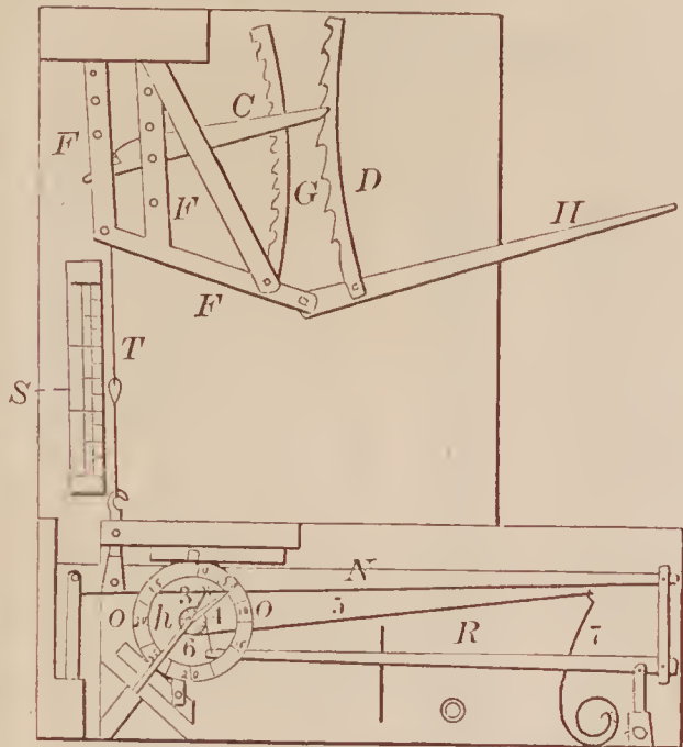
67144 —H. T. Stanard— For Applying and Measuring Forces.
