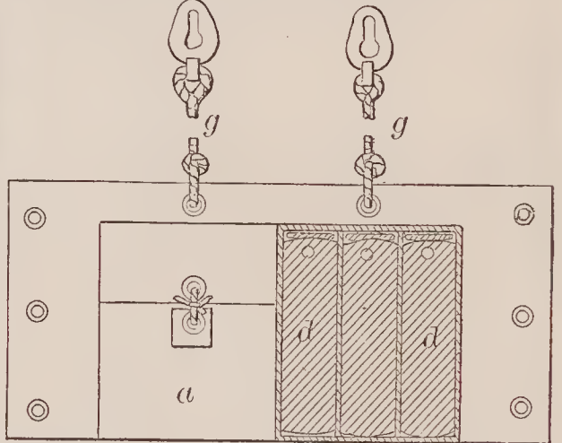
67874—D. Hale—For Attaching Weights to Submarine Armor.
