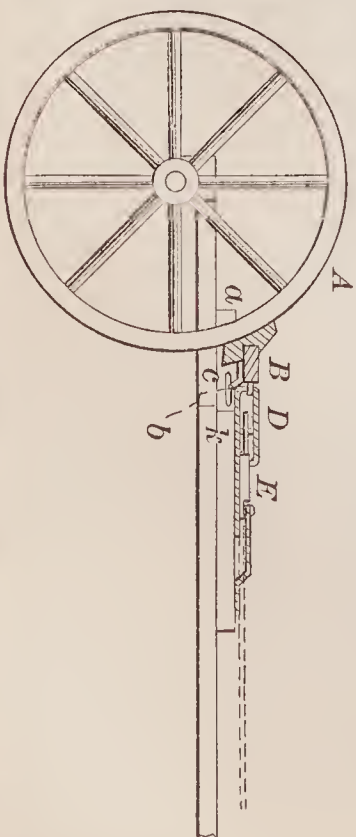
69886—L. E. Woodard—Wagon Brake.
