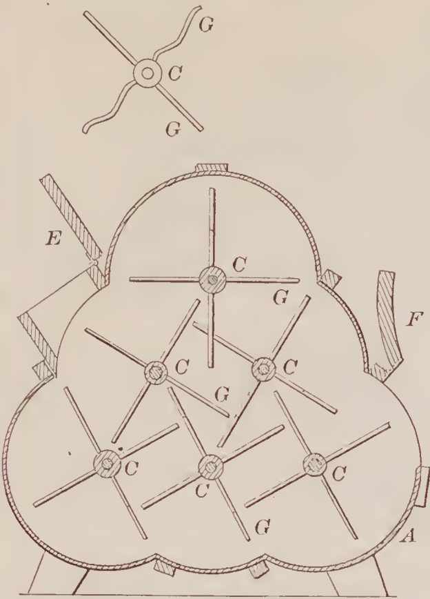
67561—J. McDonald—Brick Machine.
