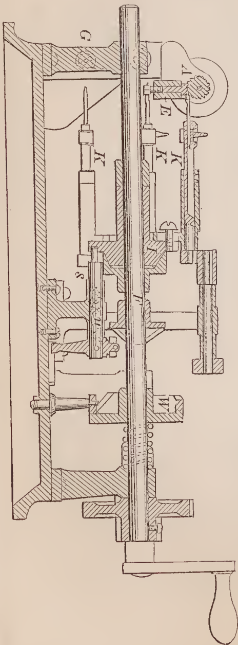
70677—W. Aiken—Needle Machine.
