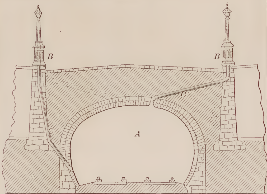
72142—H. B. Willson—Ventilating Tunnels.
