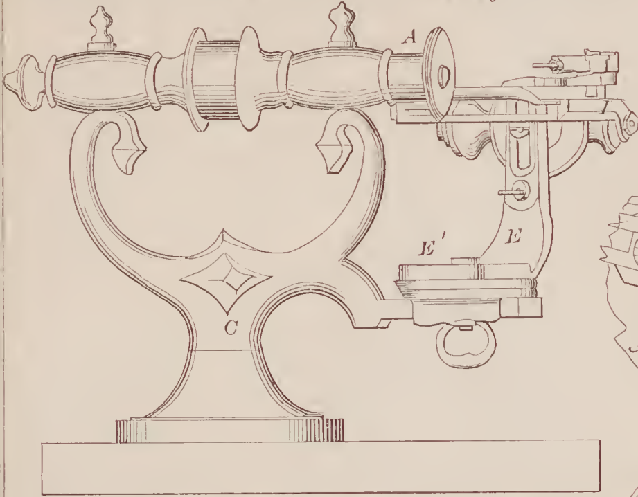
70951—I. S. & C. N. Brown— For Grinding Saw Teeth.
