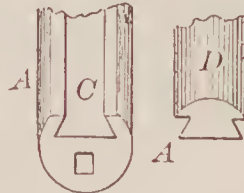
67371— W. H. Stichel— Prop Block for Carriage Tops.
