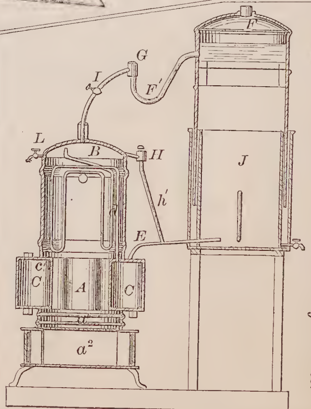
70477—W. M. Sloane— Gas Generating Furnace.
