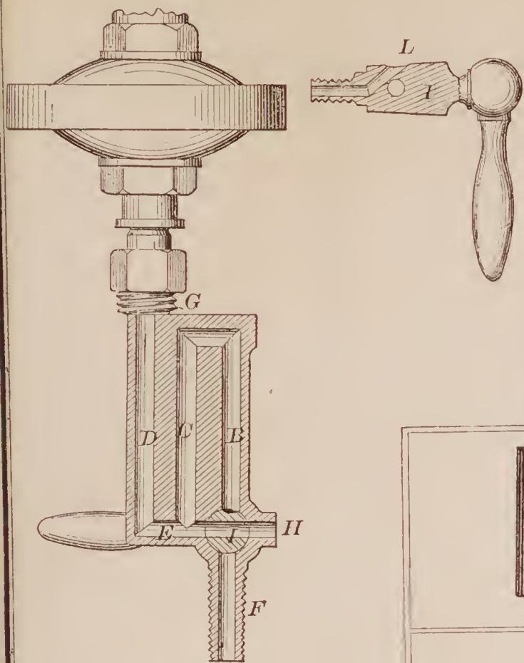
69057—C. A. Wilson—Steam Pressure Gauge.
