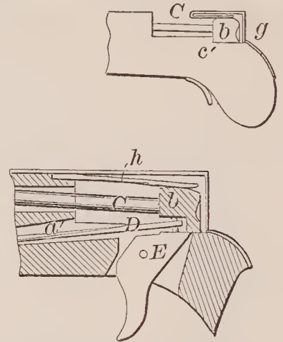
71732—F. Fuller—Toy Gun.
