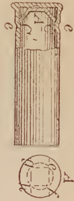
68960—J. F. Cranston—Priming Metallic Cartridges.
