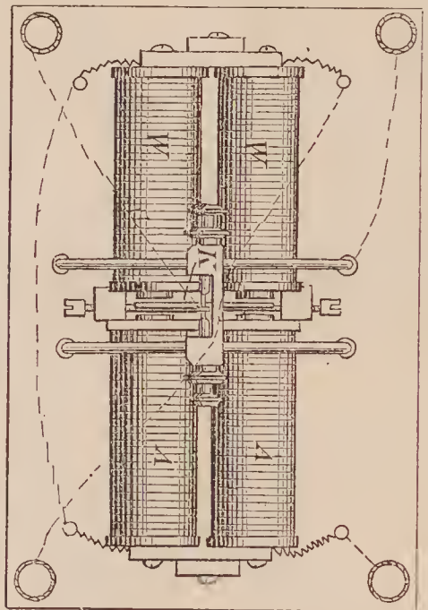
67160—W. G. Brownson—Relay Magnet.
