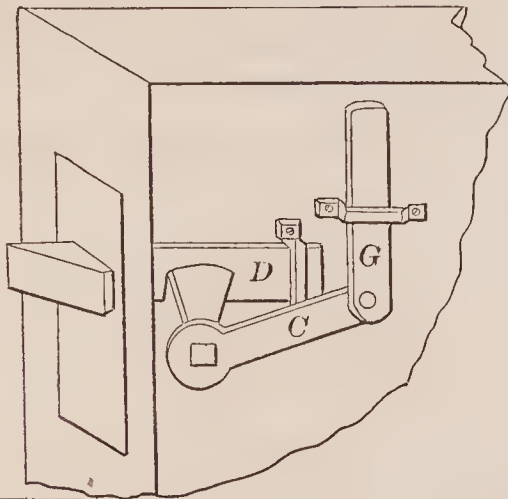
71123—N. Belvallette—Carriage Door Latch.
