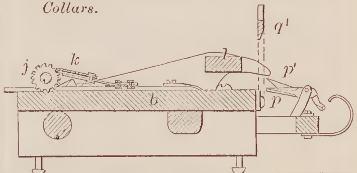
71074—D. M. Smyth—For Cutting Paper Collars.
