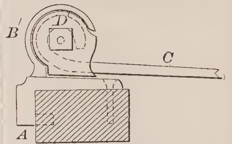
67609—B. C. Taylor— Horse Rake.
