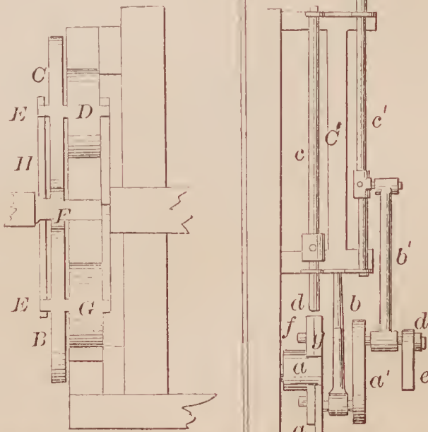
68795—C. Schilling—Harness Motion for Looms.
