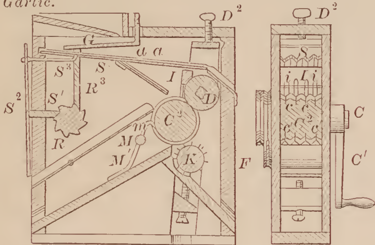
72834—S. Gantz—For Separating Wheat from Garlic.
