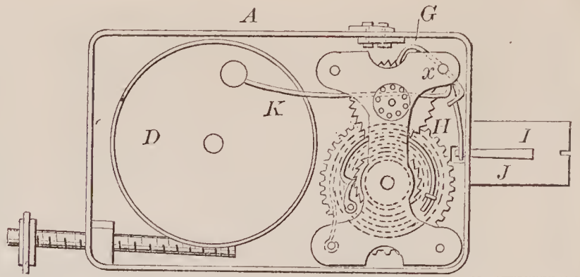
67619—S. Whitaker— Burglar Alarm.
