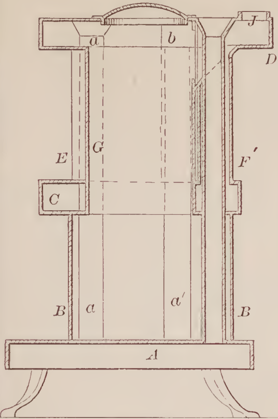
71171—T. Henney—Hot Air Stove.
