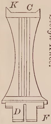
69066—Bliss & Adams—Boot Shank Laster.
