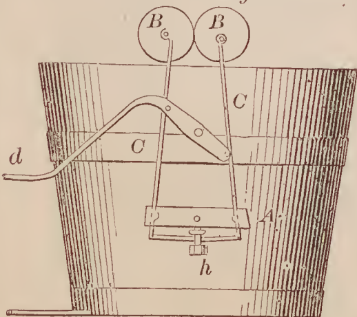
68447—Lord & Hinman—Mop Pail and Wringer.
