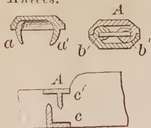
70778—H. Barber—Attaching Bolsters to Knives.
