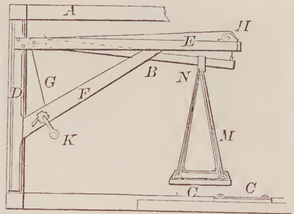
71680--C. Barry--For Making Tin Cans.
