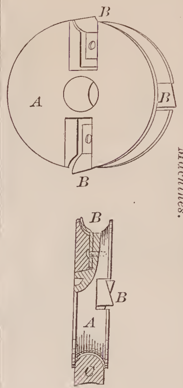
68053—B. K. Dorwart—Shutter Fastening.
