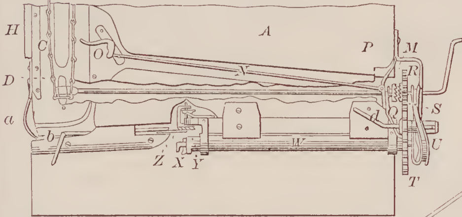
71662—Stout & Richardson— Hat Ironing Machine.
