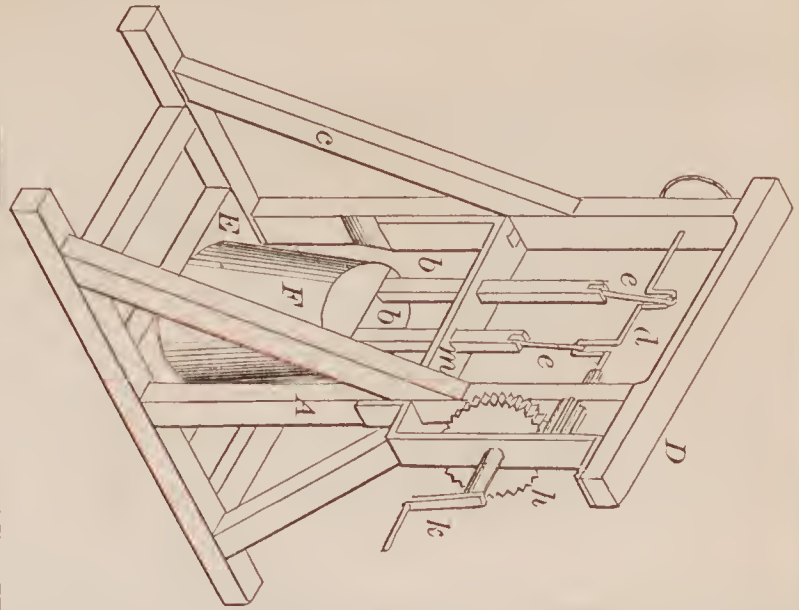
70431—Gruver & Wiggins—Churn.
