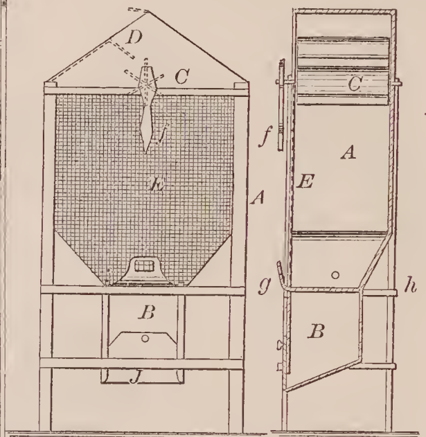
68761—N. M. Lurton— Grain Measure.
