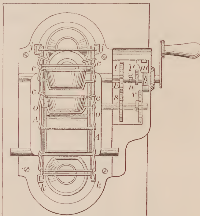
68754—G. H. Knight— Mechanical Movement.
