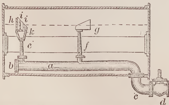
67340—R. Needham—Steam Boiler.
