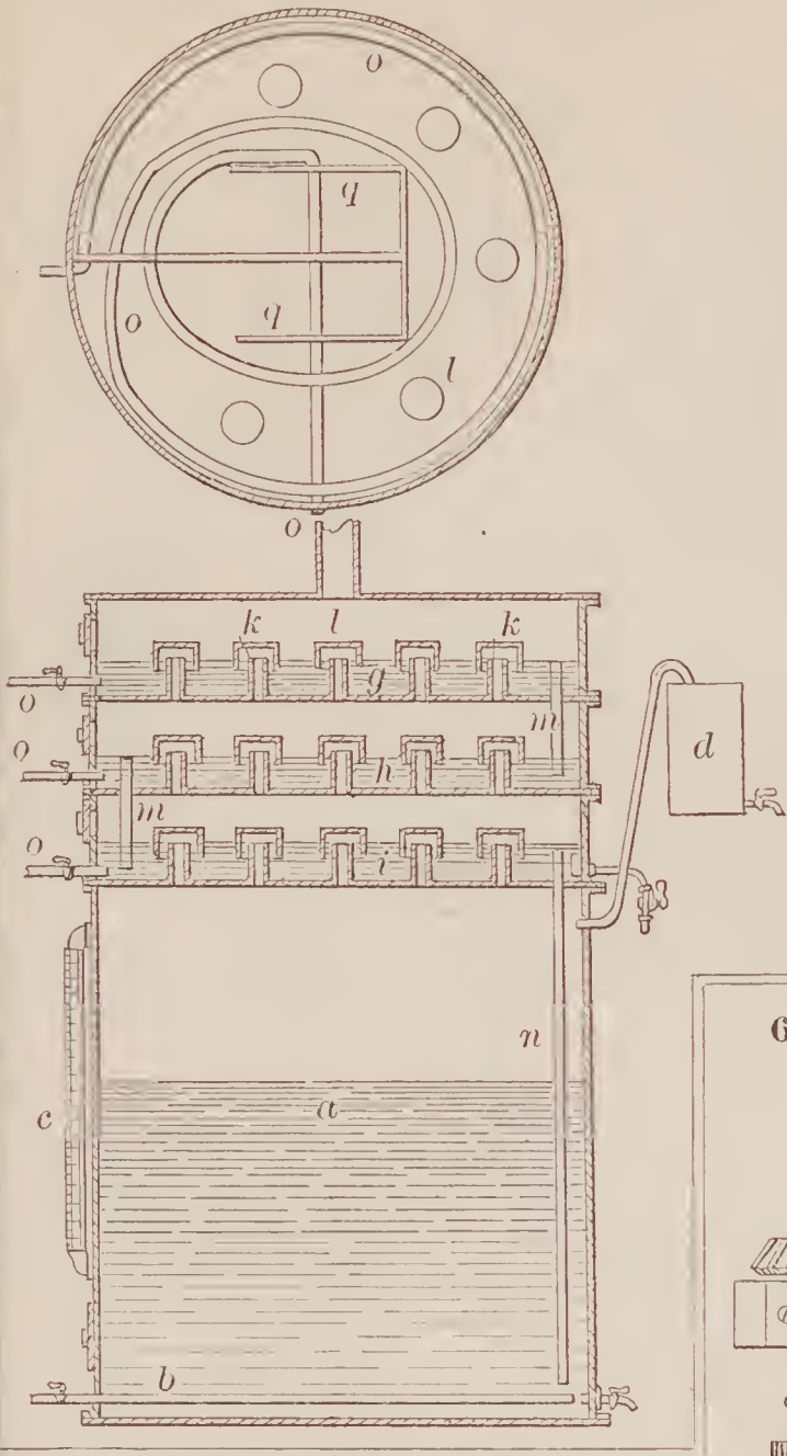
67864—A. Foubert—For Distilling Spirits.
