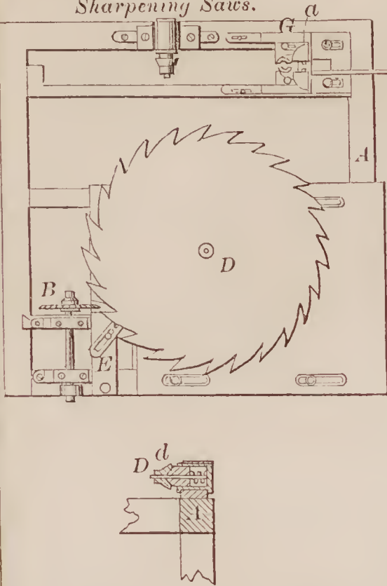
72100—J. B. Smith—For Sharpening Saws.
