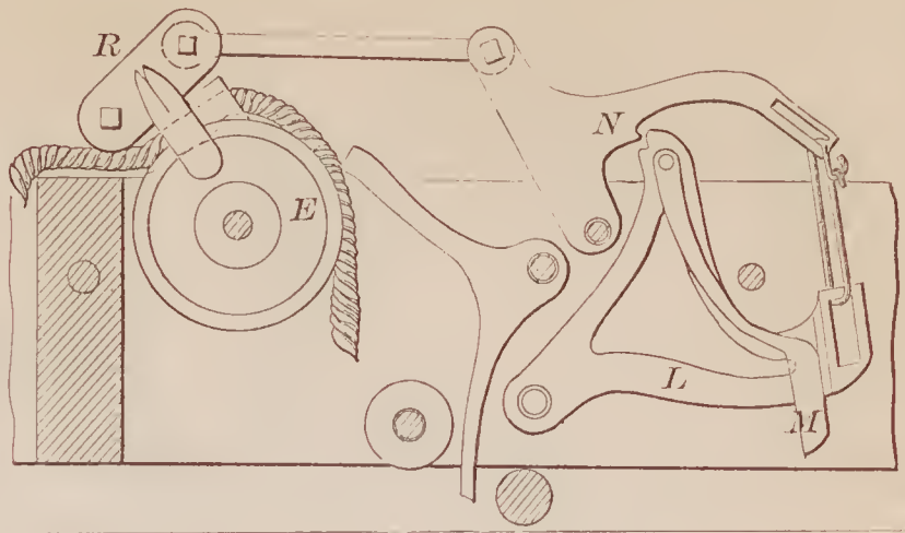
70719—W. J. Horner—Scraper.
