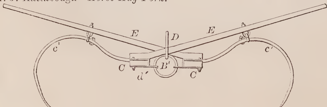
71167—I. J. Hattabough—Horse Hay Fork.
