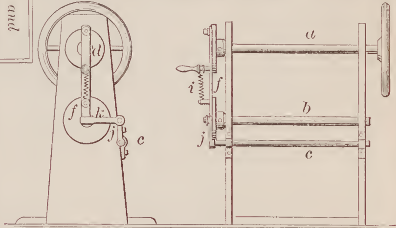
69929—J. Niebergall—Mechanical Movement.
