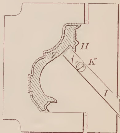
70847—R. Howdon—Moulding Facing Machine.
