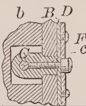
67463—C. E. Thompson—Screw Head Caps.
