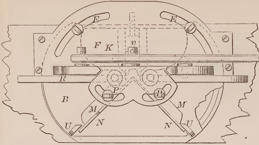
69510—R. F. Tompkins—Wood Mitering Machine.
