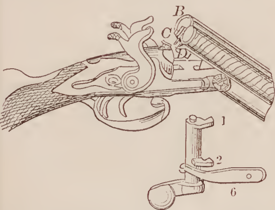
70463—W. R. Pape—Breech-Loading Fire Arm.
