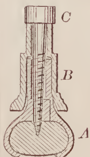
71228—A. Searls—Carriage Top Prop.
