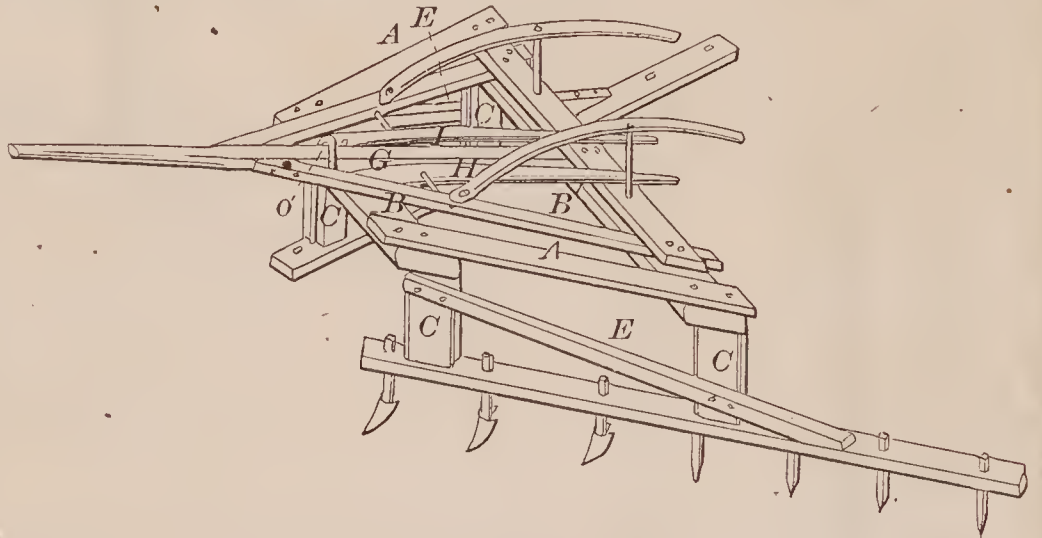
68678—M. Wilson—Corn Cultivator.
