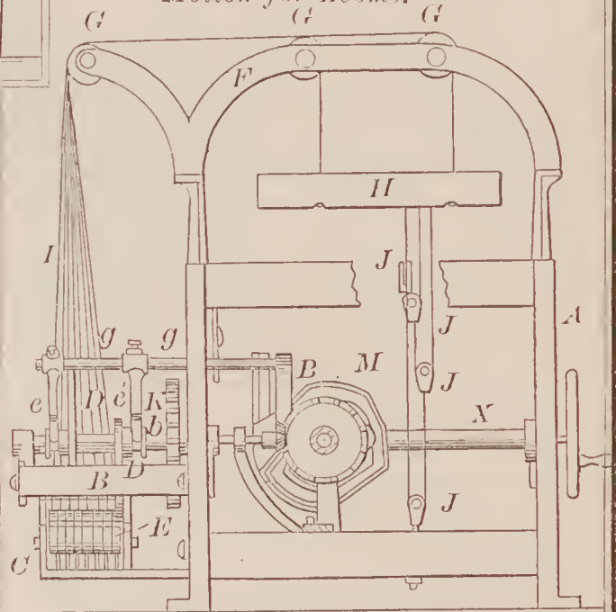
66827—J. F. Gebhart—Harness Motion for Looms.
