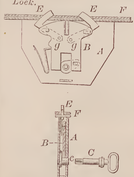
68496—E. L. Gaylord— Piano Lock.
