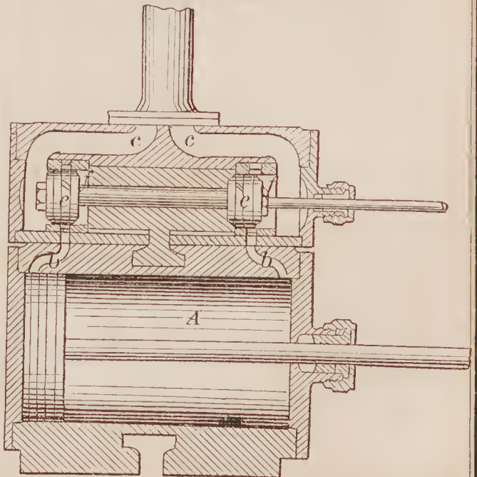
71337—I. Soule— Piston Valve.
