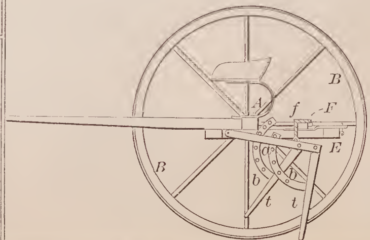
70314—Baker & Hoyt—Wheeled Harrow.
