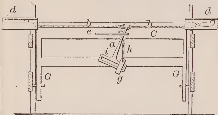
71088—J. Turner—Stump Extractor.
