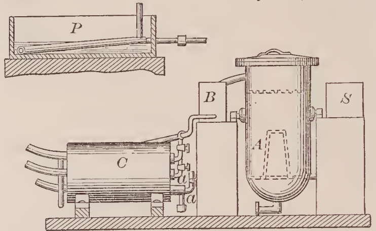
68506—C. O. Heyl— For Extracting Oil from Substances.
