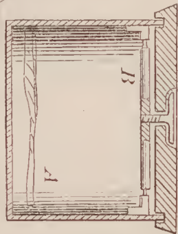
68158—G. W. Bennett—Paint Can.
