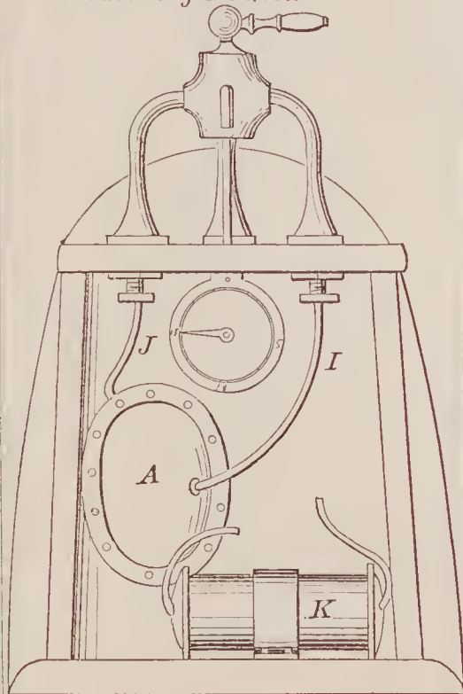
71865—E. Fitzgerald— Measuring Faucet.
