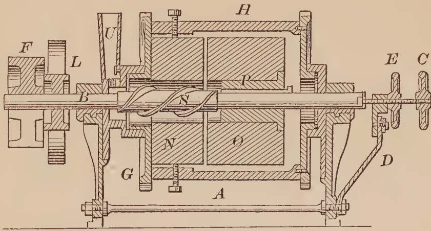
72825—Earseman & Gray—For Carburetting Coal Gas.
