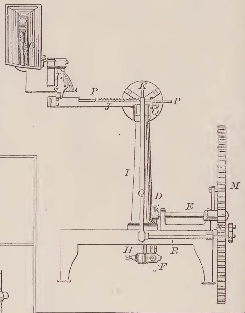
71639—O. E. Pillard— Tumbler for Permutation Locks.
