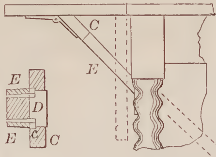
67390—W. Whitworth— Table Leaf Support.
