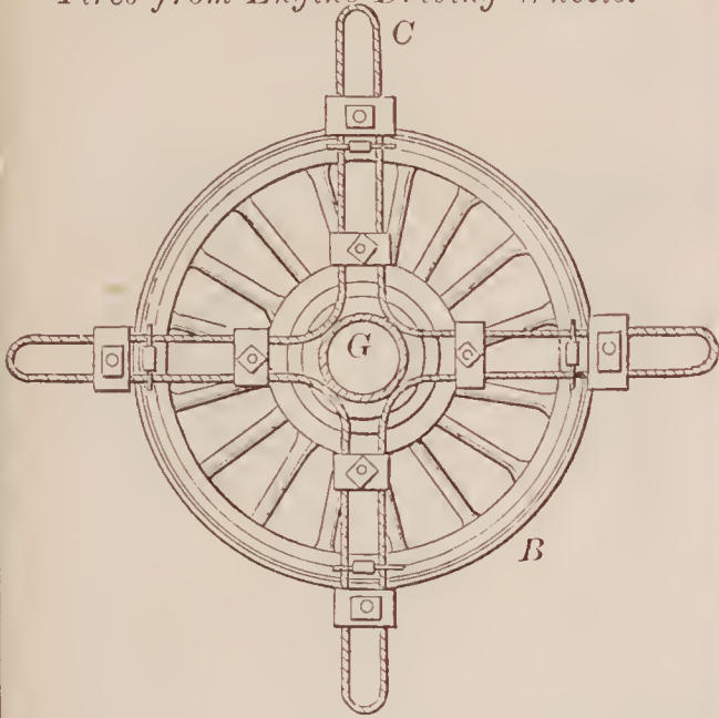
70796—W. H. Bryant—For Drawing Tires from Engine Driving Wheels.
