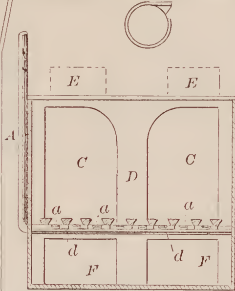
70557—D. Hargar— Furnace.
