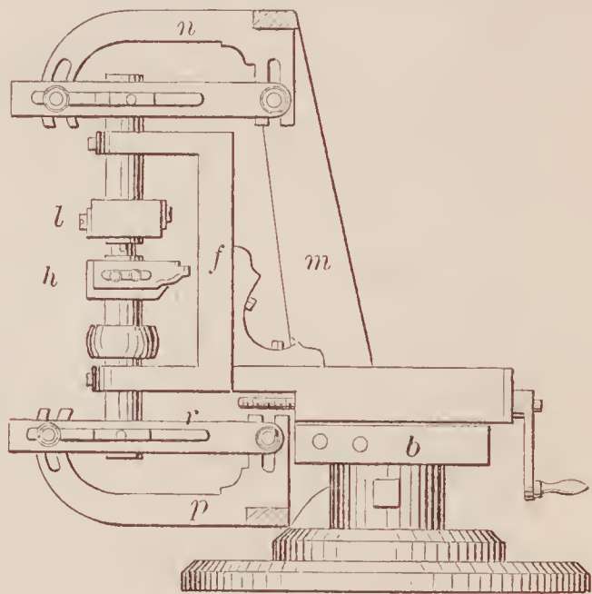
70192—T. F. Freeman—For Cutting Wood Gear.
