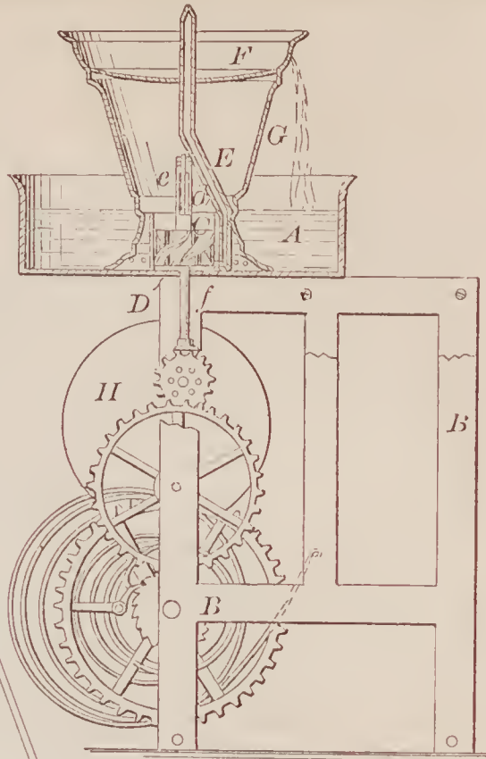
69994—J. Hegarty— Portable Fountain.
