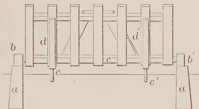
69861—J. B. Stoner— Portable Flood Fence.
