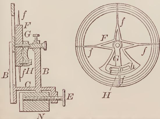
69602—Zimmerman & Baker— Plumb Level.
