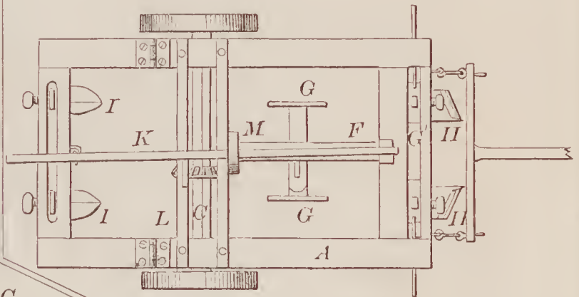
67294—W. Green— Washing Machine.
