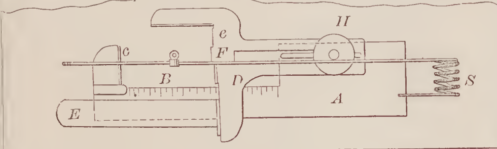
67870—H. C. Goodrich—Tuck Marker for Sewing Machines.
