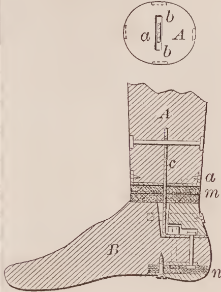
71424—C. Swett—Artificial Leg.
