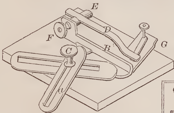
67590—Safford & Masters— Sewing Machine Guide.
