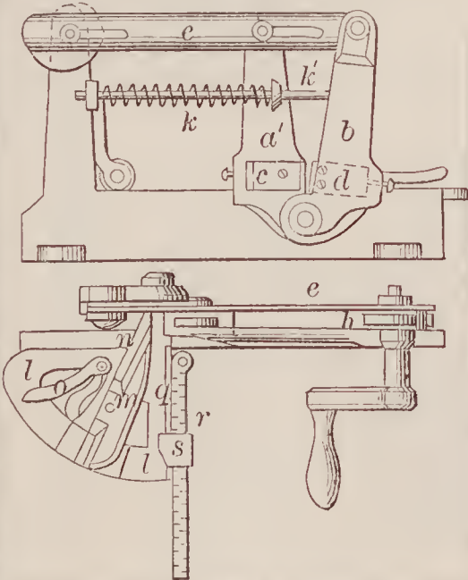
71668—R. Walker— For Cutting and Mitering Printers' Rules.
