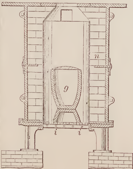
70042—W. Swindell—Furnace for the Manufacture of Steel.
