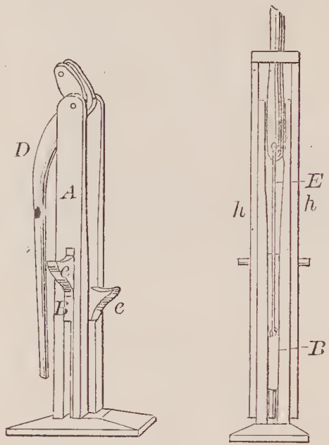
68003—R. B. Prindle—Wagon Jack.
