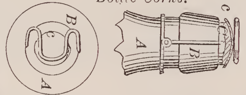
72606—F. W. Copeutt—For Labeling Bottle Corks.
