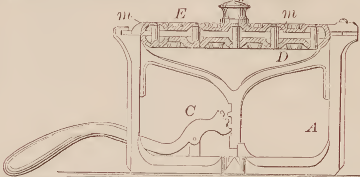
66886—L. V. Richmond—Stop Motion for Warping Machines.
