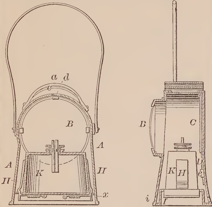
72900—Prindle & Wellfare—Lantern.
