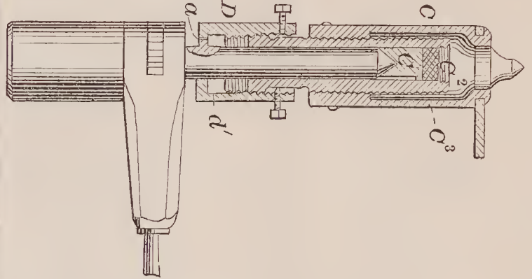
70199—J. Gray—Ratchet Drill.
