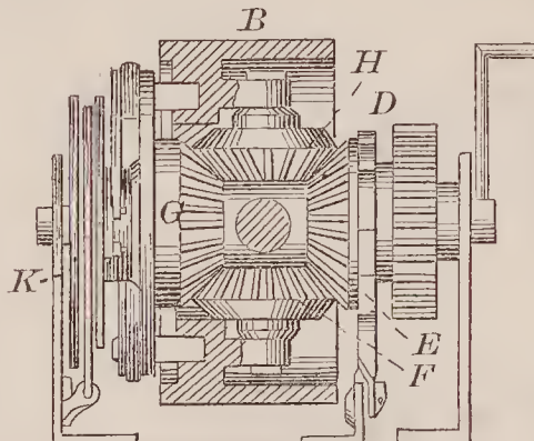
68015—E. Ware—For Propelling Steam Carriages.
