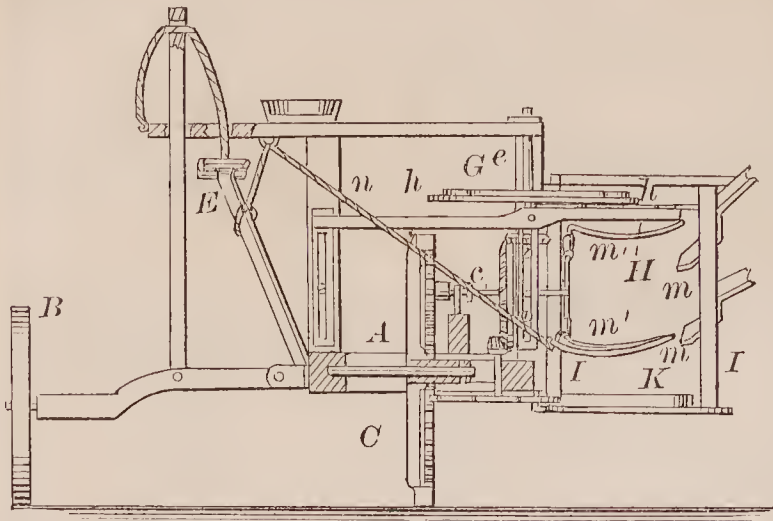
72299—J. W. Hull—For Trimming Hedges.
