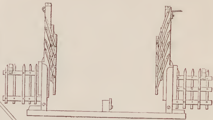
67915—J. W. Sanford— Gate and Fence.
