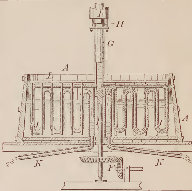
70518—F. P. Bush—Mash Cooler.
