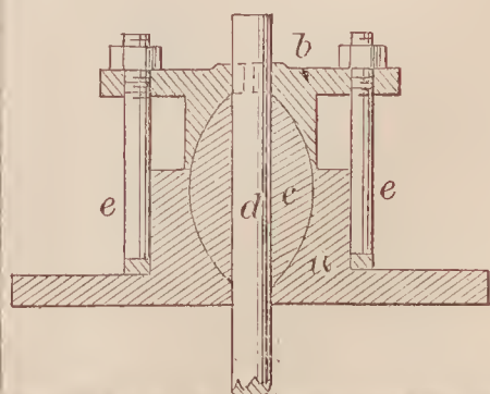
66758—J. H. Webster—Metallic Packing for Piston Rods.
