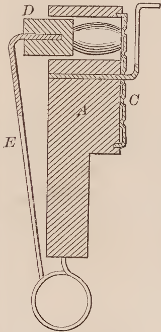
67010—Whitney & Davis—Nutmeg Grater.
