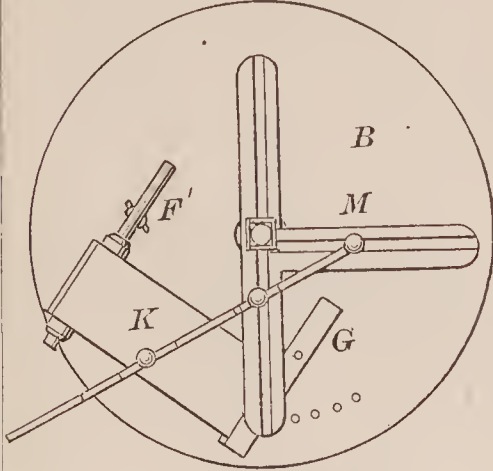
66796 —A. Clow— Instrument for Laying out Stair Railings.
