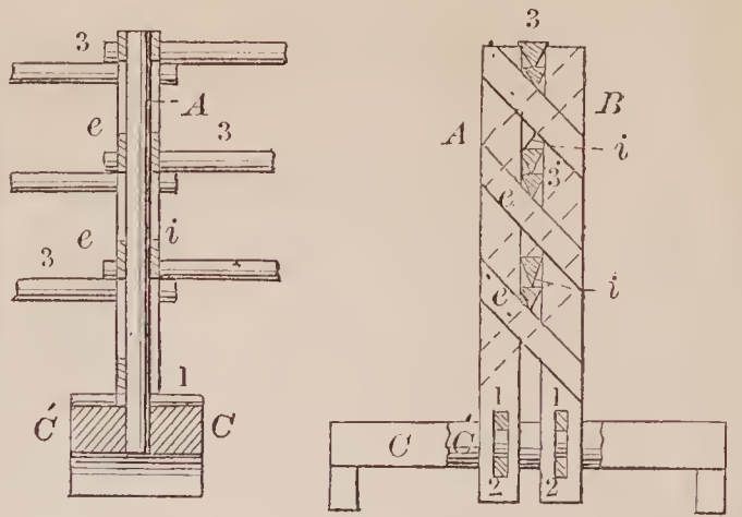
70097—J. E. Layton—Fence.
