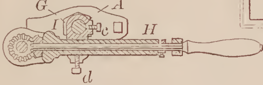
68827—Young & Whipple—Drill.
