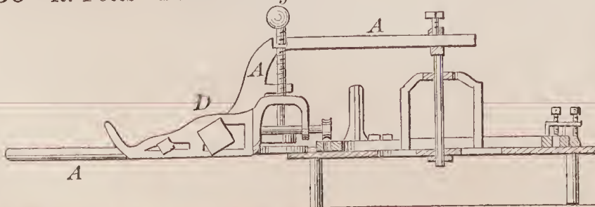
69936—R. Potts—For Bending Metals.
