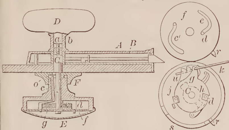
71721—C. H. Eifiler— Locking Knob Latch.
