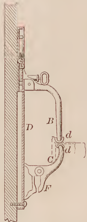
69032—W. Schmitt—Coat and Hat Hook.
