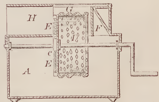
67529—J. Gardiner— Cocoa Nut Cutter and Grater.
