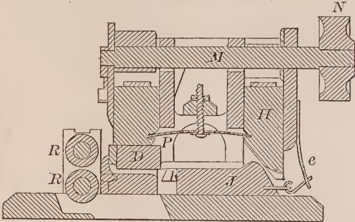
68222—R. G. McKay—For Making Spikes.
