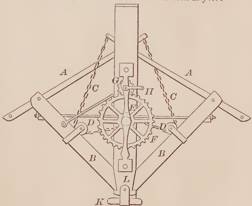
72527—J. Morton— Railroad Truck Lifter.
