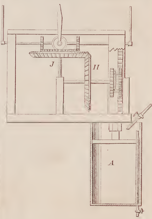
71437—O. Abbruzzo—Hydraulic Clock.
