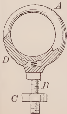
68559—E. Deming—Check Hook.
