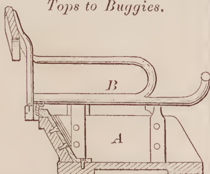
71304—H. F. Holt— Fastening Tops to Buggies.
