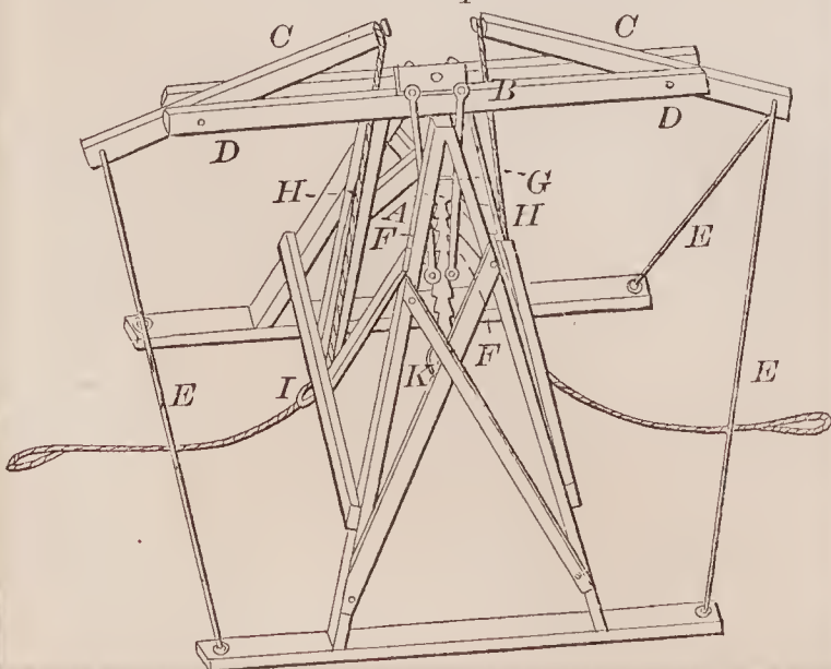
71088—J. Turner—Stump Extractor.
