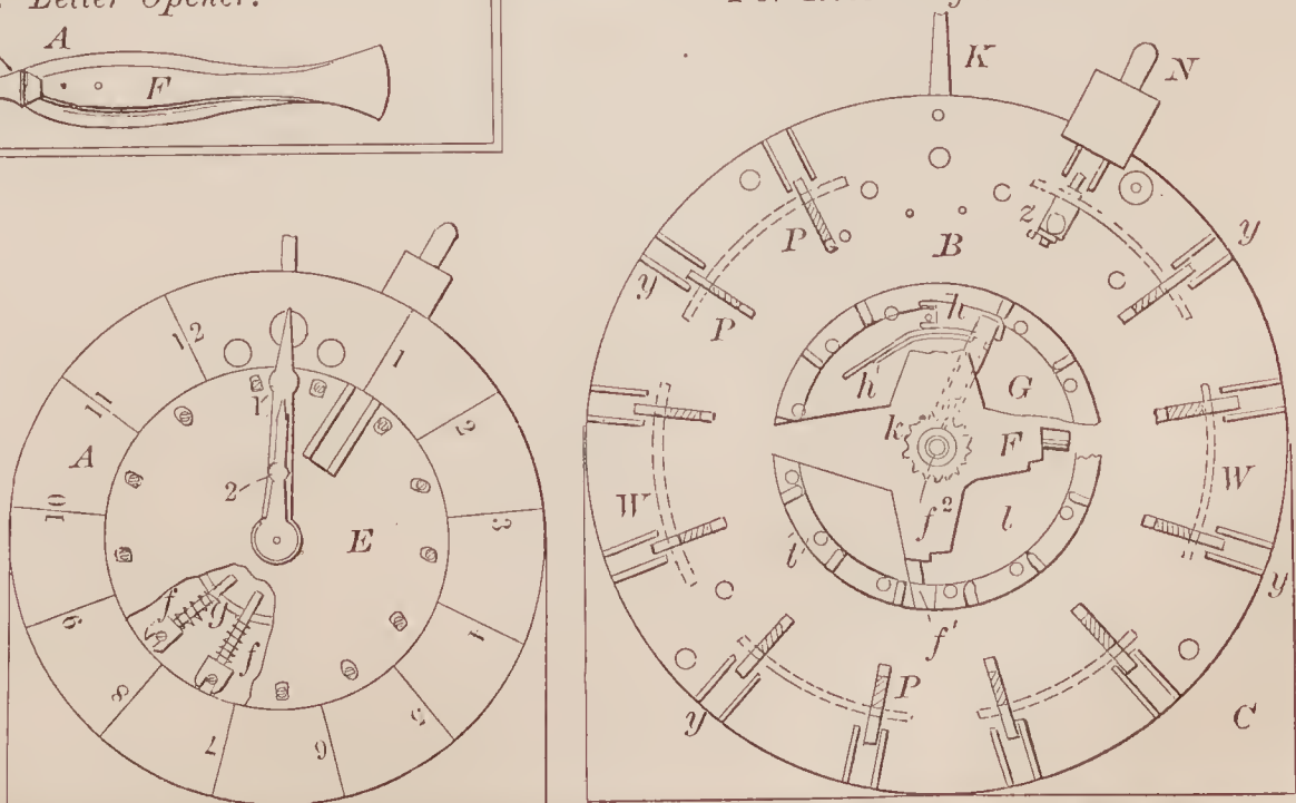
69389—Beardsley, Boyle, Lewis & Clancy—For Recording Votes.
