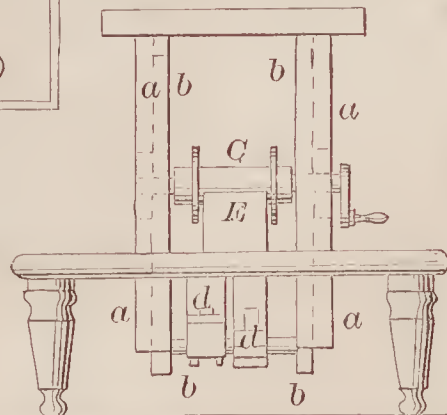
71040—J. W. Milroy— Drain Tile Machine.
