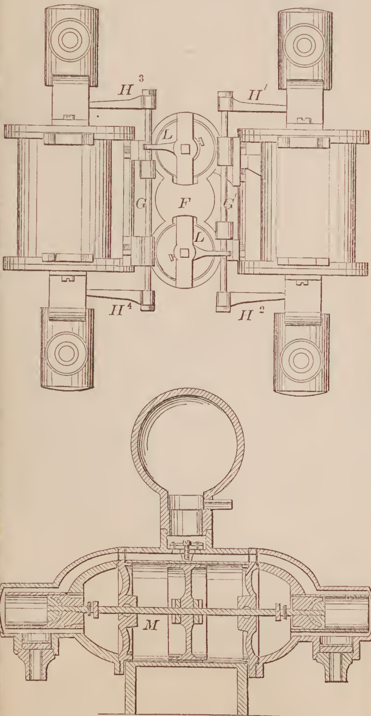
68863—M. Everett—Hydraulic Engine.
