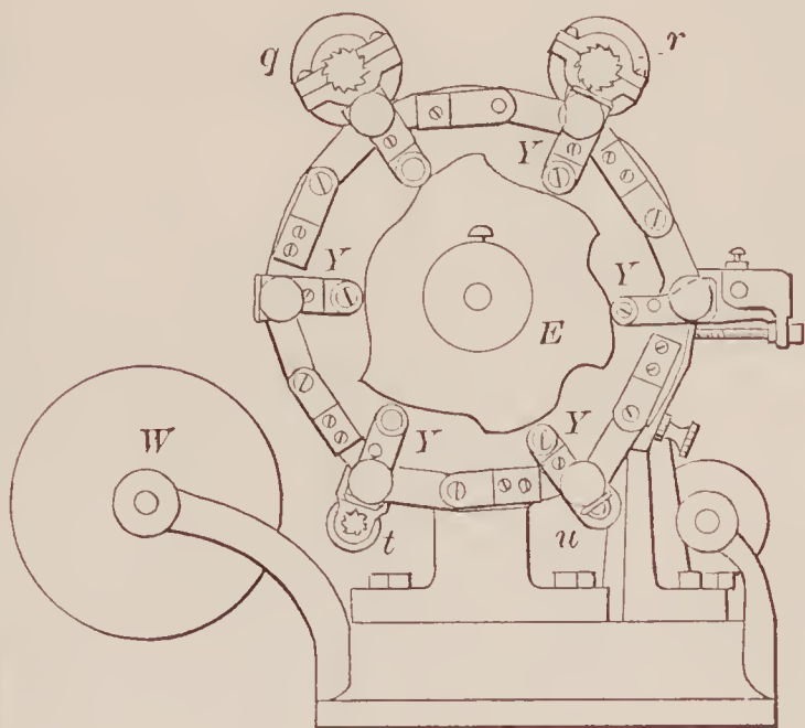
71836—W. Aikin—For Notching Knitting Needles.
