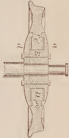
70560—J. Harris— Car Wheel.
