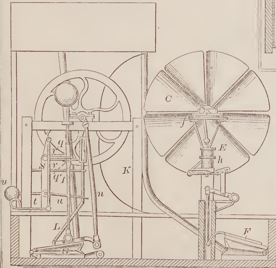
68007—J. Schenker—Windmill.
