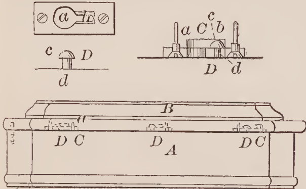
71470—Edmands & Hamblet— Escapement for Electric Clocks.
