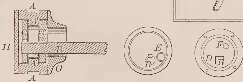
71803—L. F. Smith—Low Water Indicator.
