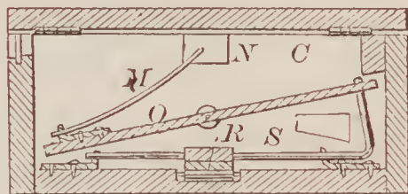
69697—J. Pierpont—Cultivator Coupling.
