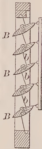
71776—J. Maunton—For Roasting and Reducing Ores.
