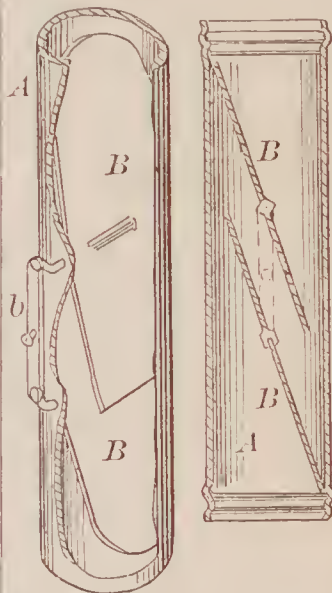
70140—West & Price—Blower for Forges.
