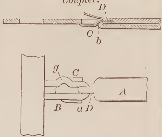
67761—P. A. Hause— Trace Coupler.
