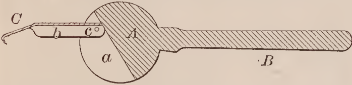
69066—Bliss & Adams—Boot Shank Laster.
