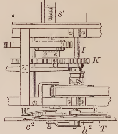
69055—T. Whitmore— Head Block for Saw Mills.
