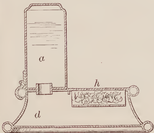
69895—Benn & Luckman— For Damping and Gumming Labels.
