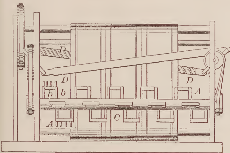
69152—G. W. Young— Carpet Cleaner.
