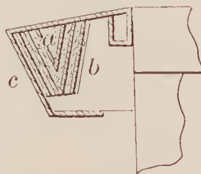
71282—H. W. Collender—Billiard Cushion.
