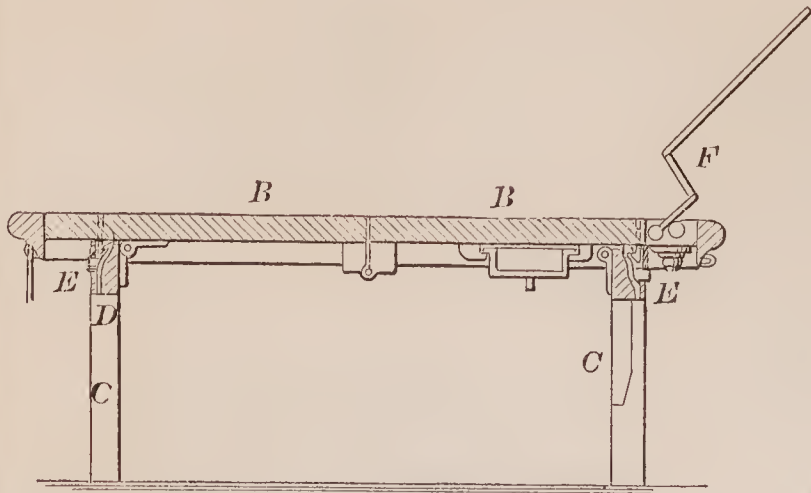
71023—I. Lancaster—Grain Binder.
