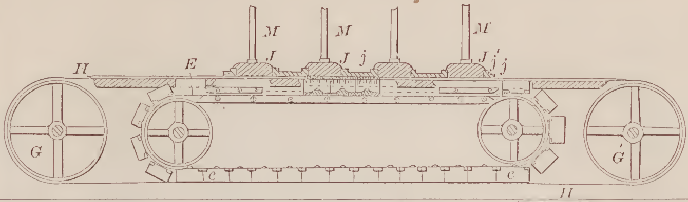
67243—Y. F. Wright—Cotton Press.
