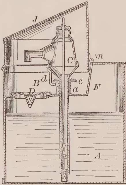
68501—R. W. Hallett— For Raising Sunken Vessels.
