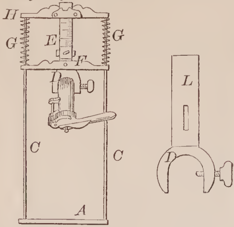
69425—Fisher & Holliday— Weighing Attachment to Faucets.
