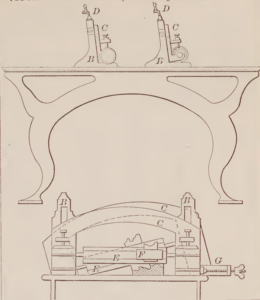
71864—L. Felker— Corn Cake Cutter.
