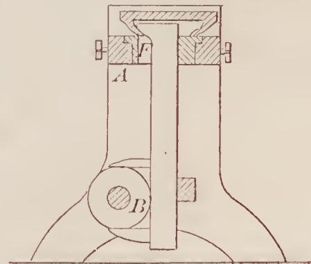
69786—D. Eynon—For Slotting the Lips of Railroad Chairs.
