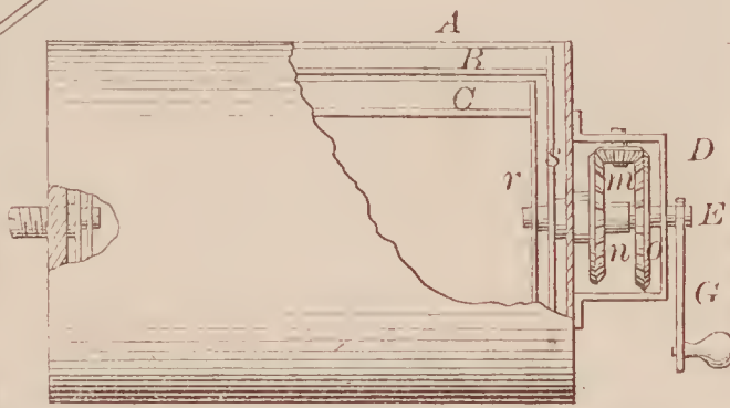
68798—L. W. Shaeffer—Churn.
