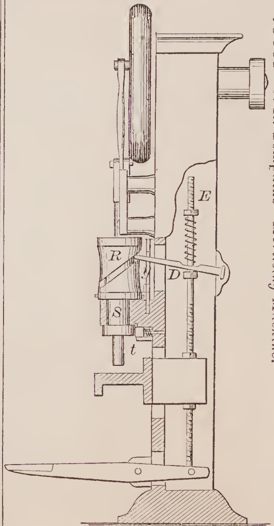
70051—C. R. Tompkins—Mortising Machine.
