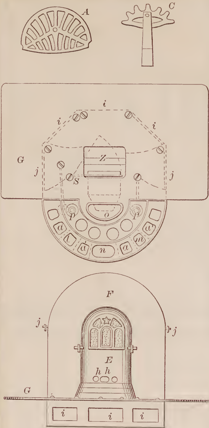
72229—C. R. Rand—Heating Furnace.
