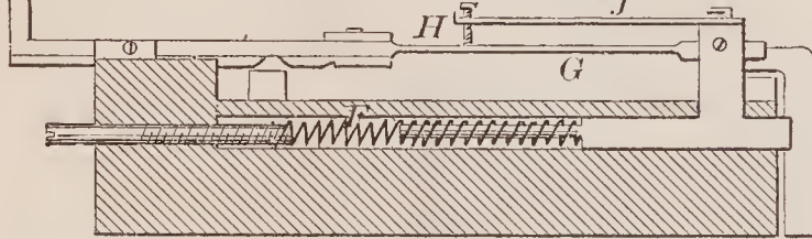
69709—J. Russell—Card Setting Machine.
