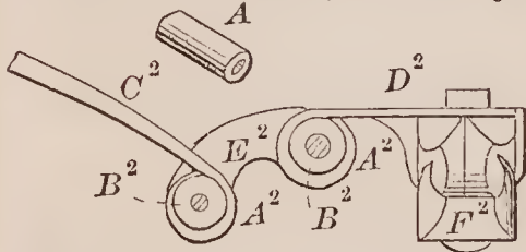
71123—N. Belvallette—Carriage Door Latch.
