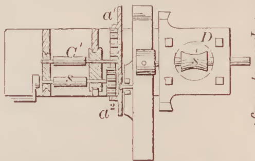
72055—G. S. Long—For Forming Elliptic Spring.
