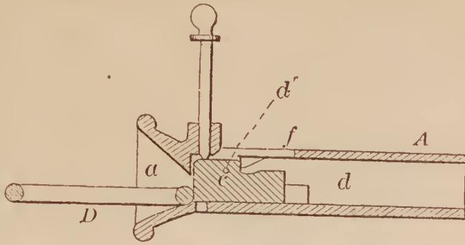
72717—E. R. Bigelow—Car Coupling.
