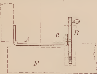
72948—Wemple & Richardson—Sash and Shutter Fastener.
