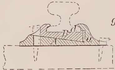
72080—L. Pollock—Railway Chair.
