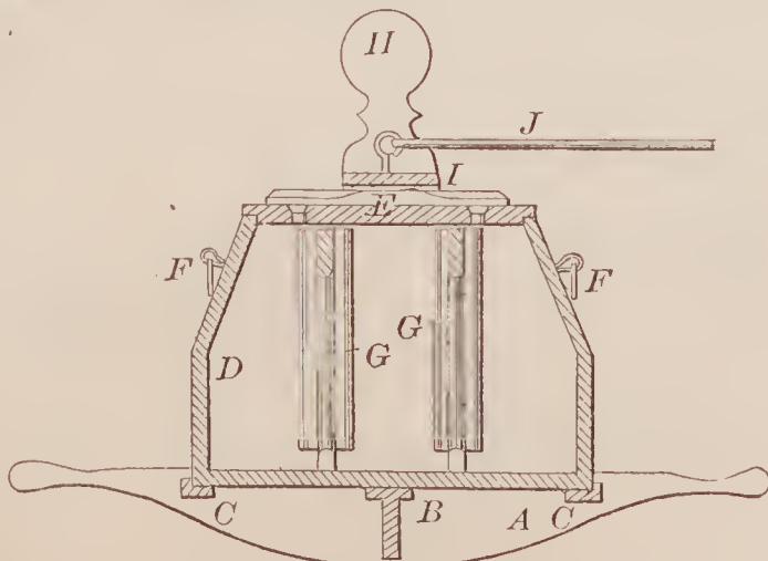
69475—W. C. Peck— Churn.
