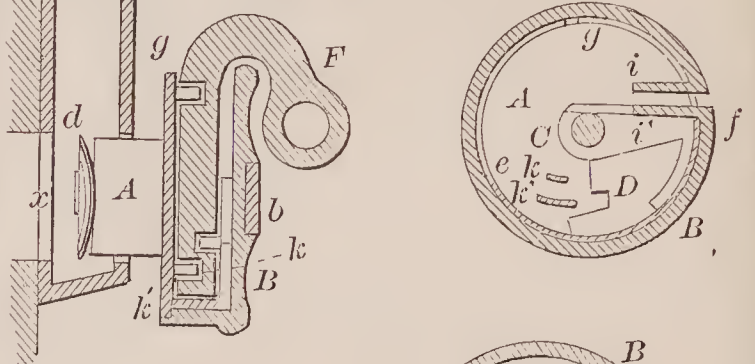
71235—Shloss, Veerkamp & Leopold—Key Hole Guard for Door Locks.
