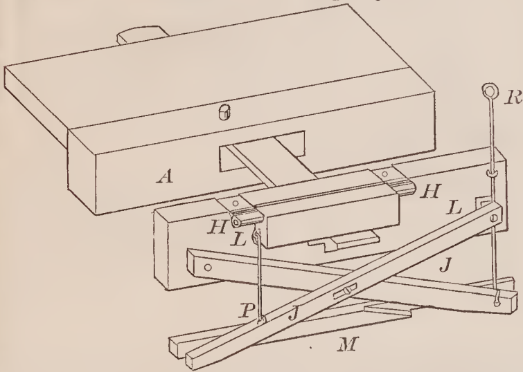
70280—C. L. Snyder—Threshing Machine.
