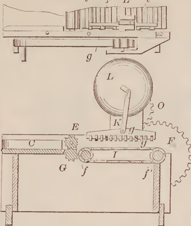
66767—H. Zellner—Breaking and Cleaning Hemp.
