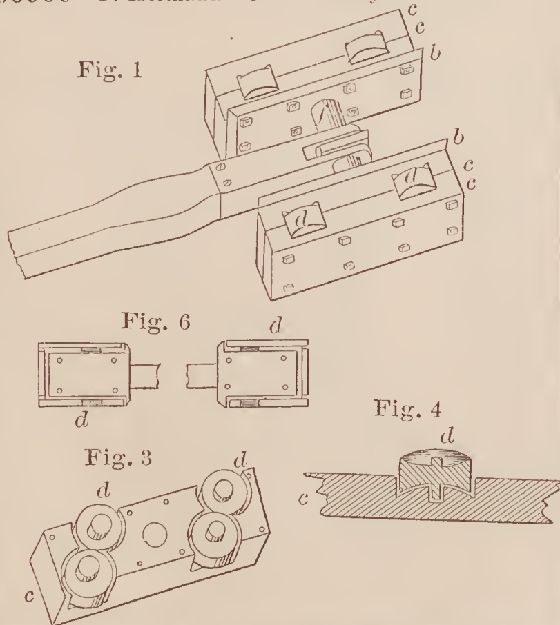
66960—F. Hermann—Cross Head for Sawmills.
