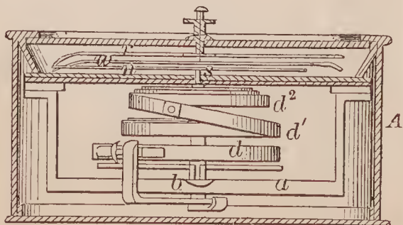
68681—M. Ames—Self-Registering Thermometer.
