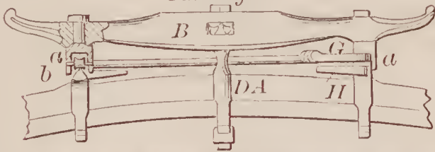
72053—F. C. Levalley—Door Fastener.
