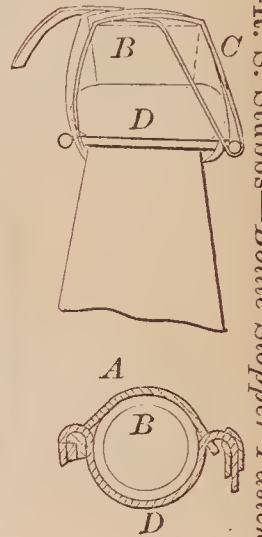
72761—R. S. Stubbs—Bottle Stopper Fastening.
