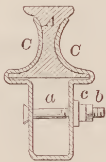
70271—B. J. Romaine— Railroad Chair.
