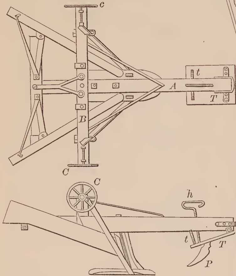
72953—D. Whisler—Ditching Machine.
