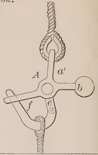
71779—G. J. Neveil—Retaining and Releasing Hook.
