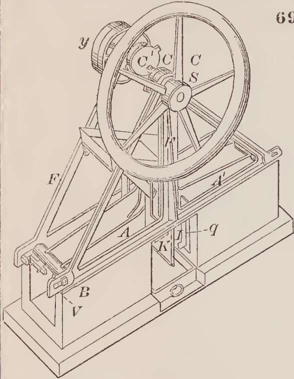
69657—T. D. Guthrie, Jr.—Baling Press.
