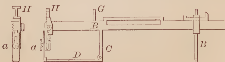
72427—D. F. Stratton— Gauge for Setting Wagon Axles.
