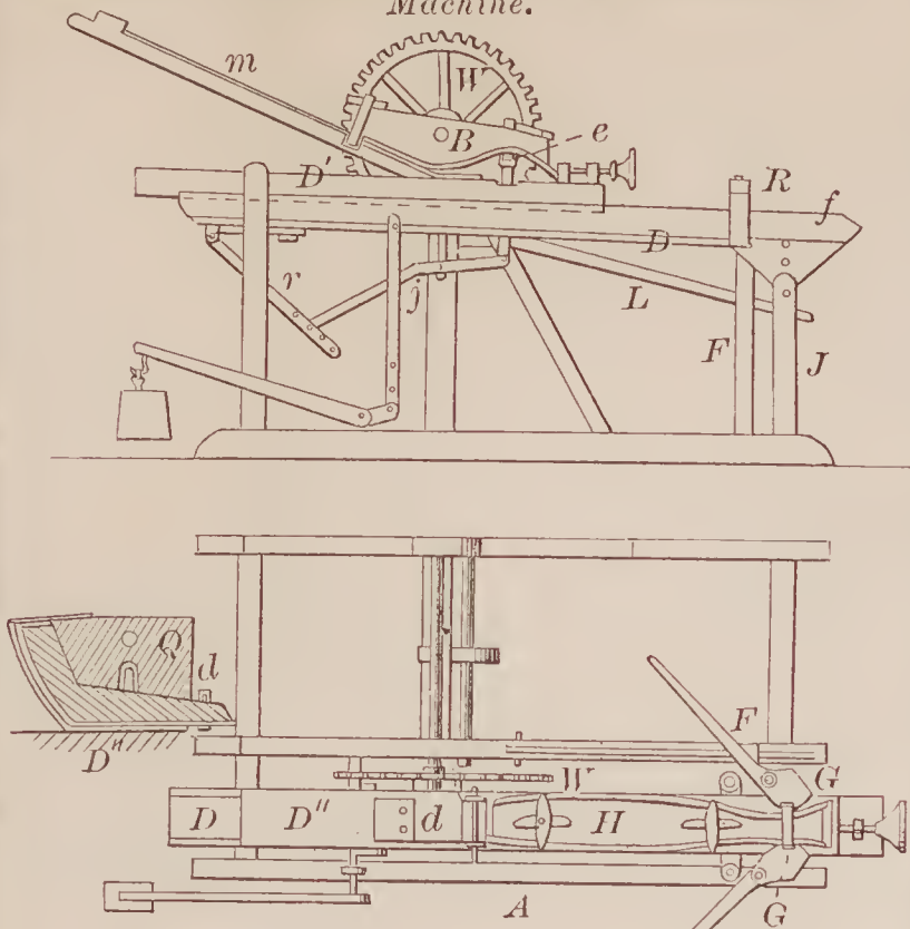
69313—Catchpole & Havens—Wood Bending Machine.
