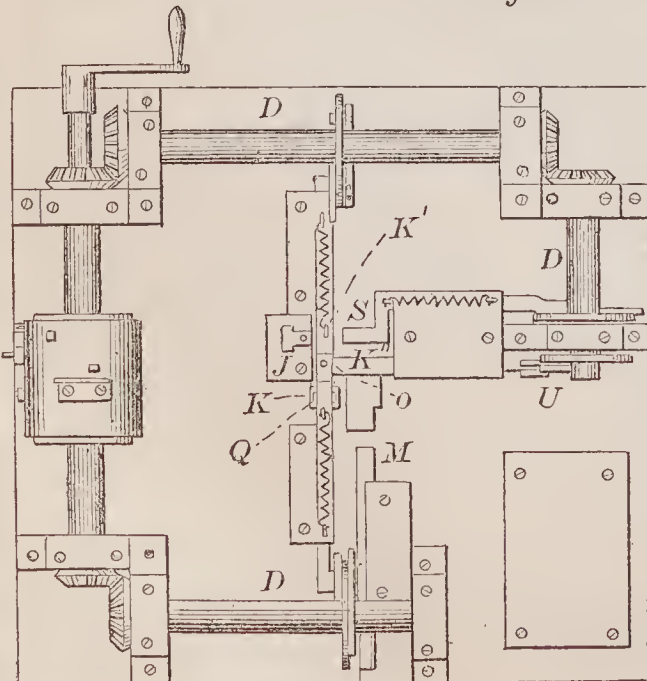
67421—G. Dunham—For Making Nuts.
