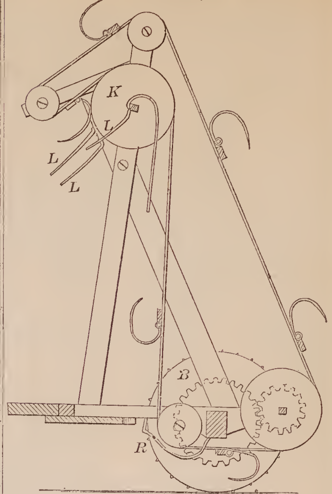
68887—Kinyon & Smith— Hay Raker and Loader.
