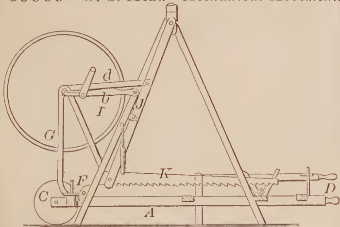
69011—W. H. Miller—Rake and Spade.
