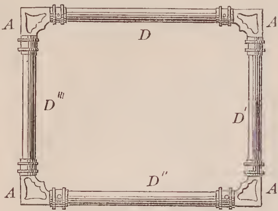
68103—W. H. Nash— Frame for Window Screens.
