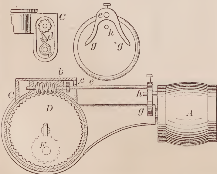
69038—J. C. Spencer— Odometer.
