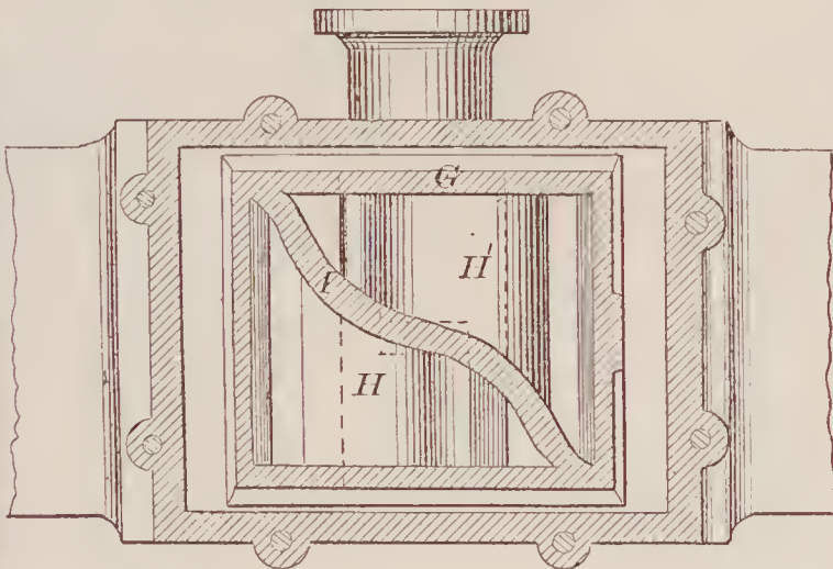
71618—B. W. Hudson—Steam Slide Valve.
