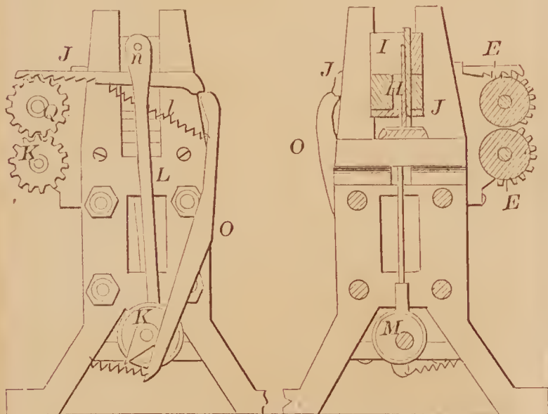
72705—O. F. Washburn— For Making Paper Collars.
