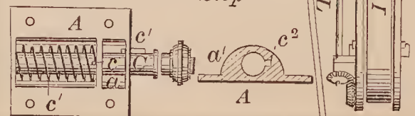
72807—R. H. Cooper—Window Sash Stop
