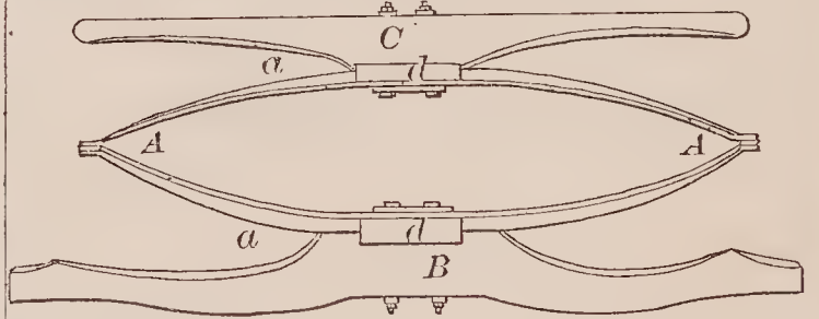
69125—E. J. Post—Vehicle Spring.
