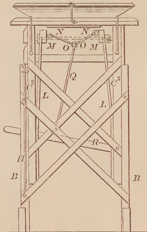
72788—C. D. Brainerd— Bag Holder.
