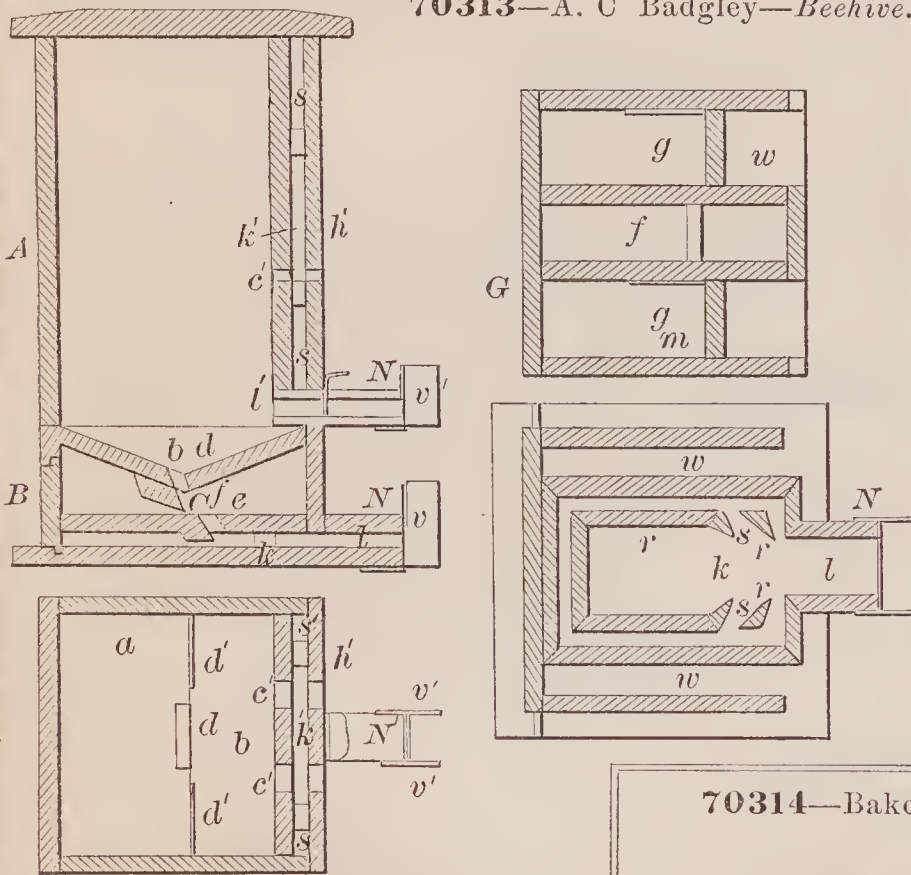
70313—A. C. Badgley—Beehive.
