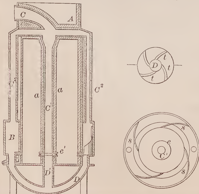
70329—H. Fayette—Cupola, Blast and Smelting Furnace.
