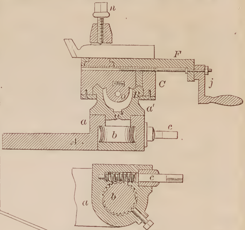
68654—J. G. Rominger—Slide Rest for Lathes.
