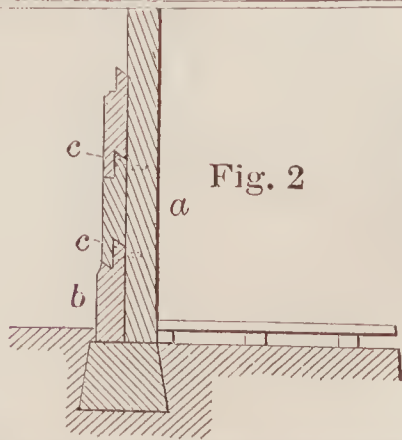
71587—W. Damerel—Building.
