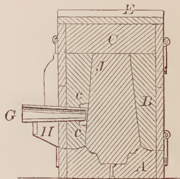
70740—B. C. Painter—Flask for Casting Tapers.
