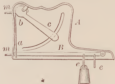
66825—L. H. Franklin—Weighing Scale.
