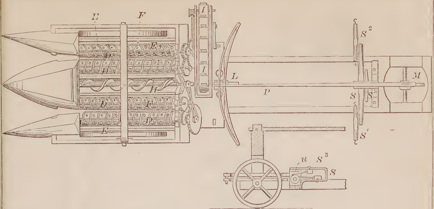
70335—Hill & Harpham— Corn Harvester.
