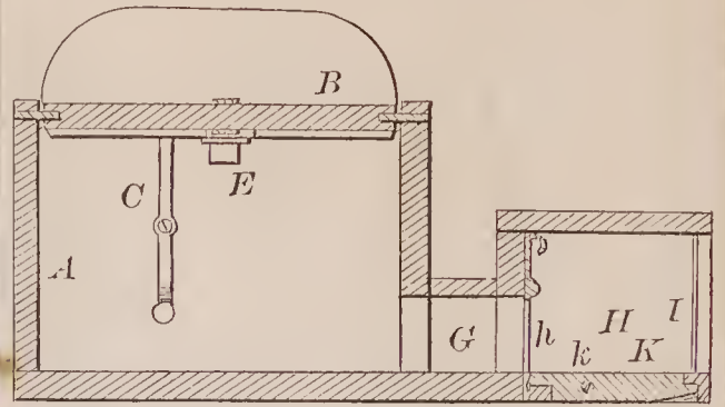
71543—T. Sillman—Animal Trap.
