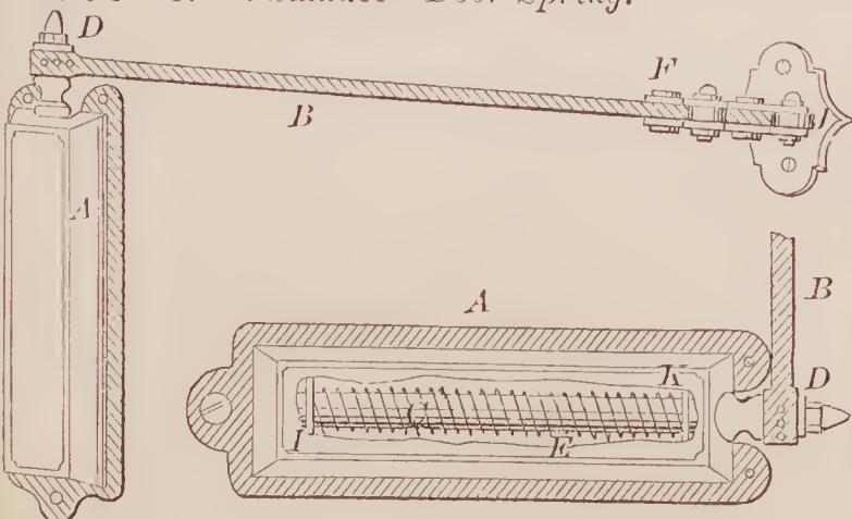
70903—C. W. Saladec—Door Spring.
