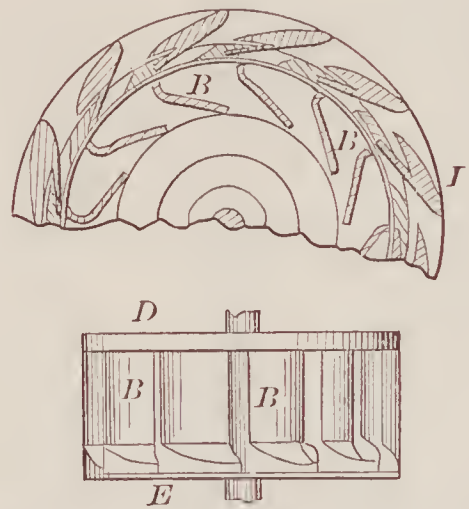
72682—J. Risher—Churn.
