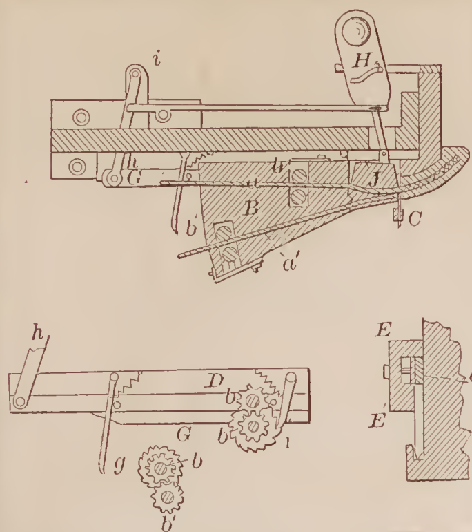
69040—H. C. Stone—Pegging Machine.
