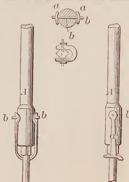
71727—S. F. Fenn— Bit Brace.
