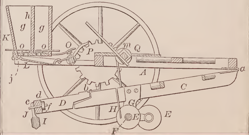
69484—E. Ritson— Seeding Machine.
