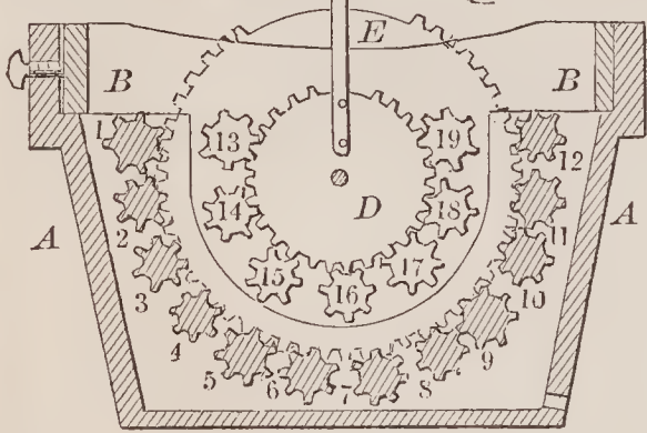
67731—R. Daily—Washing Machine.
