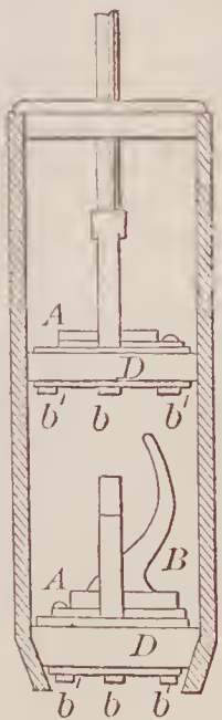
67666—Merrill & Lawrence—Pump.
