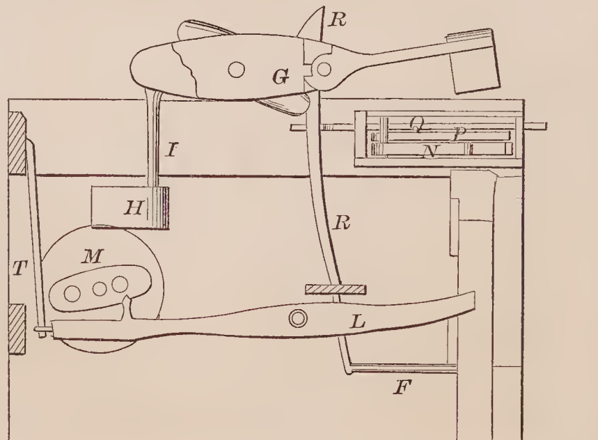
72550—A. Shaw— For Making Horse Shoe Nails.
