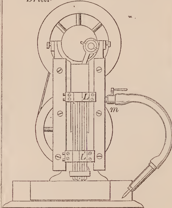
68888—E. G. Lamson— Operating Drill.
