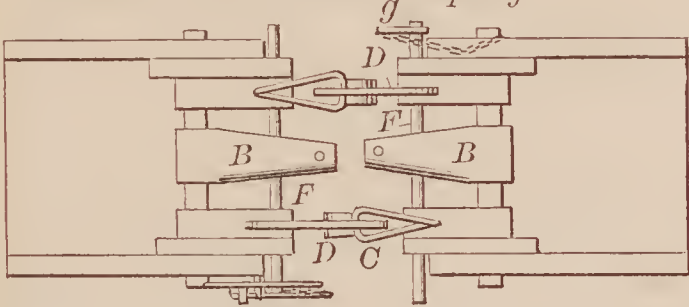
72482—R. Goole—Car Coupling.
