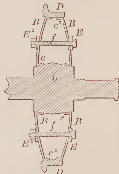
71021—C. E. Kleinschmidt— Car Wheel.
