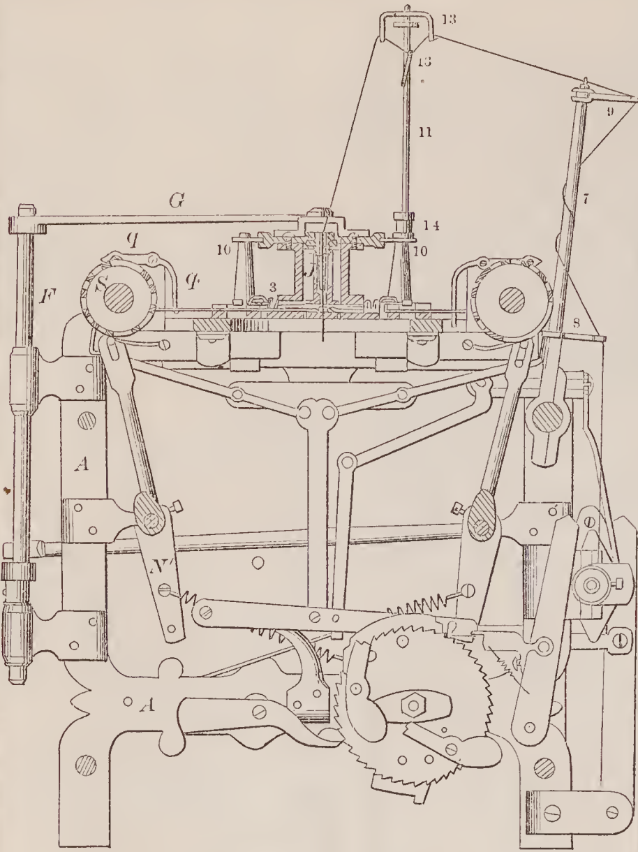
67263—A. C. Carey— Knitting Machine.
