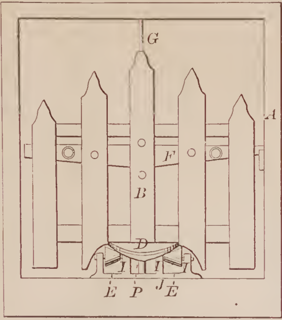
69108—H. Mansfield—Gate.
