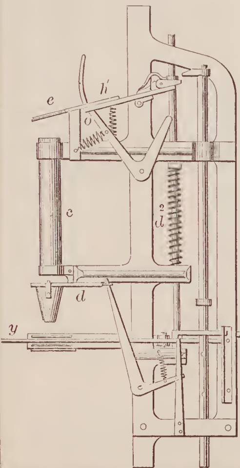
71945—I. Angell—For Presenting Palm Leaf to Looms.
