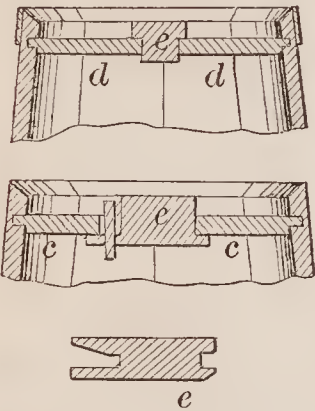
70047—A. Thoma—For Reducing Iron Ore.
