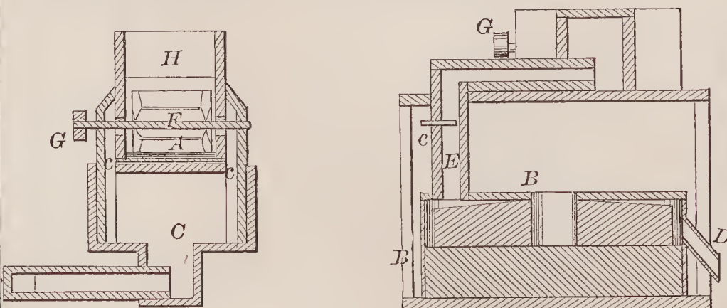
71677—D. Baird—Exhaust for Mill Stones.
