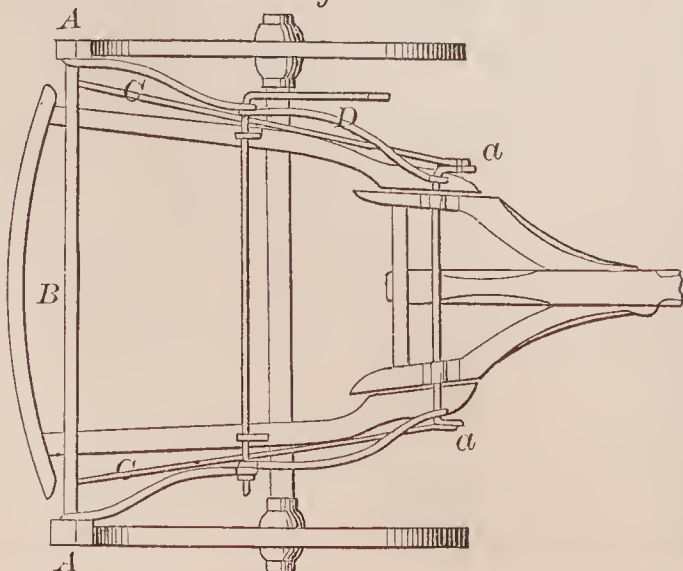
70217—W. Hull—Wagon Brake.
