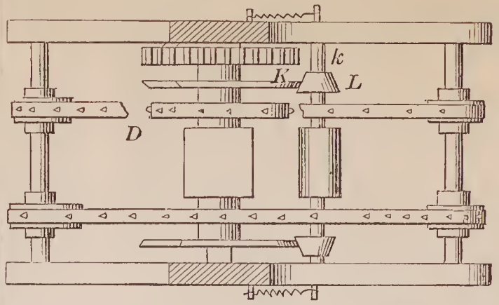
70773—E. Allen— Printing Press.
