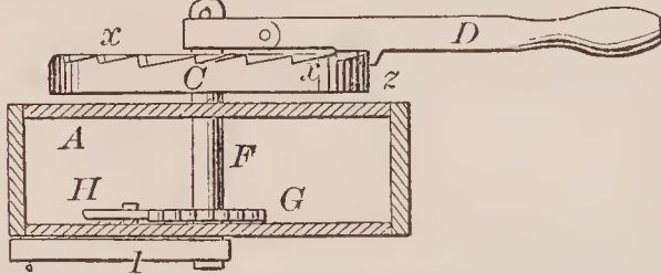
68580—A. M. Southard— Stone Drilling Machine.
