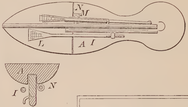
72452—E. O. Carrington—Mosquito Net.
