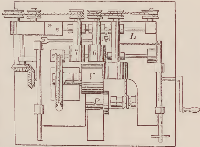
71668—R. Walker— For Cutting and Mitering Printers' Rules.
