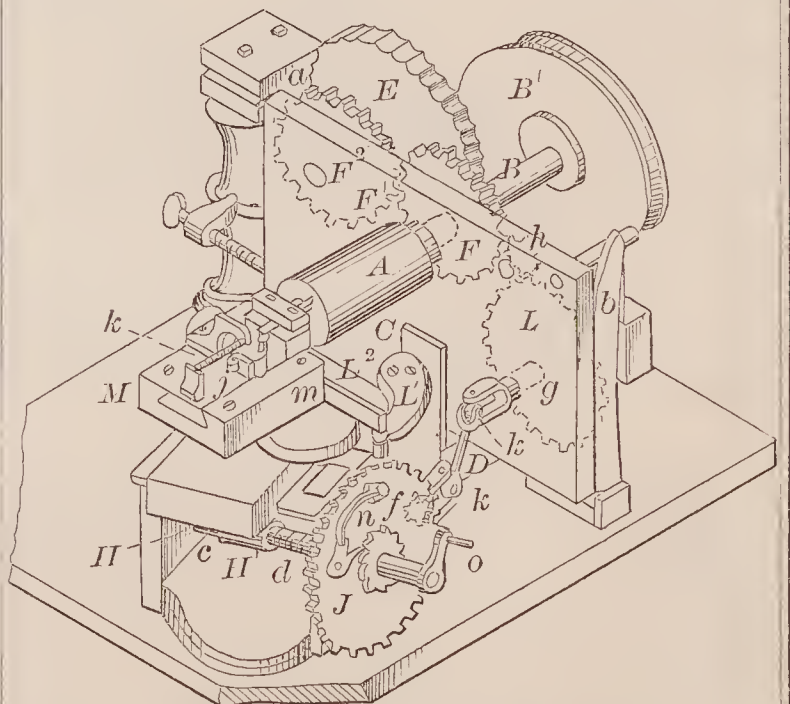
66819—C. H. Field—Rosette Engine.
