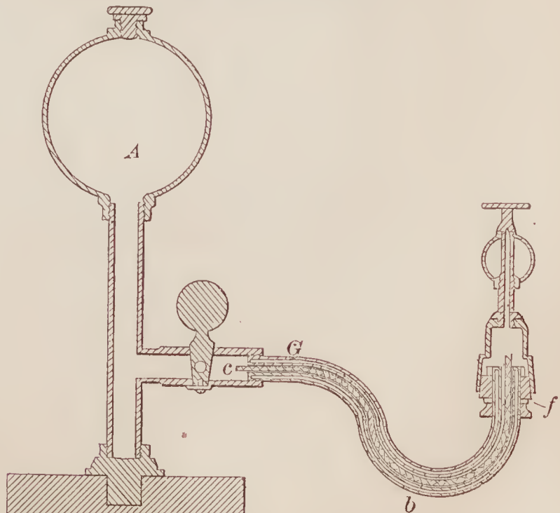
70043—D. Symonds—Vapor Burner.
