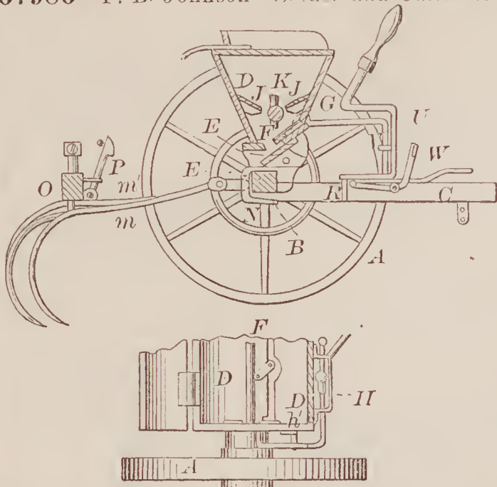
67986—F. B. Johnson—Seeder and Cultivator.
