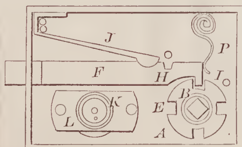
67210—P. A. Oliver—Bayonet Attachment.
