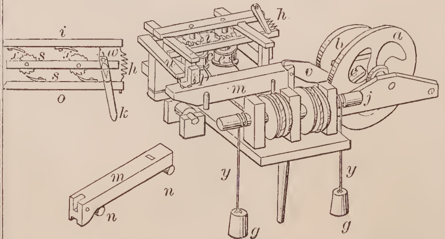
68762—J. P. Luther— For Rolling Whips.
