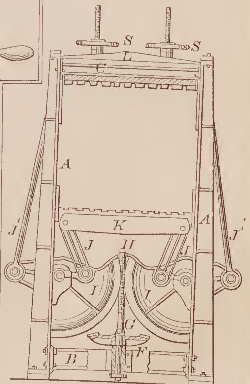
68812—C. P. Wagner—Press.
