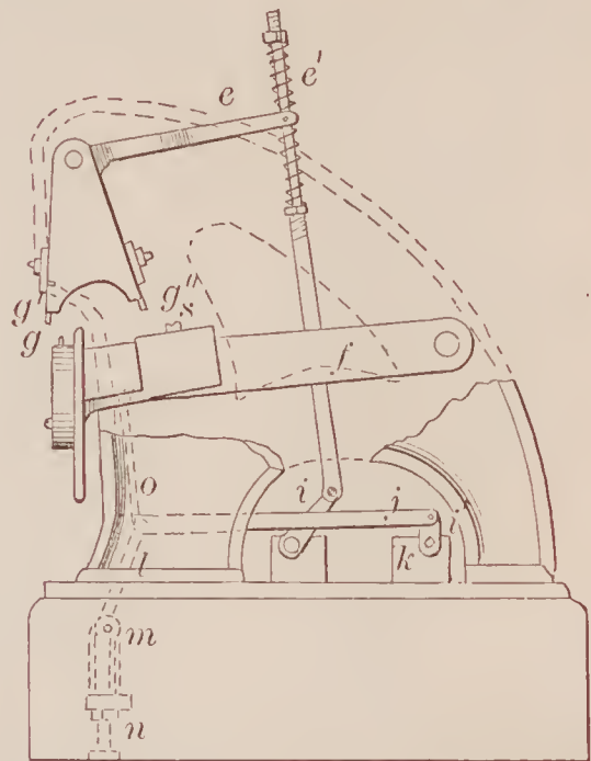
68546—Baker & Harbster—Rotary Measuring Faucet.
