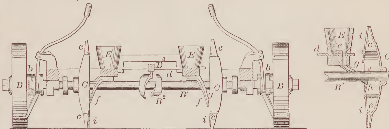
69862—L. Study— Corn Planter.
