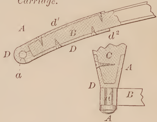
72835—R. Garter—Cultivator.
