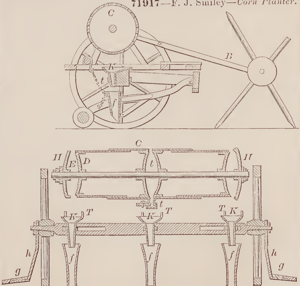
71917—F. J. Smiley—Corn Planter.
