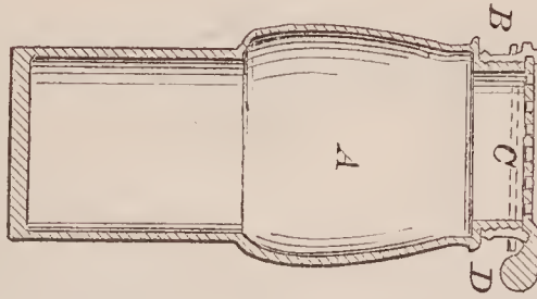
70710—J. E. Fry—Mould for Casting Steel Ingots.
