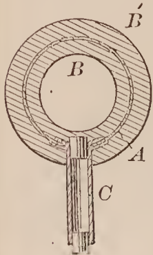
67080—N. Stephens—Tap for Cement Lined Pipe.
