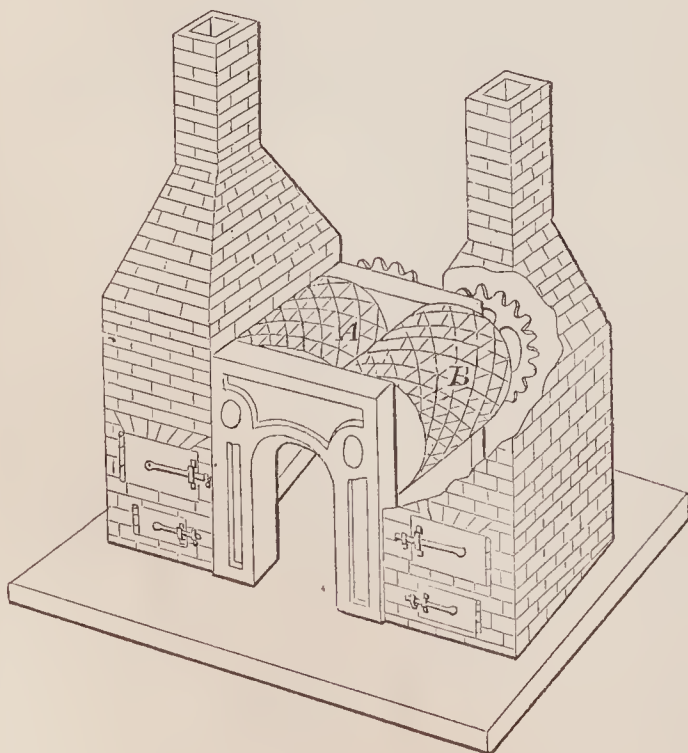
69677—J. Jones— For Compressing Peat.
