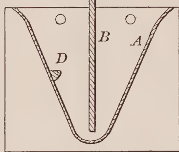
72207—Little & Bell—Summer Furnace.
