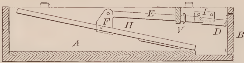
68049—J. J. Cumming—Churn Dasher.
