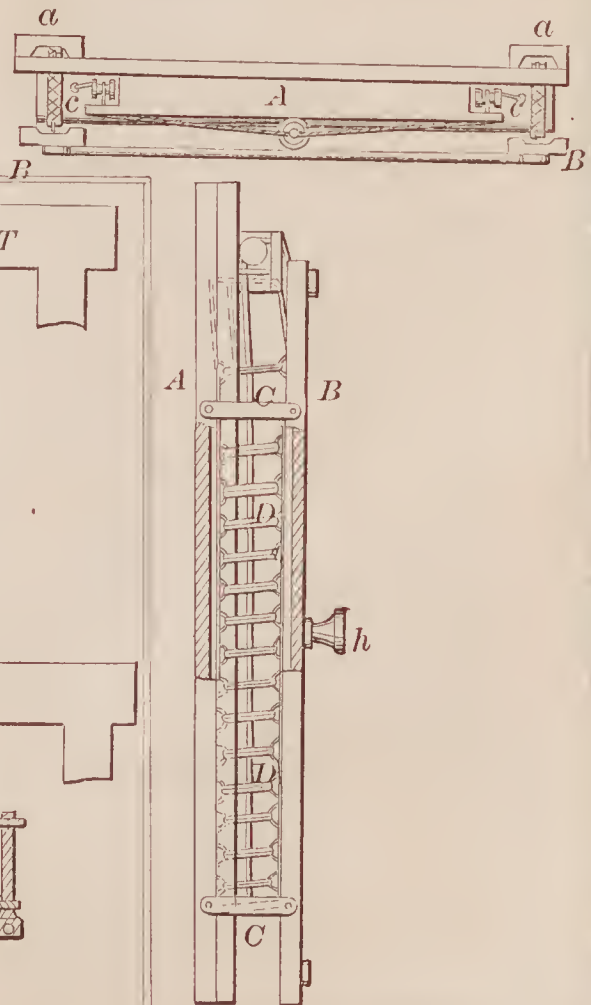
72332—S. W. Shorey—Window Blind.
