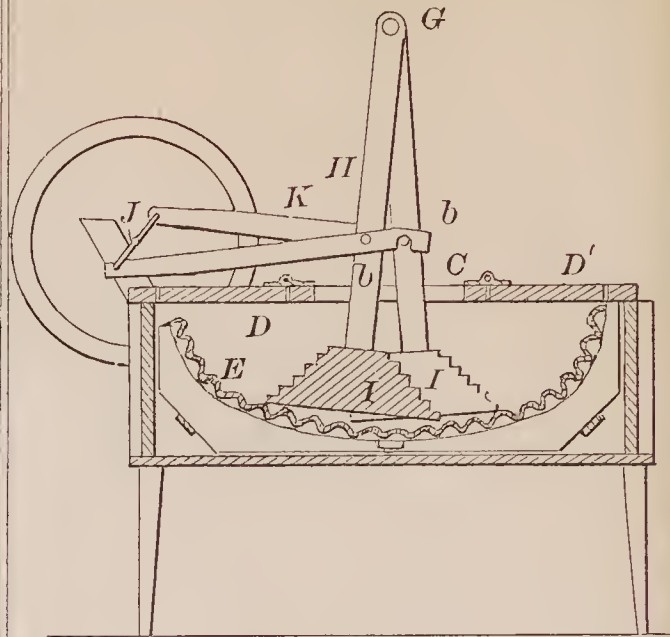
70630—G. C. Selfridge—Washing Machine.
