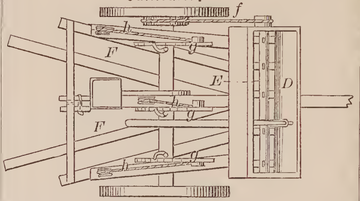
67009—W. & J. Whit—Sulky Harrow and Cultivator.
