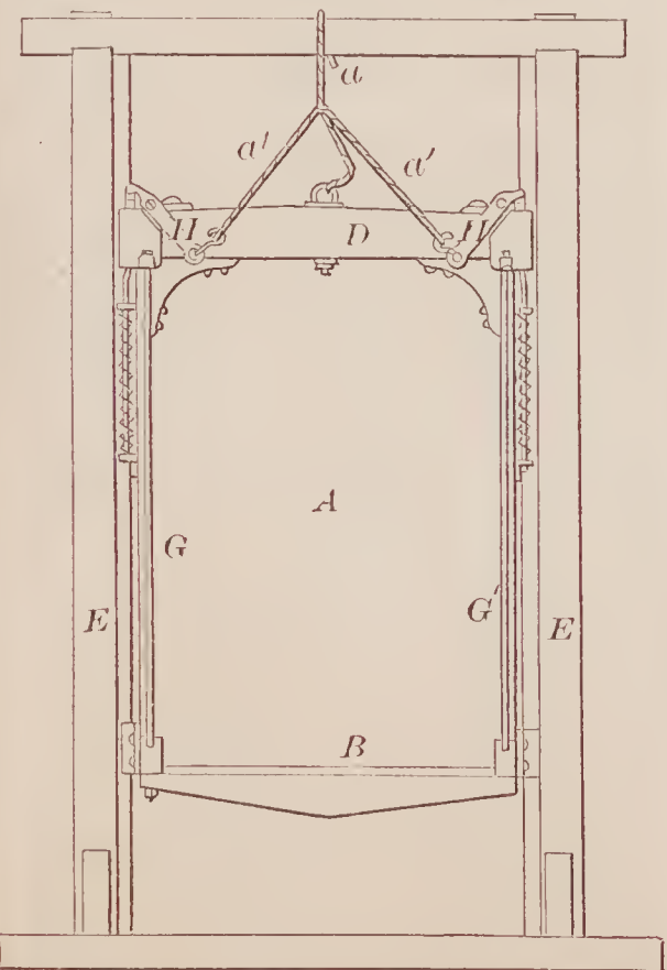
70941—C. W. Baldwin—Elevator.
