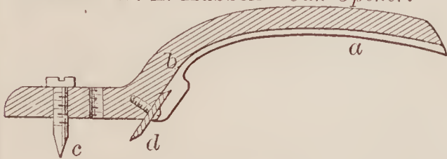
69996—W. L. Hubbell— Can Opener.
