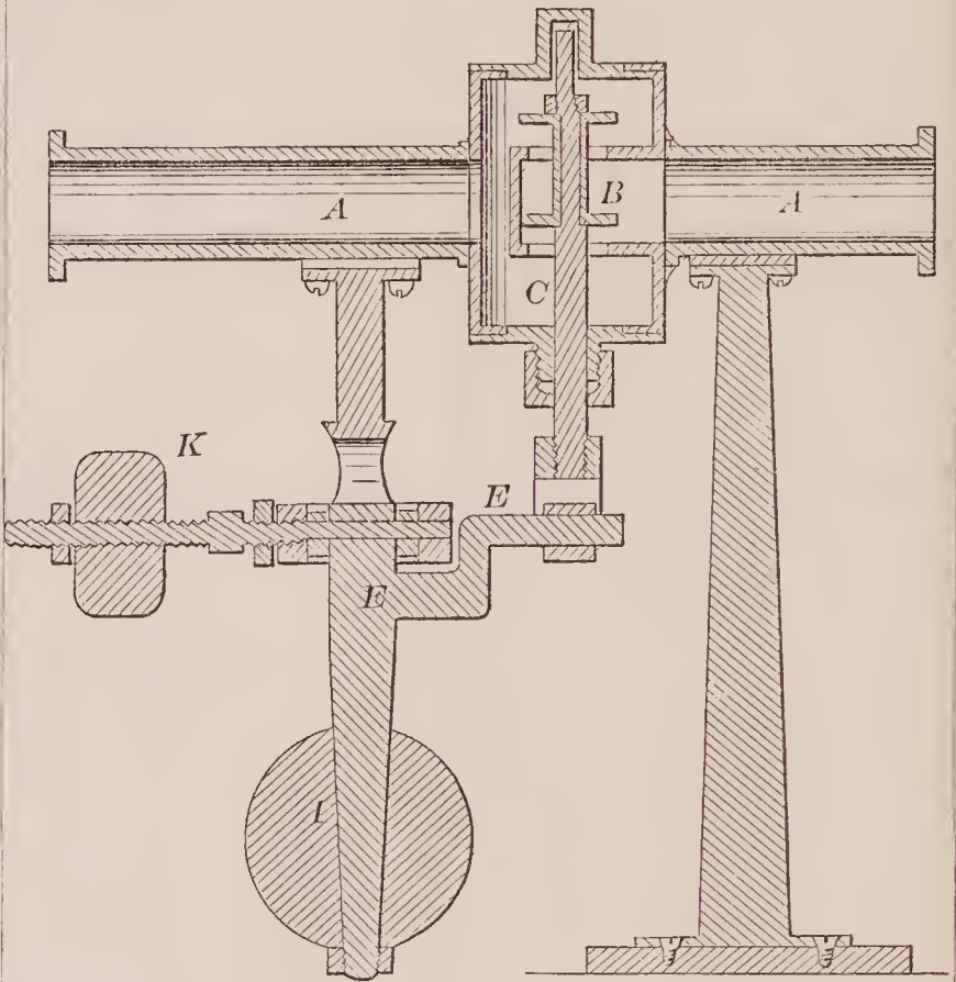
72239—J. Sullivan— Marine Engine Governor.
