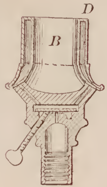
72244—E. R. Walker—Argand Burner.
