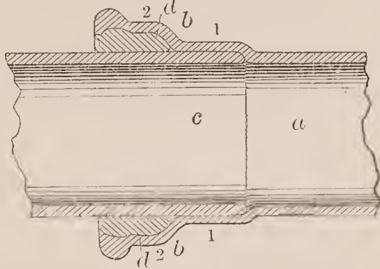
66782—E. G. Blakslee—Joint for Iron Pipes.
