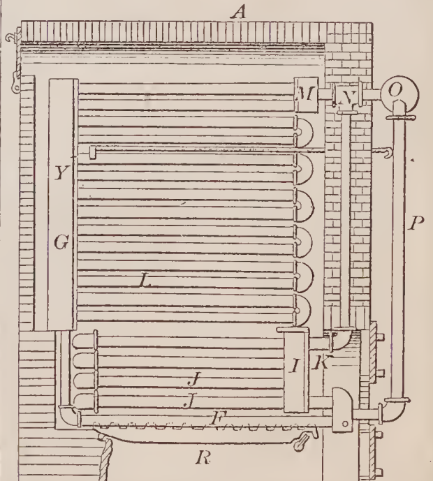
67505—R. T. Crane—Steam Generator for Heating.
