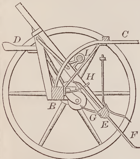
67675—M. Reilly—Trace Supporting Hook.
