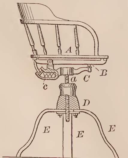
67034—R. Pitts, Jr.—Office Chair.
