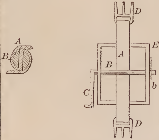
68465—T. G. Stansberry—Belt Tightener.
