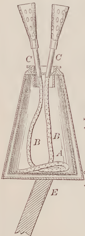
67244—J. Zimmerman—Lamp for Destroying Insects.
