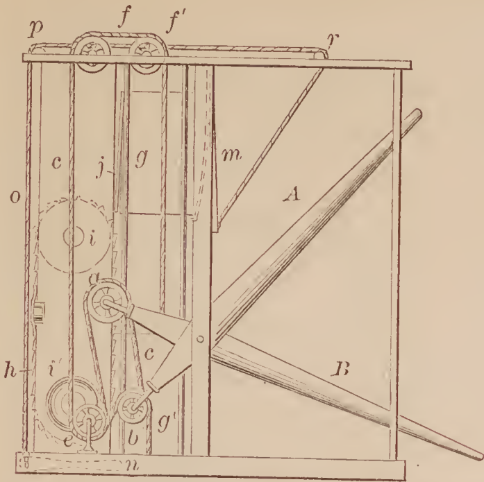
72881—D. Morrison—Carriage Motor.
