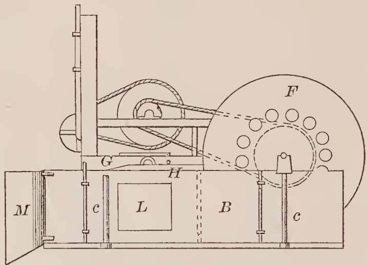
70423—H. Disston— For Setting Saw Teeth.
