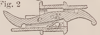
67893—H. Mansfield—Animal Trap.
