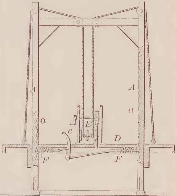
71791—C. Robinson—Scaffold.
