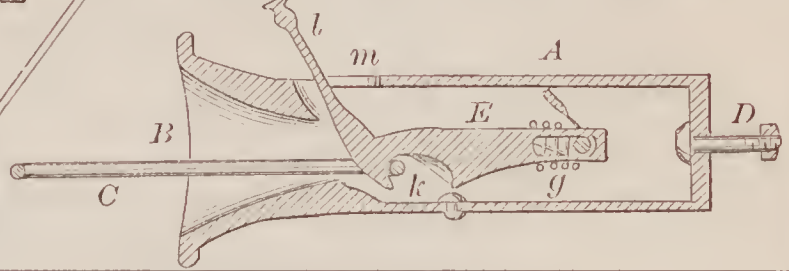
67209—S. O. Blemis—Car Coupling.
