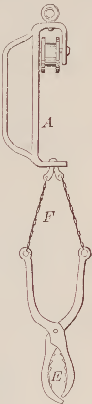
71628—J. K. Martin—For Hoisting Hogs in Slaughter Houses.
