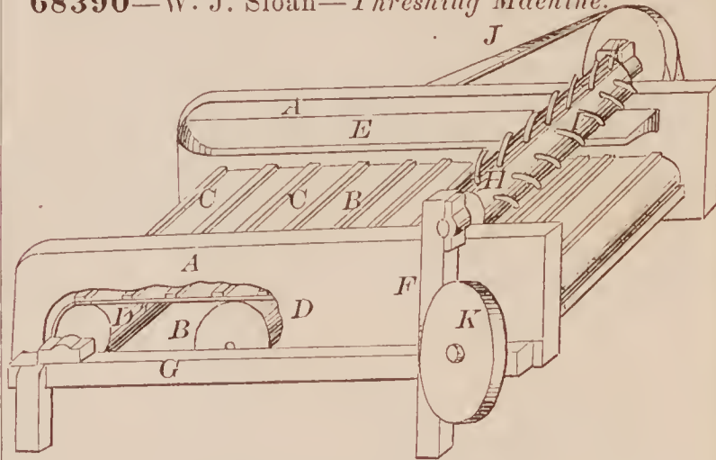
68390—W. J. Sloan—Threshing Machine.
