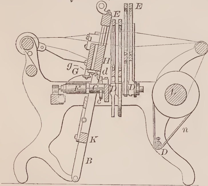
69516—W. B. Walker—Loom.
