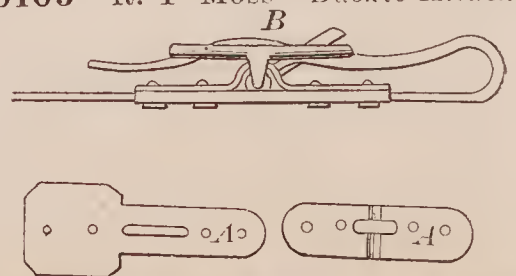
70105—R. T. Moss—Buckle Attachment.
