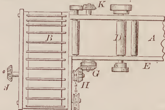
67544—A. C. Hobbs—Sewing Machine.
