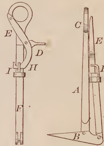
68407—A. Barbarin—Lightning Arrester.
