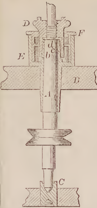
71127—J. E. Brown—Spindle Bolster.
