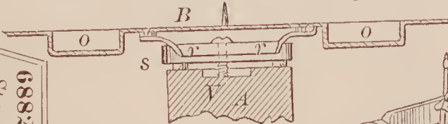
68828—A. Judson—For Sewing Oval Seams.
