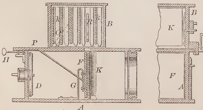
67981—D. H. Houston—Photographic Apparatus.
