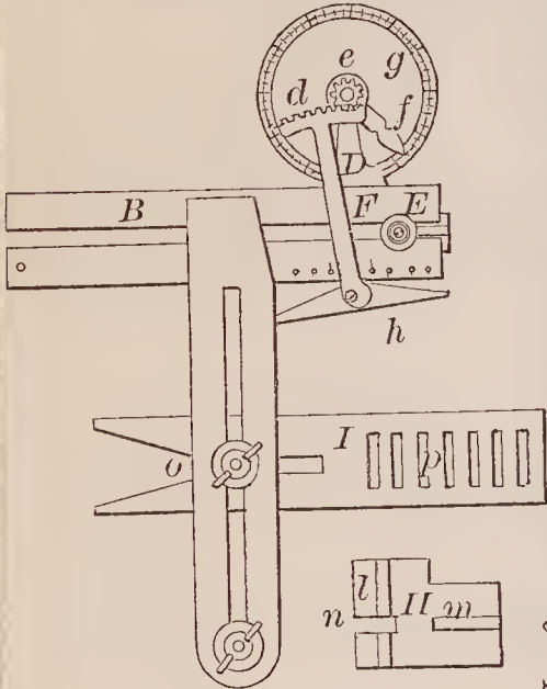
70547—J. Graham—Barel and Try Square.
