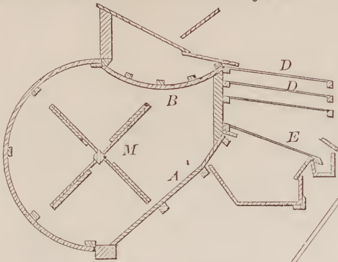
67206—Miller & Chase—Fanning Mill.
