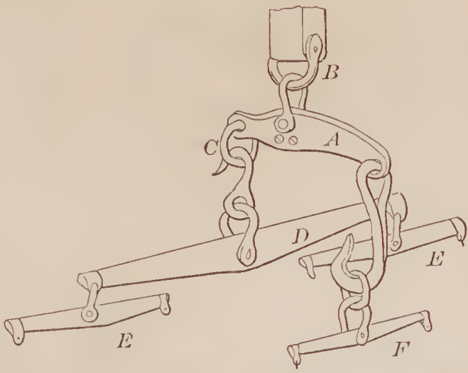
68548—J. B. Beam—For Casting Aluminium.
