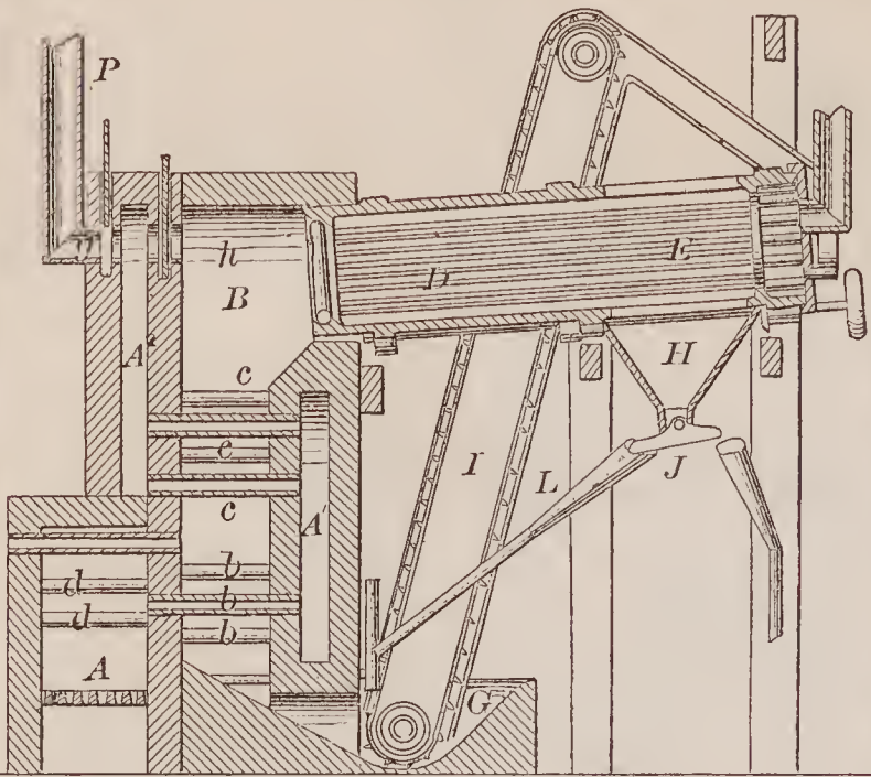
67497—T. J. Chubb—Furnace for Oxydizing Ores.
