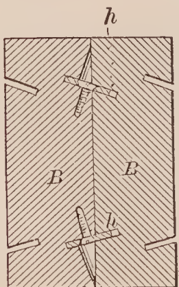
70879—E. Mets— Slide for Extension Tables.
