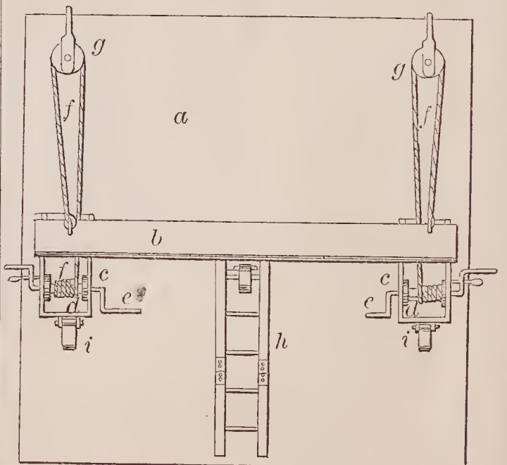
71140—N. B. Crawford—Scaffold for Roofs.
