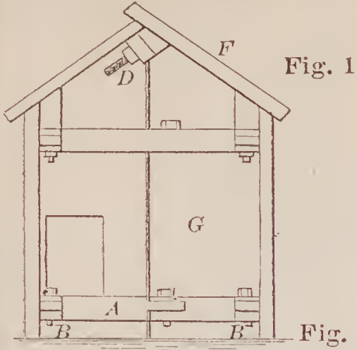
69580—D. Pangle— Sheep House.
