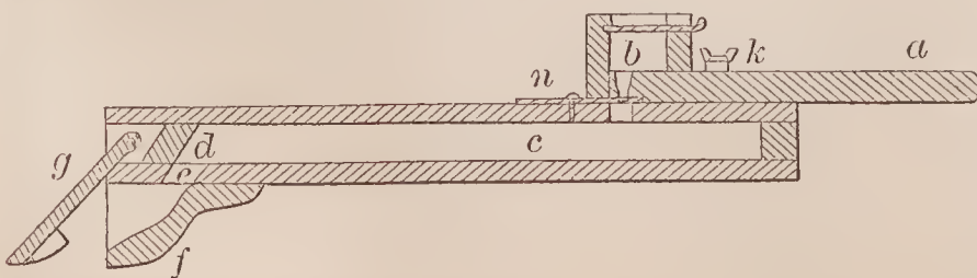
68173—H. V. Davis—Seed Drill.
