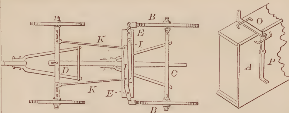
67126—G. Long—Wagon Brake.
