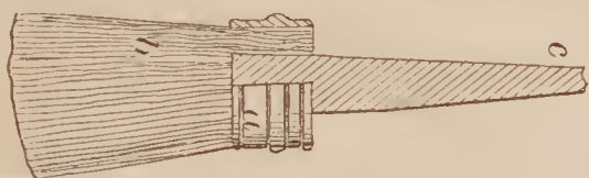
69009—W. S. Mead—Mechanical Movement.
