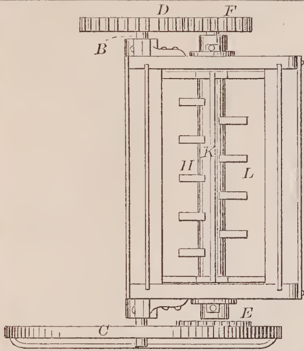
70961—J. Conver—Stove Pipe Drum.
