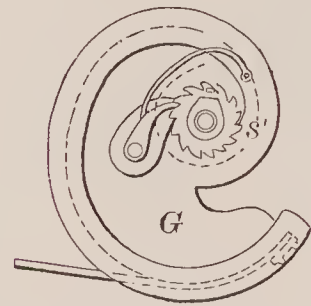
72606—F. W. Copeutt—For Labeling Bottle Corks.
