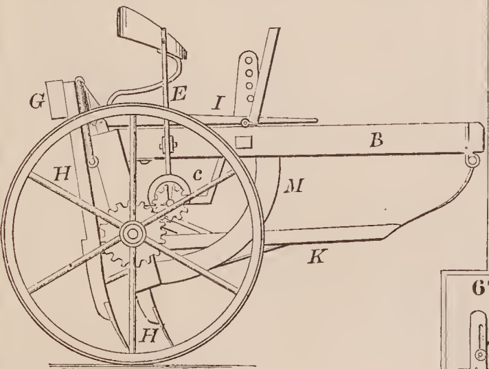
67141—J. Slauder—Broadcast Seeder.
