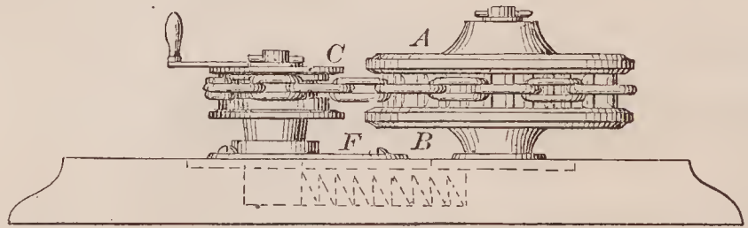
69243—S. Perry—Chain Wheel for Chain Horse Power.
