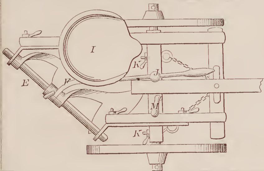
71302—P. Hatch— Saw Filing Machine.
