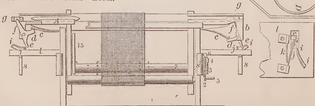
69516—W. B. Walker—Loom.
