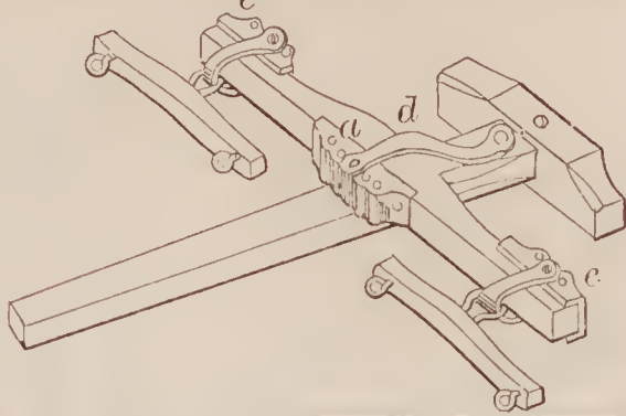
71262—C. L. Ames—Carriage Evener.
