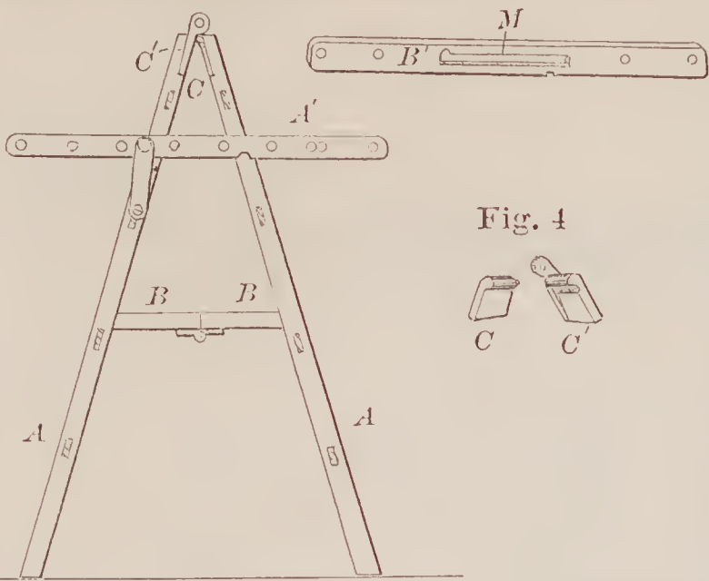
67270—I. A. Coons—Clothes Dryer.
