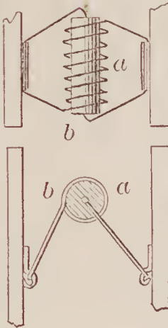
67186—F. Traps— Spring for Beds and Lounges.
