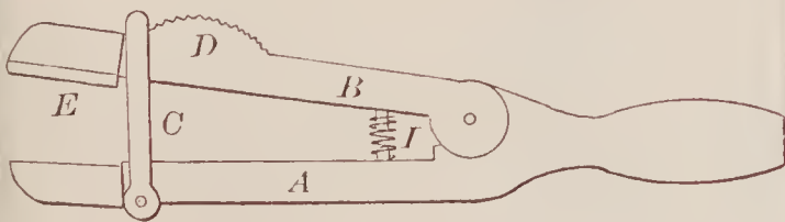
67987—J. S. Kalb—Wrench and Pruning Shears.
