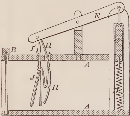
69777—J. Curtis—Animal Trap.
