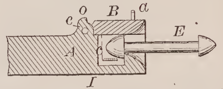
71675—W. J. Alexander—Gate.
