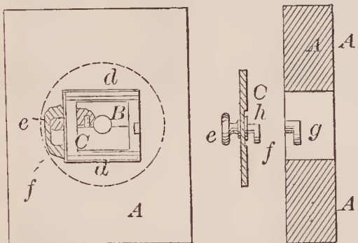
68543—C. R. Abbot—Safety Car Platform.
