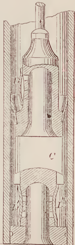
69635—J. E. Cronk—Pump Valve.
