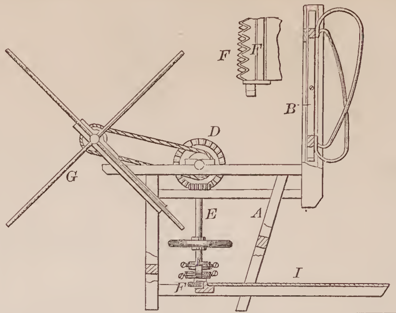
69412—J. C. Covert— Hold Back.
