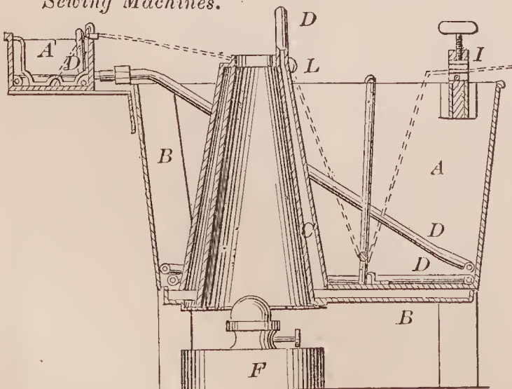
69056—L. R. Wiggin— Waxing Device for Sewing Machines.
