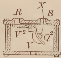
68810—H. Tyler—Pump.
