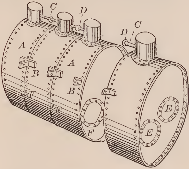
72530—A. W. Newell— Steam Generator.
