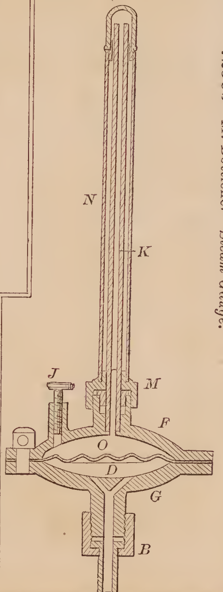
72595—M. Bötticher— Steam Gauge.
