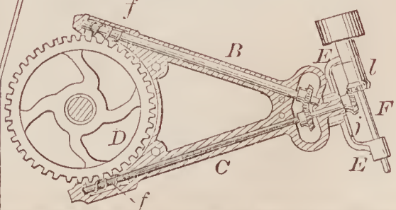
69787—L. B. Flanders—For Transmitting Rotary Motion.
