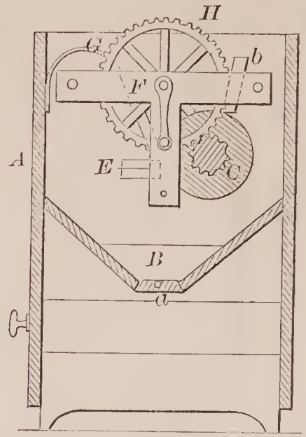
72020—J. Gould—Corn Sheller.
