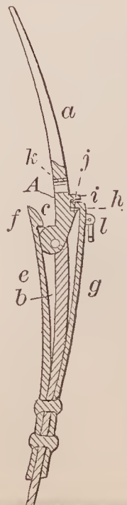
70135—W. Truby—Manure Fork, &c.
