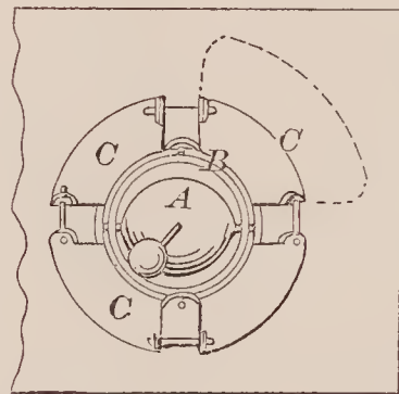
71693—G. W. Brown—Animal Trap.
