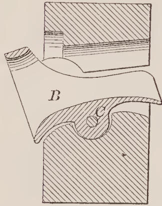
69630—J. F. Coburn—Hide Stretching Machine.
