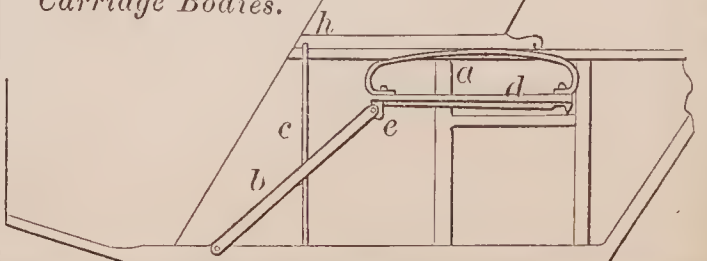
69397—R. F. Briggs—Seat for Carriage Bodies.
