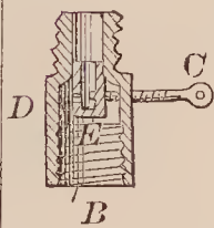
72415—G. Mooney—Gas Burner.
