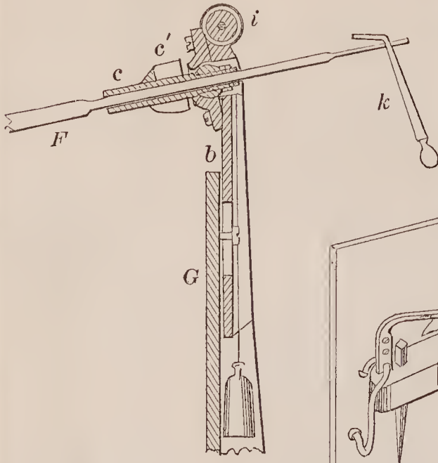
71149—J. Elson—Breech-Loading Fire Arm.
