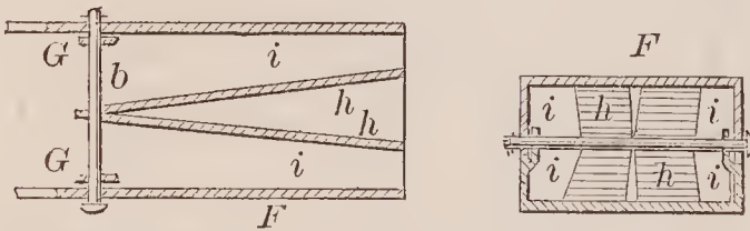
71974—Butterfield & Read—Sad Iron.
