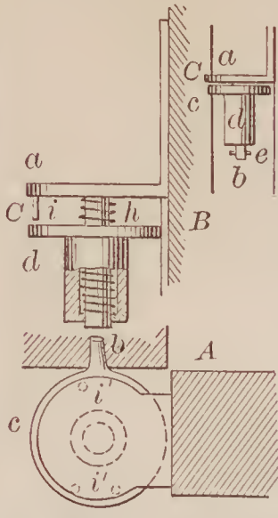
70284—J. Stewart—Attaching Axes to Handles.
