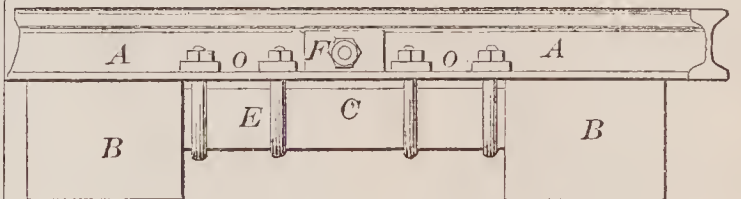
67626—J. Anthony— Joint Splicer for Railroad Rails.
