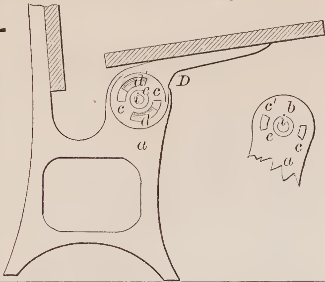
69856—G. W. Starr— Railroad Switch.
