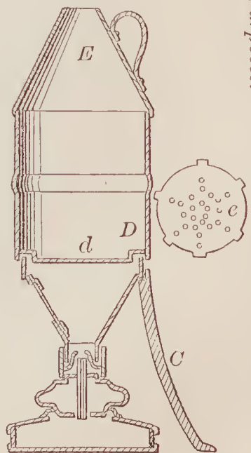
69670—J. C. House—Lamp Heater for Dental Purposes.
