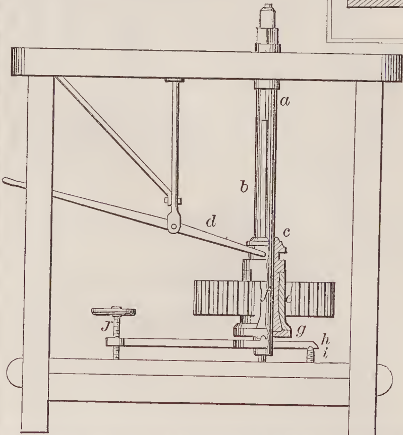
72661—J. H. McMinn—Mill Spindle.
