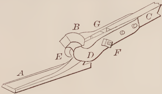
70225—W. J. Keeney—Pitman Coupling.
