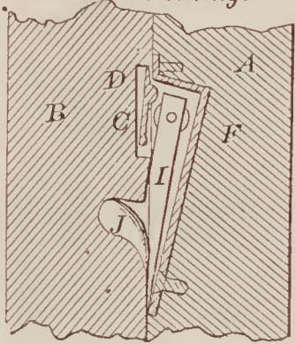
67472—M. V. B. White— Sash Fastening.
