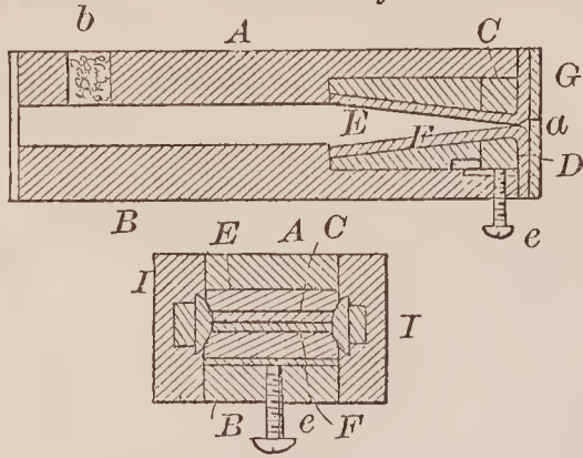
67434—I. Jewett—Knife Cleaner.
