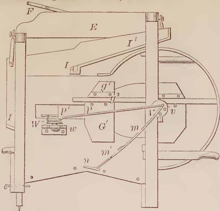
70885—H. Ogborn— Fanning Mill.
