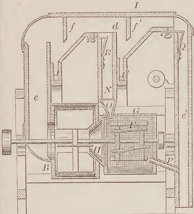
69634—W. W. Conner—Smut Machine.
