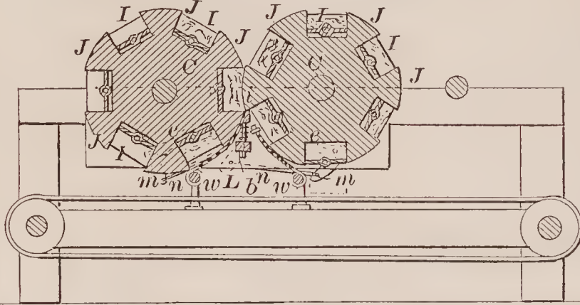
72137—P. V. Westfall—Brick Machine.
