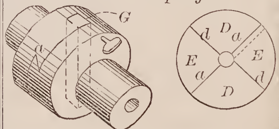
67878—H. A. Hurd—Shaft Coupling.
