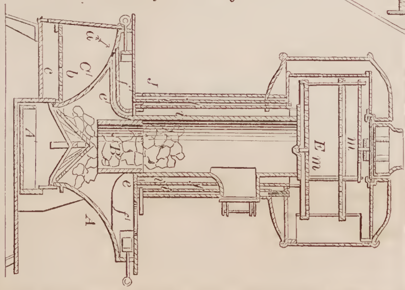
71421—H. Stickney—Cooking Stove.
