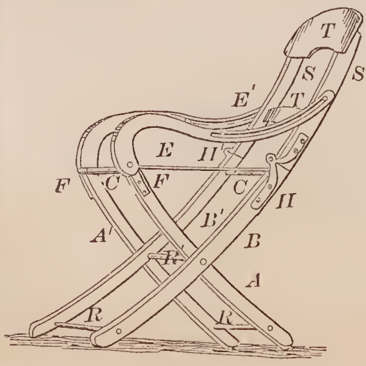
69145—E. W. Vaill—Folding Chair.
