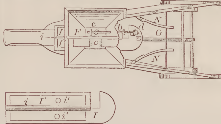
67444—Mitchell & Search—Corn Planter.
