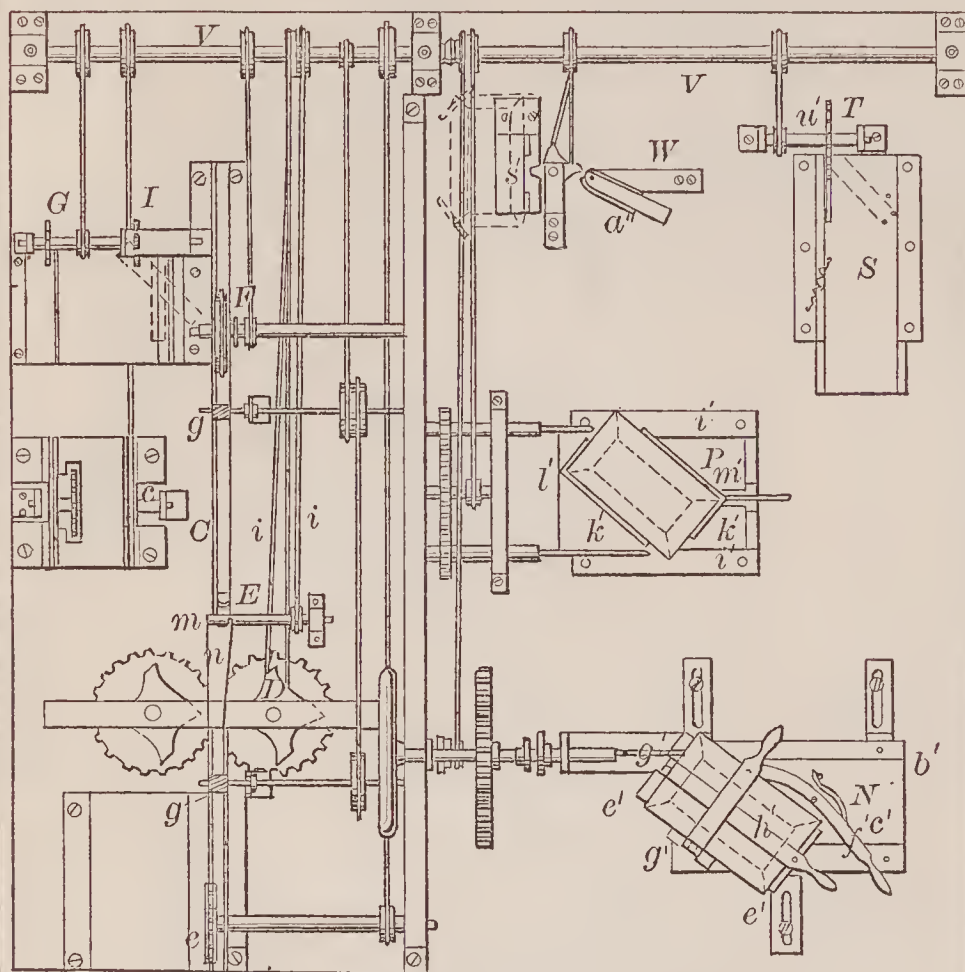
67318—P. H. Kimball—Water Elevator.
