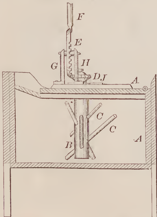
67597—H. Sidle— Washing Machine.
