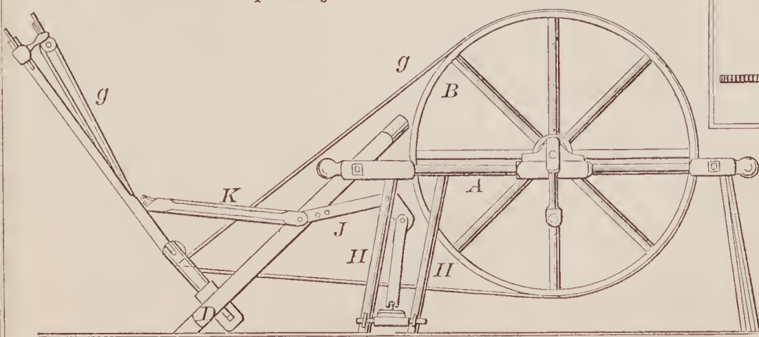
71897—H. Miller—Spinning Wheel.
