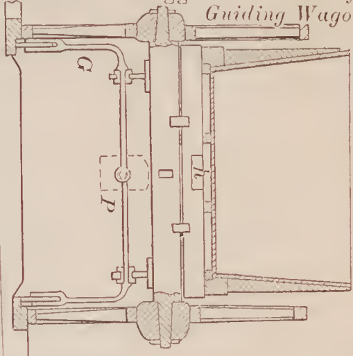
70260—M. O. Potter— Creel for Winding Yarn.
