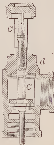
67460—J. Stowell—Safety Lock.
