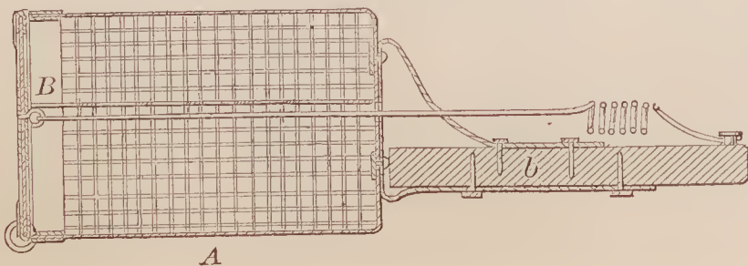
70723—E. G. Kinsley—Corn Popper.
