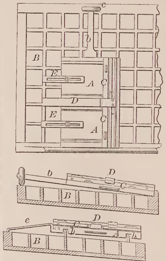
70866—V. Lapham—Bolt Fastening.
