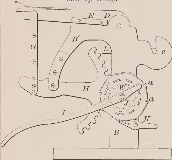
71181—A. A. Kent— For Cutting, Punching and Upsetting.
