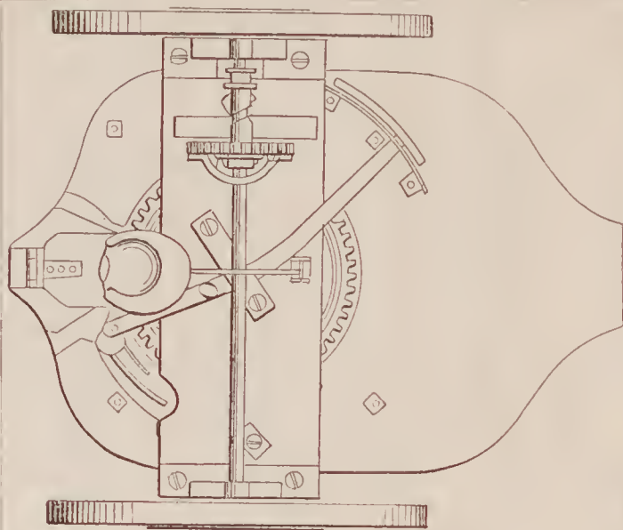
71263—J. Armstrong—For Planting Cotton Seed.
