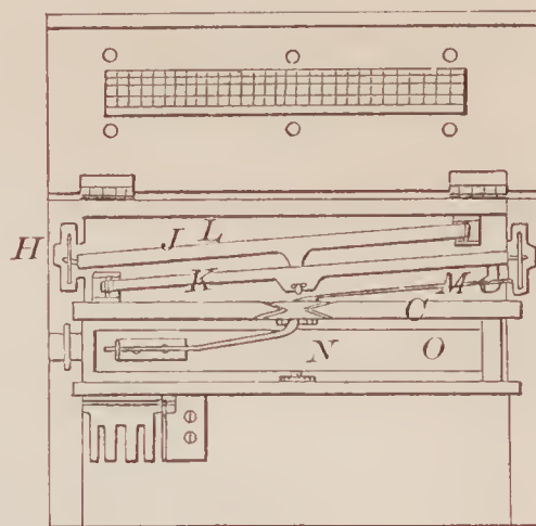
69695—S. Pence—Animal Trap.
