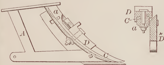
69996—W. L. Hubbell— Can Opener.
