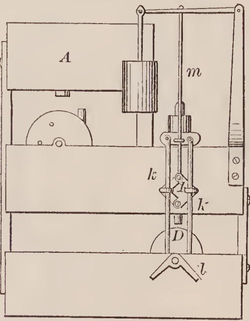
72701—I. P. Tice—Spirit Meter.
