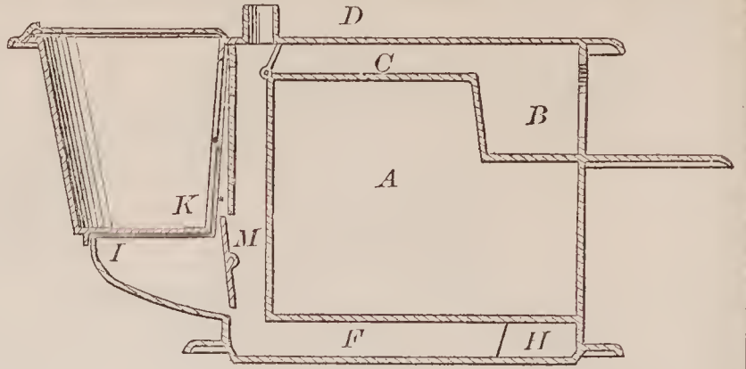
67670—D. E. Paris—Cooking Stove.
