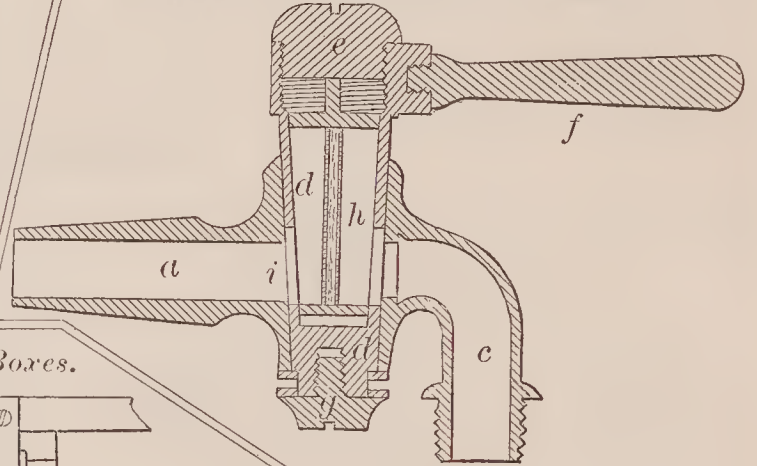
68170—R. B. Coar—Filter Faucet.
