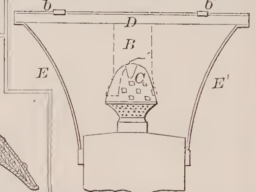
71656—T. Smith—Washing Machine.
