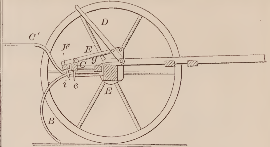
66894—D. P. Sharp—Horse Rake.
