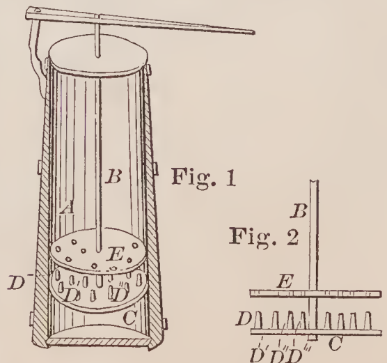
69795—M. C. Gordon—Churn.
