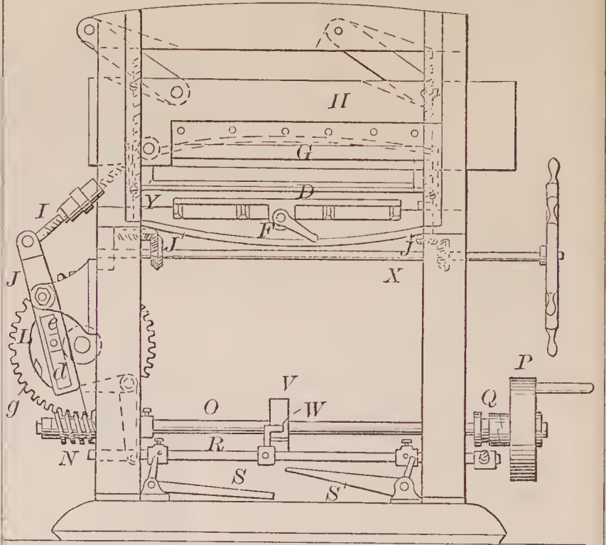
70292—S. D. Tucker— For Cutting Paper, Pasteboard, &c.
