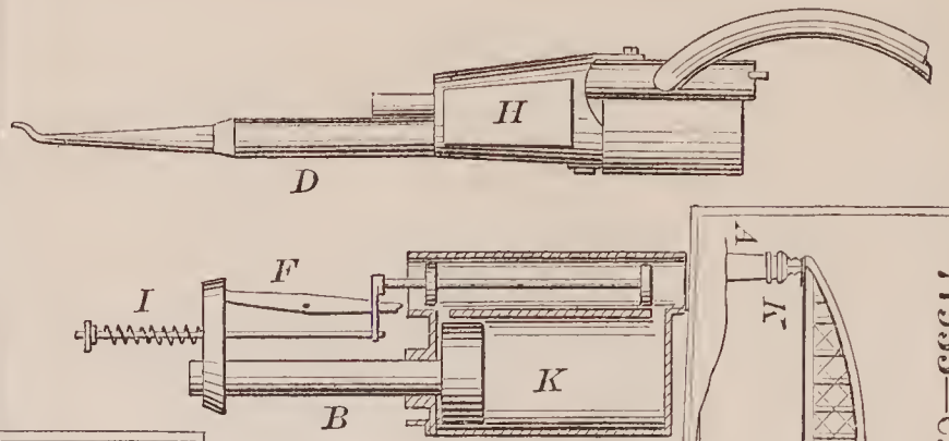
71950—Bannister & Green— Automatic Tooth Plugger.
