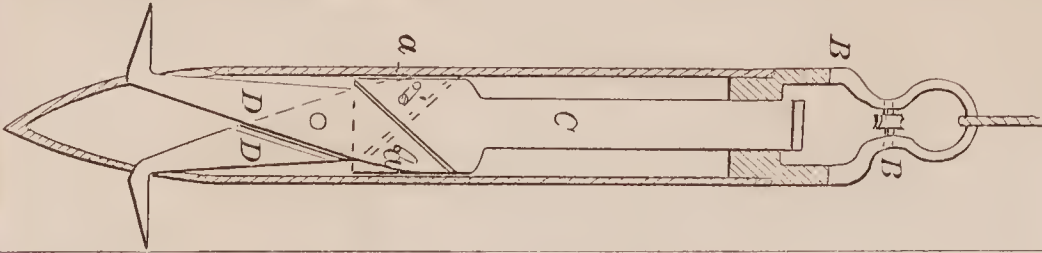
72272—D. Dick—Wood Turning Lathe.
