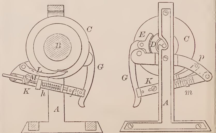
70297—R. Walker— Let-off Motion for Looms.
