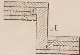
72246—Walters & Shaffer—Fagot for Manufacturing Wrought Beams.
