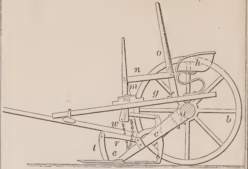
70004—G. W. King— Horse Rake.
