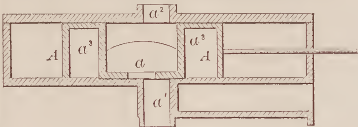
71016—A. Hutton— Steam Engine Valve.
