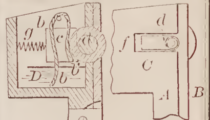
71145—W. A. Devon—Self-Lubricating Globe.
