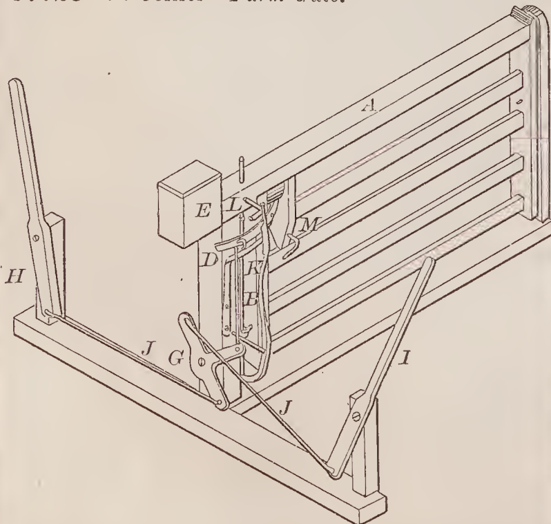
67723—L. Collier— Farm Gate.
