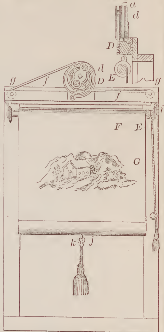
67272—Cox & Hill—Applying Window Shades to Windows.
