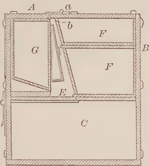
69493—J. Schermerhorn—Washing Machine.
