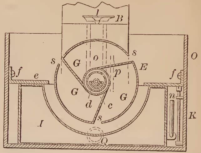
72774—M. Augenstein—Spirit Meter.
