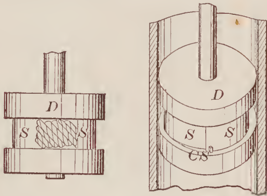
69747—M. W. Baily— Piston Packing.
