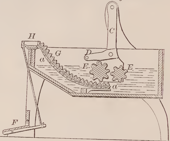
70882—A. Neilson— Washing Machine.
