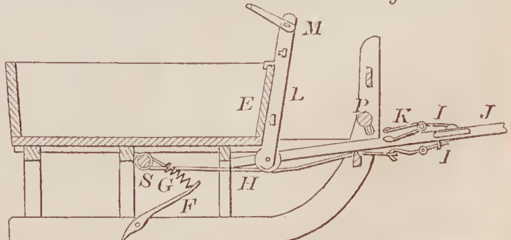
69717—H. W. & B. C. Smith—Sleigh Brake.
