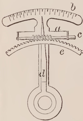
71924—W. B. Tucker—Watch Regulator.
