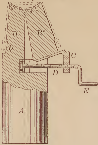
72797—H. Carpenter— Form Block for Baskets.
