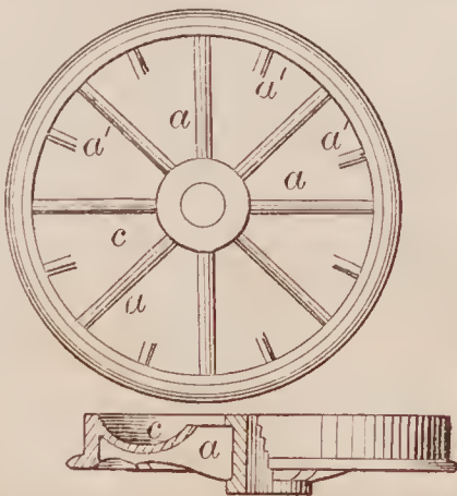
71408—G. Peacock—Cast Iron Car Wheel.
