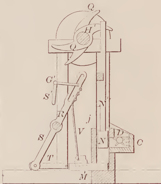
71163—E. M. Hamilton— For Pressing Peat, Clay, &c.
