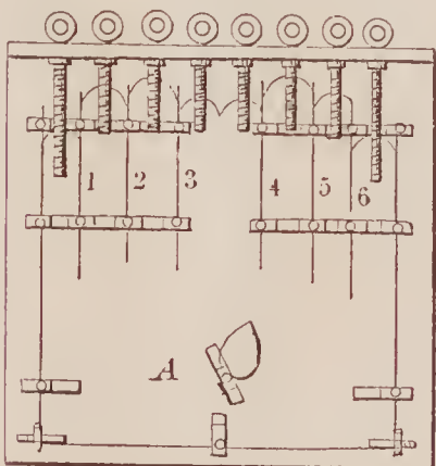
72197—Harlan & Pomeroy— For Cutting out Gloves.
