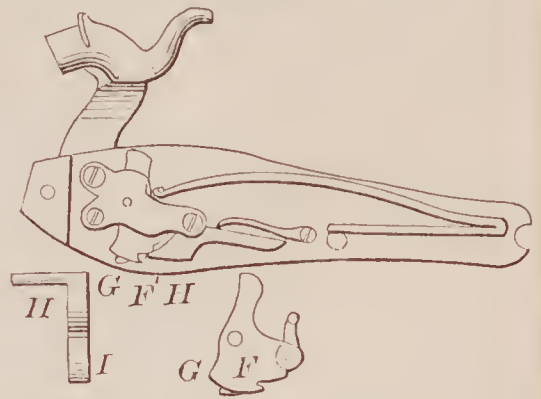
71963—C. Bowlen—Gun Lock.
