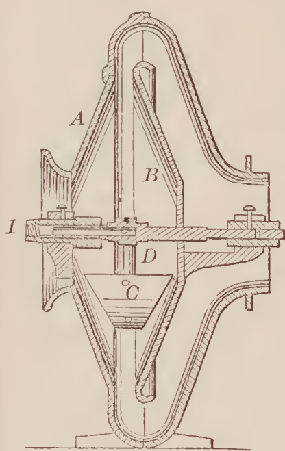
71569—Bassett & Smith—Steam Blower.
