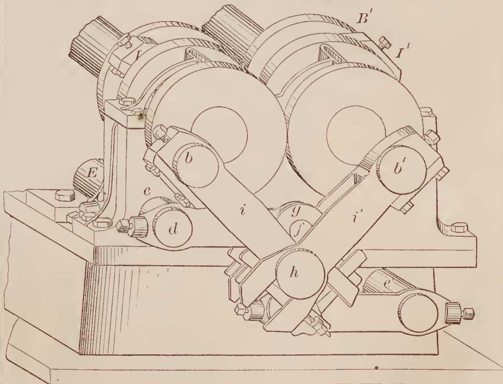
68754—G. H. Knight— Mechanical Movement.
