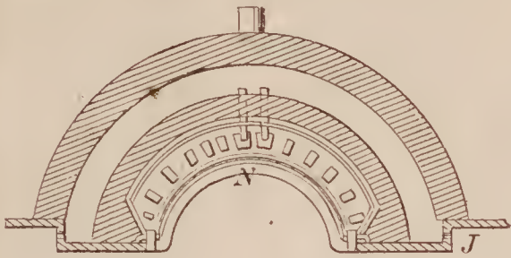
68653—E. Y. Robbins—Fireplace.
