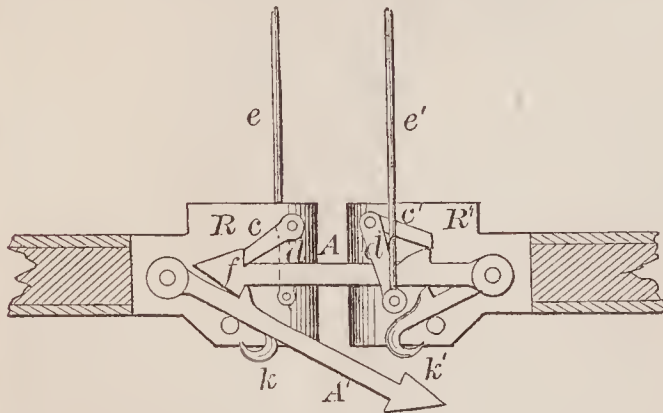
69972—T. F. Conner—Car Coupling.
