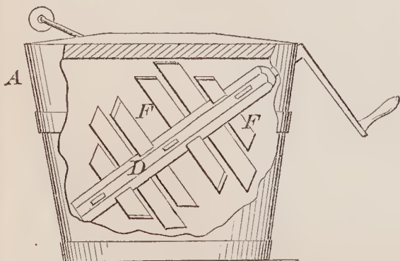
69934—E. Porter—Churn.
