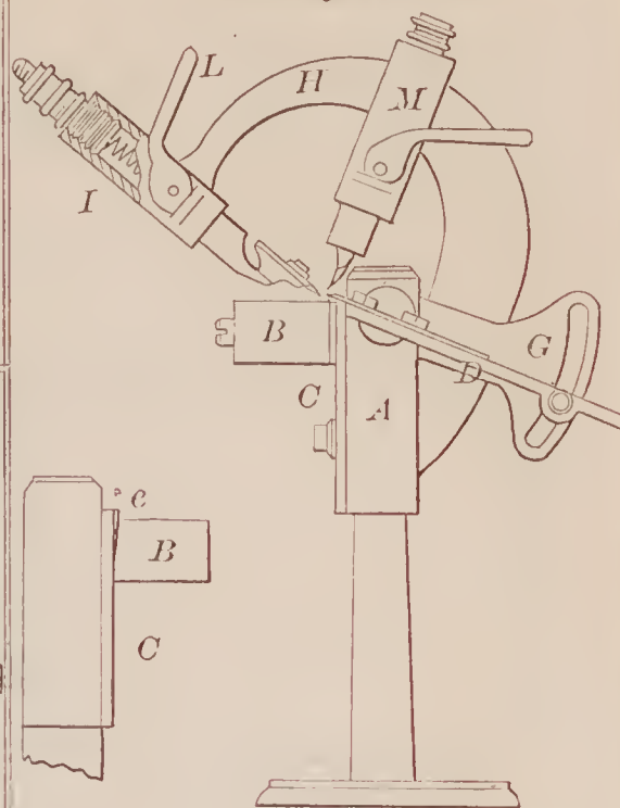
68094—I. Manning—Channeling and Beveling Machine.
