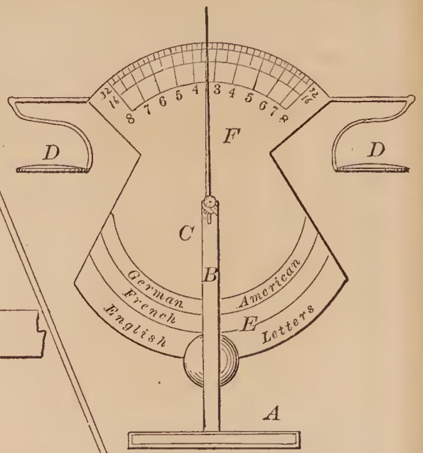
72593—I. Bisbee— Balance.
