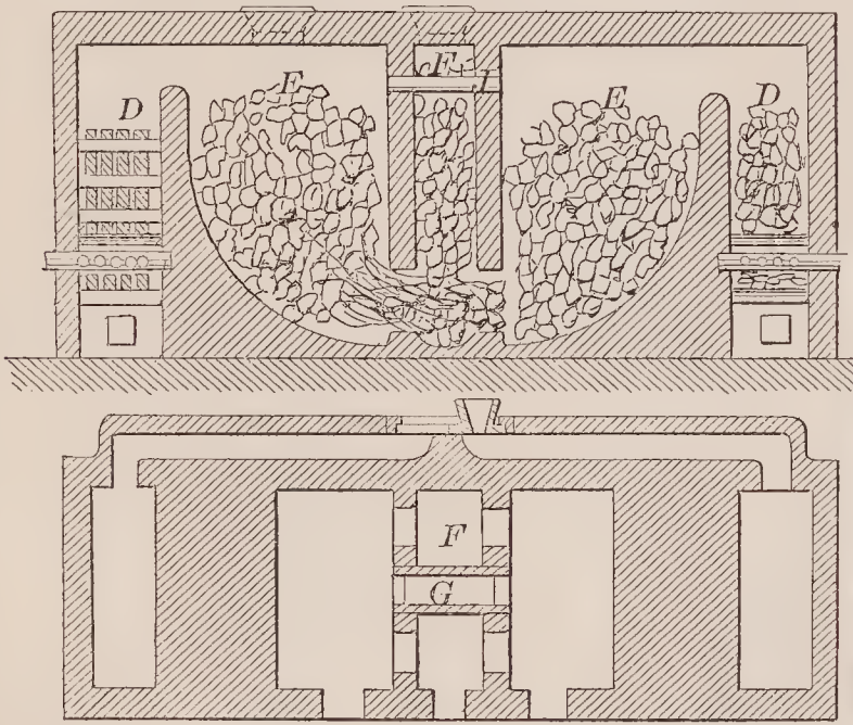
71776—J. Maunton—For Roasting and Reducing Ores.
