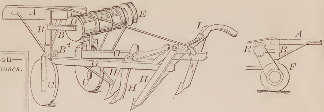
68563—P. Hackett—Seed Sower and Corn Plow.
