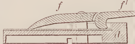
71582—I. Cook—Cow Milking Machine.
