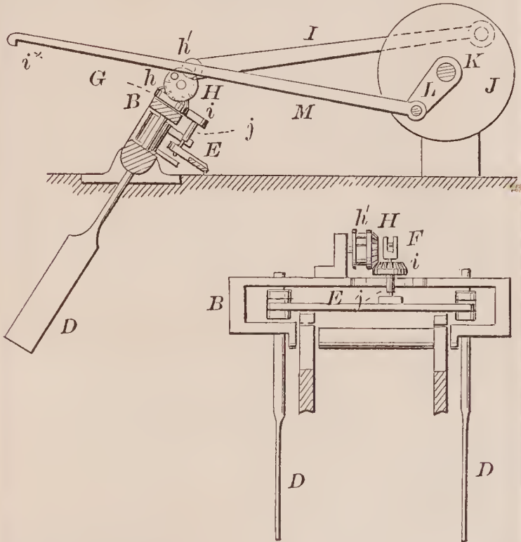
72319—N. Nolan—Propeller.
