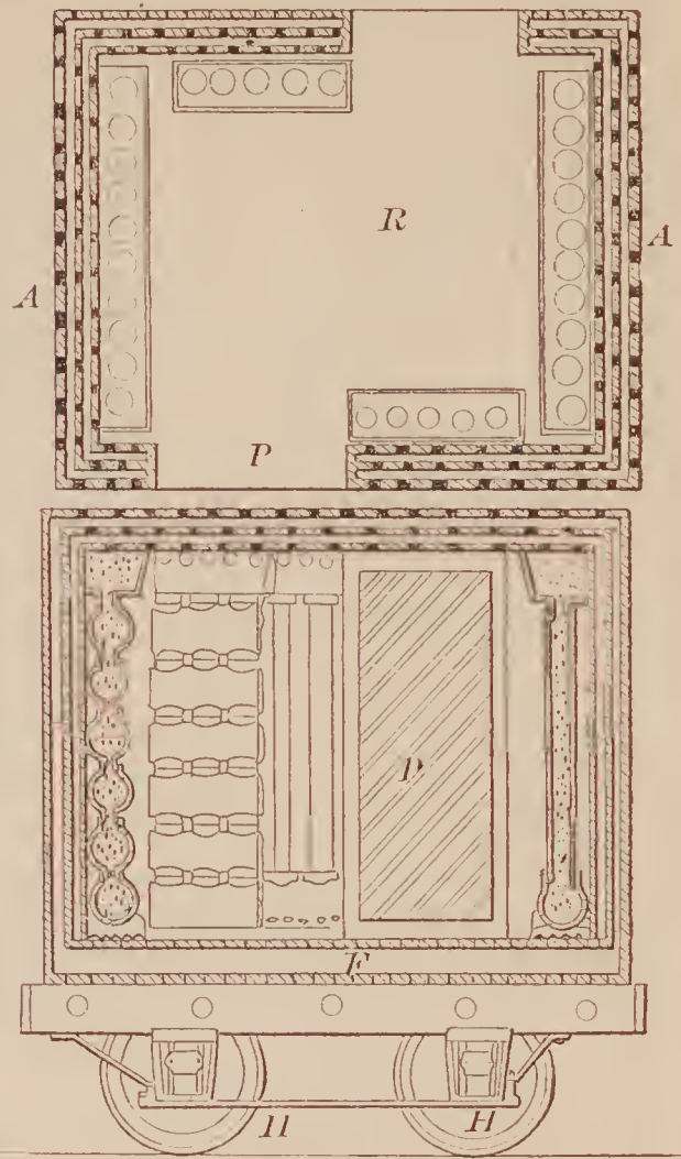
72895—C. F. Pike—Railroad Car for Preserving and Transporting Meats, &c.
