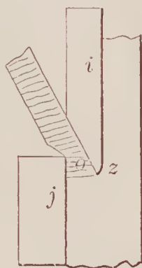
67312—E. Jewett—Manufacturing Veneers.
