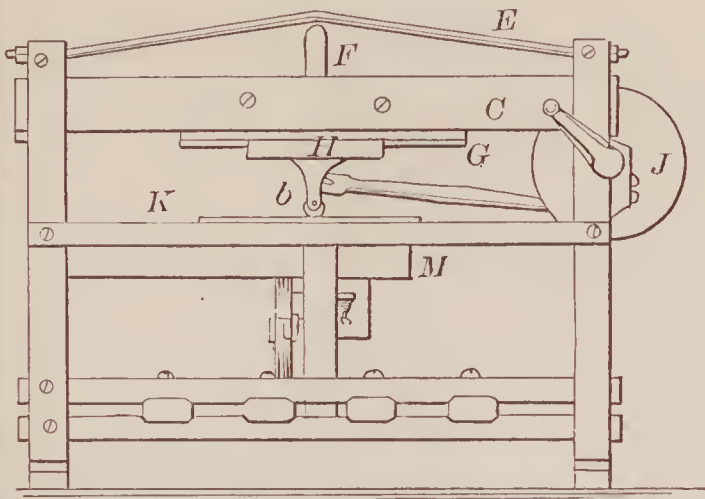
71929—J. H. Walker—For Rolling Leather.
