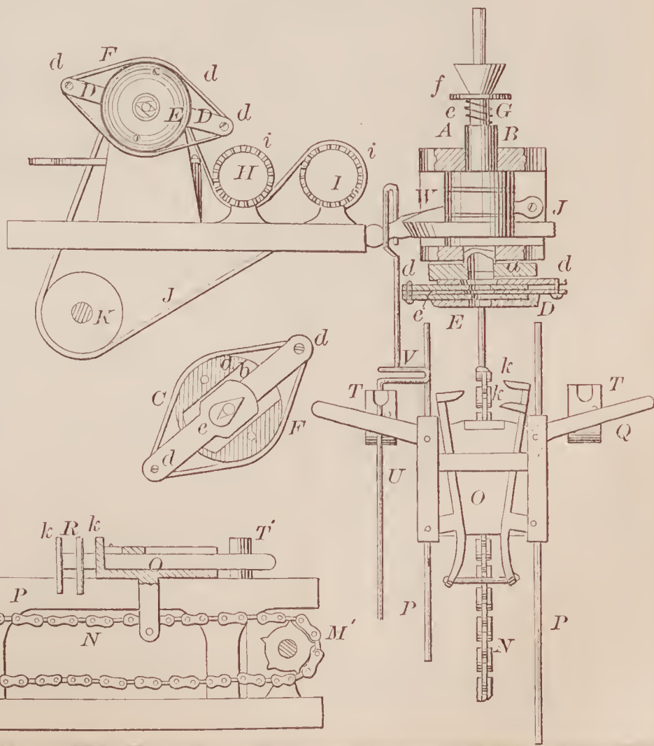
70288—J. Swan—For Stripping Willow.
