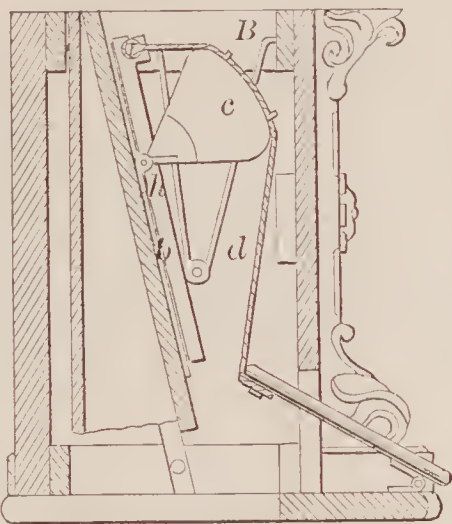
71245—E. H. Thomas, Jr.— Organ Bellows.
