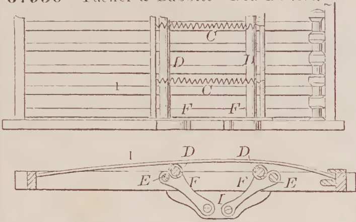
67930—Tucker & Babbitt—Bed Bottom.
