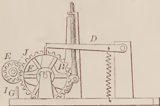
67166—Clinton & Mood— Calendar Clock.
