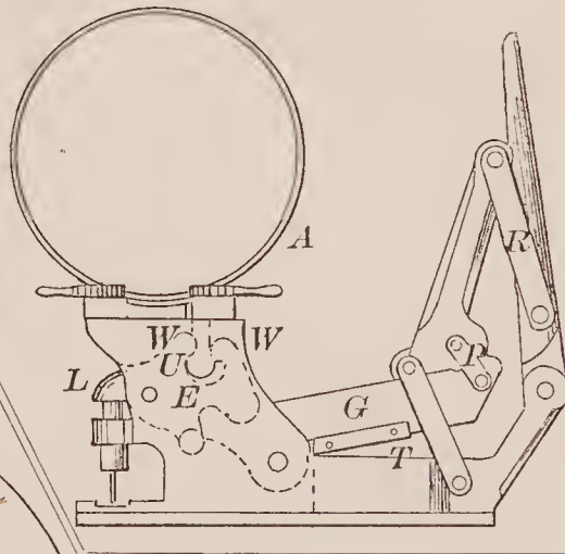
70366—J. J. Sandgren—For Shearing, Punching and Upsetting.
