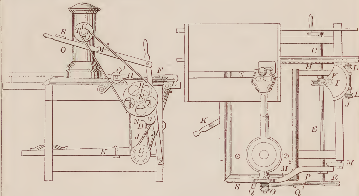
72182—S. Fountain—Concentrator and Amalgamator.
