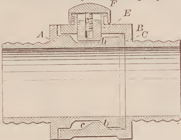
66804—Curtis & Tewksbury— Hose Coupling.
