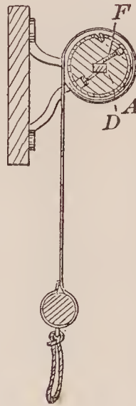
69176—W. Campbell—Window Shade Fixture.
