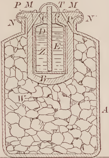
70426—Elmer & Hubert—Ozone Generator.
