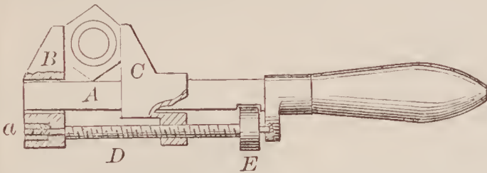
67818—G. C. Taft—Wrench.
