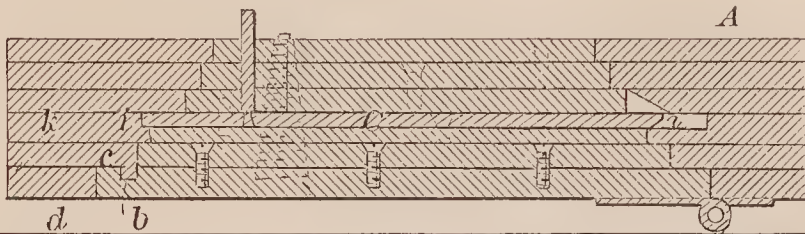
67046—J. L. Hall— Connecting Door and Casing of Safes.
