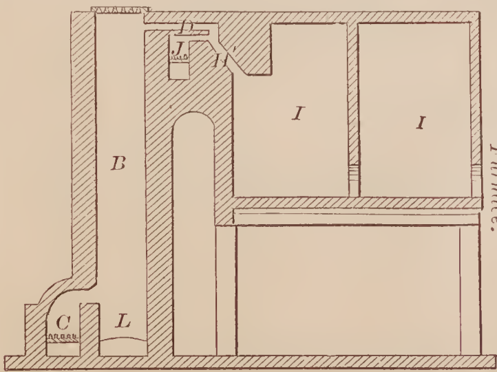
72931—C. Stetefeldt— Ore Roasting Furnace.
