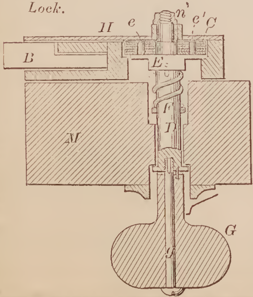
72408—I. W. Lamb— Permutation Lock.
