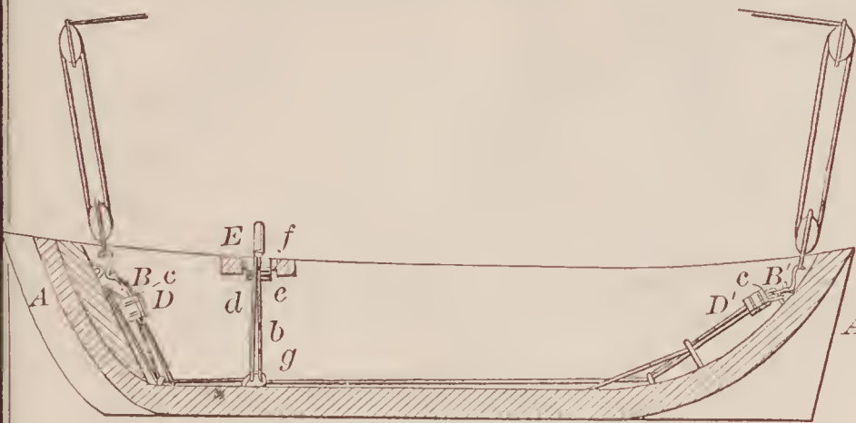
70354—Peterson & Gunner— Boat Detaching Tackle.
