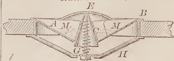
67377—M. Traver—Spittoon for Railroad Cars.
