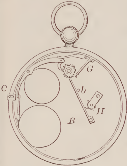
67704—T. Baker—Stop Watch.
