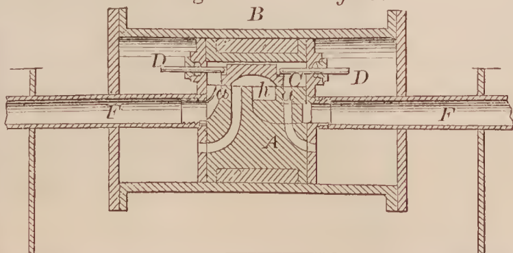
68721—J. Fairelough—Steam Engine.
