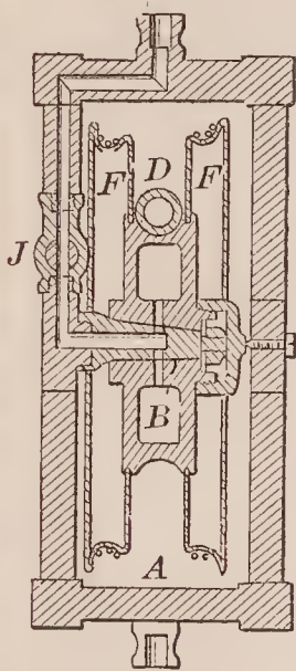
70401—G. Bowerman— Stock and Poultry Feeder.
