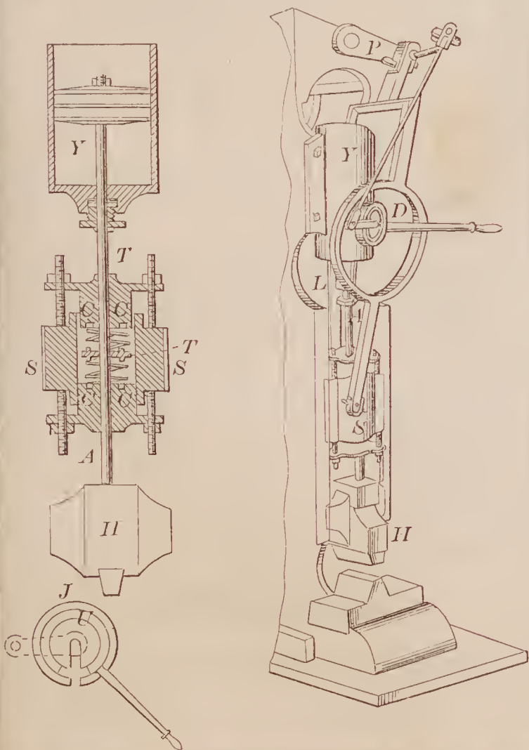
68740—T. B. Harrison— Power Hammer.
