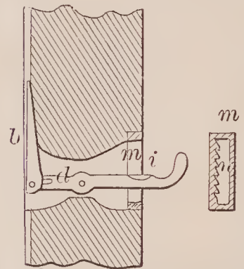
72096—J. W. Simpson— Window Sash Supporter.
