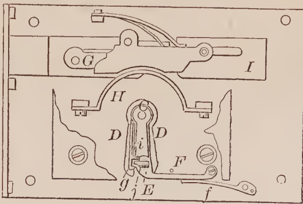
70232—R. Lewis—Safe Lock.
