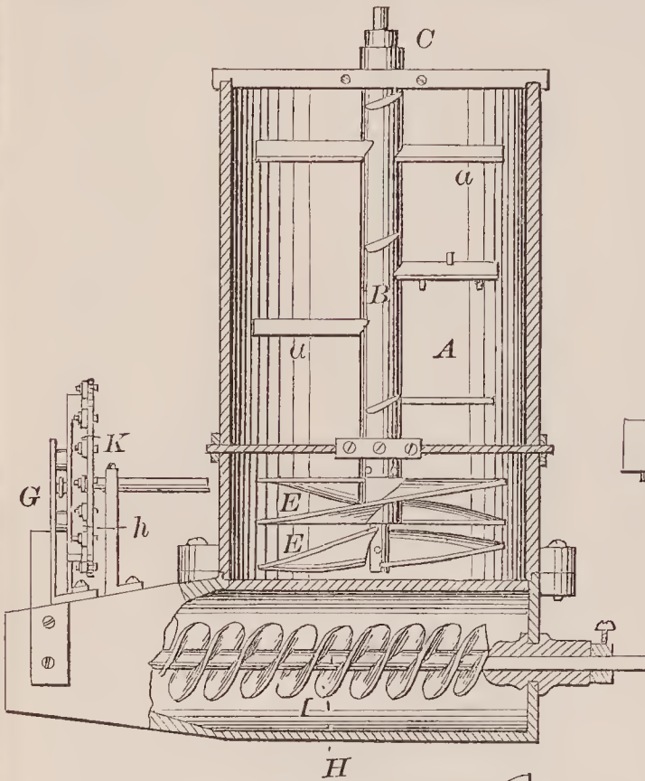
71870—G. D. Goodrich— Peat Machine.
