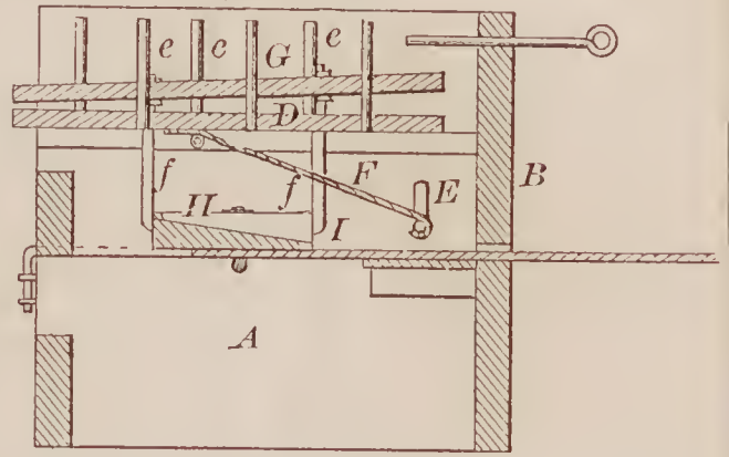
72161—S. Brackett—For Separating Roots from Peat.
