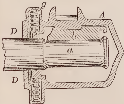
71125—W. A. Boyden—Axle Box.
