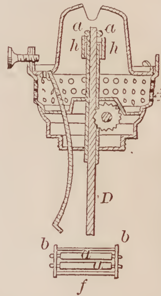
70392—W. P. Bennett— Lamp Extinguisher.
