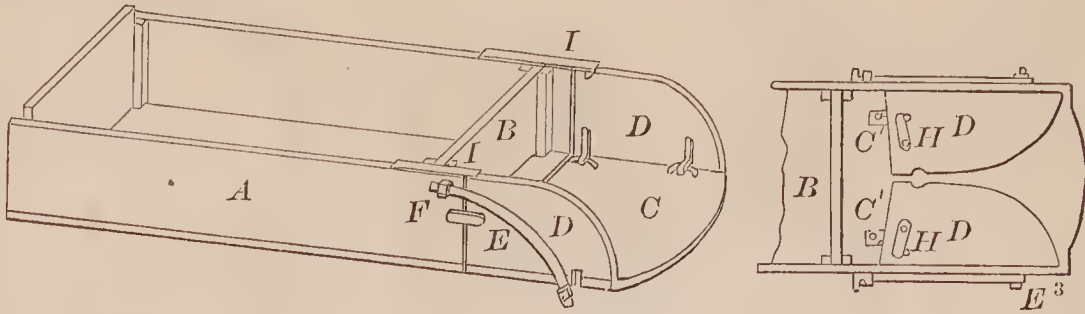
68772—Meredith & Mulligan— Extension Bed for Farm Wagons.
