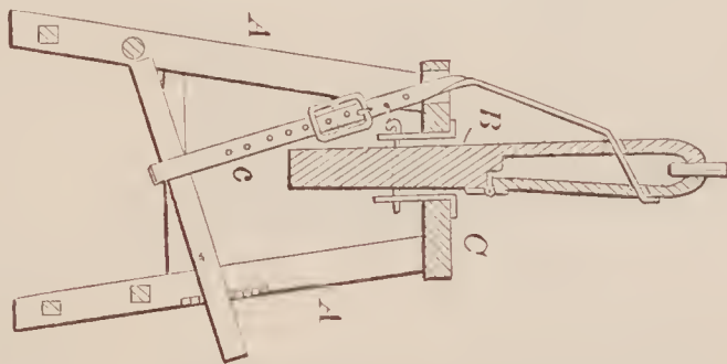
66808—O. A. Dean— Stitching Horse.
