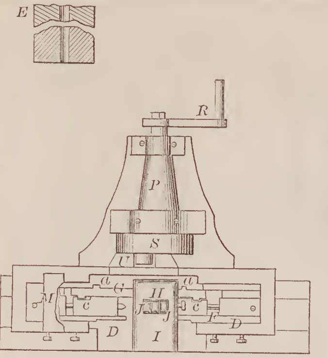
67403—J. R. Bridges—For Making Nuts.
