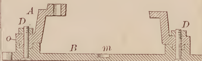
68685—H. Basch—Permutation Trunk Lock.
