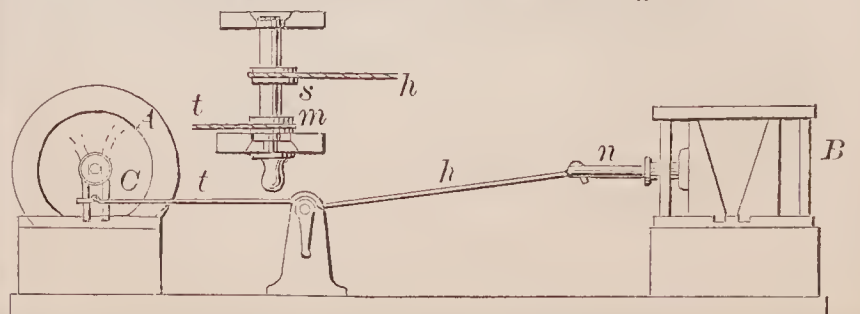
71547—W. M. Stevenson—Steam Cut-off Valve.
