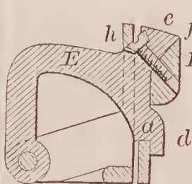
71452—Cady & Cooper—Concealed Hinge.
