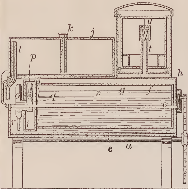
71518—C. C. Lloyd—Dry Gas Meter.
