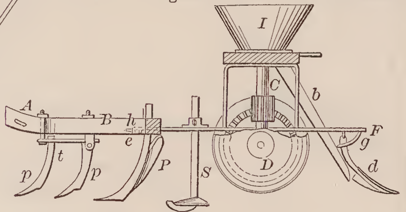
72703—J. Vaughn—Planter and Cultivator.
