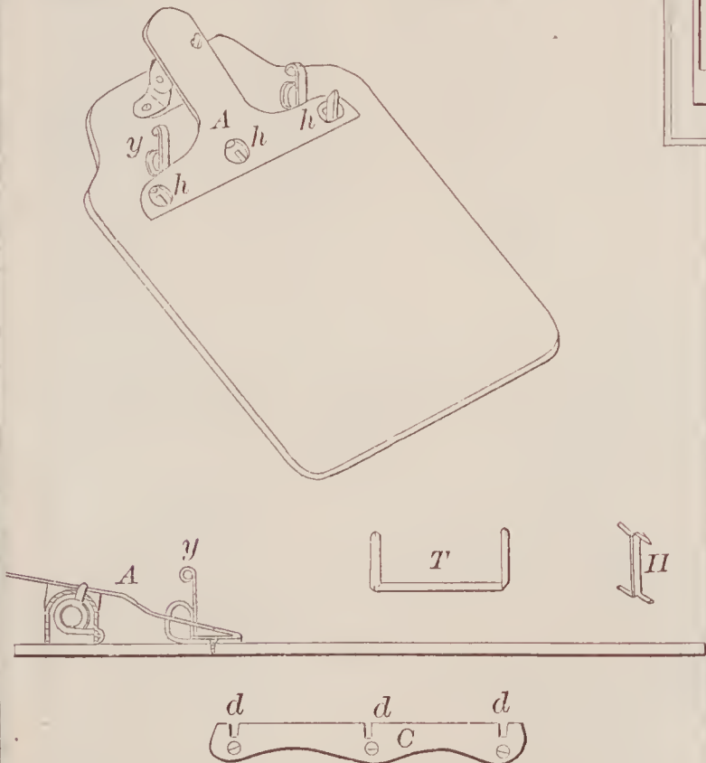
71635—J. H. Parsons—Paper Clip.
