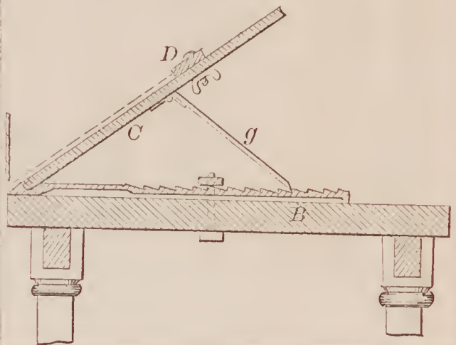
72248—G. Watt—Whiffletree.
