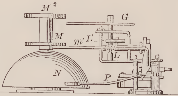
71637—C. E. Pierce— Burglar Alarm.
