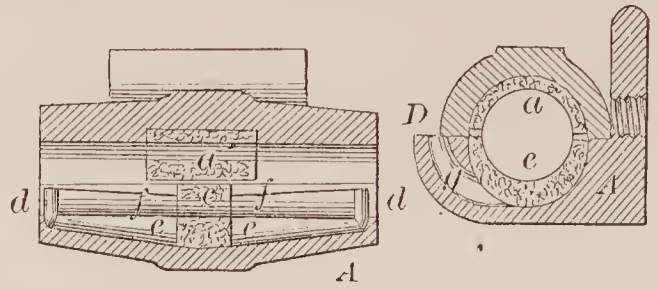
69822—E. F. Light—Journal Box.
