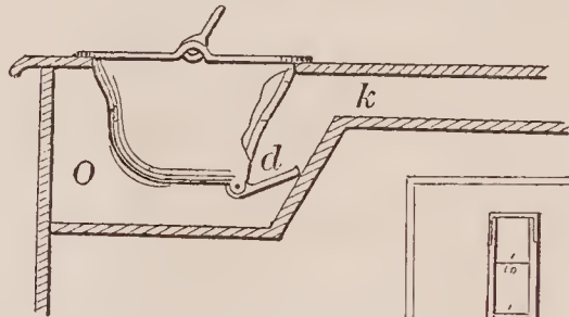
72207—Little & Bell—Summer Furnace.
