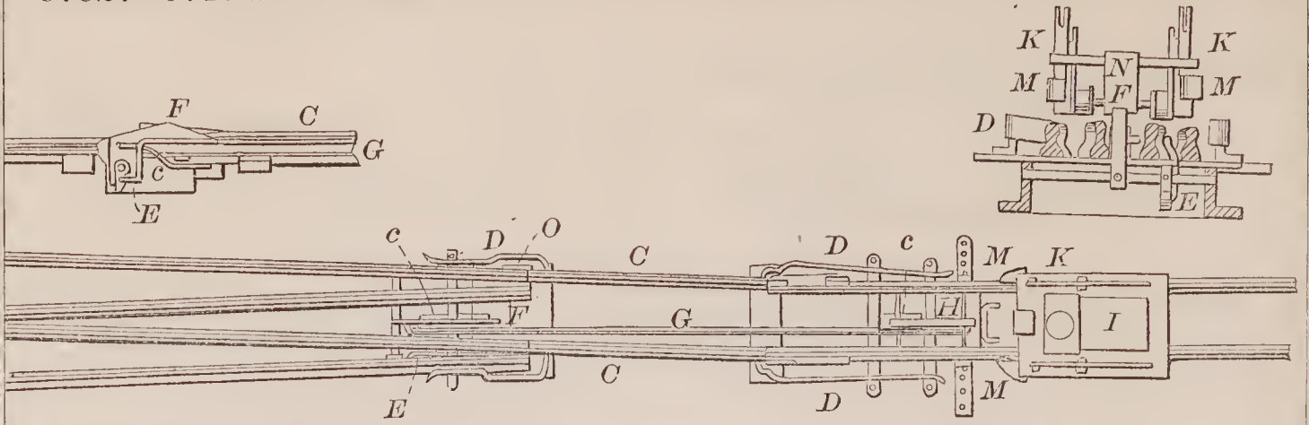
67828—W. N. Whitely—Harvester.
