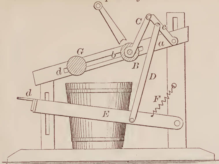
69696—Peters & Williams—Line Holder.
