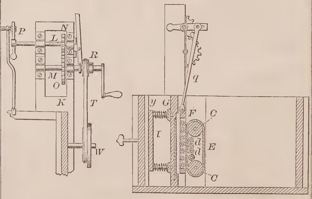
68286—C. M. Carleton—Washing Machine.
