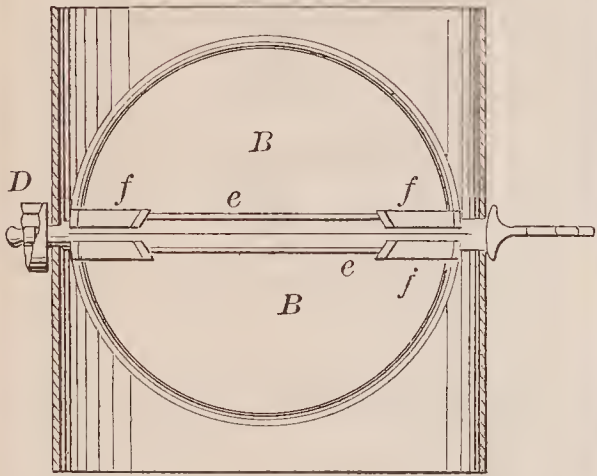
70835—T. J. Halligan—Treadle for Sewing Machines.
