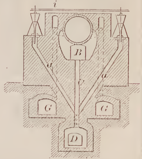
67492—J. Bühner—For the Combustion of Fuel.
