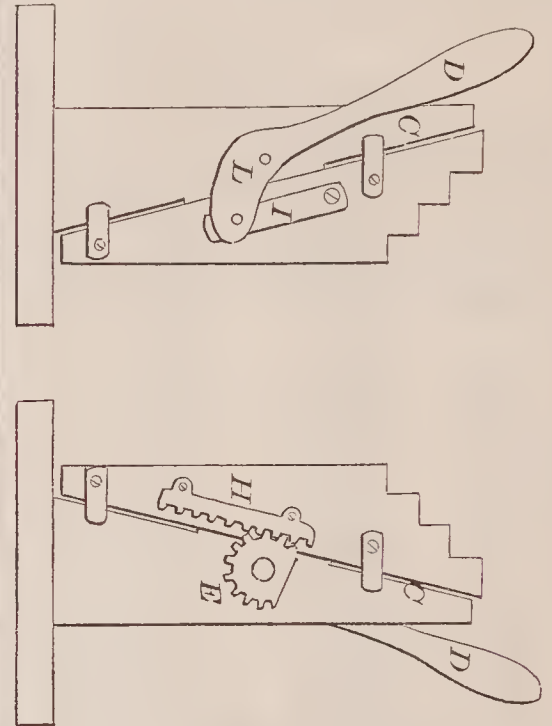
70115—O. L. Pinney—Lifting Jack.
