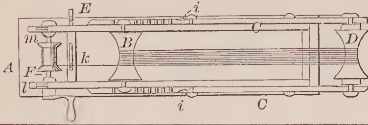
70114—Phillips, Southwick & Arnold—Starting and Stopping Cars.
