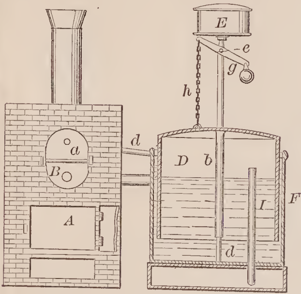
66952—McD. Darrow—For Heating Tires.
