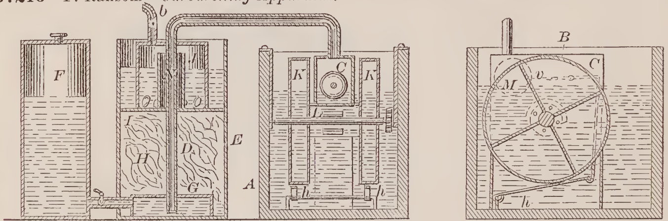
67218—Rosenberry & Worth— Sifter, Egg Beater and Spice Mixer.
