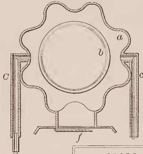
71465—J. B. Driscoll— Stove and Furnace.
