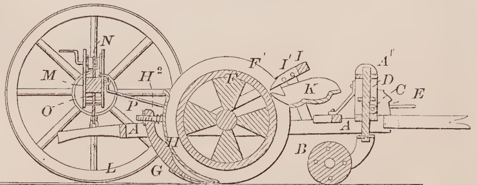
71275—Bymer & Imlay— Ditching Machine.
