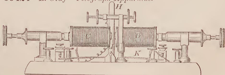
69424—E. Gray—Telegraph Apparatus.
