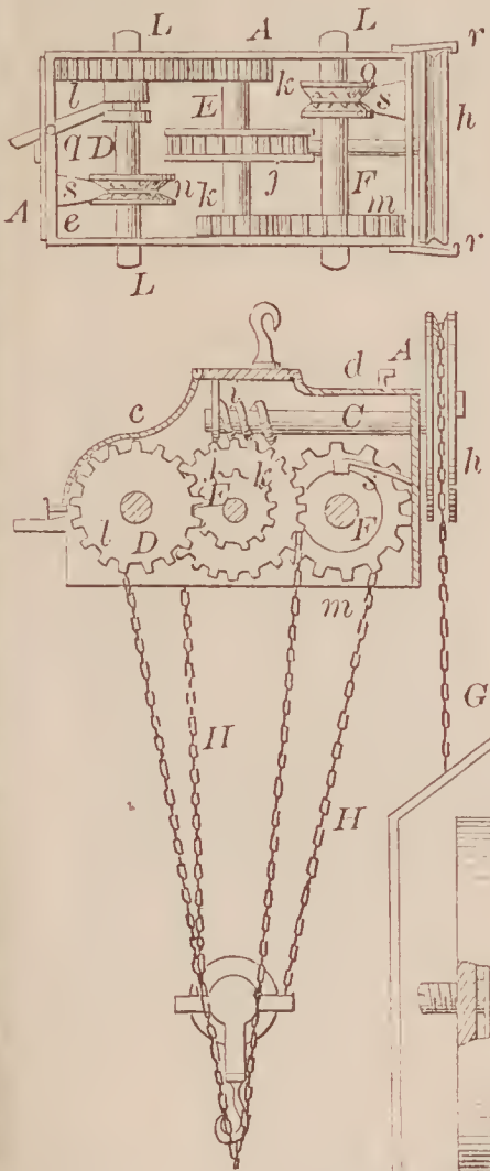
68794—W. Rung—Hoisting Apparatus.
