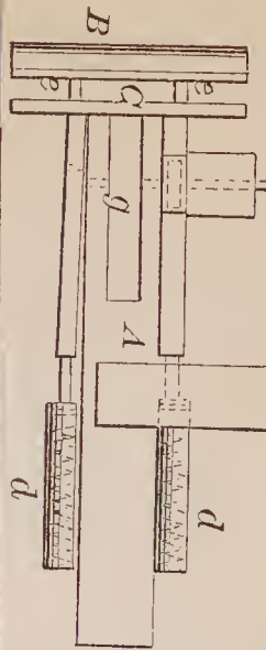
Boyd & Kriegbaum— Car Coupling.
