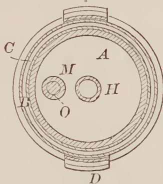
71863—J. M. Fairchild— Self-Adjusting Relay Magnet.
