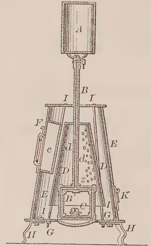
68318—J. D. Spang—Gas Heating Apparatus for Sad Irons.
