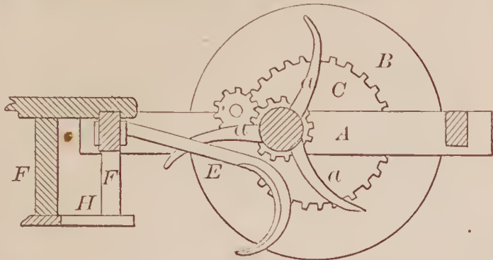
68749—A. Hunt— Cornstalk Cutter.
