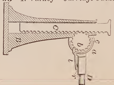
70763—I. Varney— Carriage Jack.
