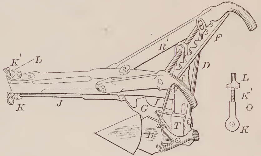
67890—W. E. Levoy—Plow.
