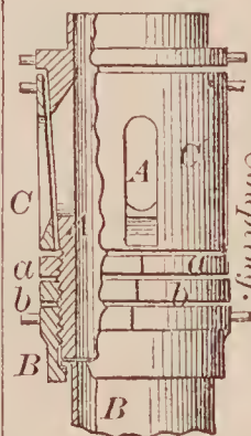
68478—A. F. Allen—Escape Valve Hose Coupling.
