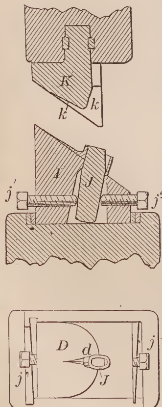
68414—Clement & Foster—For Manufacturing Hoes.
