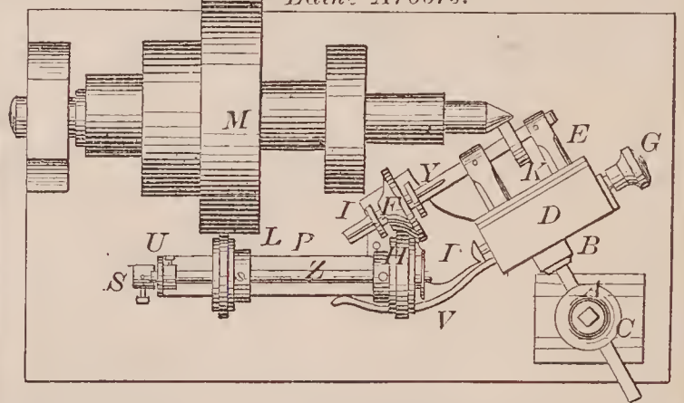
68698—Coester & Lawther—For Grinding Lathe Arbors.
