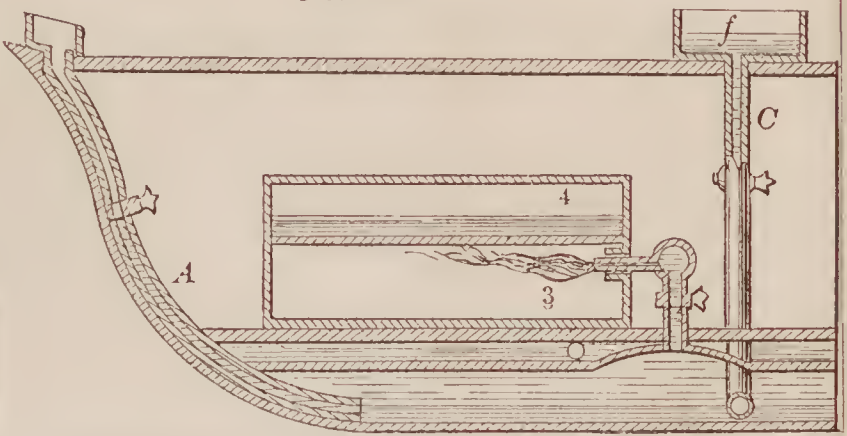
72101—J. II. Smith—Raising Oil by Pneumatic Pressure.
