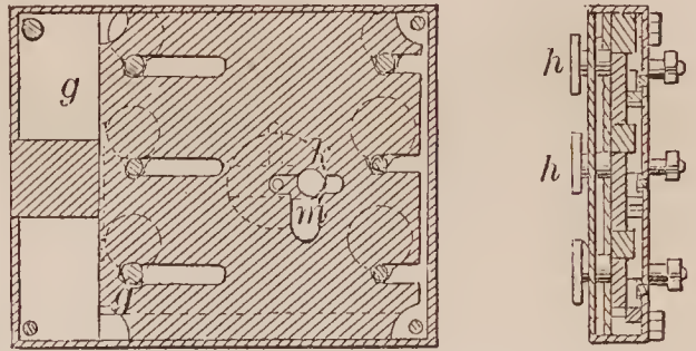
68219—C. L. Lucas—Permutation Lock.
