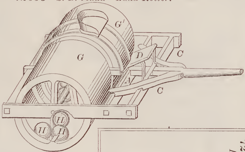
72653—S. B. Mann—Land Roller.
