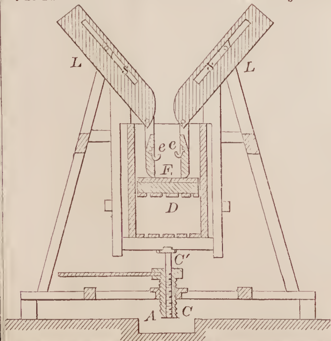
71113—B. B. Alfred—Cotton and Hay Press.
