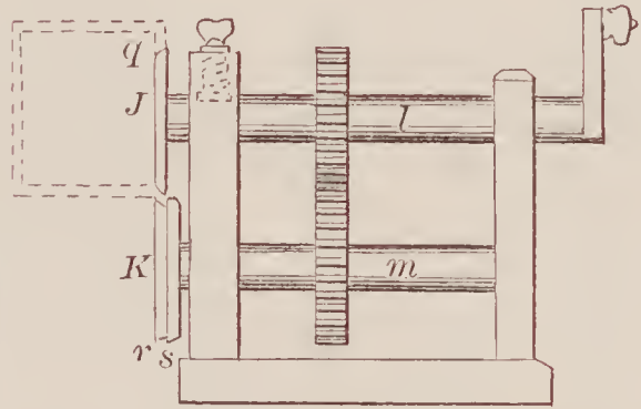
71683--P. D. Beach--For Boring Bobbins.
