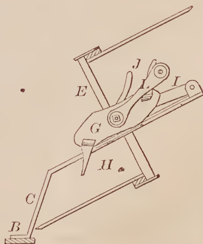
68461—E. P. Russell— Dumping Reel for Harvesters.
