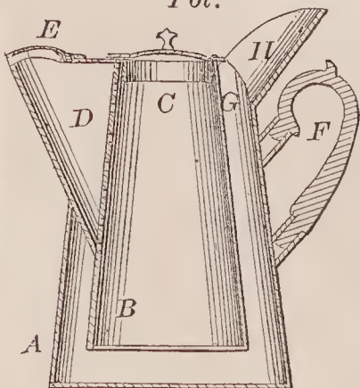
71237—J. B. Smith—Coffee Pot.
