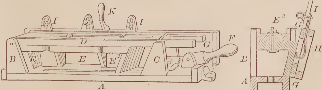
67097 —R. H. Birt— Tinners' Folding Machine.
