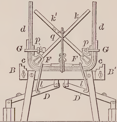
71890—E. J. Leyburn— Harvester Rake.
