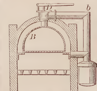
71355—C. Adams—Reducing Manganese Ores.
