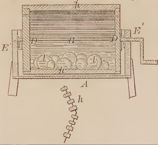
68851—A. Denison—Washing Machine.
