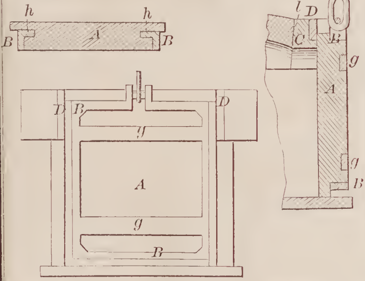
71433—J. Watson—Furnace Door.
