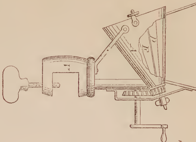
68877—T. G. Höfer— Vegetable Slicer and Grater.
