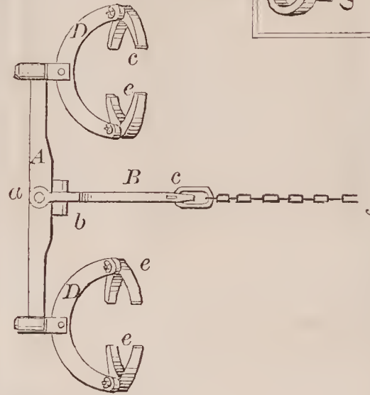
71415—E. Sanford— Drayght Attachment for Horses.
