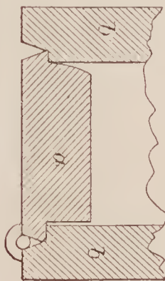
71110—L. Yale, Jr.—Burglar Proof Safe.
