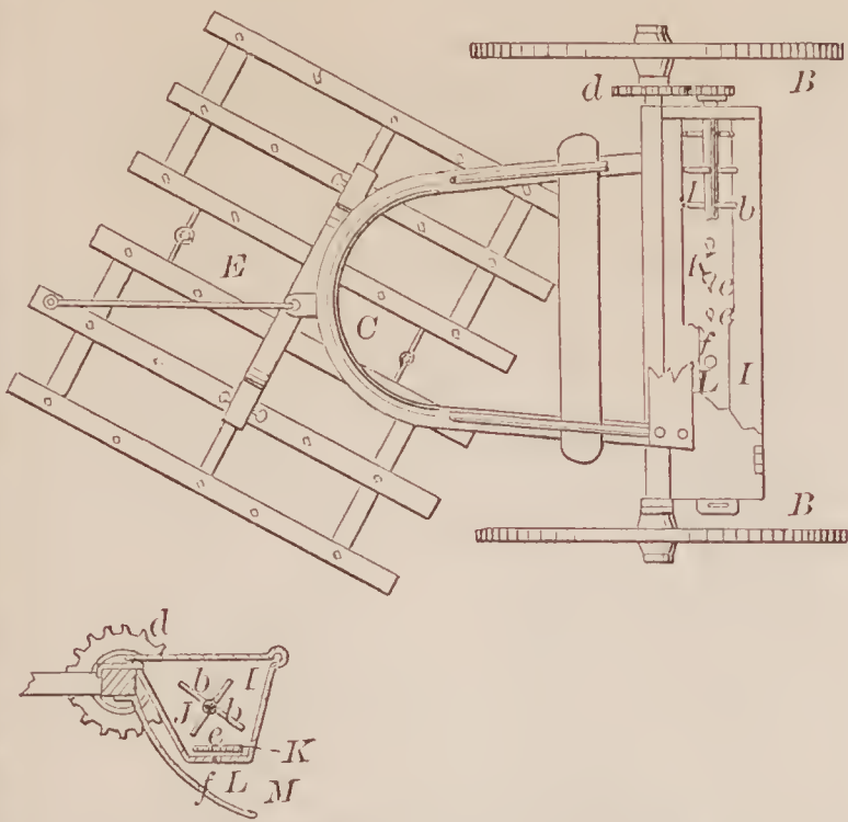
70898—B. Randall—Harrow and Seeder.
