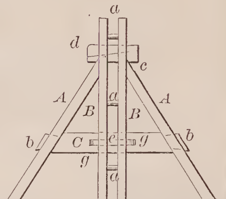
72096—J. W. Simpson— Window Sash Supporter.
