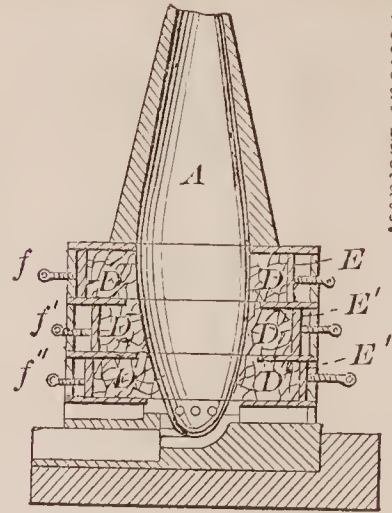
72201—H. G. Hubert—Furnace for Smelting Precious Metals.
