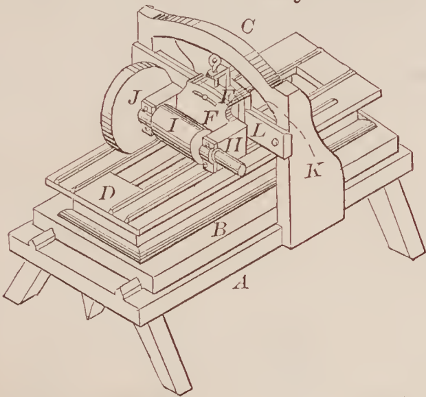
70483—A. Thomas—Lathe Way Smoother.
