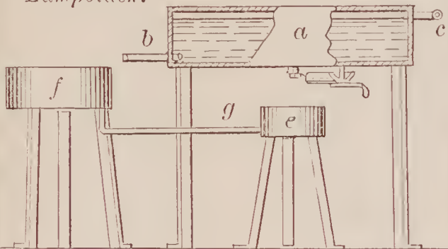
72068—A. Millochau—Manufacture of Lampblack.
