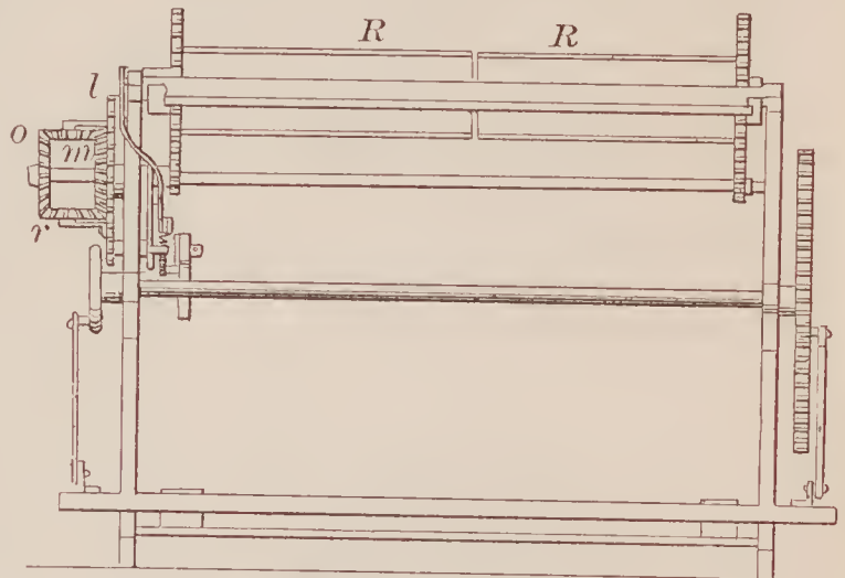
69320—Cottrell & Draper—Loom.
