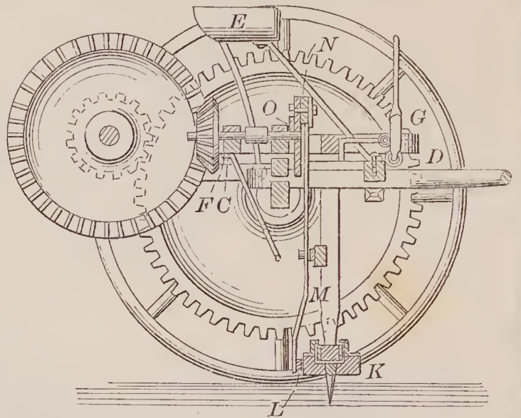
67943—S. Boone—Anchoring Stationary Machinery.
