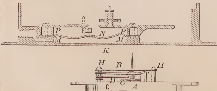
68849—G. M. Davis— Steam Gauge.
