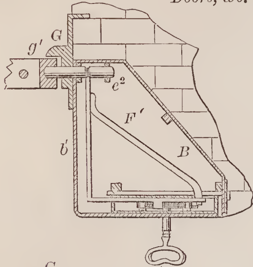
67641—C. E. Felton— Lock for Prison Doors, &c.
