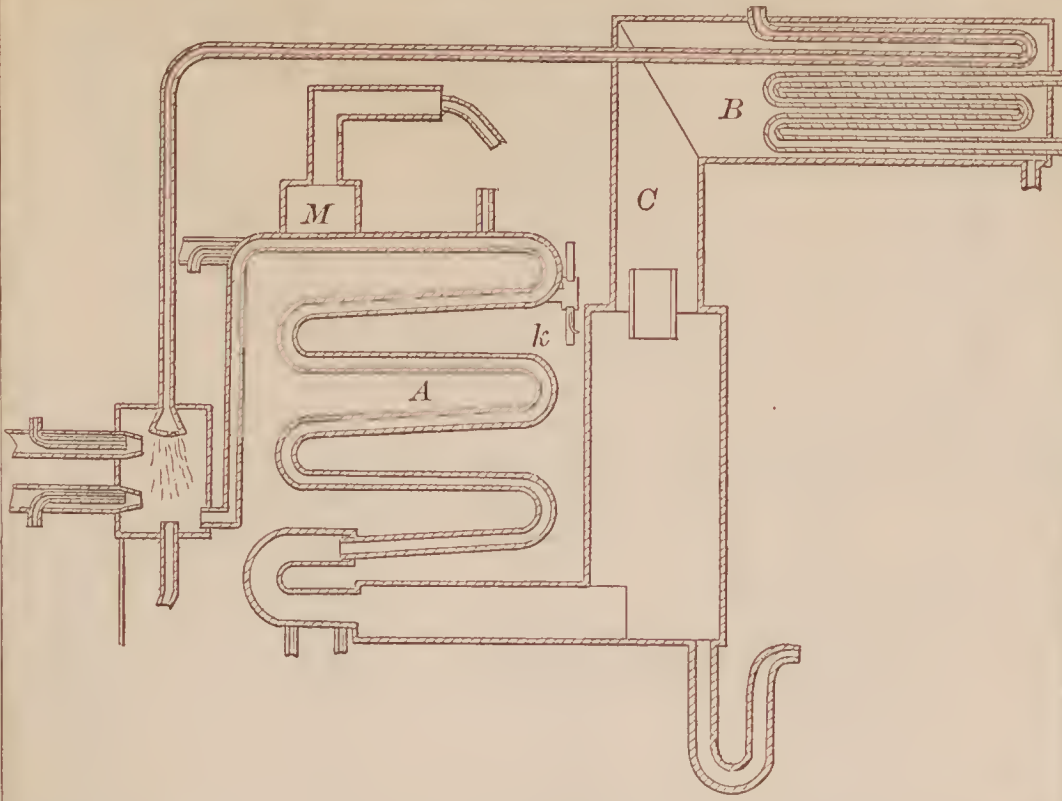
68860—Ellis & Kattell—For Distilling and Refining Oils, &c.
