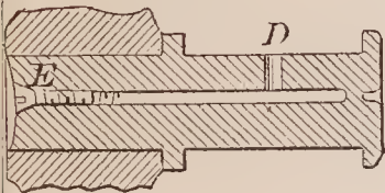
70659—E. Webster— Stove Pipe Drum.
