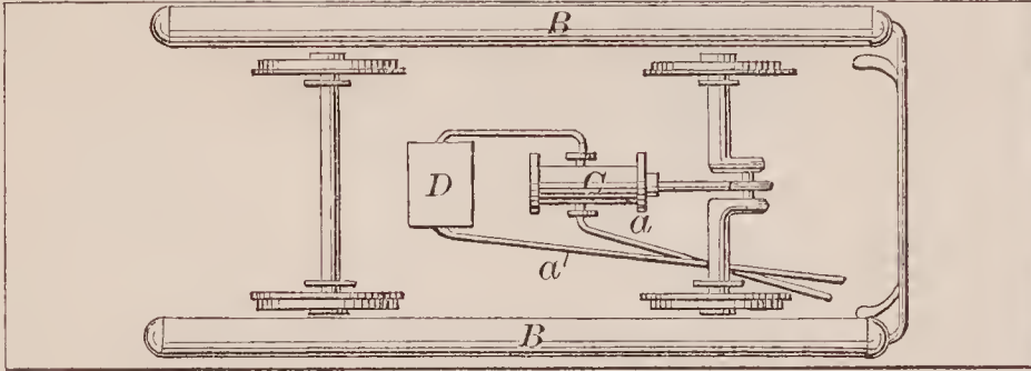
72082—L. Ransom—Pneumatic Car.
