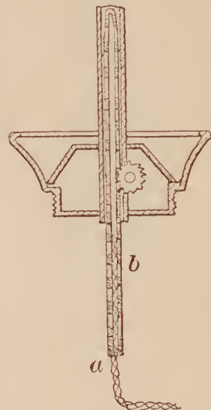
72788—C. D. Brainerd— Bag Holder.
