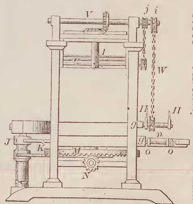
67548—W. H. Hovey—Brick Machine.
