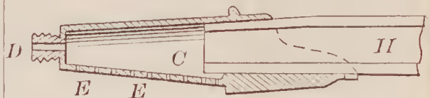
71264—W. D. Baughn—Thimble Skein for Axles.
