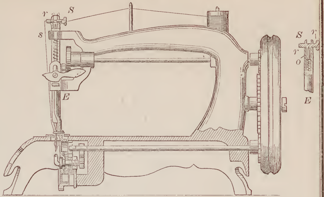
69666—C. Hodgkins—Sewing Machine.
