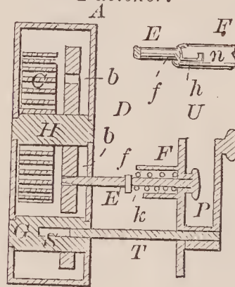
70714—E. Herbster—Sash Fastener.
