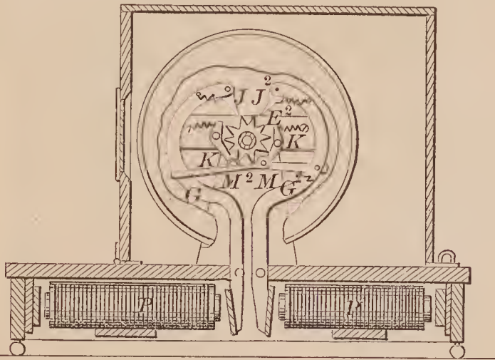
72742—S. S. Laws—Electrical Indicator.
