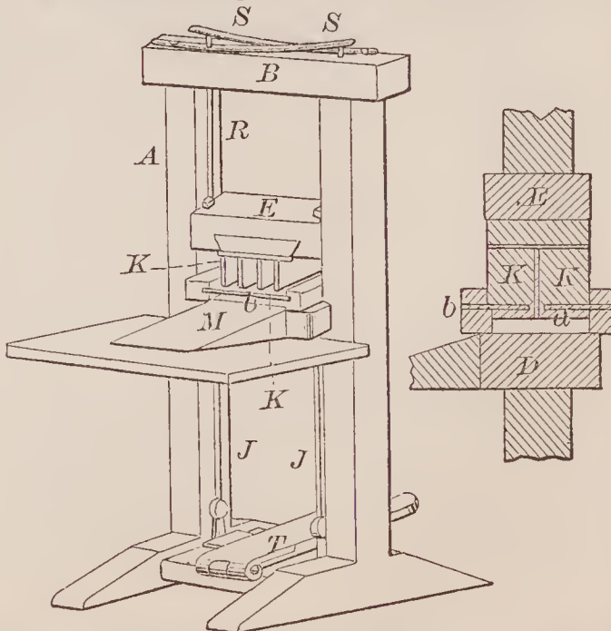
67848—D. Davenport—Corn Candy Cutter.
