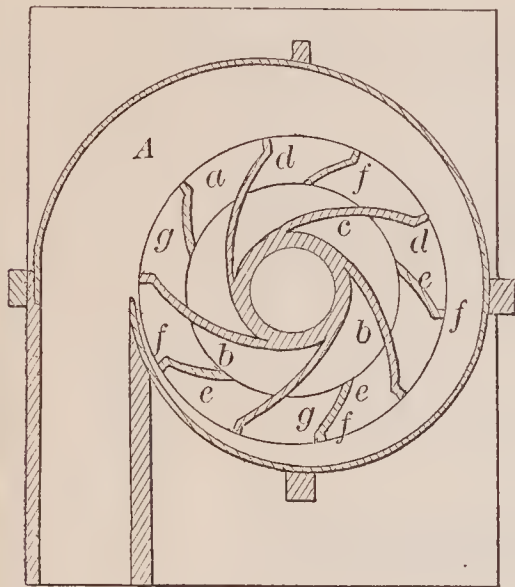
70211—G. W. Herring—Water Wheel.
