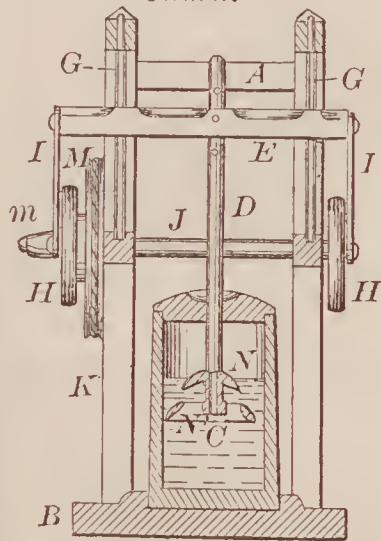
68273—S. C. Wilson—Churn.
