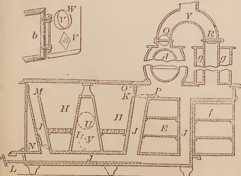
68898—G. Perkins—Cooking Stove.
