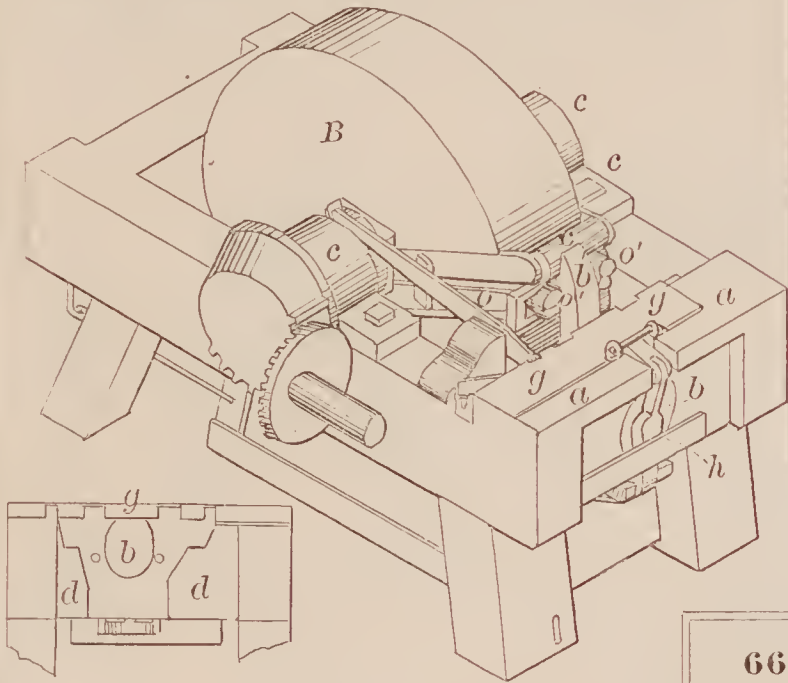
66991—A. Reese—Horse Shoe Machine.
