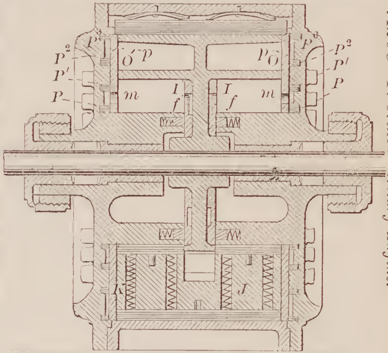
71208—F. Ortlieb— Rotary Engine.
