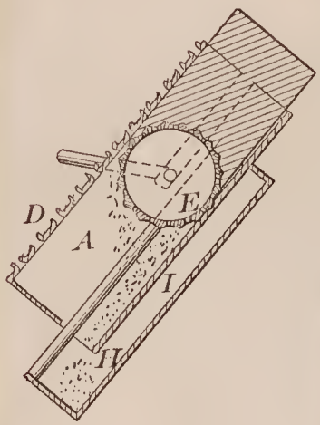
68256—H. Stone—Grater.
