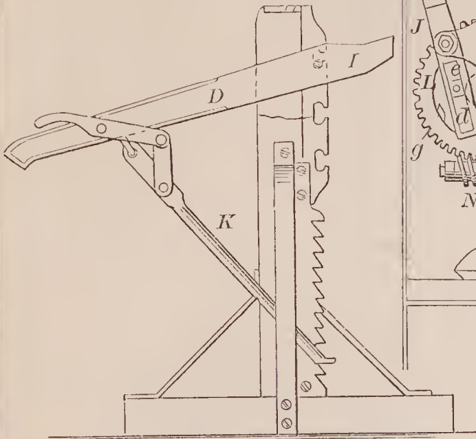
70291—W. H. Trusty— Wagon Jack.
