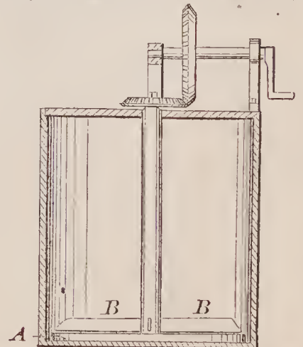
67205—F. McFarnahan—Churn Dasher.
