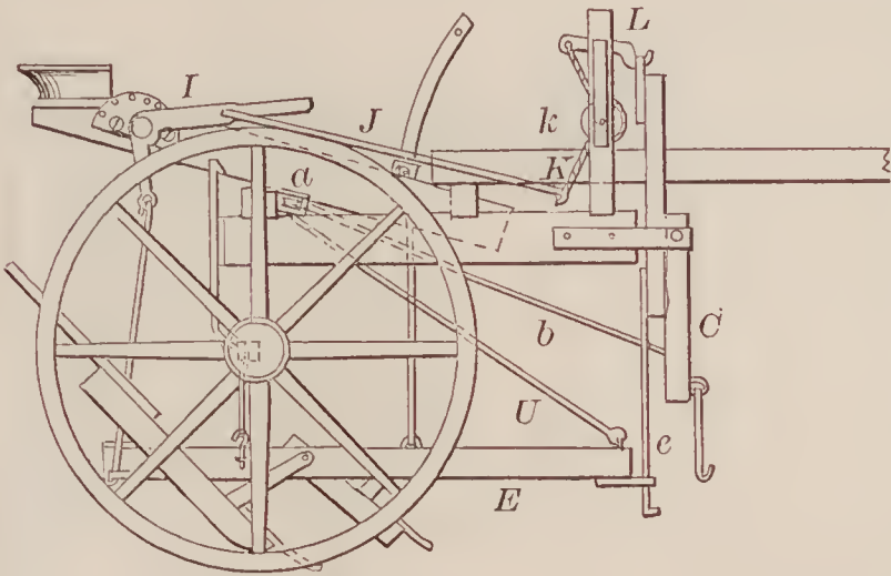
72598—J. E. Brooks—Cultivator.
