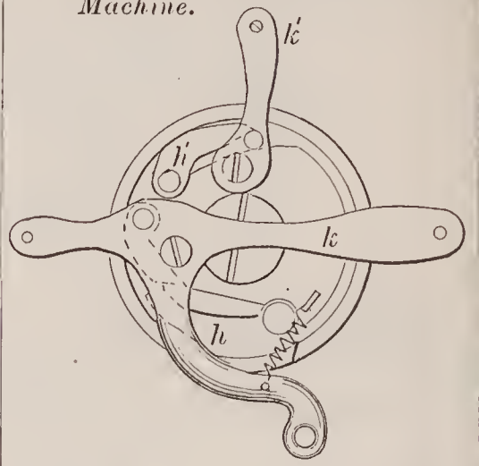
72676—G. W. Powers— Sewing Machine.
