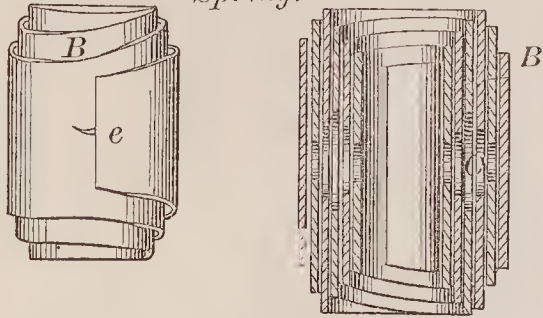
67972—Freeland & Ward—Volute Spring.
