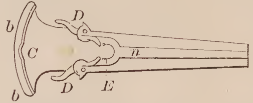
67064—J. P. Morris— Car Coupling.
