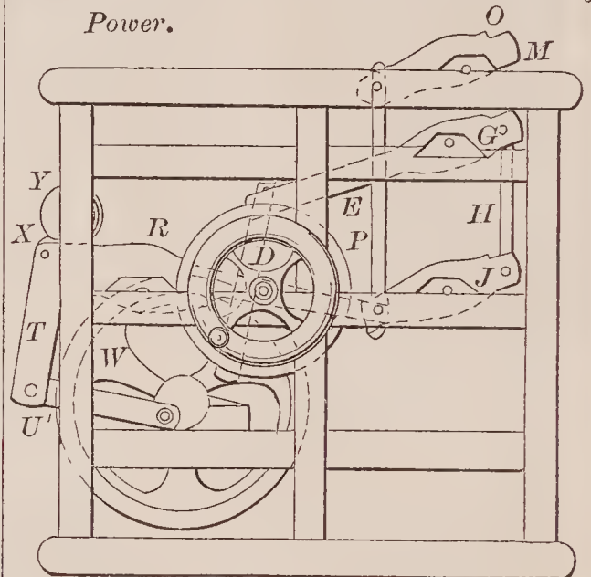
72155—A. P. Barlow—Saw Mill.
