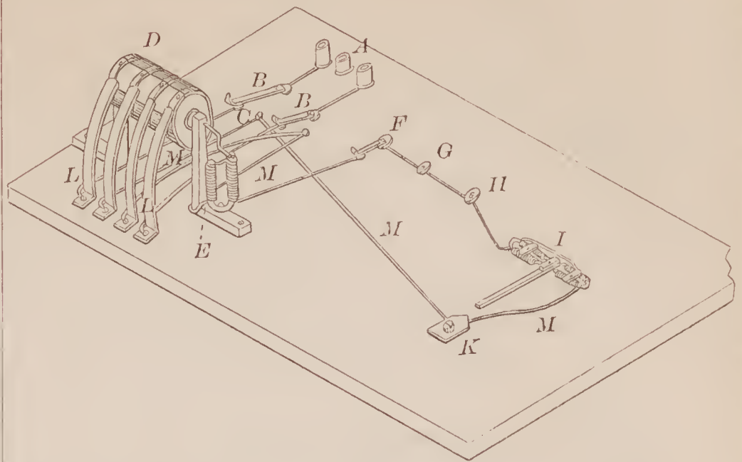
69504—Stevens & Drake—Odometer.
