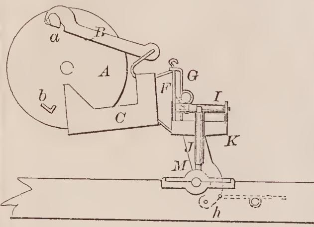
71099—E. W. Weston—Revolving Coal Screen.
