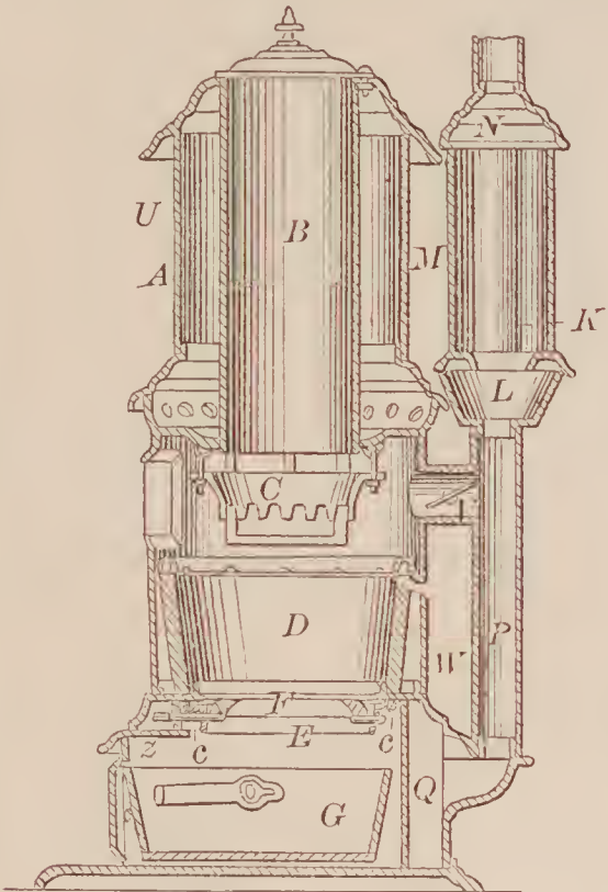
66957—W. C. Durant—Coal Stove.
