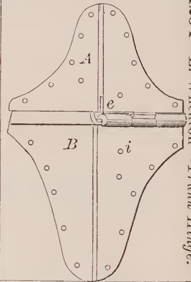
71254—L. Wheaton—Trunk Hinge.
