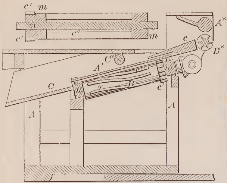
71539—J. Russell—Husking Machine.
