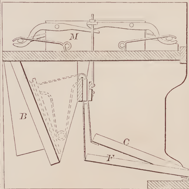
71947—C. E. Bacon—Operating Swell in Melodeons.
