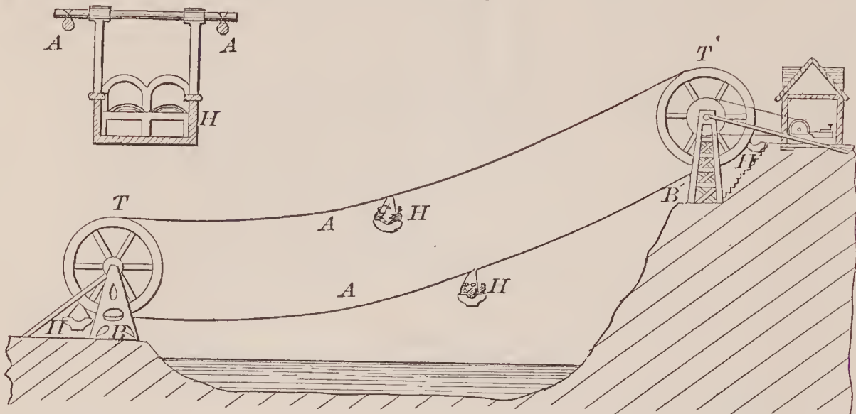
71921—D. Towse—Aerial Carriage and Way.
