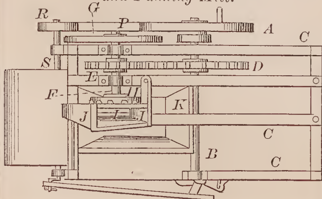
68744—Hoagland & Moser— Corn Sheller and Fanning Mill.
