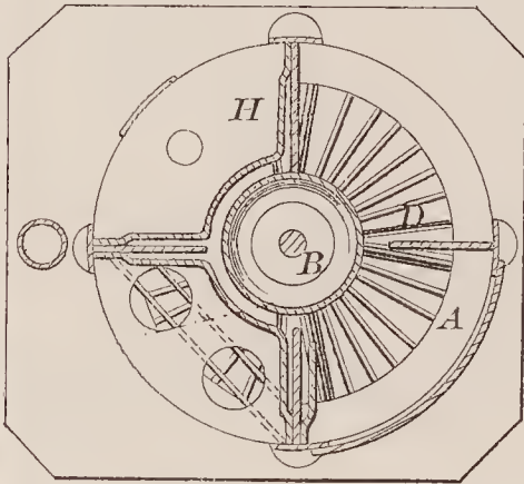
71659—S. B. Stewart—Stove Grate.
