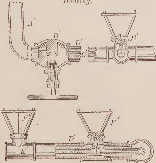
68045—Childs & Copeland—Vapor Burner for Heating.
