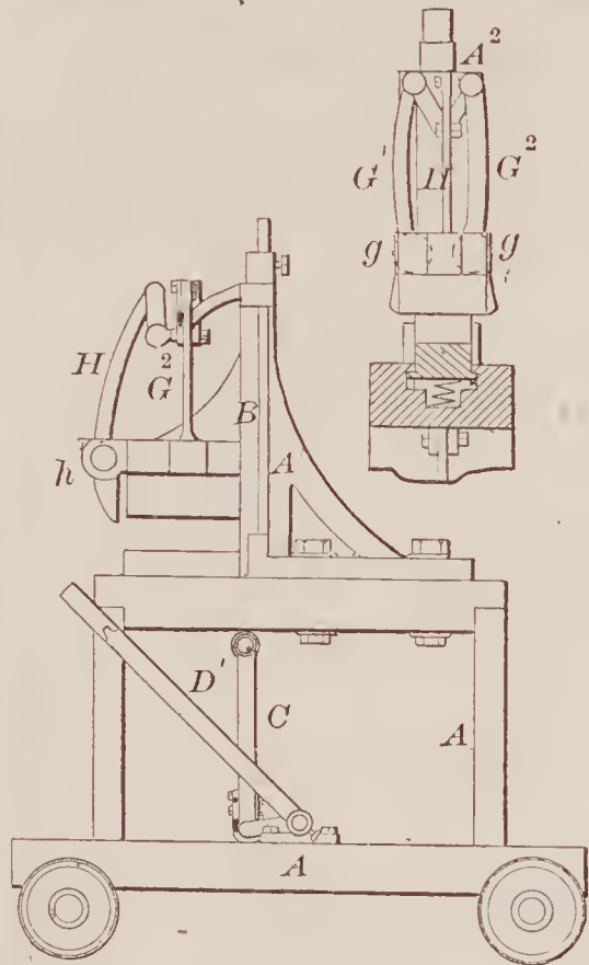
67561—J. McDonald—Brick Machine.
