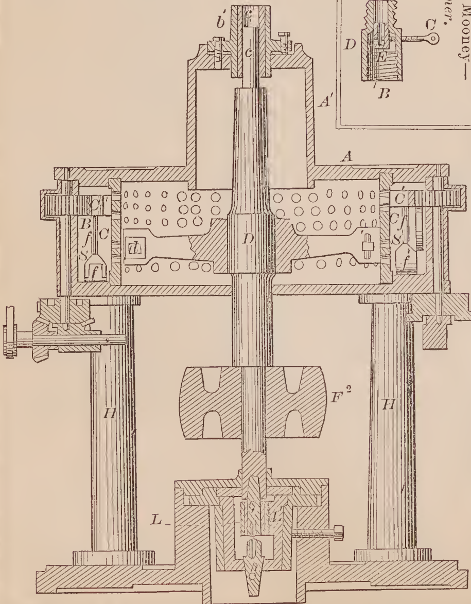
72418—S. W. Powell—Bone and Plaster Mill.
