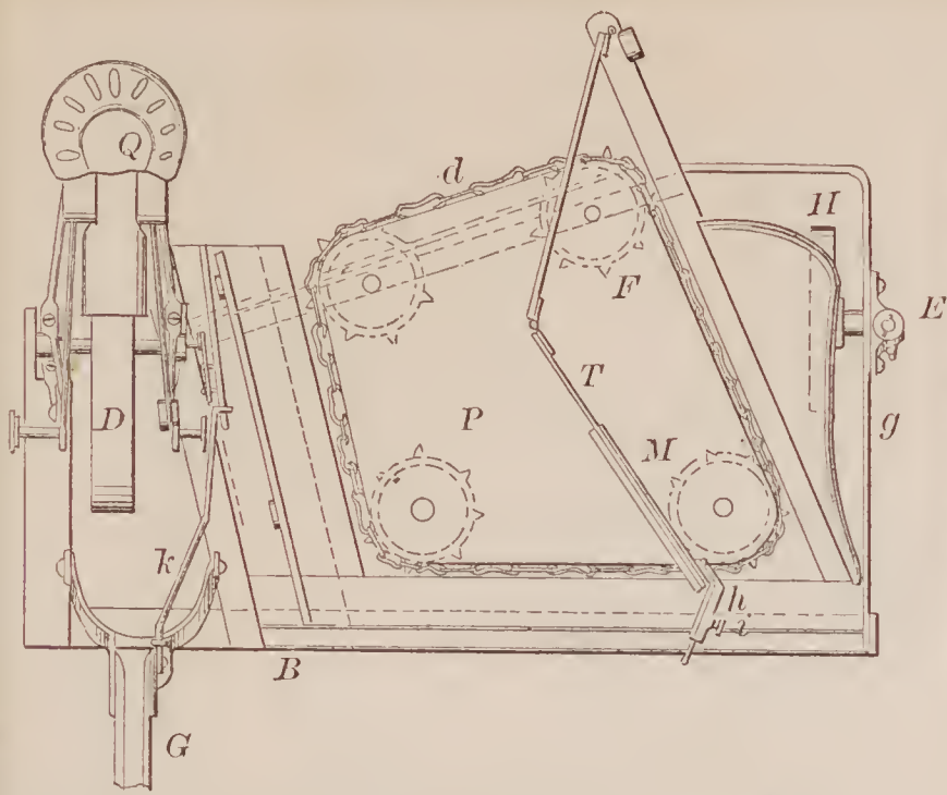
68617—P. J. Flanedy—Ironing Machine.
