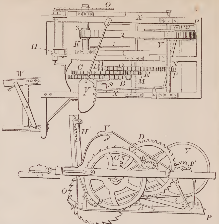
70994—W. F. Gordon— Ice Cutting Machine.
