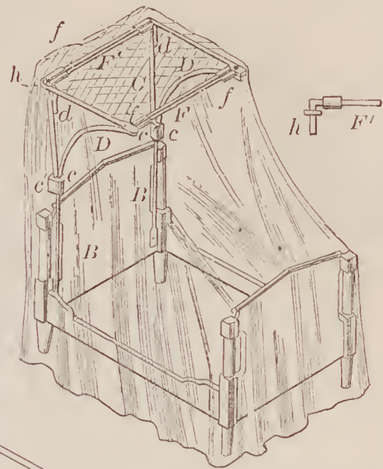
67612—M. L. Treadwell—Mosquito Net.
