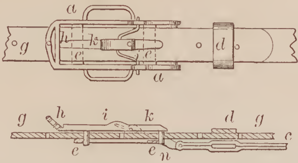
68147—R. J. Baker—Trace Buckle.
