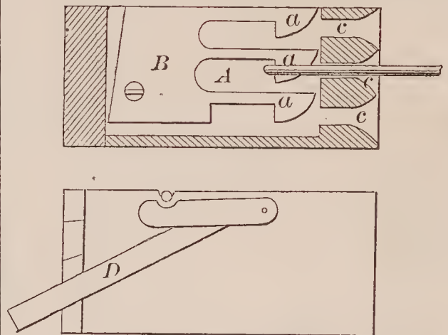
69123—H. C. Payson—Car Coupling.
