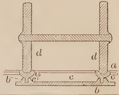
68424—E. R. Ensign—For Marking Holes for Planting.
