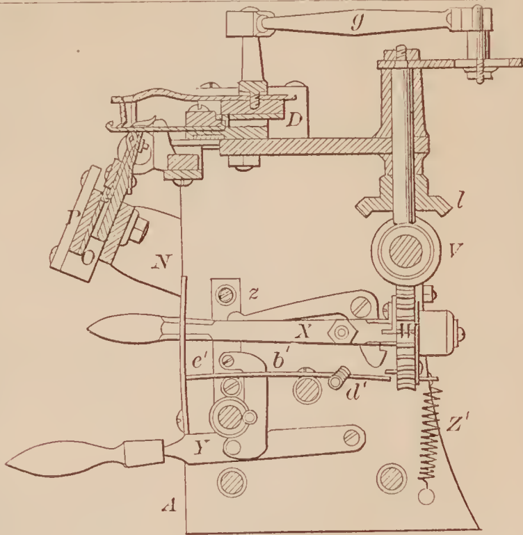
72765—F. N. Violet— Window Sash Supporter.
