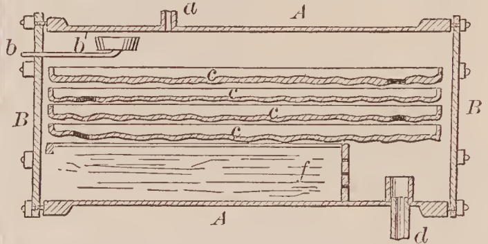
66997—T. B. Smith—For Cutting Veneers.
