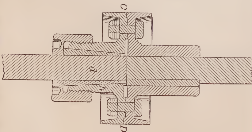
70869—W. E. London—Shaft Coupling.
