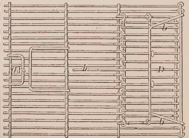
69089—J. Haddleton—Animal Trap.
