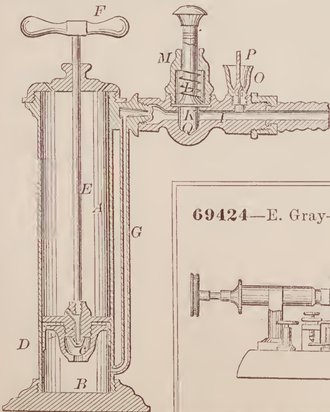
69423—H. Getty—Air Pump.
