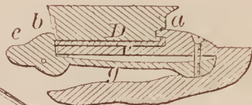
67110—G. Gunderson— Skate Fastening.
