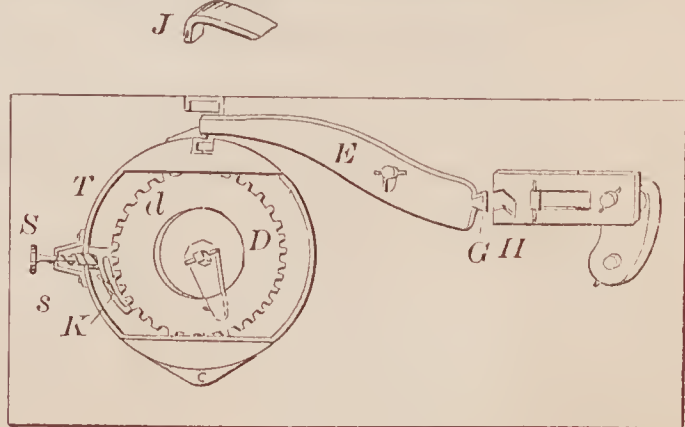
70599—J. H. Morse— Permutation Lock.
