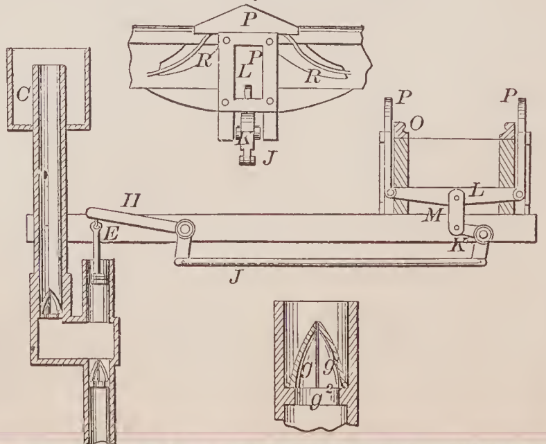
69631—M. S. Collar—Railway Water Elevator.
