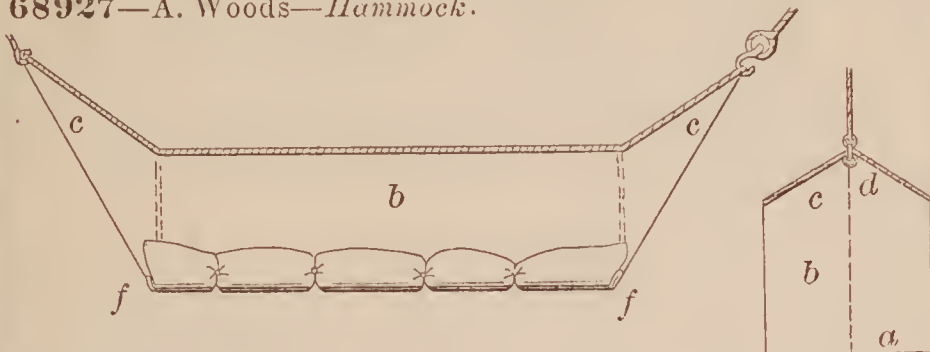
68927—A. Woods—Hammock.
