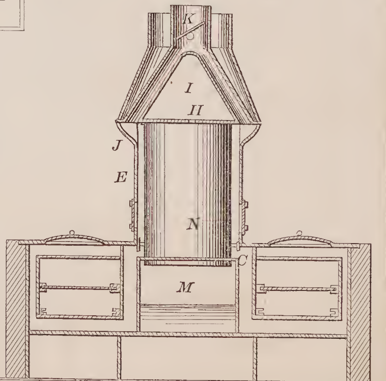
71446—N. A. Boynton—Range and Heater.
