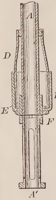
67749—A. D. Griffin— Packing for Deep Wells.
