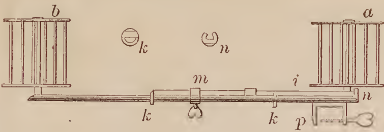
68439—G. H. Henfield—Car Coupling.
