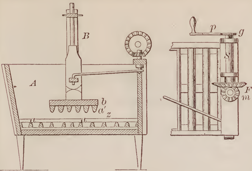
67575—N. Palmiter—Washing Machine.
