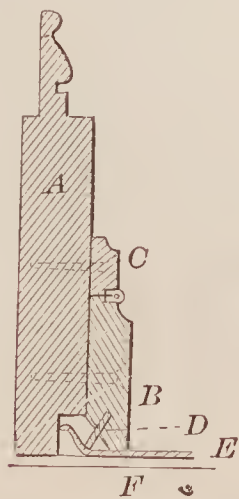
70055—West & Cunningham— Carpet Fastener.
