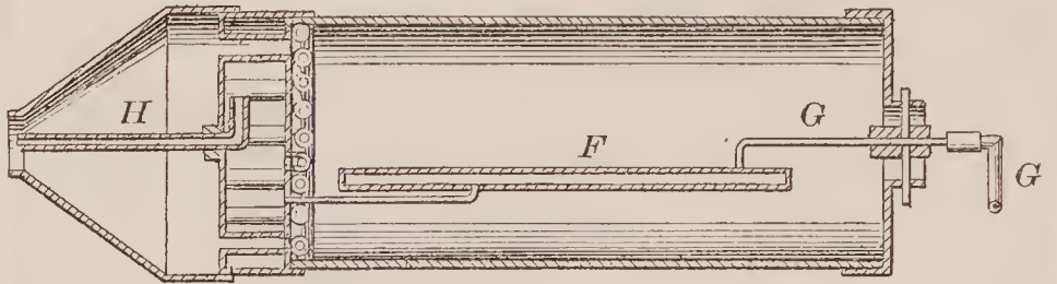
67862—G. B. Field— Ore Roasting Furnace.
