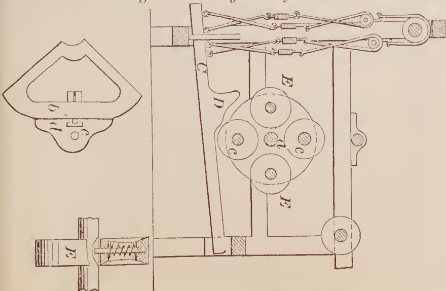
70623—R. Sargent—Rotary Cam for Looms.
