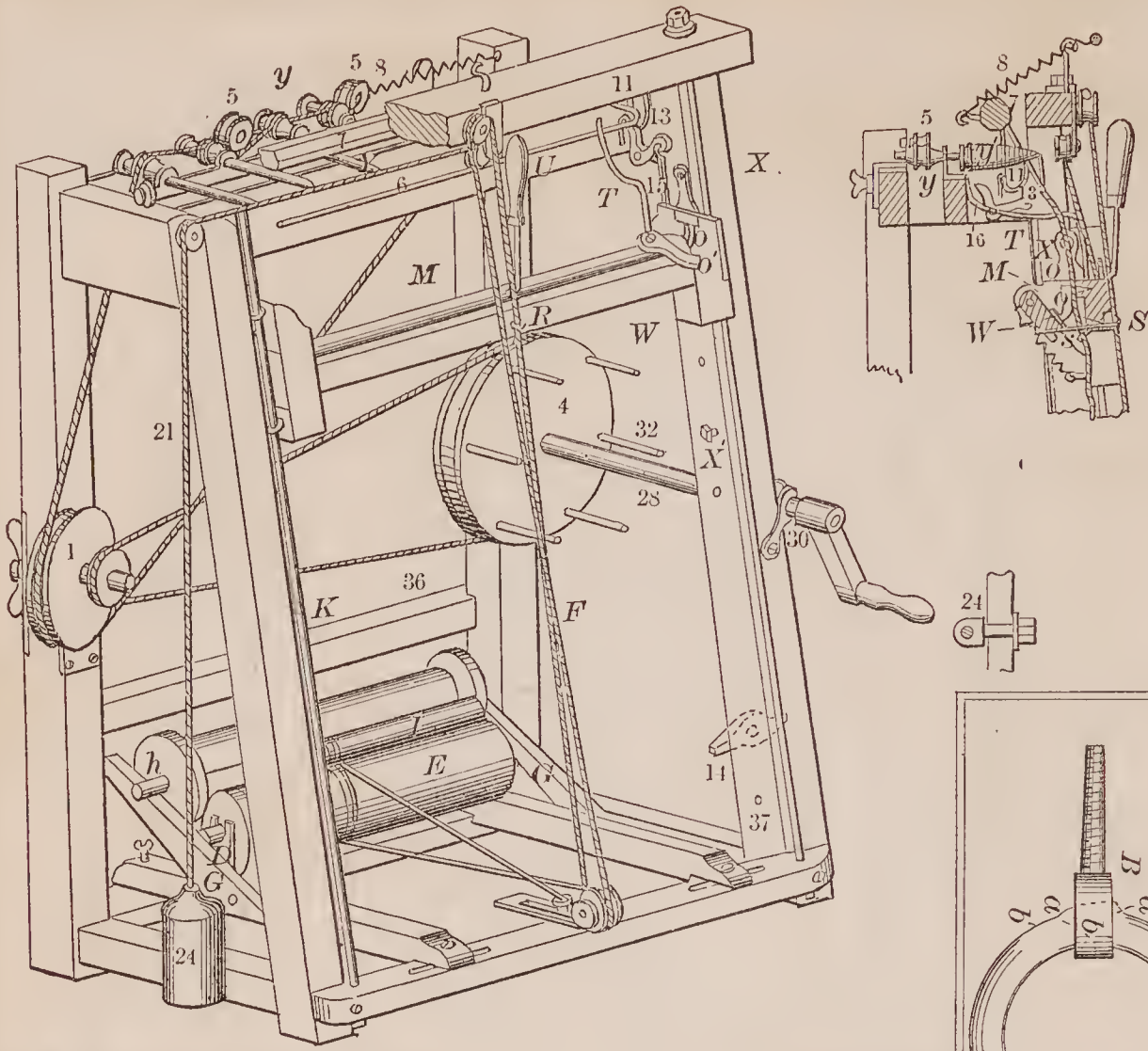
69211—Hoover & Hadley—Spinning Machine.
