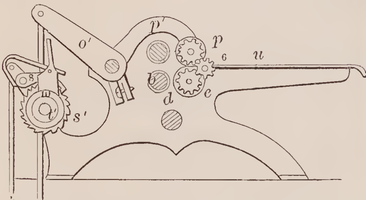
71532—Prentice & Wuterich—Cigar Machine.
