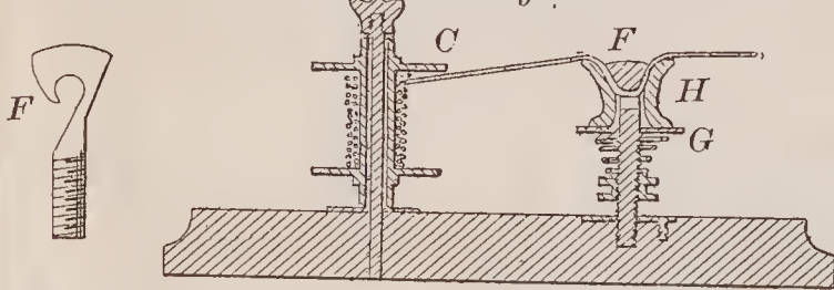
67519—J. Fewkes— Braiding Machine.
