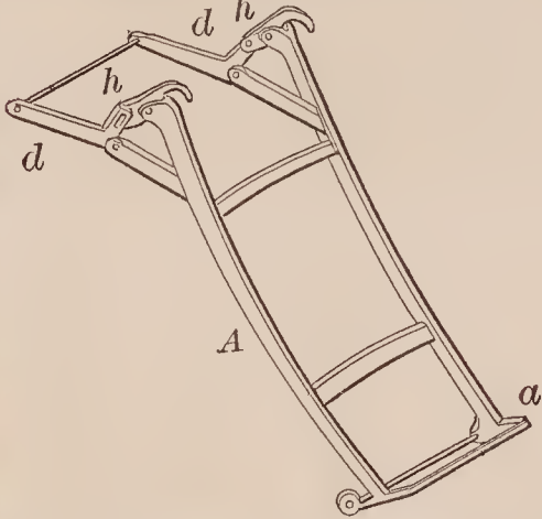
72503—T. W. Kennedy— Hand Truck.
