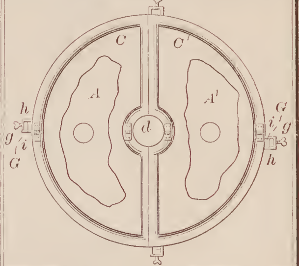
66806—S. Custer— Magnetizing Compass Needle.
