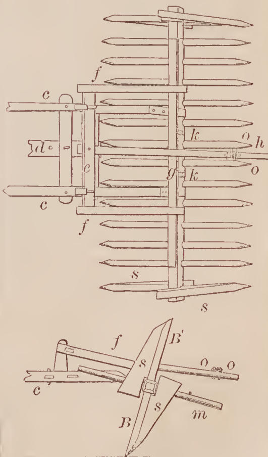
68693—I. W. Boatman—Horse Rake.
