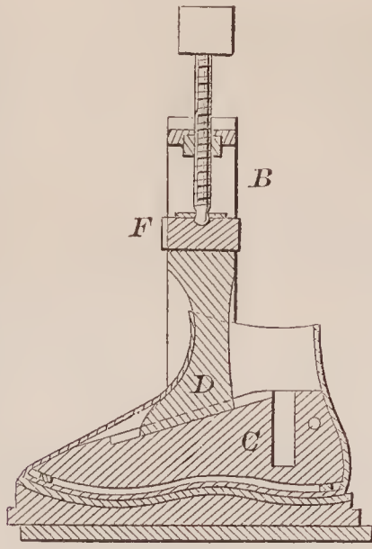
71497—W. H. N. Kimball—For Rounding up Soles
