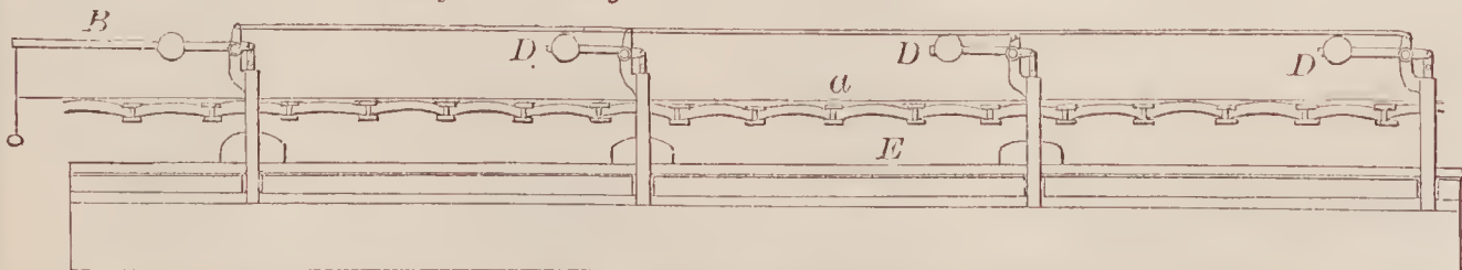
71571—D. Bievez—Oven for Cooling Glass.
