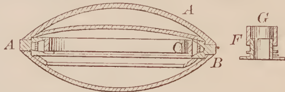
68814—N. B. Wallace—Watch.
