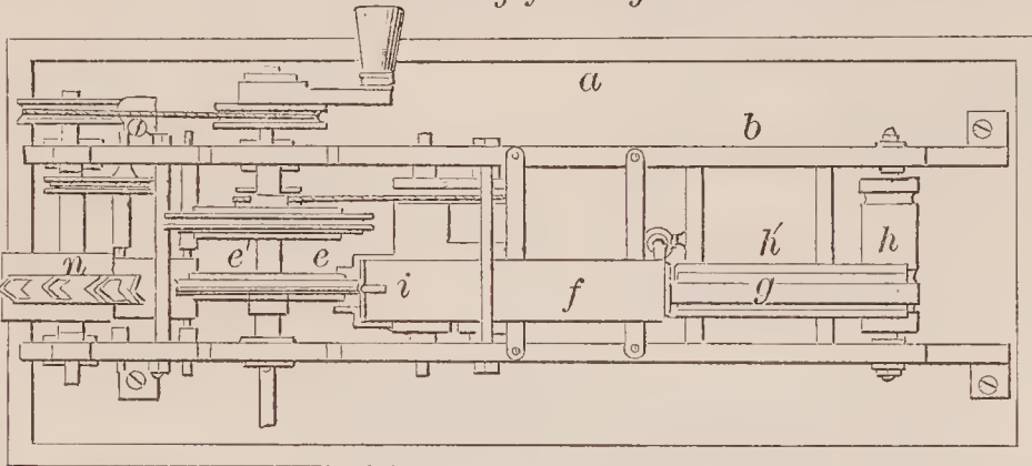
66845—W. W. Huse—For Compressing and Cutting the Filling for Cigars.
