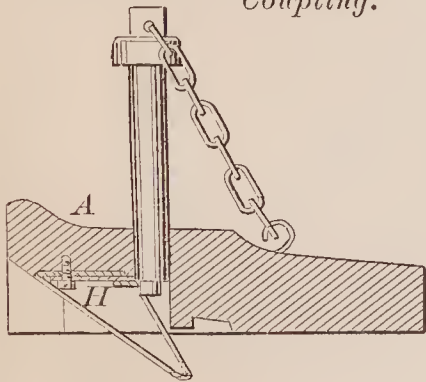
70729—S. I. Loomis— Car Coupling.
