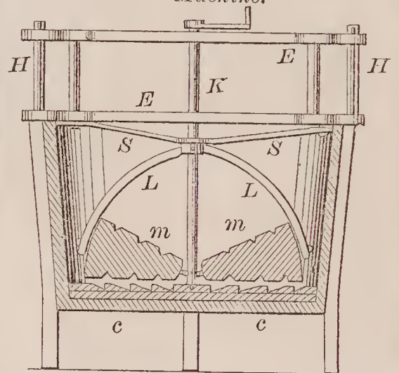
71090—H. Warner—Washing Machine.
