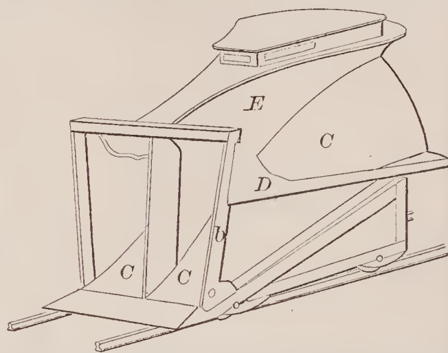
71607—S. G. Hadley— Railroad Snow Plow.
