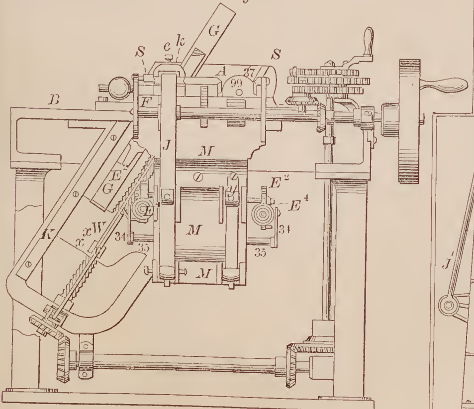
68815—S. Walton—For Cutting Files.
