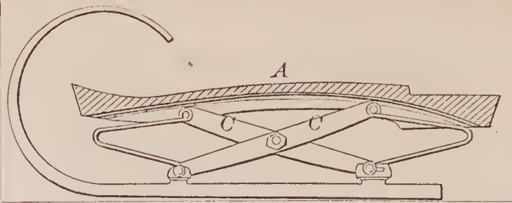
70906—G. W. Shearer—Skate.
