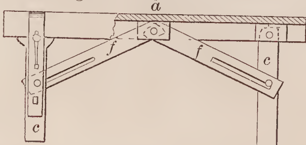
71126—J. Bragdon—Carpenters' Work Bench.
