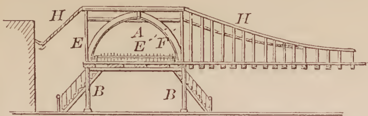
70666—W. H. Williams—Elevated Railroad.
