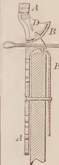
69474—B. D. Pease— Rein Holder.
