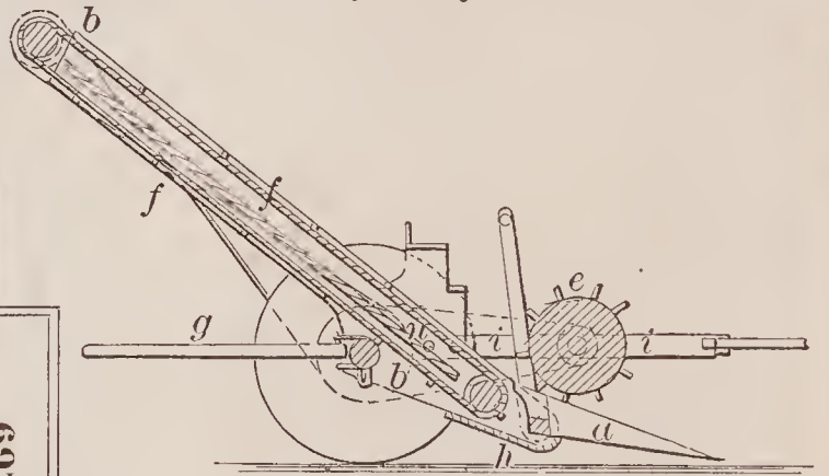
69794—A. Godfrey—Hay Raker and Loader.
