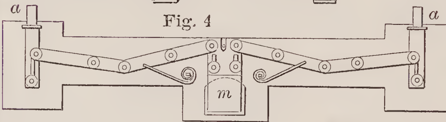
72649—Love & Ball—For Channeling Rock.
