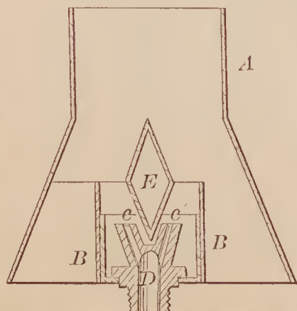
72426—L. F. Smith— Steam Blower.
