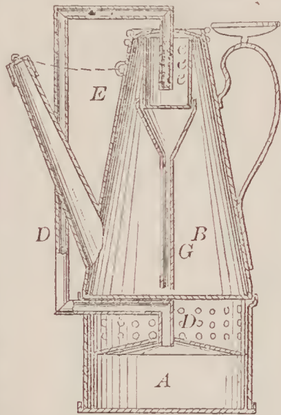
67935—C. O. Winegar—Steam Generator.
