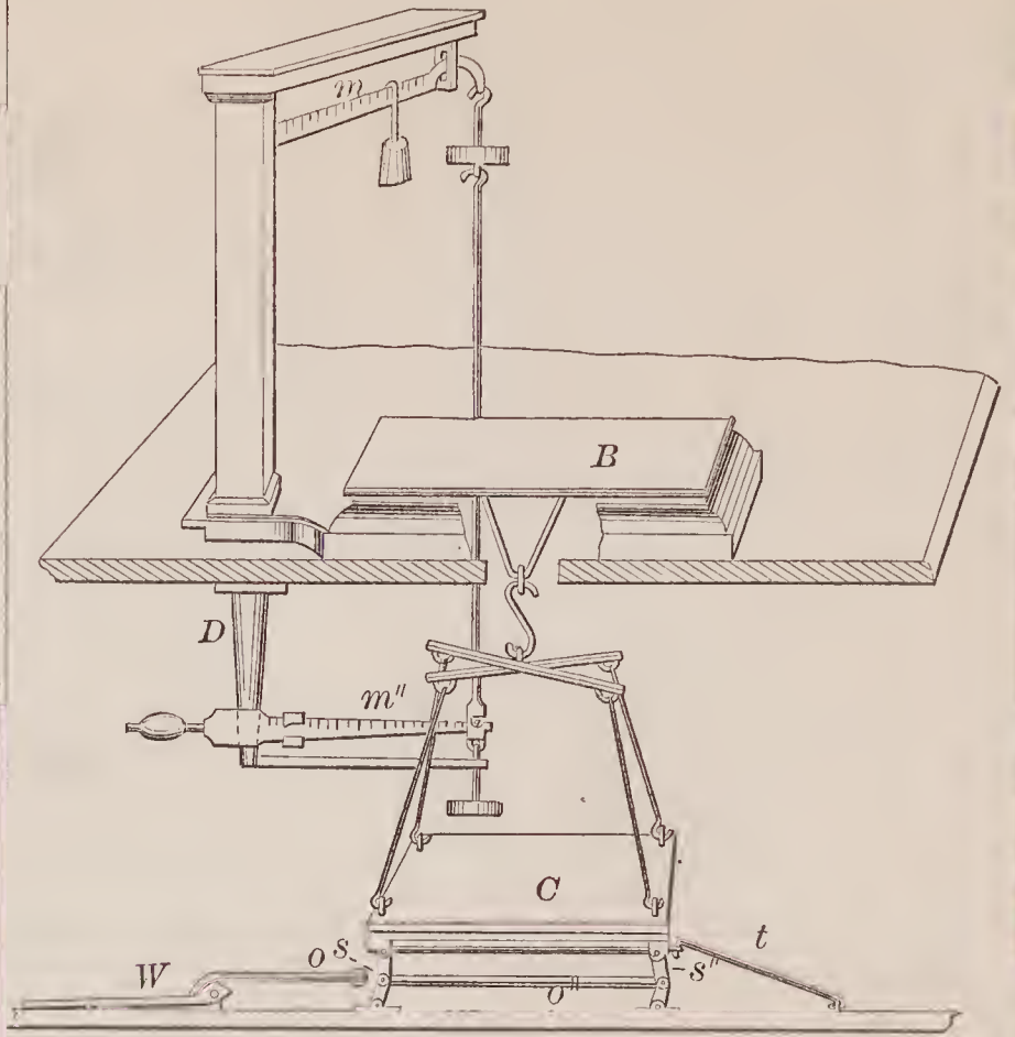
69933—Pope & Whipple—Weighing Scale.
