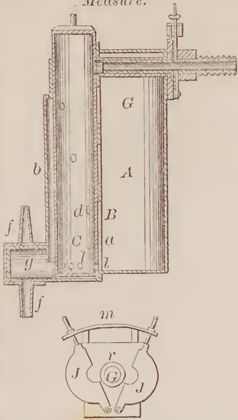
67948—P. Brinkerhoff— Liquid Measure.
