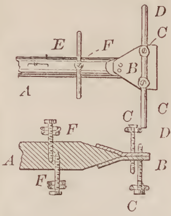
67185—C. Forbes— Coffee Generator.
