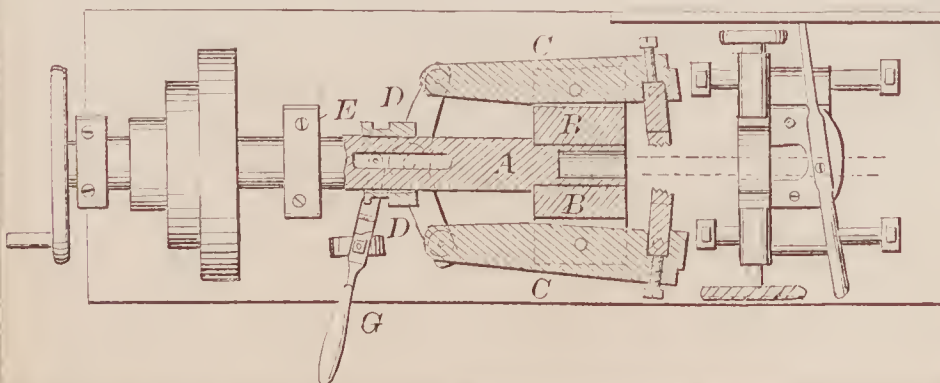
71512—E. M. Mayo— For Tapping Bolts.
