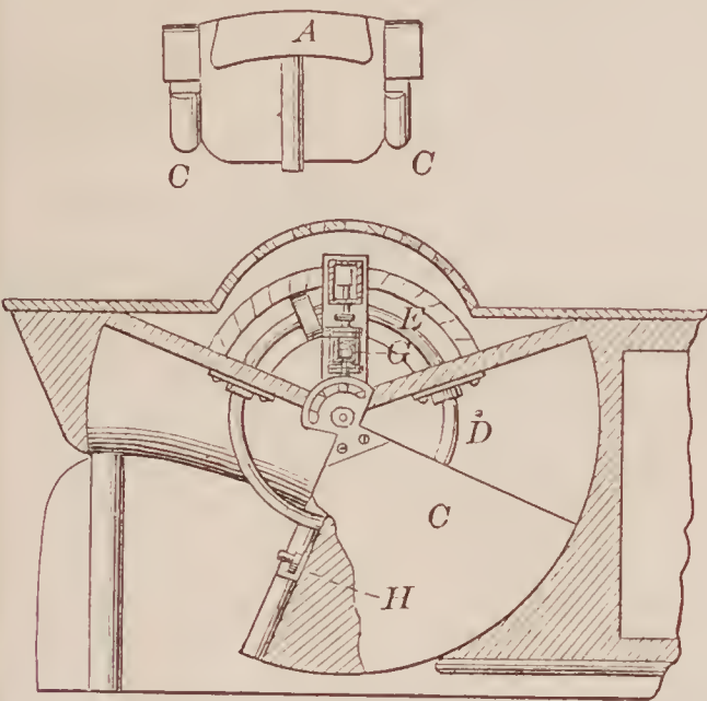
70463—W. R. Pape—Breech-Loading Fire Arm.
