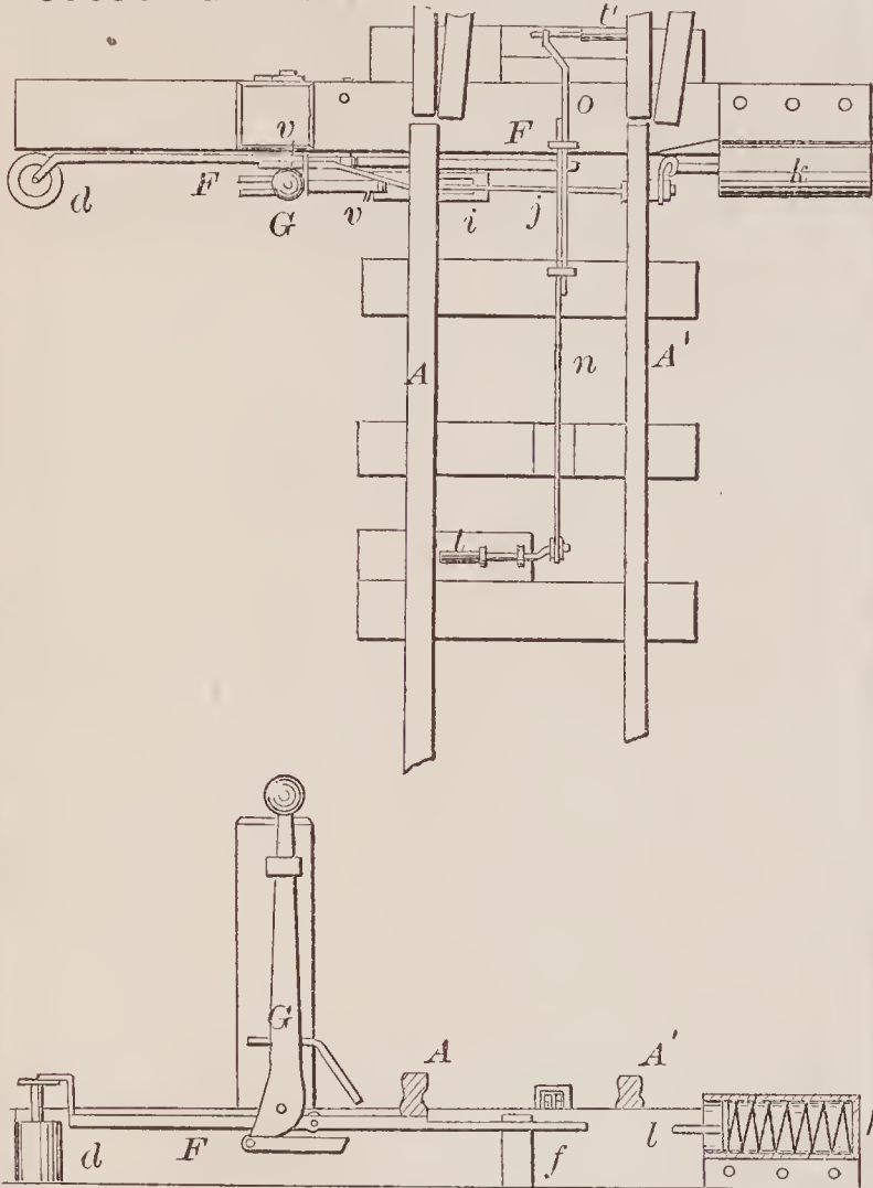
69856—G. W. Starr— Railroad Switch.
