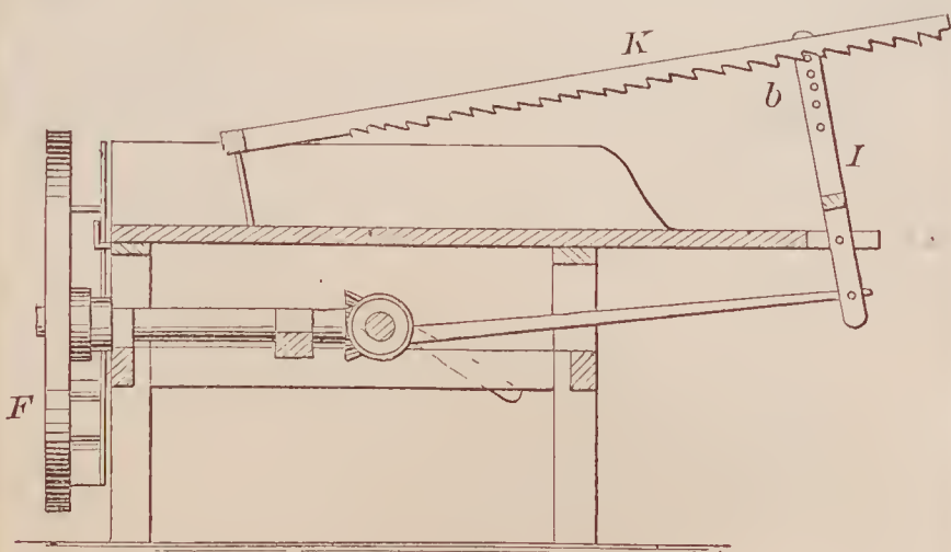
70891—H. Parks— Straw Cutter.
