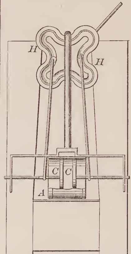
69758—G. Bruce—Pump.
