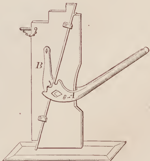
69805—T. Heaton—Carriage Tongue Holder.
