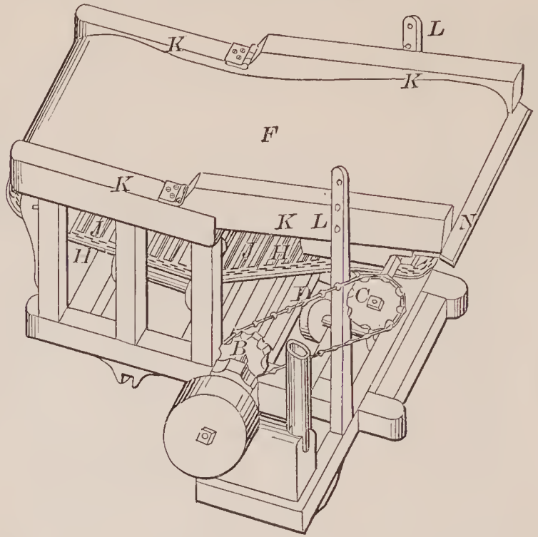
71854—E. Comeaux—For Making Levees.
