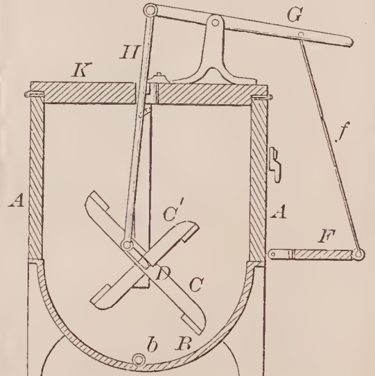
68523—D. C. McNeil—Churn.
