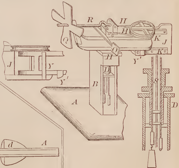
68674—L. H. Wheeler—Wind Wheel.
