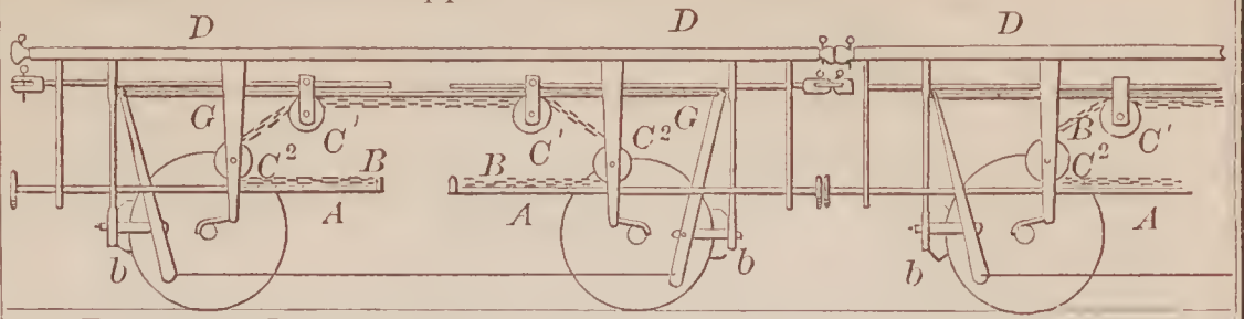
69437—T. & H. Hopper— Steam Car Brake.
