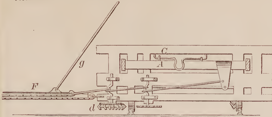
72268—A. F. Crosman— Boat Lowering Apparatus.
