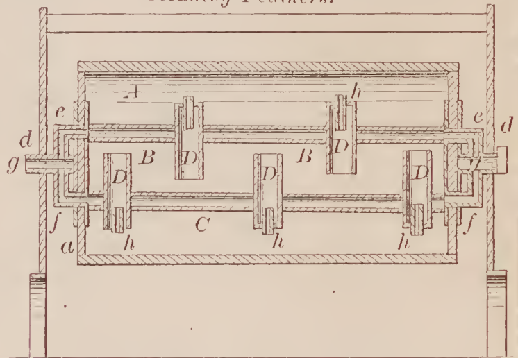
69114—O. C. Monroe—For Renovating and Cleaning Feathers.
