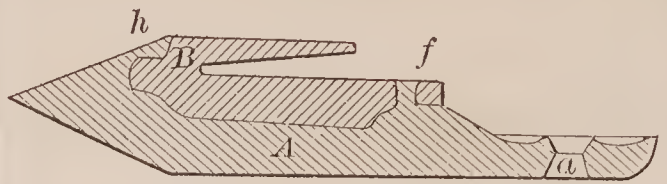
71257—W. A. Wood—Harvester Guard Finger.
