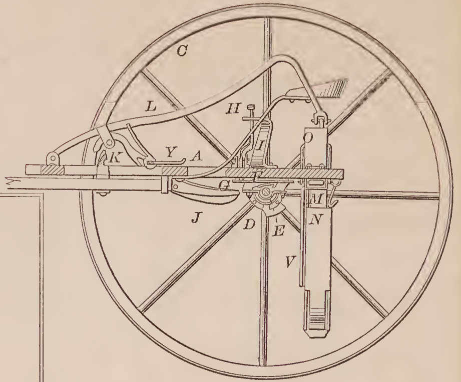
72501—H. J. Johnson— Corn Planter.
