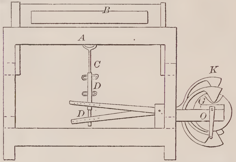
67699—H. Yount—Harness Motion for Looms.
