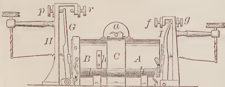
67410—S. G. Cabell—Telegraphic Instrument.
