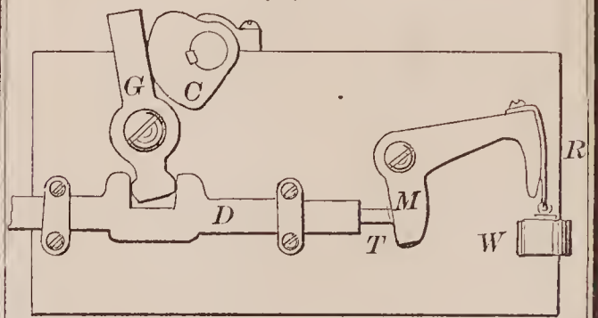
72153—A. Alexander—For Making Bolts.
