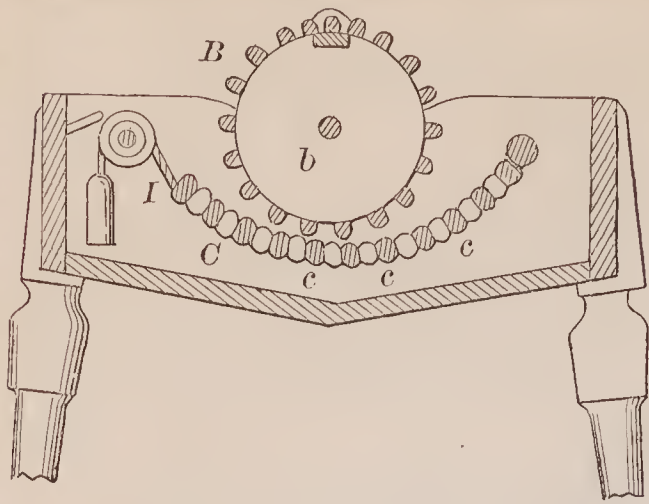
70096—G. H. Kidney—Washing Machine.
