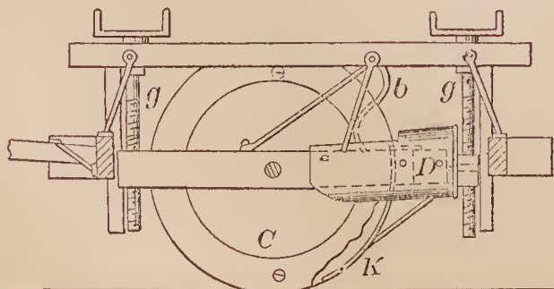
68975—Gifford & Seright—Ditching Machine.
