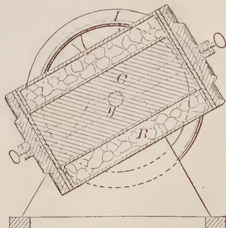
67599—W. H. Skerrett— Ice Cream Freezer.
