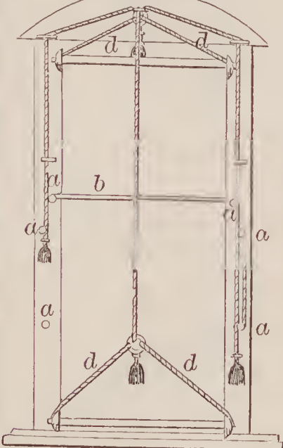
71679--A. P. Barlow--Curtain Fixture.
