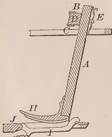
69380—E. Wright—Picker for Looms.
