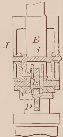
67112—W. P. Heffron— Boiler Tube Cleaner.
