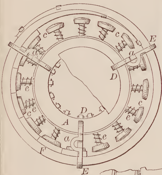
70738—J. A. Morrell—For Setting up Staves in Barrels.
