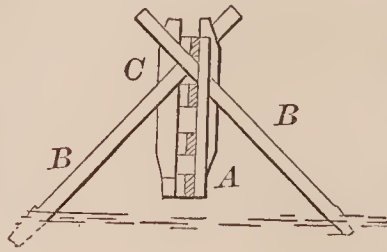
72503—T. W. Kennedy— Hand Truck.
