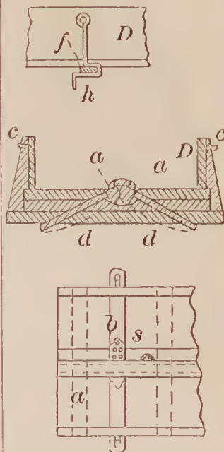
69074—W. B. Chapman—Neck Yoke.
