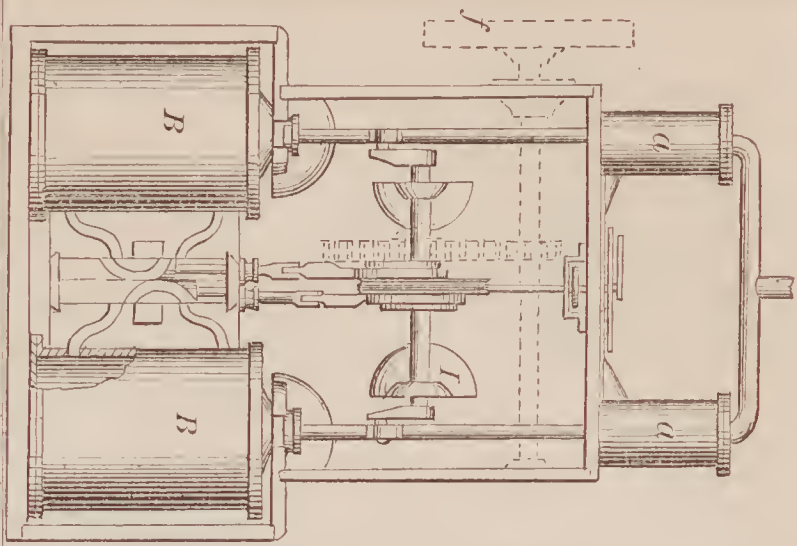
68127—E. Spencer—Water Meter and Force Pump.
