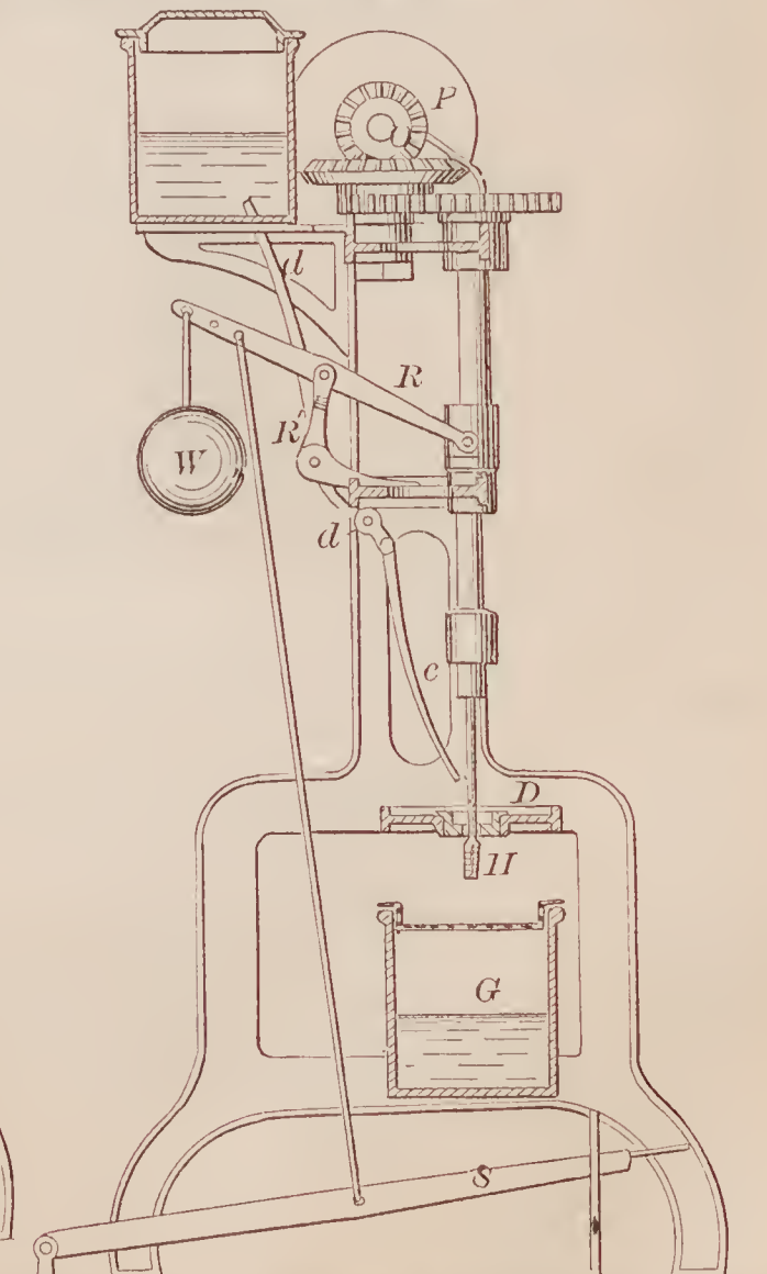
70862—J. Kirkley— Nut Tapping Machine.
