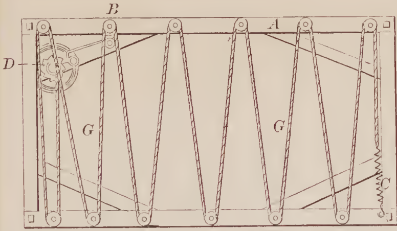
71506—D. Morrison— For Converting Motion.
