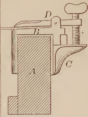
68668—A. Storm—Bed Clothes Clamp.
