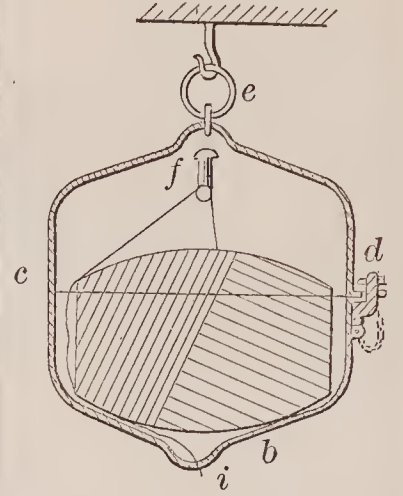
71655—R. L. Smith—Twine Holder.
