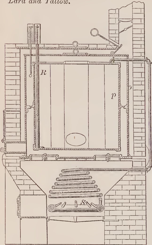
69897—A. Broadnax—For Rendering Lard and Tallow.
