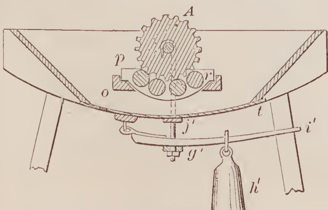
67565—P. H. Munson—Washing Machine.
