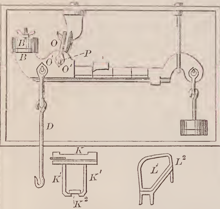
67879—W. G. Hyndman—Brick Machine.
