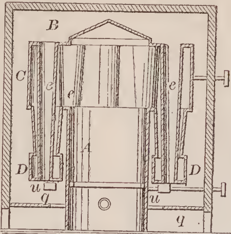
69571—D. E. McSherry—Seed Drill Tooth.
