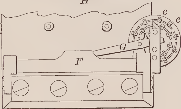
71873—J. Harris— Car Axle Box.
