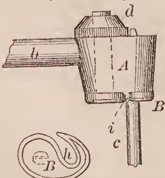
69086—J. B. Fellows—Brace for Boring Bits.
