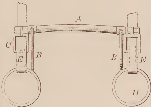
66943—W. G. Brownson—Telegraphic Switch Board.
