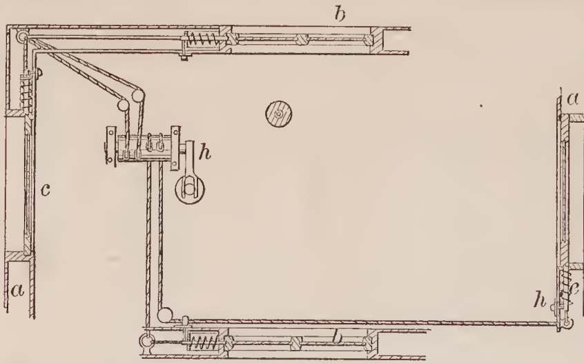
69753—A. H. Boyd—For Locking Doors and Windows.
