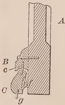
72543—H. A. Robinson— Weather Strip.
