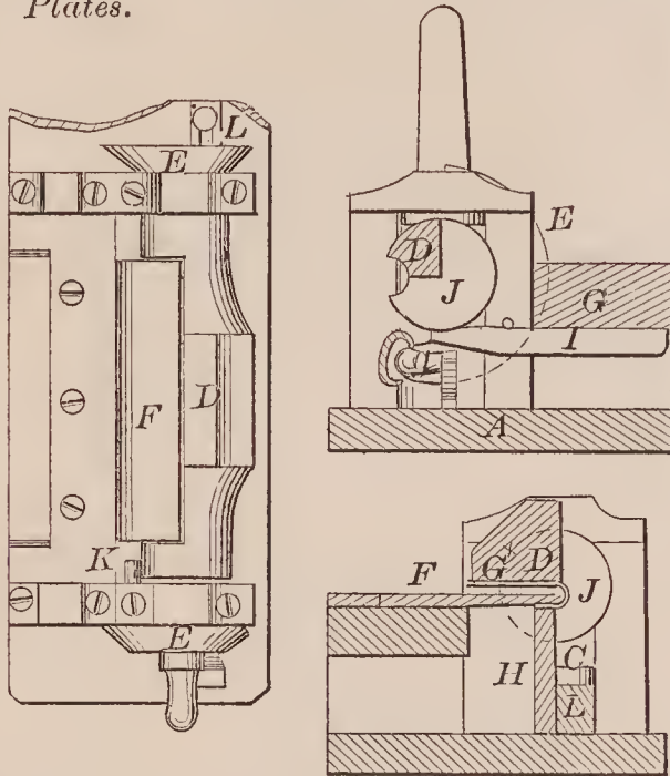
72561—O. W. Stow— For Folding Tinned Plates.
