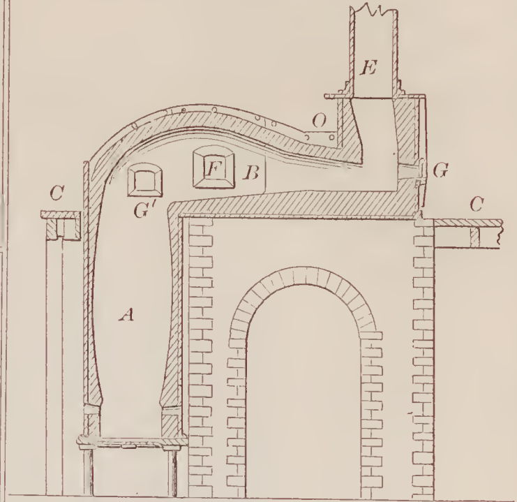
67646—Green & Kay—Reverberatory and Cupola Furnace.
