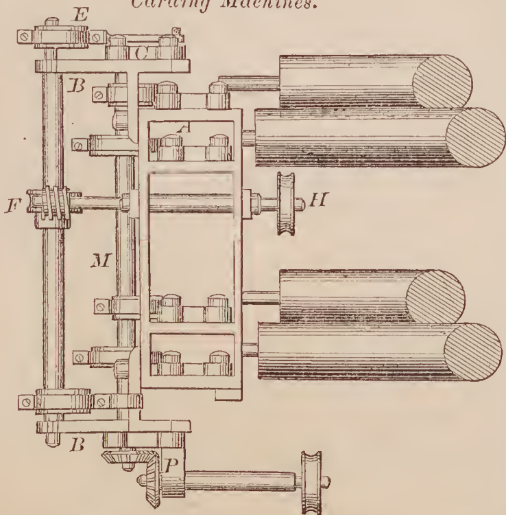
68464—E. Stafford— Condensing Roller in Carding Machines.
