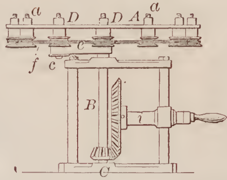
67740—M. Esselen—For Raising and Drying the Naps of Hats.
