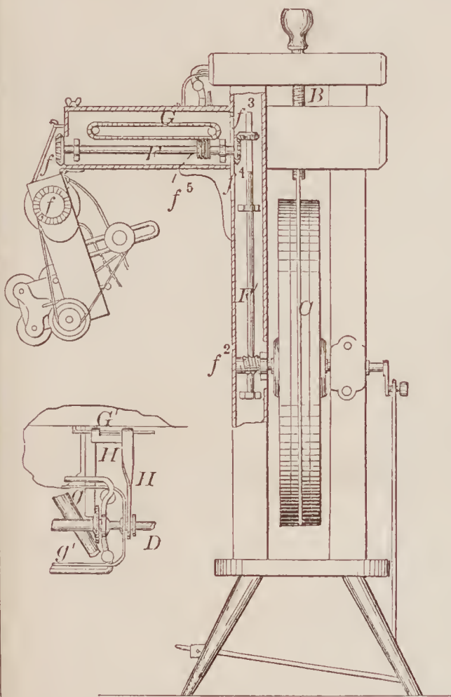
69729—J. C. Walker—Hot Air, Steam and Water Gauge.
