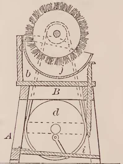
70571—S. W. Huntington—Boot Blacking Machine.
