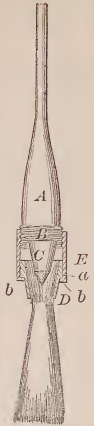
70185—O. H. P. Fancher—Anti-Kicking Attachment for Horses.
