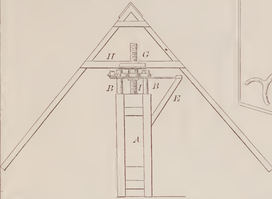
67243—Y. F. Wright—Cotton Press.
