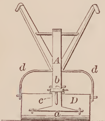
72510—W. C. Lewis—Head Block.
