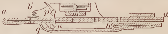
69058—E. B. Winslow—Trace and Pad Buckle.
