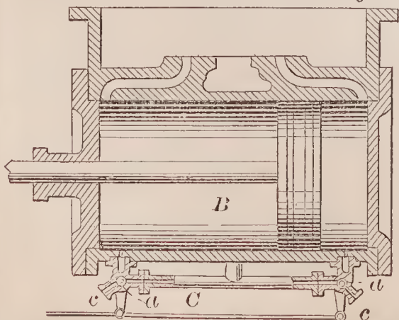
70948—E. Bourson—Steam Engine.
