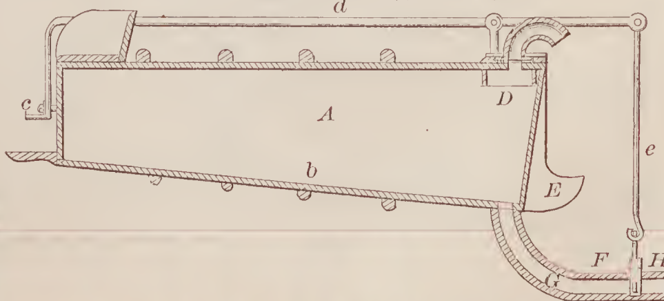
67805—L. Rodenhausen— Street Sprinkling Cart.
