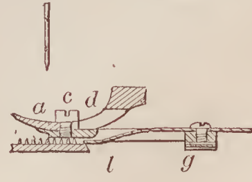
67582—T. K. Reed—Gathering Device for Sewing Machines.
