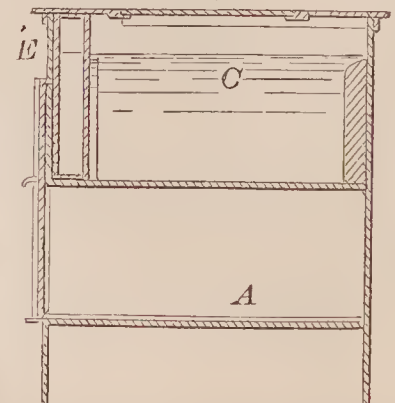
66955—R. E. Deane—Cooking Range.
