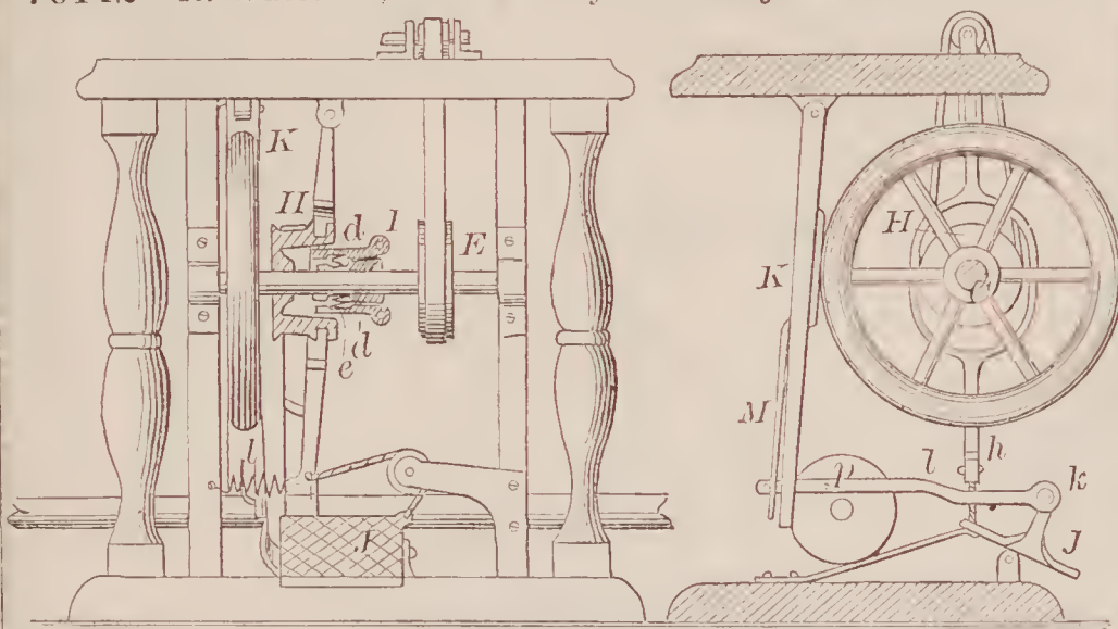
70142—R. Whitehill, Jr.—Motor for Sewing Machines.
