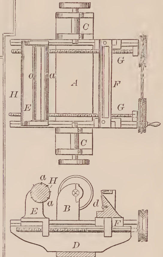
66997—T. B. Smith—For Cutting Veneers.
