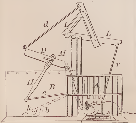
70133—J. Trainer—Animal Trap.
