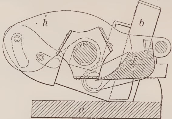
67623—G. E. Woodbury— Planing Machine.
