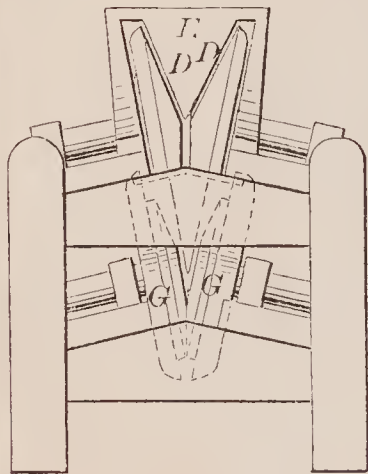
71165—J. H. Harper—Cider Press.
