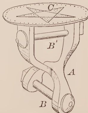
66954—J. H. Deal—Step for Spring Wagons.
