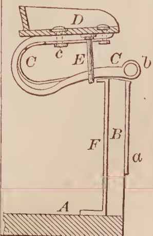
68479—R. L. Allen—Wagon Seat and Spring.
