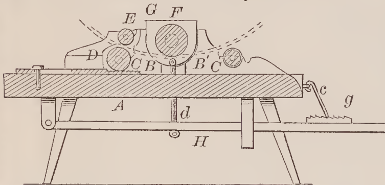
67788—F. Mills— For Bending Tires.
