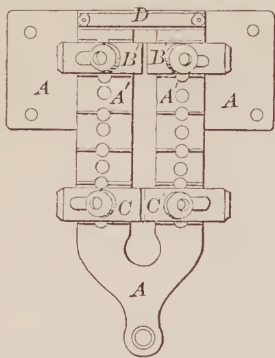
71859—H. P. Dillingham— Guide for Saws in Saw Mills.
