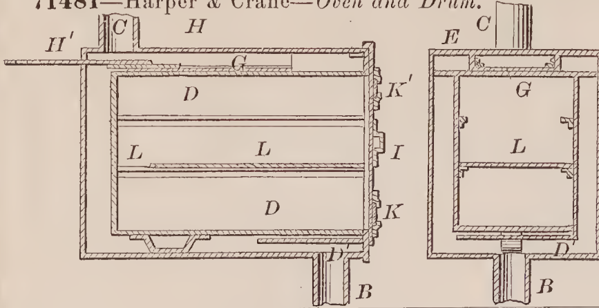
71481—Harper & Crane— Oven and Drum.
