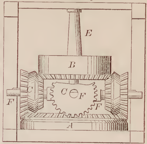
70970—J. C. Cunningham—Mill Gearing.
