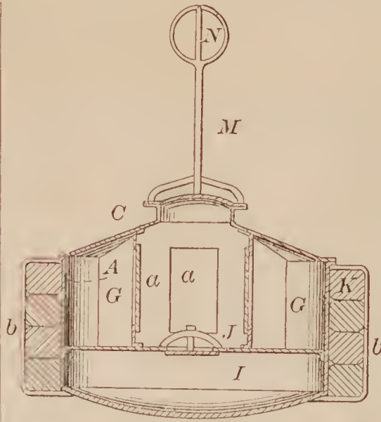
68349—F. C. Buisson—Buoy Safe.
