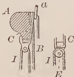
67876—C. F. Herrick—Curtain Fixture.
