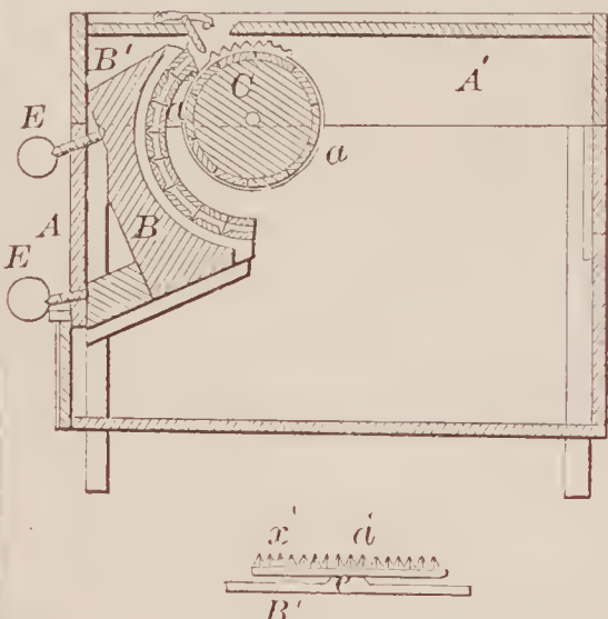
71551—S. Terry— Corn Sheller.
