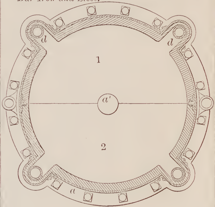
67762—J. Heaton— Converting Cast Iron into Bar Iron and Steel.
