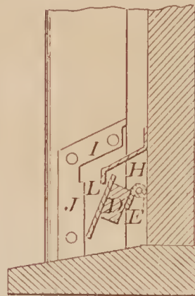
69010—J. H. Miller—Weather Strip for Doors.
