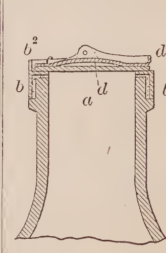
69143—N. Thompson—For Closing the Mouths of Bottles
