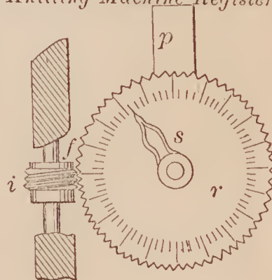
68928—Wyman & Hartshorn—Knitting Machine Register.
