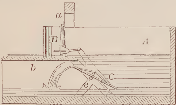
66795—W. L. Clark— Flood or Waste Gate.
