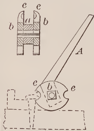
67552—H. Jeffrey—Nail Extractor.
