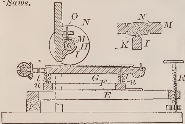
67480—E. C. Atkins—For Grinding Saws.
