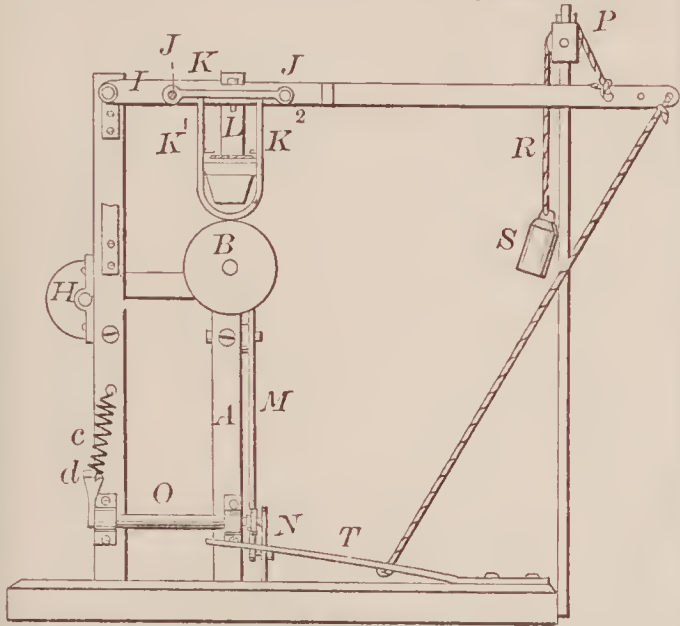
68621—S. C. & E. O. Frink—Wood Bending Machine.
