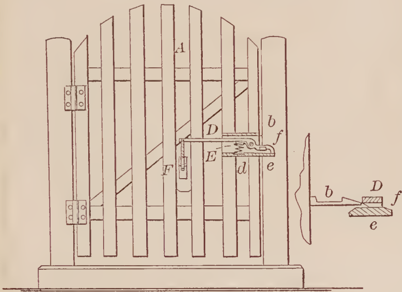
72536—W. W. Peck—Gate Fastening.
