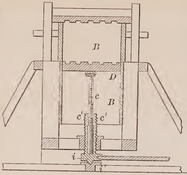
71442—A. B. Bean—Knife Sharpener.
