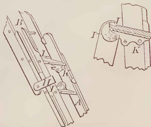
67636—C. Croley—Ladder.
