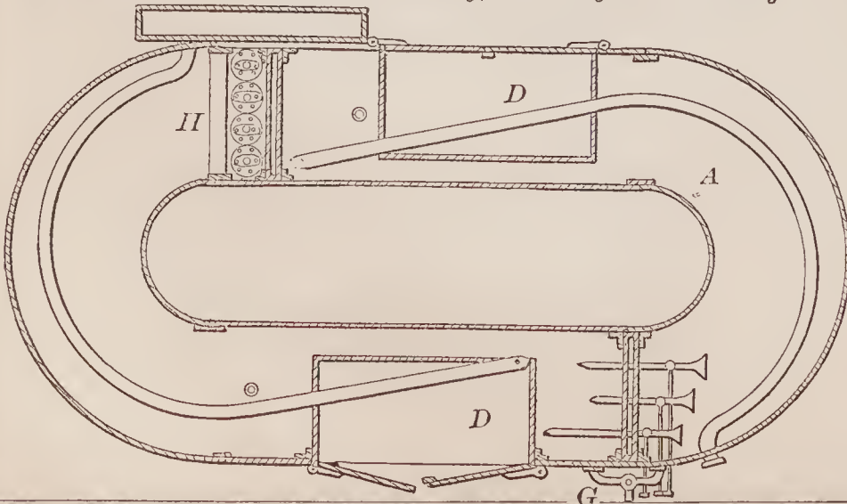
69955—D. E. Somes— For Cooling, Freezing and Heating.
