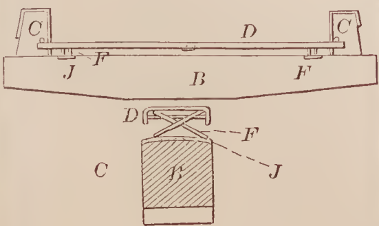
69094—B. Hershey—Wagon Spring.
