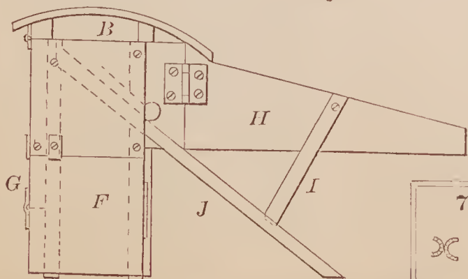
72377—D. Durfee—Fruit Dryer.
