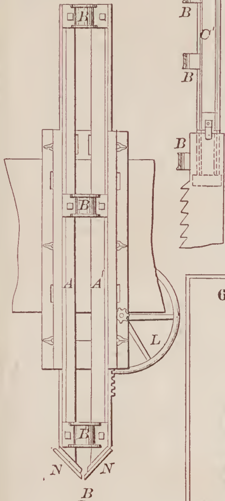
69744—L. Anderson— Saw Mill.
