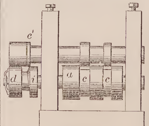
71062—A. Reese—Shaping Dies of Grooved Rolls.
