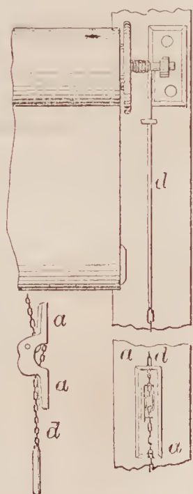
71114—G. Allix—For Raising Window Curtains.
