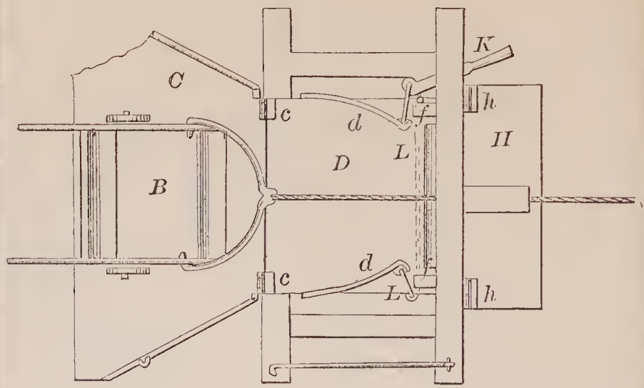
70196—W. Goff—Portable Dumping Machine.
