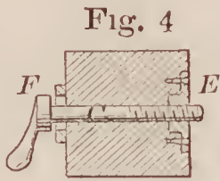
70354—Peterson & Gunner— Boat Detaching Tackle.
