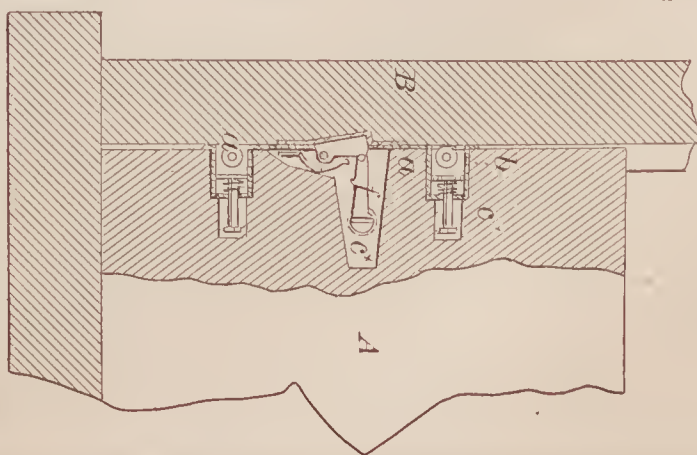
69456—D. D. Mackay—Sash Lock and Stop.
