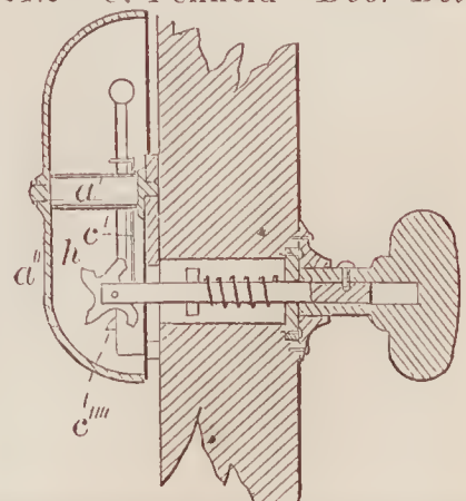
67212—C. Penfield—Door Bell.
