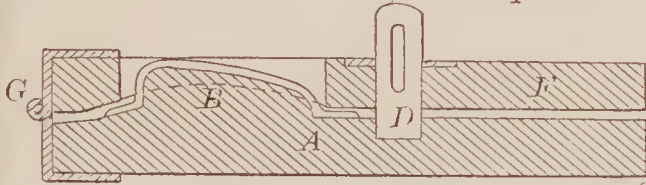
68156—H. H. Beers—Pad Crimp Press.
