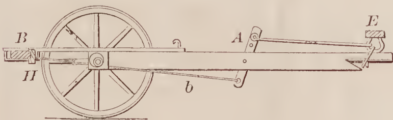
71054—C. Phelon—Brake for Vehicles.
