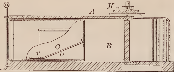
70625—L. O. Schultz—Car Coupling.
