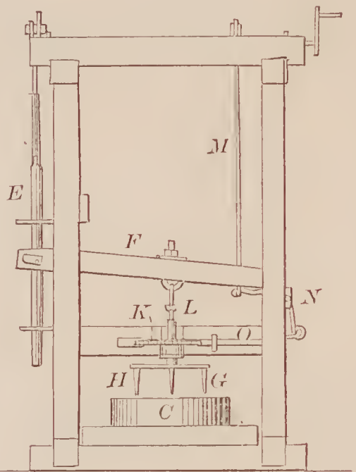
66990—W. L. Overhiser—Hay Elevator.
