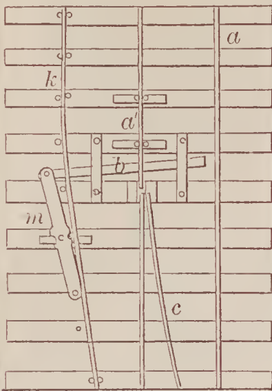
67443—McLaughlin & Jones—Railroad Switch.
