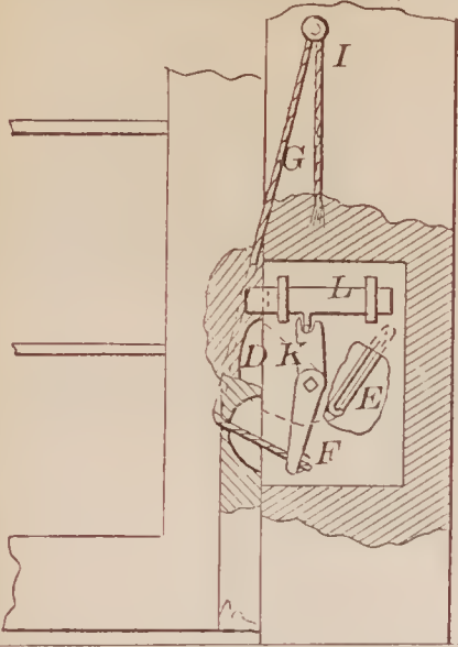
70796—W. H. Bryant—For Drawing Tires from Engine Driving Wheels.
