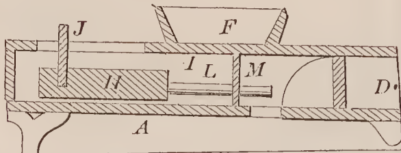
67604—W. Stickney—Bed Bottom.
