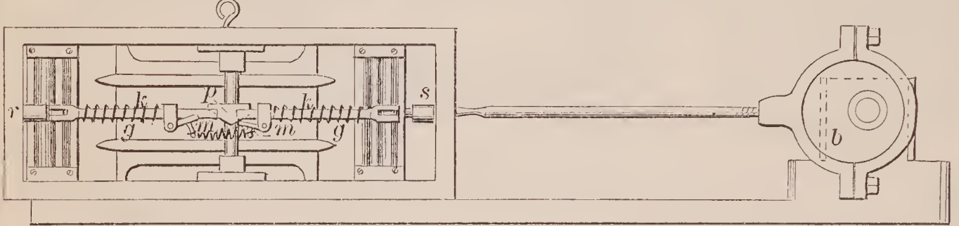
70743—G. W. Rawson— Steam Engine Cut-off.
