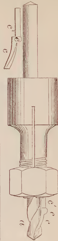
70686—J. A. Bidwell—Tapering Drill.
