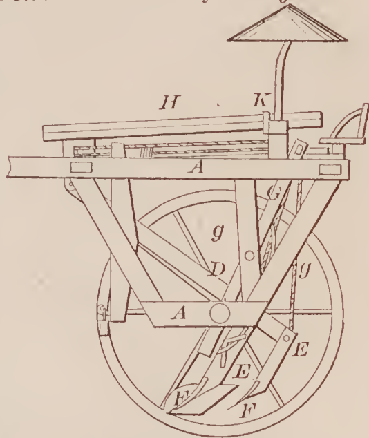
68277—G. C. Avery—Gang Plow.
