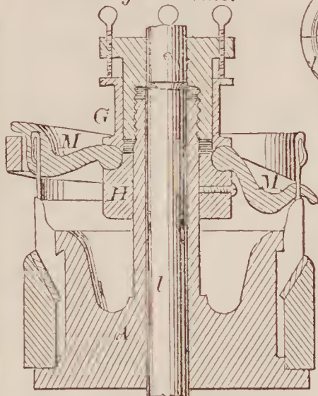
72117—J. Teachout—Knitting Machine.
