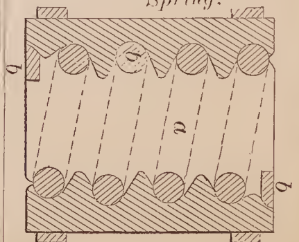
72941—R. Vose—Car Spring.
