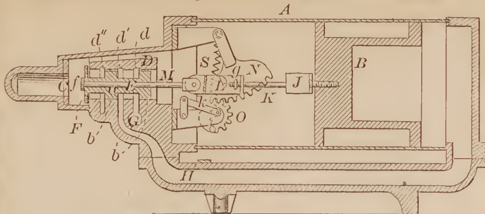
69007—J. Mason—Liquid and Gas Meter.
