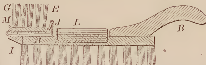
70515—G. R. Burdon—Blacking Brush.
