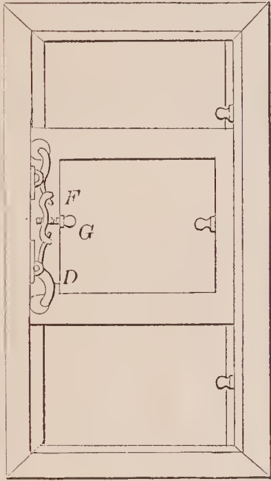
70818—A. Cutter—Sash Supporter and Fastener.
