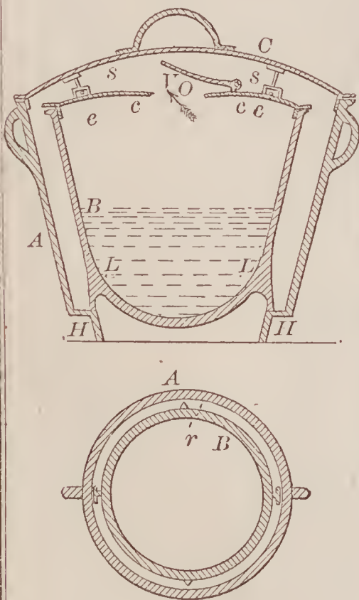
67452—Purdy & Barger—Boiler.
