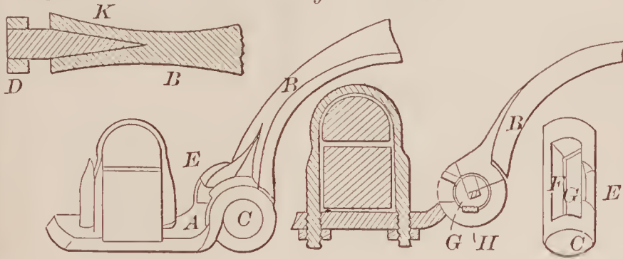
70357—T. D. Powers— Wagon Shackle.
