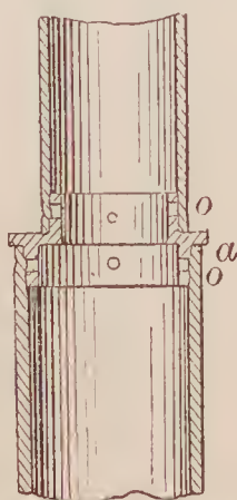
69506—W. Stine—Stove Pipe Joint.
