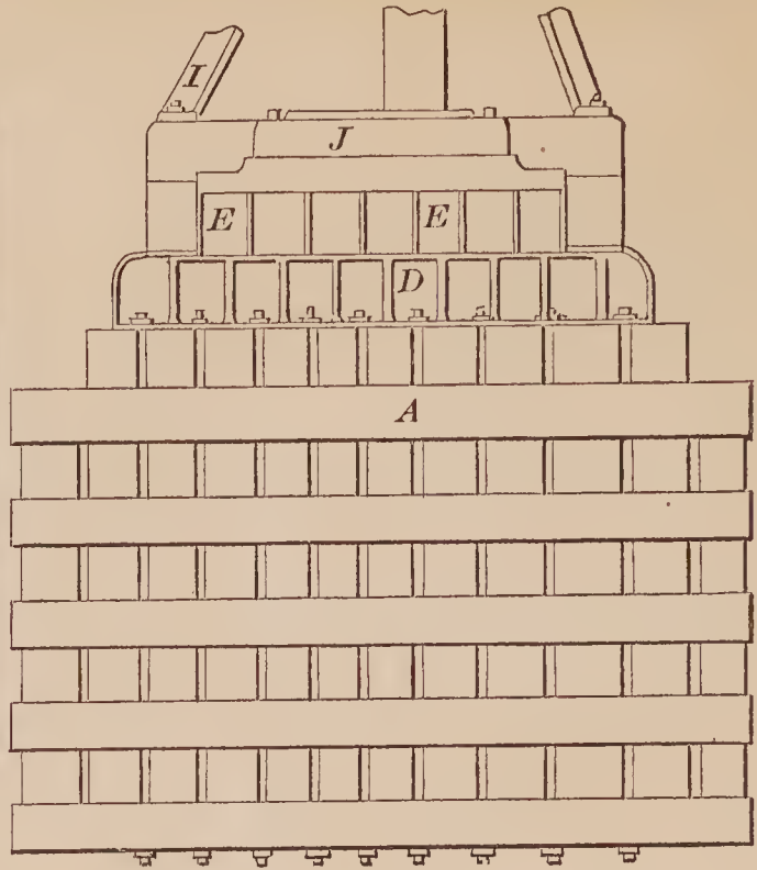
72715—W. Ball— For Stamping Ores.
