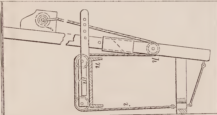
71139—N. B. Crawford—Building Scaffold.
