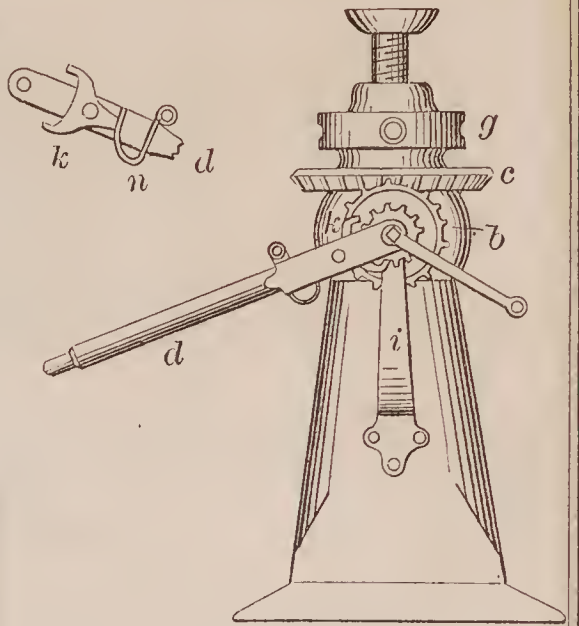
68241—C. H. Sawyer—Jack Screw.
