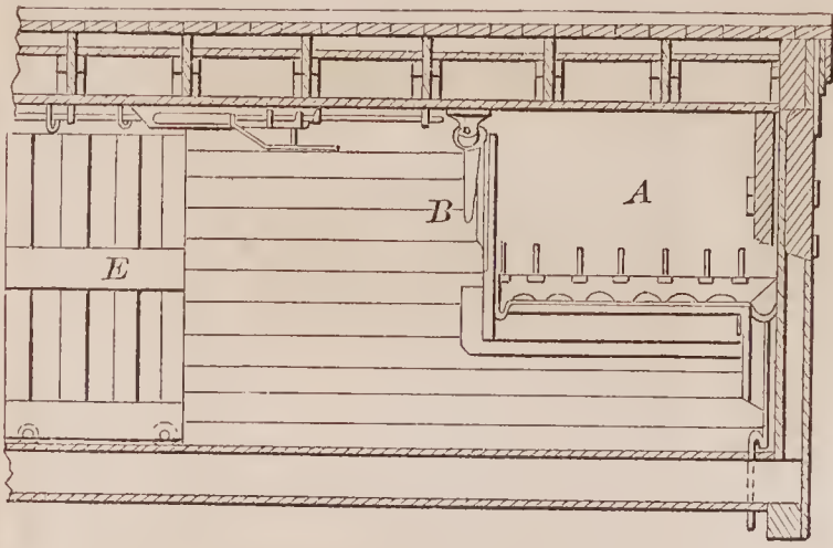
71423—J. B. Sutherland—Refrigerator Car.
