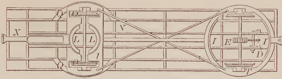
9332—S. Freet— Horse Rake.
