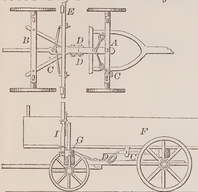
69604—Alley & Williamson— Wagon Brake.
