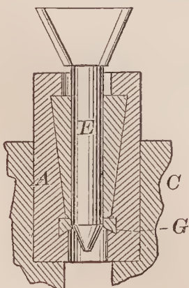
68187—H. M. Hamilton—Die for Forming the Eyes of Picks.
