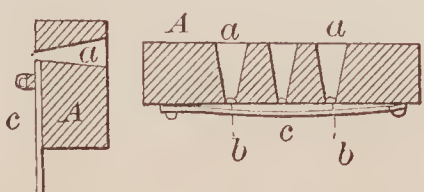
69997—A. Huston— Needle Threader.
