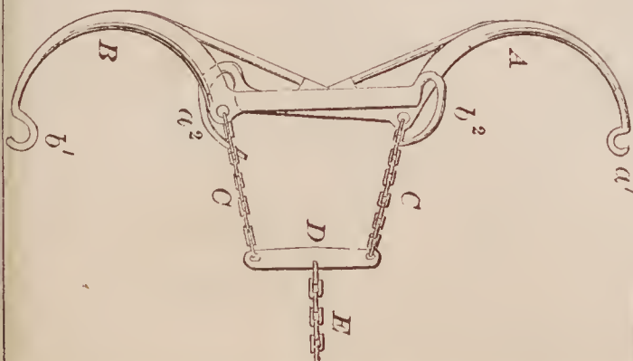
70502—T. J. Barnes— Horse Yoke.
