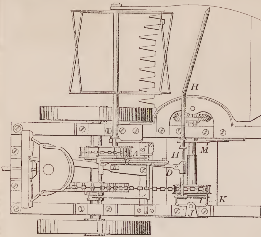
71098—P. Werni—Harvester Rake.
