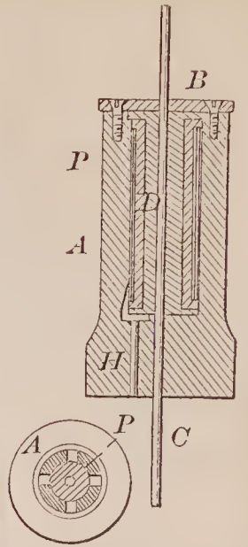
72340—S. S. Turner—Piston Rod Packing.
