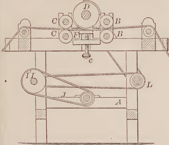
69219—W. C. Joslin—For Reducing Roller Leather to a Uniform Thickness.
