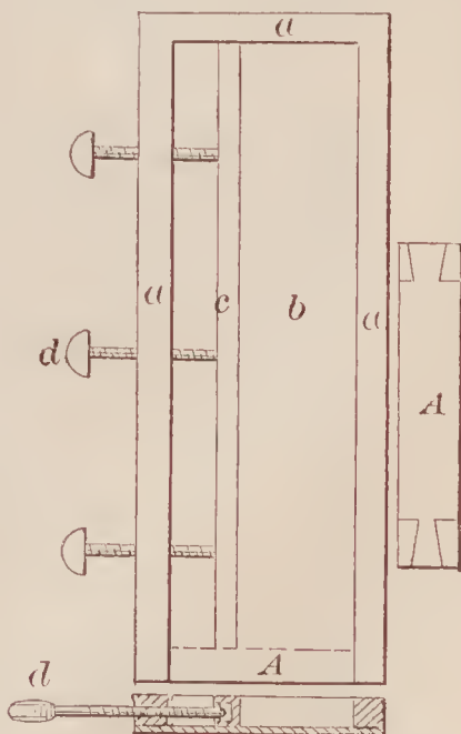
66776—J. W. Baker—Printers' Galleys.
