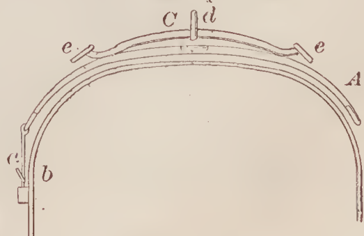
67566—J. M. Myers—Breast Collar and Spreader.
