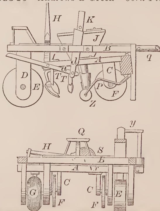
68544—Andrews & Green—Corn Planter.
