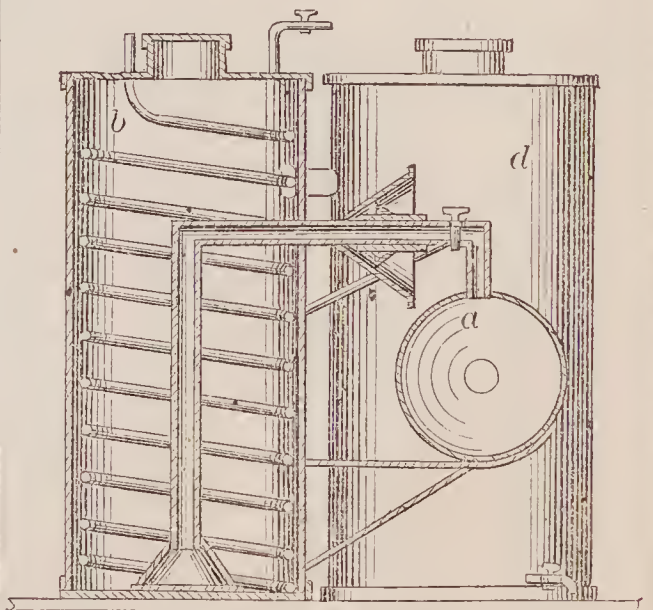
67796—J. C. Pedrick— For Treating Petroleum.
