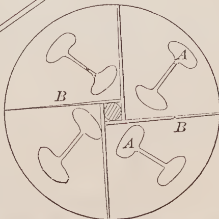
67205—F. McFarnahan—Churn Dasher.
