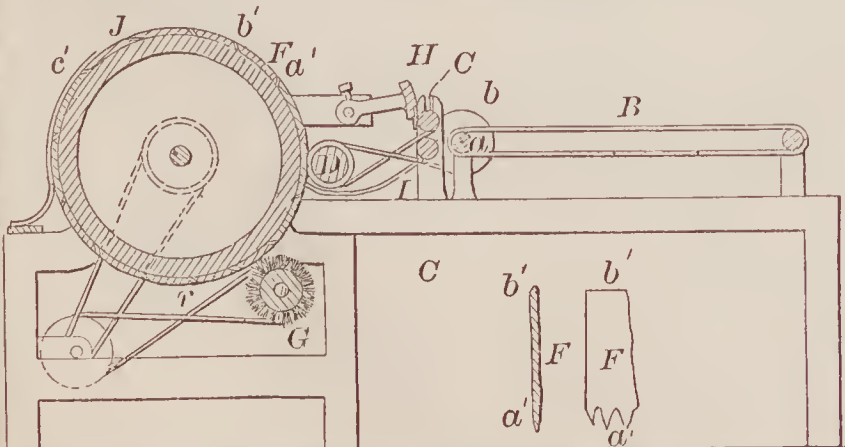
67394—R. J. Clay— For Barring Wool.
