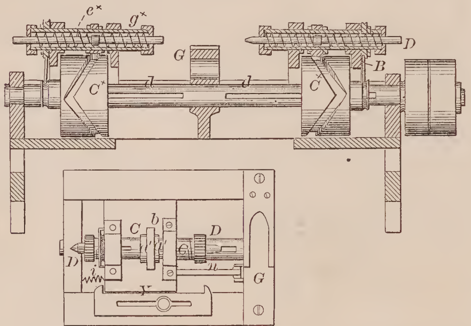
68682—E. B. Armstrong—Cut-off for Water Conductors.
