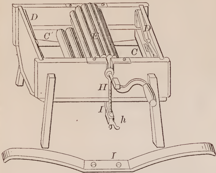
70348—J. W. Melcher—Detachable Whiffletree.
