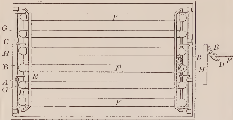
71935—M. Winger—Cider Mill and Press.
