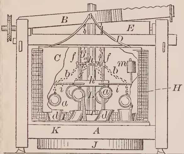
69360—J. Mumma— Water Wheel.
