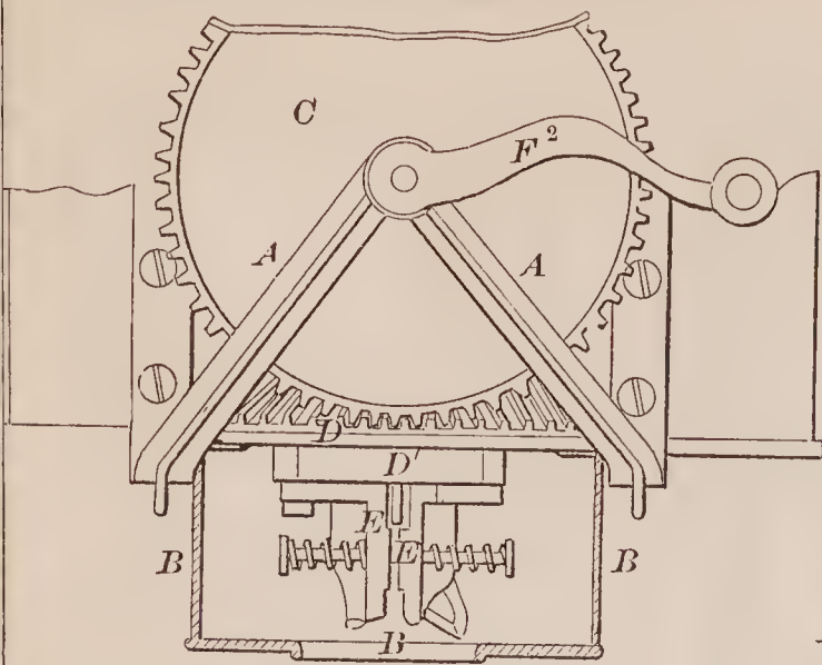
70396—T. W. Bishop— Corn Sheller.
