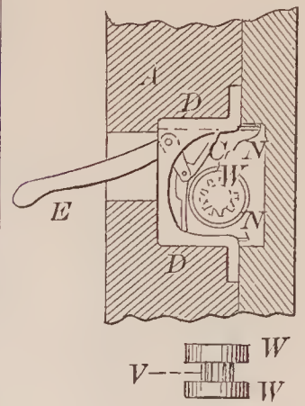
69540—F. P. Canfield—Sash Lock and Support.
