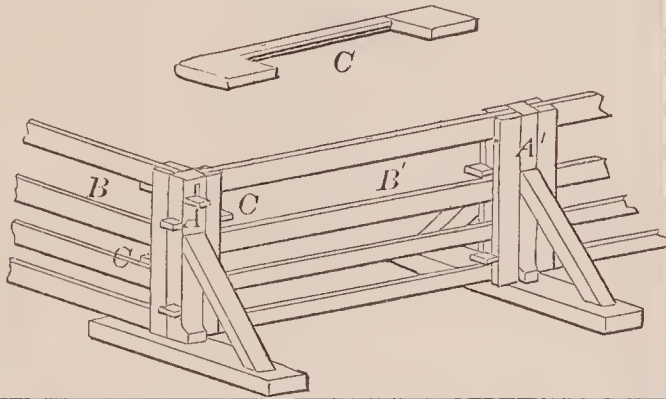
68167—M. D. Cheek—Cotton Bale Tie.
