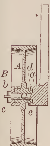
67513—G. Dodge—Plow Wheel.
