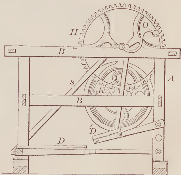
67315—Kenworthy & Silvers—Manual Power Machine.
