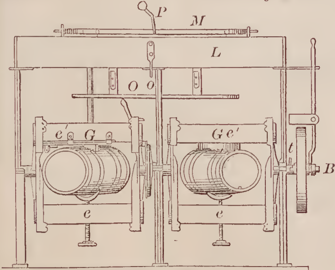
68311—J. Peacock—Barrel Washing Machine.
