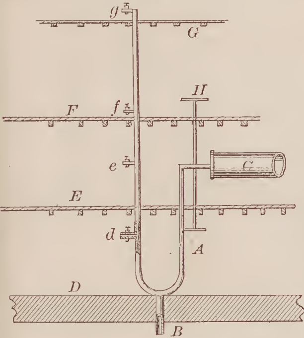
69267—D. Spooner— For Extinguishing Fire in Steamships.
