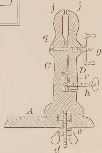
66756—W. Weaver—Rock Drill.
