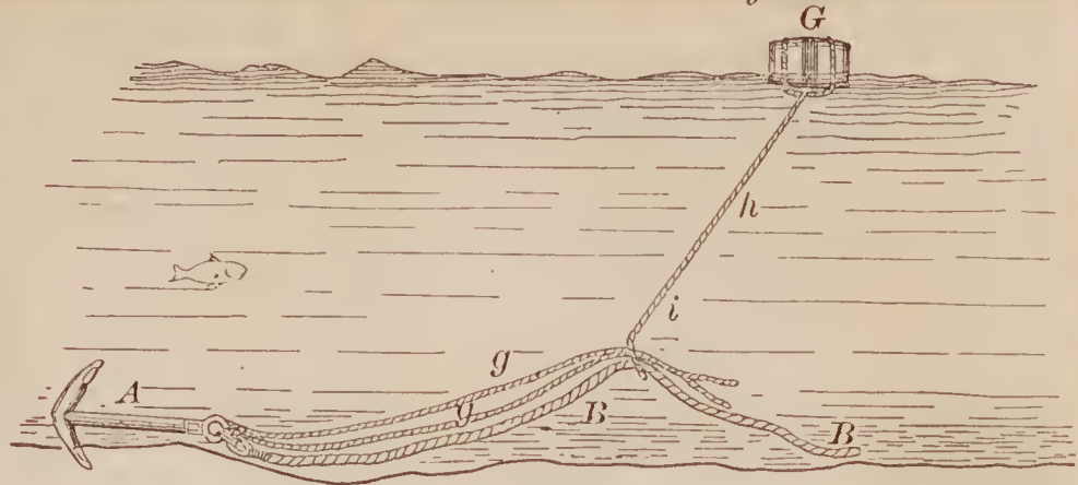
68402—C. B. Whittemore—For Recovering Lost Anchors.
