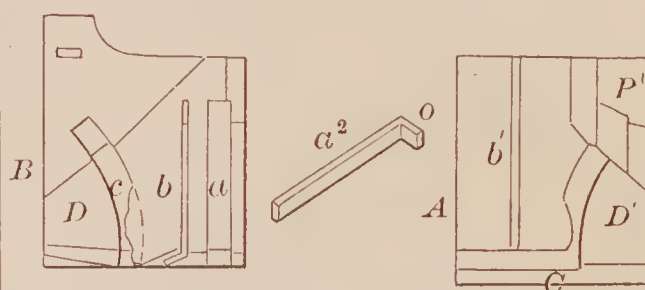
67132—J. Myers—Sleigh Brake.
