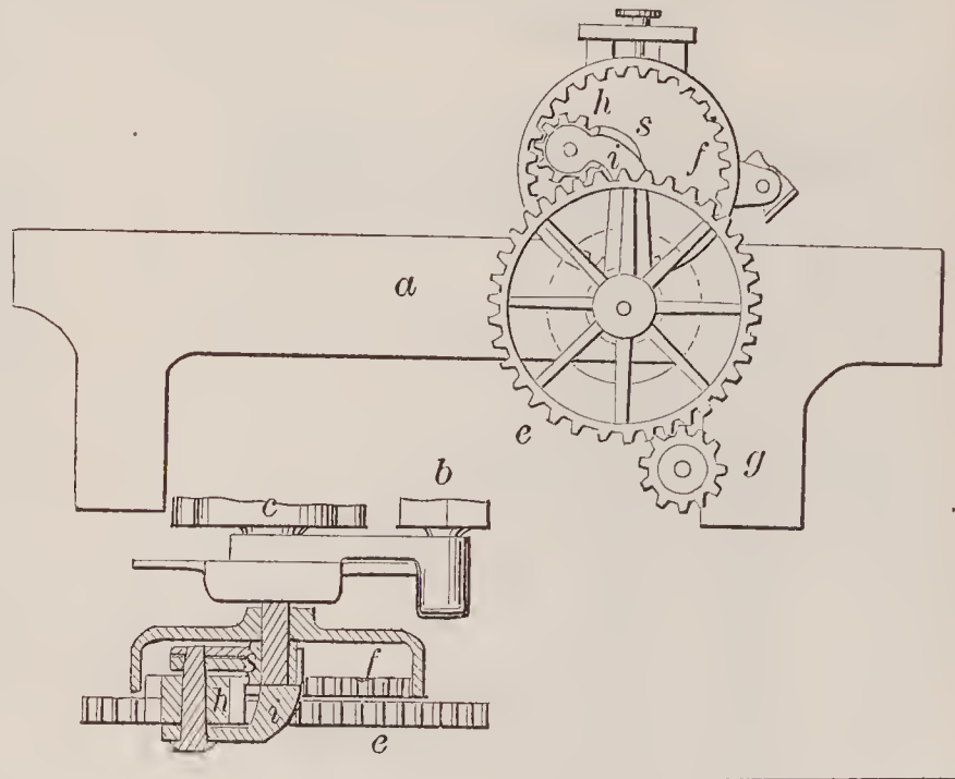
72618—B. Fitts—Planing Machine.
