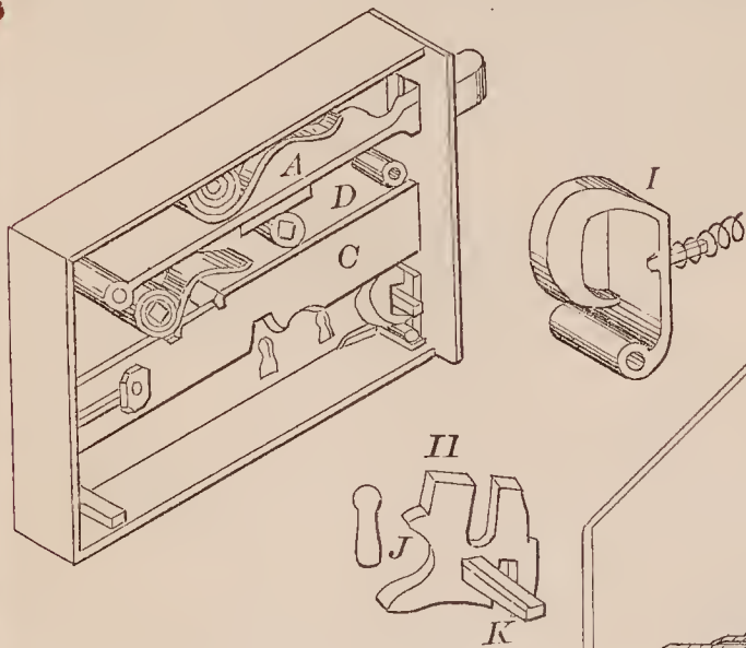
67116—G. Hubert—Compound Lock for Doors.
