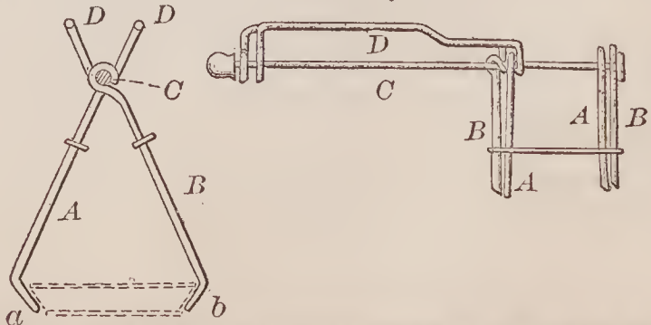
67402—C. F. Bosworth—Plate Lifter.
