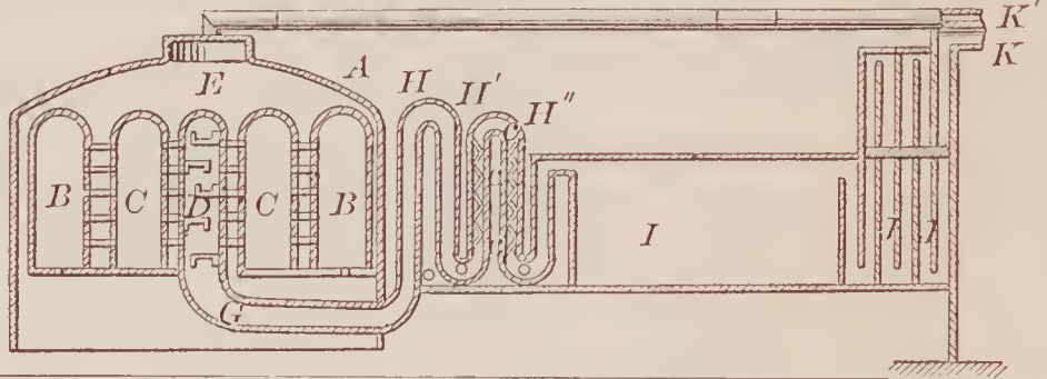
70321—J. C. Coult—For Reducing Quicksilver Ores.
