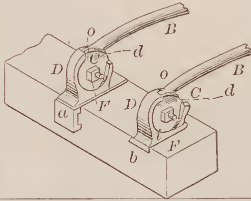
67703—R. S. Arnall—Car Coupling.
