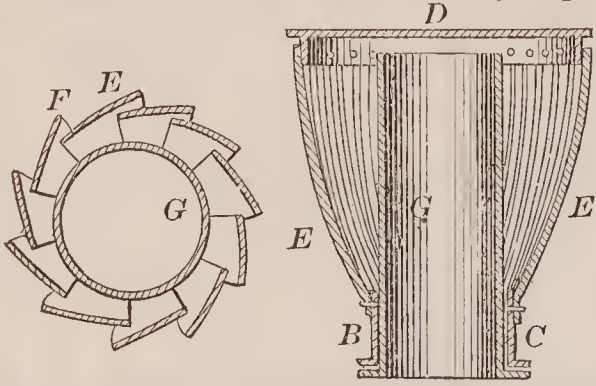
67480—E. C. Atkins—For Grinding Saws.
