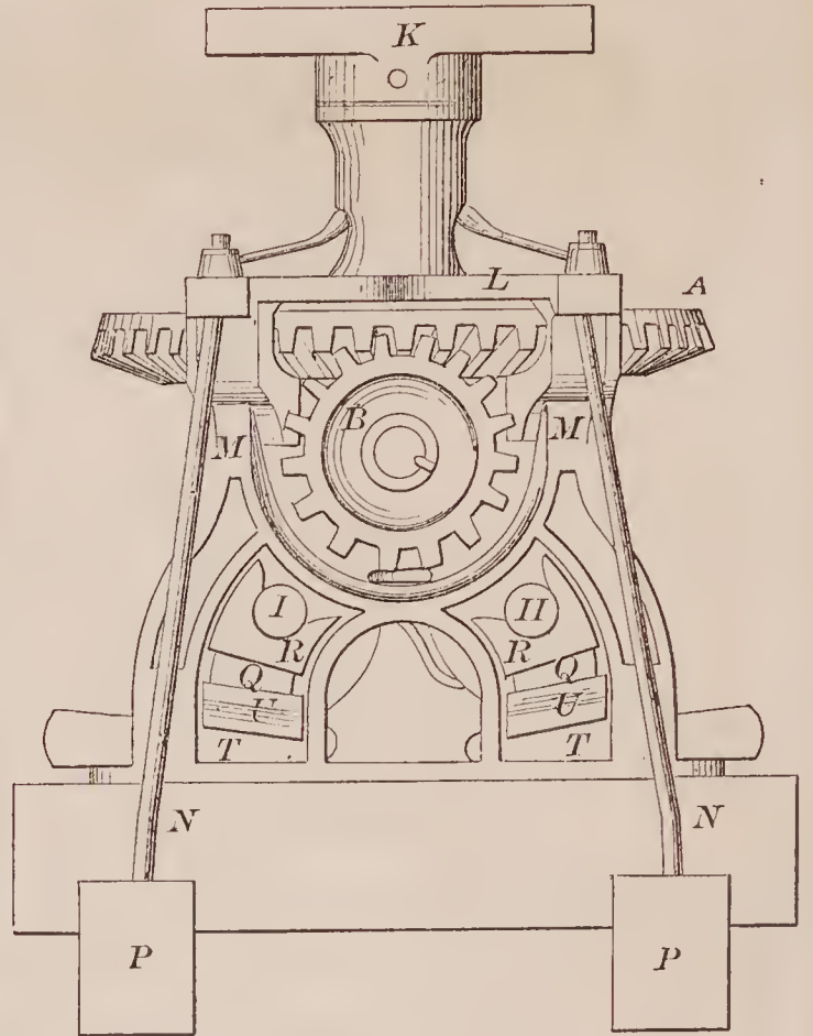
69244—Powers & Stevens—Sugar Cane Mill.
