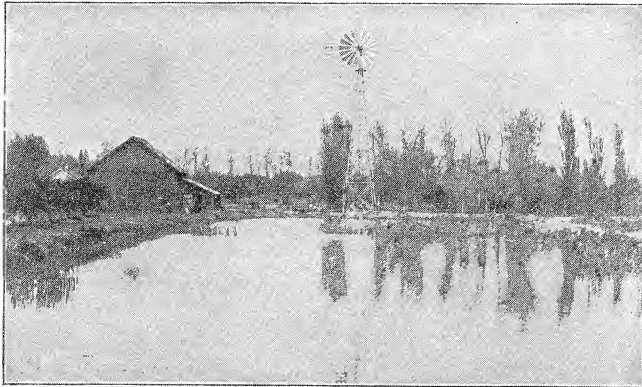
Fig. 76. Rectangular reservoir for windmill irrigation.
