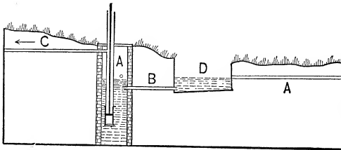
Fig. 150. Method of draining sinks by wind power.
