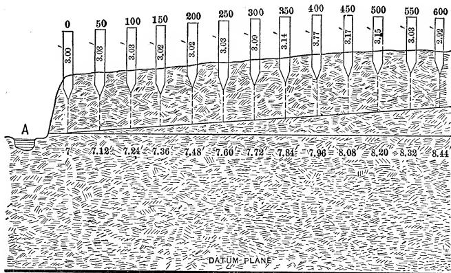
Fig. 157. Determining grade line and depth of ditch.
