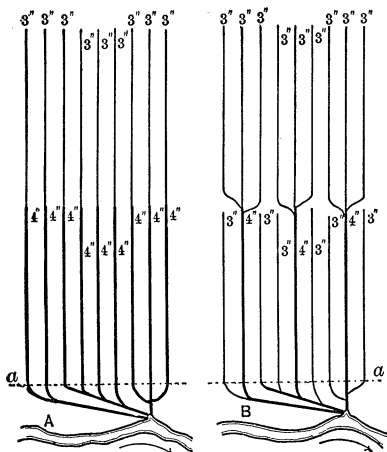
Fig. 146. Two systems of laying out drains.
