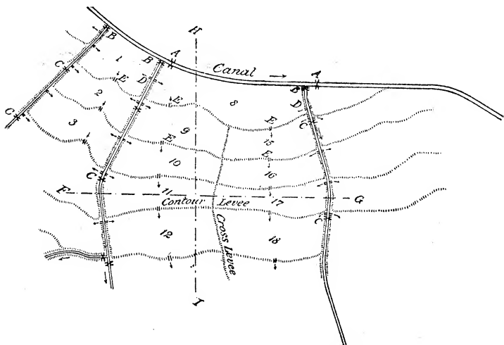
Fig. 88. Flooding field by contour checks. (Grunsky.)
