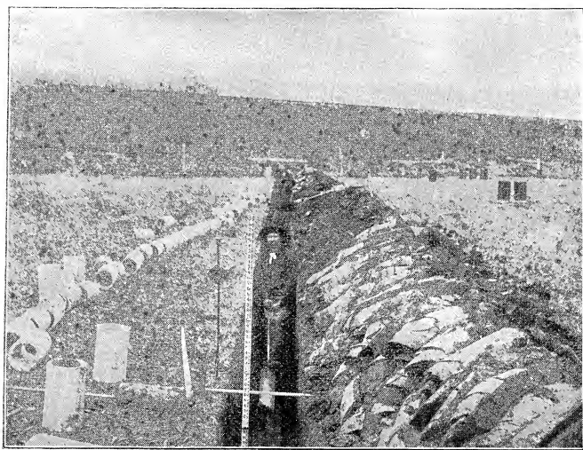
Fig. 160. Removing the last two spadings from the ditch.
