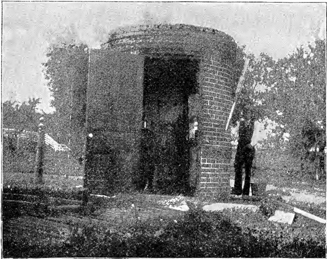
Fig. 121. Small gasoline pumping plant for garden and lawn irrigation.
