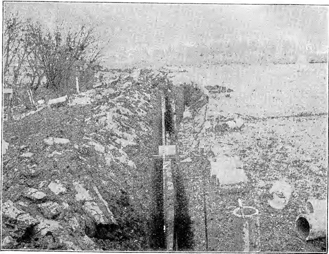
Fig. 162. Placing tile with tile hook.
