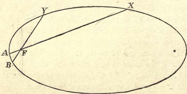
FIG. 2.—AN ELLIPTIC ORBIT
