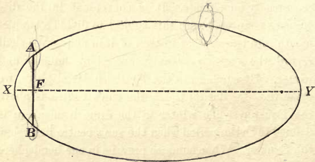
FIG. 3.—AN EXTREME CASE FOR ILLUSTRATION
