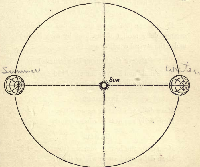
FIG. 5 —A GENIAL NORTHERN HEMISPHERE
