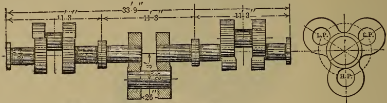
STEEL CRANK SHAFT, S.S. "ALASKA" Constructed by Messrs. John Elder & Co.
