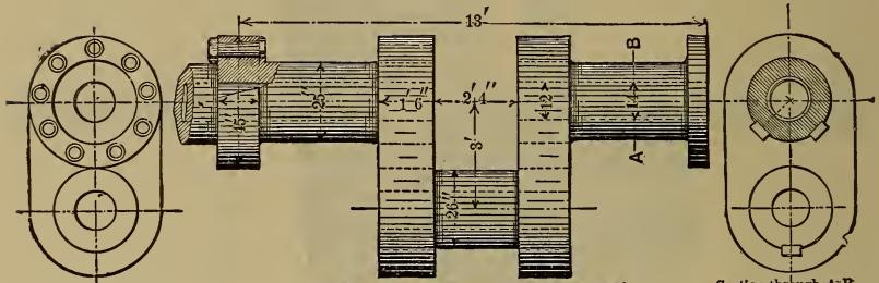
CRANK SHAFT, "CITY OF ROME" Constructed of Whitworth's Fluid Pressed Steel.
