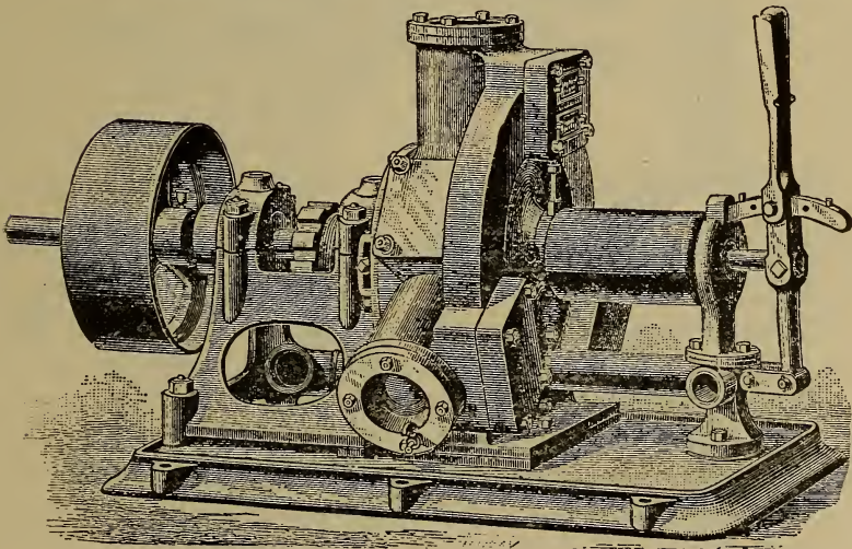
REVERSING ENGINE.
