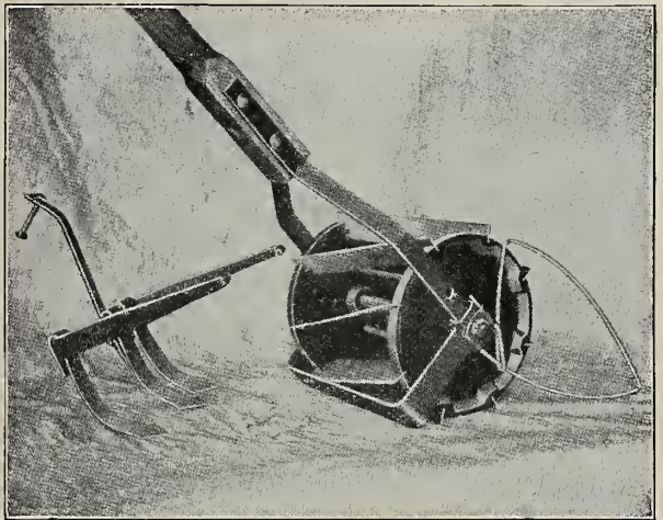
THE BARKER WEEDER
