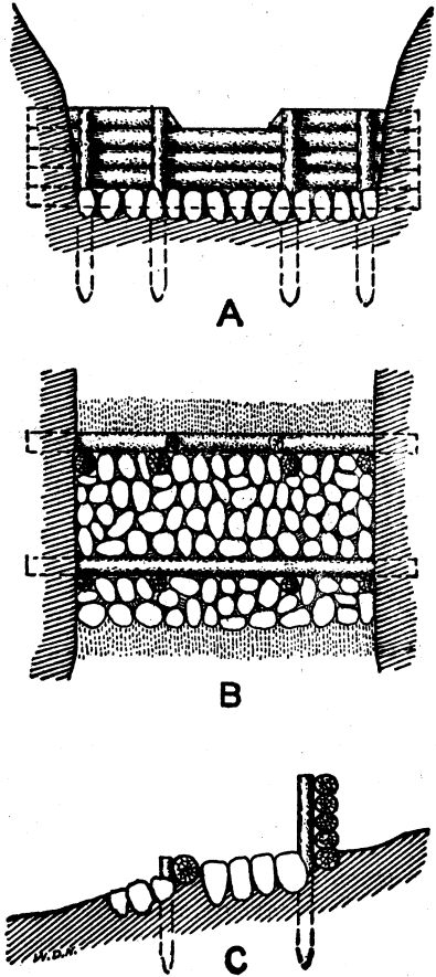
FIG. 16.—Dam built of logs and posts with spillway at center and stone pavement below the dam. A, Front view. B, Top view. C, Side view.
