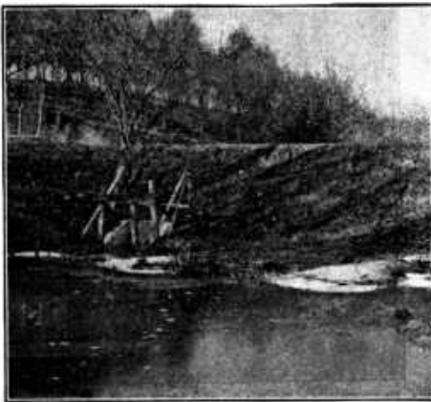
FIG. 30.—Road embankment and concrete drop inlet replacing an old bridge that was 60 feet long and 35 feet high. Depth of fill is 12 feet. Near Falls City, Nebr.
