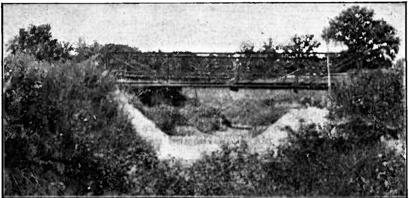
FIG. 20.—Concrete dam across large gully with sides of spillway extending to top of the banks of the gully. This dam was built to fill the gully and prevent enlargement where the highway bridge crosses. A fill of 8 feet has occurred above the dam. Near Mason City, Ill.
