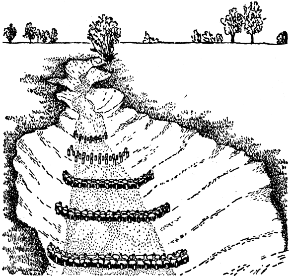
Fig. 12.—A series of stake dams in a gully. The spaces between the stakes in the three lower dams are filled with stones
