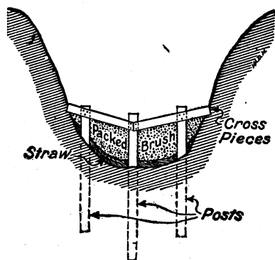
FIG. 13.—Straw and brush dam held in place by the crosspieces and posts 5
