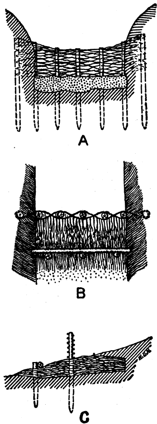
FIG. 14.—A woven-willow brush dam. A, Front view. B, Top view. C, Side view
