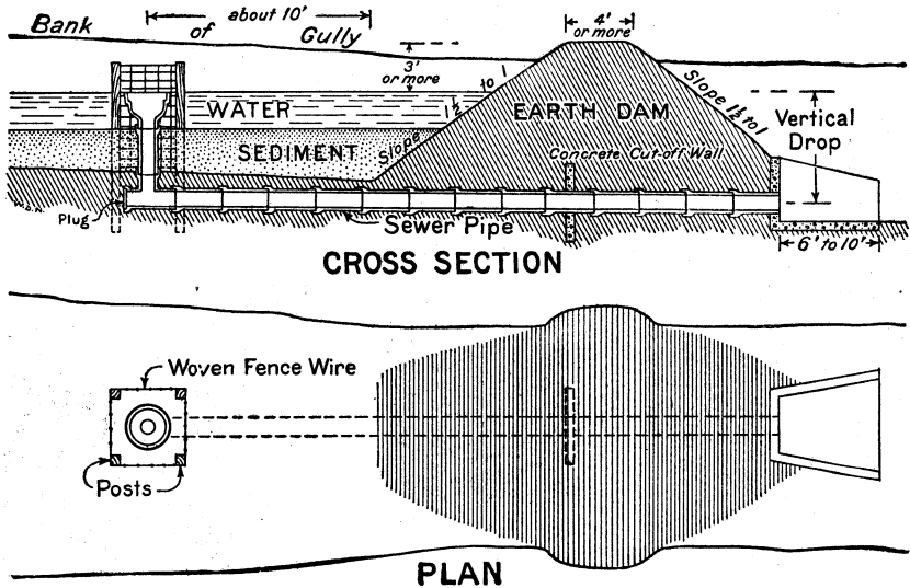
FIG. 23.—Drop-inlet and earth soil-saving dam
