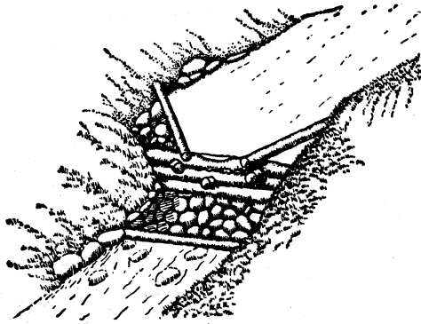
FIG. 17.—Log dam held by notched logs extending obliquely into the sides of the gully
