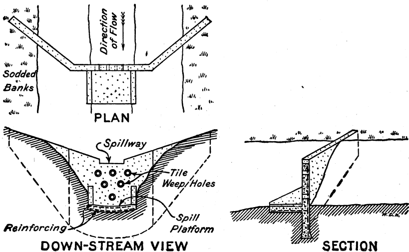
FIG. 21.—Plan, section, and downstream view of a concrete dam especially designed to guard against the common causes of failure 6
