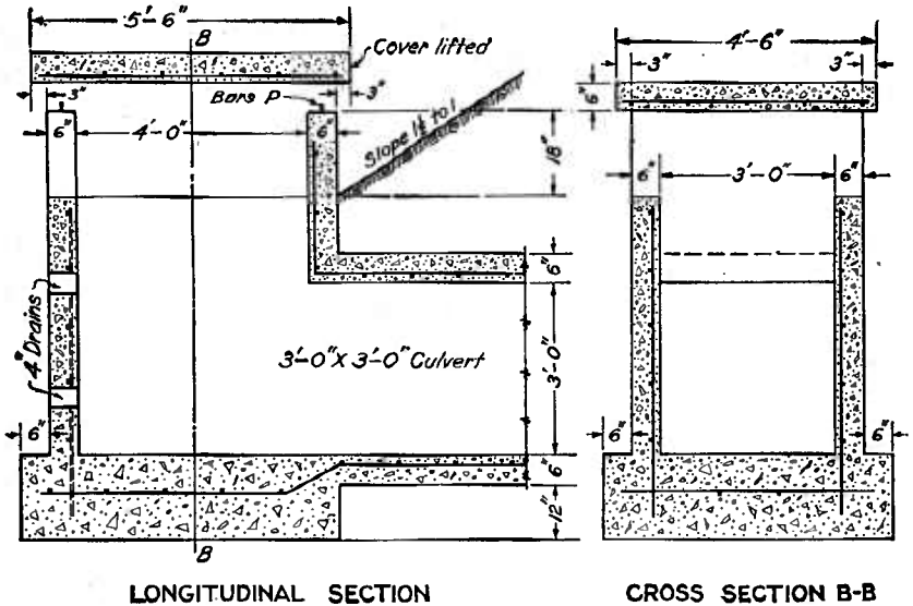
FIG. 29.—Reinforced concrete drop inlet for box culvert 7 shown in Figure 28
