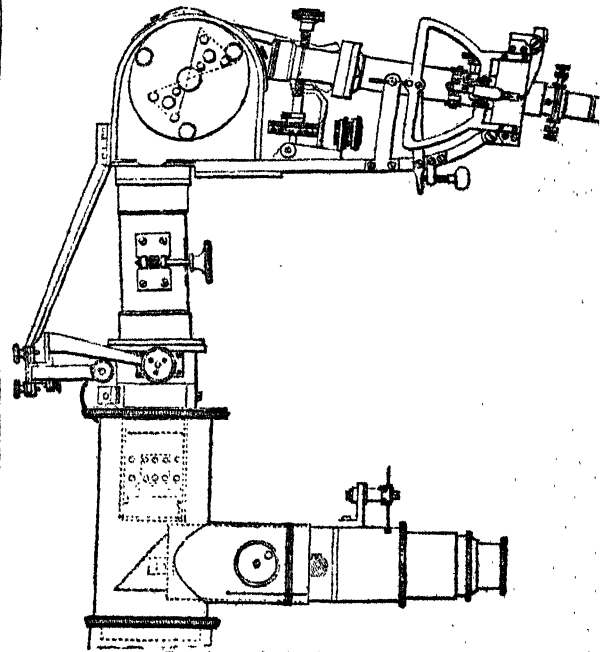
FIG. 6.—Cambridge Spectroscope.
