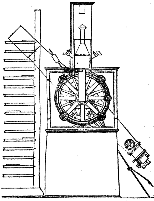
FIG. 4.—Cambridge Meridian Circle.
