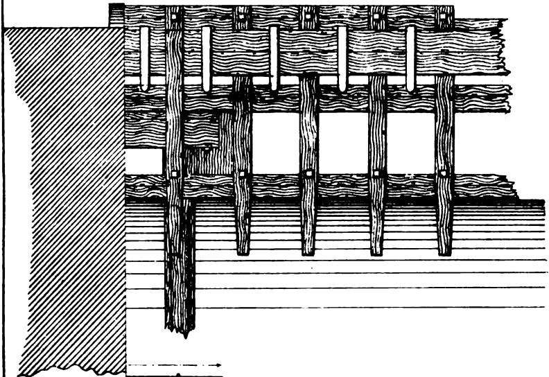
Plan of Grating Footway removed
