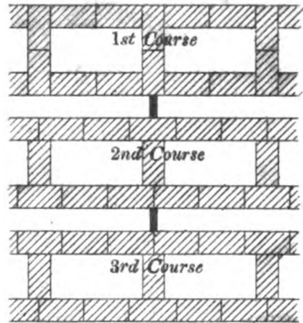
FIG. 1. —Shows the bond for a two brick wall, when it is desirable to use up half and quarter bricks.
