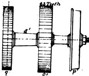
Fig. 16. Wheel Axle
