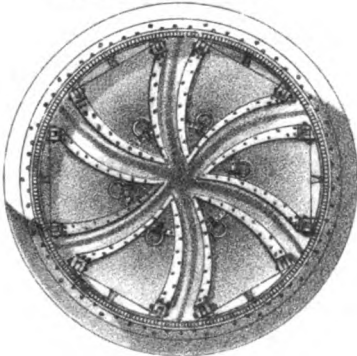
Plan of bottom of Dredger showing doors neatly closed.
