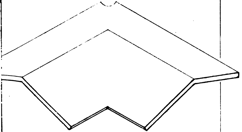
PROJECTION OF THE HIP CAP.
