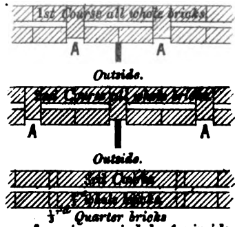
The recesses A serving as pin holes for inside plastering.
