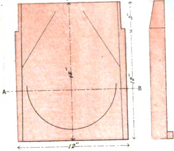
PLAN OF FLAT TILE. Fig. 11.
