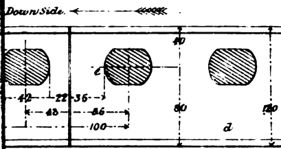
Fig. 14. Transverse Section of Ladder Rail
