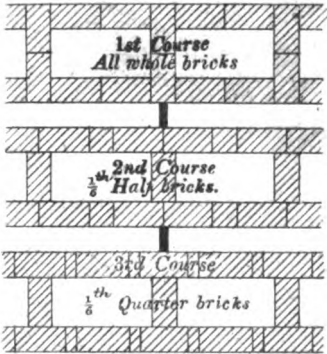
FIG. 1. —Shows the bond for a two brick wall, when it is desirable to use up half and quarter bricks.
