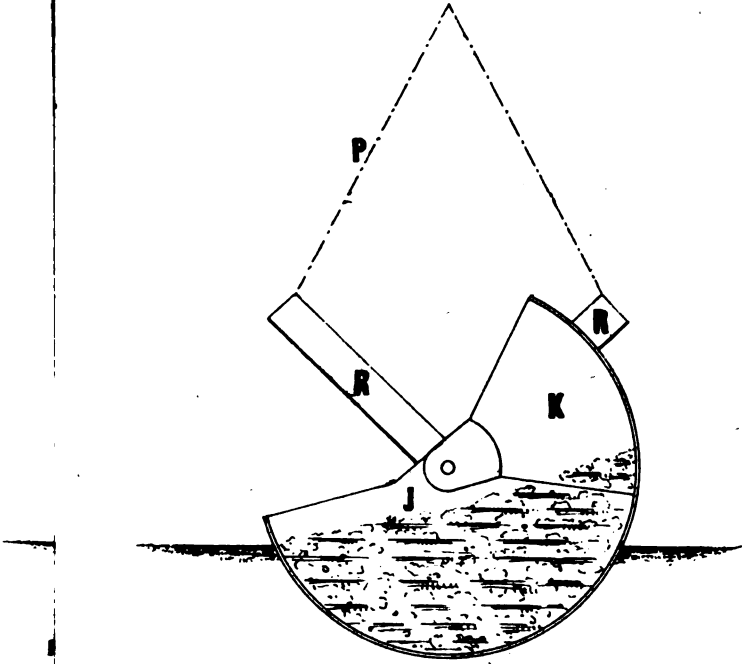
FIG 3. DREDGER AS RAISED.
