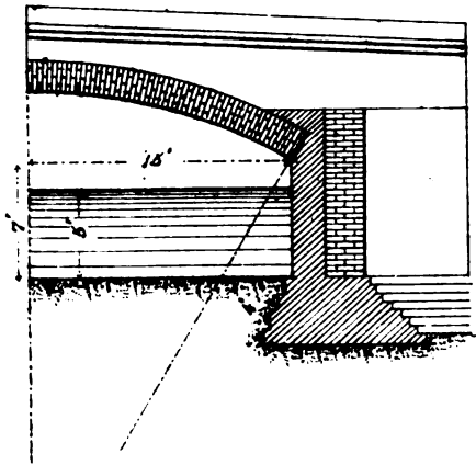
Fig. 4. Luftabad Road Bridge Half Section
