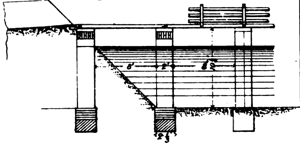
Fig. 1. Bridge, 1/2 mile of Shahpore Canal Longitudinal Section
