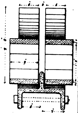
Fig. 6 Section on C, D
