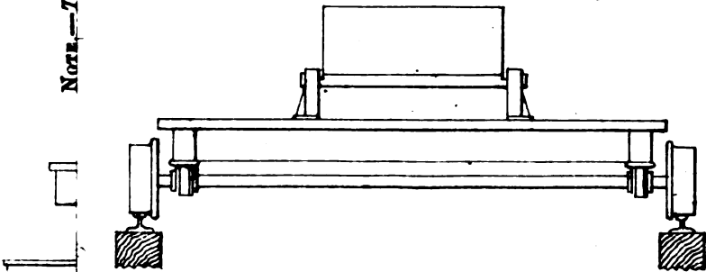
FIG 5. END VIEW OF TIPPING TRUCK.
