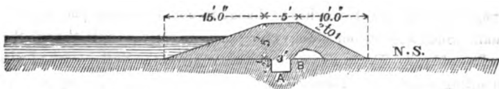
Water tight Section.
