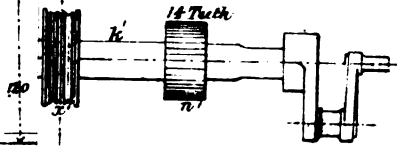
Fig. 15. Driving Axle
