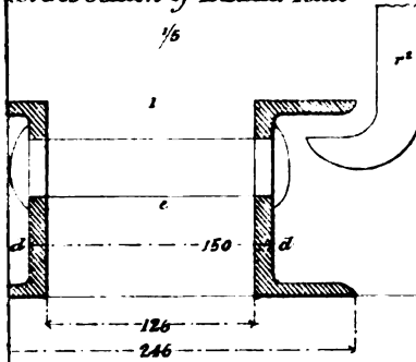
Fig. 14. Transverse Section of Ladder Rail
