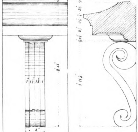
Elevation and Section of Cornice & Console to Doors & Windows.
