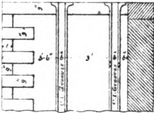
ENLARGED PLAN OF PIER HEADS.
