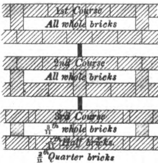
FIG. 5. Showing closing in of the hollows by a vertical section of wall.
