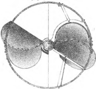
Plan of bottom of Dredge showing position of cutting bits: half with the bottom covering plate removed.
