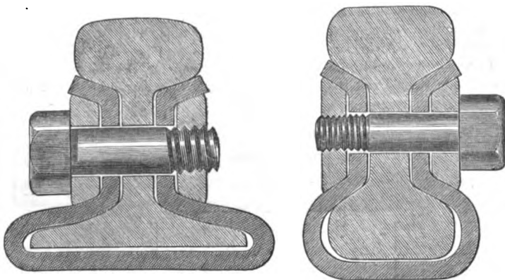
Sectional view of the joint as made for flat bottomed rails.
