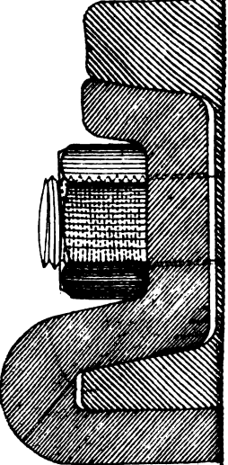
Joint of 36 lbs. Rail Lucknow and C
