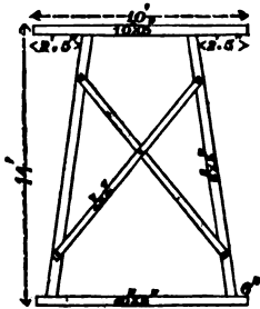
Head and sill of chr. Legs and braces of sal.
