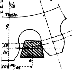
Fig. 17. Ladder Cog and Ladder Cog
