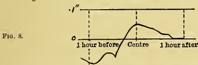
Fig. 5, tornado St. Louis, Mo. (Jan. 12, 1890, 5.16 P.M.); Fig. 6, tornado Owensboro, Ky. (March 27, 1890, 6.17 P.M.); Fig. 7, tornado Cincinnati, O. (March 27, 1890, 8.30 P.M.); Fig. 8, thunder-storm Washington, D.C. (June 22, 1890, 9.8 P.M.).
