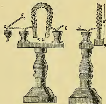
FIGS. 1 AND 2.—STURGEON'S FIRST ELECTRO-MAGNET.
