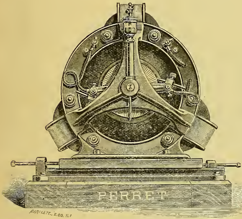
FIGS. 1 AND 2. — PERRET MULTIPOLAR ELECTRIC MOTOR.
