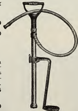
"Prize" Pump
