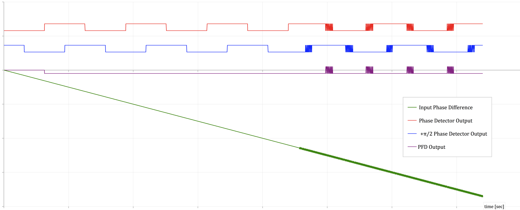
Bang-bang PFD with a constant frequency difference (noiseless and noisy input)
