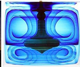
Rolling around a spinning top by Bavand Keshavarz. Visualization of the flow around a spinning top as it rotates inside a liquid, showing how the injected dye gradually gets trapped inside the spiral of toroidal vortices.
