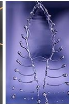
Fluid droplet jets by Bavand Keshavarz. High-speed photography of droplets formed from two colliding water jets.
