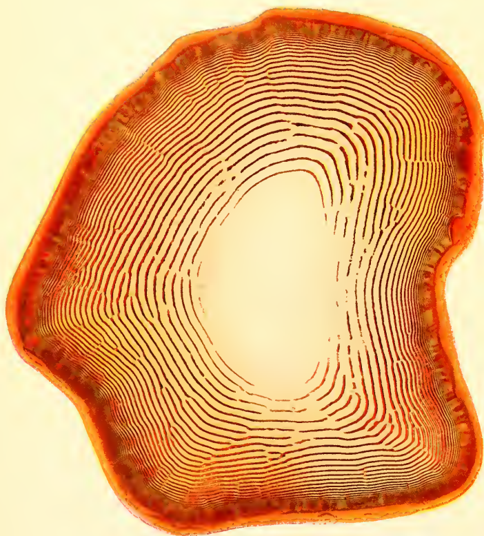
AGATE-LIKE BANDING PRODUCED BY DIFFUSION IN GELATINE. "LIESEGANG'S RINGS"
