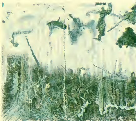
IMITATION OF MOSS AGATE. PRODUCED BY ADDING IRON VITROL TO WATER GLASS.
