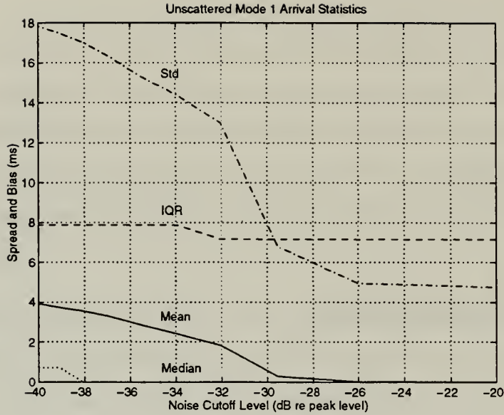
Figure 5-1: The mean (-), median ( \cdots ), standard deviation ( -- ), and interquartile range ( - - ) of an unscattered mode 1 arrival plotted as a function of noise cutoff level. The median reaches its correct value of zero at a noise cutoff level of -38 dB relative to the peak of the arrival.
