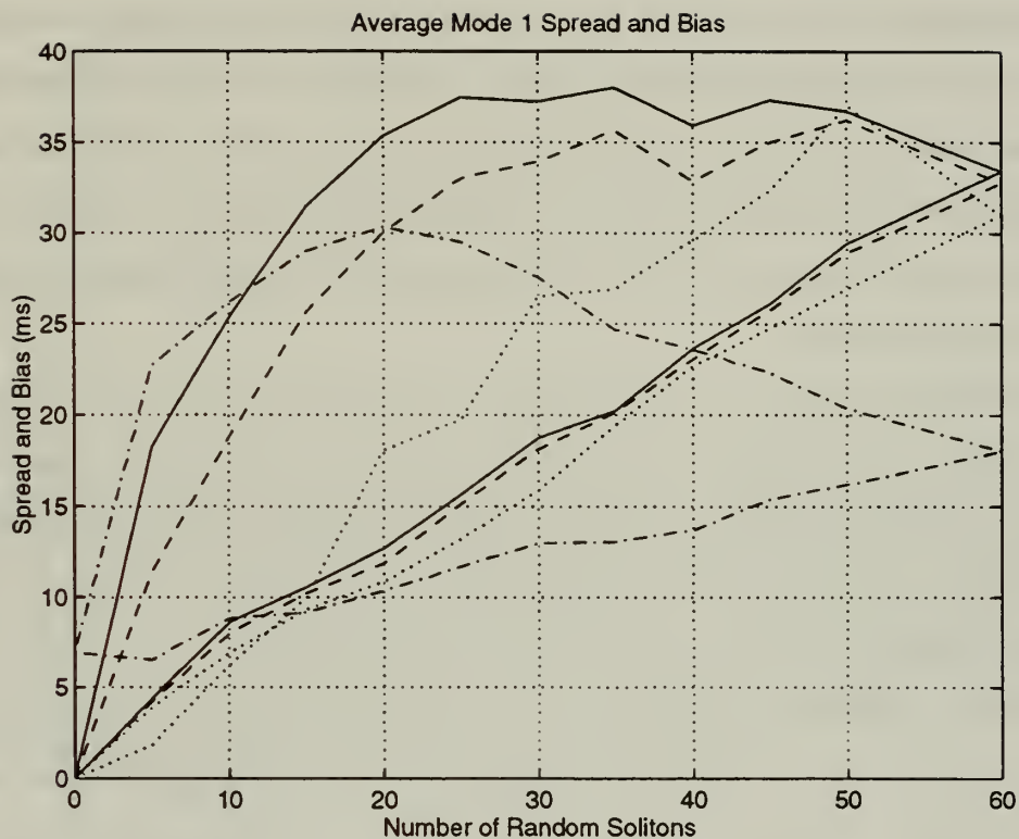
Figure 5-8: The average mean (-), median (- -), and peak (···) lag with respect to the pseudo-adiabatic arrival, and standard deviation (-·-) of scattered mode 1 arrivals plotted as a function of the number of solitons placed between the source and the receiver. The upper curves, averages over 50 realizations, represent the case where the solitons are added starting at the receiver end. The lower set of curves is replotted from figure 5-5. 60 solitons is essentially saturation, and the same points are used in both sets of curves.
