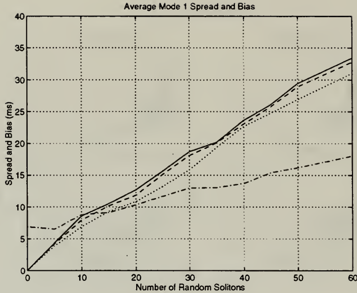
Figure 5-7: The average mean (-), median (- -), and peak (···) lag with respect to the pseudo-adiabatic arrival, and standard deviation (-·-) of scattered mode 1 arrivals plotted as a function of the number of solitons placed between the source and the receiver, where the solitons are added starting from the source end. The upper three lines are all bias measures, and the lower line is a measure of spread.
