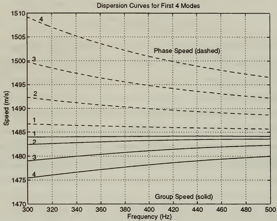
Figure 4-8: Phase and group speeds for the standard field measured SSP. Mode 1 has the lowest phase speed and the highest group speed. The remaining phase speeds increase monotonically with mode number, and the group speeds decrease monotonically with mode number.
