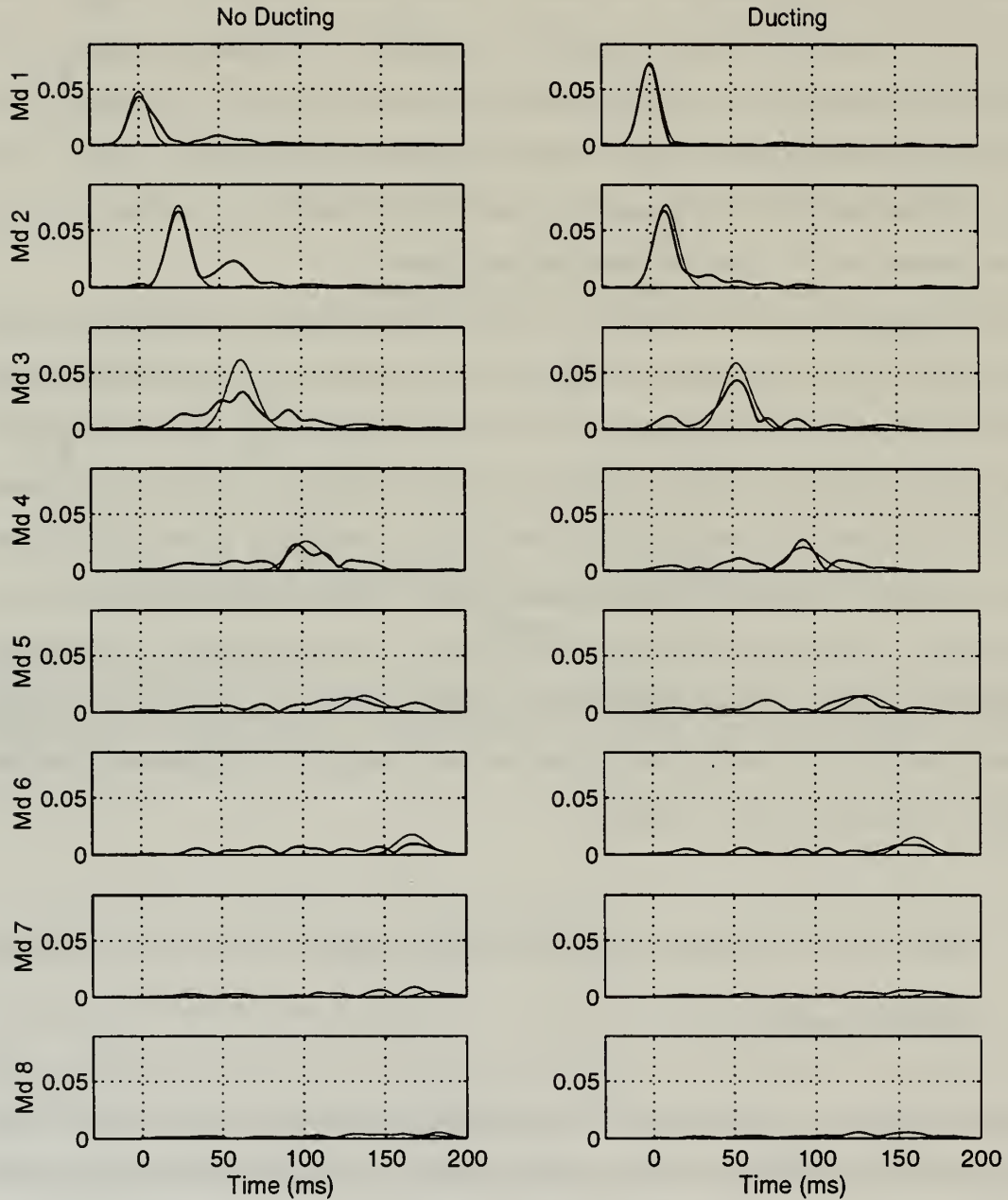
Figure 4-11: Mode coupling effects of the bottom topography shown in Figure 2-1 when the SSP is a modified version the “non-soliton” SSP of Figure 4-6. The “No Ducting” modification consists of imposing the 50.5 m temperature from 50.5 m to the bottom depth, and the “Ducting” modification consists of imposing the 60.5 m temperature from 50.5 m to the bottom depth. The thinner lines in this figure represent predicted arrival shapes for modes that propagate adiabatically.
