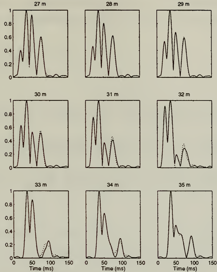
Figure B-3: Single hydrophone RIP pulse arrivals computed from the PPM (solid) and KFS (dotted) methods using various source depths with the receiver depth fixed at 50m.
