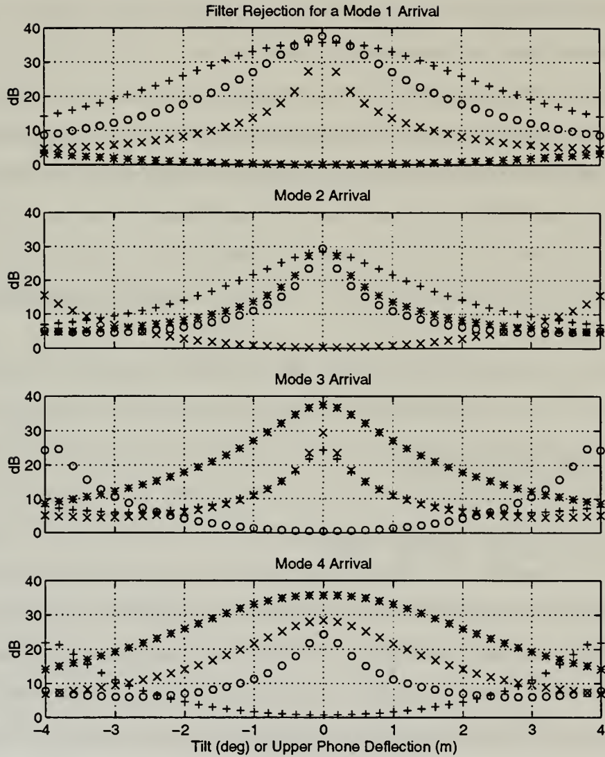
Figure 3-1: Mode rejection levels from mode-filter outputs, A_1 (*), A_2 (x), A_3 (o), and A_4 (+), as a function of array tilt. The four plots represent tilted inputs of pure mode 1, mode 2, mode 3, and mode 4 arrivals. These plots use mode filters and mode arrivals generated from the same typical SWARM SSP.
