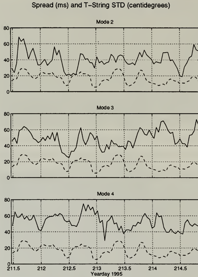
Figure 5-18: A comparison of 1 hour bin averaged IQR levels for the simulated mode 2-4 data (solid lines) and a 1 hr bin average of the Standard Deviation of the Temperature at 22.5 m depth over the previous 4.3 hrs (dashed lines). The standard deviation of the temperature is in tenths of a degree centigrade to facilitate comparison with the IQR levels in milliseconds.
