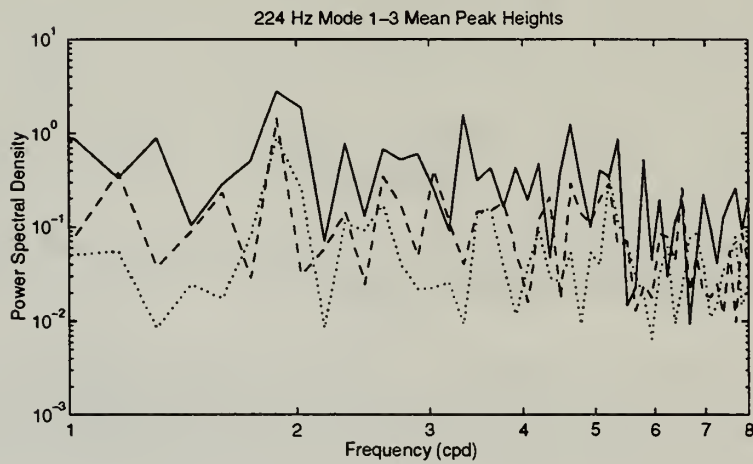
Figure 6-16: Power spectral densities for the 224 Hz 1.4 hr bin averaged peak arrival time and peak height time series of Figure 6-15. Mode 1 is solid, mode 2 is dashed, and mode 3 is dotted.
