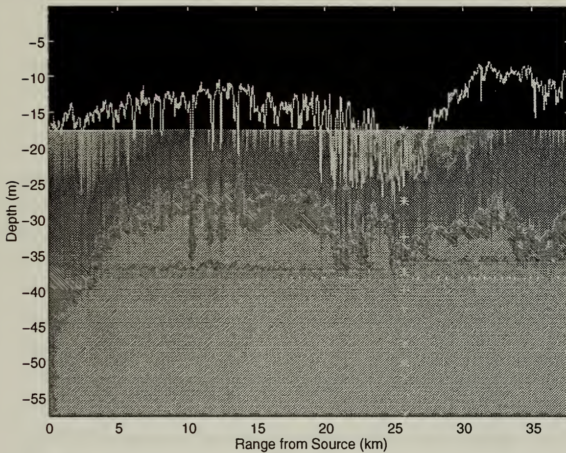
Figure 5-14: Pycnocline displacements from an Orr backscatter record compared to a thermistor string record using a propagation speed of .62 m/s over the distance between the back scatter instrument and the thermistor string at each backscatter reading.
