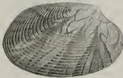
Venus Deshayesi Nob
