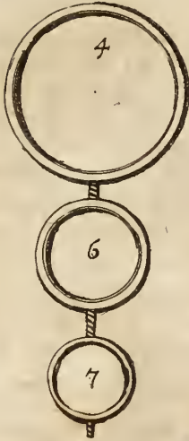
Fig. LXII. ad obs. penult.
