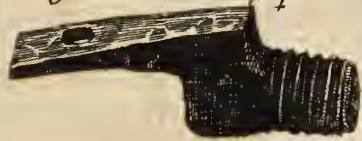
Fig. LXII. ad obs. penult.
