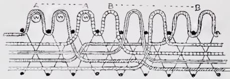
Diagram 4.—Showing in a longitudinal section of a Brussels carpet how the variously-coloured worsted threads are successively brought to the surface. At 'A A' the wires, WW, are shown in position; at 'B B' they have been removed.
