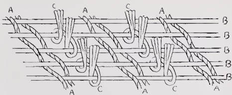
Diagram I.—Showing one method of hand-knotting. BB are the warp threads; AA, the weft; CC, the tufts knotted round the warp.
