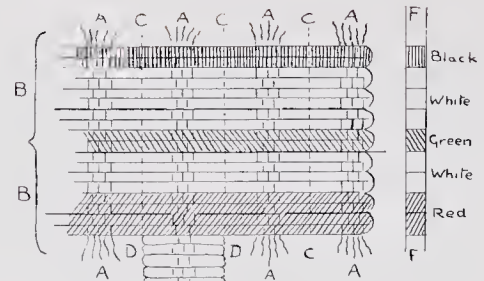
Diagram 4.—Showing in a longitudinal section of a Brussels carpet how the variously-coloured worsted threads are successively brought to the surface. At 'A A' the wires, WW, are shown in position; at 'B B' they have been removed.
