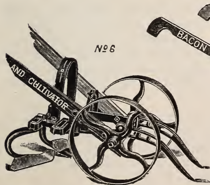
No. 6 Double Wheel Expansion Arch Cultivator with 6 teeth, 2 hoes, 1 plow.
