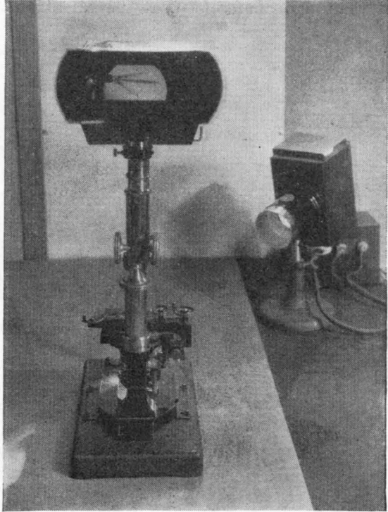
Figure 5.—Apparatus used in the Department of Agriculture for measuring external parts of bees. A micrometer eyepiece with a movable scale is attached to the microscope.
