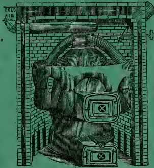
The Boynton Heater.
