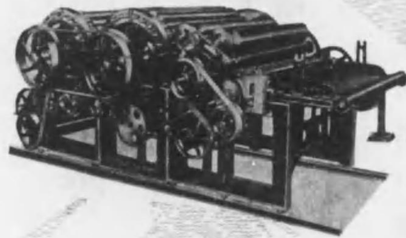
"X,, Type 2 Swift with Garnett Breast.
