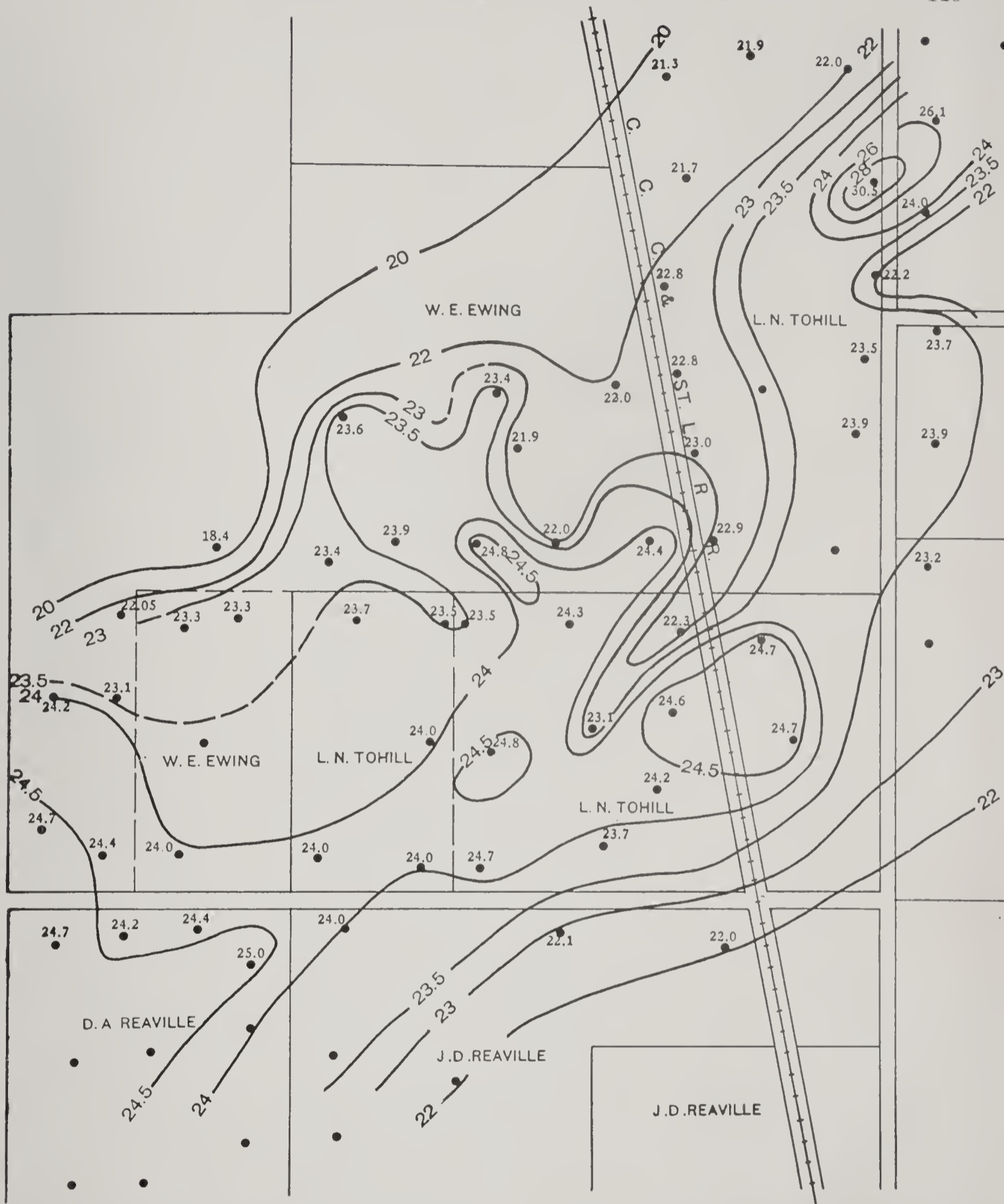
Fig. 21. Map showing contours on Beaumé oil gravities. The lighter oils are in the higher parts of the structure. (Compare Plates X and XI.)
