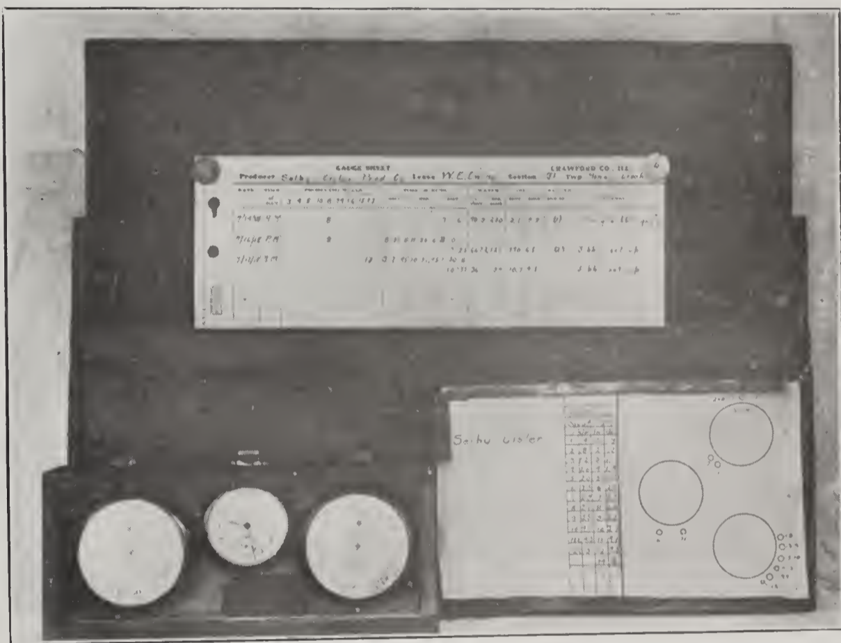
Fig. 30. Photograph of the gage board devised for protection of the records while in use on the lease.
