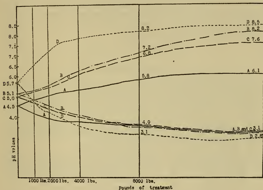
FIG. 1. TITRATION CURVES FOR SOILS A, B, C, AND D, WITH DIFFERENT AMOUNTS OF \text{Ca}(\text{OH})_2 AND \text{H}_2\text{SO}_4 ADDED \text{Ca}(\text{OH})_2 Curve—upper graph \text{H}_2\text{SO}_4 Curve—lower graph
