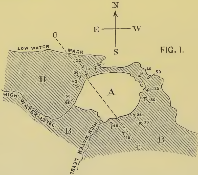
FIG. 1. MAP OF STRATA AT WHITBERRY POINT. Scale, 6 in. to the mile.
