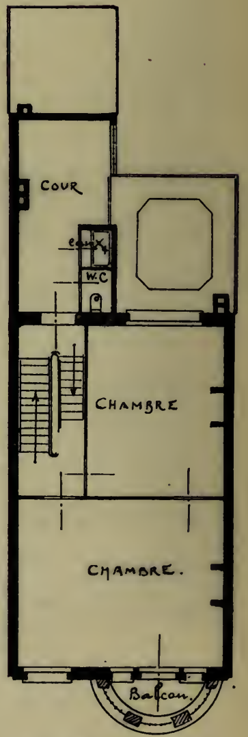
SECOND ETAGE.
