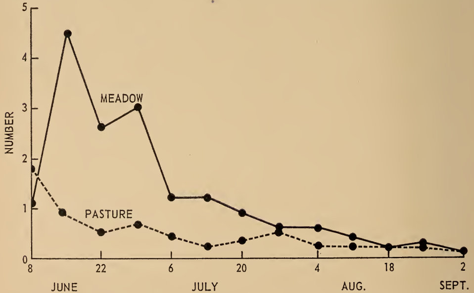
Fig. 1. Average numbers of nymphs of M. religiosa per square yard in weekly samples from two fields near Chatterton, 1949.
