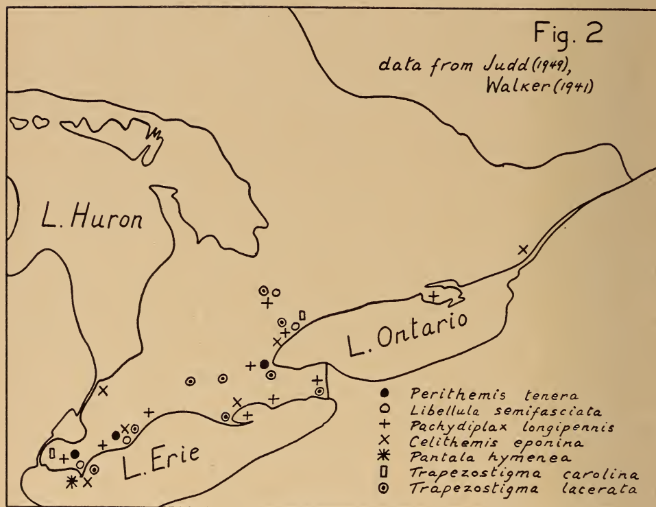
Fig. 2—Distribution of Carolinian Anisoptera in Southern Ontario.
