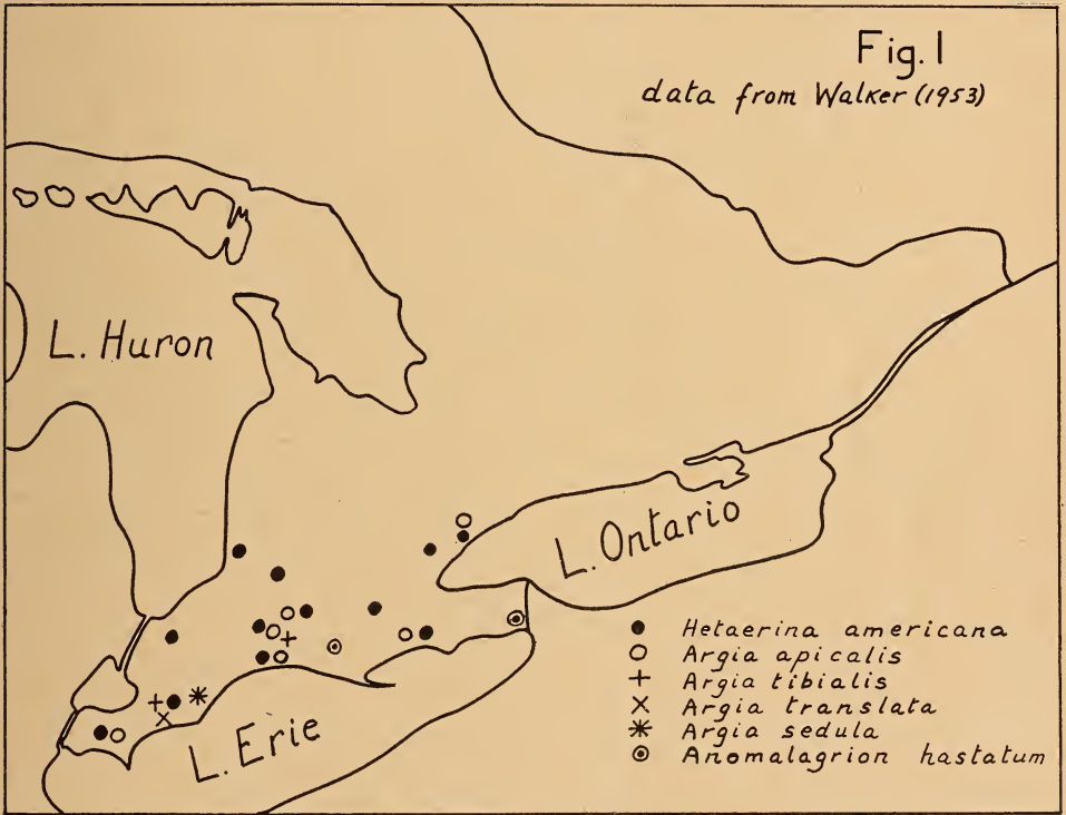
Fig. 1—Distribution of Carolinian Zygoptera in Southern Ontario.
