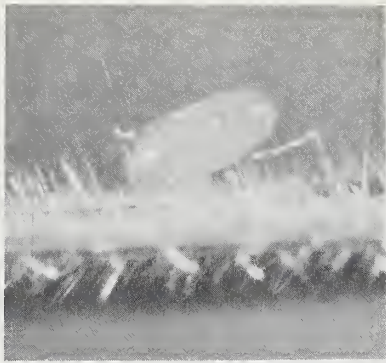
Right: An adult cereal leaf beetle oviposits on the leaf of C18616, a long-pubescent wheat line (0275X152-27). Above: Larvae hatched from eggs on long-haired wheats are less likely to survive than those on wheats with short hairs (0275X154-3).
