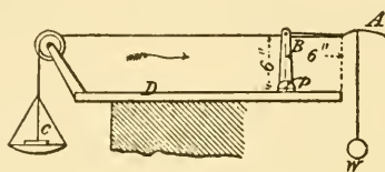
FIG. 2.—Phillips' balance.
