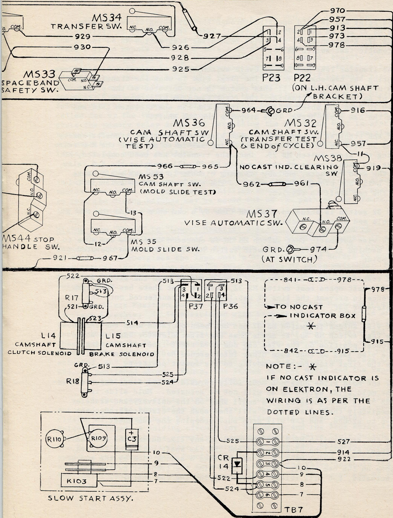
WIRING DIAGRAM
