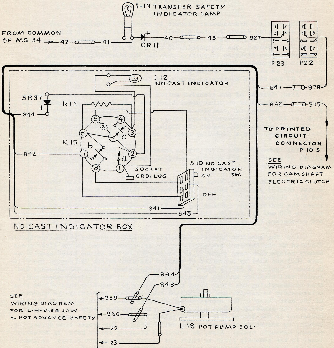
WIRING DIAGRAM
