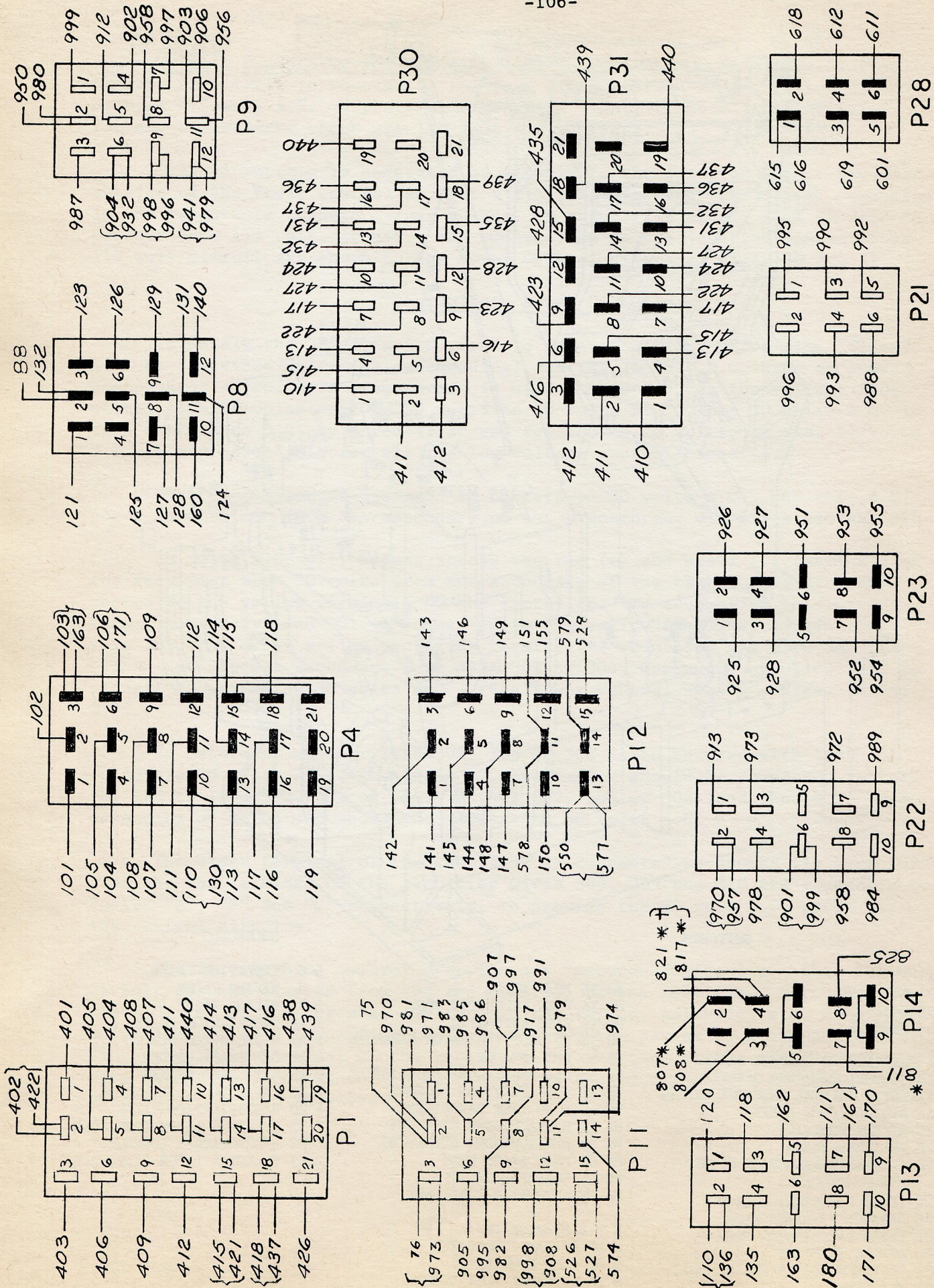
COMPLETE WIRE CONNECTIONS TO PLUGS & RECEPTACLES
