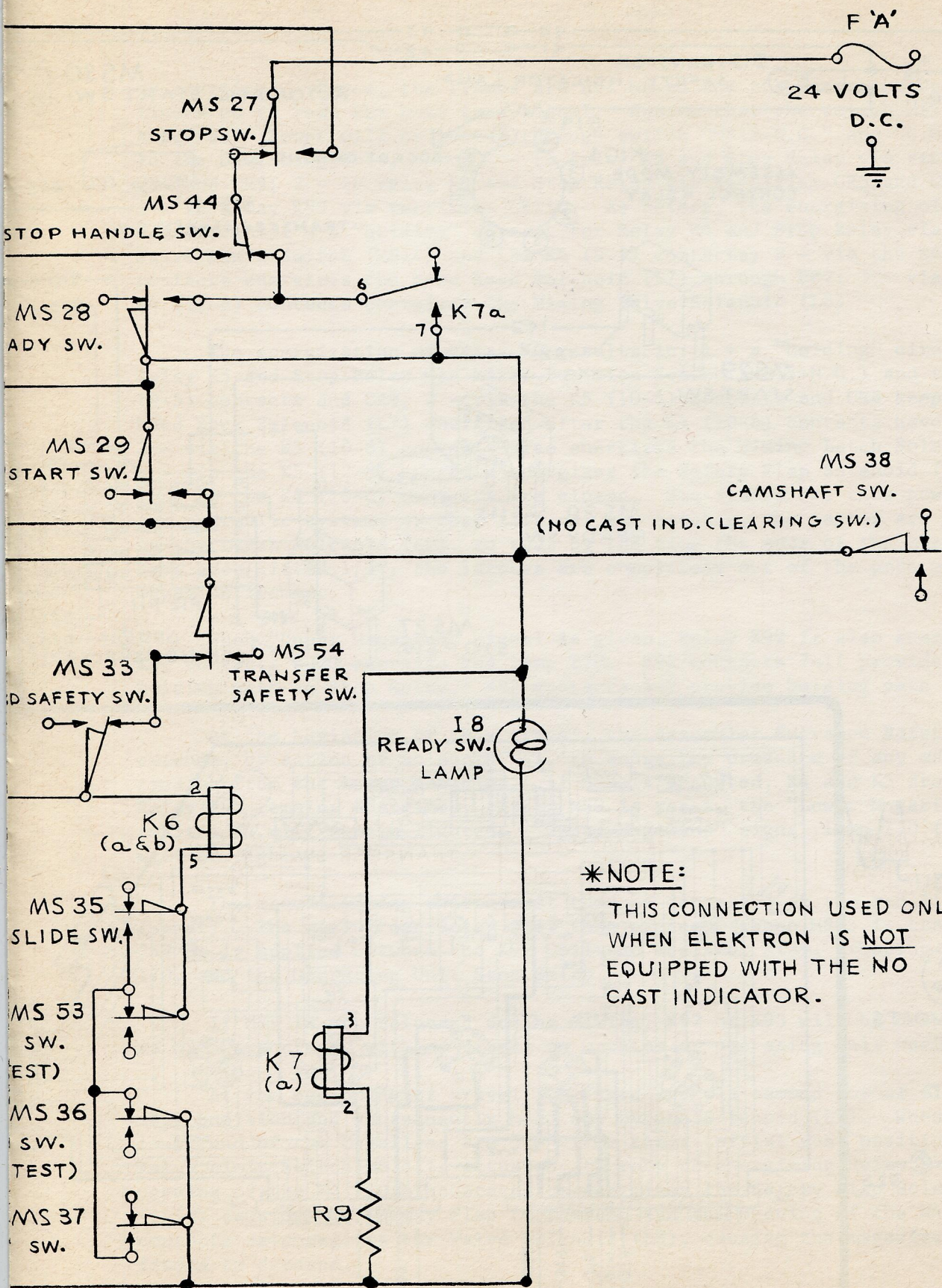
SCHEMATIC
