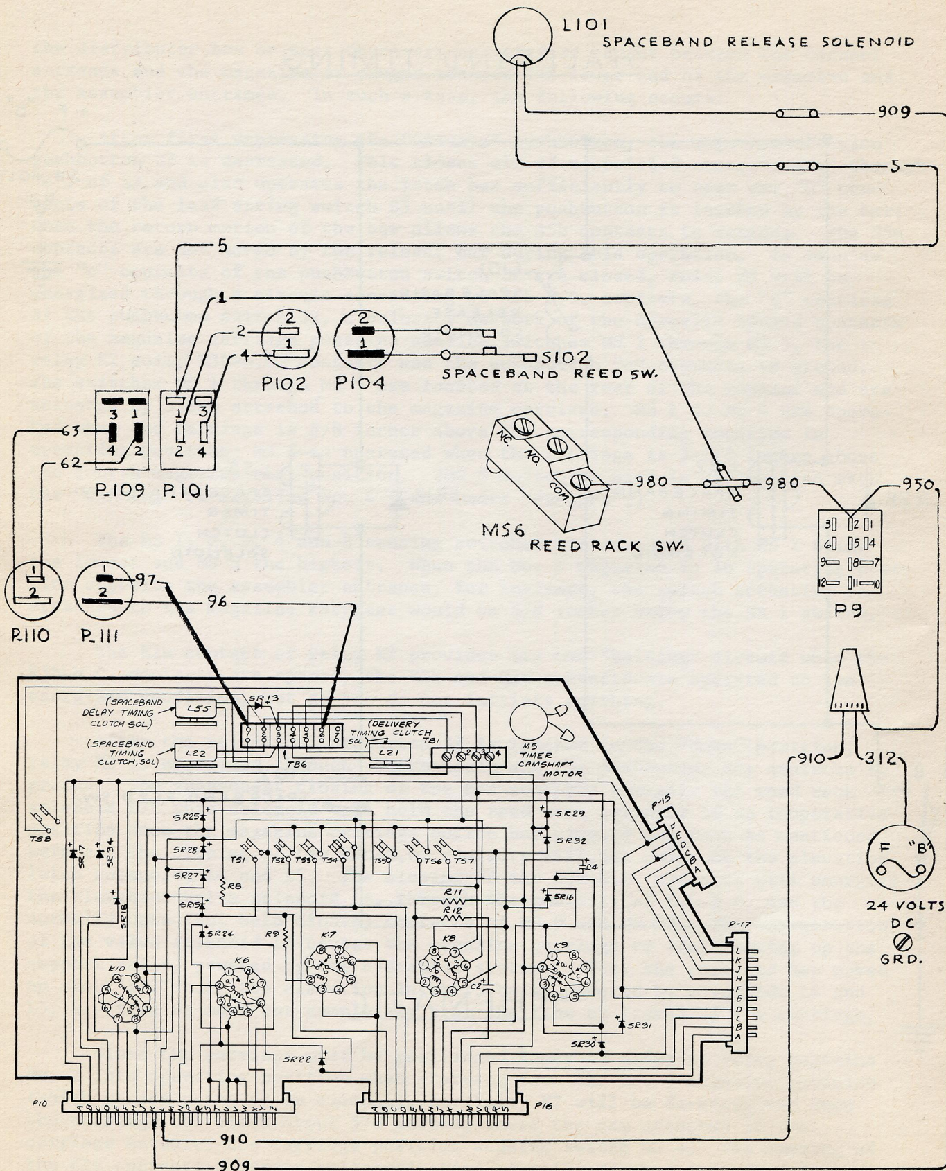
WIRING DIAGRAM
