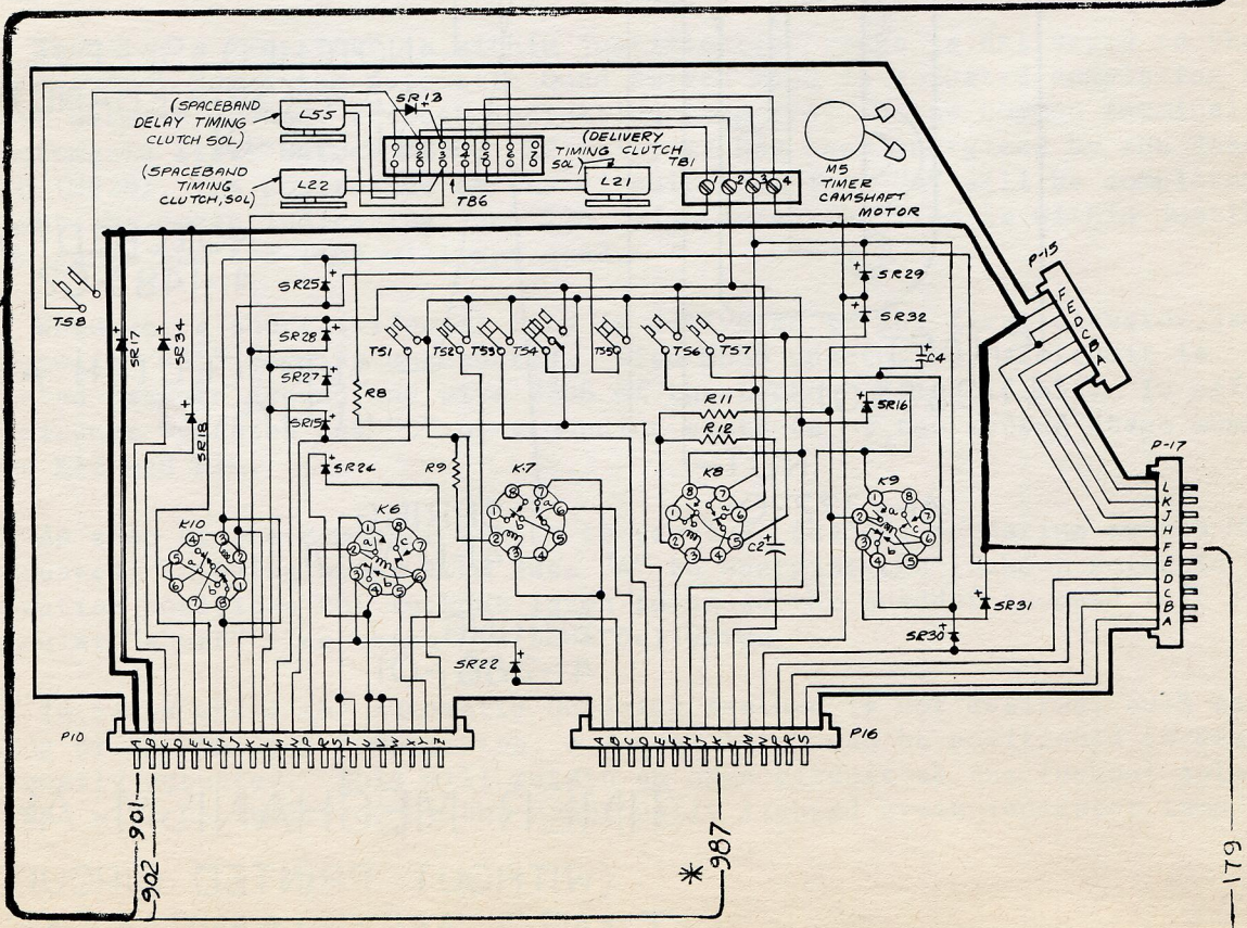
WIRING DIAGRAM
