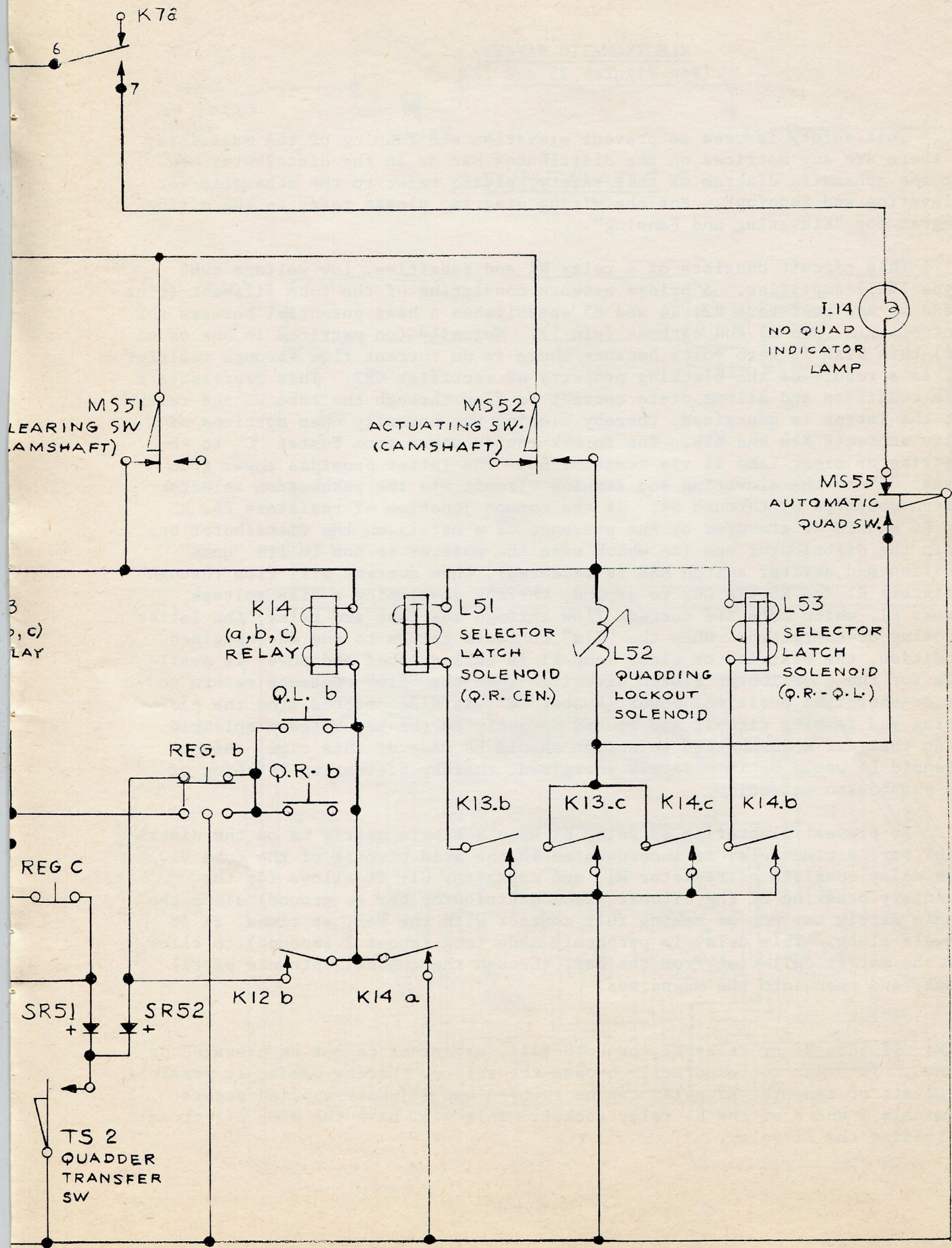
SCHMATIC
