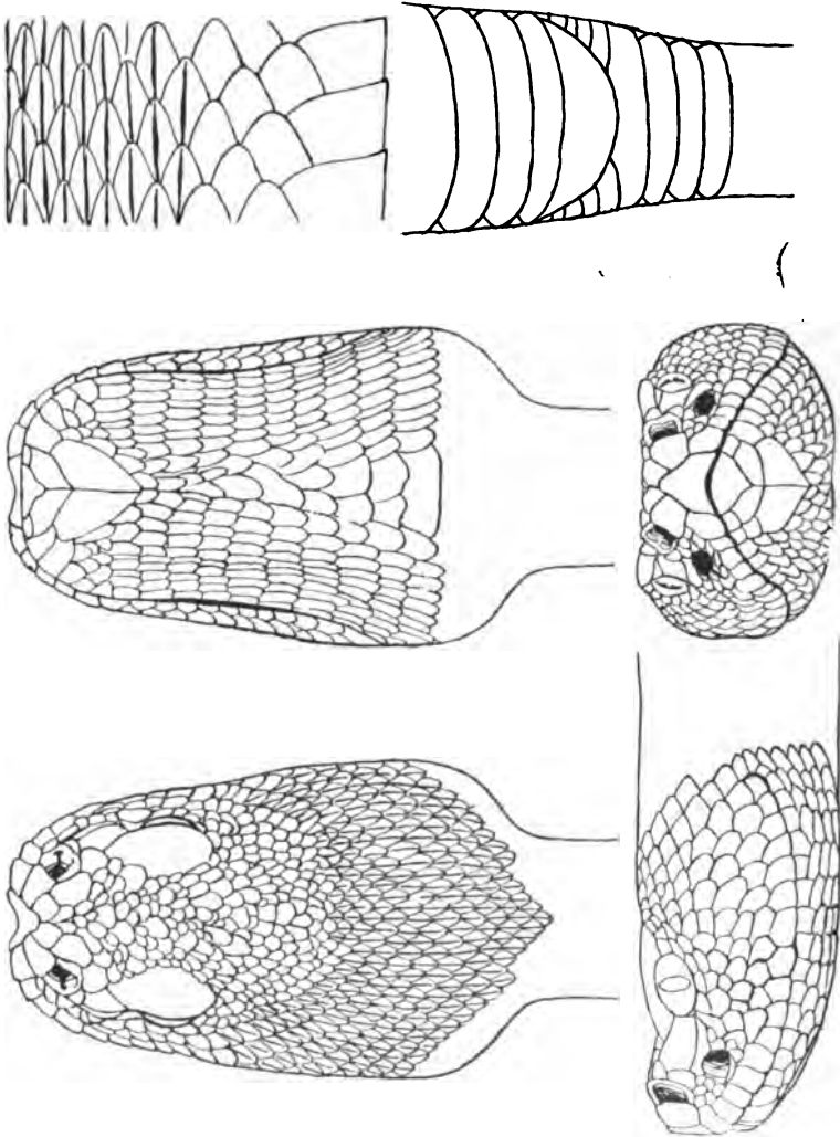
FIG. 385. CROTALUS RUBER COPE. = 1. Southern California. Cat. No. 9009, U.S.N.M.
