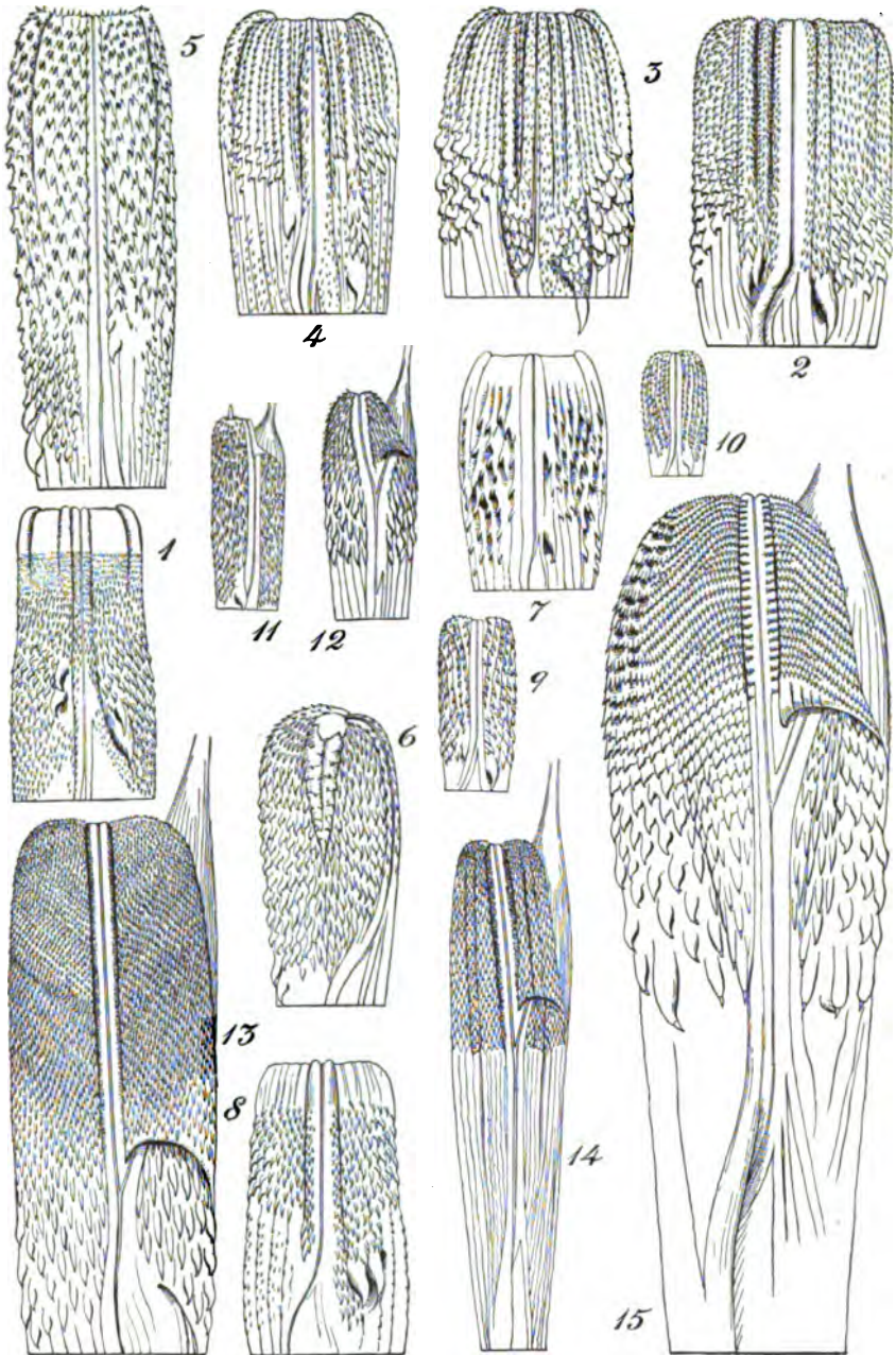
HEMIPENES OF NATRICINÆ AND HOMALOPSINÆ.
