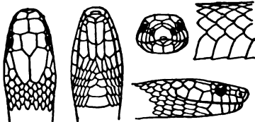
Fig. 159. DIADOPHIS AMABILIS DOCILIS BAIRD AND GIRARD.
