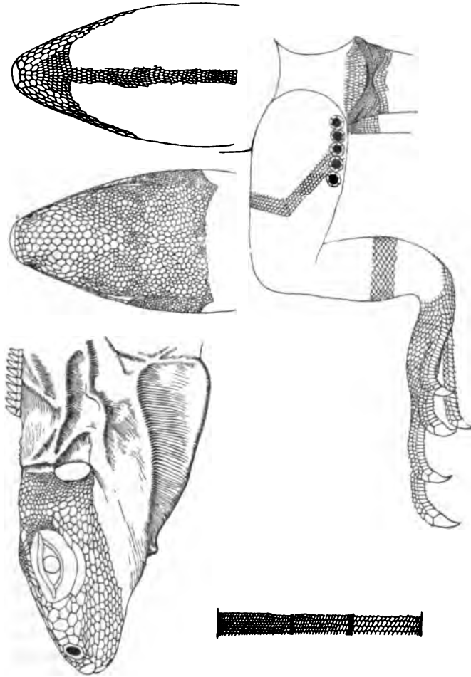
Fig. 17. UROSAAURUS HEMILOPHA COPE. × 3. La Paz, Lower California. Cat. No. 1863, U.S.N.M.
