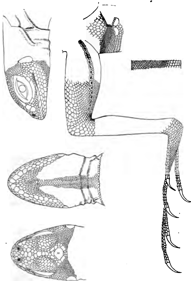
Fig. 25. CALLISAURUS DRACONOIDES VENTRALIS HALLOWELL. Mojave Desert, California. Cat. No. 6838, U.S.N.M.
