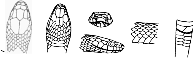
Fig. 158. DIADOPHIS AMABILIS DOCILIS BAIRD AND GIRARD. × 2.
