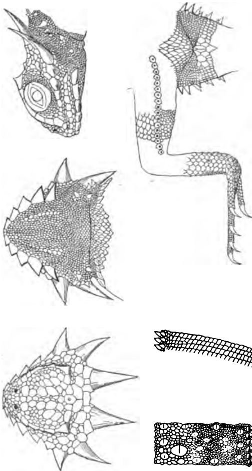
Fig. 82. ANOTA MACCALLII HALLOWELL. × \frac{3}{4} Desert of Gila and Colorado. Cat. No. 164, U.S.N.M.
