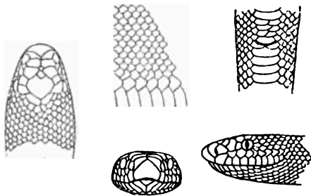
Fig. 150. CHARINA BOTTÆ BLAINVILLE. × 1.5. Showing two rows of loreal plates.
