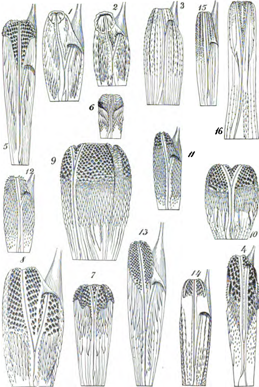
HEMIPENES OF XENODONTINÆ, DROMICINÆ, AND SCYTALINÆ.
