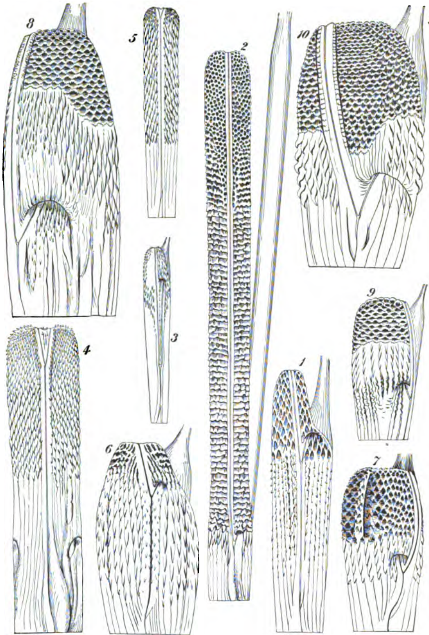
HEMIPENES OF PROTEROGLYPHA, PLATYCERCA, AND SOLENOGLYPHA.
