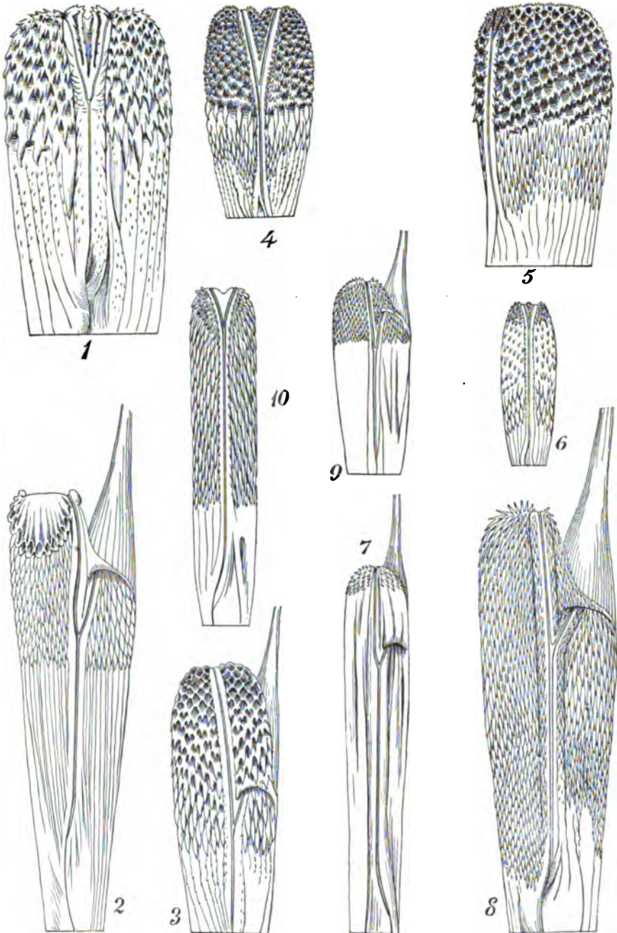
HEMIPENES OF PROTEROGLYPHA AND PLATYCERCA.
