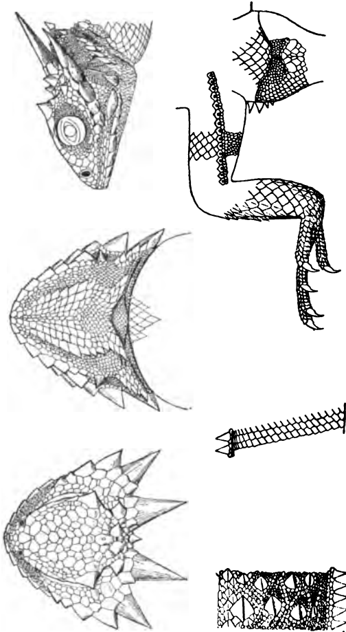
Fig. 74. PHRYNOSOMA BLAIRVILLEI GRAY. × 8.
