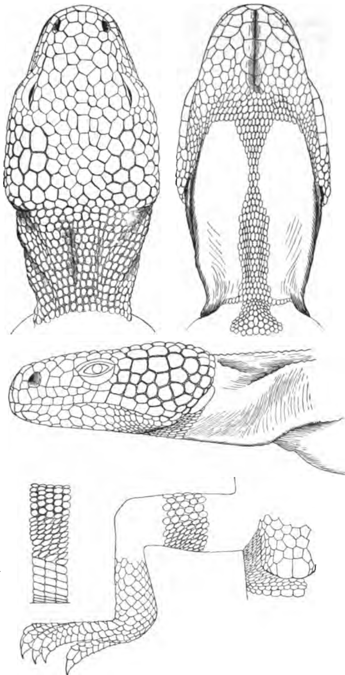
Fig. 87. HELODERMA SUSPECTUM COPR. = 1. ARIZONA. Collection of E. D. Cope.
