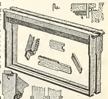
Hoffman Frames—Showing Foundation Starter
