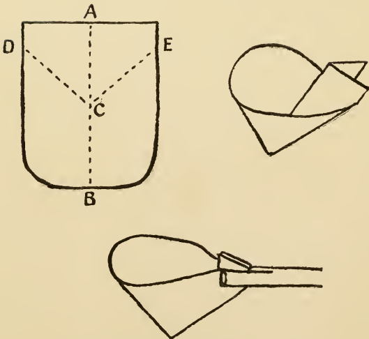
FIG. 19. Bark Dipper.
