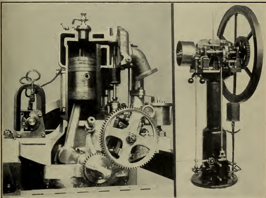
GAS AND OIL ENGINES.
