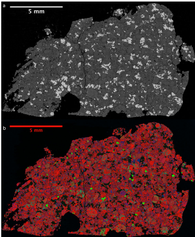
Fig. 5. a) Backscattered electron image and (b) composite RGB EDS map of the “Strawberry Lake” Hamburg type specimen section ME 6108.3. Red = Mg; green = Ca; blue; Al.
