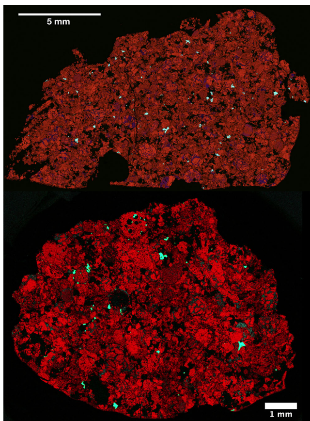
Fig. 10. RGB map of phosphates from top: type specimen ME6108.3 studied by LA-ICPMS, and bottom: specimen (aliquot from MSU-Abrams 2018-001) studied by SIMS (Mg—red, P—green, Ca—blue).
