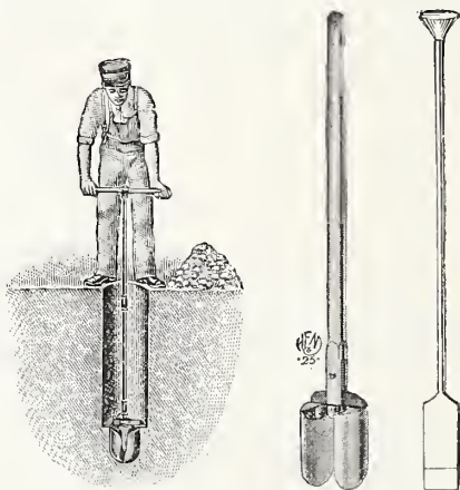
No. 8 Digger
