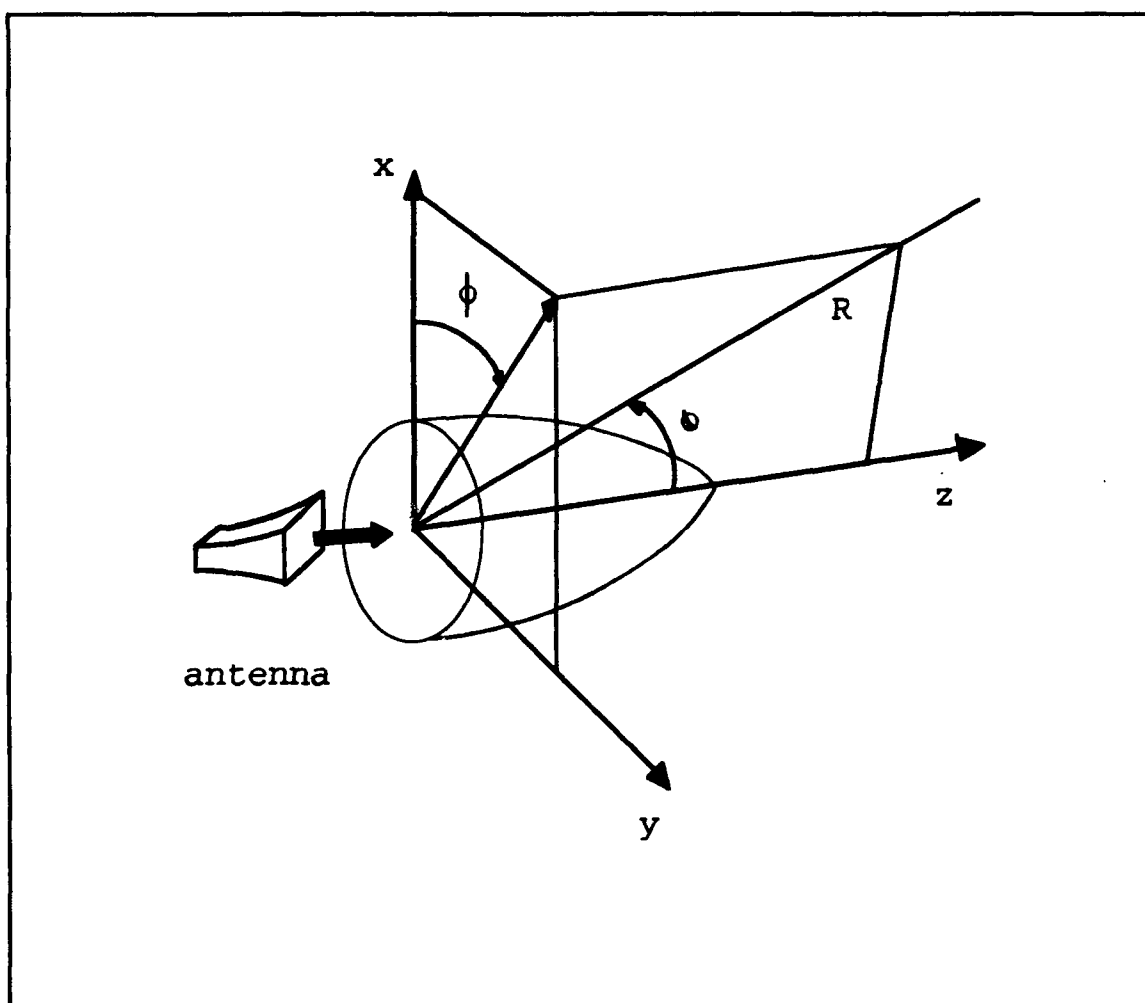
Figure 5.1 Spherical coordinate system.
